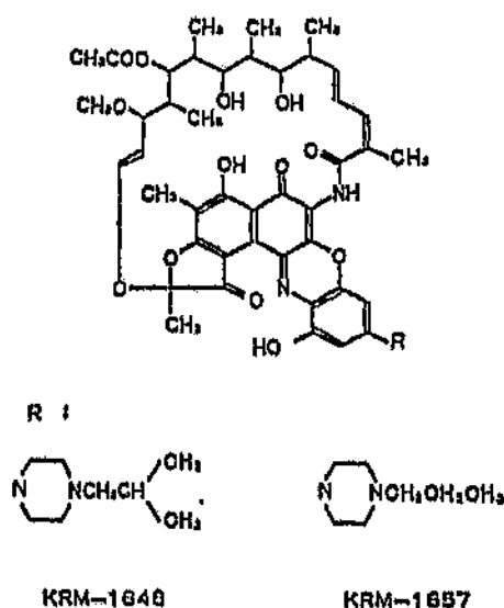
Figure 4.3 Structures of KRM 1648 and KRM 1657
