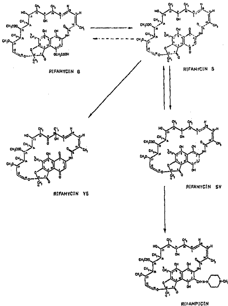
Figure 1.1 Structures of rifamycins
