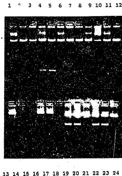
Figure 3.29 Plasmid c screened for deletions of AgeI , Asp718 , ClaI and NotI fragments. Lanes 1-6: Potential \Delta Age cut with AgeI 7-12: Potential \Delta Asp cut with Asp718 13-18: Potential \Delta Cla cut with Asp718 19-24: Potential \Delta Not cut with NotI
