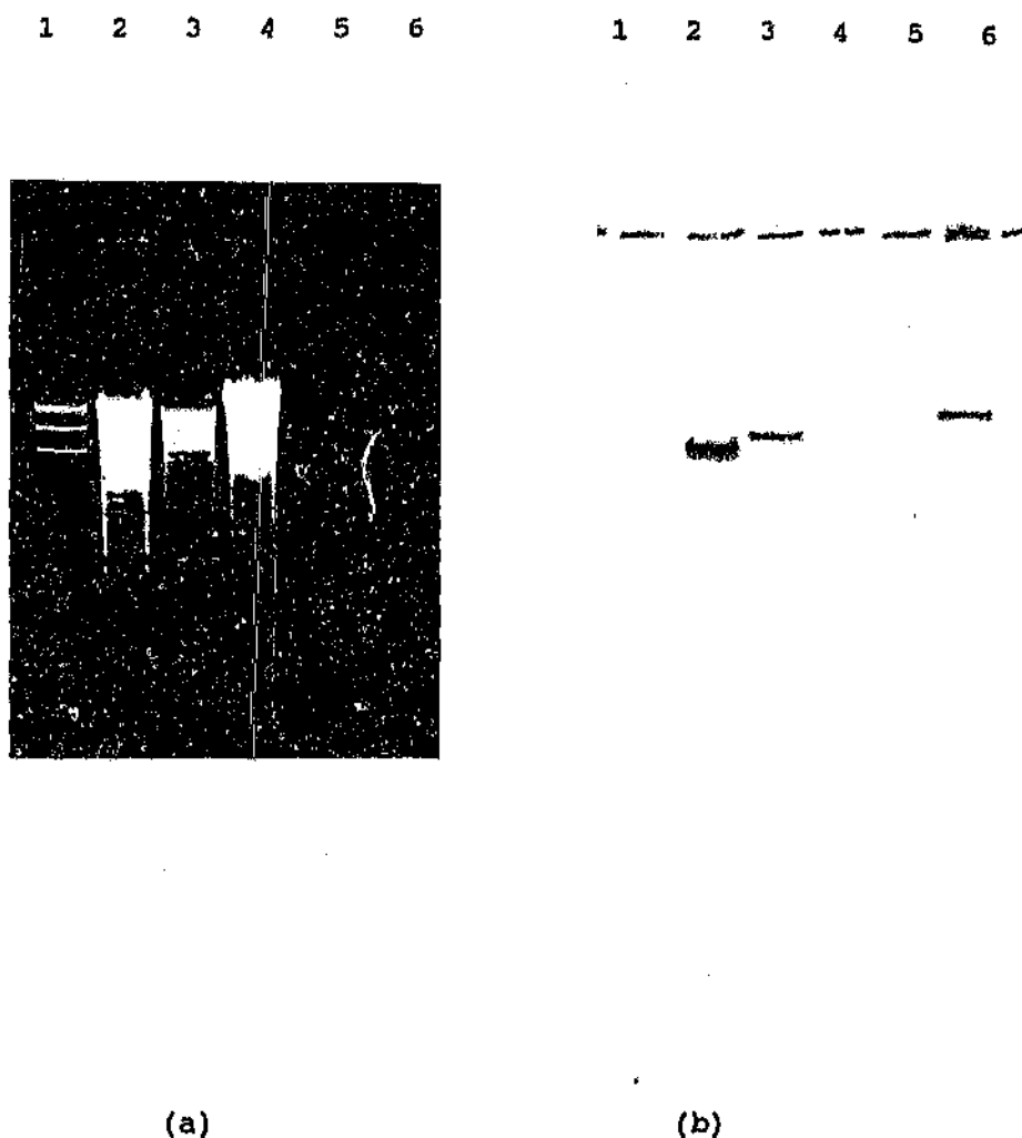
Figure 3.23 Hybridisation of R.erythropolis DNA and E.coli DNA with the 8.3kb fragment. a) 1.8% agarose gel that was blotted b) Nitrocellulose filter lane 1: DNA molecular weight marker; lane 2: ATCC12674; lane 3: ATCC4277; lane 4: \lambda MM294; lane 5: pDA37; lane 6: #6
