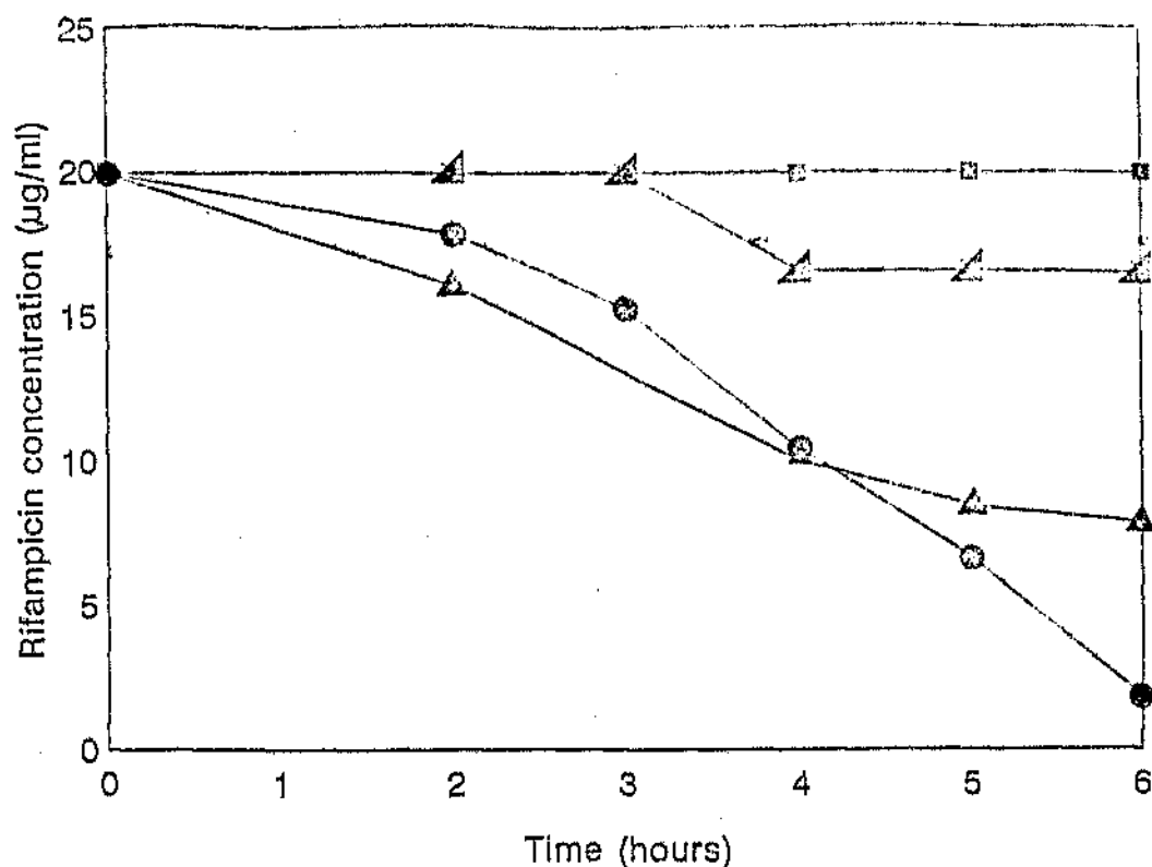
Figure 3.28 Inactivation of rifampicin by two cloned iri genes from Rhodococcus species. (▲)-from R.erythropolis , (●)-from R.equi , (▲)-Ri8-1 containing pDA71, (■)-cell free control.
