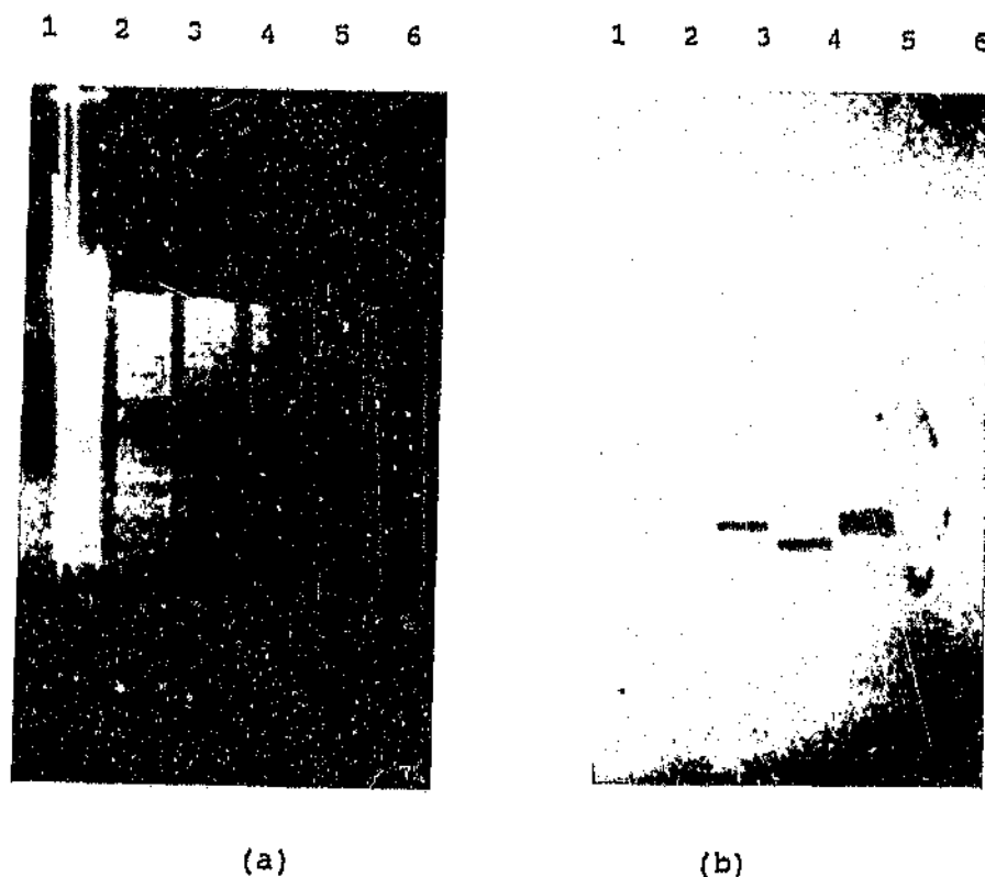
Figure 3.24 Hybridisation of iri + DNA to R.erythropolis , R.australis , M.smegmatis and E.coli DNA. a) 0.8% agarose gel that was blotted b) Nitrocellulose membrane Lane 1: \lambda MM294; lane 2: ATCC12674; lane 3: ATCC4277; lane 4: A448; lanes 5 and 6: M.smegmatis
