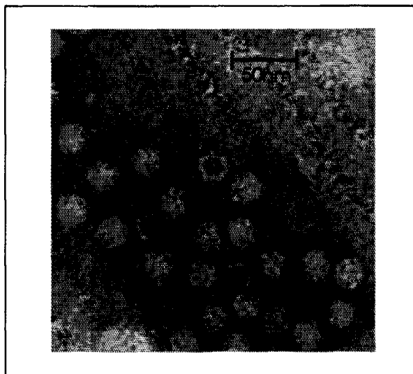
Fig. 2 Electron micrograph of B19 virus particles.
