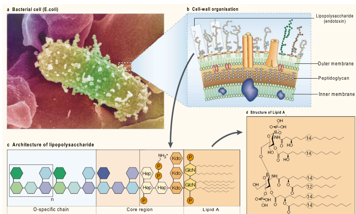
Figure 1.1 A Gram-negative bacterium. Electron micrograph of Escherichia coli (a), together with a schematic representation of the location of lipopolysaccharide, (endotoxin, LPS) in the bacterial cell wall (b) and the architecture of LPS (c). Also shown is the primary structure of the toxic centre of LPS, the lipid A component (d). GlcN, D-glucosamine; Hep, L-glycero-D-manno-heptose; Kdo, 2-keto-3-deoxy-octulosonic acid; P, phosphate (Beutler and Rietschel, 2003).
