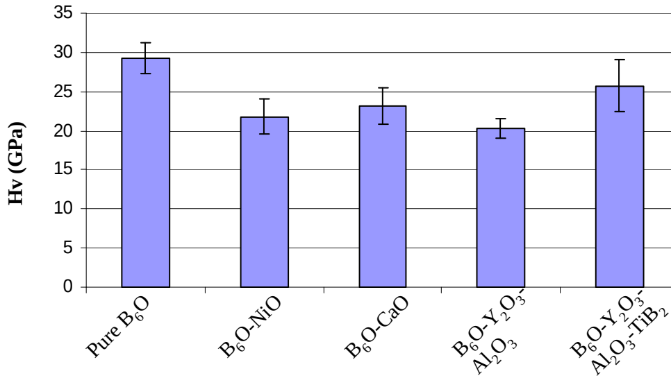
Figure 5-23: Comparison of the hardness of the SPS sintered boron suboxide materials
