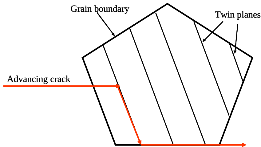
Figure 5-12: Illustration of a transgranular crack deflecting along a twin plane
