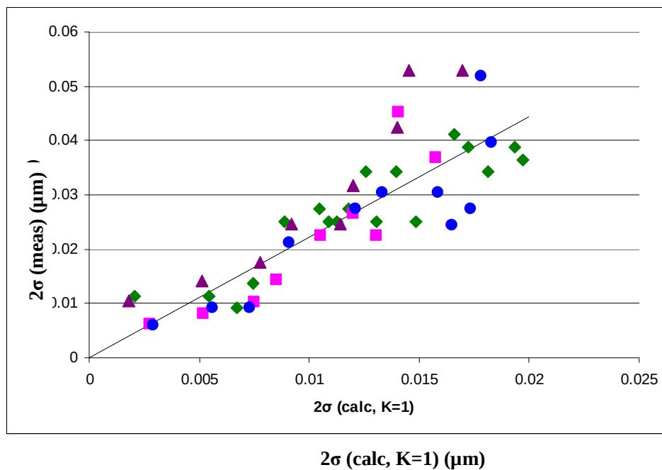
Figure 4-12: COD analysis for pure boron suboxide
