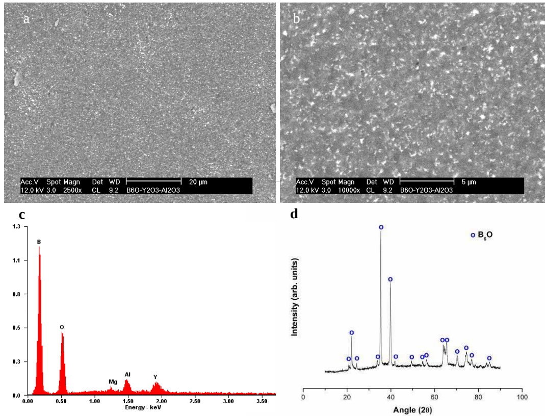
Figure 4-5: Structure (a,b), accompanying EDS spectrum (c) and XRD trace of B 6 O-Y 2 O 3 -Al 2 O 3 . EDS spectrum area of mapped image b.
