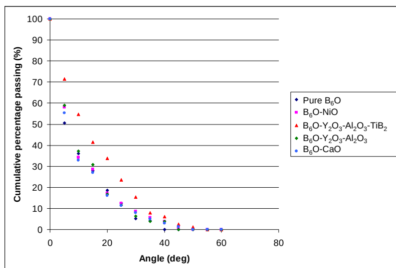
Figure 4-13: Crack deflection angles for the various boron suboxide based materials
