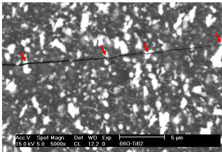
Figure 5-9: A crack running through the B_6O - Y_2O_3 - Al_2O_3 - TiB_2 sample. The red arrows indicated where the crack has sheared a TiB_2 grain.
