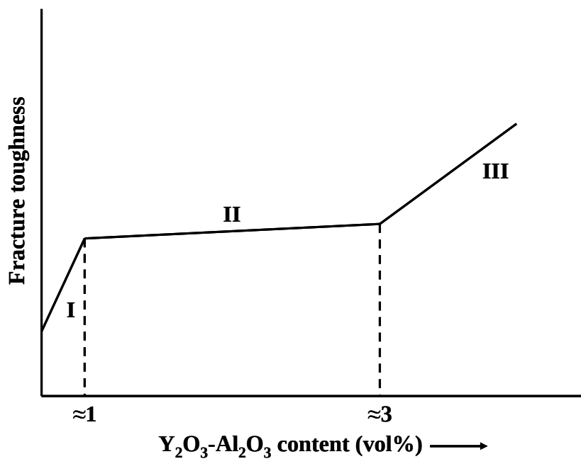
Figure 5-5: Schematic plot of trend of the effect of \text{Y}_2\text{O}_3\text{-Al}_2\text{O}_3 content upon the fracture toughness of boron suboxide materials. (Herrmann (2010))
