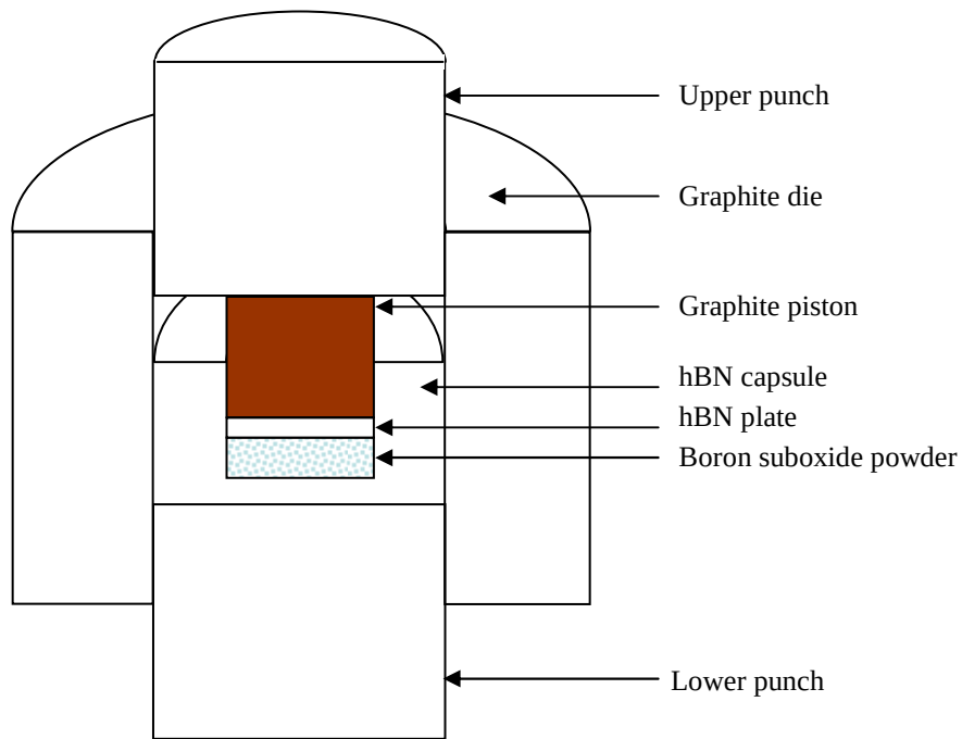
Figure 3-1: Capsule assembly and punch and die configuration
