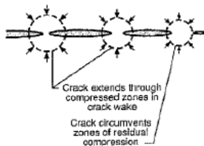
Figure 2-20: Ductile bridging in the wake of a crack (Evans (1990))
