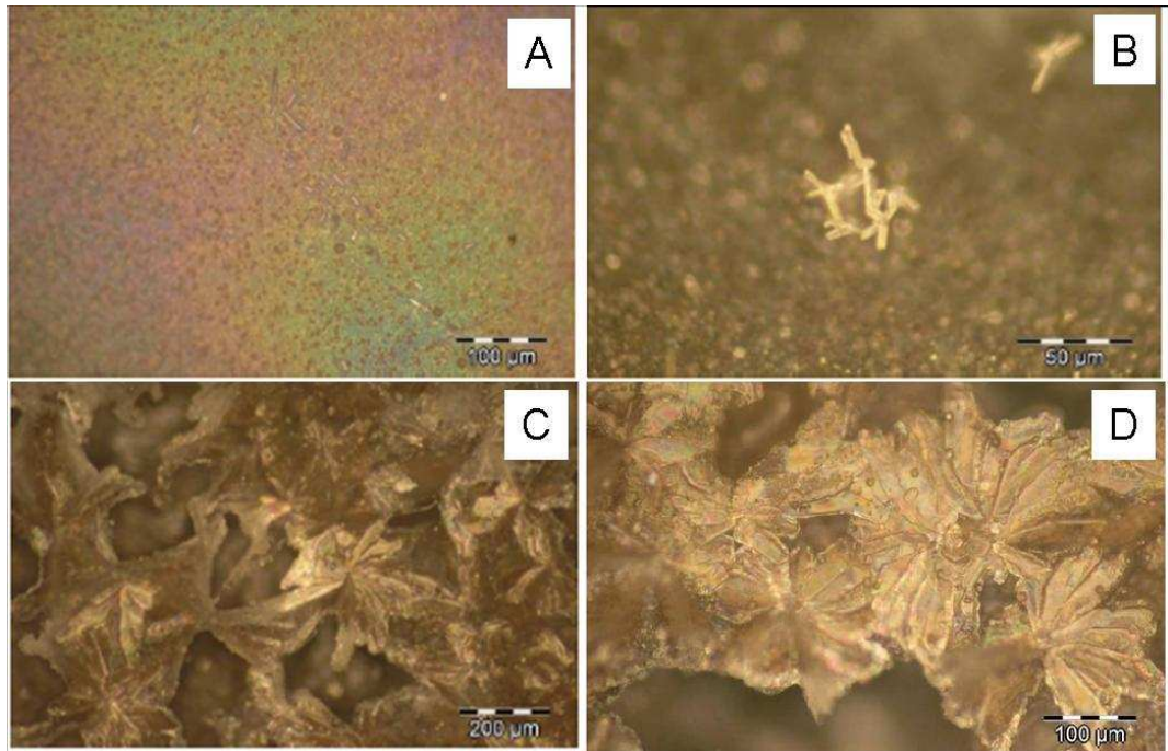
Figure 2-14: Optical micrographs after 10 hours of heat treatment. A and B are from the pure B_6O sample. C and D are from the B_6O-Al_2O_3-Y_2O_3 sample. Freemantle (2009)
