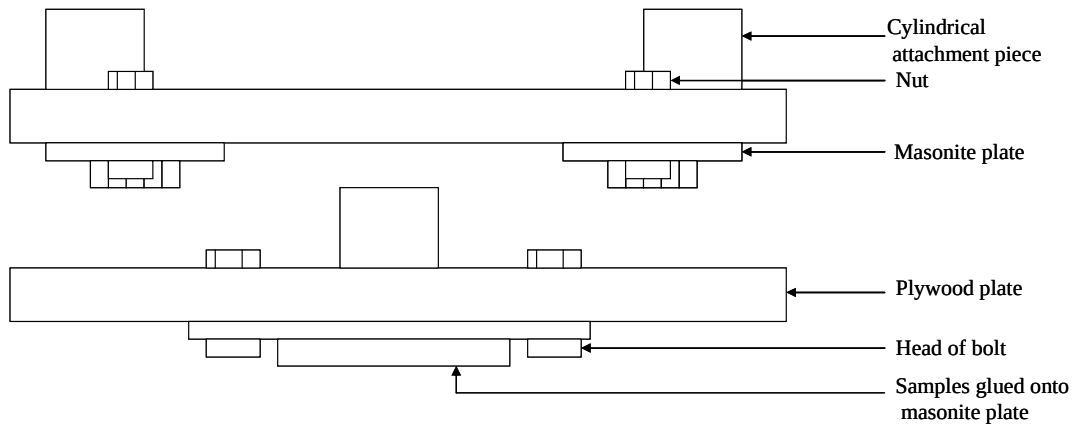
Figure 3-5: Schematic diagram of arrangement used for lapping
