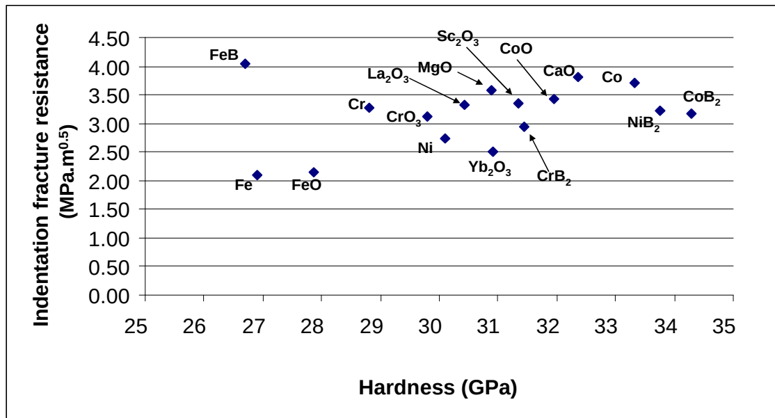
Figure 2-9: Hardness and fracture toughness values for various B 6 O composites (Johnson (2008) and Ogunmuyiwa (2009))
