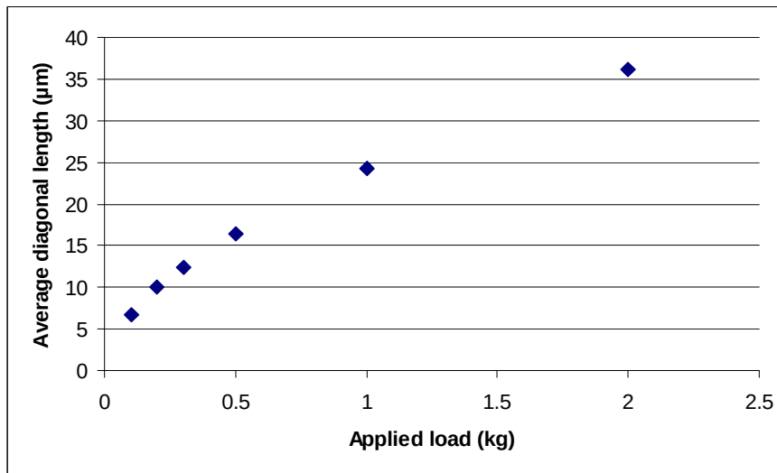
Figure 4-7: Effect of load on the measured diagonal length during hardness testing
