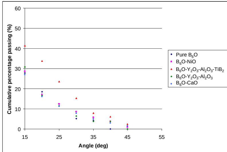
Figure 4-14: Crack deflection angles from Figure 12, redrawn between 15 and 45°
