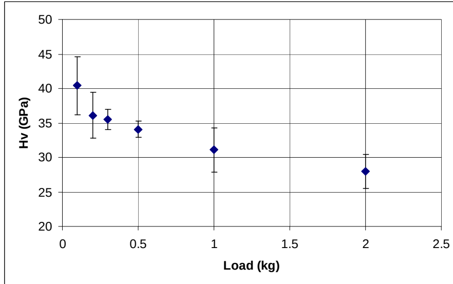
Figure 4-8: Effect of load on the measured Vickers hardness of hot-press, pure B 6 O
