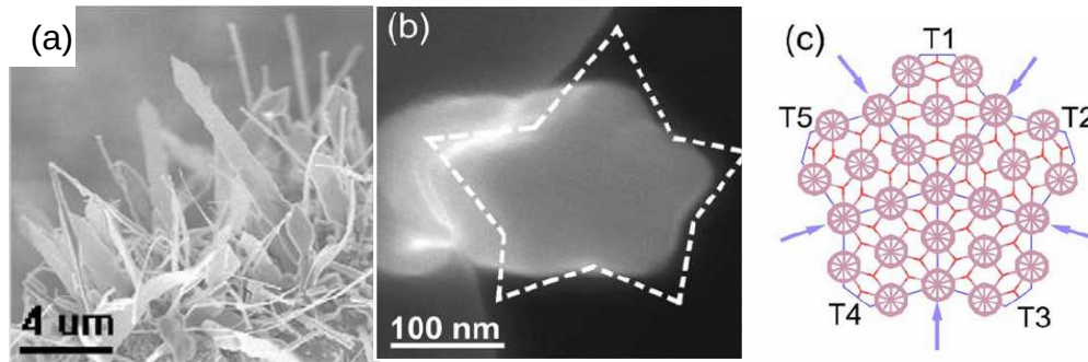
Figure 2-5: (a) SEM of B_6O platelets (Yu (2010)); (b) a cross-section of a nanowire with the proposed star geometry (Jiang (2006)); (c) a schematic of the cross-section showing the planes of twinning (Jiang (2006))
