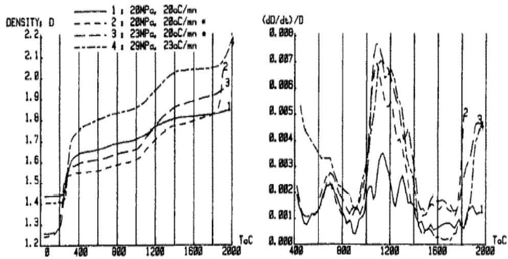
Figure 2-6: Densification of boron suboxide during hot pressing and reactive sintering (indicated by a *). Figure from Brodhag et al. (1986)
