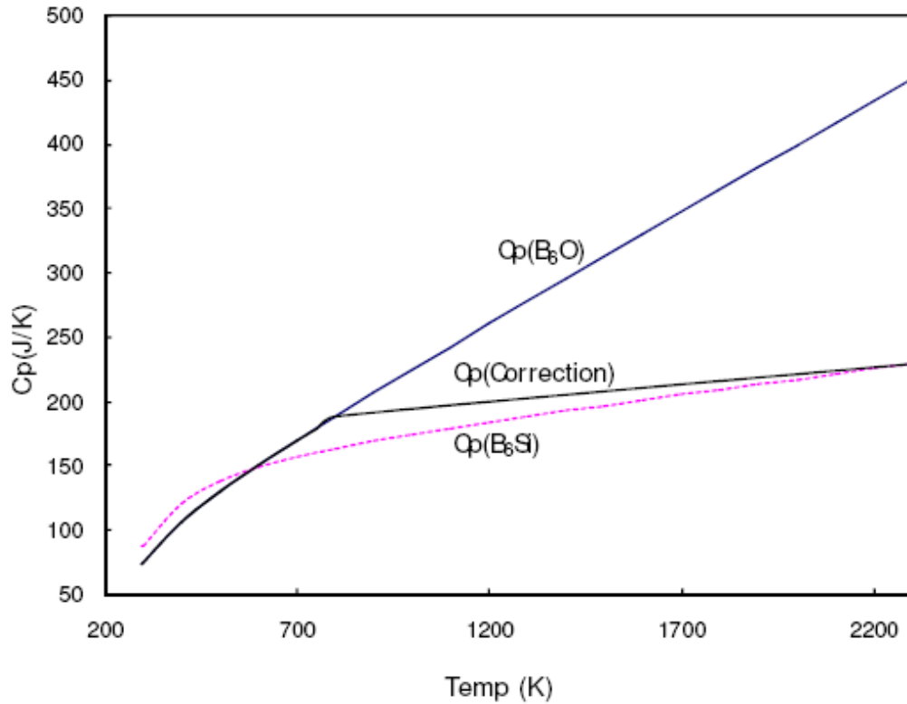
Figure 2-12: The effect of temperature upon heat capacity for B_6Si , B_6O (extrapolated experimental) and for B_6O after correction. (Andrews (2008))
