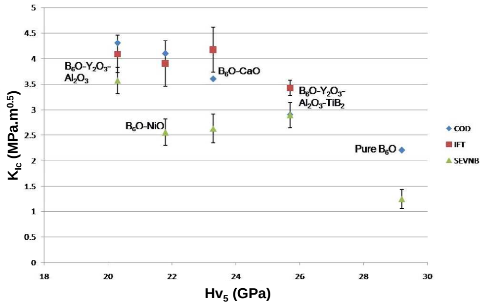
Figure 5-2: Fracture toughness data for pure boron suboxide with and without different sintering additives. Note that pure B_6O was tested under a 1kg load
