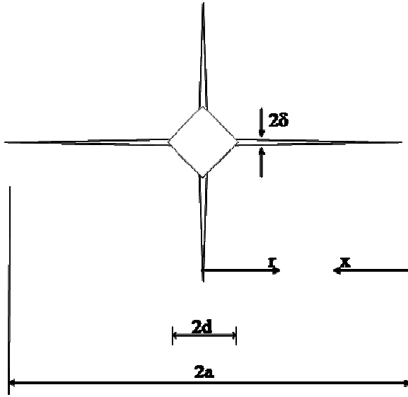
Figure 3-8: Schematic of an indentation showing measured dimensions for COD analysis
