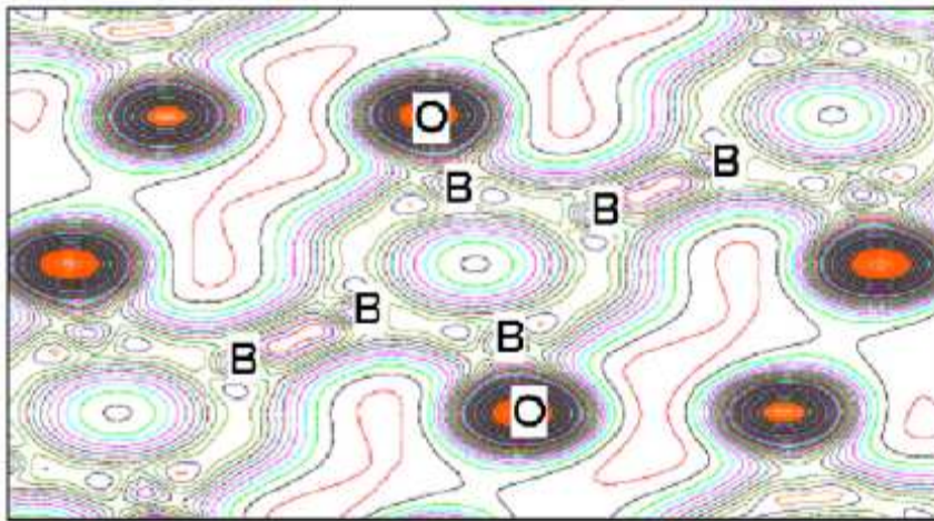
Figure 2-2: Electron density map for boron suboxide (calculated) Letsoala and Lowther (2008)
