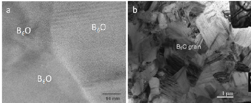
Figure 2-8: Bright field TEM images showing the clean interface between grains (a) (Andrews (2008)) and the multiple twinning within the B_6O grains (b) (Shabalala et al. (2008))
