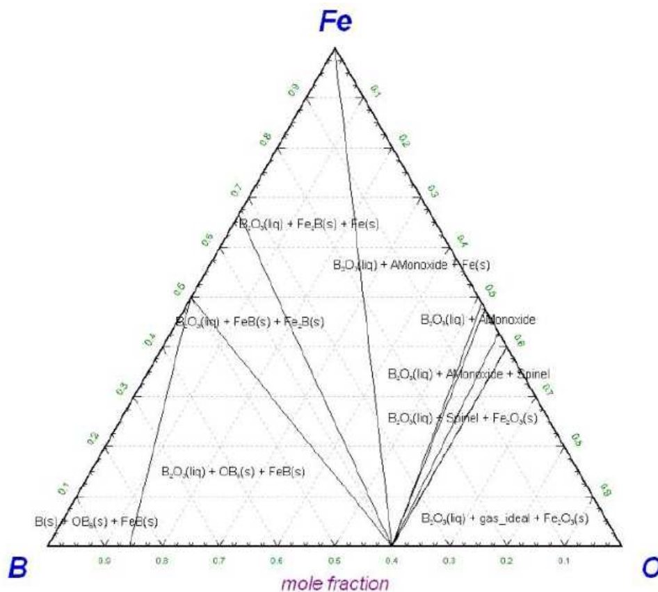
Figure 2-13: The B-O-Fe ternary phase diagram calculated for 700°C (Freemantle (2009))
