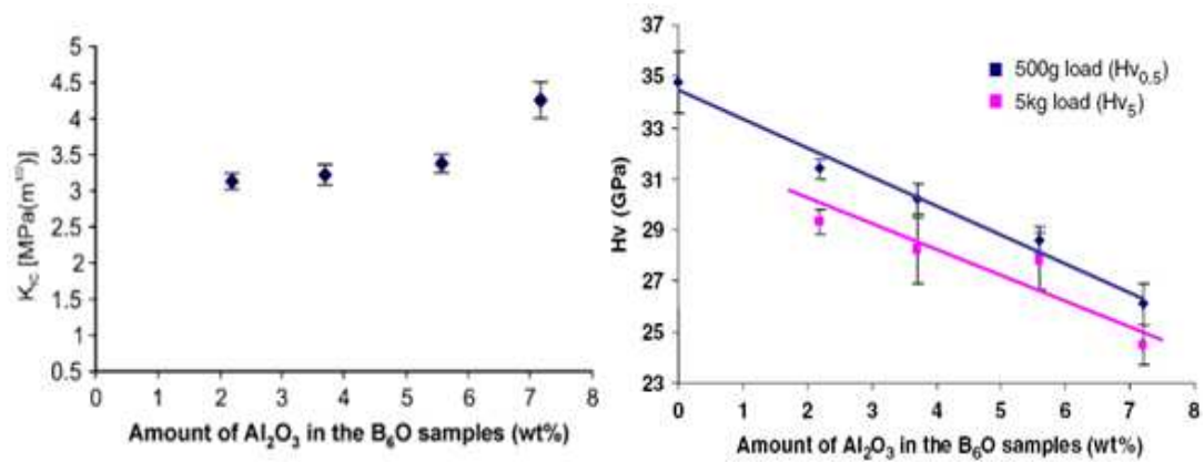
Figure 2-7: The effect of alumina on the fracture toughness and hardness of boron suboxide.
