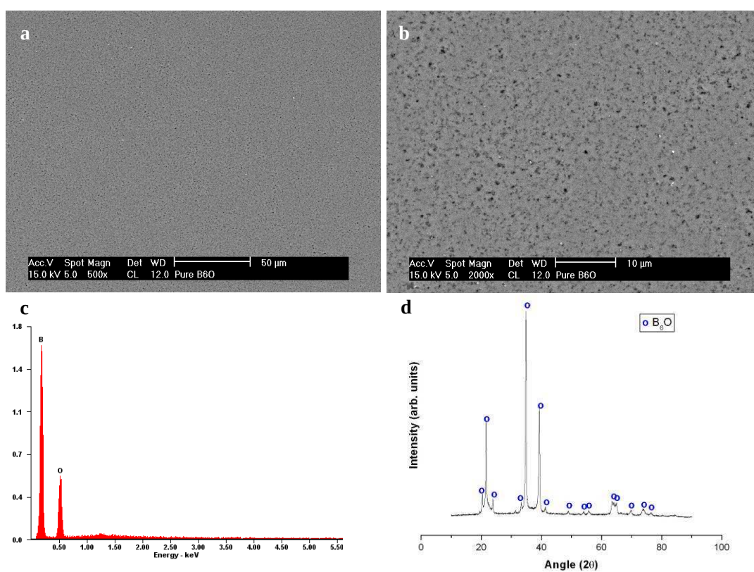
Figure 4-2: Structure (a,b), accompanying EDS spectrum (c) and XRD trace of pure B_6O .
