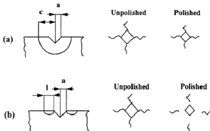
Figure 3-7: (a) Half-penny and (b) Palmqvist cracks as introduced by a Vickers indenter
