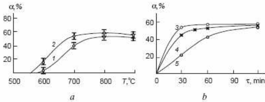
Figure 2-15: Temperature (a) and kinetic (b) curves for the reaction of powdered boron suboxide (1) and boron (2). Kinetic curves for boron suboxide under isothermal conditions at 900 (3), 800 (4) and 700°C (5) (Karamov (2002))
