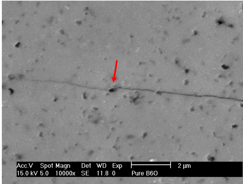
Figure 5-7: Crack deflection around a pore in pure boron suboxide
