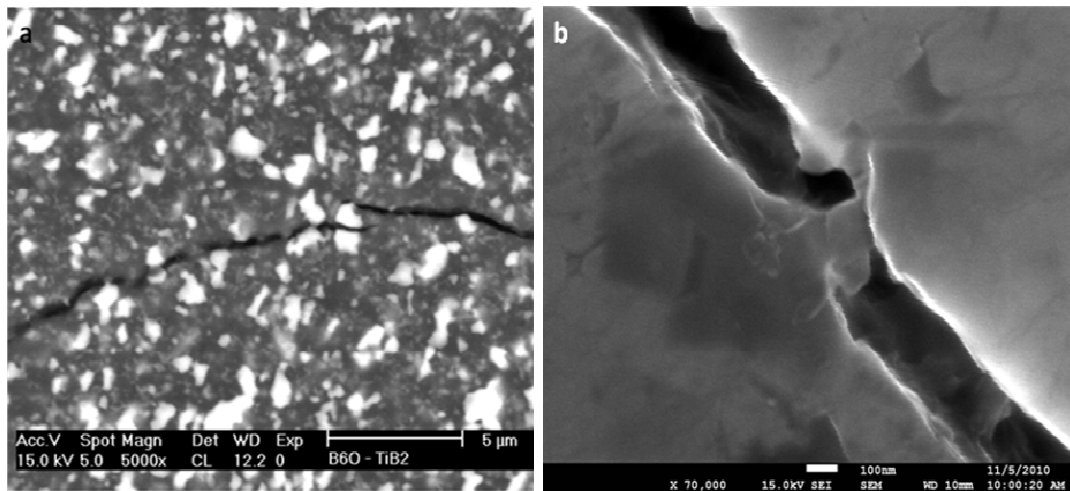
Figure 5-10: Crack bridging in (a) the \text{B}_6\text{O}-\text{Y}_2\text{O}_3-\text{Al}_2\text{O}_3-\text{TiB}_2 and (b) \text{B}_6\text{O}-\text{Y}_2\text{O}_3-\text{Al}_2\text{O}_3 composites
