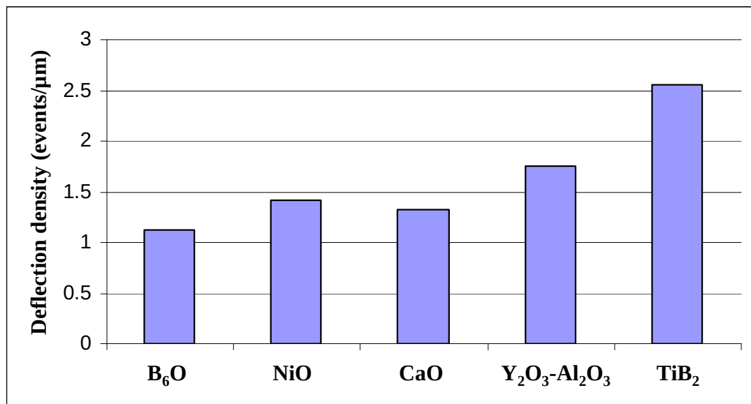
Figure 5-8: Crack deflection density for the boron suboxide materials
