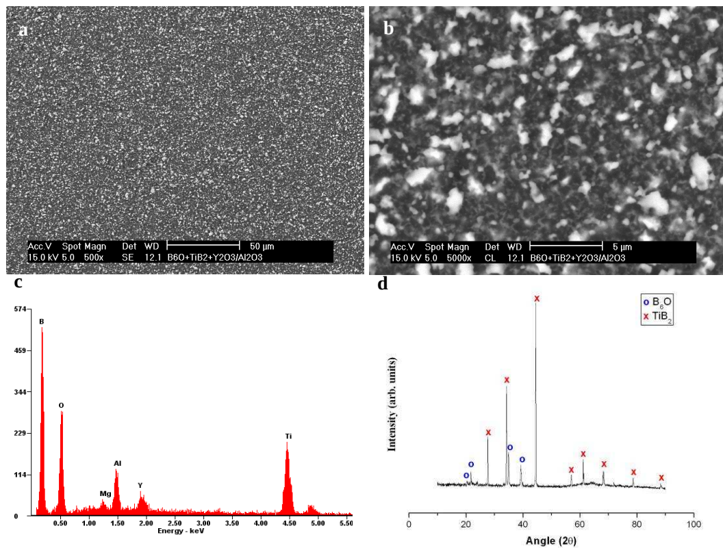
Figure 4-3: Structure (a,b), accompanying EDS spectrum (c) and XRD trace of B_6O - Y_2O_3 - Al_2O_3 - TiB_2 . EDS spectrum mapped area of image b.
