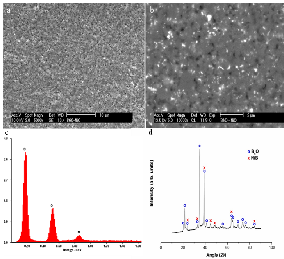
Figure 4-5: Structure (a,b), accompanying EDS spectrum (c) and XRD trace of B_6O -NiO.
