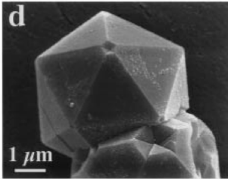
Figure 2-4: Indented apex, indicative of twinning, observed by Hubert et al. (1997)
