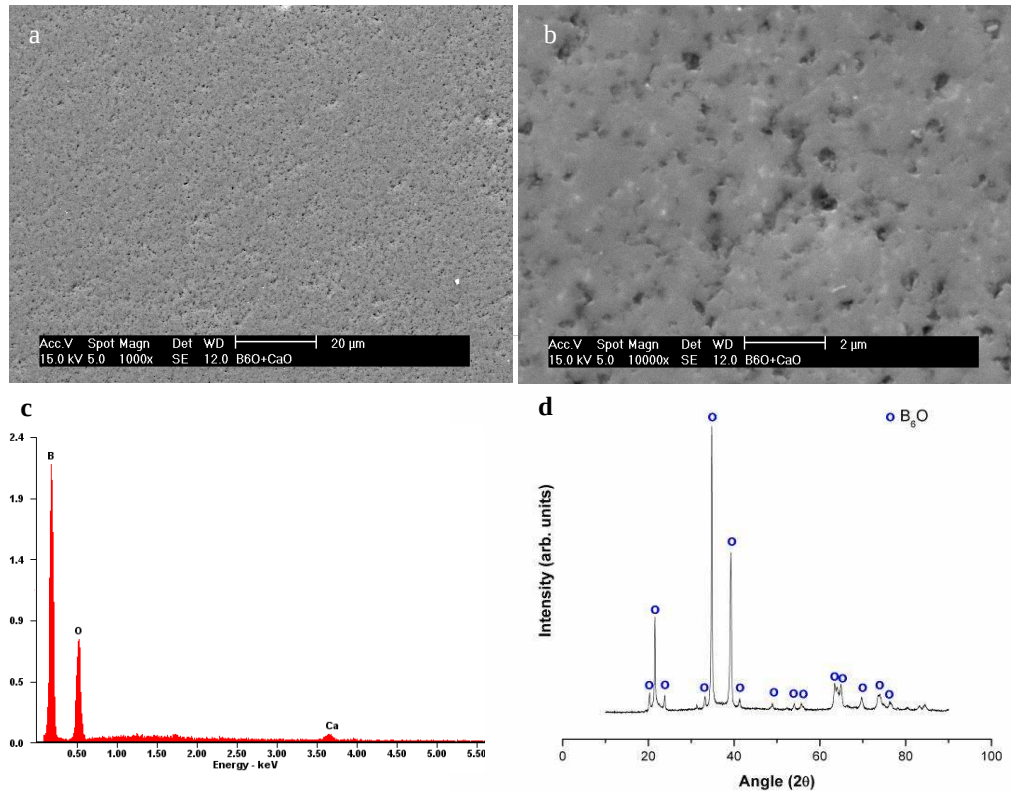
Figure 4-4: Structure (a,b), accompanying EDS spectrum (c) and XRD trace of B_6O -CaO. EDS spectrum area of mapped image b.
