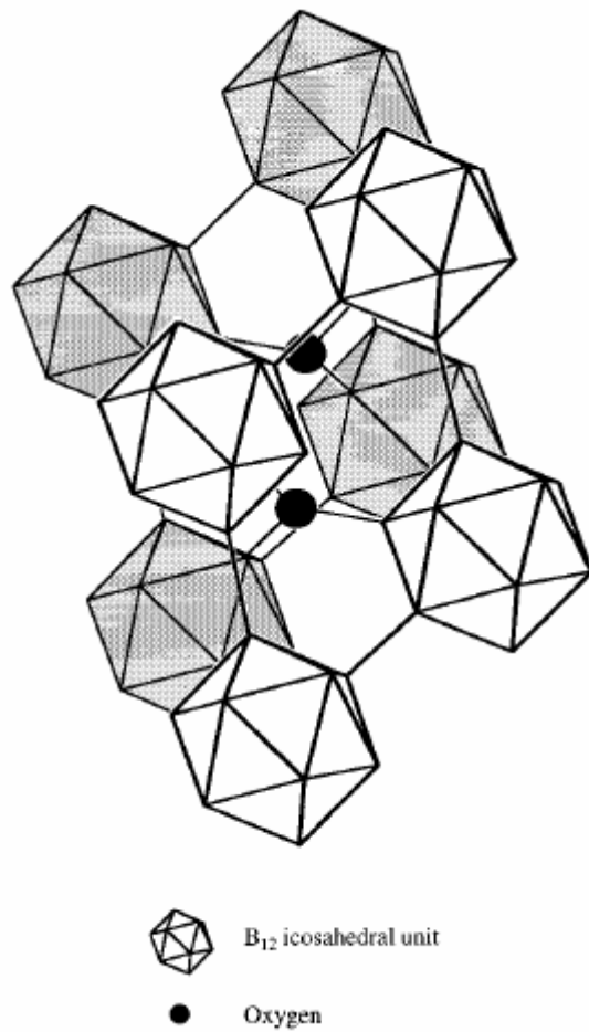
Figure 2-1: Rhombohedral cell of boron suboxide (Hubert (1998))
