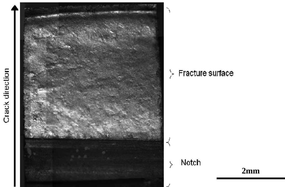
Figure 4-10: Optical image of a B_6O -NiO sample after SEVNB testing. The height of the sample is 4mm.
