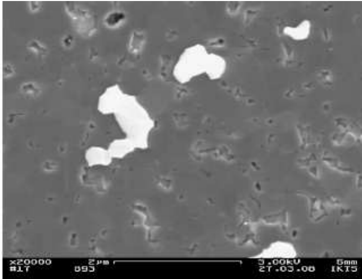
Figure 2-10: A B_6O - TiB_2 (without yttria additions) composite showing the TiB_2 grains (light phase) and partial removal of oxide grain boundary phase (Herrmann et al. (2009))
