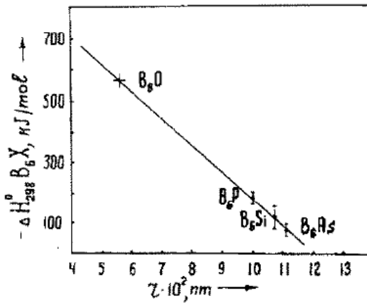
Figure 2-11: Standard enthalpy of formation as a function of atomic radius of X species in B_6X (Makarov and Ugai (1986))
