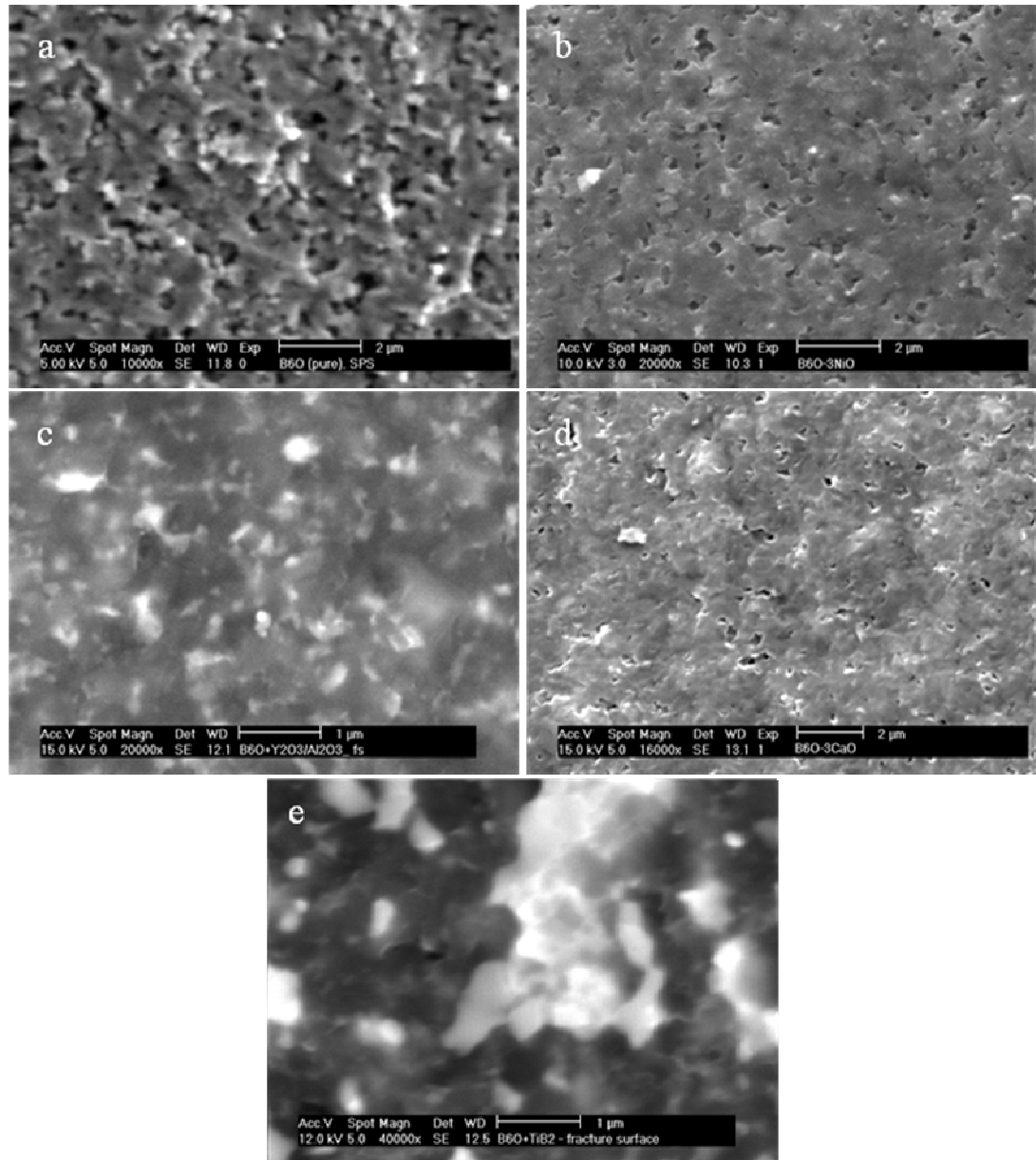
Figure 4-11: SEM images of the fracture surfaces of (a) pure B 6 O; (b) B 6 O – NiO; (c) B 6 O-Y 2 O 3 -Al 2 O 3 ; (d) B 6 O-CaO and (e) B 6 O – Y 2 O 3 - Al 2 O 3 – TiB 2
