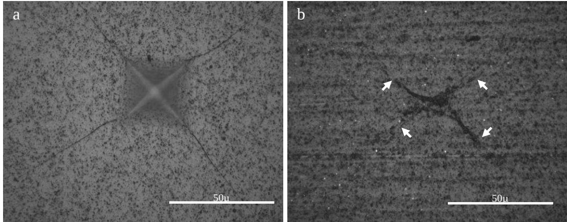
Figure 4-9: An indentation in \text{Y}_2\text{O}_3\text{-Al}_2\text{O}_3\text{-B}_6\text{O} before (a) and after (b) polishing. The white arrows indicate where the cracks are still attached indentation.
