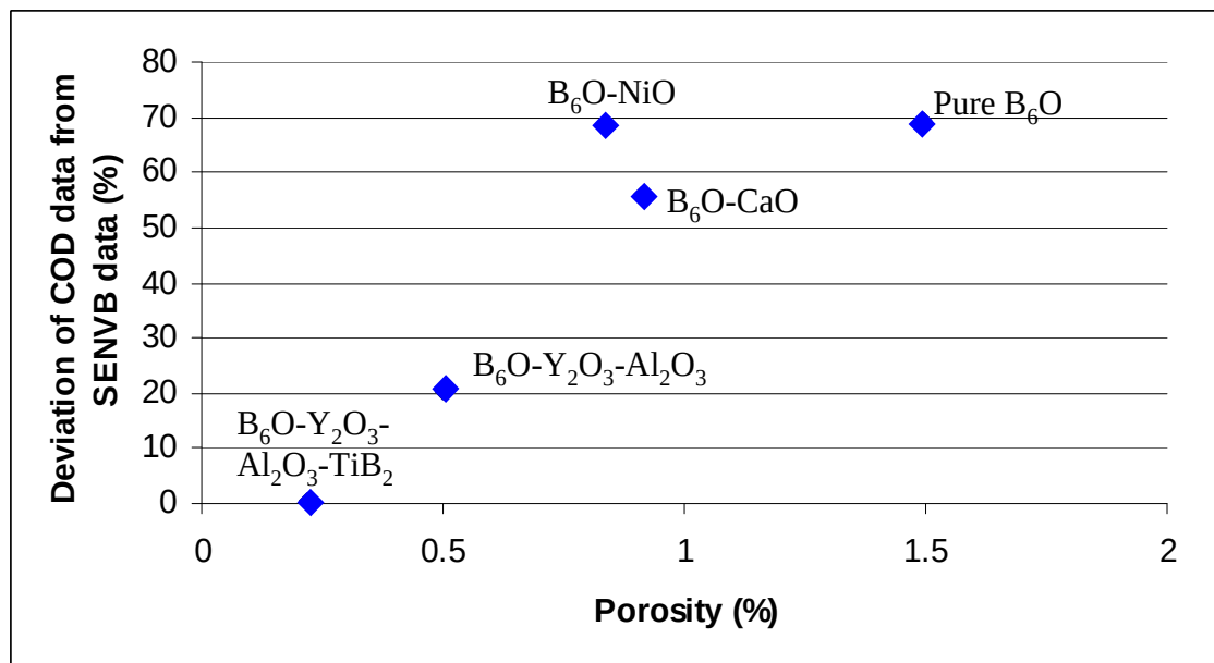
Figure 5-4: Effect of open porosity upon the COD measurements deviation from SEVNB measurements
