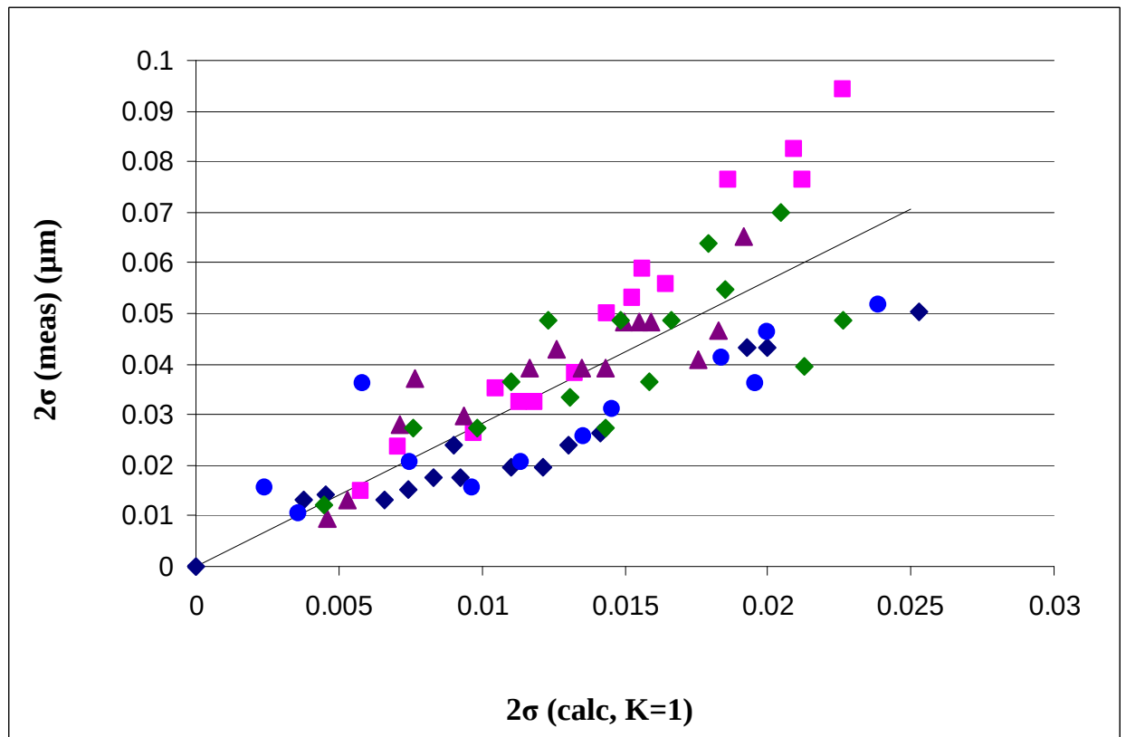
Figure B4: COD analysis for the \text{TiB}_2\text{-Y}_2\text{O}_3\text{-Al}_2\text{O}_3\text{-B}_6\text{O} composite. K_{\text{Ic, COD}} = 2.8 \text{ MPa}\cdot\text{m}^{0.5}
