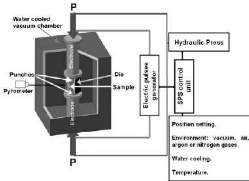
Figure 3-2: Schematic drawing of an SPS configuration (Hungria et al. (2009))
