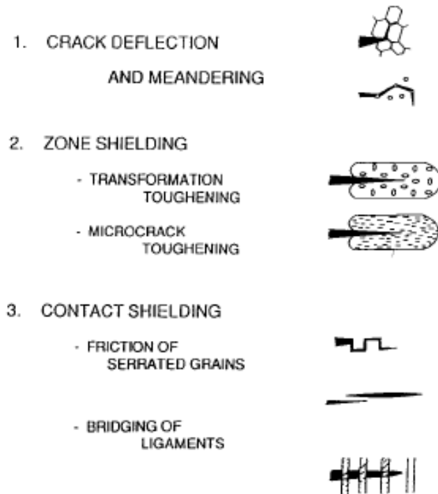
Figure 2-19: The three types of toughening mechanisms (Steinbrech (1992))
