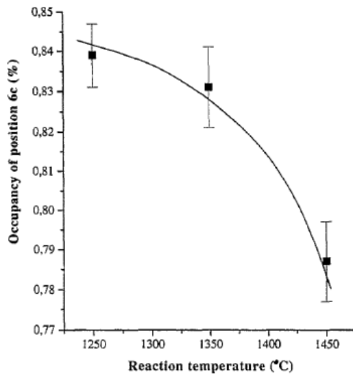
Figure 2-3: Occupancy of the 6c position in B_6O by oxygen. From Lundström (1997)
