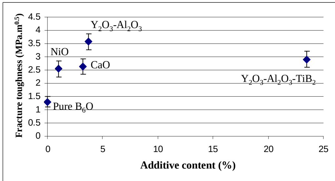
Figure 5-3: SEVNB fracture toughness of boron suboxide materials as a function of additive content
