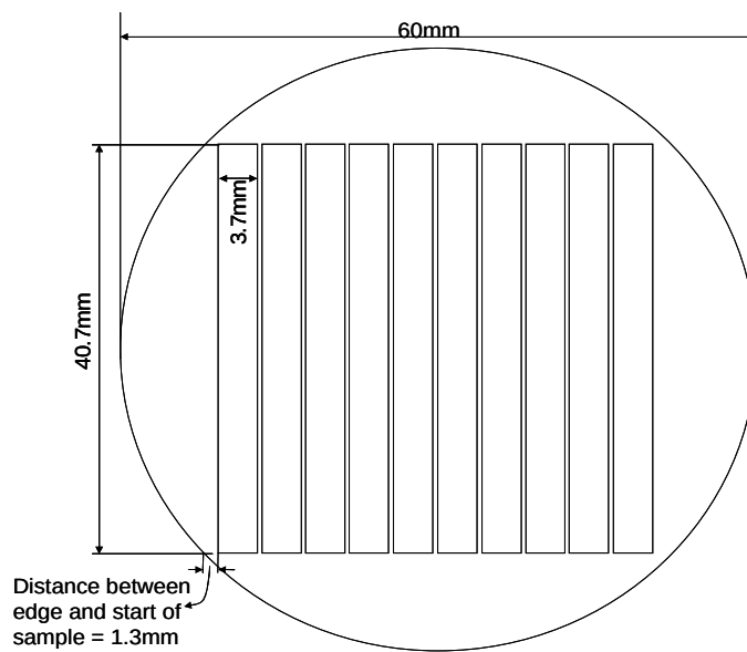
Figure 3-3: Schematic diagram of the layout of the rectangular bars as cut out of the composite discs
