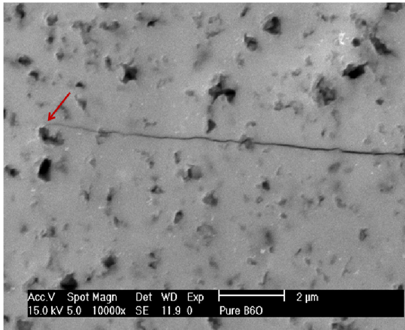
Figure 5-11: Crack arrest by a pore in pure boron suboxide
