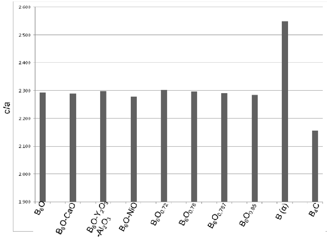
Figure 5-15: c to a ratio for the boron based materials.
