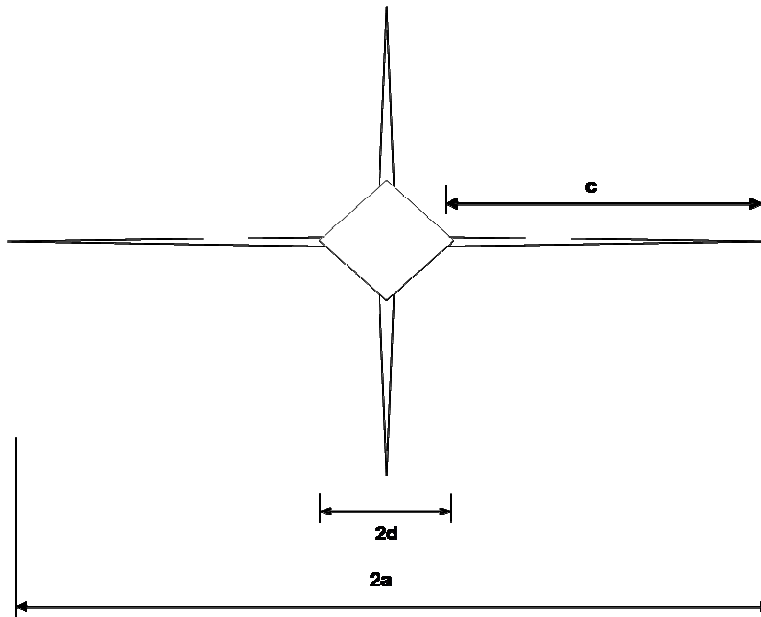
Figure 3-6: An indentation, showing measured dimensions for IFT
