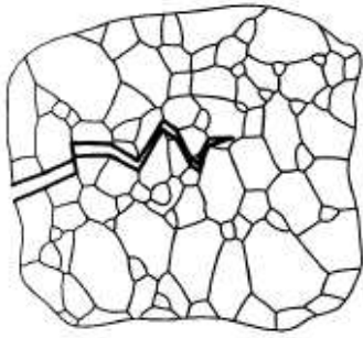
Figure 2-21: Ligaments toughening a brittle ceramic by frictional action (Roesler (2007))
