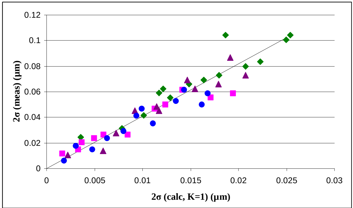
Figure B2: COD analysis for B 6 O-NiO
