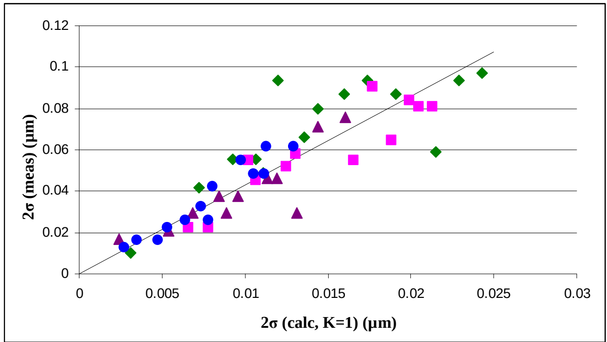
Figure B1: COD analysis for \text{B}_6\text{O-Y}_2\text{O}_3\text{-Al}_2\text{O}_3
