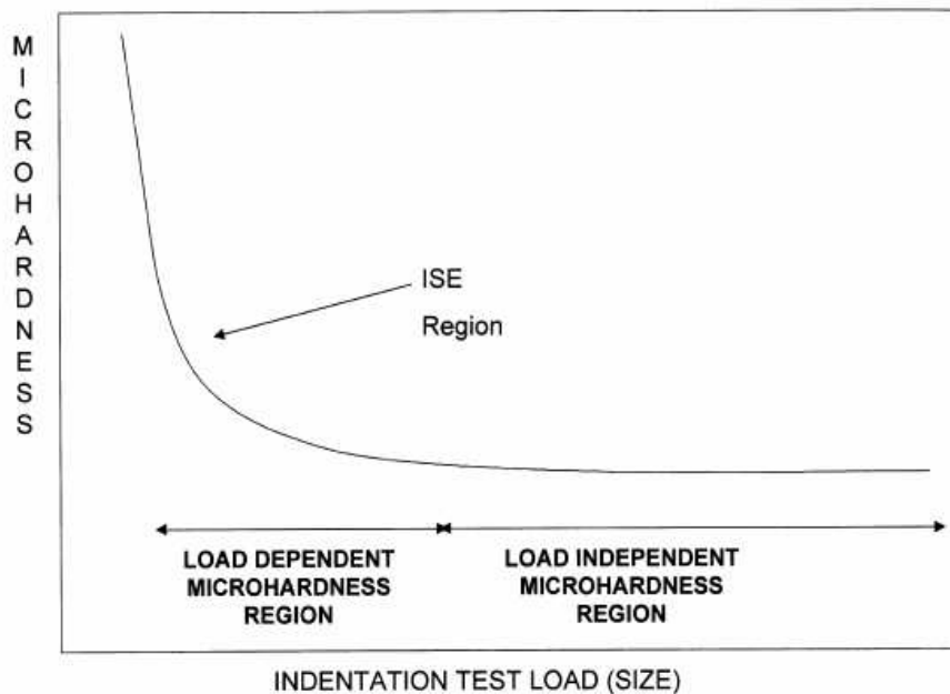
Figure 2-16: Effect of load on microhardness (Stevenson et al. (2002))
