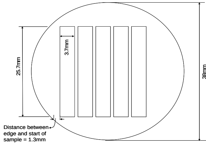
Figure 3-4: Schematic diagram of the layout of the rectangular bars as cut out of the pure B_6O discs
