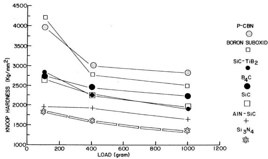
Figure 2-17: Hardness against load for various ceramics (Ellison-Hayashi (US Patent 5330937))
