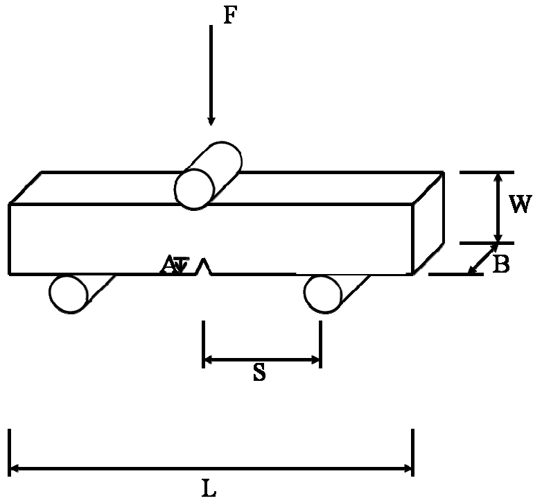
Figure 3-10: Schematic of SEVNB testing layout (Kübler (2002)).
