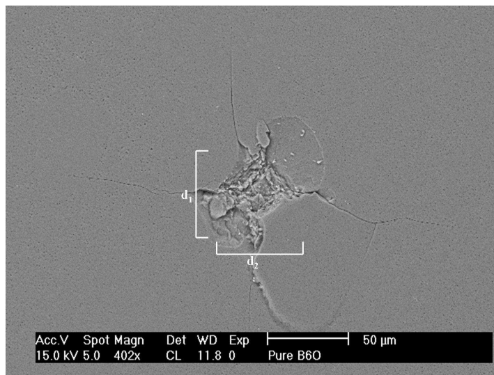
Figure 3-9: An approximation of the diagonal lengths for an indentation in pure boron suboxide
