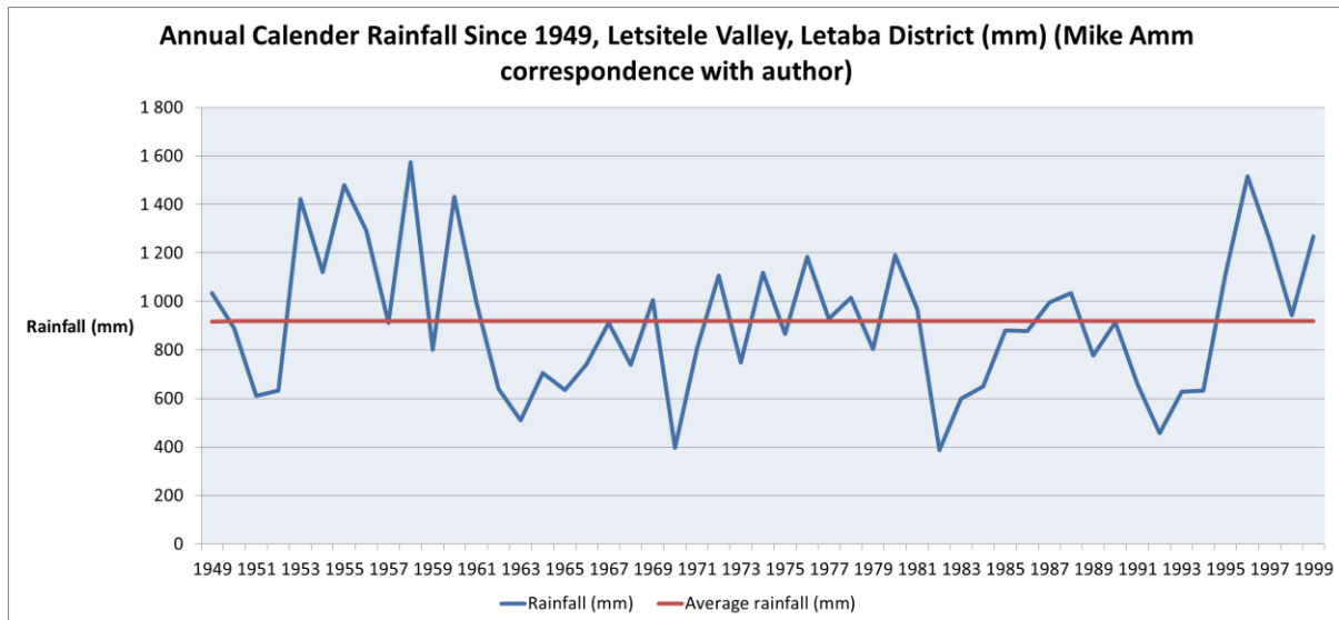
Fig. 7. Annual Calender Rainfall 1949 - 1999, Letsitele Valley, Letaba District
