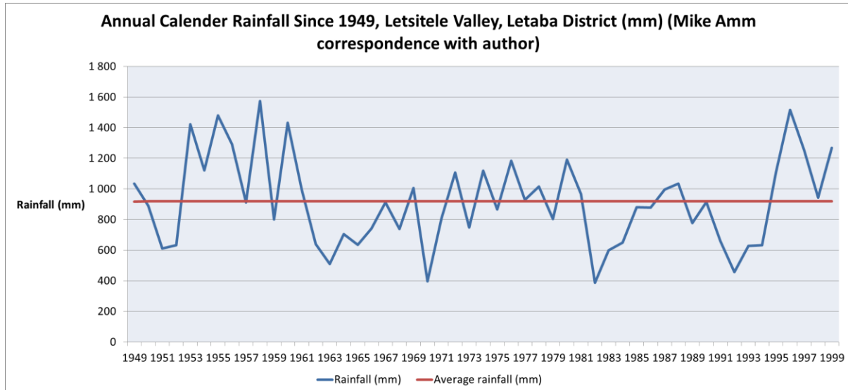
Fig. 9. Annual Calendar Rainfall 1949 - 1999, Letsitele Valley, Letaba District
