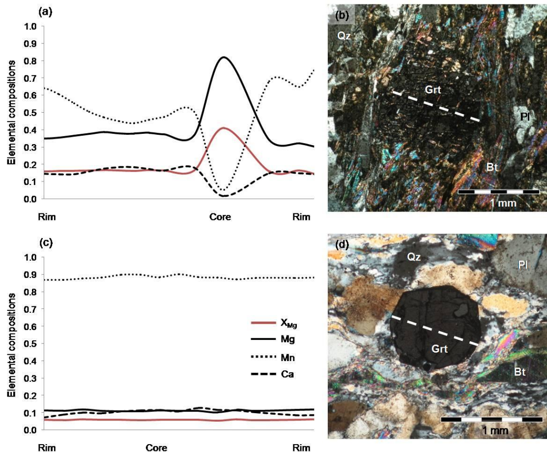
Figure 4.4: Elemental compositional profiles for garnet in the lower basement-derived (a) mica schist (sample RG53 n = 15 ) with (b) accompanying reference photomicrograph (XPL), and in the lower basement-derived (c) granite (sample RG40; n = 15 ) with (d) accompanying reference photomicrograph (XPL). White dashed lines in the photomicrographs indicate the approximate locations of each compositional profile. Abbr.: Bt = biotite; Grt = garnet; n = number of analyses; Pl = plagioclase; Qz = quartz; XPL = cross polarised light.
