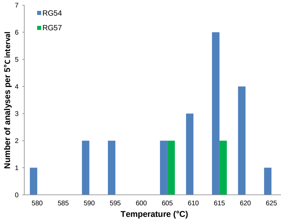
Figure 4.10: Distribution of temperatures calculated from Zr-in-rutile thermometry (assuming 0.4 GPa) for the lower basement-derived samples RG54 and RG57.
