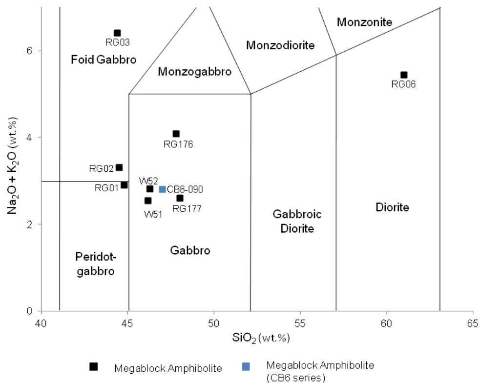
Figure 3.19: Bi-variate TAS diagram illustrating possible protoliths for the megablock amphibolite rock unit (after Middlemost, 1994) of the Eyreville-B borehole core. All data in wt%.
