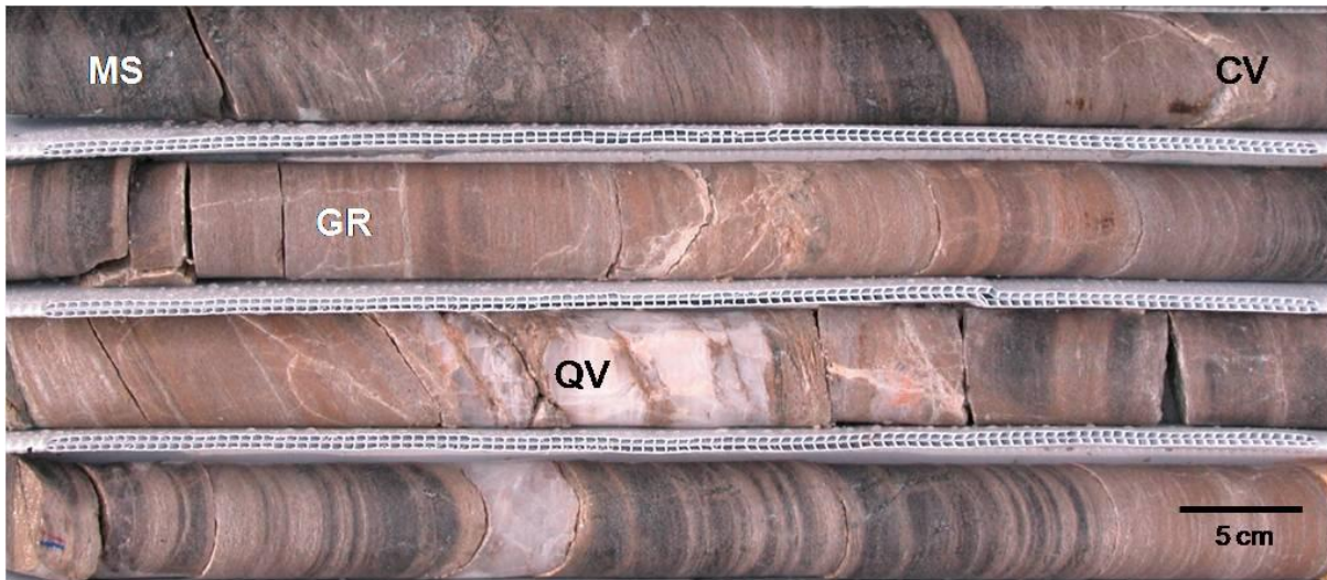
Figure 2.8: Photograph of corebox 310 illustrating the fine-grained alternating mica schist and granite layers in the lower basement-derived mylonite zone. Abbr.: CV = chlorite vein; GR = granite; MS = mica schist; QV = quartz vein.
