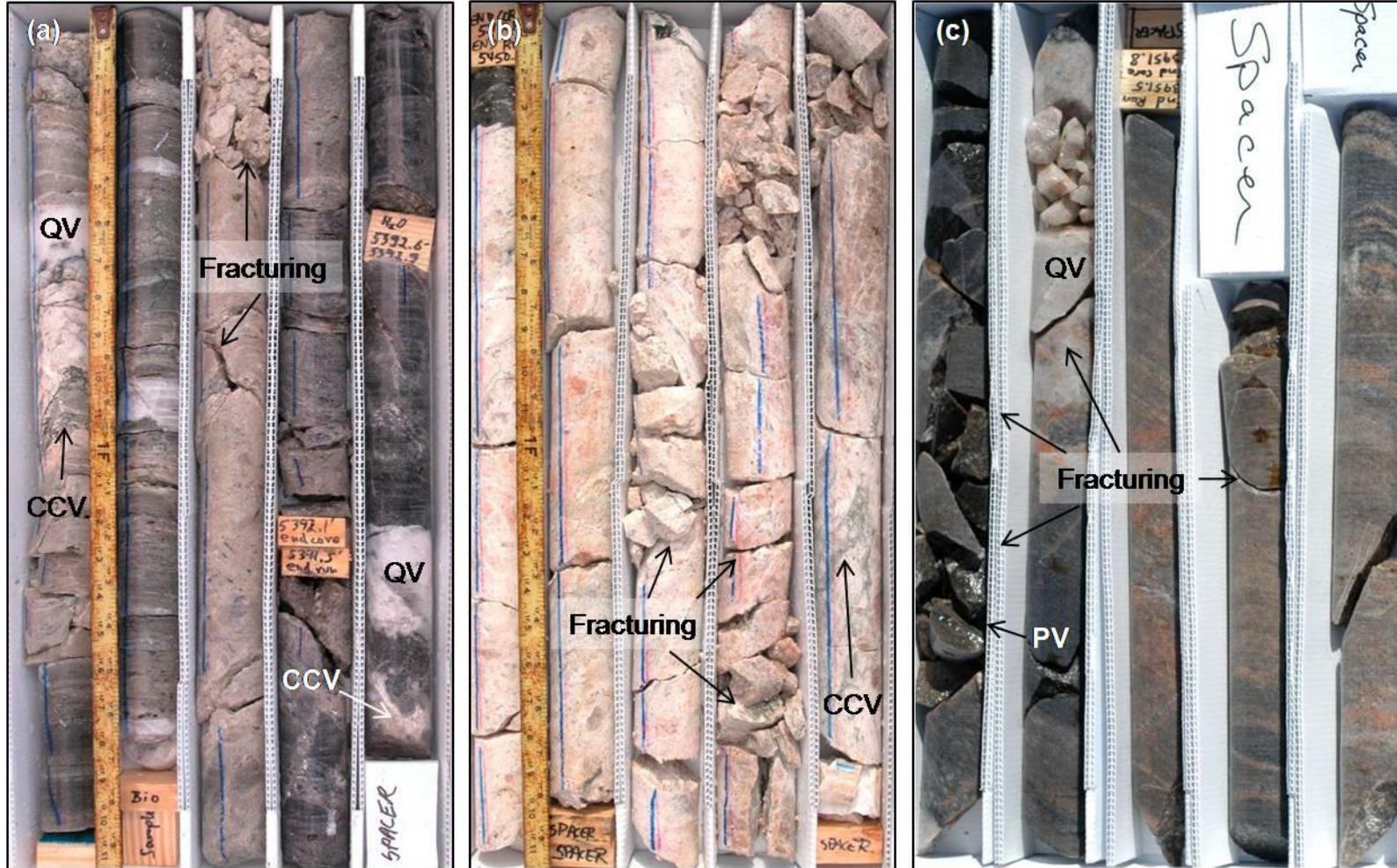
Figure 2.20: Corebox photographs showing fracturing containing varying amounts of Cal, Chl, Py and Qz within the (a) the lower basement-derived mica schist (Corebox 307) and granite (Corebox 314), and within the (c) gneissic megablock granite (Corebox 159). Abbr.: Cal = calcite; CCV = calcite and chlorite vein; Chl = chlorite; PV = pyrite vein; Py = pyrite; QV = quartz vein; Qz = quartz.
