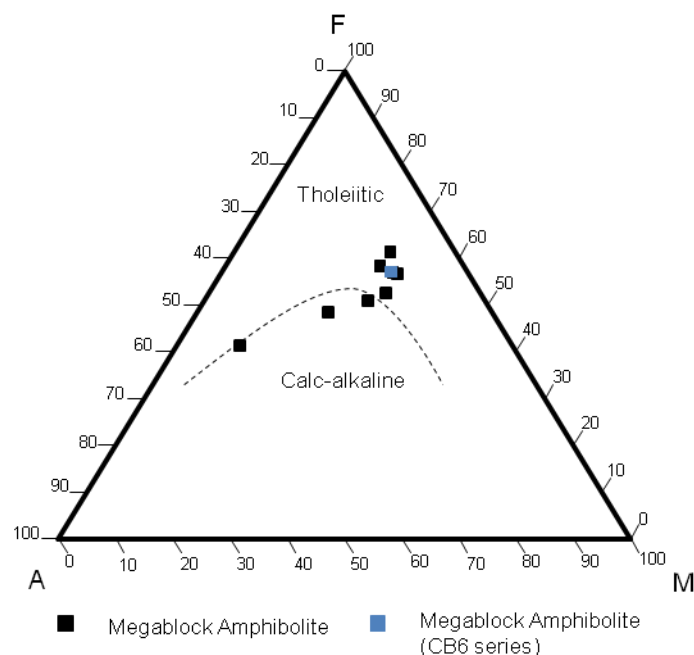
Figure 3.20. Ternary diagrams indicating AFM abundances (wt%) for the megablock amphibolite rock units of the Eyreville-B borehole core. Black dashed line shows the chemical boundary between tholeiitic and calc-alkaline magma series (after Irving and Baragar, 1971). Abbr.: A (alkalis) = \text{Na}_2\text{O} + \text{K}_2\text{O} ; F = \text{Fe}_2\text{O}_{3(\text{total})} ; M = \text{MgO} .
