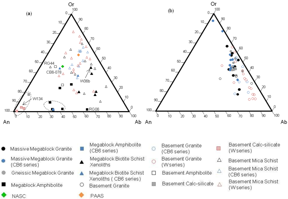
Figure 3.4: Ternary diagrams indicating normative An-Or-Ab content calculated for (a) the mica schist, amphibolite and calc-silicate, and (b) the granite rock units of the Eyreville-B borehole core. Abbr.: An = anorthite; Or = orthoclase; Ab = albite; NASC = North American Shale Composite (after Gromet et al. , 1984); PAAS = Post-Achaeon Australian Shale (after Taylor and McLennan, 1985). Dashed lines represent observed groupings.
