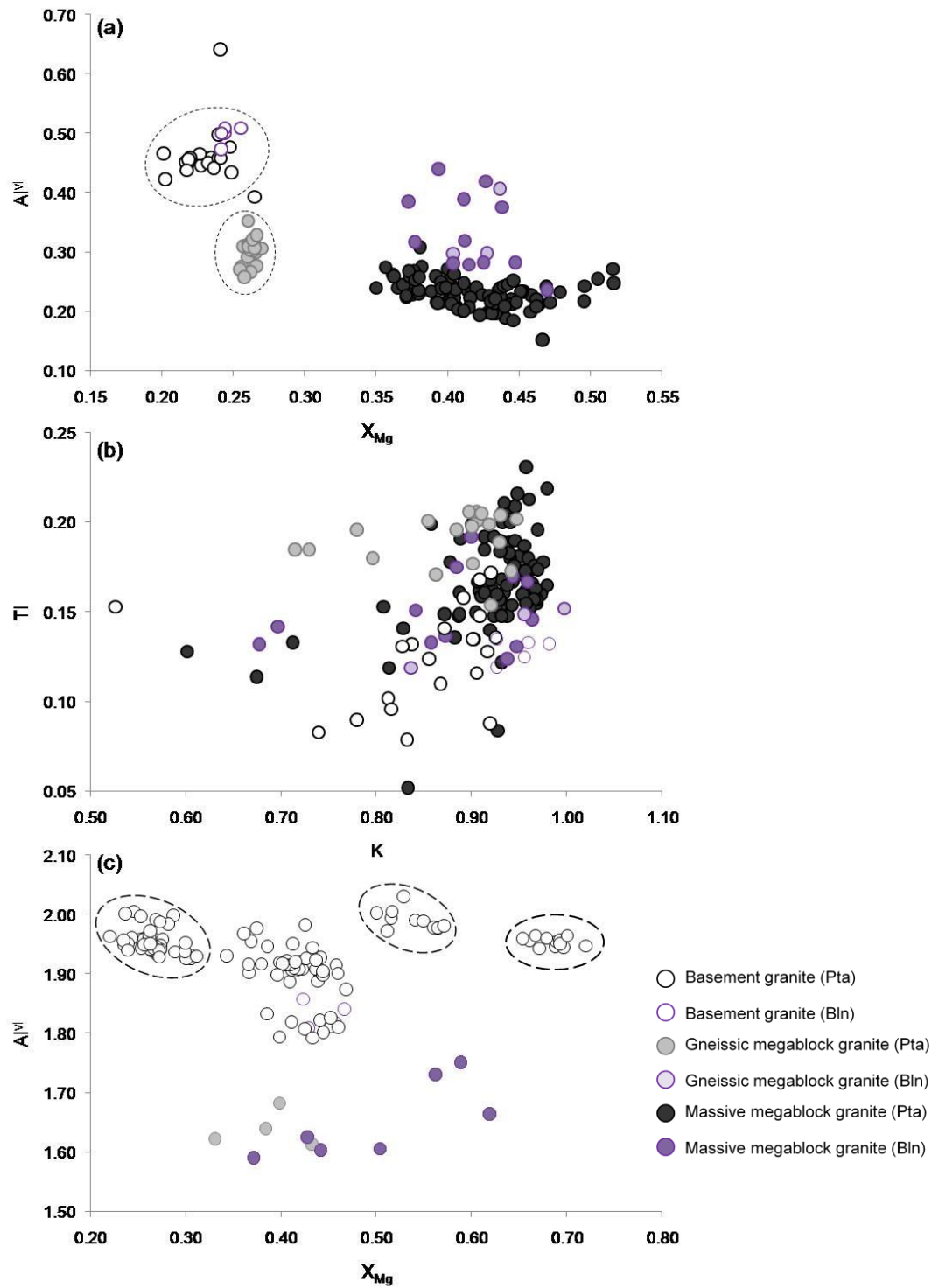
Figure 4.8: (a) X_{Mg} vs. Al^{VI} and (b) K vs. Ti abundances (apfu for 11 oxygens) in Bt and (c) X_{Mg} vs. Al^{VI} abundances (apfu for 11 oxygens) in Ms for the lower basement-derived granite (Bt n = 25; Ms n = 115) and upper gneissic (Bt n = 22; Ms n = 4) and massive (Bt n = 105; Ms n = 9) megablock granites. Dashed lines represent observed groupings. Abbr.: Bln = EMP analyses obtained in Berlin; Bt = biotite; Ms = muscovite (white mica); n = number of analyses; Pta = EMP analyses obtained in Pretoria.
