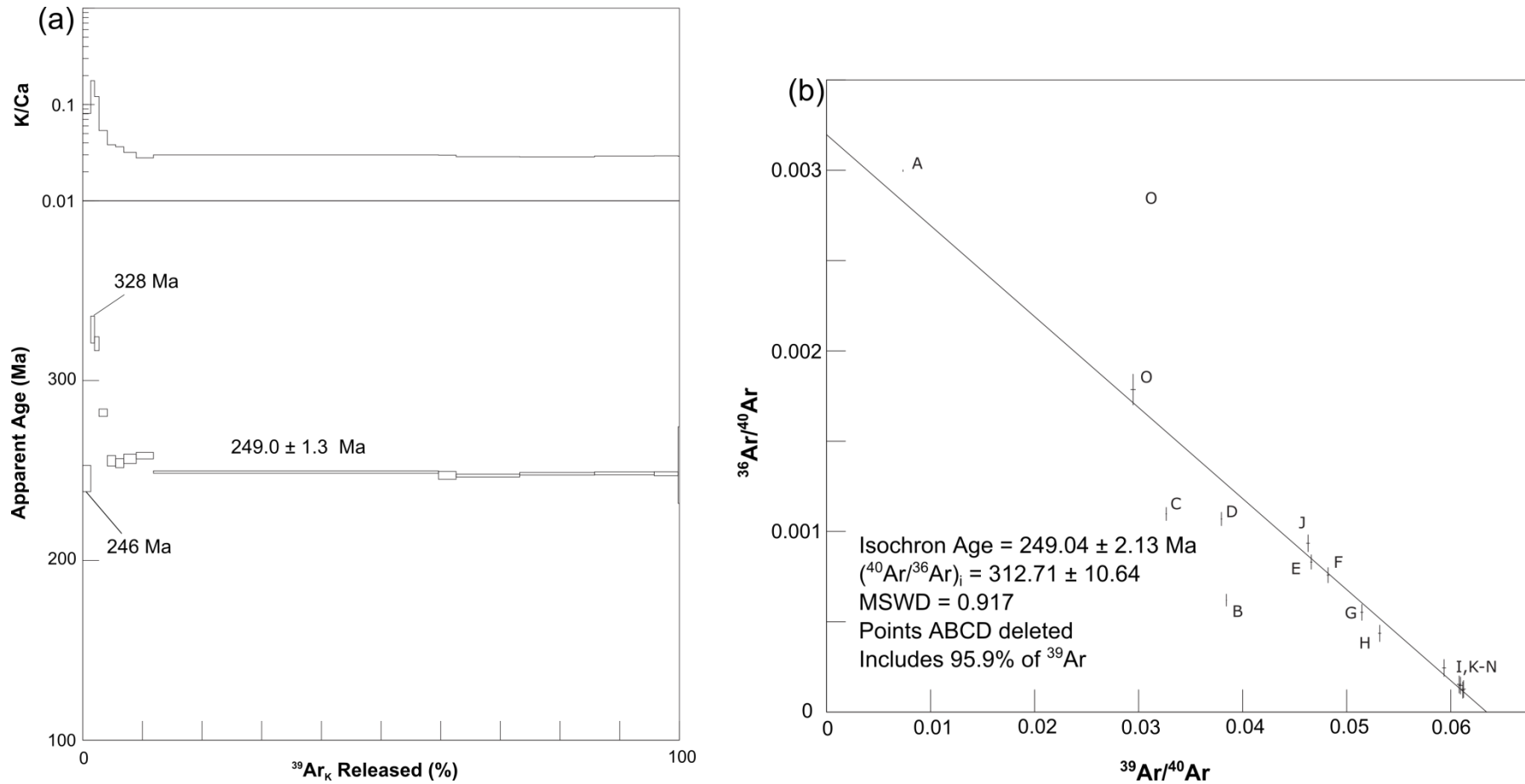
Figure 5.6: Amphibole (a) age spectrum, K/Ca and (b) inverted isochron diagrams for the amphibolite megablock sample RG177. For (a) plateau ages ( \pm 1\sigma ), age maxima and age minima are as indicated. For (b), the inverted isochron age is meaningful as \text{MSWD} < 2.5 and (^{40}\text{Ar}/^{36}\text{Ar})_i \geq 295.5 (Kunk et al. , 2005). Points A, B, C and D were dropped to improve the fit of the data. Abbr.: MSWD = mean square of weighted deviates.
