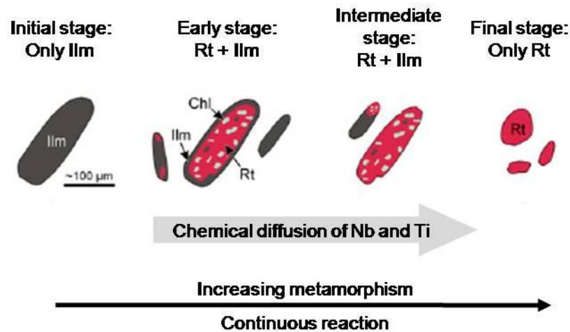
Figure 5.2: Schematic of the prograde formation of rutile from ilmenite under low- to medium-grade metamorphic conditions (after Luvizotto et al. , 2009b, and Meinhold, 2010). Abbr. Chl = chlorite; Ilm = ilmenite; Rt = rutile.
