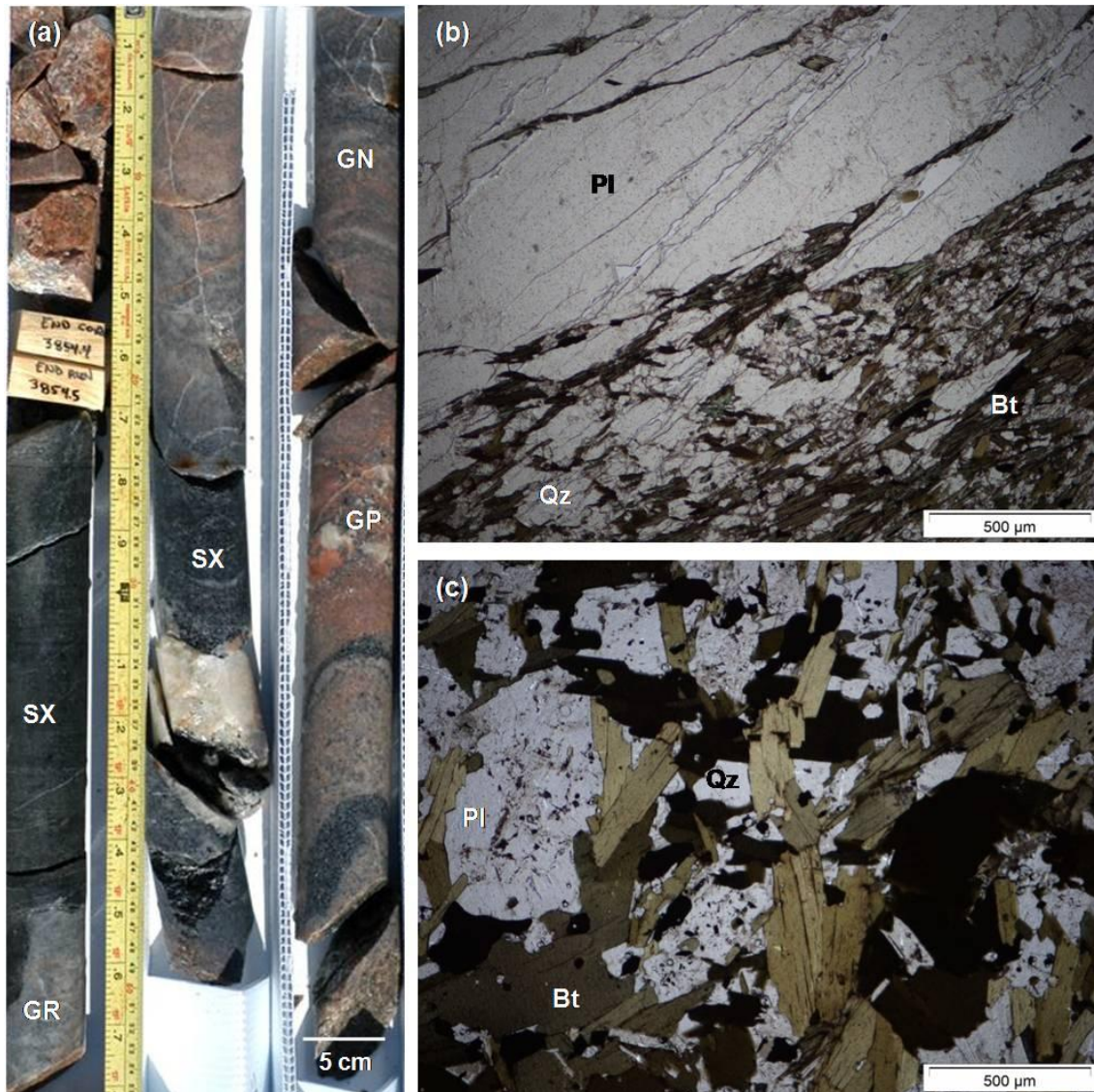
Figure 2.15: Photographs of the schist xenoliths in the upper granite megablock. (a) Corebox 147 illustrating the location of the xenoliths within the massive and gneissic granite. Photomicrographs (PPL) of sample W39 showing (b) the irregular contact between the schist and granite. (c) Photomicrograph of sample W36b showing the relative size and abundance of Bt compared to the massive and gneissic megablock granites. Abbr.: Bt = biotite; GN = gneissic granite; GP = granite pegmatite; GR = massive granite; Pl = plagioclase; PPL = plane polarised light; Qz = quartz; SX = schist xenoliths.
