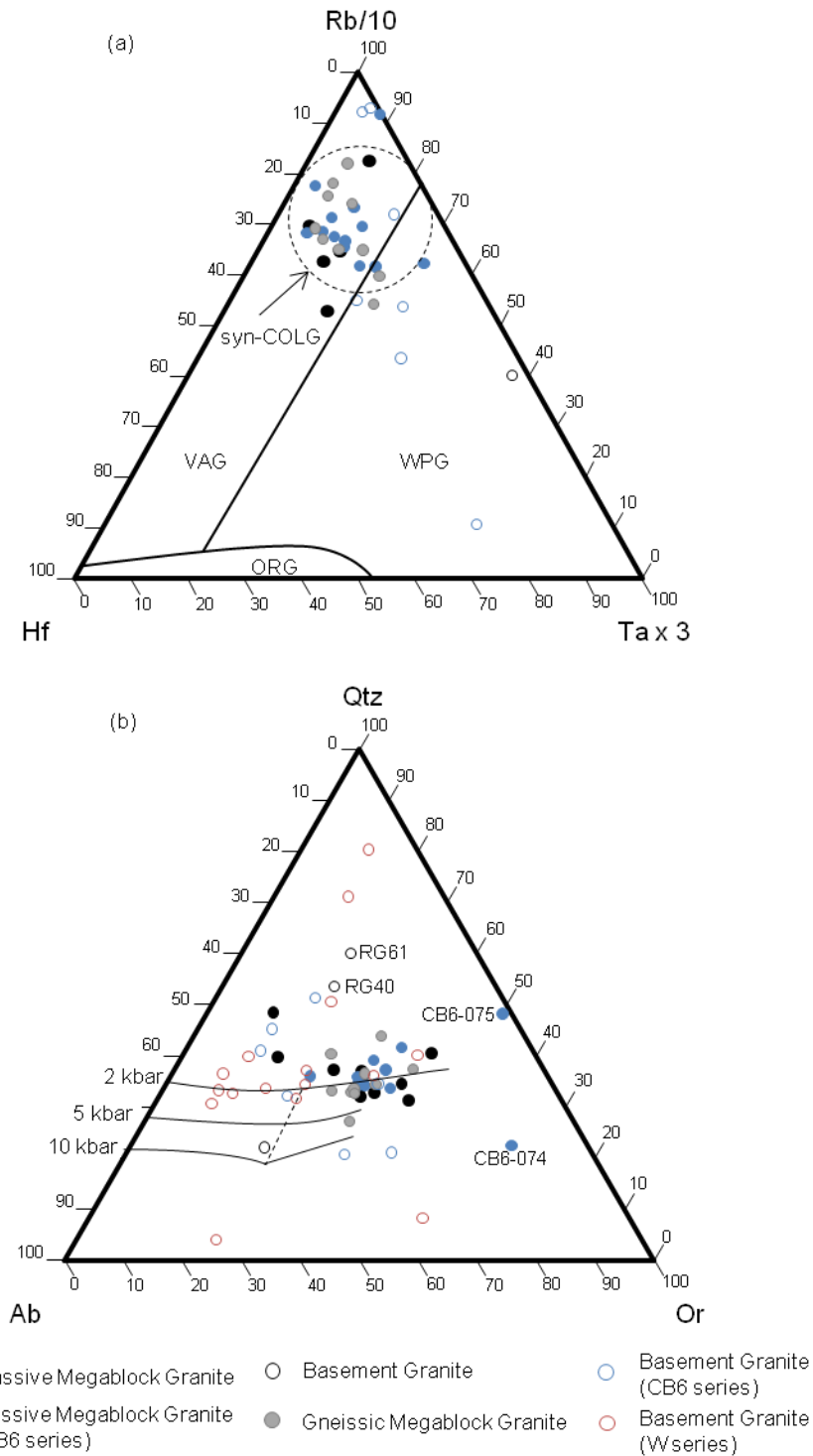
Figure 3.23: Ternary discrimination diagrams for the granites of the Eyreville-B borehole core. (a) Hf-Rb/10-Tax3 diagram showing different tectonic settings (data in ppm; after Harris et al. , 1986). (b) Ab-Qtz-Or diagram showing cotectic curves in an H 2 O-undersaturated system. Dashed line represents the water-undersaturated curve for a_{H_2O} = 0.8 crustal fluids in equilibrium with graphite (after Johannes and Holtz, 1991). Abbr.: VAG = volcanic-arc granite; syn-COLG = syncollisional granite; WPG = within-plate granite; ORG = ocean-ridge granite; Ab = albite; Q = quartz = Or = orthoclase.
