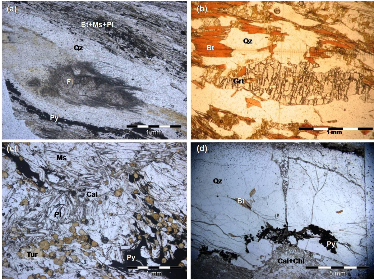
Figure 2.3: Photomicrographs of samples from the lower basement-derived mica schist. (a) Sample RG44 showing a Fi knot (PPL). (b) Skeletal and elongated garnet in sample RG53 (PPL). (c) Sample RG38 illustrating the intercalation of Tur and Py with Ms and Pl (PPL). (d) Brecciated fracture in Qz with Py, Cal and Chl fracture-fill in sample RG43 (PPL). Abbr.: Bt = biotite; Cal = calcite; Chl = chlorite; Fi = Fibrolite; Gr = Graphite; Grt = garnet; Ms = muscovite; Pl = plagioclase; PPL = plane polarised light; Py = pyrite; Qz = quartz; Tur = tourmaline.
