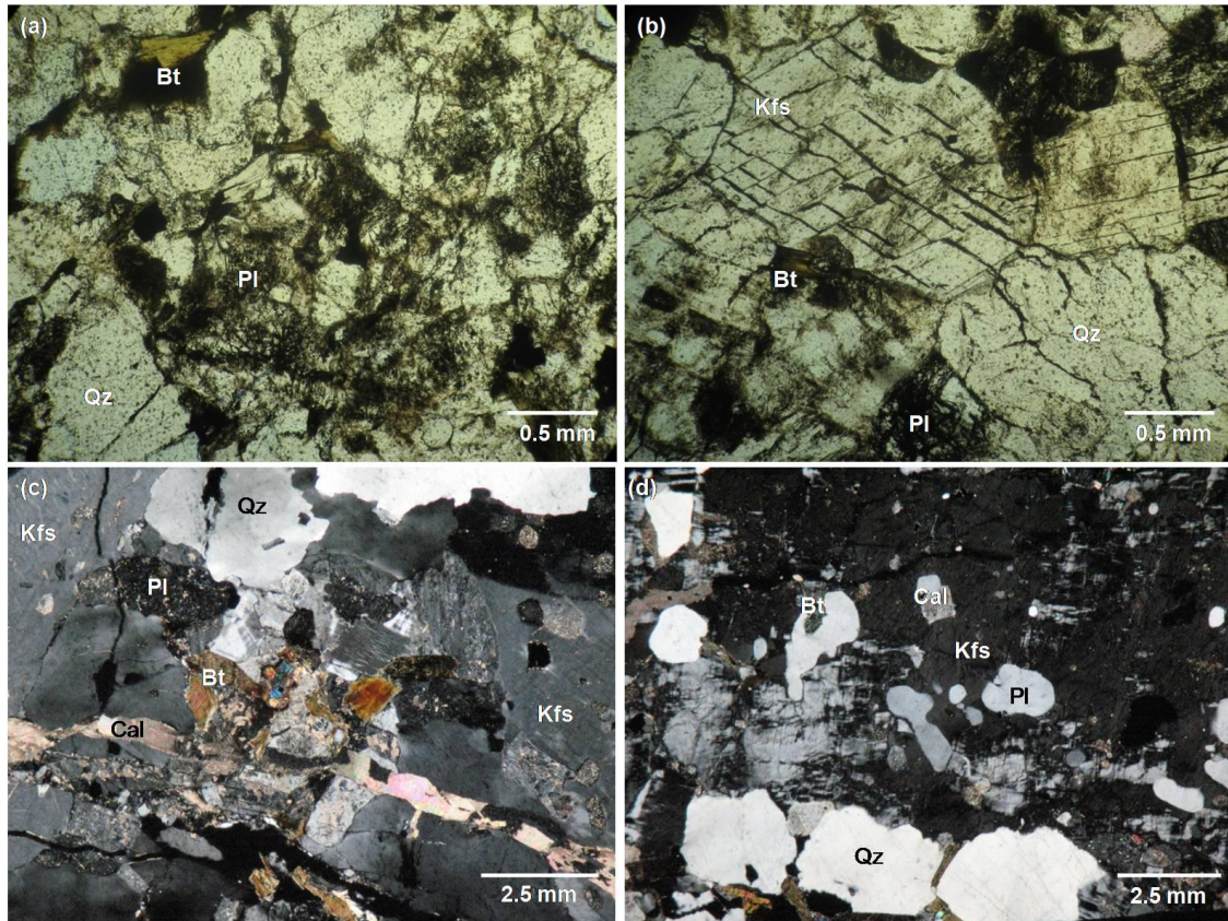
Figure 2.24: Photomicrographs of (a) sample RG154 showing the extensive seritisation of plagioclase grains in the gneissic megablock granite (PPL), (b) sample RG158 showing bent twins in K-feldspar phenocrysts in the gneissic megablock granite (PPL), and sample W49 showing (c) the less altered nature of the massive megablock granite (XPL) with (d) K-feldspar bent twins and myrmekitic textures (XPL). Abbr.: Bt = biotite; Cal = calcite; Kfs = K-feldspar; Pl = plagioclase; PPL = plane polarised light; Qz = quartz; XPL = cross polarised light.
