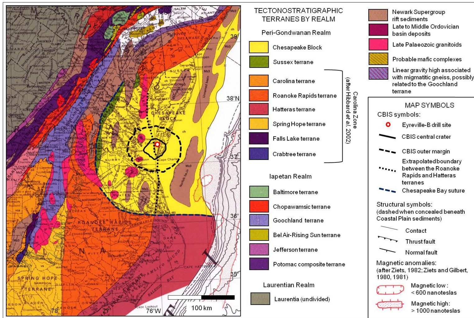
Figure 1.9: Tectonostratigraphic terrane map of the Central Appalachians showing the location of the Chesapeake Bay suture (after Horton et al. , 1991), Chesapeake block, CBIS, ICDP-USGS Eyreville-B drill site and the proposed extrapolated boundary between the Roanoke Rapids and Hatteras terranes (modified slightly, after Horton et al. , 1991; 2005b). Terranes have been grouped according to the three orogenic realms (Laurentia, Iapetan and Gondwanan) proposed by Hibbard et al. (2007a).
