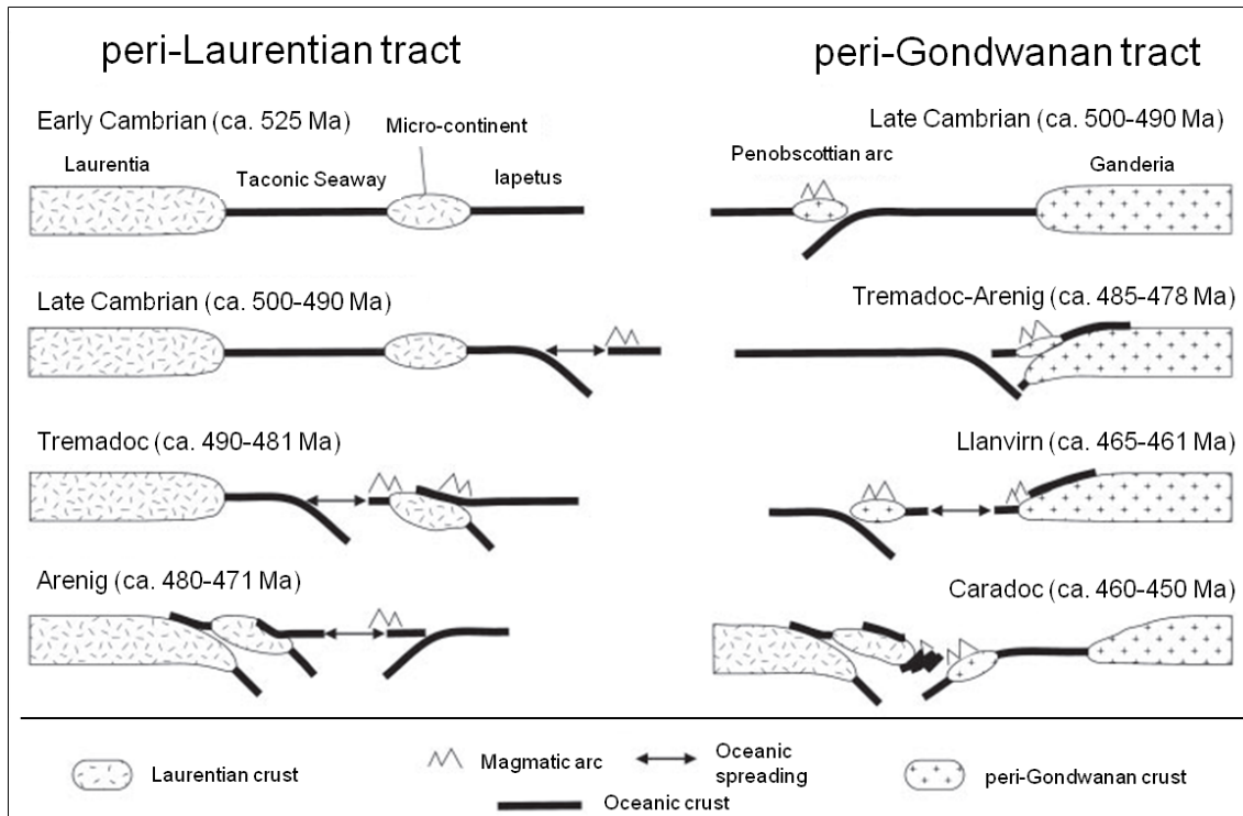
Figure 1.4: Illustration of the proposed tectonic models for the Taconian (left) and Penobscottian (right) orogenies along the Laurentian and Gondwanan margins in the Dunnage domain of the Northern Appalachians (modified after Hibbard et al. , 2007a and Murphy et al. , 2010). The details and timing depicted may not be necessarily true for the Central and Southern Appalachians but is used here to illustrate subduction processes of the Iapetus Ocean.
