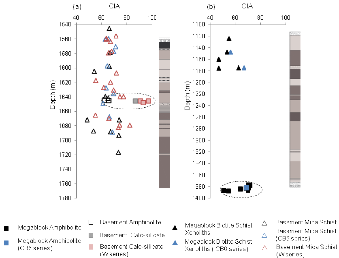
Figure 3.9: Variations in CIA with depth (m) for the metasedimentary target rock units of the (a) lower basement-derived section and (b) upper granite and amphibolite megablocks of the Eyreville-B borehole core. The geologic column, as described in Chapters 1 and 2 (after Horton et al. , 2009a), has been placed on the right side for reference purposes. Abbr.: CIA = chemical index of alteration. Dashed lines represent observed groupings.
