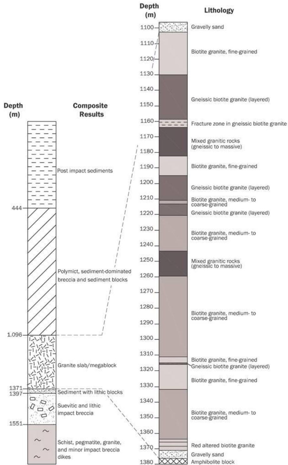
Figure 2.11: Composite stratigraphic column for the Eyreville-B borehole core (after Gohn et al. , 2006) with the detailed column for the upper megablocks section from 1095.74 m to 1389.71 m depth (after Horton et al. , 2009a).
