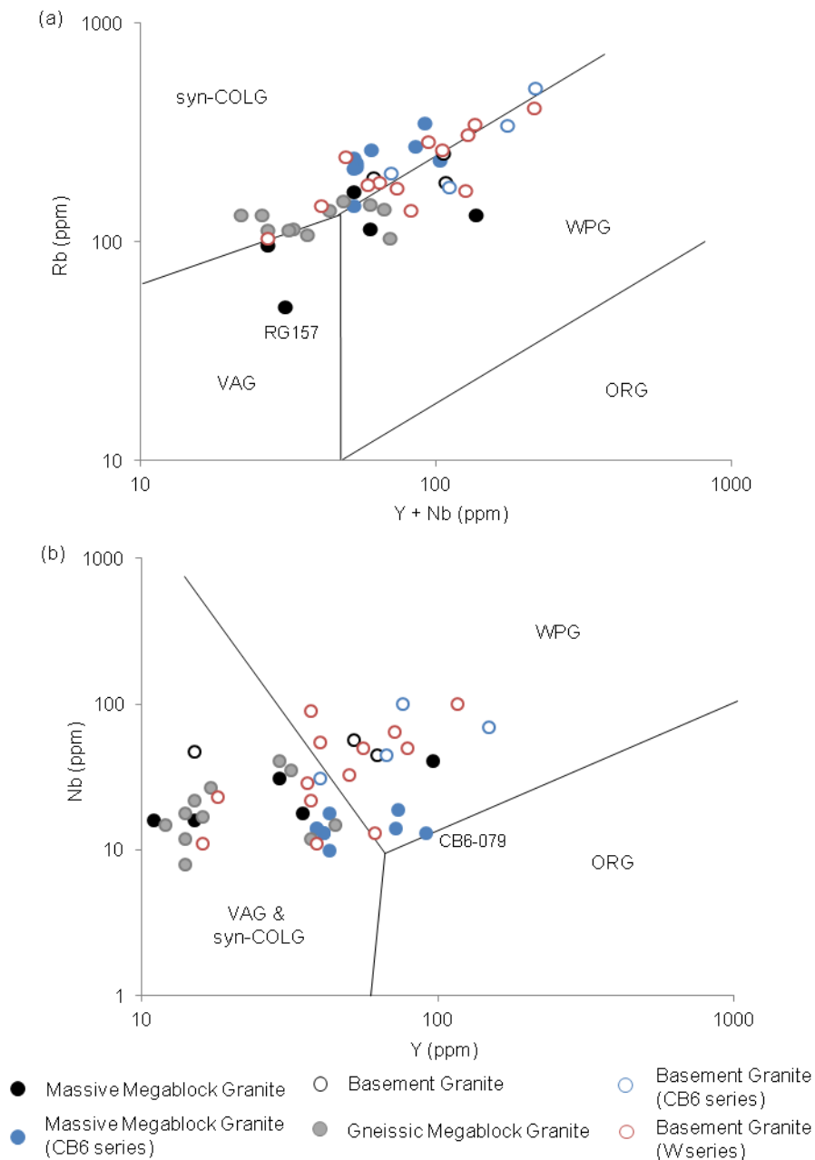
Figure 3.22: (a) Rb versus Y + Nb and (b) Nb versus Y discriminant diagrams for the granites of the Eyreville-B borehole core, indicating different tectonic setting (after Pearce et al. , 1984). All data in ppm. Abbr.: VAG = volcanic-arc granite; syn-COLG = syncollisional granite; WPG = within-plate granite; ORG = ocean-ridge granite.
