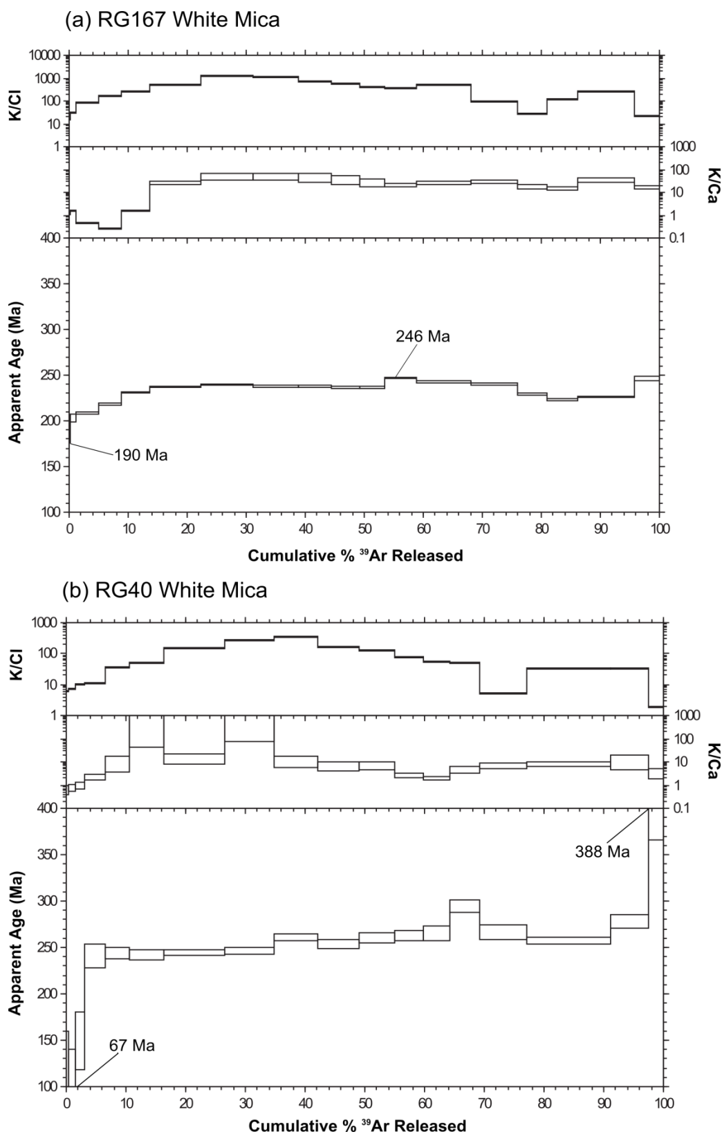
Figure 5.9: White mica age spectra, K/Cl and K/Ca diagrams for granitic samples (a) RG167 and (b) RG40. Plateau ages ( \pm 1\sigma ), age maxima and age minima are as indicated.
