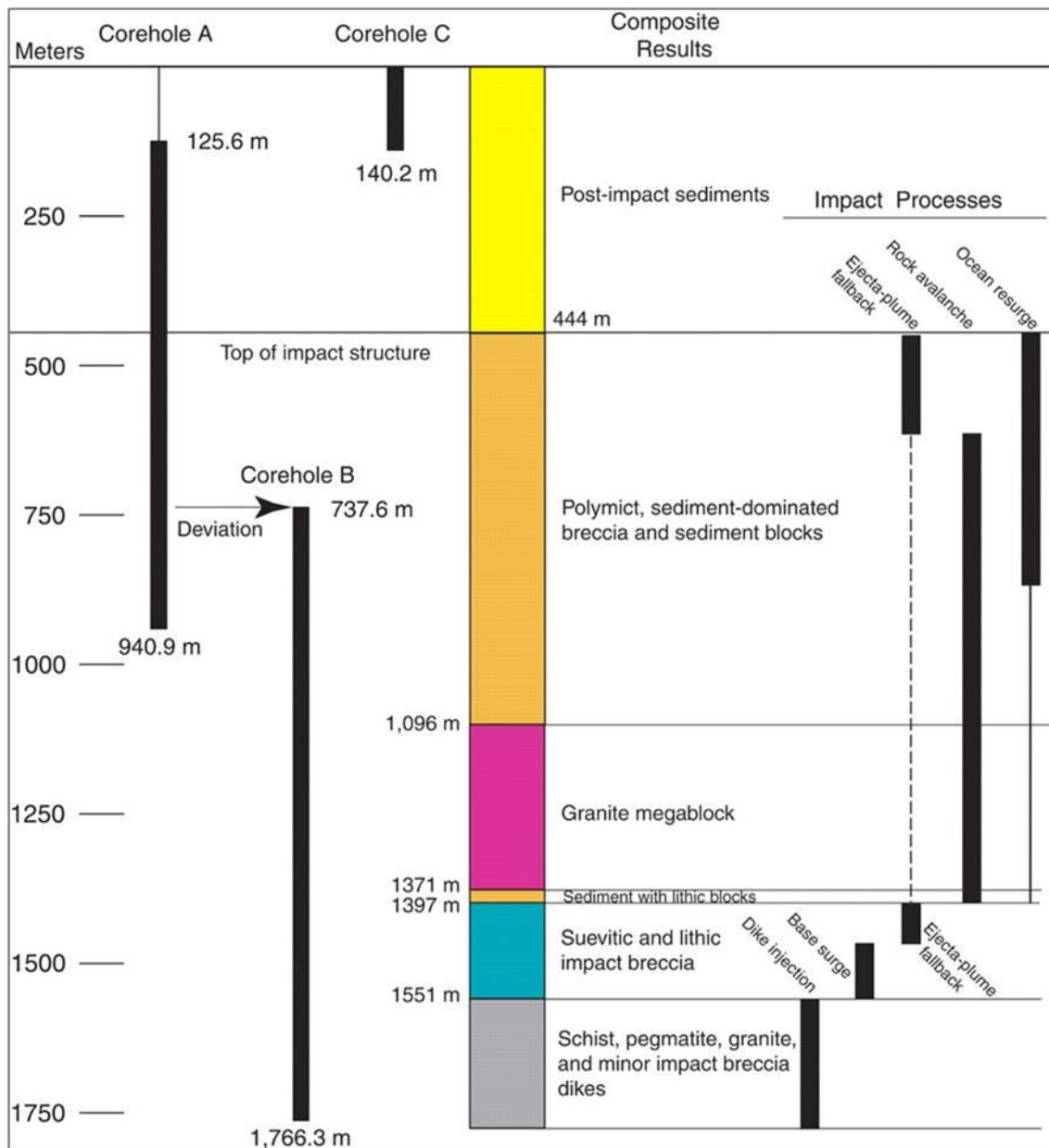
Figure 1.15: Composite geological column of the Eyreville borehole core with cored intervals A, B and C (after Gohn et al. , 2006).
