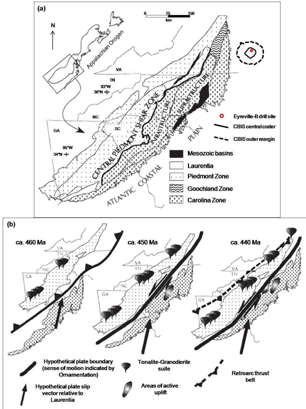
Figure 1.10: (a) Location of the suprastructural and infrastructural terranes of the Carolina Zone separated from the Piedmont Zone by the Central Piedmont shear zone within the Appalachian orogen. The approximate location of the CBIS has been included for reference purposes. (b) Depiction of the progressive accretion model for the docking of the Carolina Zone onto the Laurentian passive margin during the Salinic orogeny. Both diagrams modified after Hibbard (2000) and references therein, and Horton et al. (2005b) and references therein.
