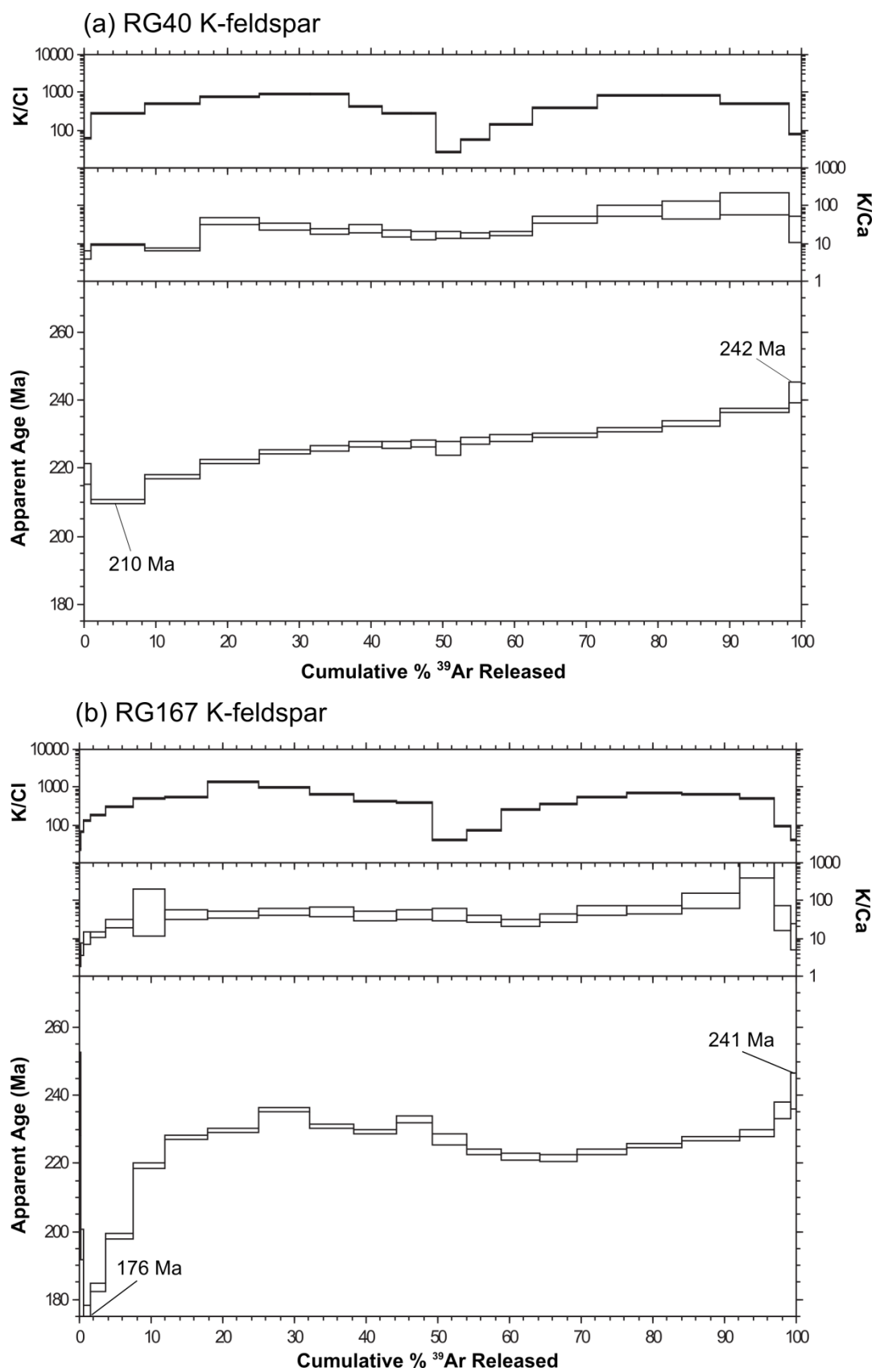
Figure 5.7: K-feldspar age spectra, K/Cl and K/Ca diagrams for samples (a) RG40 and (b) RG167. Age maxima and age minima are as indicated.
