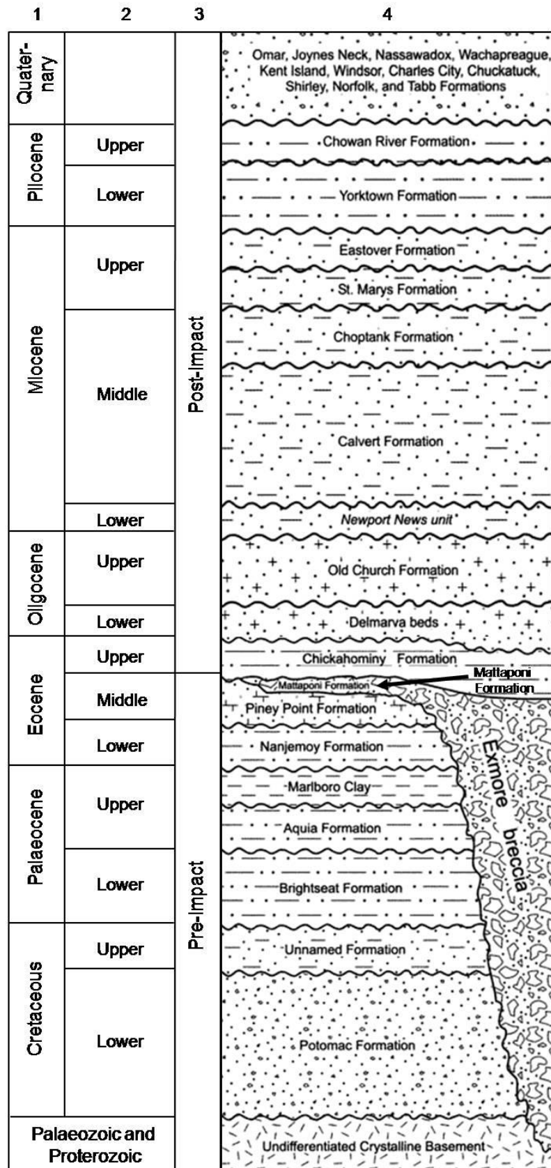
Figure 1.11: Generalised stratigraphic column for the pre-impact and post-impact sediments in southeastern Virginia in the vicinity of the CBIS (modified after Poag et al. , 2004). Undulating horizontal lines represent unconformities. Legend: 1 = Era; 2 = Epoch; 3 = Time of deformation relative to the impact; 4 = Rock units.
