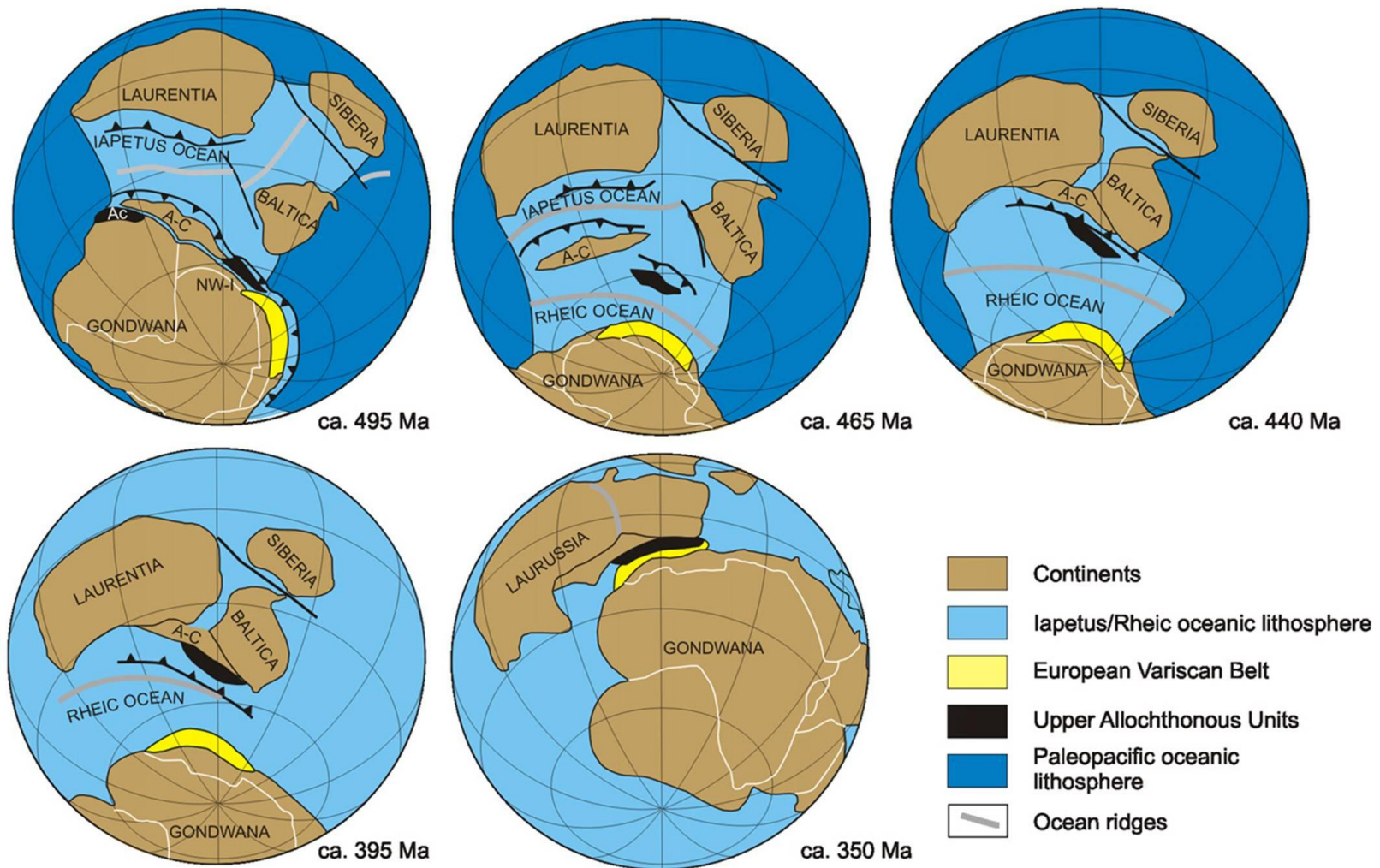
Figure 1.5: Palaeozoic reconstructions of the formation of Pangaea through the preferential subduction of the Iapetus and Rheic oceanic lithosphere (diagram modified after Murphy and Nance, 2013 and references therein). Abbr. A-C- Avalonia-Carolina.
