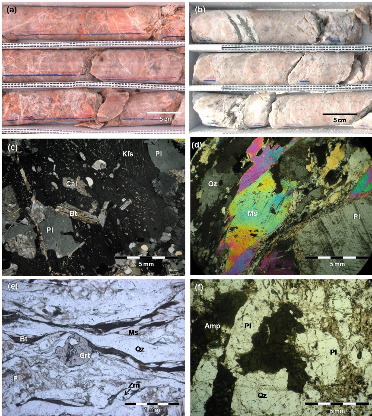
Figure 2.7: Corebox and thin section photographs of the lower basement-derived granite. Coreboxes (a) 313 and (b) 324 showing the pink/orange and white granite varieties, respectively. (c) Poikilitic Kfs grain with Bt and Pl inclusions and local replacement by Cal in sample RG40a (XPL). (d) Large Ms and Pl grains within dynamically recrystallised Qz grains in sample RG32 (XPL). (e) Fractured and locally poikilitic Grt in sample RG40a (PPL). (f) Fractured Amp grains in a Qz-Pl matrix in sample RG61 (PPL). Abbr.: Amp = amphibole; Bt = biotite; Cal = calcite; Kfs = K-feldspar; Ms = muscovite; Pl = plagioclase; PPL = plane polarised light; Qz = quartz; XPL = cross polarised light; Zrn = zircon.
