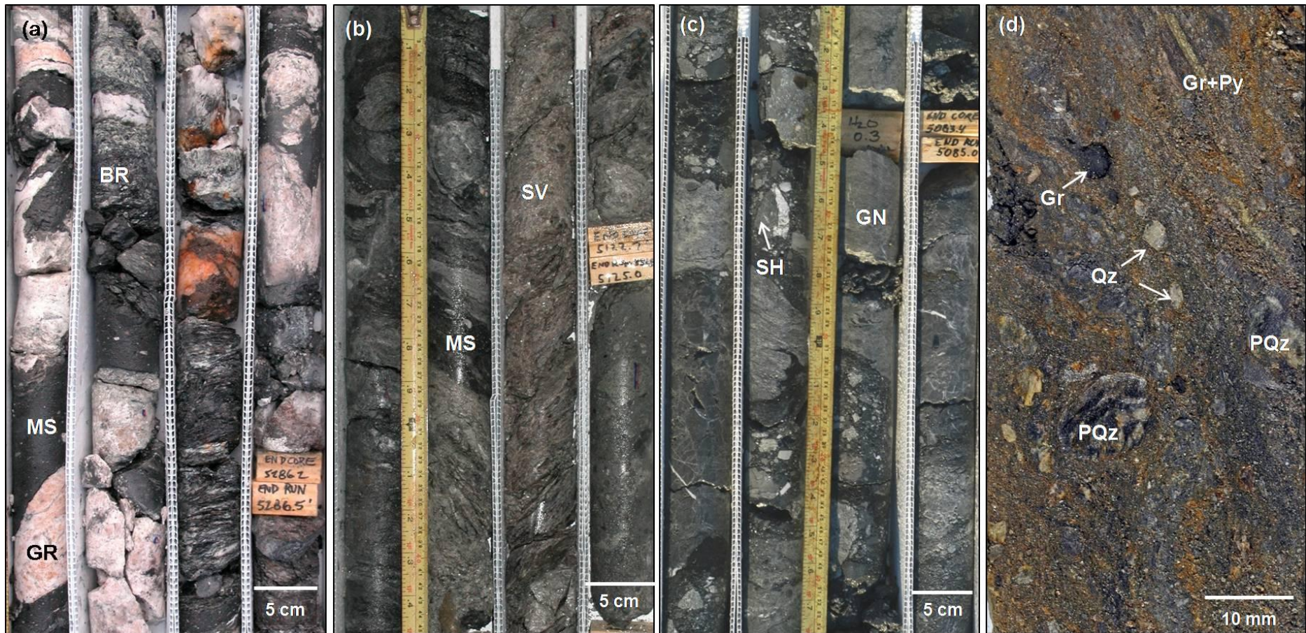
Figure 2.9: Photographs of the suevite and polymict impact breccia dykes in the lower basement-derived section. (a) Corebox 297 showing the deepest suevite dyke intercalated with MS and GR. (b) Corebox 285 showing interplay between the SV dykes and MS. (c) Corebox 282 showing the beginning of the polymict impact breccia dyke. (d) Hand specimen of sample RG71 showing the local brecciation with plucked PQz clasts. Abbr.: BR = breccia; GN = granite gneiss; GR = granite; Gr = graphite; M = melt; MS = mica schist; PQz = polycrystalline quartz; Py = pyrite; SH = shale; SV = suevite.
