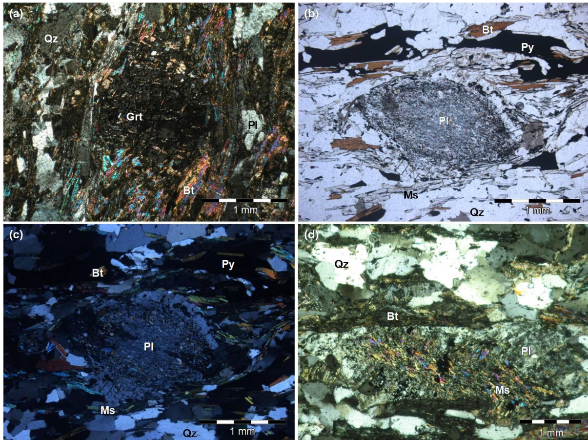
Figure 2.26: Photomicrographs of (a) sample RG53 showing a poikilitic garnet porphyroblast in the lower basement-derived mica schist with a weak internal foliation defined by biotite, rutile needles and elongated quartz inclusions (XPL), sample RG68 showing an internally zoned plagioclase porphyroblast in (b) PPL and (c) XPL views in the lower basement-derived mica schist, and (d) sample RG34 showing an internally zoned plagioclase porphyroblast with deformed muscovite inclusions in the lower basement-derived mica schist (XPL). Abbr.: Bt = biotite; Grt = garnet; Ms = muscovite; Pl = plagioclase; PPL = plane polarised light, Py = pyrite; Qz = quartz; XPL = cross polarised light.
