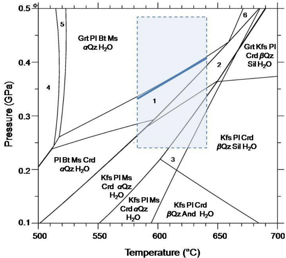
Figure 4.12: P - T phase equilibria diagrams using THERIAK-DOMINO for the basement granite sample RG40. Assemblages: 1 = Grt Pl Bt Ms Crd \alpha Qz H 2 O; 2 = Grt Kfs Pl Ms Crd \alpha Qz H 2 O; 3 = Kfs Pl Crd \alpha Qz Sil H 2 O; 4 = Pl Bt Ms Chl \alpha Qz H 2 O; 5 = Grt Pl Bt Ms Chl \alpha Qz H 2 O; 6 = Grt Kfs Pl Bt Ms \alpha Qz H 2 O. Symbols: Blue shaded area/dashed line = range of estimated peak P - T conditions; thick blue line = possible minimum P - T constraint. Abbr.: And = andalusite; Bt = biotite; Chl = chlorite; Crd = cordierite; Grt = garnet; Kfs = K-feldspar; Ms = muscovite (white mica); Pl = plagioclase; Qz = quartz; Sil = sillimanite.
