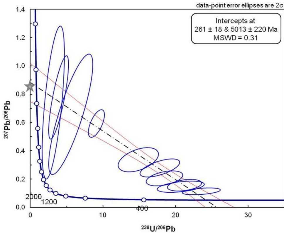
Figure 5.4: Tera-Wasserburg diagram illustrating uncorrected data for rutiles from samples RG54 and RG57. The regression line (black dashed line) intersects the y-axis ^{207}\text{Pb}/^{206}\text{Pb} ratio within error of the current estimate for the continental crust (grey star; Stacey and Kramers, 1975) Abbr.: MSWD = mean square of weighted deviates.
