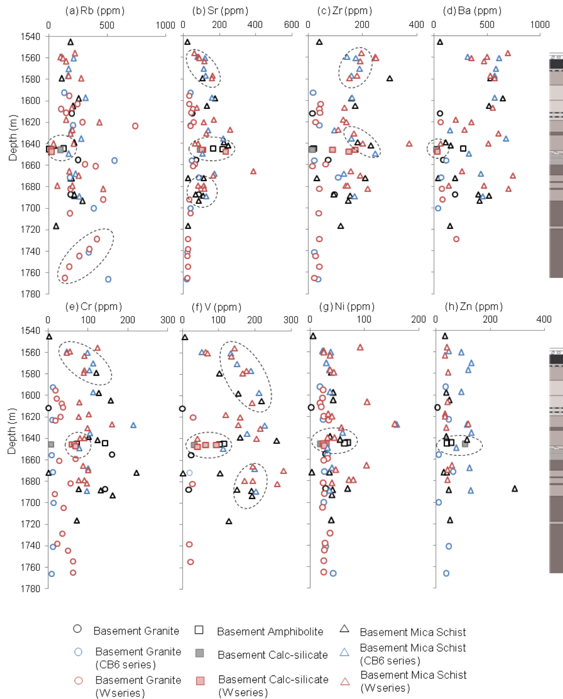
Figure 3.10: Variations in trace element concentrations (ppm) with depth (m) for the four target rock units in the lower basement-derived section of the Eyreville-B borehole core. Not all samples could be plotted for Zr, Ba, V and Zn graphs as their concentrations were below the lower limit of detection. Samples from the CB6 and W series (after Schmitt et al. , 2009) have been included to increase the data set size. The geologic column, as described in Chapters 1 and 2 (after Horton et al. , 2009a), has been placed on the right side for reference purposes. Dashed lines represent observed groupings.
