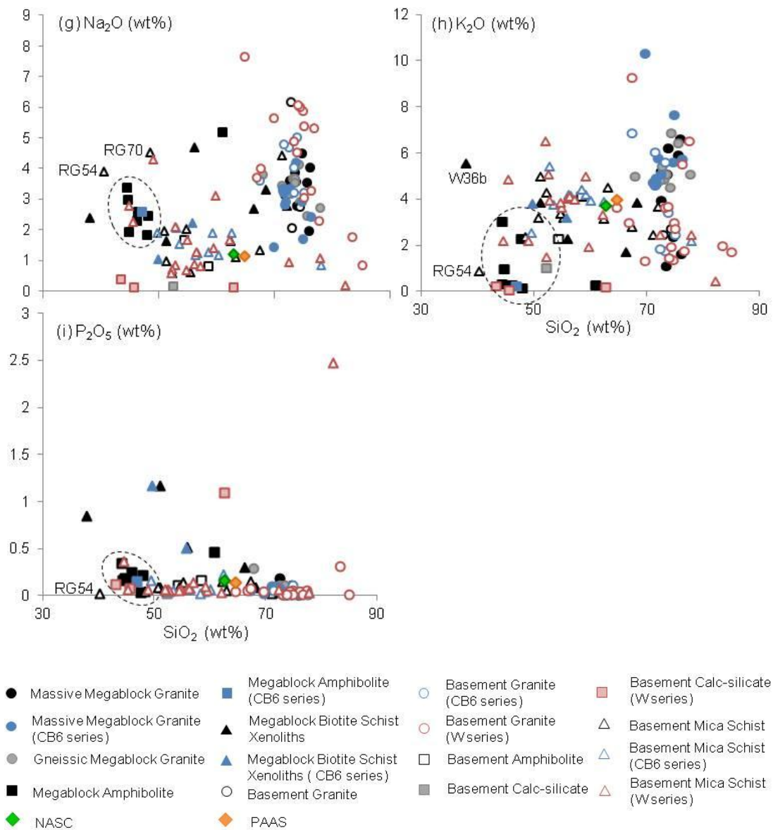
Figure 3.3 (continued): Harker diagrams showing major element oxides ( \text{TiO}_2 , \text{Al}_2\text{O}_3 , \text{Fe}_2\text{O}_3 , \text{MnO} , \text{MgO} , \text{CaO} , \text{Na}_2\text{O} , \text{K}_2\text{O} and \text{P}_2\text{O}_5 ) plotted against \text{SiO}_2 for the eight target rock units of the Eyreville-B borehole core. Abbr.: NASC = North American Shale Composite (after Gromet et al. , 1984); PAAS = Post Achaean Australian Shale (after Taylor and McLennan, 1985). Dashed lines represent observed groupings.
