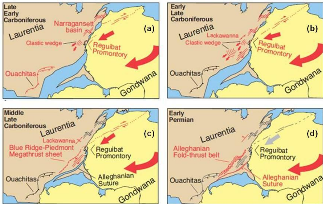
Figure 1.6: Illustrations of the oblique rotational collision between Laurentia and Gondwana as suggested by Hatcher (2002). The red lines and symbols represent active features in the interval shown in each figure (after Hatcher, 2002; Nance and Linnemann, 2008).
