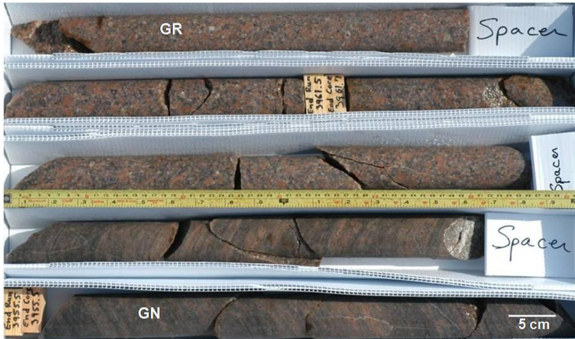
Figure 2.18: Photograph of corebox 160 showing the gneissic foliation in GN and the massive nature of GR in the upper granite megablock. Abbr.: GN = gneissic megablock granite; GR = massive megablock granite.
