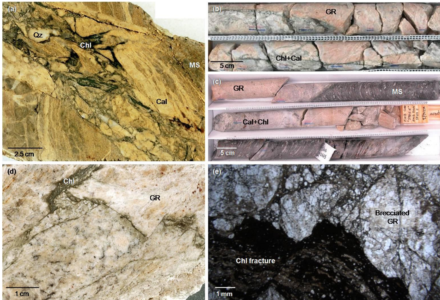
Figure 2.22: Photographs of fracturing and brecciation in the lower basement-derived section. (a) Hand specimen of MS sample RG178 showing a Chl+Cal fracture that is locally brecciated. (b) Portion of corebox 328 showing splaying Chl+Cal fractures in the GR. (c) Portion of corebox 317 showing a Cal+Chl fracture between the MS and GR. (d) Hand specimen and (e) photomicrograph (PPL) of sample RG46 showing D2 chloritic fracturing in the GR. Abbr.: Cal = calcite; Chl = chlorite; GR = granite; MS = mica schist; PPL = plane polarised light.
