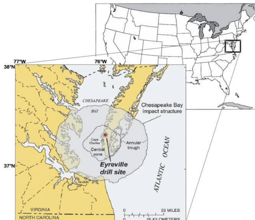
Figure 1.1: Locality map of the CBIS and the ICDP-USGS Eyreville drill site (after Gohn et al. , 2006).
