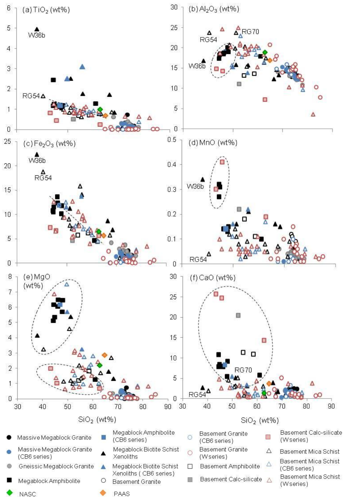
Figure 3.3: Harker diagrams showing major element oxides ( \text{TiO}_2 , \text{Al}_2\text{O}_3 , \text{Fe}_2\text{O}_3 , \text{MnO} , \text{MgO} , \text{CaO} , \text{Na}_2\text{O} , \text{K}_2\text{O} and \text{P}_2\text{O}_5 ) plotted against \text{SiO}_2 for the eight target rock units of the Eyreville-B borehole core. Abbr.: NASC = North American Shale Composite (after Gromet et al. , 1984); PAAS = Post Achaean Australian Shale (after Taylor and McLennan, 1985). Dashed lines represent observed groupings.
