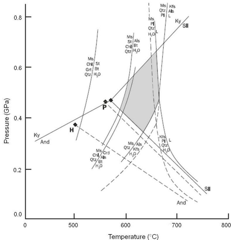
Figure 4.9: P-T diagram indicating the relative positions of reactions occurring within the lower basement-derived mica schists within the CKNASH system (modified after Pattison and Tracy, 1991) with the Als phase boundaries (after Holland and Powell, 1998) superimposed. Dashed lines represent the fluid-present Ms melting curves within the CKNASH system (Thompson and Tracy, 1990). Solid lines represent the displaced Ms melting curves where the fluid is in equilibrium with Gr at X(\text{H}_2\text{O}) = 0.8 (Ashworth and Tyler, 1983). Grey area represents the probable P-T conditions, based on mineral stability, under which the basement mica schists formed. P (after Pattison, 1992) and H (after Holdaway, 1971) are triple points that delimit the possible range in P-T space for the And-Sil transition as discussed in Pattison and Tracy (1991). Abbr.: Als = aluminosilicate; And = andalusite; Bt = biotite; Chl = chlorite; Crd = cordierite; Gr = graphite; Grt = garnet; Kfs = K-feldspar; Ky = kyanite; L = liquid; Ms = muscovite; Pl = plagioclase; Qtz = quartz; Sil = sillimanite; St = staurolite.
