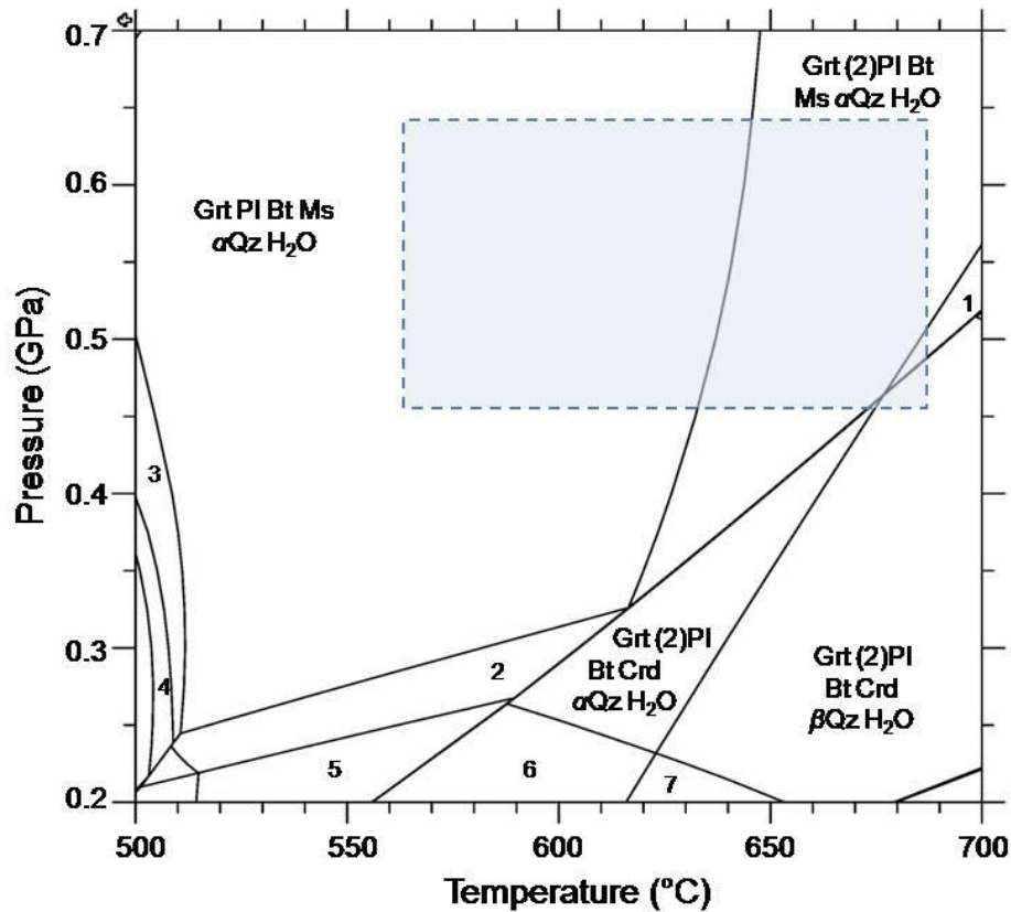
Figure 4.11: P-T phase equilibria diagrams using THERIAK-DOMINO for the basement mica schist sample RG53. Assemblages: 1 = Grt (2)PI Bt Ms \beta Qz H 2 O; 2 = Grt PI Bt Ms Crd \alpha Qz H 2 O; 3 = Grt PI Bt Ms Chl \alpha Qz H 2 O; 4 = Grt (2)PI Bt Ms Chl \alpha Qz H 2 O; 5 = PI Bt Ms Crd \alpha Qz H 2 O; 6 = (2)PI Bt Crd \alpha Qz H 2 O; 7 = (2)PI Bt Crd \beta Qz H 2 O. Symbols: Blue shaded area/dashed line = range of estimated peak P-T conditions. Abbr.: Bt = biotite; Chl = chlorite; Crd = cordierite; Grt = garnet; Ms = muscovite (white mica); PI = plagioclase; (2)PI = albite and anorthite; Qz = quartz.
