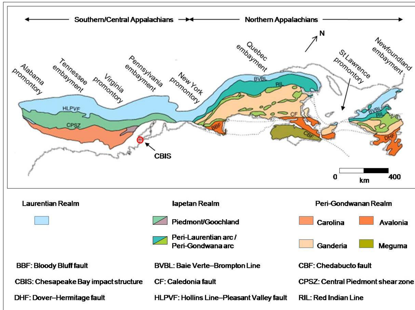
Figure 1.2: Simplified tectonic map of the Appalachian orogen showing the exposed Northern and Central/Southern Appalachians divisions as well as pre-Silurian lithotectonic divisions with respect to the current North American eastern coastline (diagram modified after Hibbard et al. , 2007a and Pollock, 2008). The location of the CBIS has been included for reference purposes.
