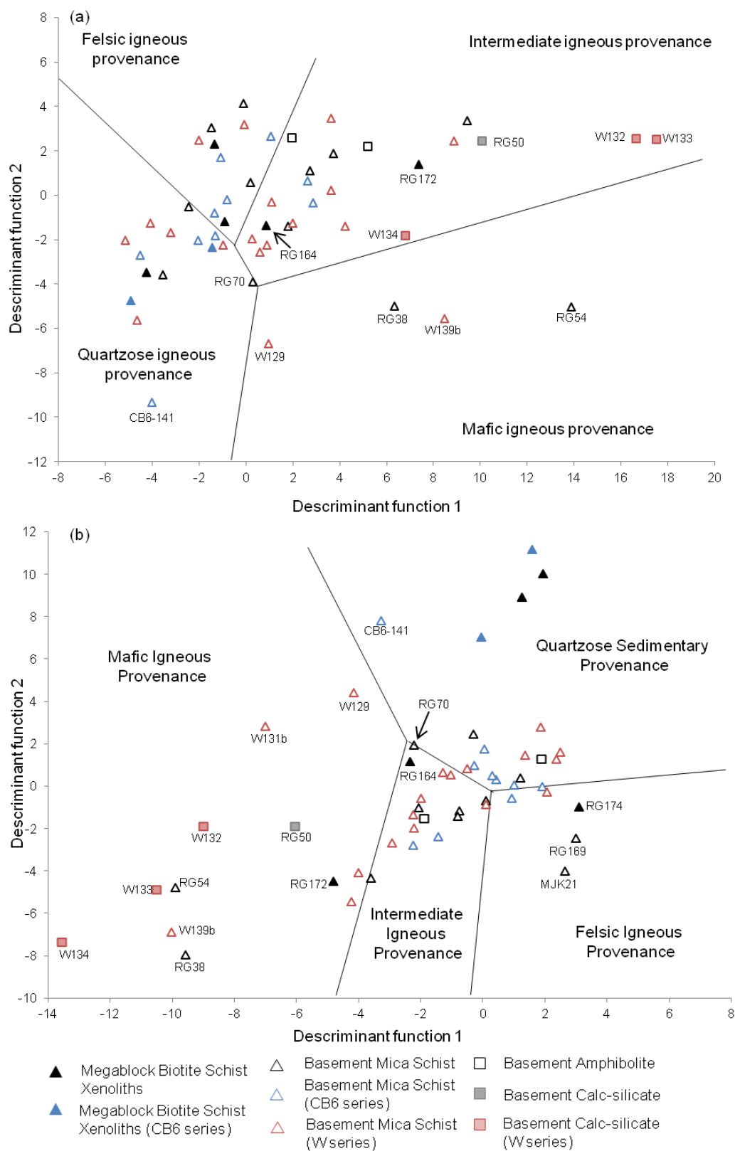
Figure 3.17: Discriminant diagrams showing provenance signatures for sandstone-mudstone suites using major elements based on (a) raw oxides and (b) oxide ratios for the megablock and basement mica schists and basement amphibolite and calc-silicate rock units of the Eyreville-B borehole core (after Roser and Korsch, 1988). All data in wt%.
