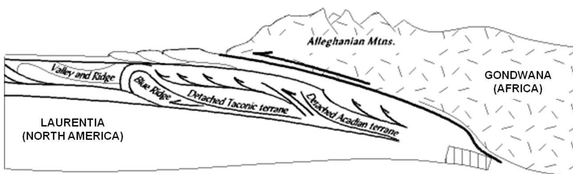
Figure 1.7: Schematic cross-section of the Alleghanian orogeny (modified after Fichter and Baedke, 1999) showing Gondwana over-riding Laurentia to the west through décollement tectonics.
