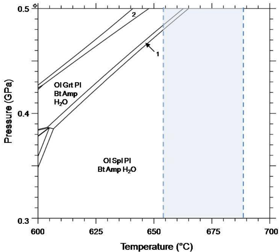
Figure 4.13: P-T phase equilibria diagrams using THERIAK-DOMINO for the megablock amphibolite sample W51. Assemblages: 1 = Ol Spl Grt Pl Bt Amp H 2 O; 2 = Ol Grt Pl Bt Omp Amp H 2 O. Symbols: Blue shaded area/dashed line = range of estimated peak T for P range of 0.3-0.5 GPa. Abbr.: Amp = amphibole; Bt = biotite; Grt = garnet; Ol = olivine; Omp = omphacite; Pl = plagioclase; Spl = spinel; Qz = quartz.
