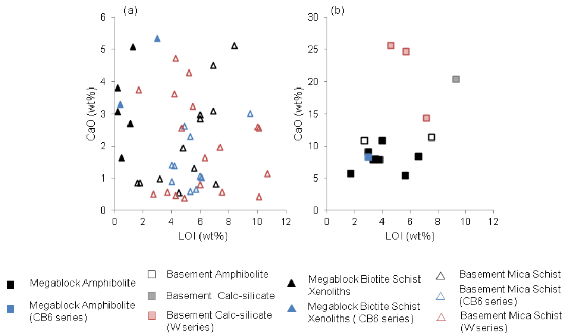
Figure 3.8: Variations in LOI with CaO concentrations for (a) the mica schists and (b) the amphibolites and calc-silicate rock units of the Eyreville-B borehole core. All data in wt%.
