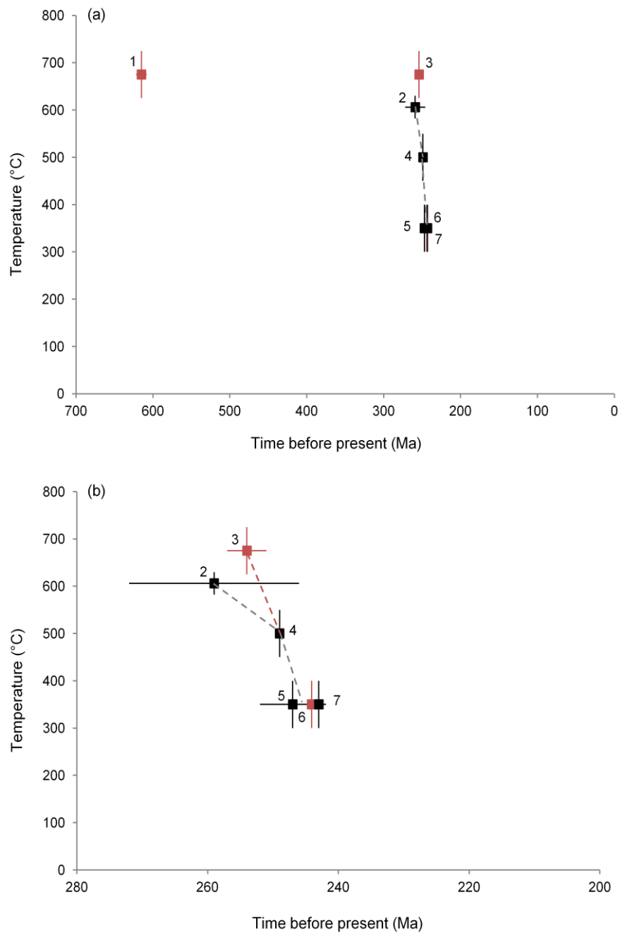
Figure 5.11: (a) Thermal-decay curve showing complete crystallisation and cooling history as recorded in the target rocks of the Eyreville-B borehole core. (b) Magnified view of the cooling history from 280 to 200 Ma. Refer to the explanation of numbered labels in text. Granite crystallisation temperature is 675 \pm 50^\circ\text{C} (after Kerrick, 1972). Closure temperatures: rutile = 606 \pm 18^\circ\text{C} (Chapter 4, Section 4.3.4.1); amphibole = 500 \pm 50^\circ\text{C} (Harrison, 1981); muscovite/white mica = 350 \pm 50^\circ\text{C} (Hames and Bowring, 1994). Symbols: red squares and lines = data points with errors derived from Horton et al. (2009b); black squares and lines = data points with errors from this study; grey dashed lines = projected cooling history; red dashed line = alternative cooling history.
