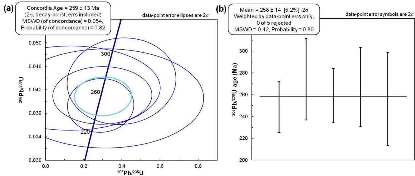
Figure 5.3: (a) Concordia plot and (b) ^{206}\text{Pb}/^{238}\text{U} ages for LA-ICP-MS data of rutiles from samples RG54 and RG57. Errors, MSWD (mean square of weighted deviates) and degree of concordance were calculated using Isoplot (after Ludwig, 2003; Zack et al. , 2011).
