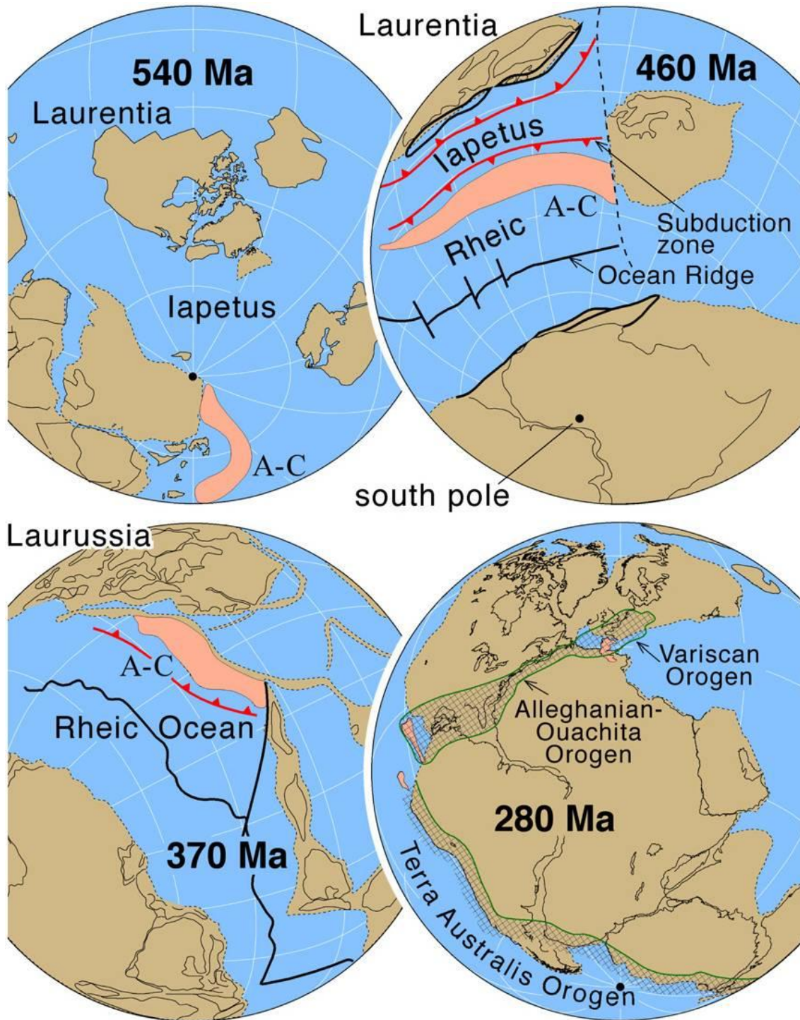
Figure 1.3: Reconstructions of Pangaea during the Palaeozoic, illustrating the closing of the Iapetus and Rheic oceans between Gondwana and Laurentia (diagram modified Stampfli and Borel, 2002, and Murphy et al. , 2010). Abbr. A-C = Avalonia-Carolina.
