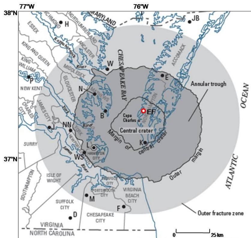
Figure 1.13: Regional map of the CBIS with the locations of borehole cores in southeastern Virginia, including the ICDP-USGS Eyreville borehole core (after Horton et al. , 2005a, 2005b; Gohn et al. , 2008, 2009). Symbols: B = Bayside; D = Dismal Swamp; E = Exmore; EF = ICDP-USGS Eyreville; F = Fentress; H = Haynesville; J = Jamestown; JB = Jenkins Bridge; K = Kiptopeke; L = USGS-NASA Langley; M = MW4-1; N = North; NN = Newport News Park 2; W = Windmill Point; WS = Watkins School.
