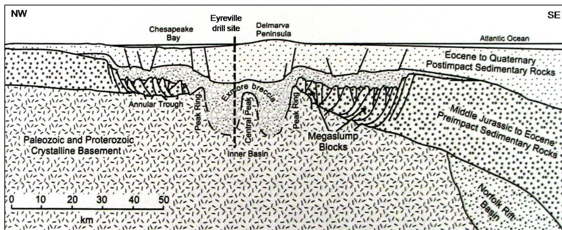
Figure 1.12: Geological cross-section of the CBIS from NW to SE showing the relative locations of the central zone (inner basin, central peak, peak ring), the annular trough and the ICDP-USGS Eyreville drill site (modified after Poag et al. , 1999, 2004; Gohn et al. , 2008, 2009).
