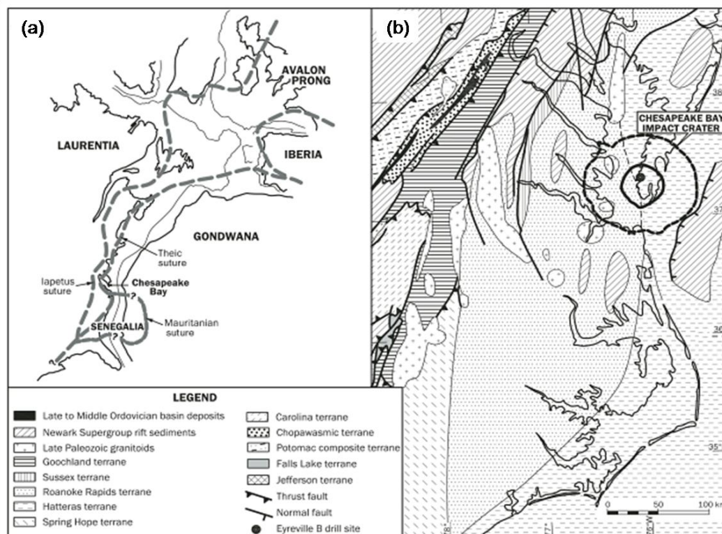
Figure 6.1: (a) Plate reconstruction of the Palaeozoic sutures between Laurentia and Gondwana showing the location of the CBIS (after Lefort, 1988; Lefort and Max, 1991). (b) Tectonostratigraphic terrane map of the Central Appalachians showing the location of the CBIS (after Horton et al. , 2005b).
