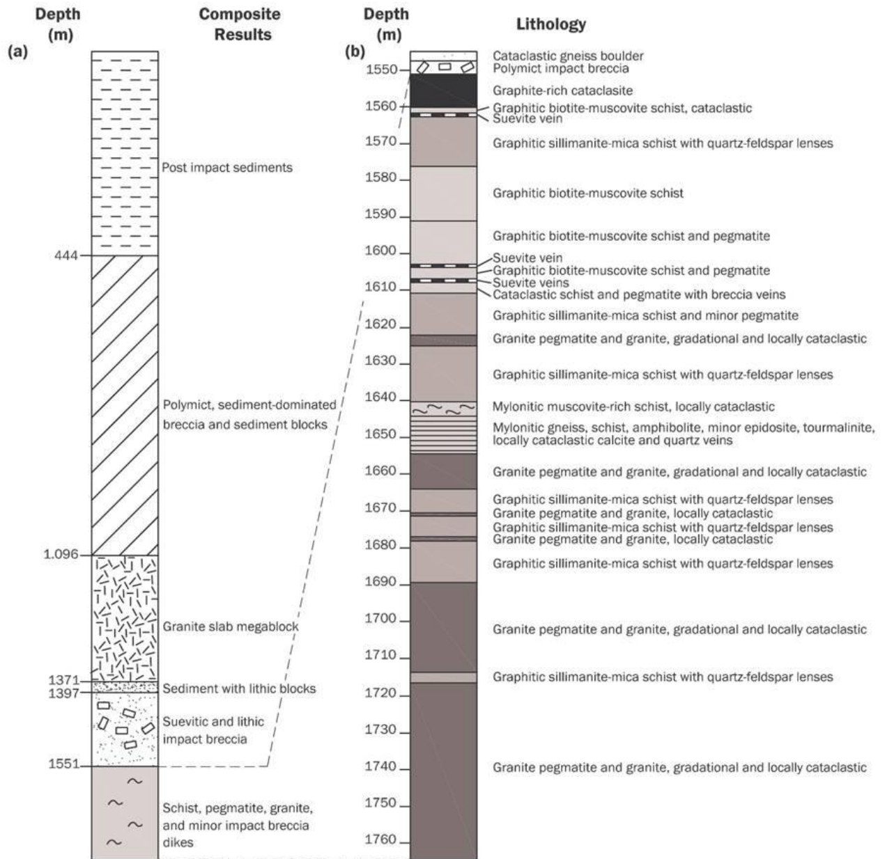
Figure 2.1: (a) Composite stratigraphic column for Eyreville-B borehole core (after Gohn et al. , 2006) with (b) a detailed column for the lower basement-derived section between 1551 m and 1766 m depth (after Horton et al. , 2009a).
