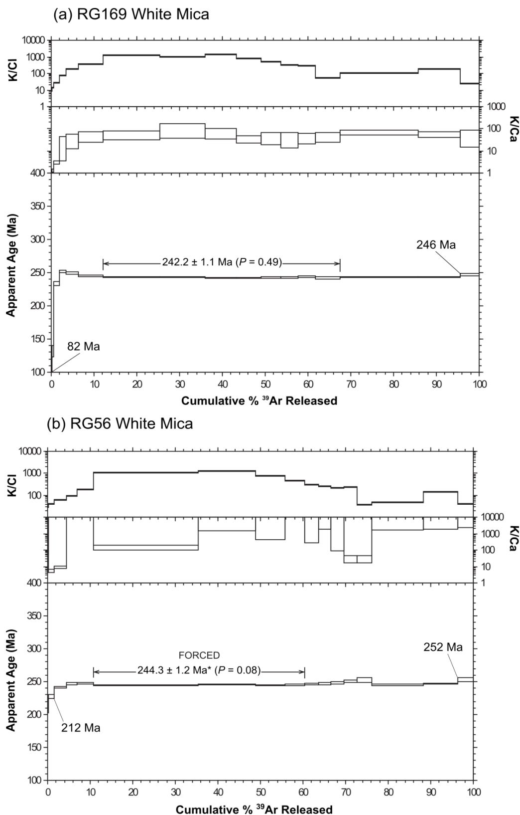
Figure 5.8: White mica age spectra, K/Cl and K/Ca diagrams for mica schist samples (a) RG169, (b) RG56, (c) MJK18 and (d) MJK21. Plateau ages ( \pm 1\sigma ), age maxima and age minima are as indicated. Symbols: * = forced plateau age; P = probability.
