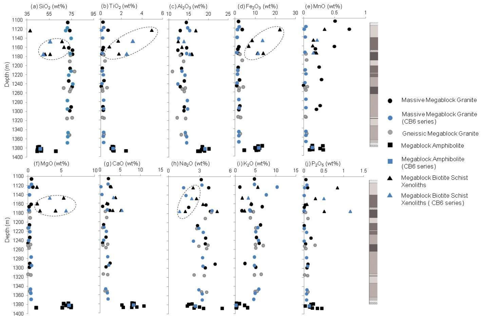
Figure 3.2: Variations in major element concentrations (wt%) with depth (m) for the four target rock units in the upper granite and amphibolite megablocks of the Eyreville-B borehole core. Samples from the CB6 series (after Schmitt et al. , 2009) have been included to increase the data set size. The geologic column, as described in Chapters 1 and 2 (after Horton et al. , 2009a), has been placed on the right side for reference purposes. Dashed lines represent observed groupings.
