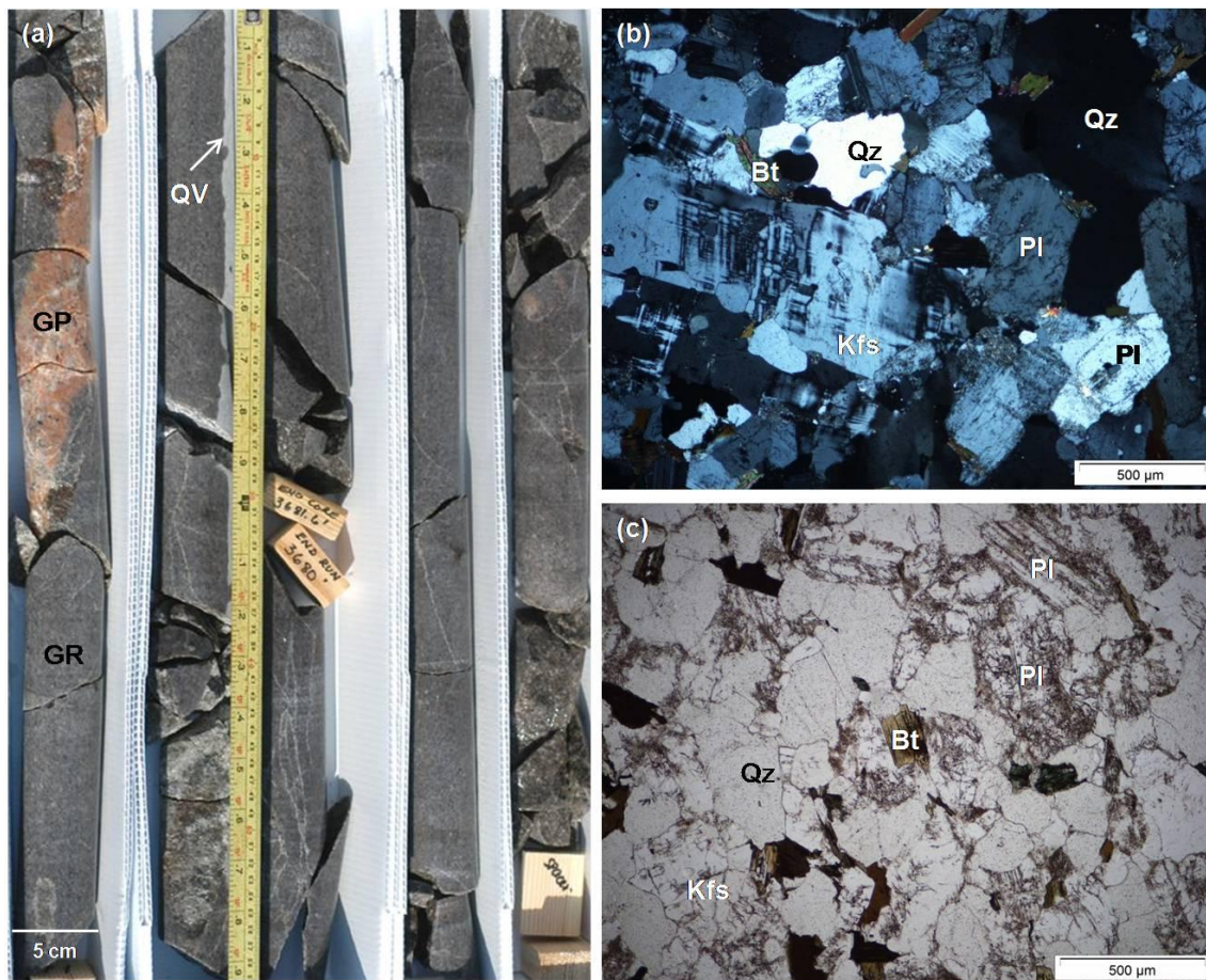
Figure 2.14: Photographs of the massive granite of the upper megablock. (a) Corebox 142 showing the medium-grained nature of the massive megablock granite with an intruding GP and QV. (b) Photomicrograph of sample W46 showing the poikilitic Kfs phenocrysts exhibiting microcline twinning and myrmekitic texture (XPL). (c) Photomicrograph of sample W37 showing alteration in Kfs and PI (PPL). Abbr.: Bt = biotite; GP = granite pegmatite; GR = massive granite; Kfs = K-feldspar; PI = plagioclase; PPL = plane polarised light; Qz = quartz; QV = quartz vein; XPL = cross polarised light.
