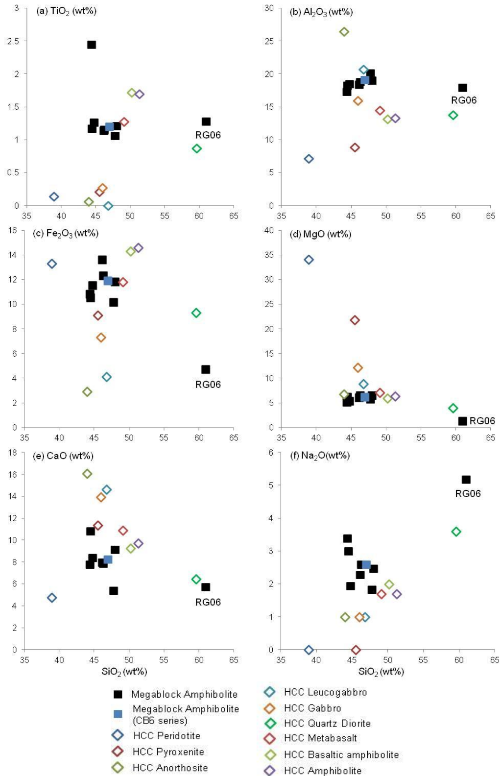
Figure 6.3: Harker diagrams showing selected major element oxides ( \text{TiO}_2 , \text{Al}_2\text{O}_3 , \text{Fe}_2\text{O}_3 , \text{MgO} , \text{CaO} and \text{Na}_2\text{O} ) plotted against \text{SiO}_2 for the megablock amphibolite of the Eyreville-B borehole core and the mafic-ultramafic rocks of the Halifax County Complex (data from Kite and Stoddard, 1984). Abbr.: HCC = Halifax County Complex.
