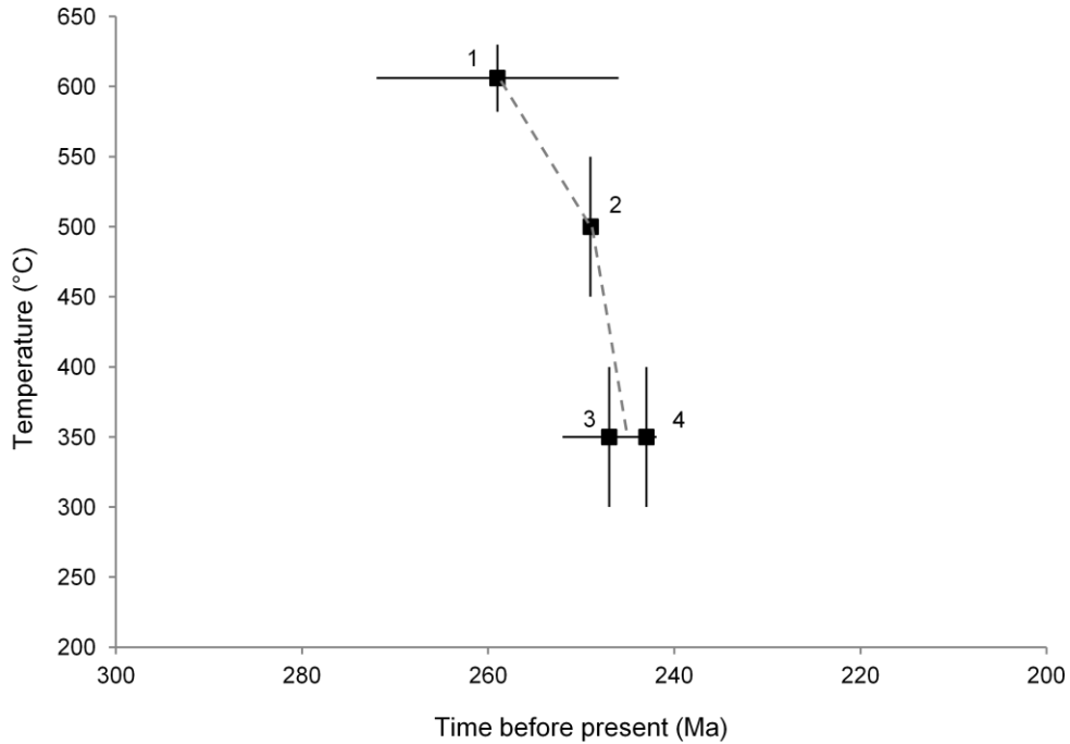
Figure 5.10: Thermal decay curve showing the cooling path for the target rocks of Eyreville-B borehole core based on this study's results. Refer to the explanation of numbered labels in text. Closure temperatures used: rutile = 606 \pm 18^\circ\text{C} (Chapter 4, Section 4.3.4.1); amphibole = 500 \pm 50^\circ\text{C} (Harrison, 1981); muscovite/white mica = 350 \pm 50^\circ\text{C} (Hames and Bowring, 1994). Symbols: black squares and lines = data points with errors from this study; grey dashed line = projected cooling history.
