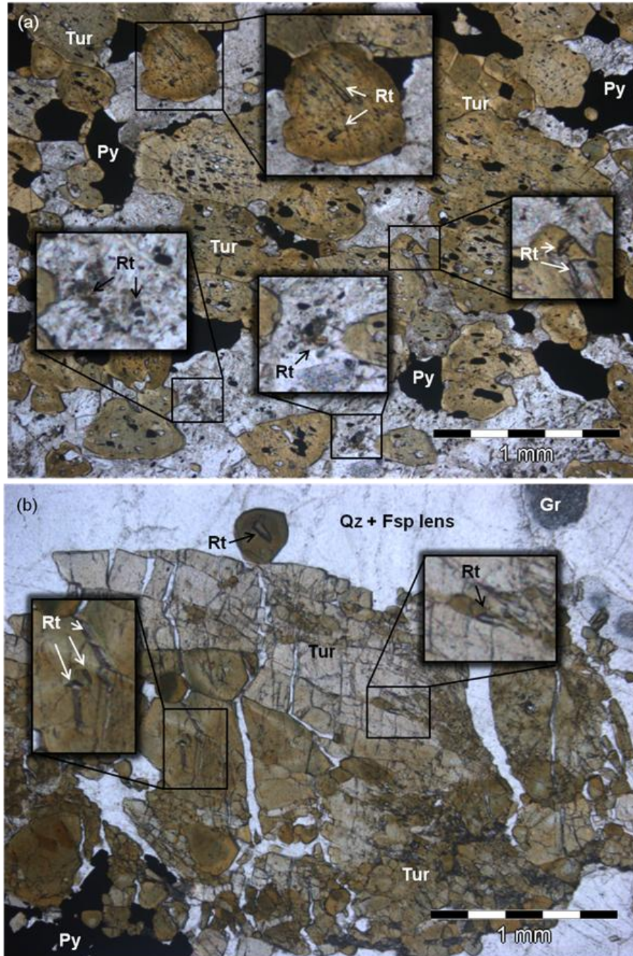
Figure 5.1: Photomicrograph of (a) RG54 (tourmalinite) and (b) RG57 (tourmaline-rich schist) showing the rutile-bearing mineral assemblages. Abbr. (after Siivola and Schmid, 2007; Whitney and Evans, 2010): Fsp – feldspar; Gr – graphite; Py – pyrite; Qz – quartz; Rt – rutile; Tur – tourmaline.
