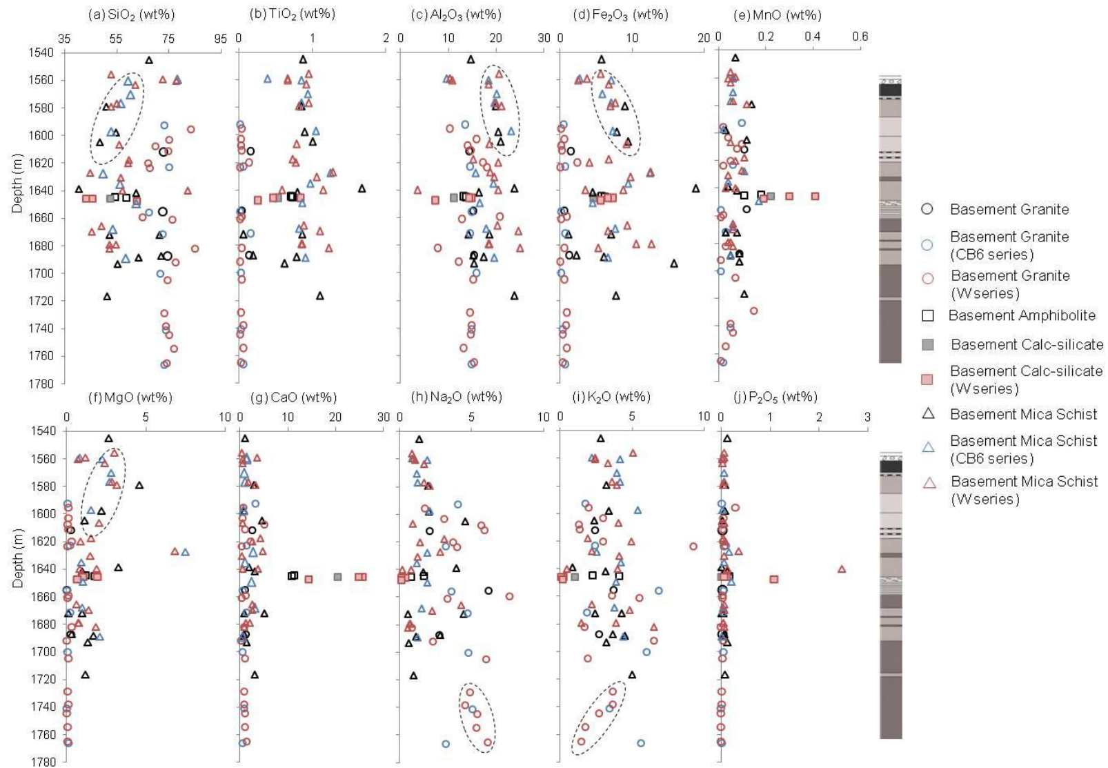
Figure 3.1: Variations in major element concentrations (wt%) with depth (m) for the four target rock units in the lower basement-derived section of the Eyreville-B borehole core. Samples from the CB6 and W series (after Schmitt et al. , 2009) have been included to increase the data set size. The geologic column, as described in Chapters 1 and 2 (after Horton et al. , 2009a), has been placed on the right side for reference purposes. Dashed lines represent observed groupings.
