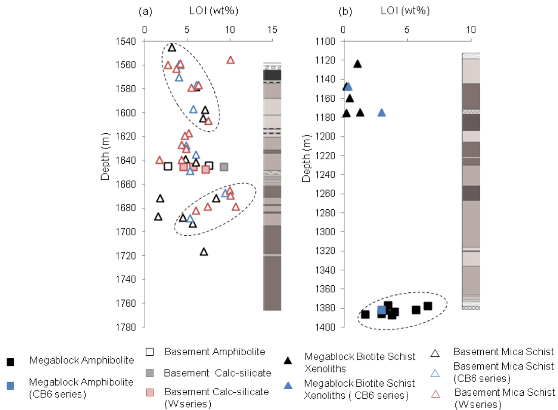
Figure 3.7: Variations in LOI (wt%) with depth (m) for the metasedimentary target rock units of the (a) lower basement-derived section and (b) upper granite and amphibolite megablocks of the Eyreville-B borehole core. The geologic column, as described in Chapters 1 and 2 (after Horton et al. , 2009a), has been placed on the right side for reference purposes. Dashed lines represent observed groupings.
