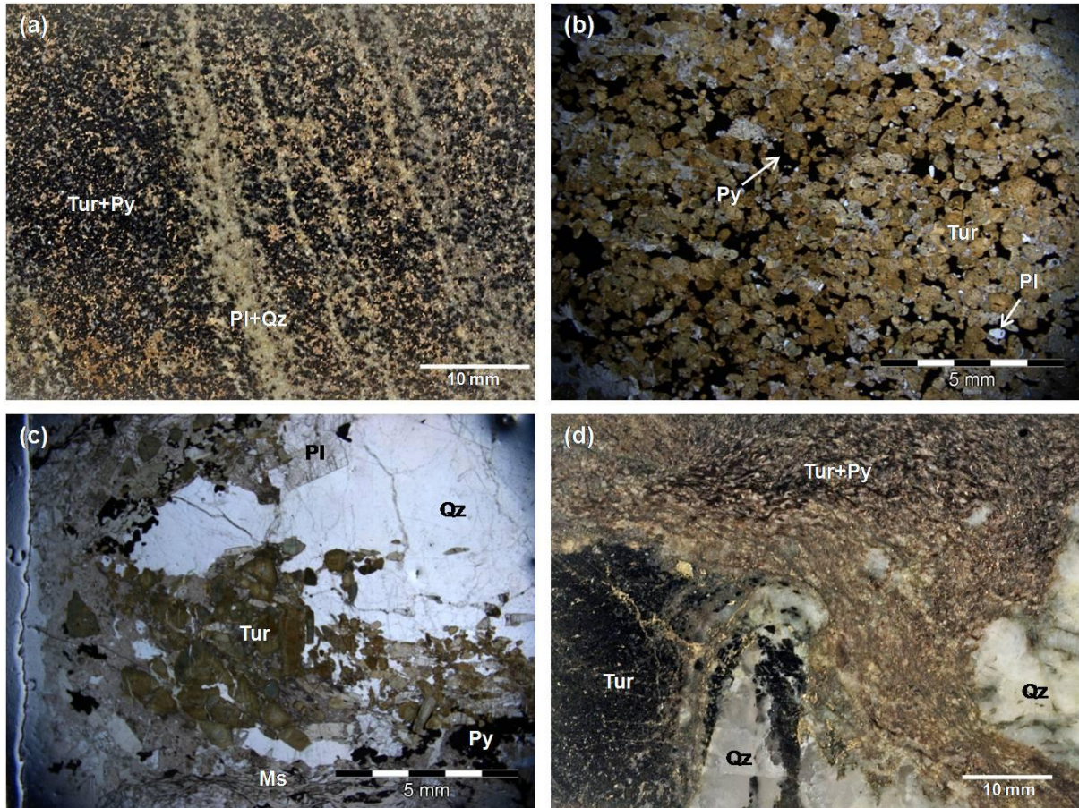
Figure 2.6: (a) Hand specimen and (b) thin section (PPL) photographs of sample RG54 showing the abundance and fine-grained nature of the lower basement-derived tourmalinite. (c) Thin section (PPL) and (d) hand specimen photographs of sample RG57 showing the coarse grain size of Tur-rich layers within the lower basement-derived mica schist. Abbr.: Ms = muscovite; Pl = plagioclase; PPL = plane polarised light; Py = pyrite; Qz = quartz; Tur = tourmaline.
