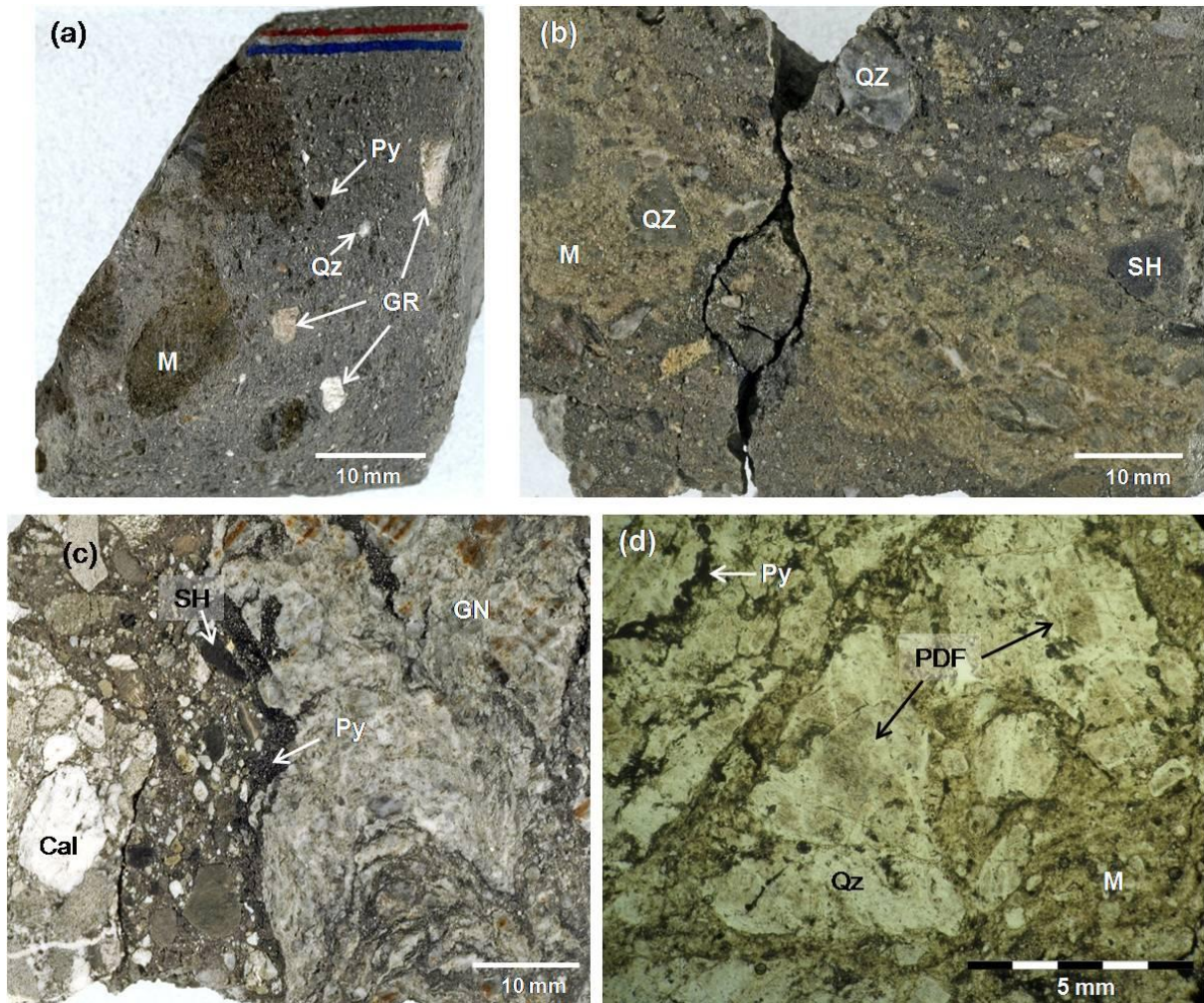
Figure 2.10: Photographs of the suevite and polymict impact breccia dykes in the lower basement-derived section. (a) Hand specimen of sample RG62 showing the variation in clast size and type within a matrix-support suevite. (b) Hand specimen of sample RG73 showing a clast-supported suevite with a melt vein and quartzite clasts. (c) Hand specimen of sample RG77 showing the large variation in grain size and clast type in polymict impact breccia. (d) Photomicrograph of sample RG77 showing fractured and toasted quartz with PDFs within an altered matrix (PPL). Abbr.: Cal = calcite; GN = granite gneiss; GR = granite; M = melt; PDF = plane deformation features; PPL = plane polarised light; Py = pyrite; QZ = quartzite; Qz = quartz; SH = shale.
