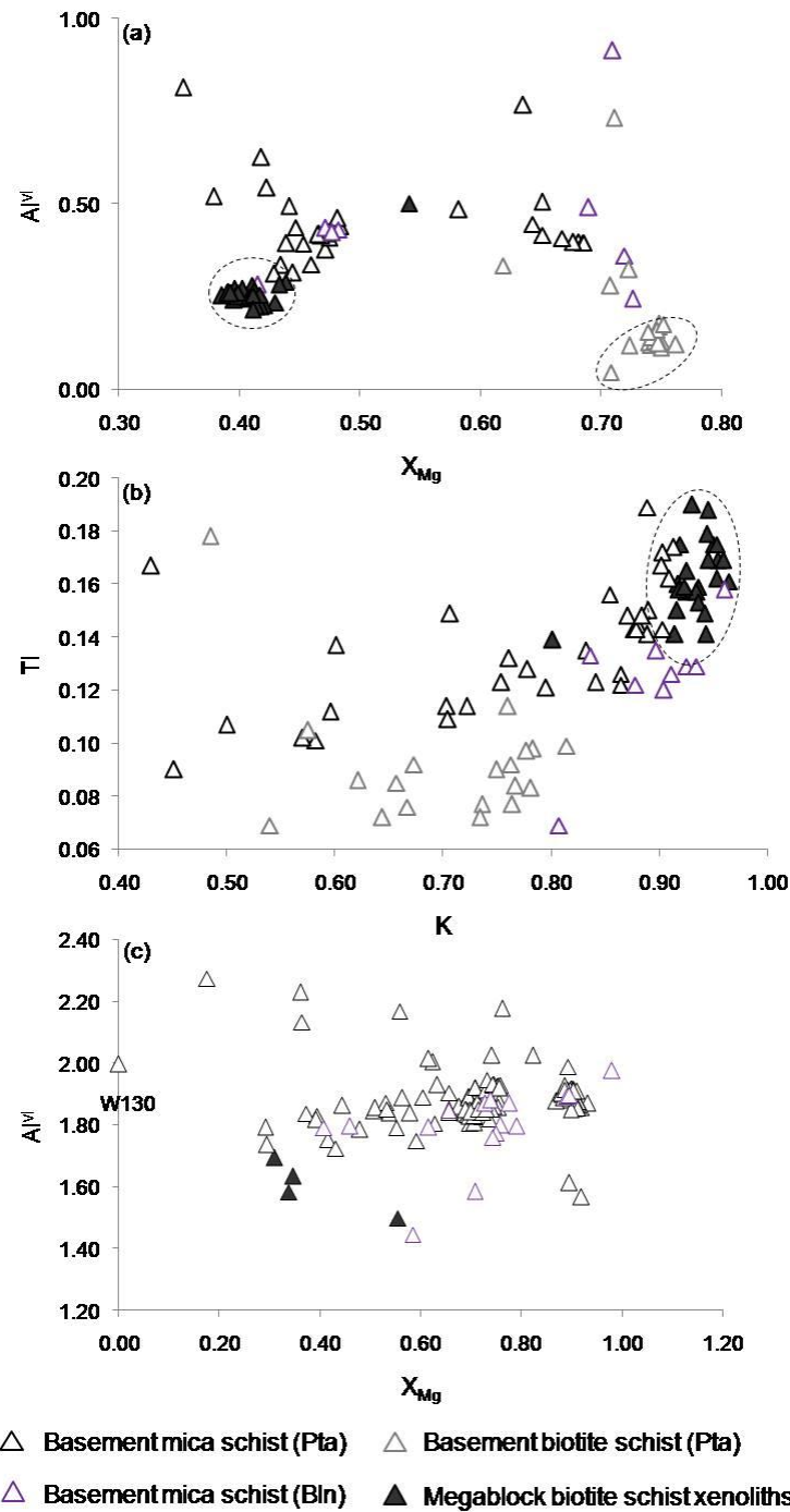
Figure 4.2: (a) X_{Mg} vs. Al^{vi} and (b) K vs. Ti abundances in Bt (apfu for 11 oxygens) and (c) X_{Mg} vs. Al^{vi} abundances in Ms (apfu for 11 oxygens) for the lower basement-derived mica schist (Bt n = 41 ; Ms n = 130 ) and biotite schist (Bt n = 19 ) and upper megablock biotite schist xenoliths (Bt n = 25 ; Ms n = 4 ). Dashed lines represent observed groupings. Abbr.: Bln = EMP analyses obtained in Berlin; Bt = biotite; Ms = muscovite (white mica); n = number of analyses; Pta = EMP analyses obtained in Pretoria.
