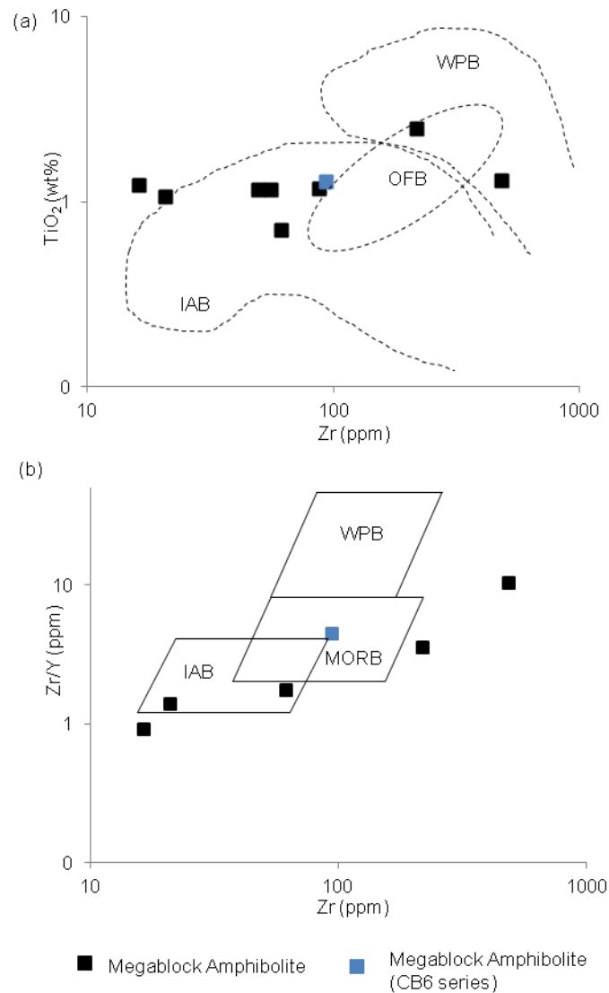
Figure 3.21: Discriminant diagrams showing the tectonic setting for the amphibolite rock units of the Eyreville-B borehole core. (a) \text{TiO}_2 versus Zr diagram (after Pearce et al. , 1981), and (b) Zr/Y versus Zr diagram (after Pearce and Norry, 1979). Abbr.: IAB = island arc basalt; OFB = ocean floor basalt; WPB = within-plate basalt; MORB = mid-oceanic ridge basalt.
