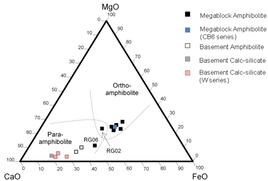
Figure 3.18. Ternary diagram indicating CaO-MgO-FeO abundances for the discrimination between ortho- and para-amphibolites for the megablock and basement amphibolites and calc-silicate (after Walker et al. , 1960) of the Eyreville-B borehole core. FeO was calculated using the CIPW norm.
