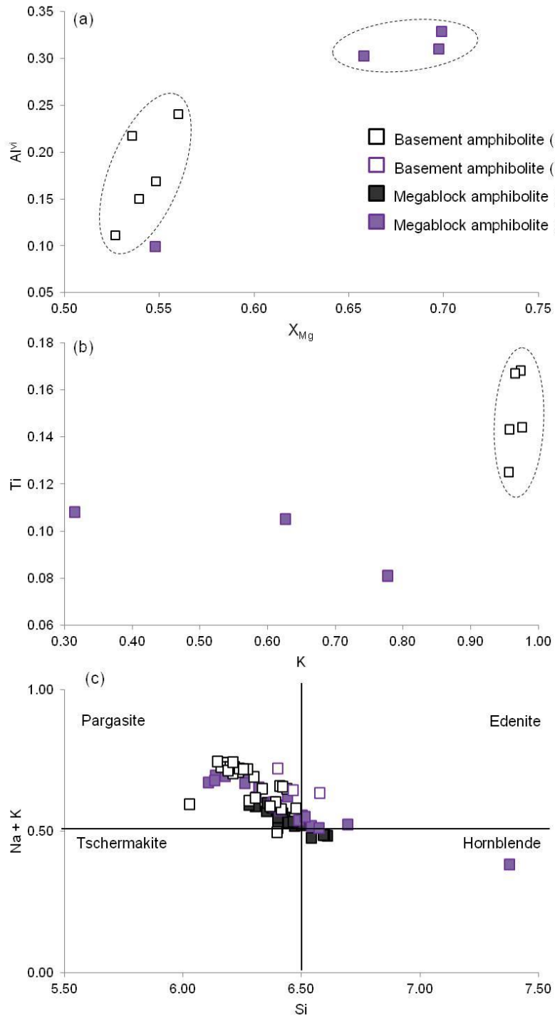
Figure 4.6: (a) X_{Mg} vs. Al^{VI} and (b) K vs. Ti abundances (apfu for 11 oxygens) in Bt for the lower basement-derived amphibolite ( n = 5 ) and megablock amphibolite ( n = 4 ). (c) Amphibole classification diagram (after Leake, 1978; Deer et al. , 1992) using Na + K abundances plotted against Si (apfu for 23 oxygens) for the lower basement-derived amphibolite ( n = 31 ) and the upper megablock amphibolite ( n = 44 ). Dashed lines represent observed groupings. Abbr.: Bln = EMP analyses obtained in Berlin; Bt = biotite; n = number of analyses; Pta = EMP analyses obtained in Pretoria.
