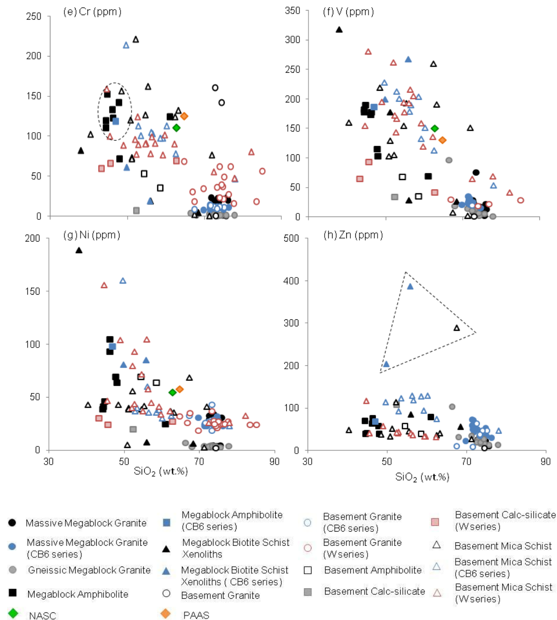
Figure 3.12 (continued): Harker diagrams showing trace element (Rb, Sr, Zr, Ba, Cr, V, Ni and Zn) concentrations (in ppm) plotted against \text{SiO}_2 for the eight target rock units of the Eyreville-B borehole core. Abbr.: NASC = North American Shale Composite (after Gromet et al. , 1984); PAAS = Post Archean Australian Shale (after Taylor and McLennan, 1985). Dashed lines represent observed groupings.
