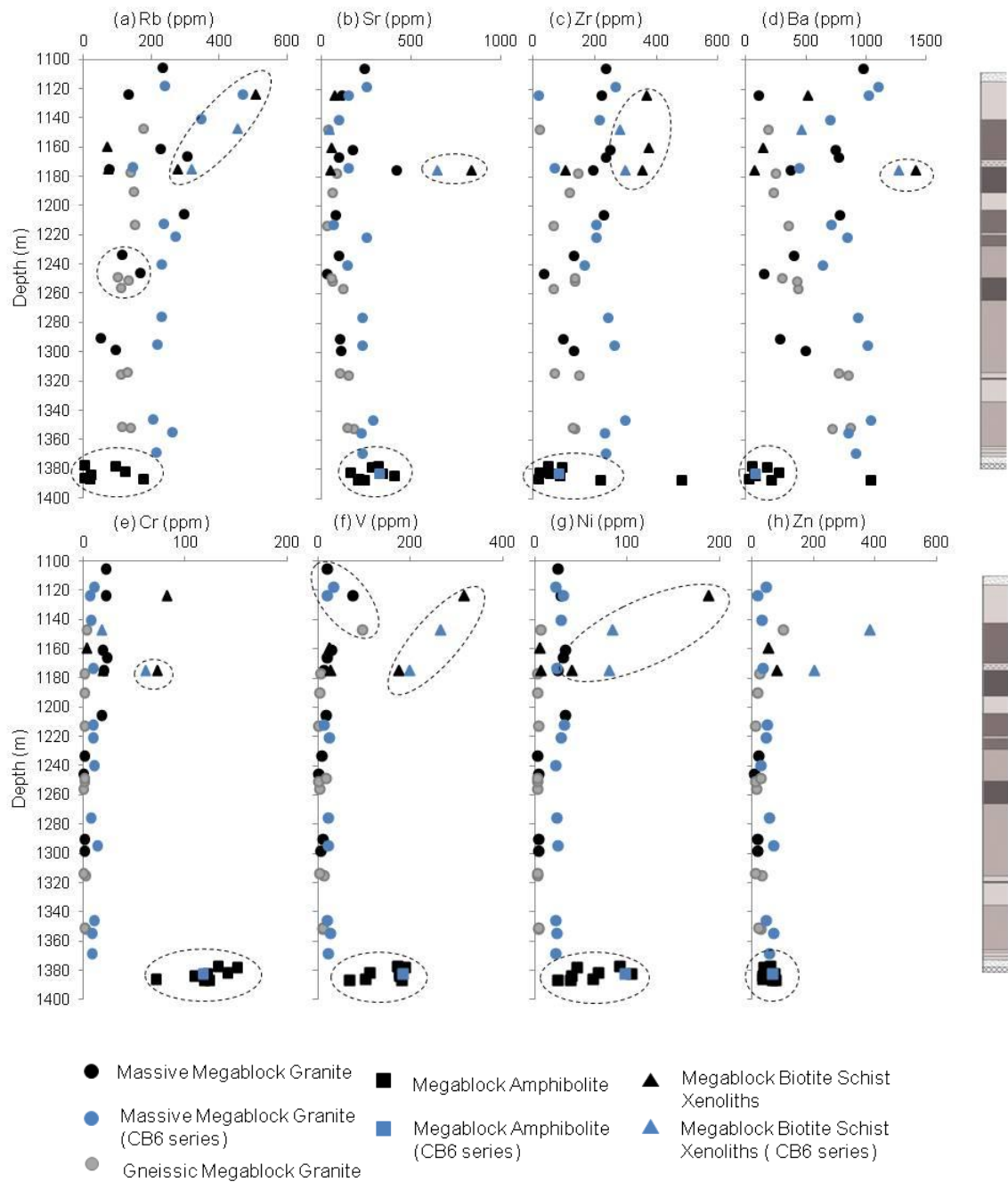
Figure 3.11: Variations in trace element concentrations (ppm) with depth (m) for the four target rock units in the upper granite and amphibolite megablocks of the Eyreville-B borehole core. The geologic column, after Horton et al. (2009), has been placed on the right side for reference purposes. Not all samples could be plotted for Rb, Cr, Ba, V and Zn graphs as their concentrations were below the lower limit of detection. Samples from the CB6 series (after Schmitt et al. , 2009) have been included to increase the data set size. The geologic column, as described in Chapters 1 and 2 (after Horton et al. , 2009a), has been placed on the right side for reference purposes. Dashed lines represent observed groupings.
