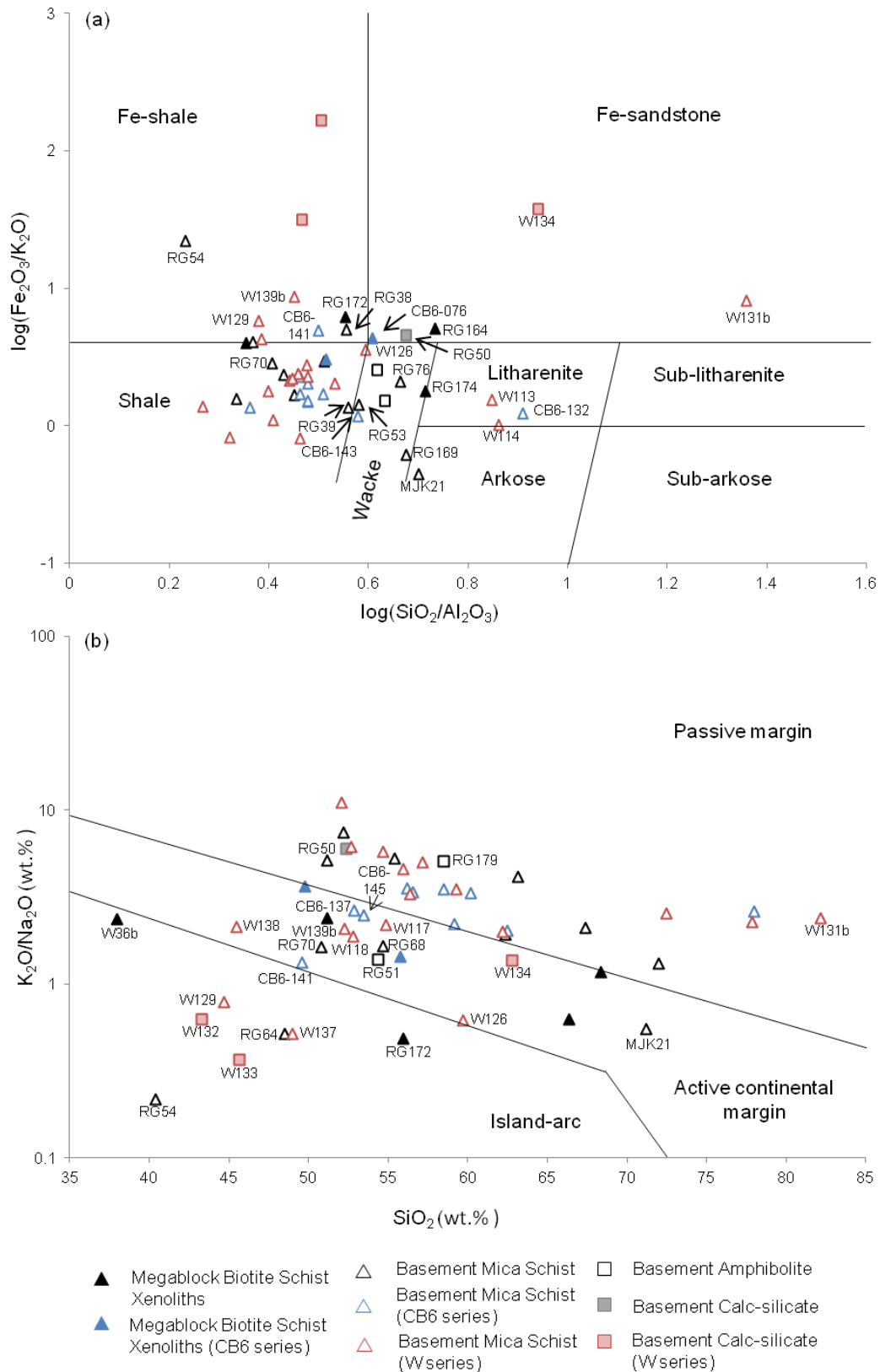
Figure 3.16: Bivariate diagrams for the basement and megablock mica schists and basement amphibolite and calc-silicate rock units of the Eyreville-B borehole core. (a) Classification scheme for terrigenous clastic sediments (after Herron, 1988); and (b) \text{K}_2\text{O}/\text{Na}_2\text{O} versus \text{SiO}_2 diagram indicating tectonic environment for sandstone-mudstone suites (after Roser and Korsch, 1986). All data in wt%.
