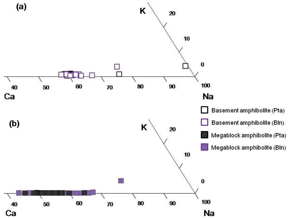
Figure 4.5: Ca-K-Na ternary diagrams for Pl in (a) the lower basement-derived amphibolite (n = 25) and (b) the upper megablock amphibolite (n = 55). Abbr.: Bln = EMP analyses obtained in Berlin; n = number of analyses; Pl = plagioclase; Pta = EMP analyses obtained in Pretoria.
