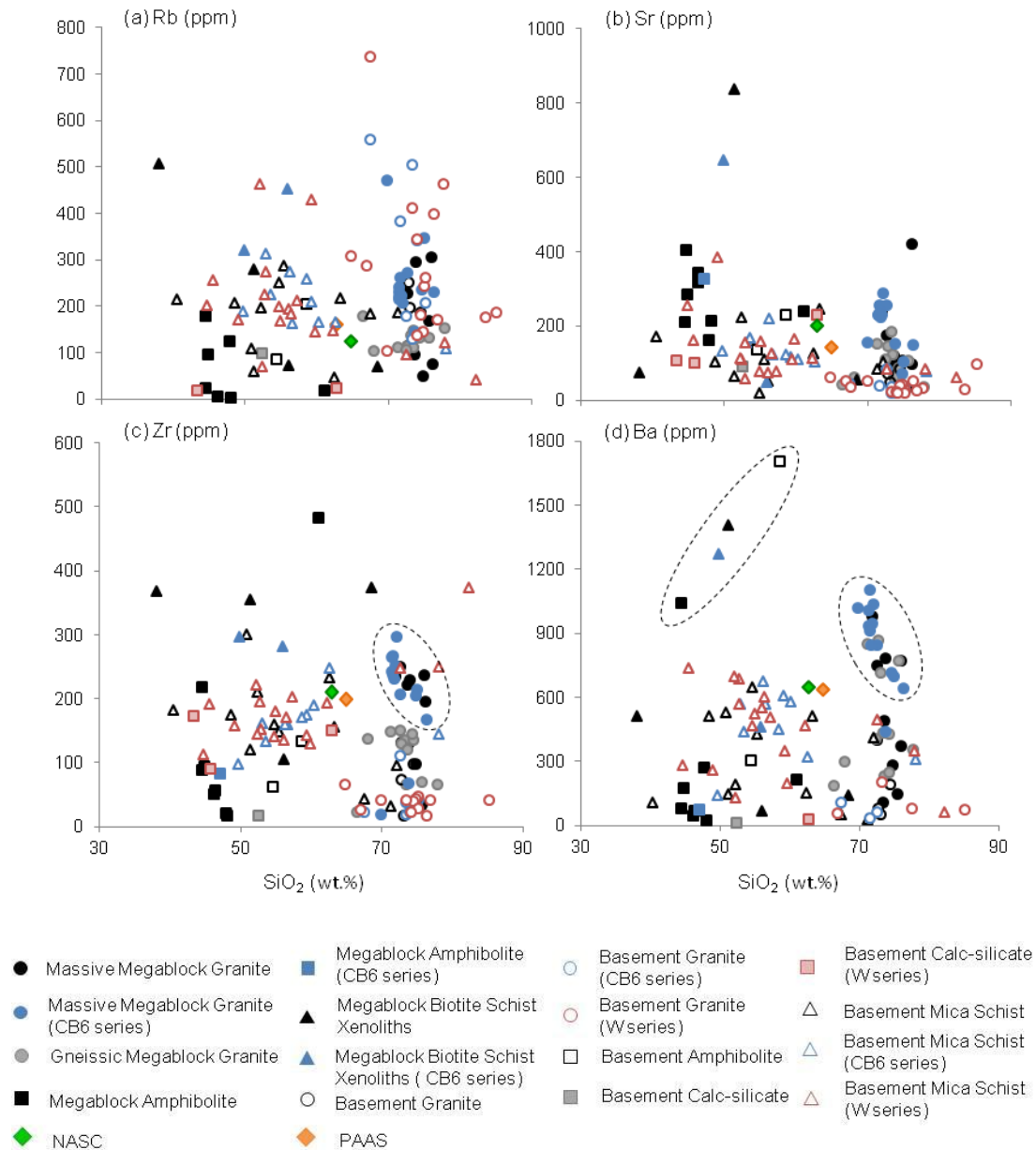
Figure 3.12: Harker diagrams showing trace element (Rb, Sr, Zr, Ba, Cr, V, Ni and Zn) concentrations (in ppm) plotted against \text{SiO}_2 for the eight target rocks units of the Eyreville-B borehole core. Abbr.: NASC = North American Shale Composite (after Gromet et al. , 1984); PAAS = Post Archean Australian Shale (after Taylor and McLennan, 1985). Dashed lines represent observed groupings.
