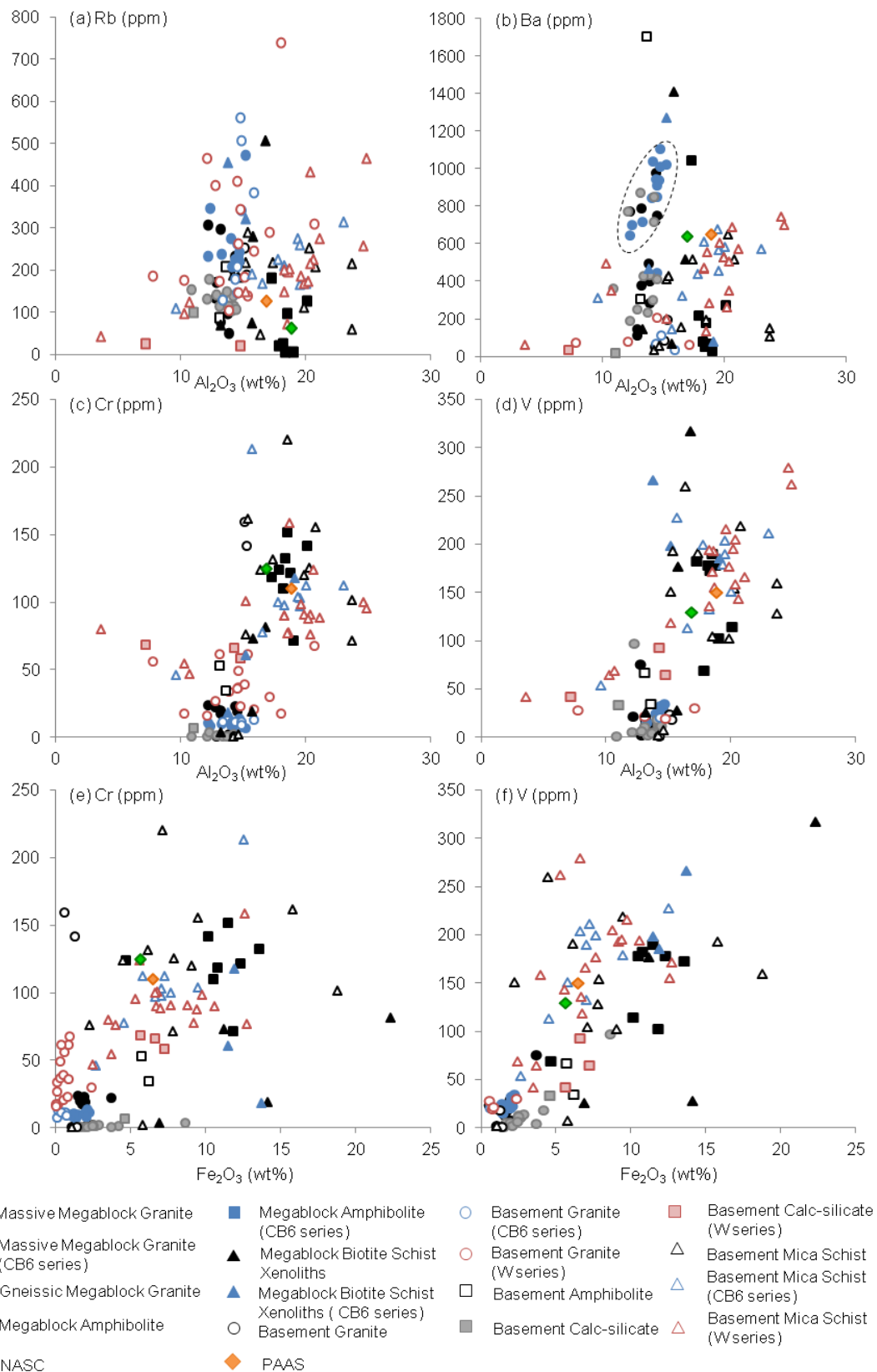
Figure 3.13: Harker diagrams showing trace element concentrations (in ppm) plotted against \text{Al}_2\text{O}_3 (Rb, Ba, Cr and V) and against \text{Fe}_2\text{O}_3 (Cr and V) for the eight target rocks units of the Eyreville-B borehole core. Abbr.: NASC = North American Shale Composite (after Gromet et al. , 1984); PAAS = Post Archean Australian Shale (after Taylor and McLennan, 1985). Dashed lines represent observed groupings.
