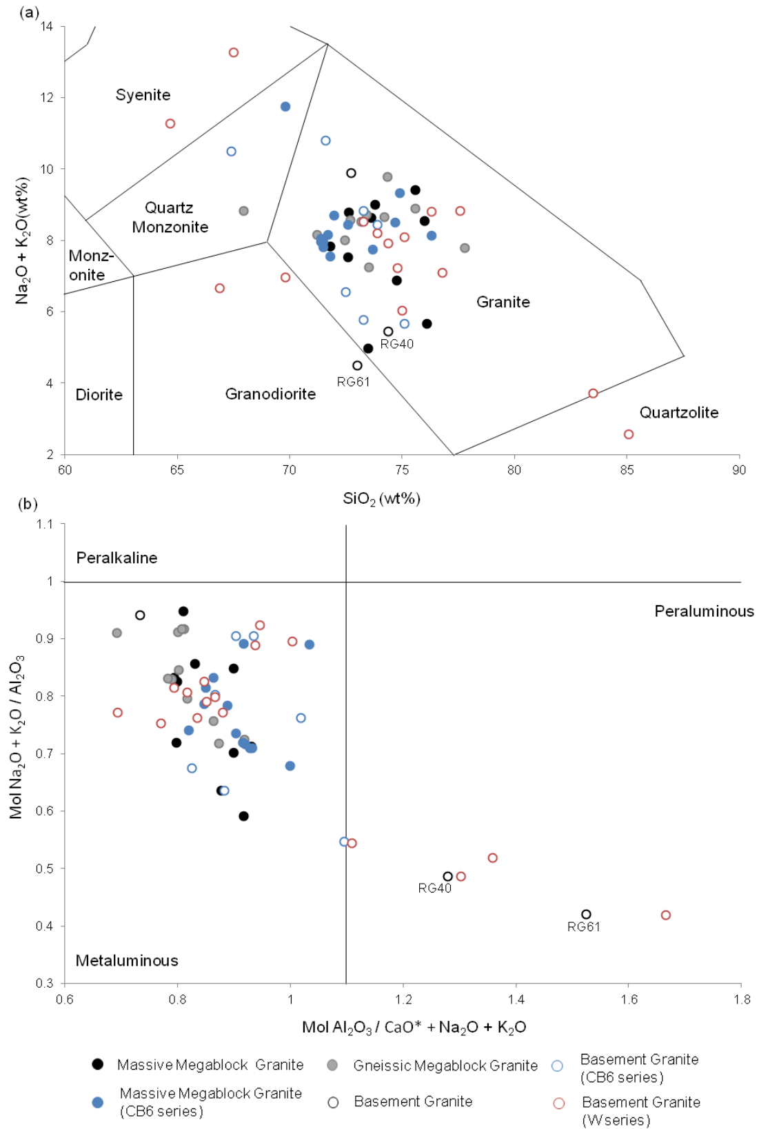
Figure 3.5: Bivariate diagrams for the granite rock units of the Eyreville-B borehole core: (a) TAS diagram for the classification of plutonic rocks (after Middlemost, 1994), and (b) ASI (after Shand, 1927; Chappell and White, 1974). All data in wt%.
