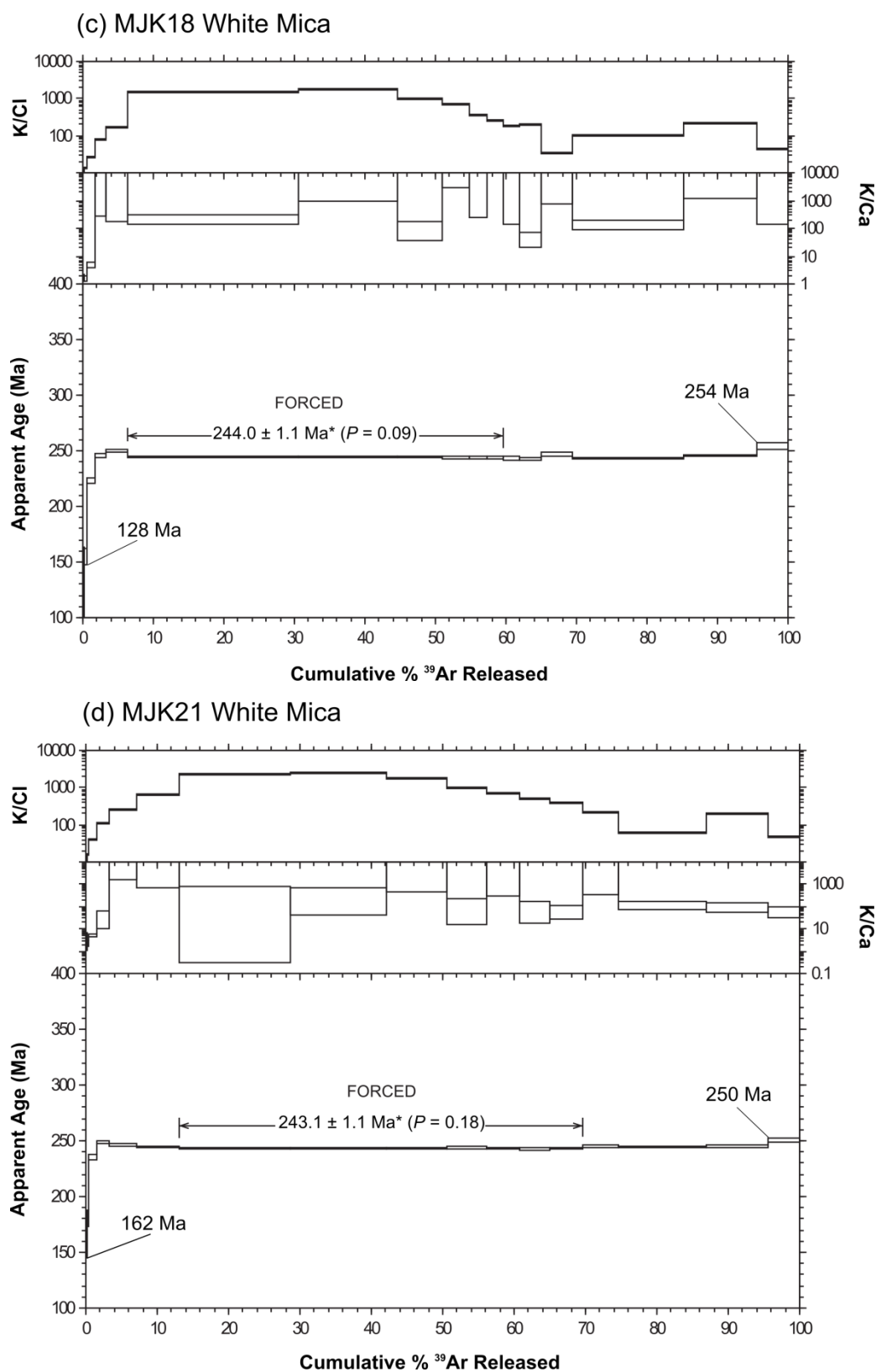
Figure 5.8 continued: White mica age spectra, K/Cl and K/Ca diagrams for mica samples (a) RG169, (b) RG56, (c) MJK18 and (d) MJK21. Plateau ages ( \pm 1\sigma ), age maxima and age minima are as indicated. Symbol: * = forced plateau age; P = probability.
