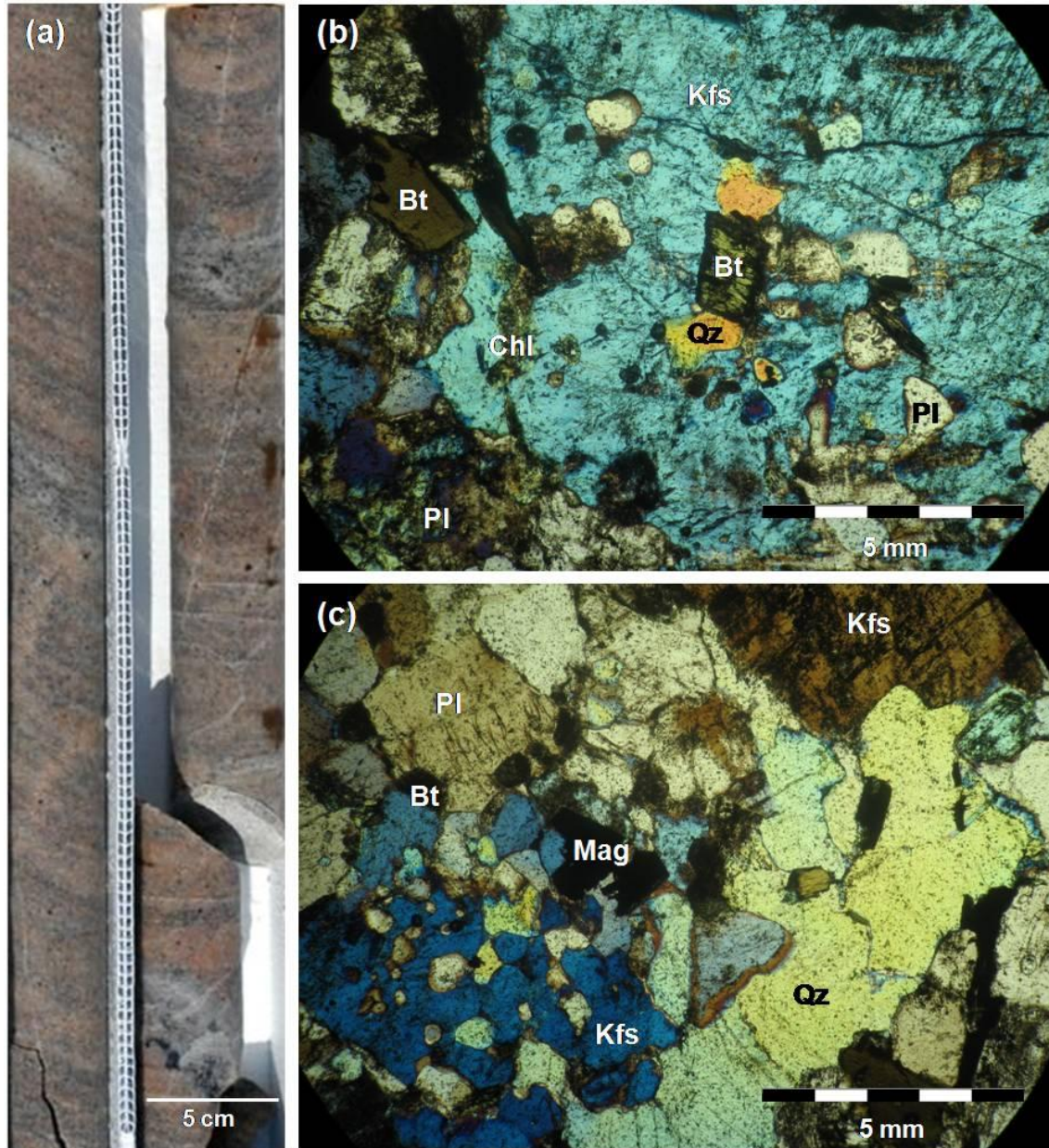
Figure 2.13: Photographs of the gneissic granite in the upper megablock. (a) Corebox 158 illustrating the gneissic banding. Photomicrographs (XPL) of (b) sample RG151 and (c) sample RG152 illustrating altered, poikilitic Kfs and altered PI grains as well as Bt retrogressing to Chl in the gneissic megablock granite. Abbr.: Bt = biotite; Chl = chlorite; Kfs = K-feldspar; Mag = magnetite; PI = plagioclase; Qz = quartz; XPL = cross polarised light.
