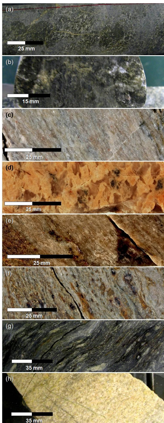
Figure 5.5: Hand specimen photographs for samples (a) RG177, (b) RG176, (c) RG40, (d) RG167, (e) RG169, (f) RG56, (g) MJK18 and (h) MJK21.
