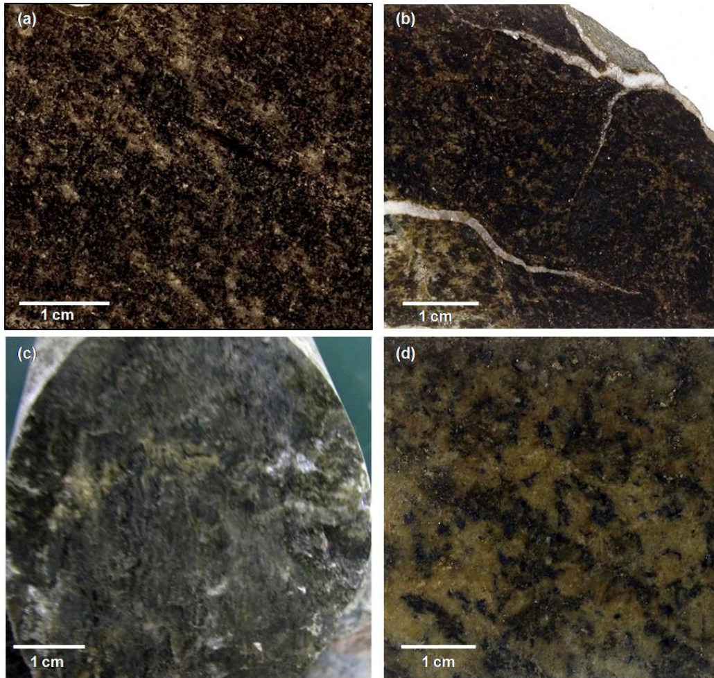
Figure 2.19: Hand specimen photographs of (a) sample RG172 showing the biotite-defined foliation in the biotite schist xenoliths in the upper granite megablock, (b) sample RG02 showing the foliation in the upper amphibolite megablock that is locally cut by Cal and Qz veins, (c) sample RG176 showing the mineral lineation relative to the orientation of the core in the upper amphibolite megablock, and (d) sample RG06 showing the coarse-grained, phaneritic texture preserved in parts of the upper amphibolite megablock. Abbr.: Cal = calcite; Qz = quartz.
