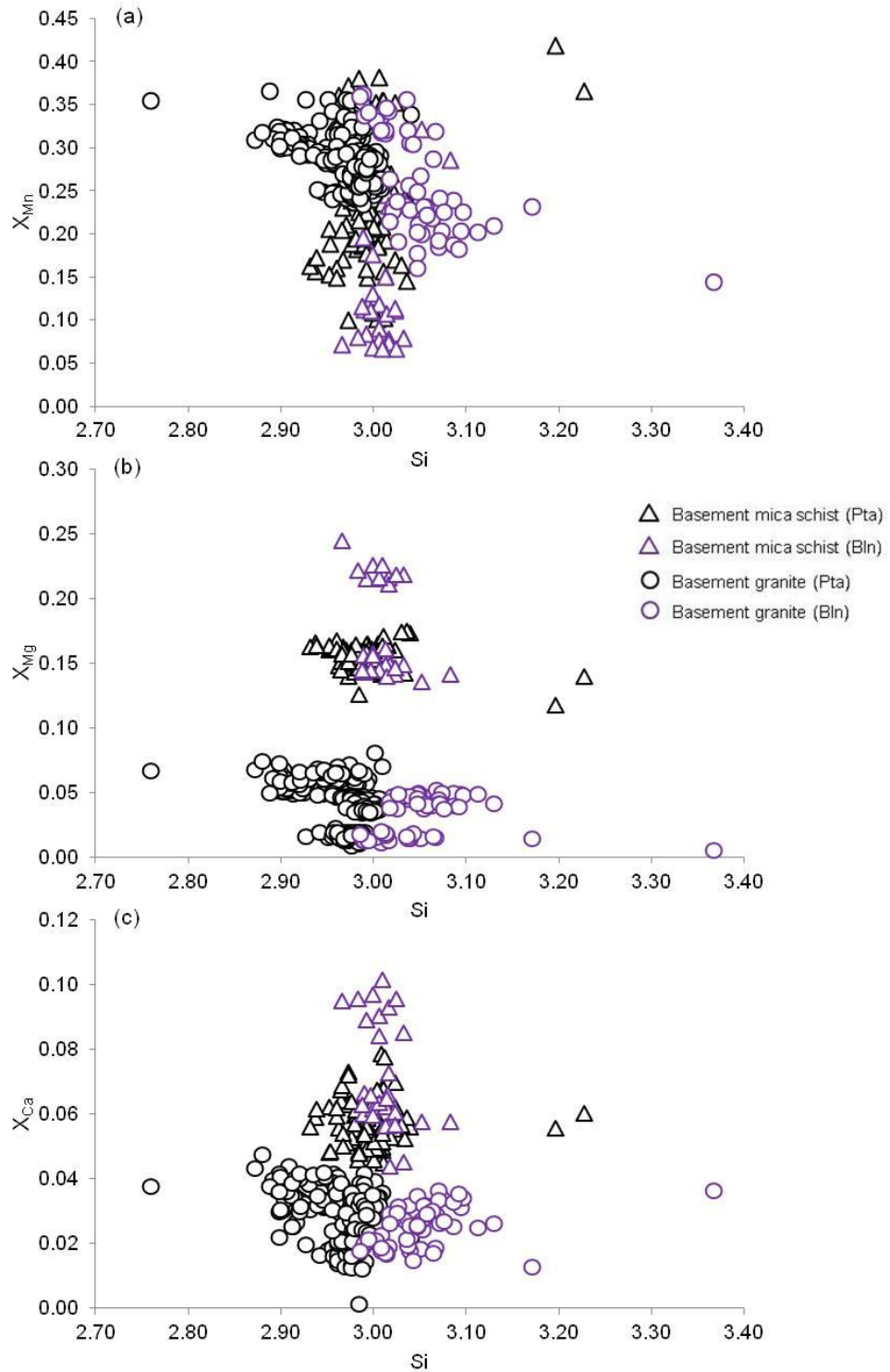
Figure 4.3: Bivariate diagrams showing (a) X_{Mn} , (b) X_{Mg} and (c) X_{Ca} elemental ratios of Grt plotted against Si (apfu for 12 oxygens) for both mica schist ( n = 109 ) and granite ( n = 296 ) in the lower basement-derived section. Abbr.: Bln = EMP analyses obtained in Berlin; Grt = garnet; n = number of analyses; Pta = EMP analyses obtained in Pretoria.
