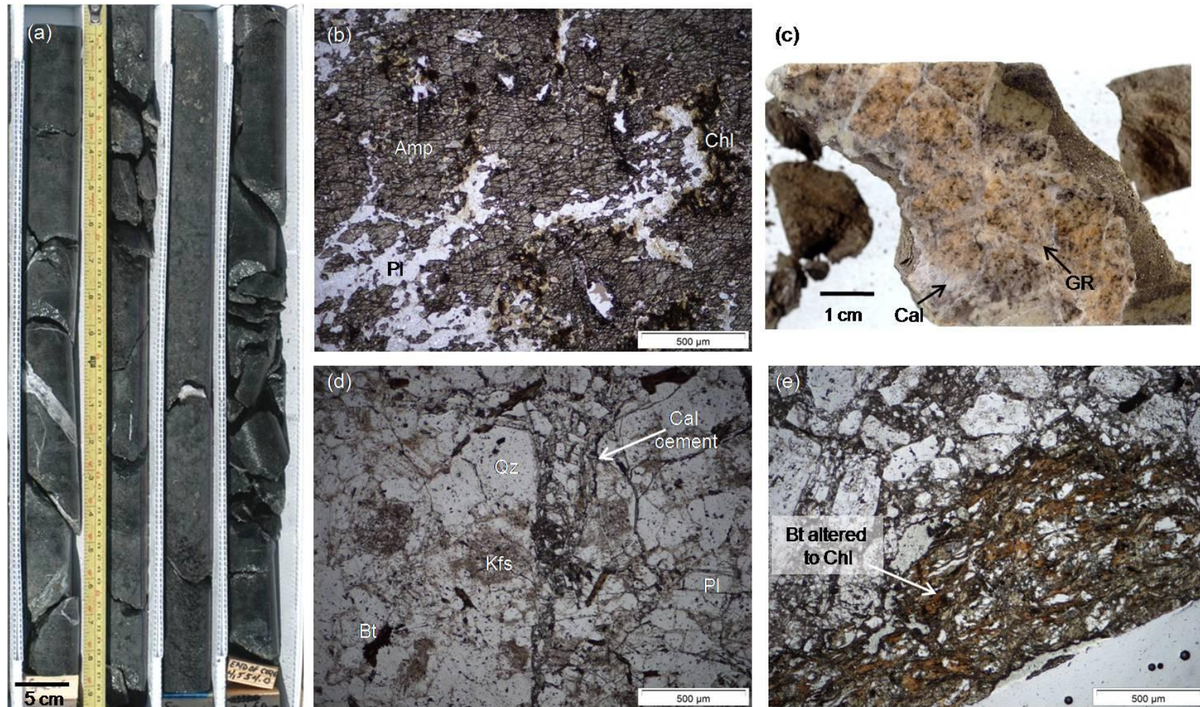
Figure 2.12: Photographs of the upper amphibolite megablock. (a) Corebox 226 showing the zone of coarse-grained amphibolite that contains a relict igneous texture within the generally homogenous megablock. (b) Photomicrograph (PPL) of sample W51 showing aggregates of Amp in certain parts of the megablock. (c) Hand specimen and (d) photomicrograph (PPL) of the brecciated GR vein within a Cal matrix (sample RG04) showing the brecciation at macro and microscopic scale. (e) Photomicrograph (PPL) of sample RG04 showing the contact zone between the granite-bearing calcite vein and the amphibolite where Bt has been intensely altered to Chl. Abbr.: Amp = amphibole; Bt = biotite; Cal = calcite; Chl = chlorite; GR = granite; Kfs = K-feldspar; Pl = plagioclase; Qz = quartz.
