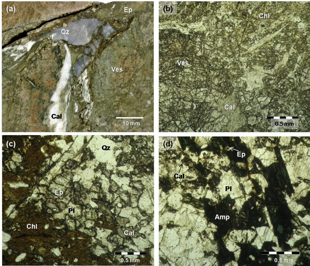
Figure 2.5: Hand specimen and thin section (PPL) photographs of the lower basement-derived calc-silicate sample RG50 showing (a) its highly brecciated nature, (b) the peak metamorphic assemblage, (c) the retrograde metamorphic assemblage and (d) the Amp component. Abbr.: Amp = amphibole; Cal = calcite; Chl = chlorite; Ep = epidote; Pl = plagioclase; PPL = plane polarised light; Qz = quartz; Ves = vesuvianite.
