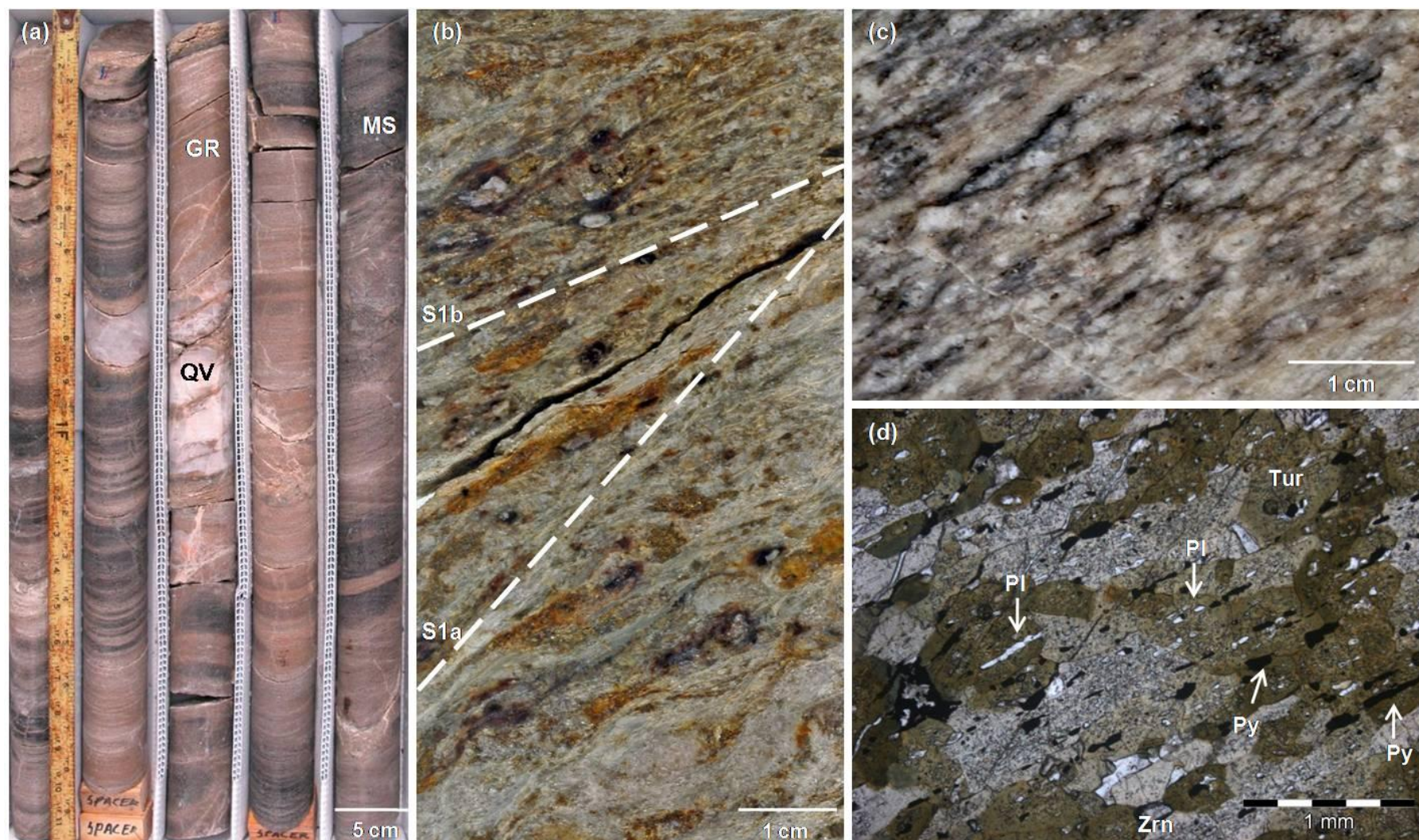
Figure 2.17: Photographs of the S1b foliation in the lower basement-derived mylonite. (a) Corebox 310 showing the mylonite zone with interlayered GR, MS and QV. (b) Hand specimen of sample RG56 showing the S1a and S1b foliations in the retrogressed MS. (c) Hand specimen of sample RG40 showing the S1b foliation in the fine-grained mylonitised Gr. (d) Photomicrograph (PPL) of sample RG57 showing the S1a foliation defined by elongated PI and Py inclusions in Tur. Abbr.: GR = granite; MS = mica schist; PI = plagioclase; PPL = plane polarised light; Py = pyrite; QV = quartz vein; Tur = tourmaline; Zrn = zircon.
