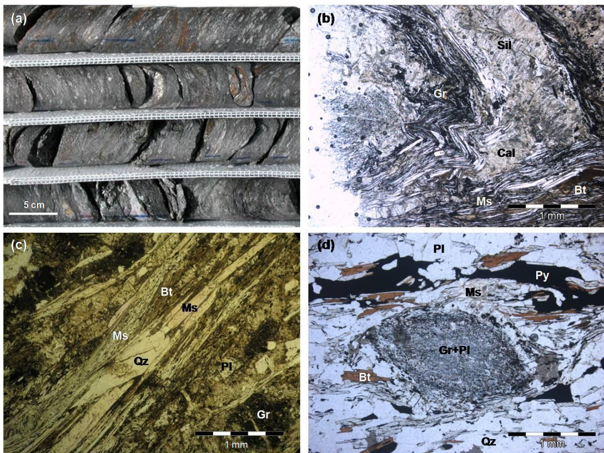
Figure 2.2: Corebox and thin section photographs of the lower basement-derived mica schists. (a) Corebox 322 showing the highly foliated nature of the mica schists. (b) Sample RG60 showing folds that locally deform the mica schist foliation (PPL). (c) Sample RG34 showing an elongated Qz grain within the Ms-Bt foliae and adjacent irregular masses of Gr (PPL). (d) Zoned Pl porphyroblasts with Gr-rich cores in sample RG68 (PPL). Abbr.: Bt = biotite; Cal = calcite; Gr = Graphite; Ms = muscovite; Pl = plagioclase; PPL = plane polarised light; Py = pyrite; Qz = quartz; Sil = sillimanite (mineral abbreviations after Whitney and Evans, 2010).
