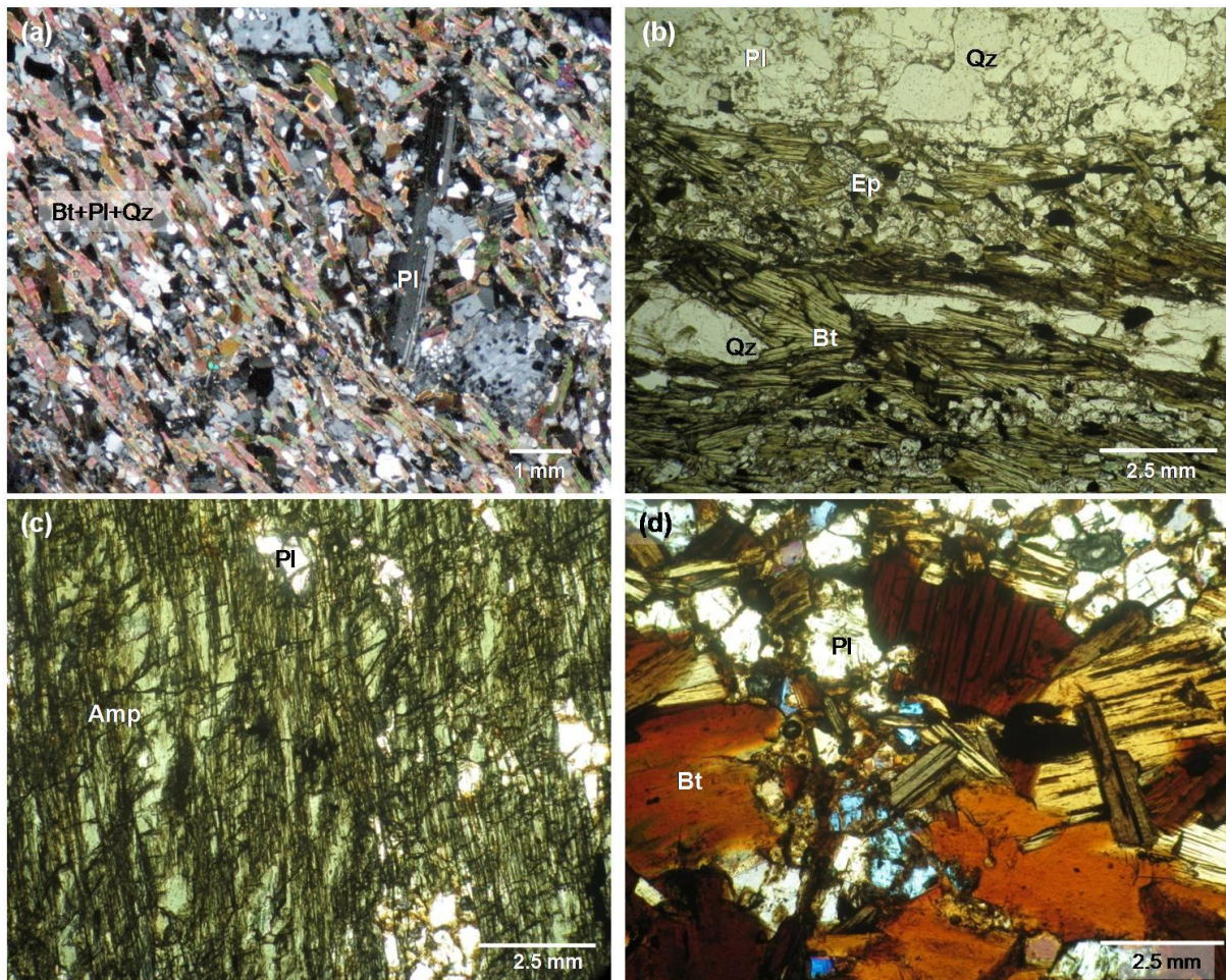
Figure 2.25: Photomicrographs of (a) sample W39 showing rotated plagioclase porphyroblasts (XPL) and (b) boudinaged quartz ribbons (PPL) in the biotite schist xenoliths of the upper granite megablock, and (c) samples RG177 (PPL) and (d) RG176 (XPL) showing monomineralic aggregates of amphibole and biotite, respectively. Abbr.: Amp = amphibole; Bt = biotite; Ep = epidote; Pl = plagioclase; PPL = plane polarised light; Qz = quartz; XPL = cross polarised light.
