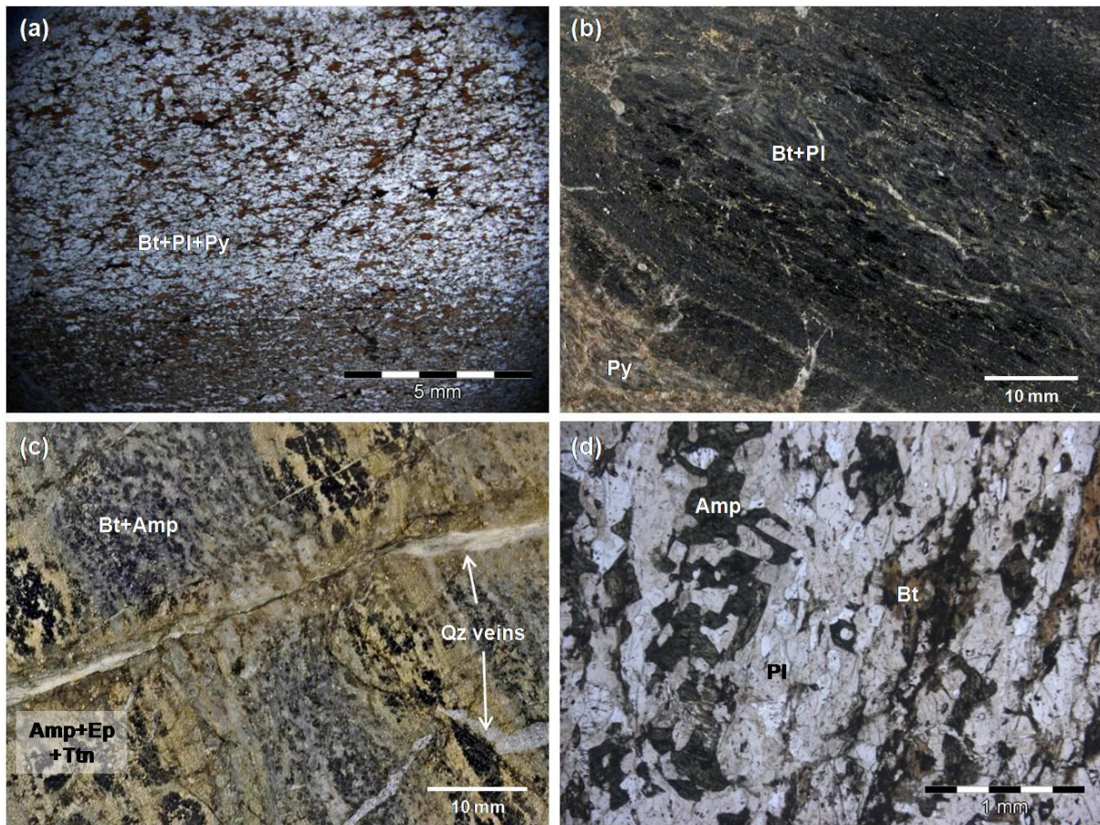
Figure 2.4: (a) Photomicrograph (PPL) and (b) hand specimen photograph of the lower basement-derived biotite schist sample RG70 showing the large amount of Bt that defines the lithology. (c) Hand specimen and (d) photomicrograph (PPL) of the lower basement-derived amphibolite sample RG51 where alternating bands of Bt-rich and Bt-poor assemblages are shown. Abbr.: Amp = amphibole; Bt = biotite; Ep = epidote; Pl = plagioclase; PPL = plane polarised light; Py = pyrite; Qz = quartz; Ttn = titanite.
