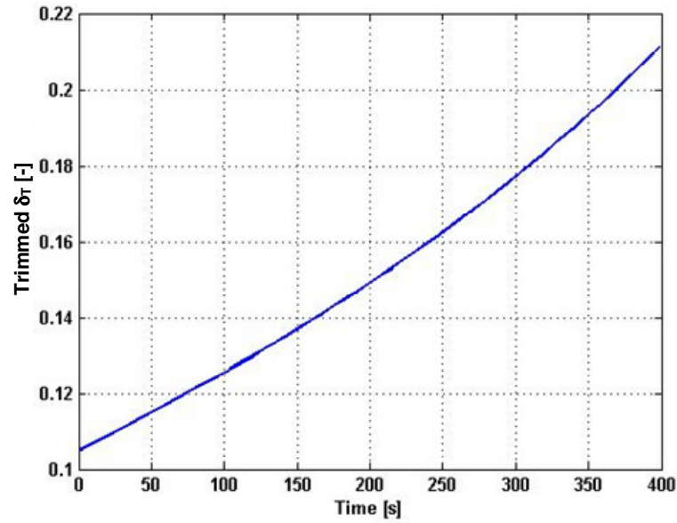
Figure 6.5: Refuelling trimmed throttle position change with mass
