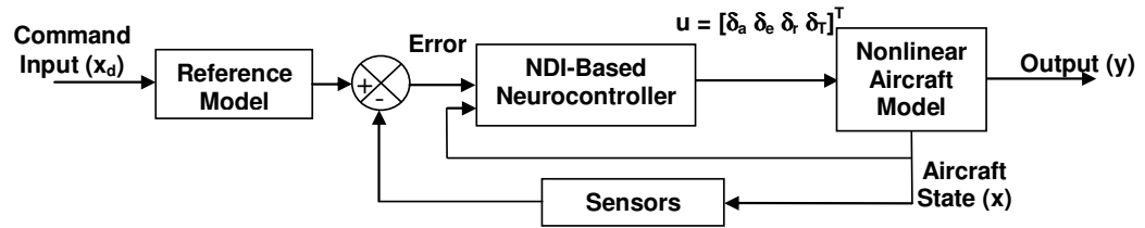
Figure 4.2: Overall controller model
