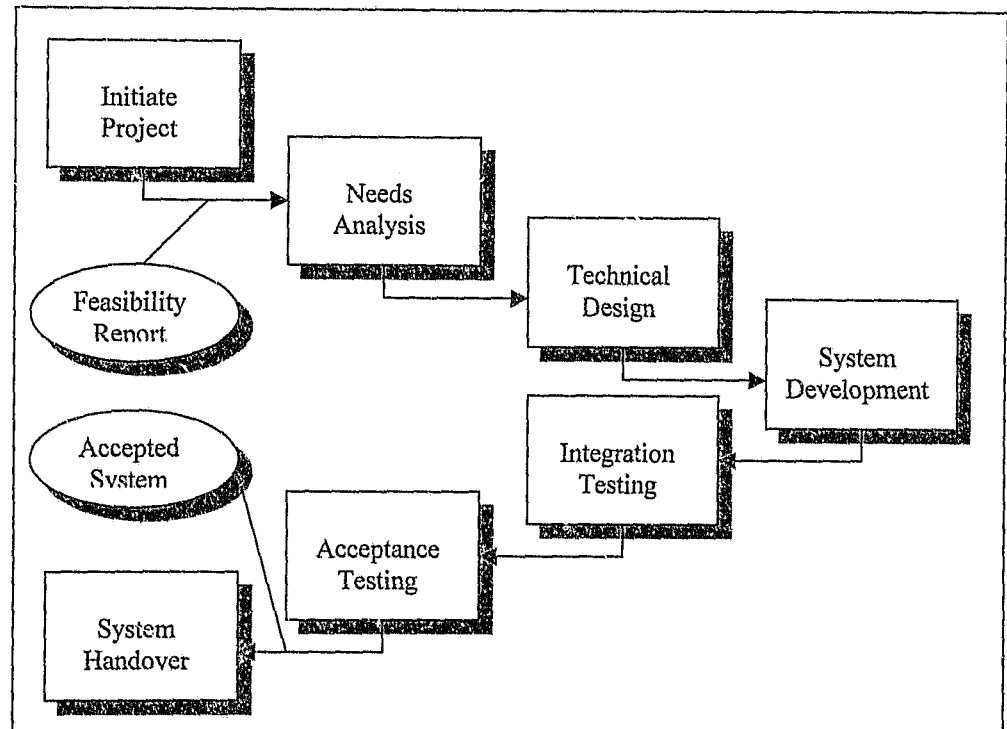
Figure 1: V-model
