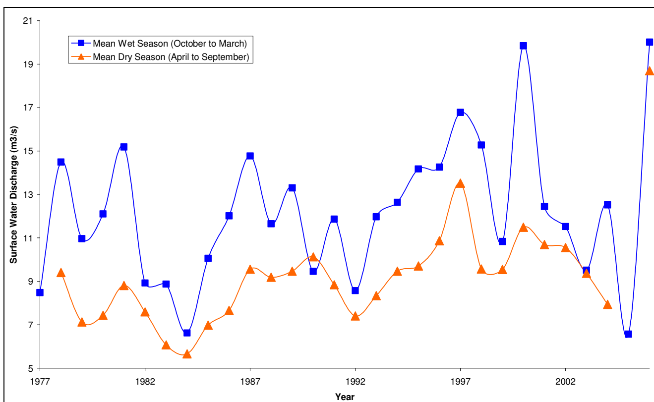
Figure 5.5.1: Mean wet and dry season trends for water discharge data at Witkop Station (C2H141) between 1977 and 2006.
