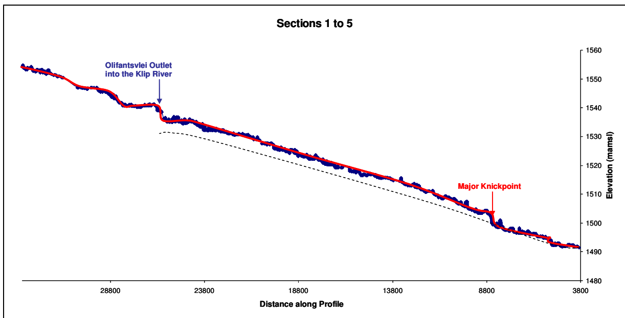
Figure 6.1: Long river profile from Lenasia to the Zwartkoppies Pump Station.
