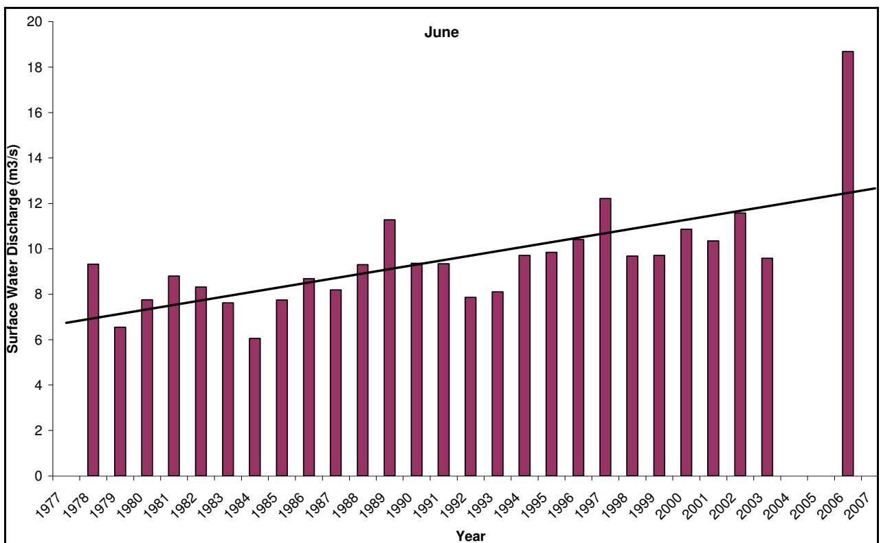
Figure 5.5.3: Water discharge in June at Witkop Station (C2H141) between 1977 and 2006.
