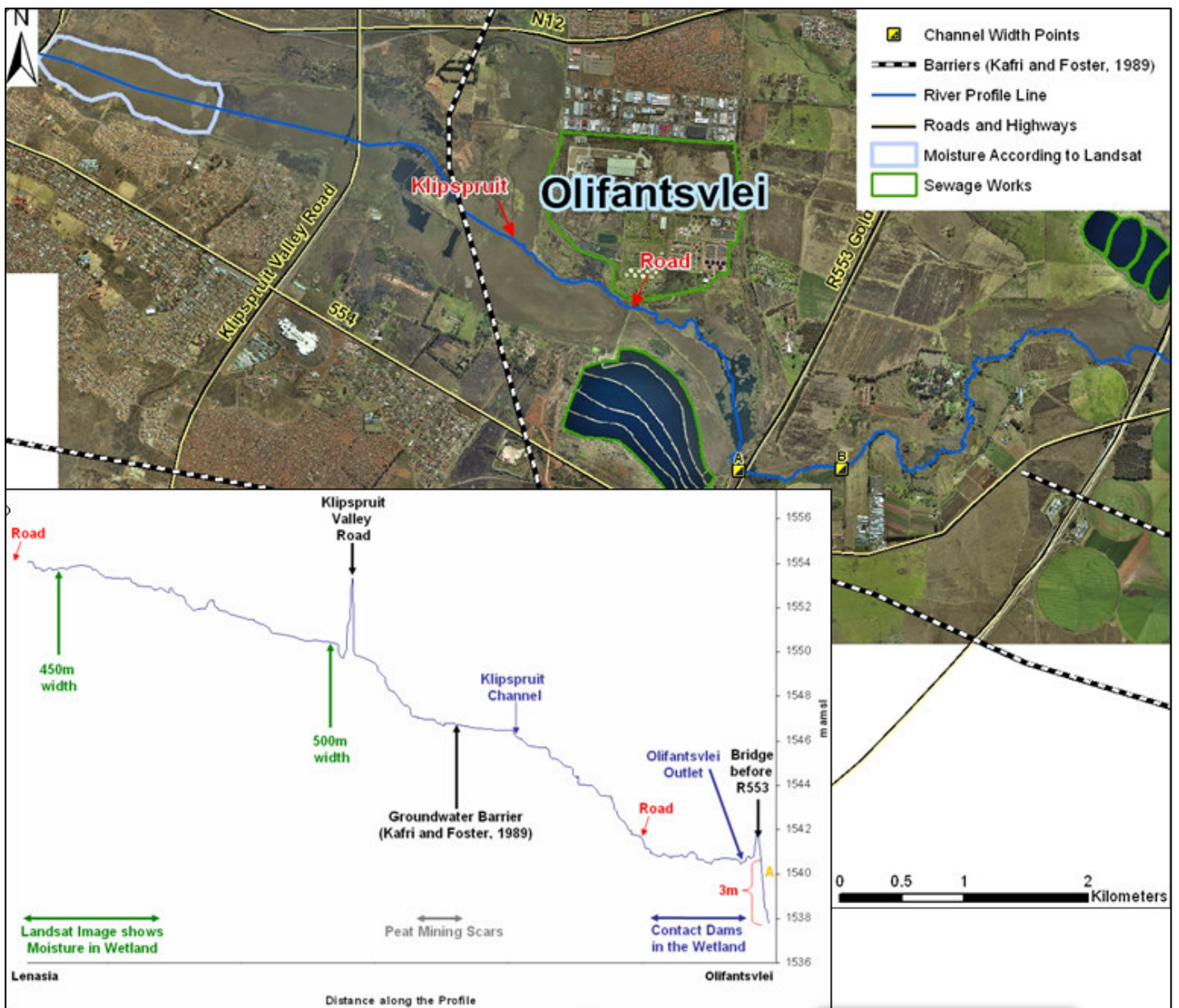
Figure 5.2.2: Long river profile from the road east of the golf course to the Golden Highway in relation to 2006 photography.
