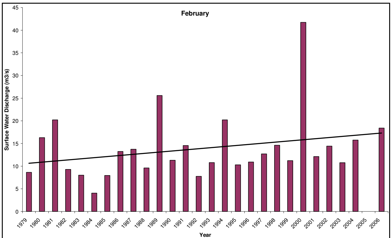
Figure 5.5.2: Water discharge in February at Witkop Station (C2H141) between 1979 and 2006.
