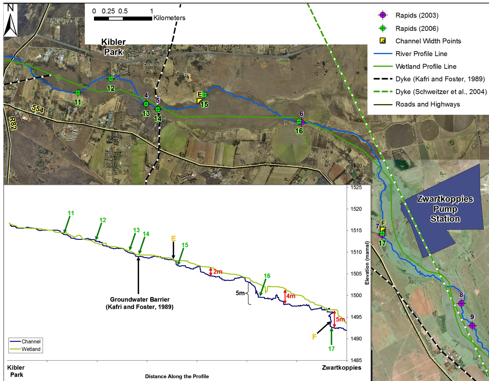
Figure 5.2.6: Long river profile from the Kibler Park to Zwartkoppies Pump Station in relation to 2006 photography.
