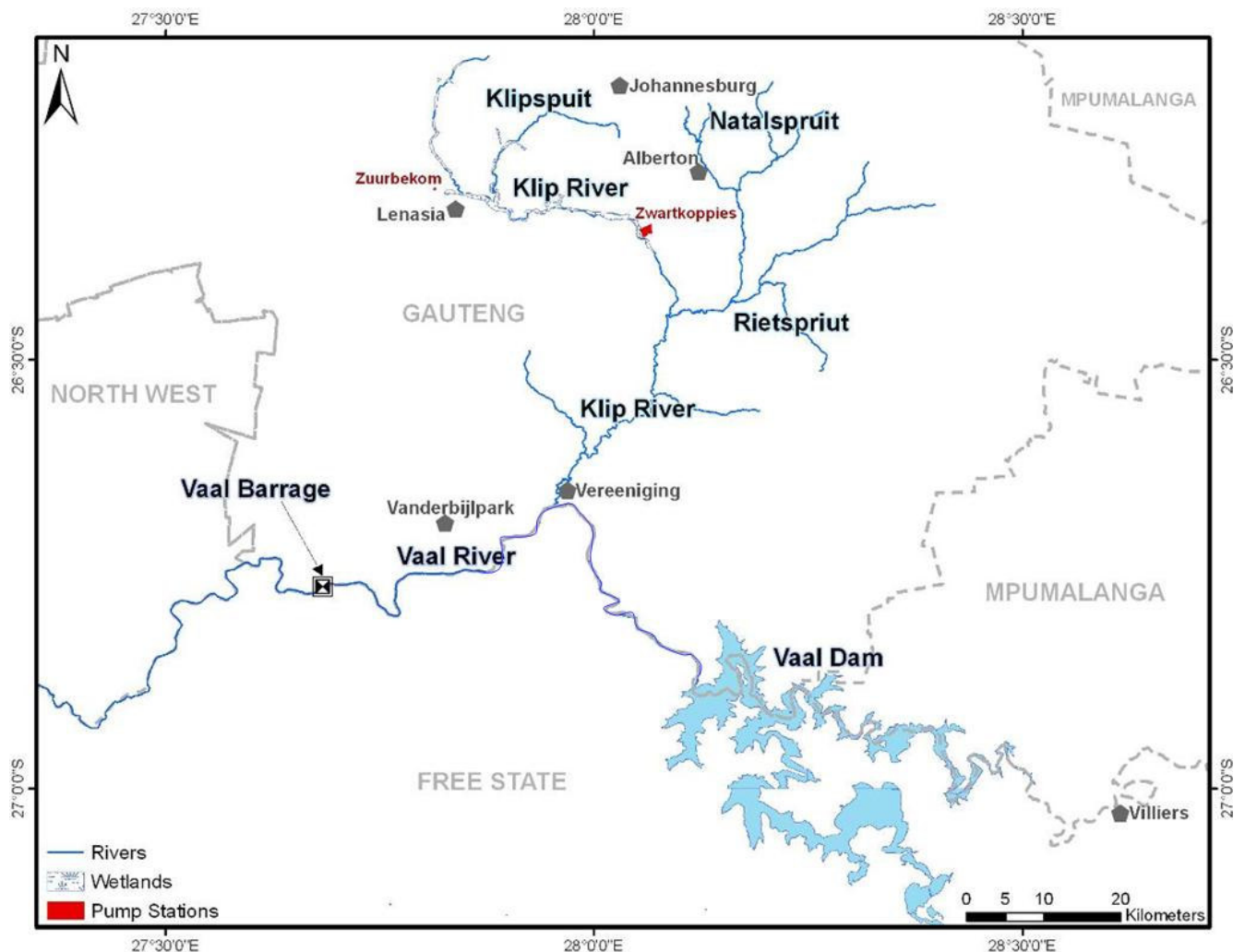
Figure 3.2.1: The Klip River in relation to the Vaal Barrage and the Vaal Dam.
