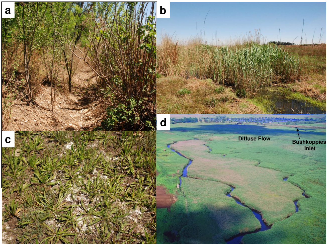
Figure 5.1.14: Field and aerial reconnaissance photos between the N1 Highway and Lenasia (d is courtesy of T.S. McCarthy, November 2007).
