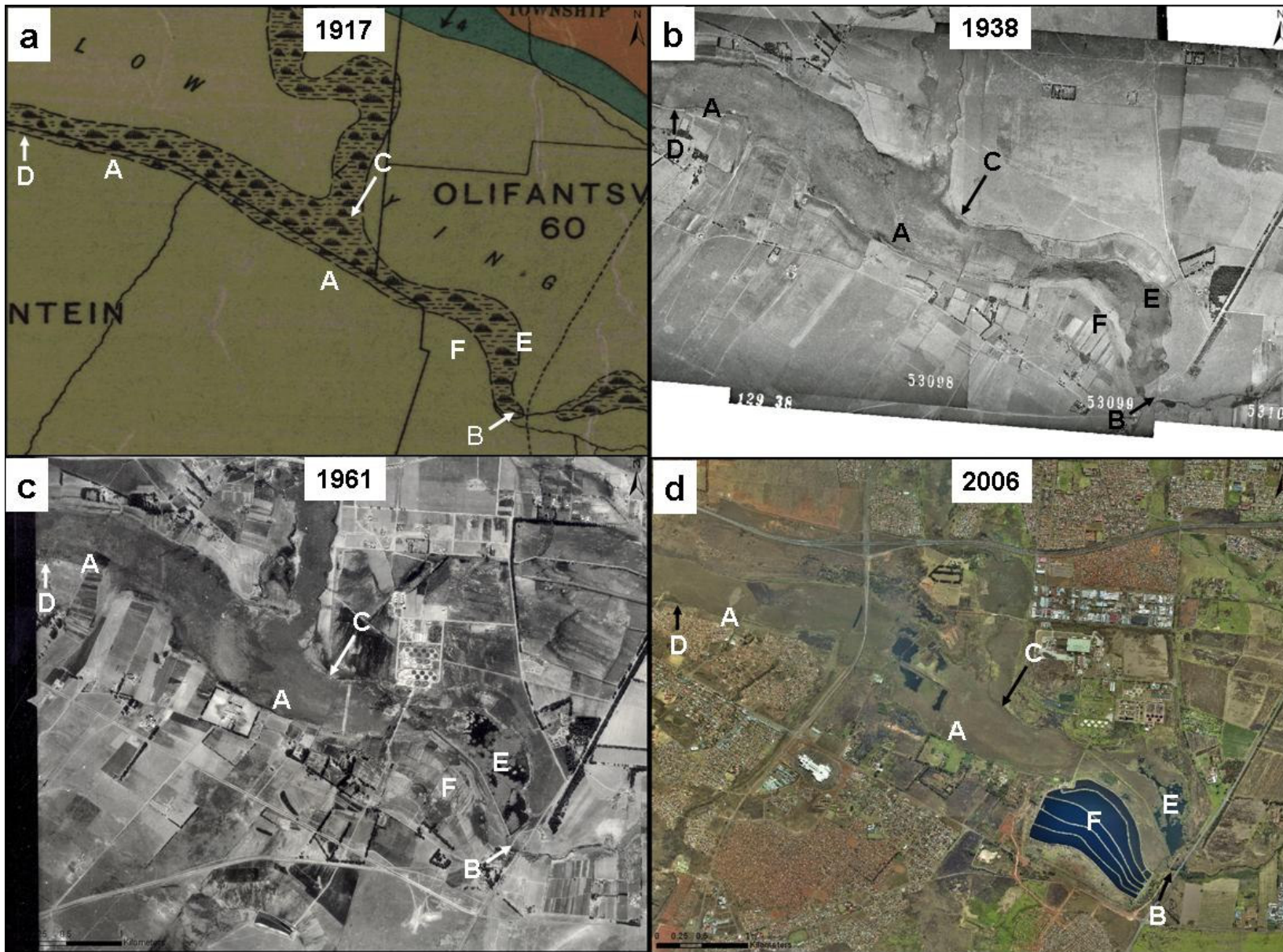
Figure 5.1.8: The wetland in the Lenasia area in (a) 1917, (b) 1938, (c) 1961 and (d) 2006.
