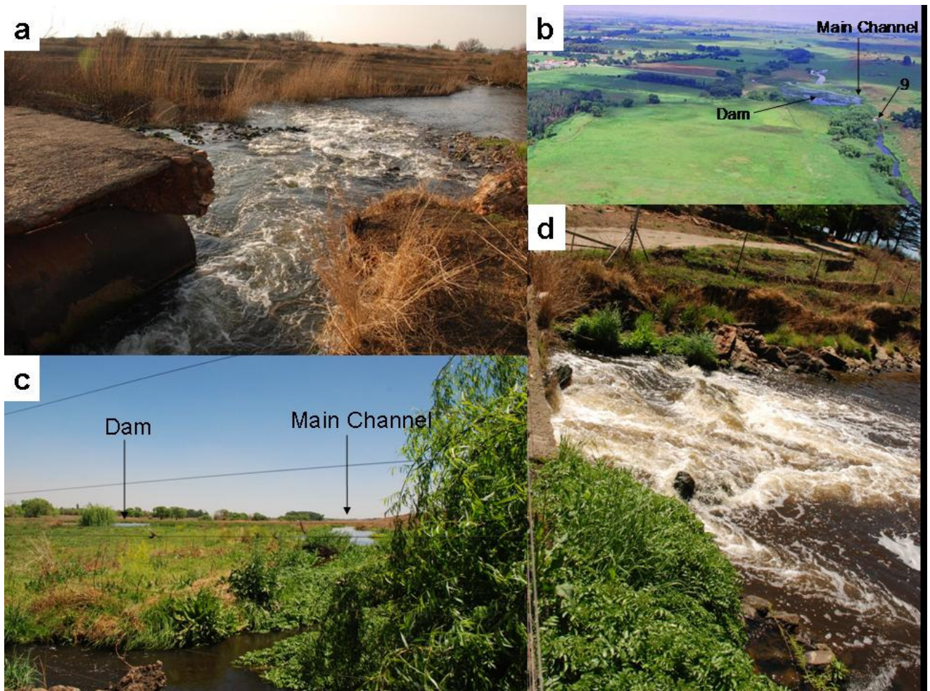
Figure 5.2.5: Field and aerial reconnaissance photos of the rapids between the N1 Highway and Lenasia (c courtesy of T.S. McCarthy, November 2007).
