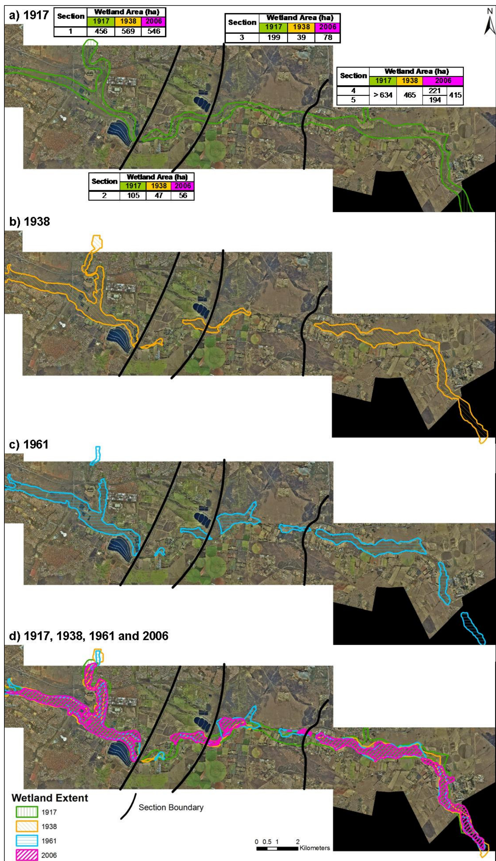
Figure 6.2: Wetland area in (a) 1917, (b) 1938, (c) 1961, and (d) 2006.
