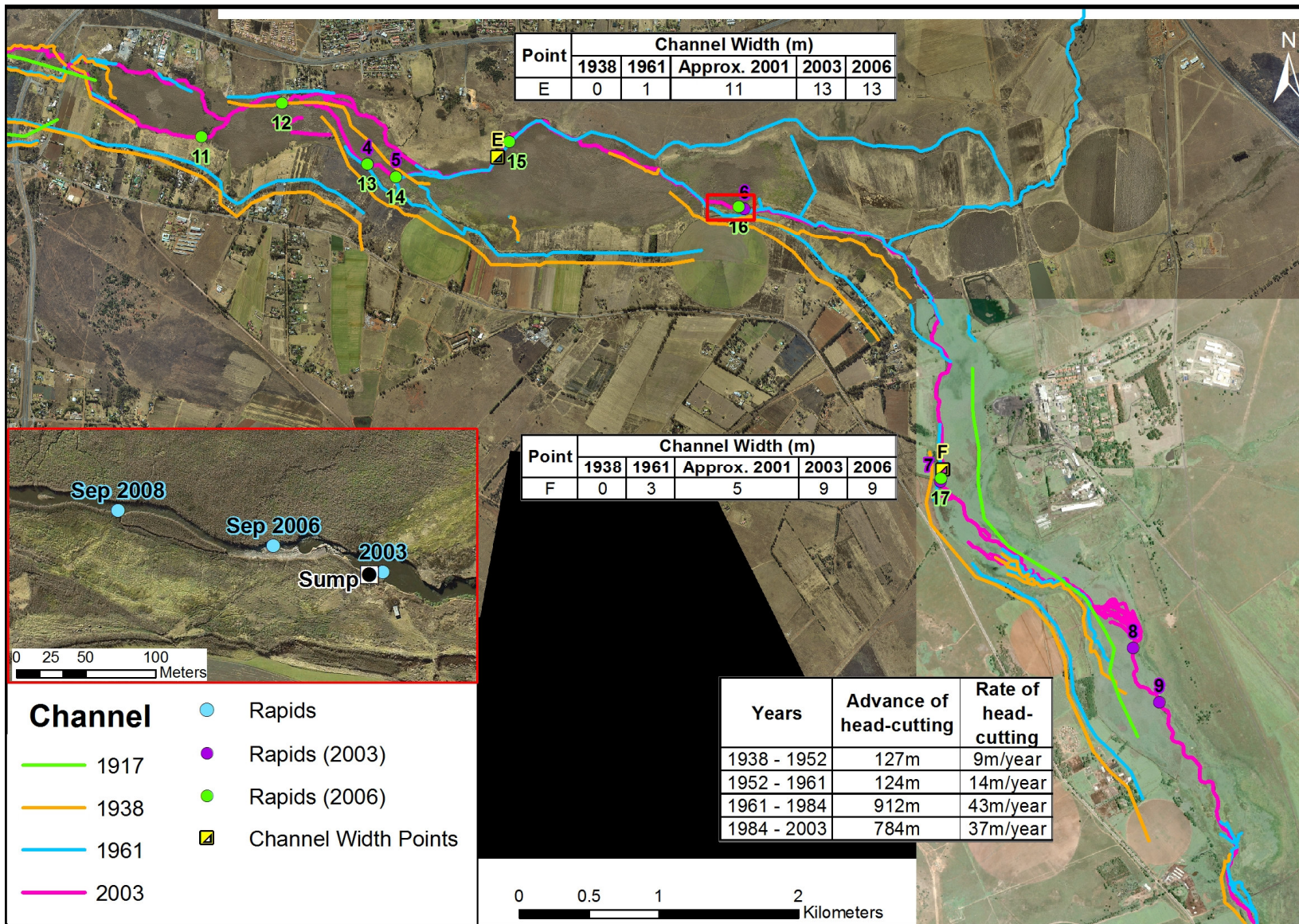
Figure 6.4: Channel formation, propagation, widening and knick point migration from Kibler Park to the Zwartkoppies Pump Station between 1917 and 2006.
