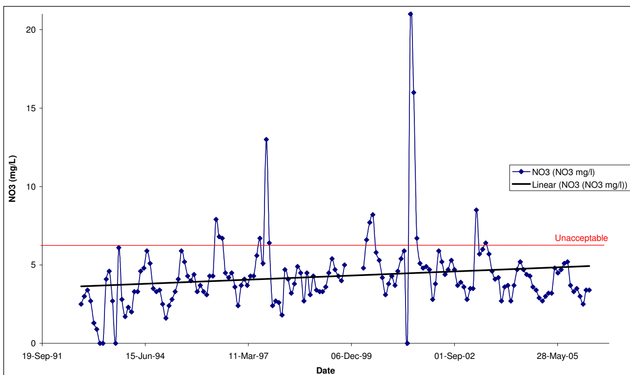
Figure 5.4.3: K21 nitrate levels from 1992 to 2006 (acceptability according to DWAF domestic water quality standards).
