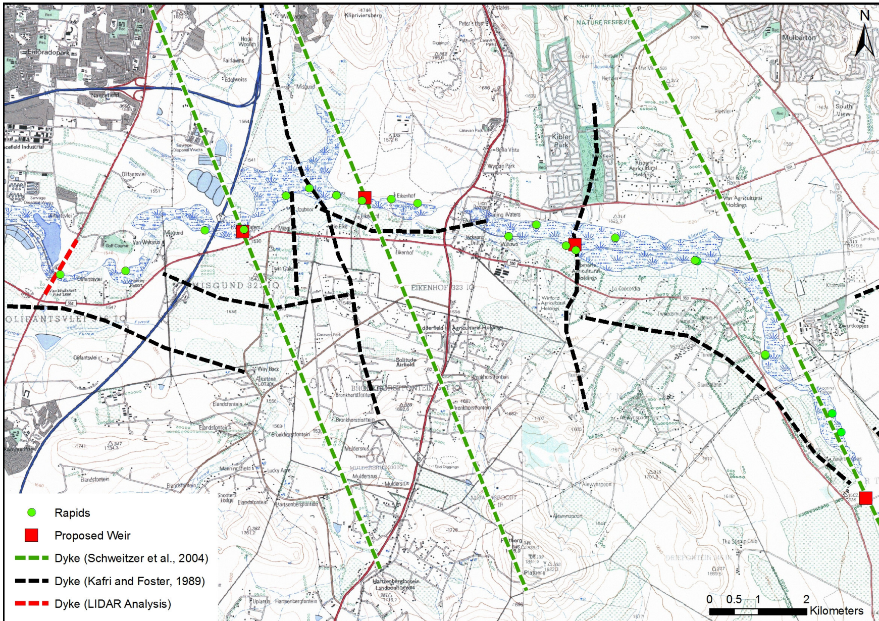
Figure 7.1: Proposed weir locations according to dyke positions.
