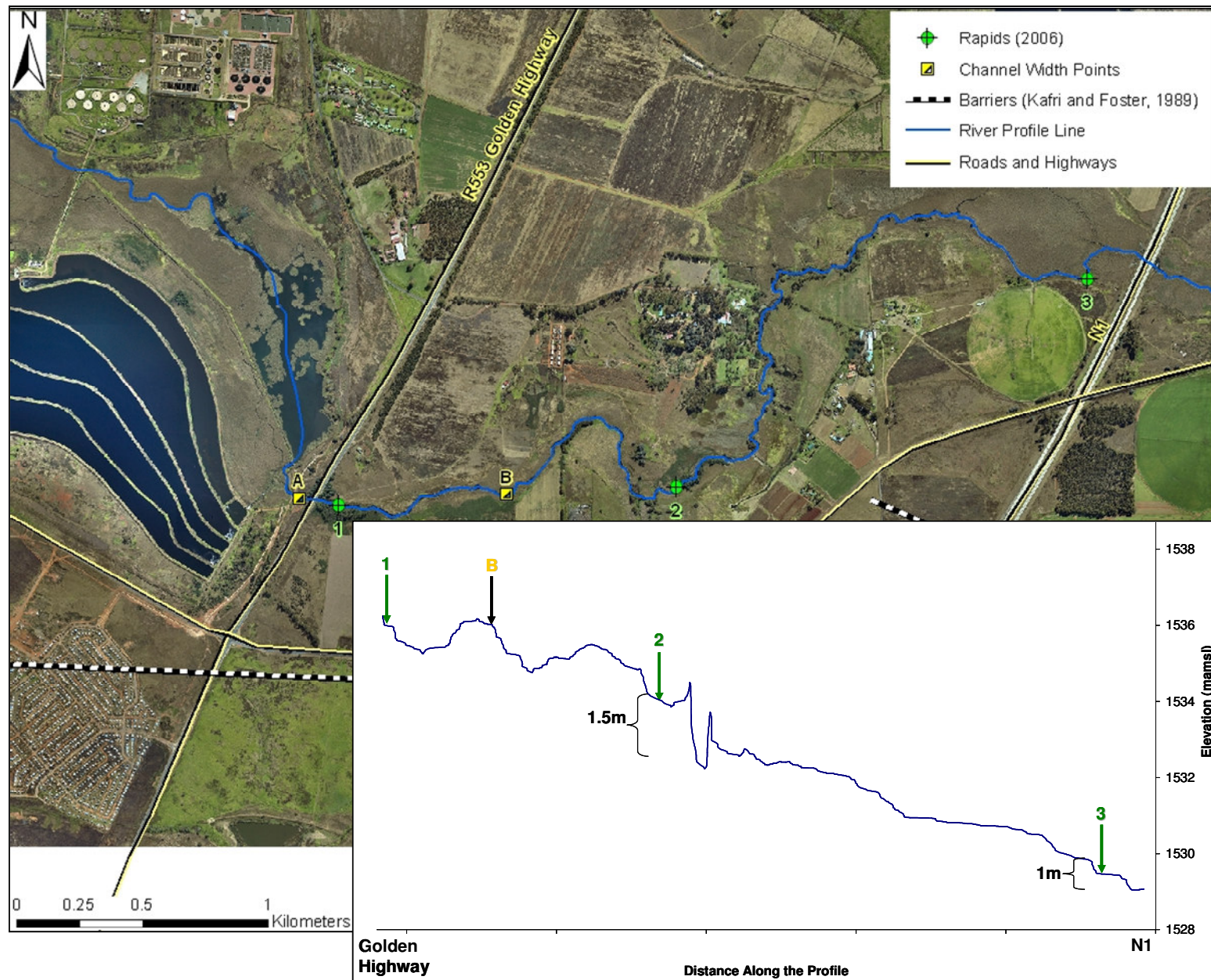
Figure 5.2.3: Long river profile from the Golden Highway to the N1 in relation to 2006 photography.
