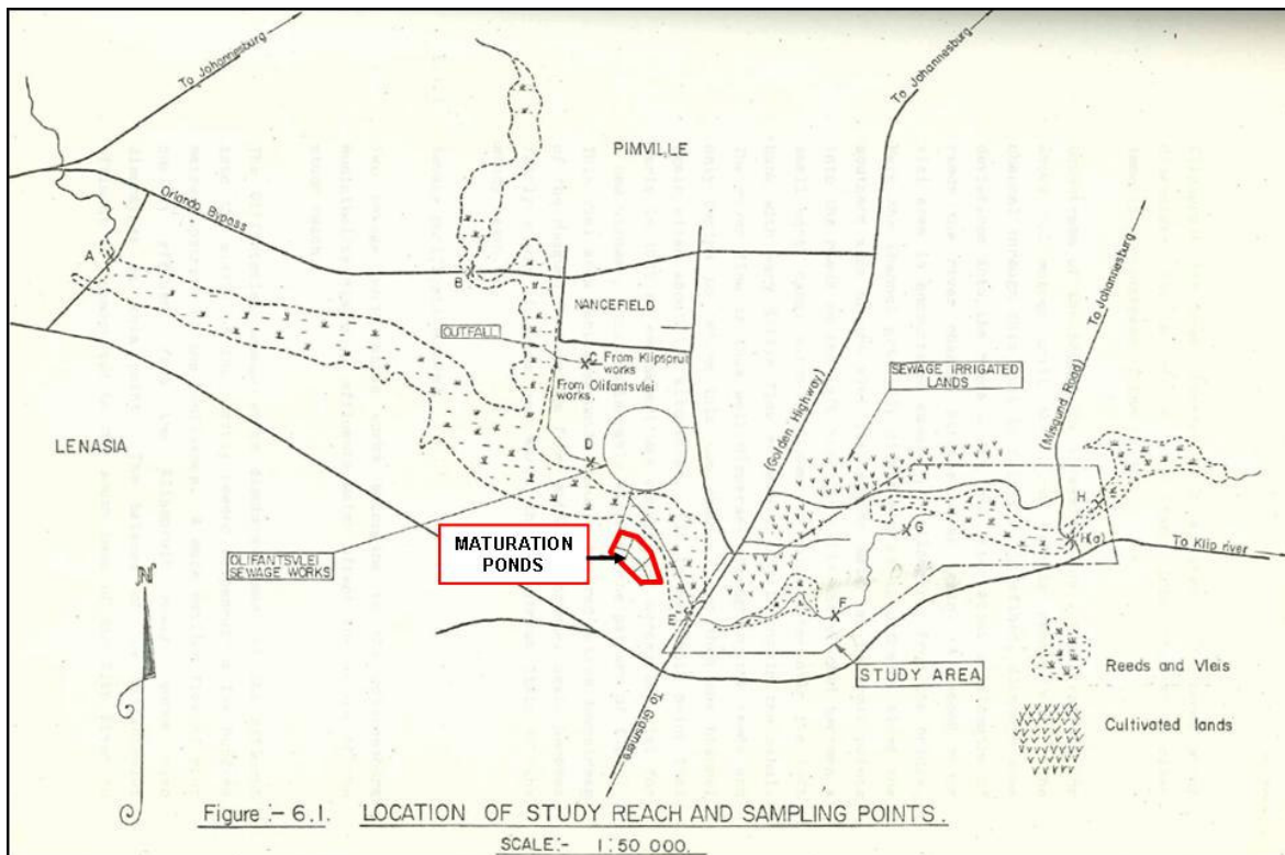
Figure 5.1.10: Study site of Arnold (1980), showing the extent of the wetlands at this time, the maturation ponds and his sampling points (after Arnold, 1980).
