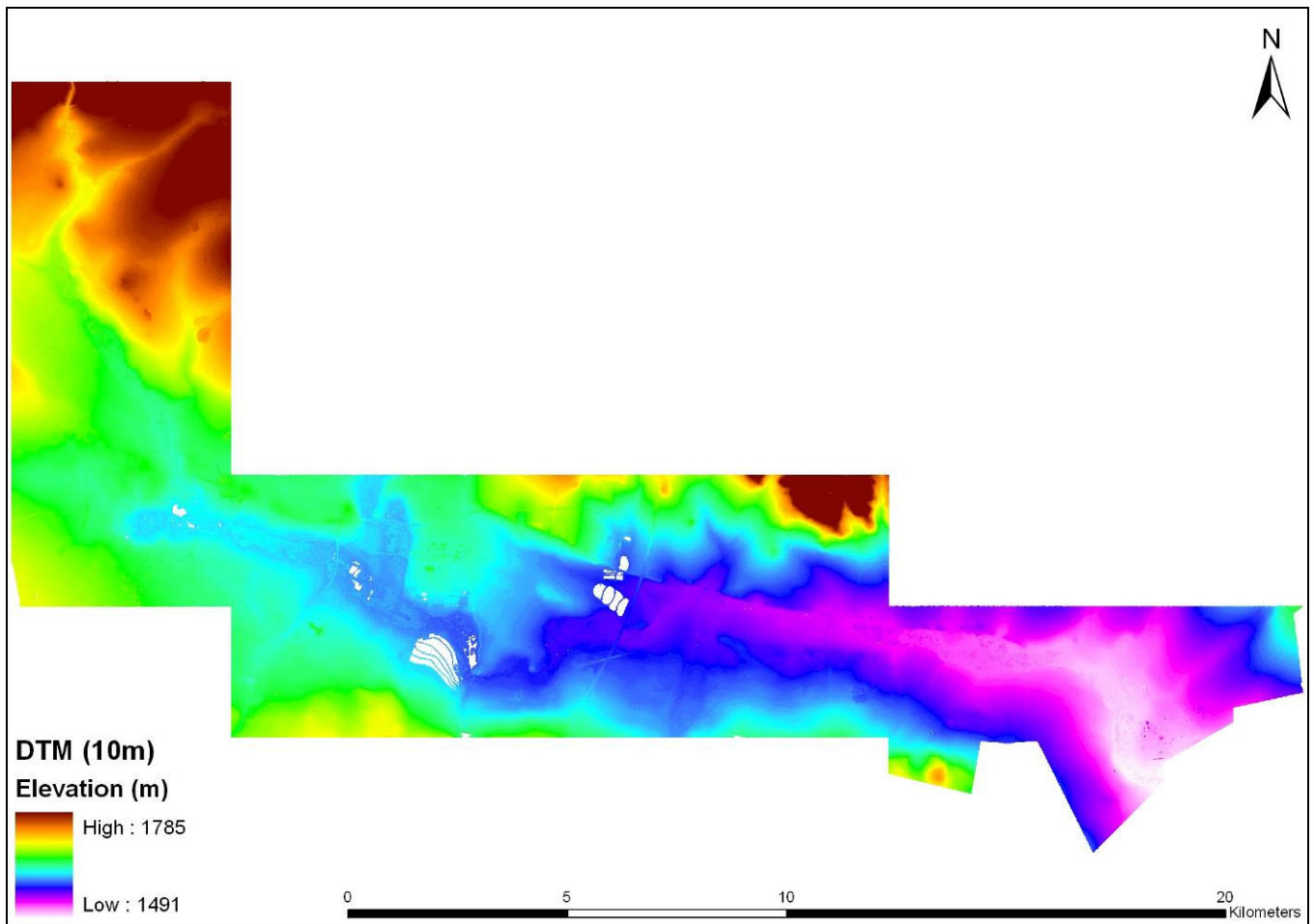
Figure 5.3.2: DTM derived from the original LIDAR point data at 10 m resolution.
