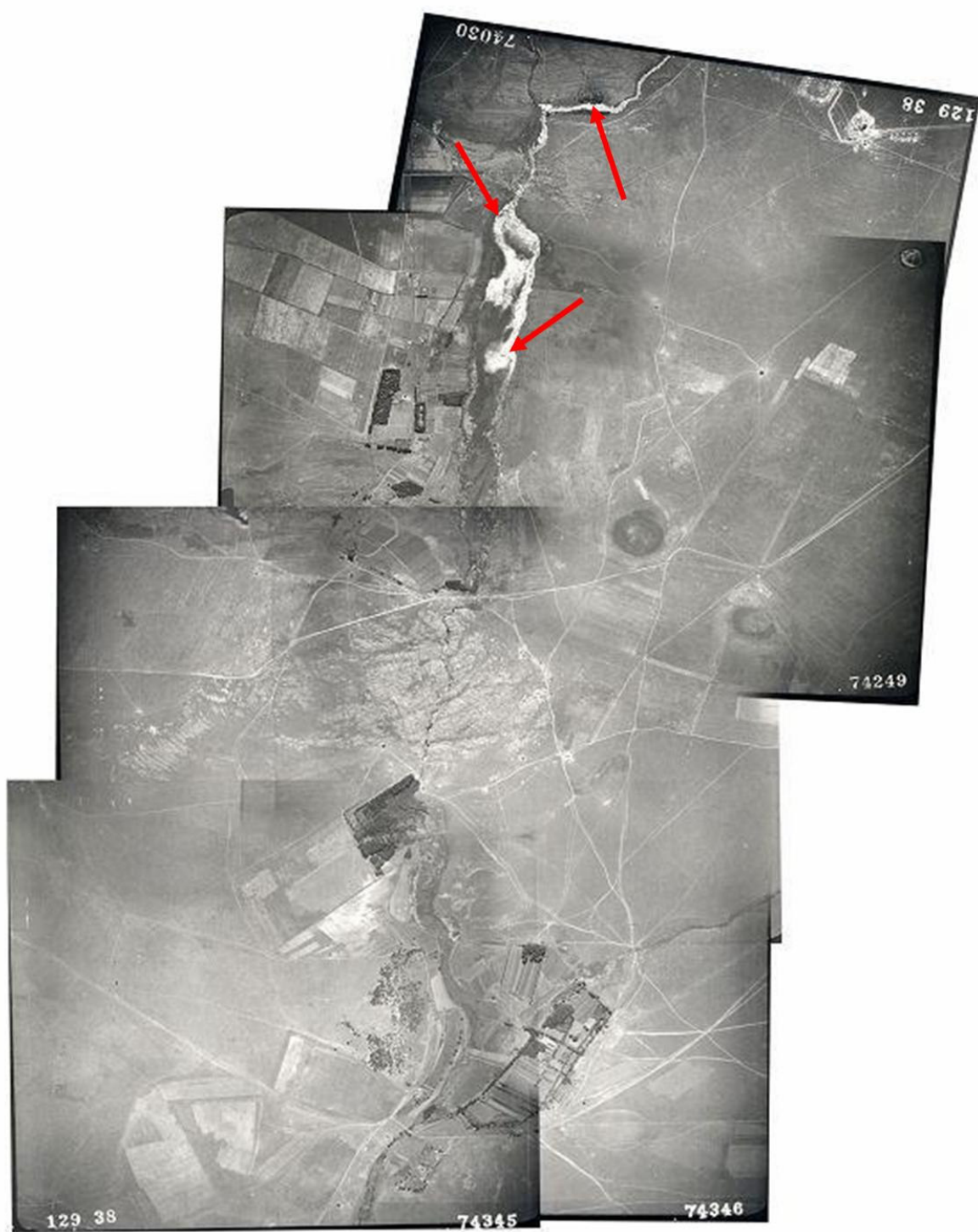
Figure 3.3.1: Acid Mine Drainage during 1938 impacting the Klip River Wetland. Areas impacted indicated by red arrows (Arnold, 2004).
