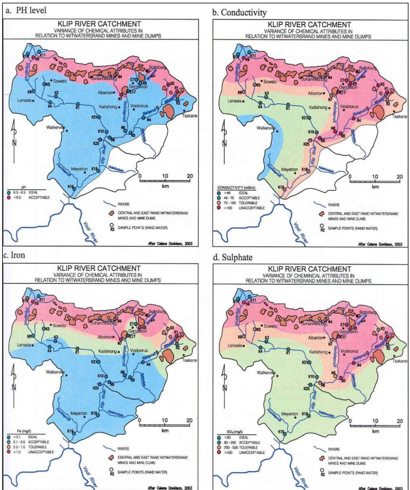
Figure 3.5.1: Klip River catchment showing distribution of a) pH b) conductivity, c) iron and d) sulphate (Davidson, 2003).
