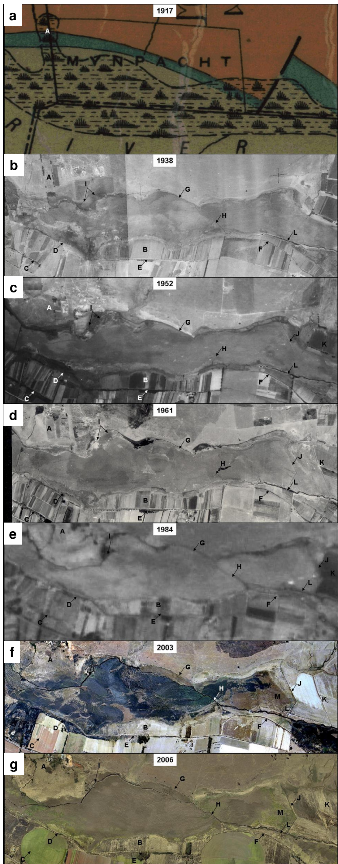
Figure 5.1.19: The wetland downstream of Kibler Park in (a) 1917, (b) 1938, (c) 1952, (d) 1961, (e) 1984, (f) 2003 and (g) 2006.
