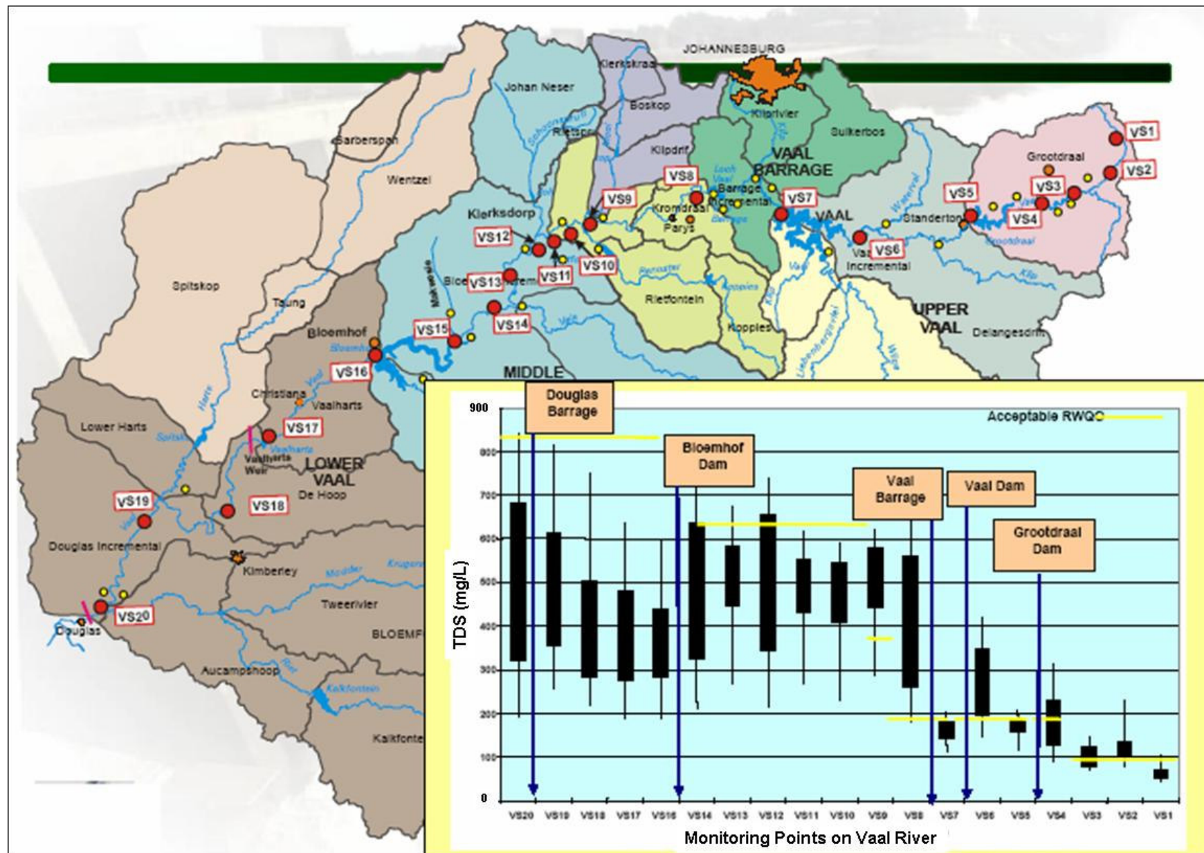
Figure 3.3.3: Total Dissolved Solids concentration map of the Vaal River Basin (DWAf, 2007).
