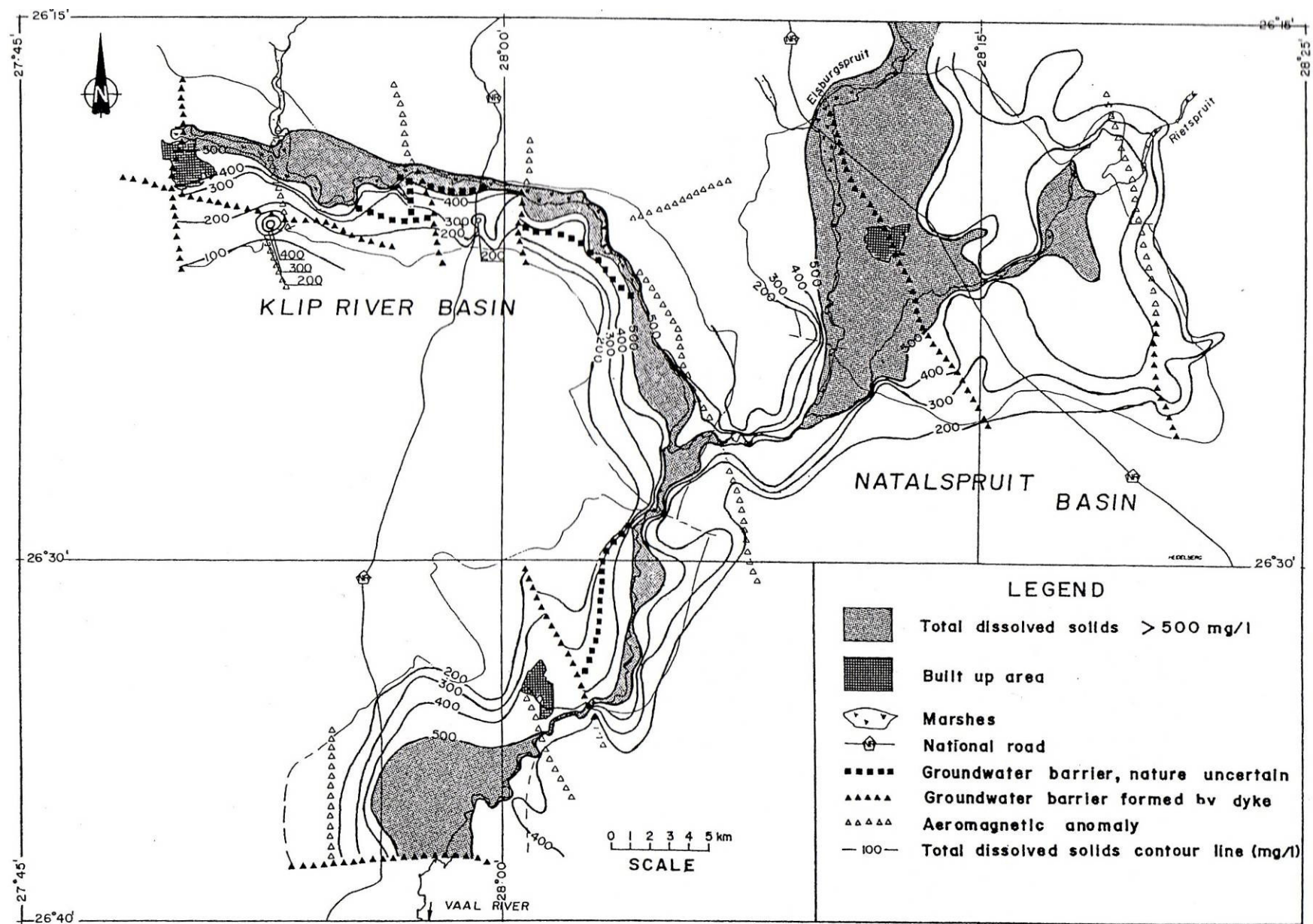
Figure 3.3.2: Total Dissolved Solids concentration map of the Klip River Basin (Kafri and Foster, 1989).
