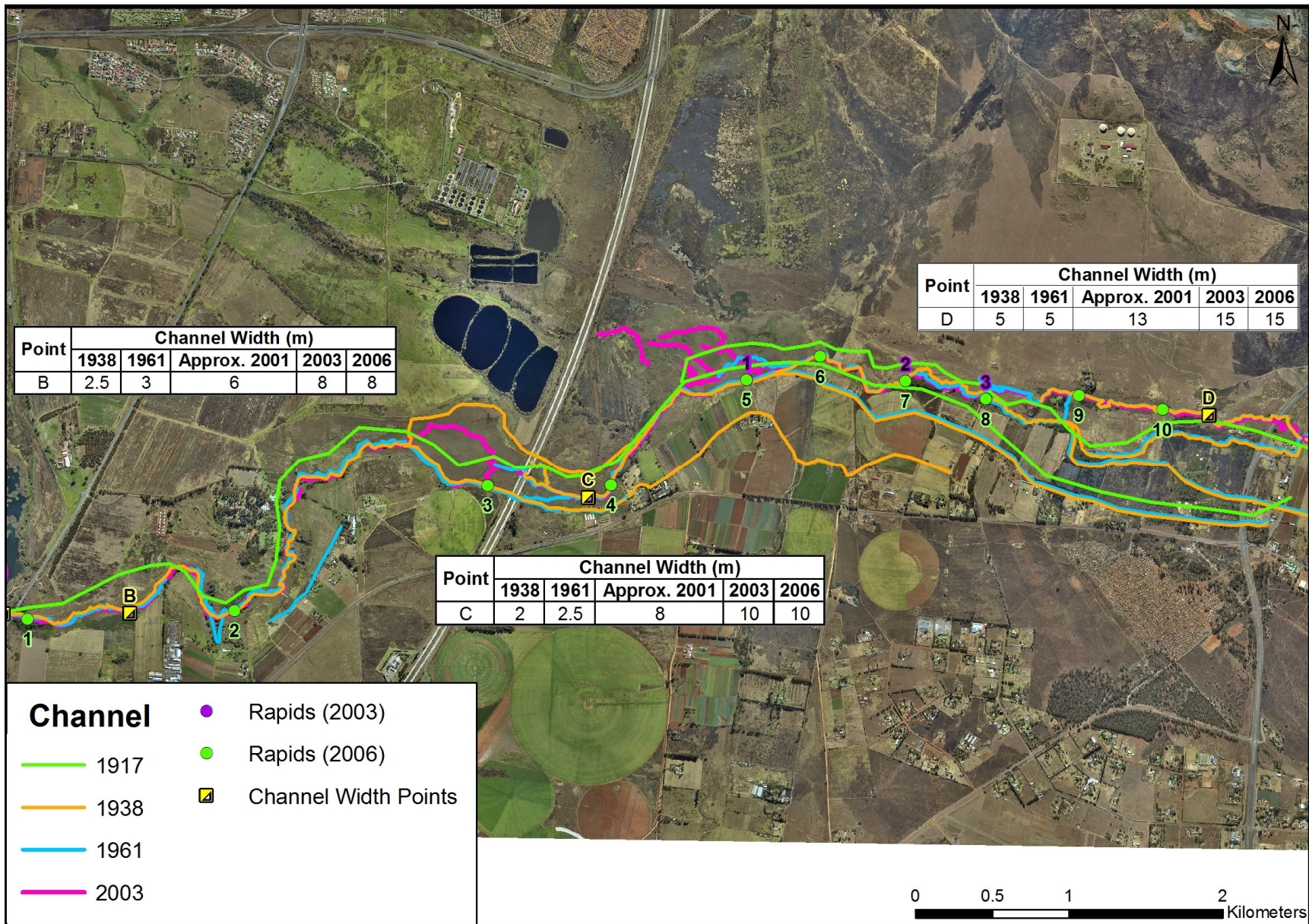
Figure 6.3: Channel formation, propagation and widening from the Golden Highway to Kibler Park between 1917 and 2003.
