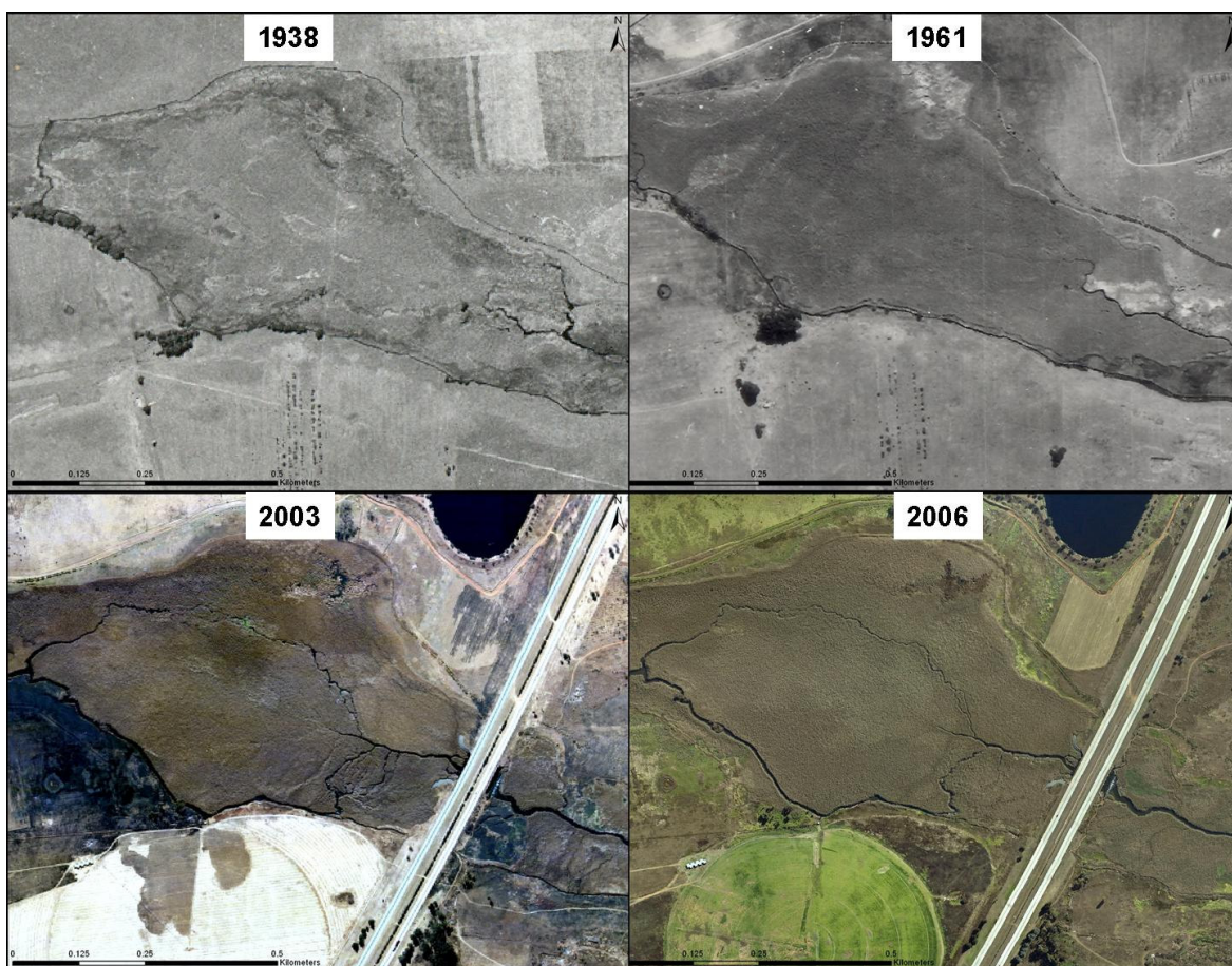
Figure 5.1.12: Detail of the wetland at the N1 Highway in (a) 1938, (b) 1961, (c) 2003 and (d) 2006.
