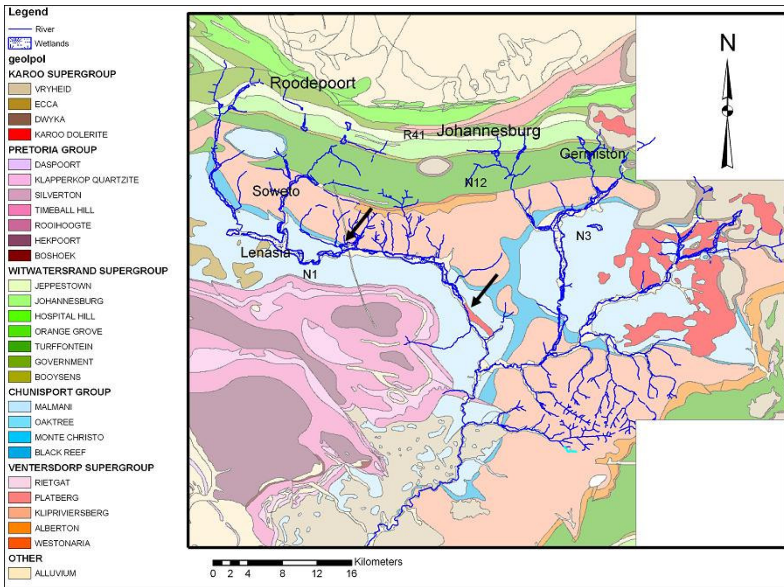
Figure 3.1.2: Surface geology of the Klip River Catchment (black arrows highlight dykes; after Arnold, 2004).
