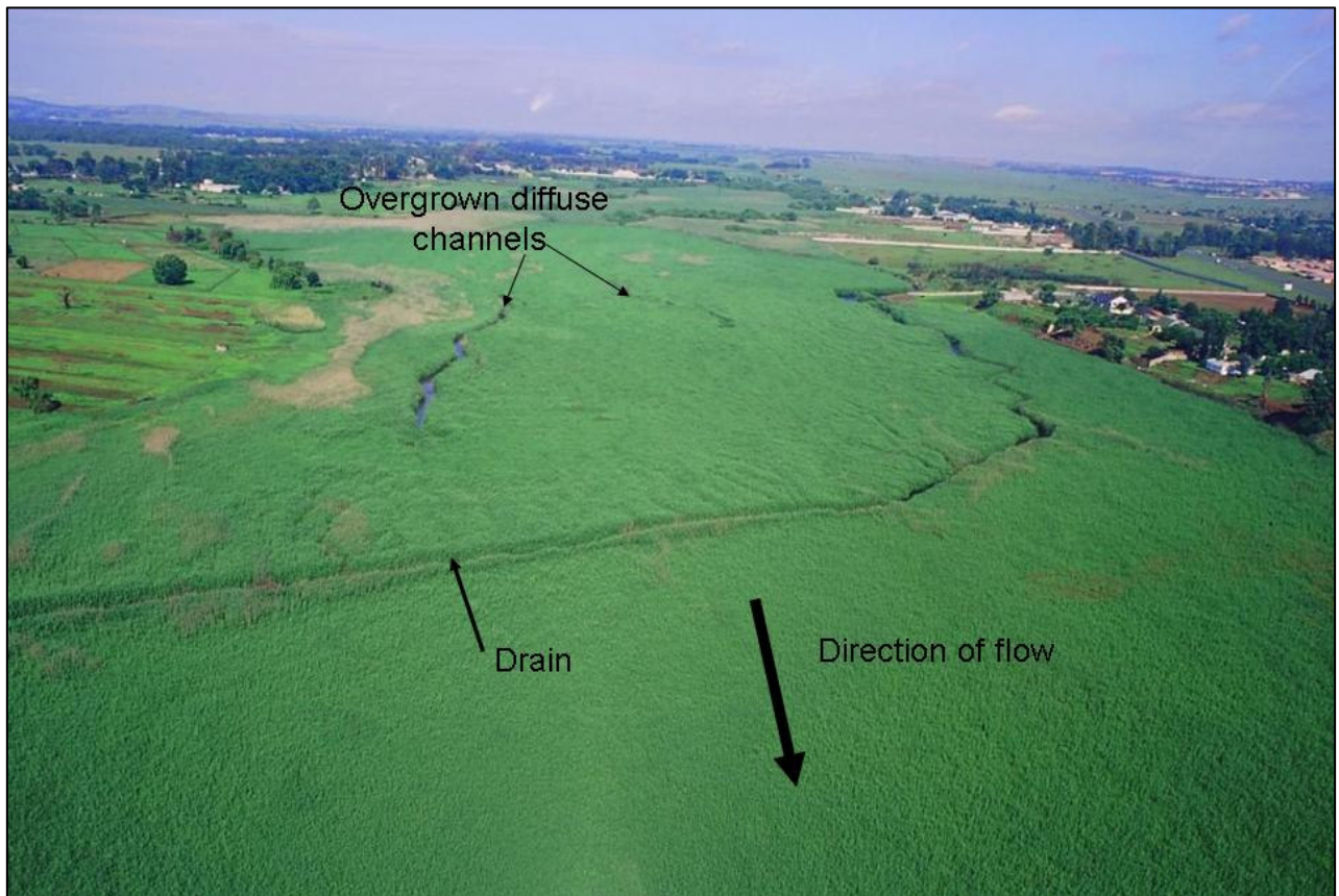
Figure 5.1.18: Diffuse channels as seen in an aerial survey eroding upstream of the drain (courtesy of T.S. McCarthy, November 2007).
