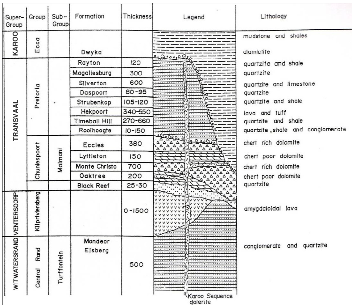
Figure 3.1.3: Lithostratigraphy of the Malmani Subgroup (Kafri and Foster, 1989).
