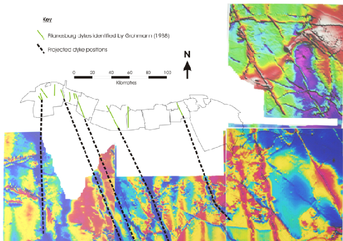
Figure 3.1.5: Aeromagnetic map with dykes projected onto Central Rand Goldfield (Schweitzer et al., 2004).
