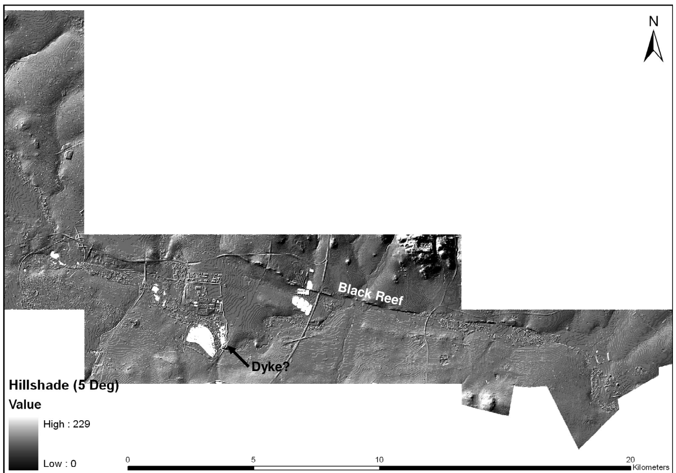
Figure 5.3.3: Hillshade at 5° sun angle derived from the DTM at 10 m resolution.
