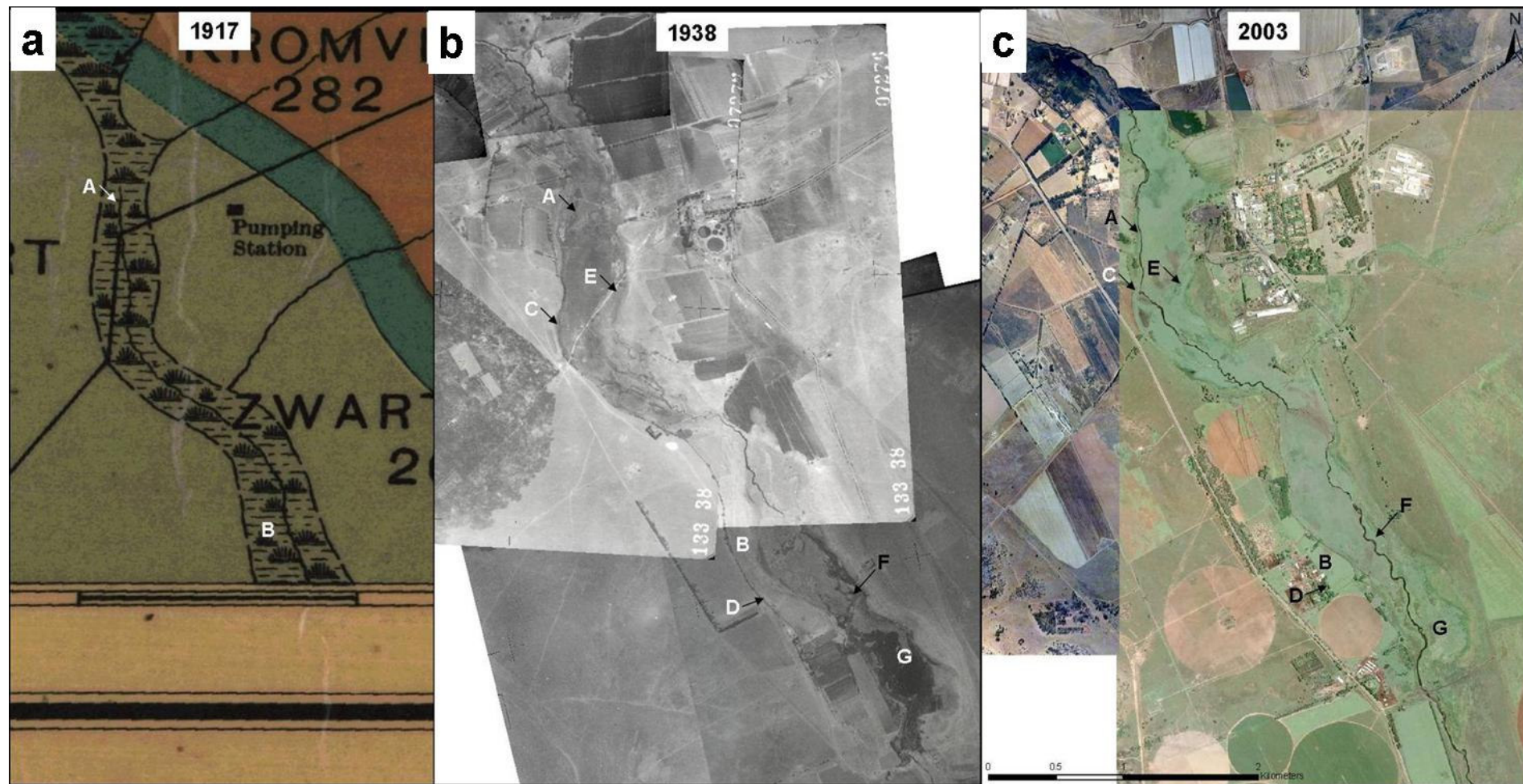
Figure 5.1.20: The wetland of Section 5 in (a) 1917, (b) 1938 and (c) 2003 (a and b have the same scale as c).
