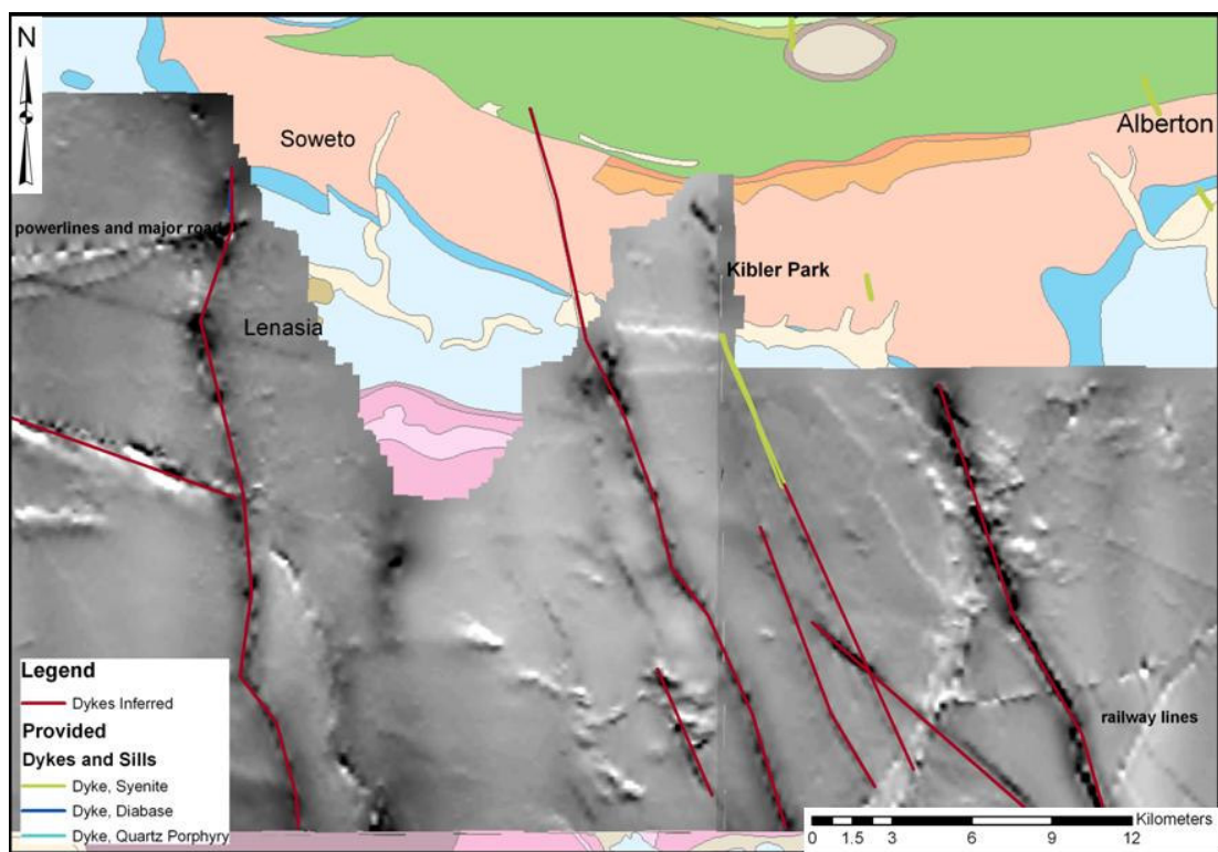
Figure 3.1.4: Aeromagnetic anomaly map with dykes inferred (Arnold, 2004).
