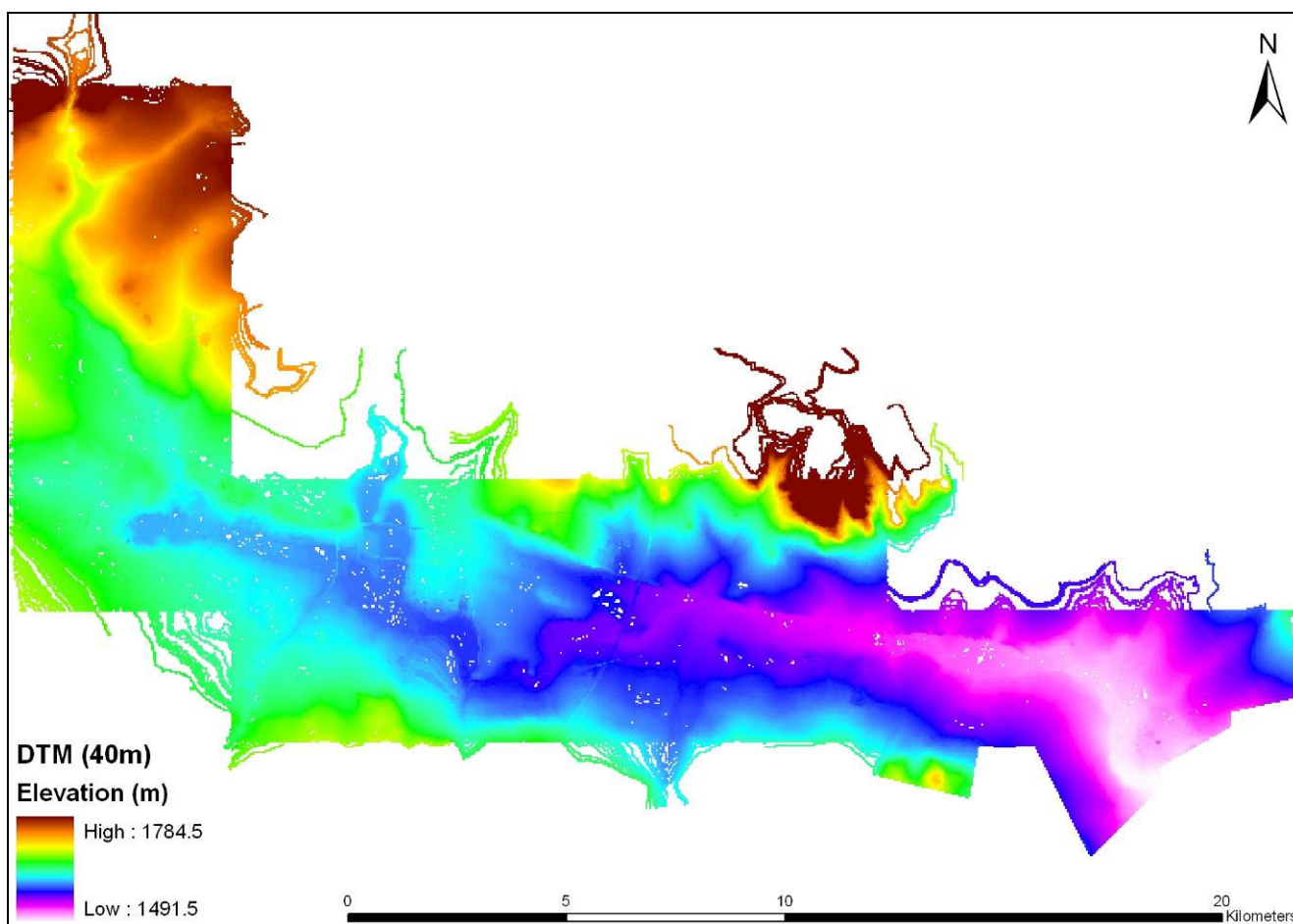
Figure 5.3.1: DTM derived from the contour LIDAR data at 40 m resolution.
