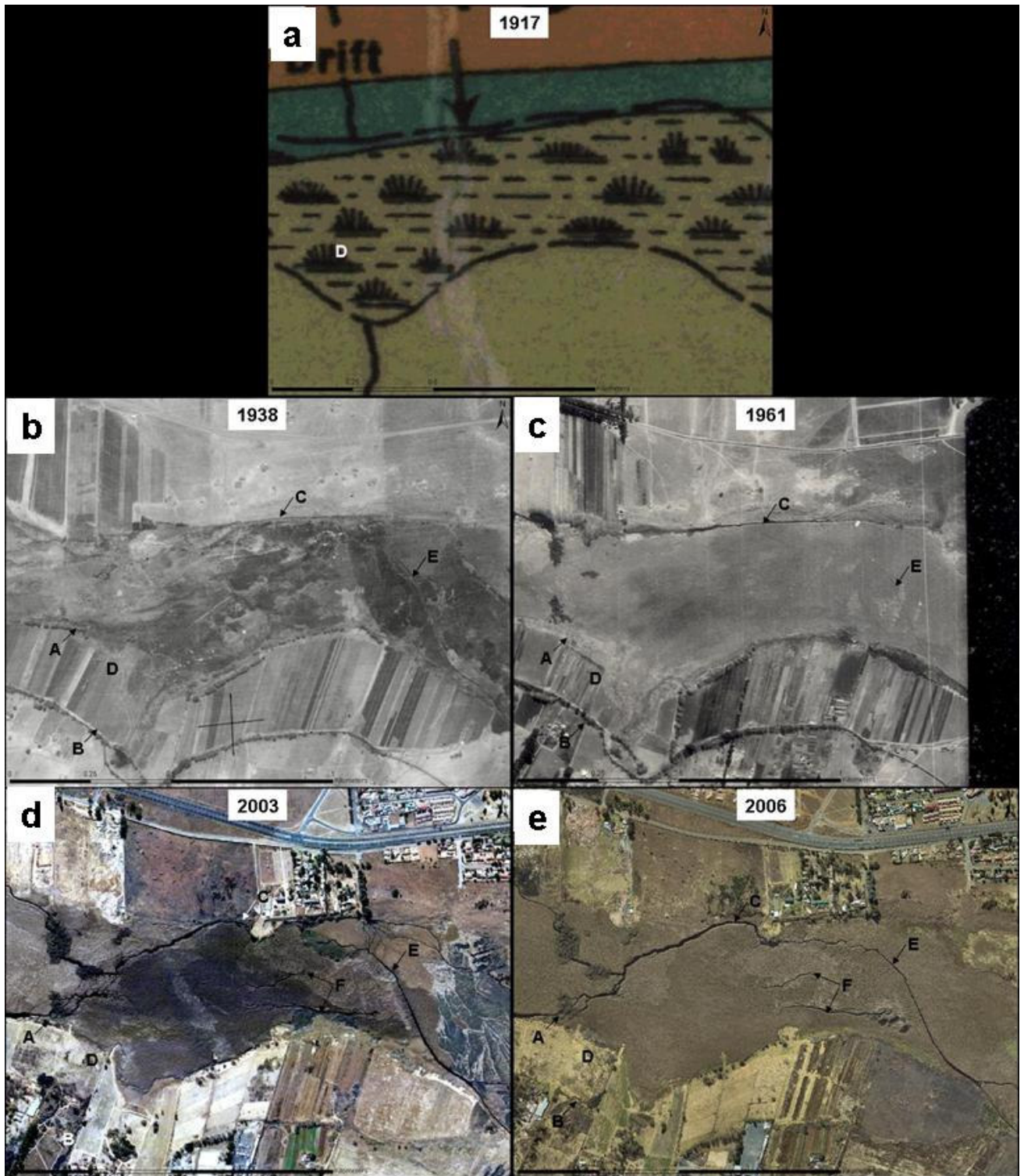
Figure 5.1.17: The wetland south of Kibler Park in (a) 1917, (b) 1938, (c) 1961, (d) 2003 and (e) 2006.
