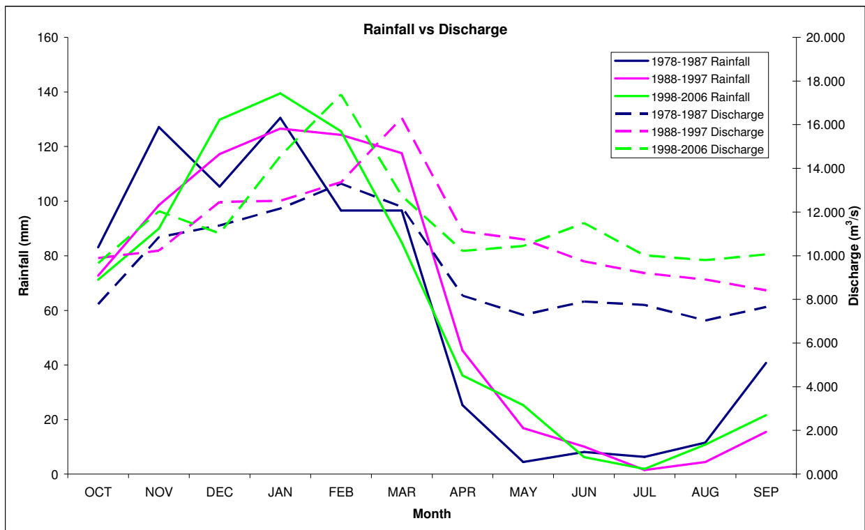
Figure 5.5.5: Water discharge at Witkop Station (C2H141) per month compared to rainfall data (OR Tambo Airport).
