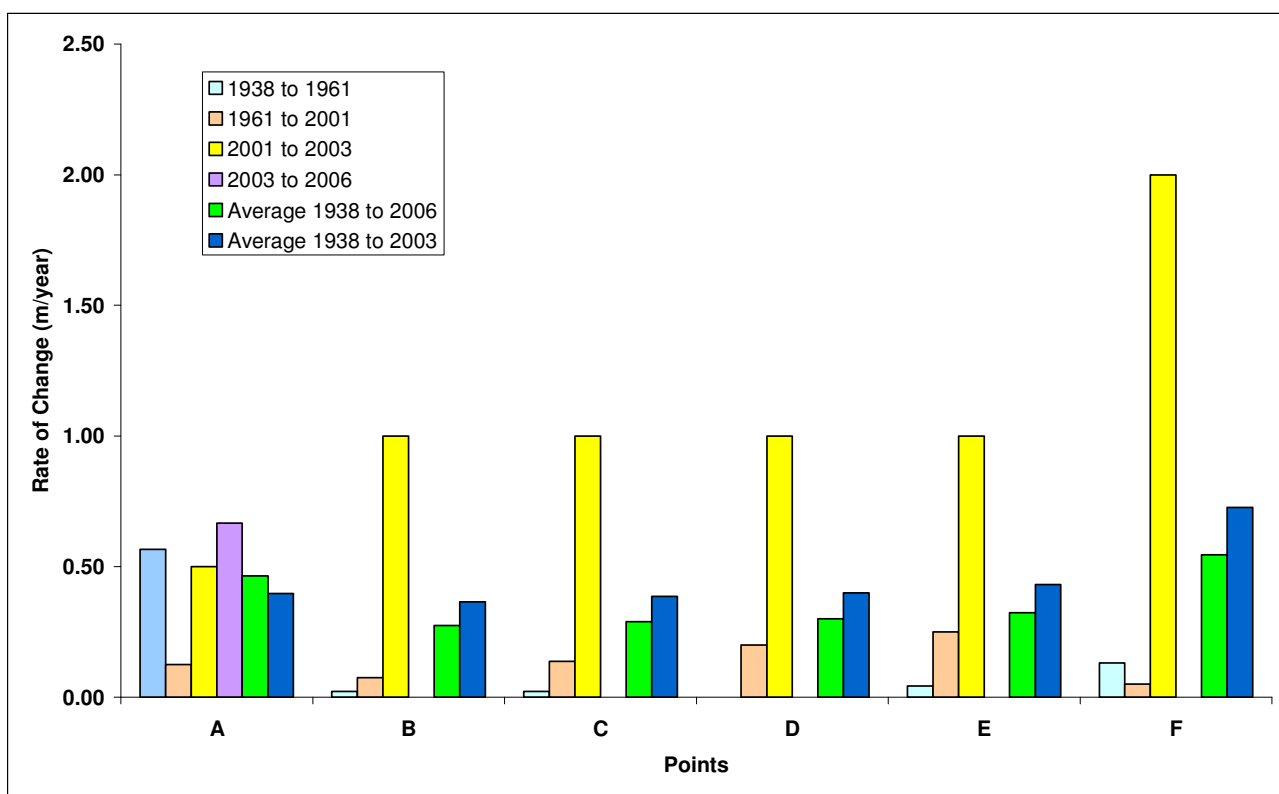
Figure 5.1.5: Rate and average rate (m/year) of change of channel width over time.
