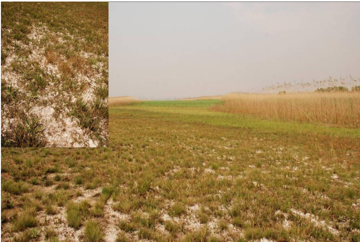
Figure 5.1.7: Gypsum crust accumulated on the banks of the Klip River Wetland at Lenasia.
