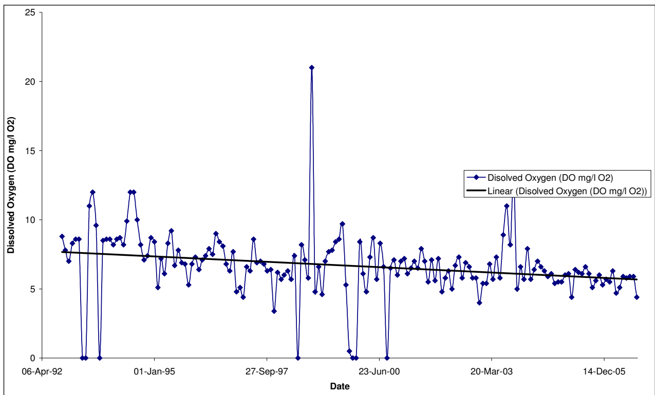
Figure 5.4.4: K21 dissolved oxygen levels from 1992 to 2006.
