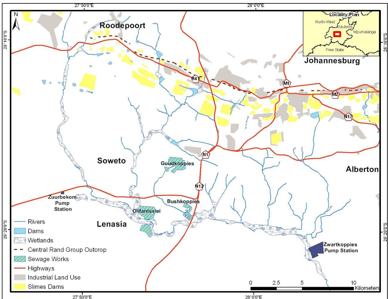
Figure 1.1: Location of the Klip River Wetland in relation to industrial, urban and mining development in the Johannesburg area.
