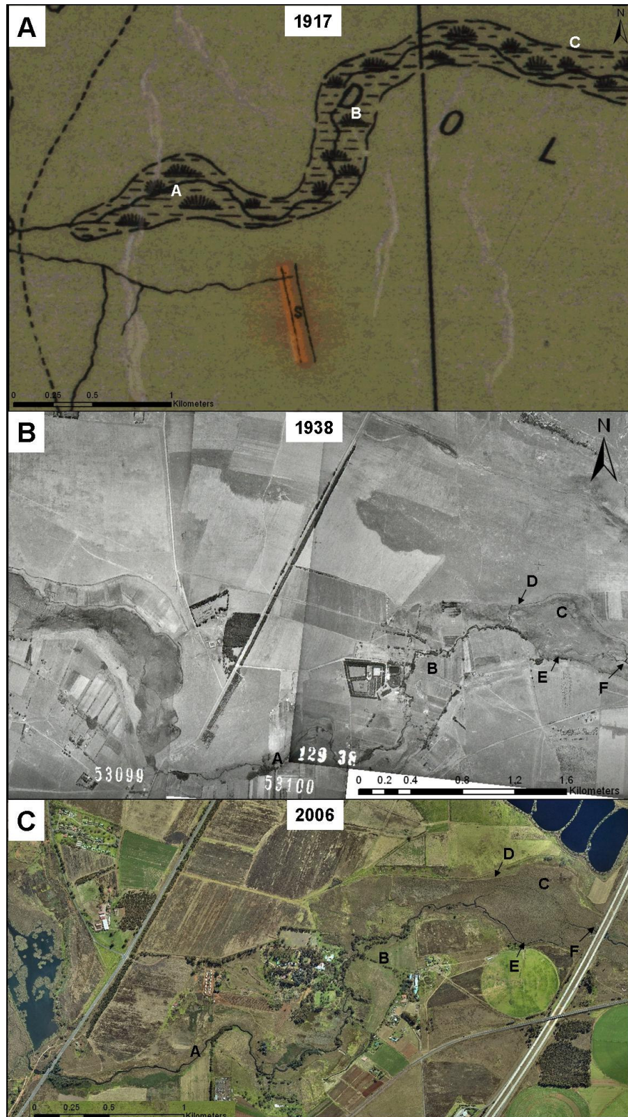
Figure 5.1.11: The wetland between the Golden Highway and the N1 in (a) 1917, (b) 1938 and (c) 2006.
