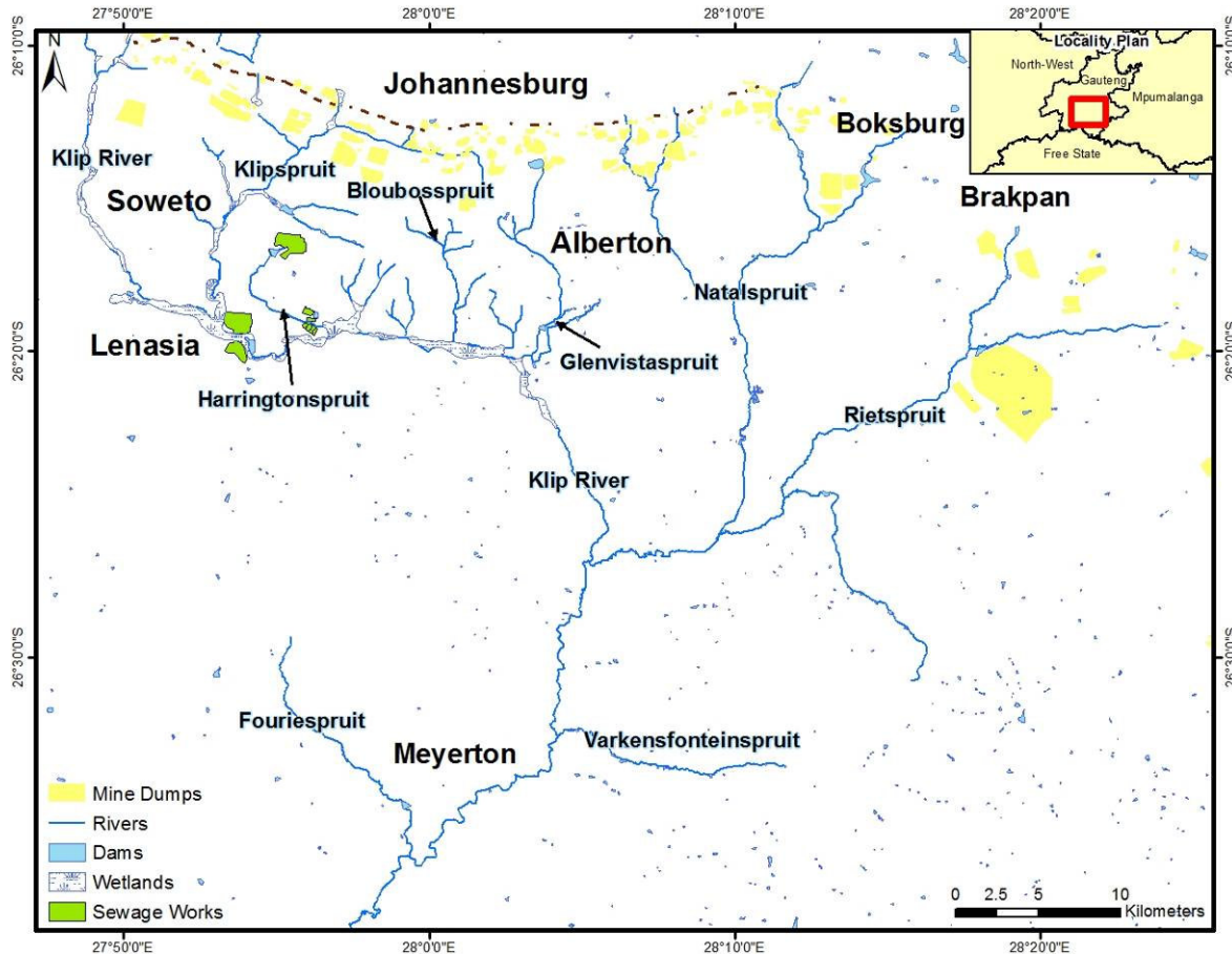
Figure 3.1.1: Location of the river system and water resources around the Klip River Wetland.
