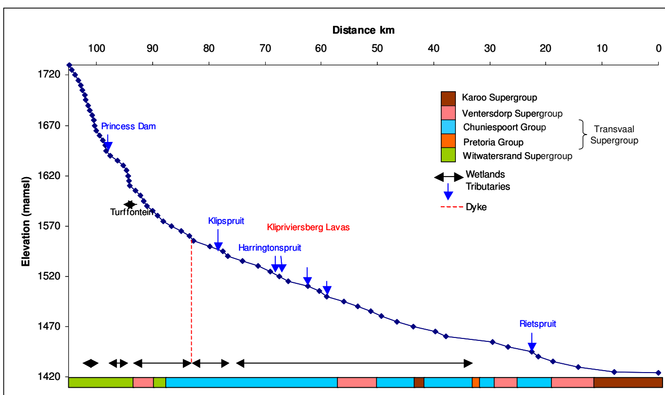
Figure 5.2.1: Long river profile as recorded from 1 : 10 000 orthophotos (after Arnold, 2004).
