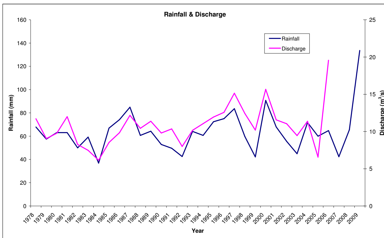
Figure 5.5.4: Water discharge at Witkop Station (C2H141) between 1977 and 2006 compared to rainfall data (OR Tambo Airport).
