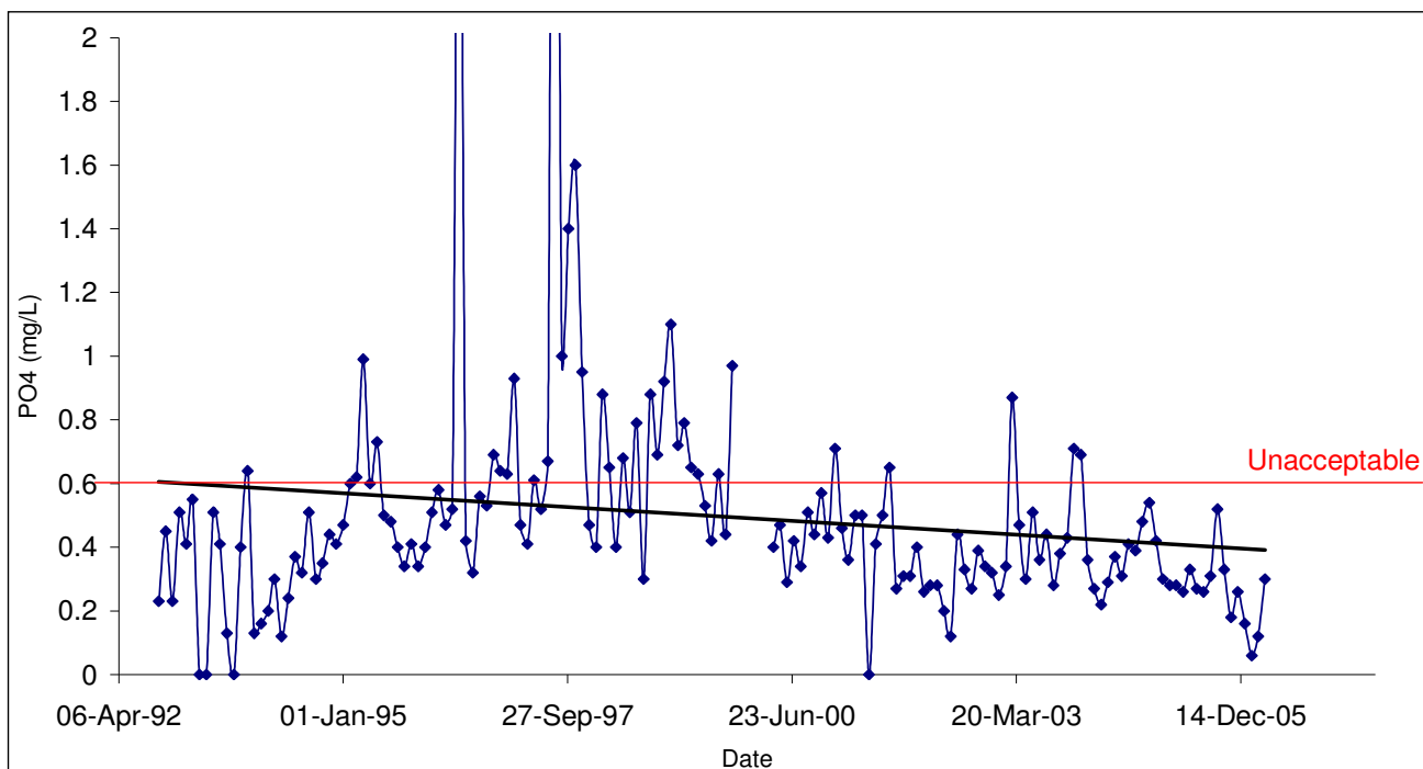
Figure 5.4.1: K21 phosphate levels from 1992 to 2006 (acceptability according to DWAF domestic water quality standards).
