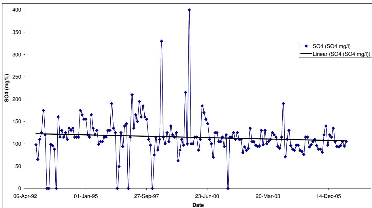
Figure 5.4.2: K21 sulfate levels from 1992 to 2006.
