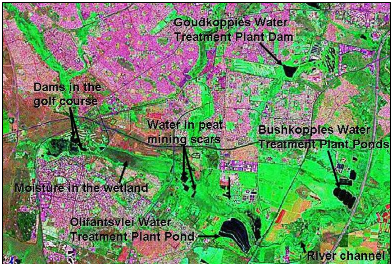
Figure 5.1.2: Landsat image showing the water and moisture content of the wetland.
