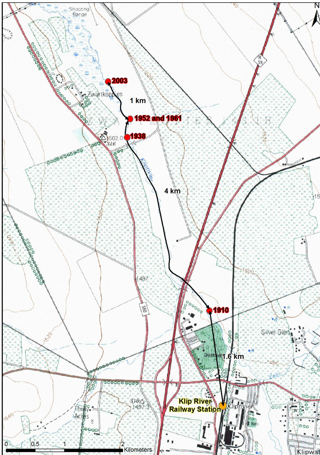
Figure 5.1.21: Wetland retreat from the Klip River Railway Station between 1910 and 2003.
