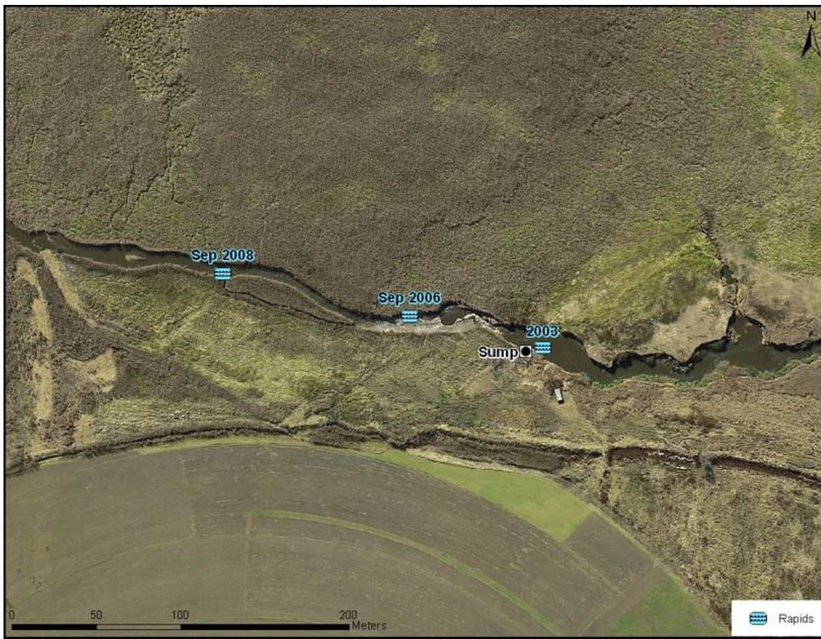
Figure 5.2.7: Knick point migration between 2003 and 2008 at Point 16.
