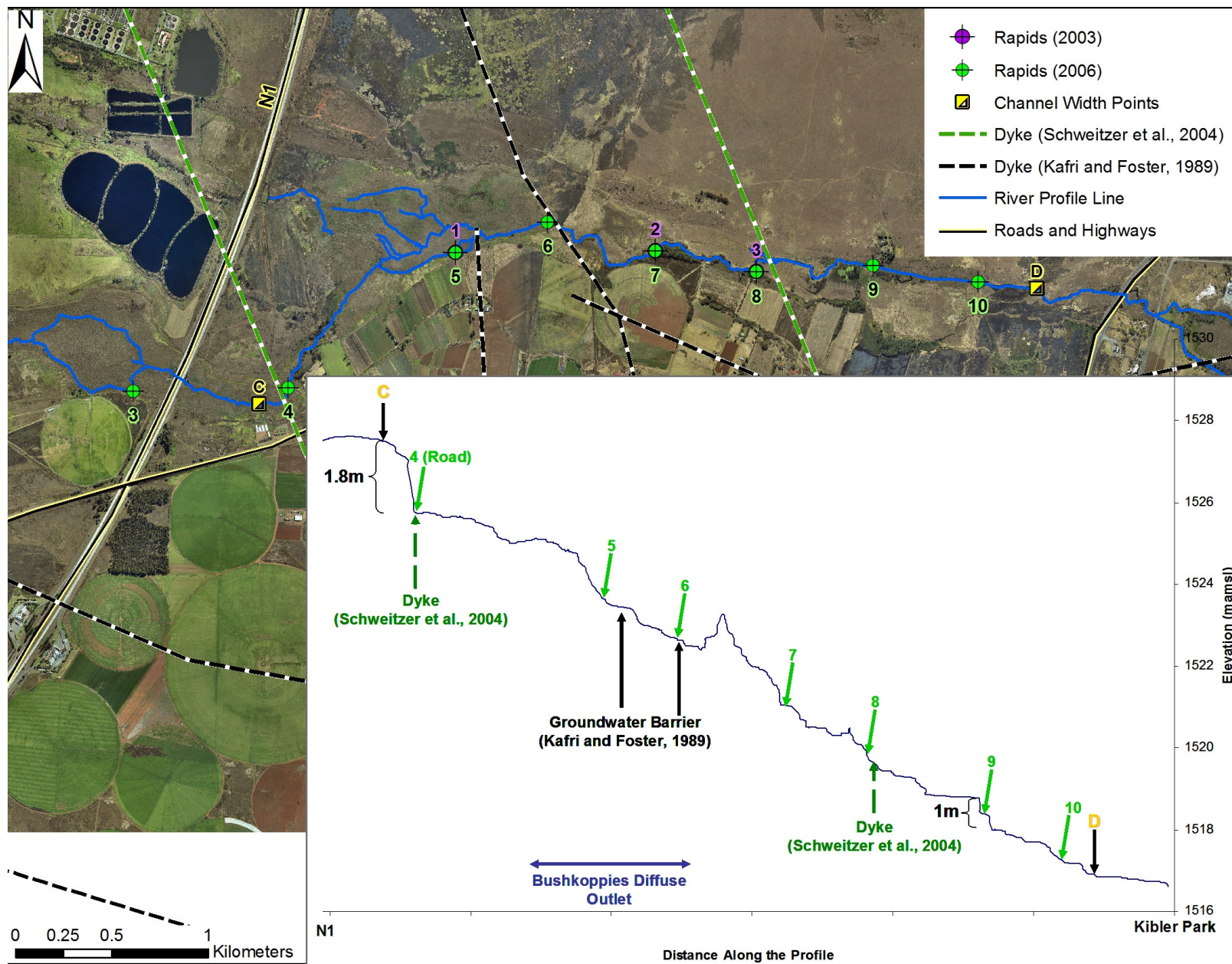
Figure 5.2.4: Long river profile from the N1 Highway to Kibler Park in relation to 2006 photography.
