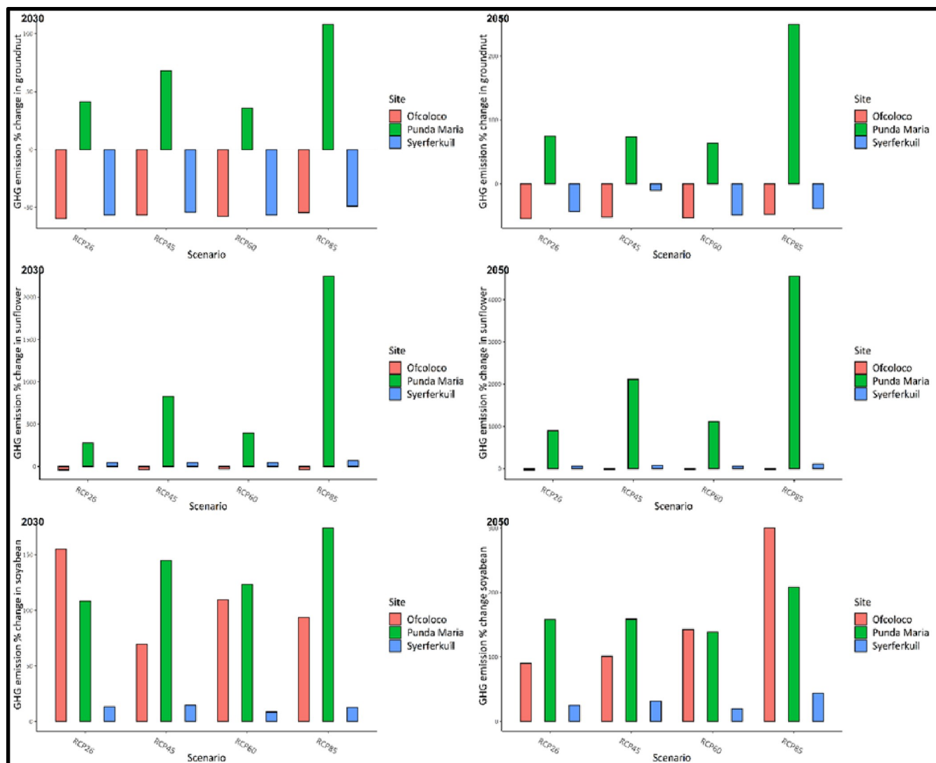
Fig 8. Predicted climate change impacts on GHG emission percentage change on groundnuts, sunflower and soybean production at Ofcoloco, Syferkuil and Punda Maria, Limpopo, South Africa by 2030 and 2050 under four climate change scenarios.
