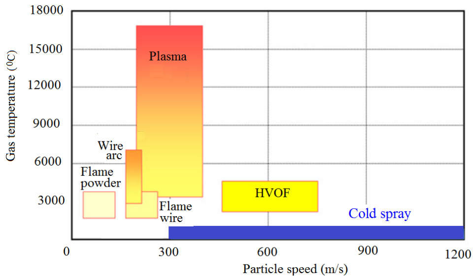
Figure I.1: Comparison between CS and thermal spray processes.
