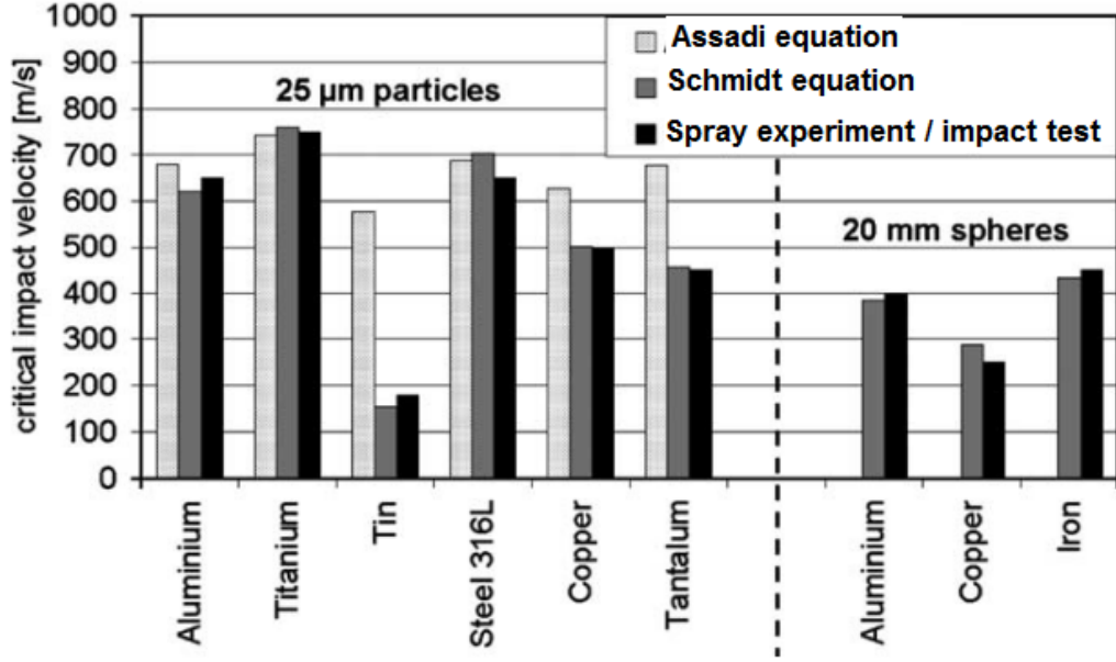
Figure L.8: Calculated and experimental critical velocities Source: (Schmidt et al., 2006)
