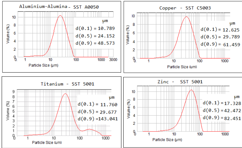
Figure 4.4: Size distributions of powders for strategy 1.
