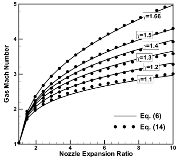
Figure L.11: Variation of Mach with nozzle expansion.
