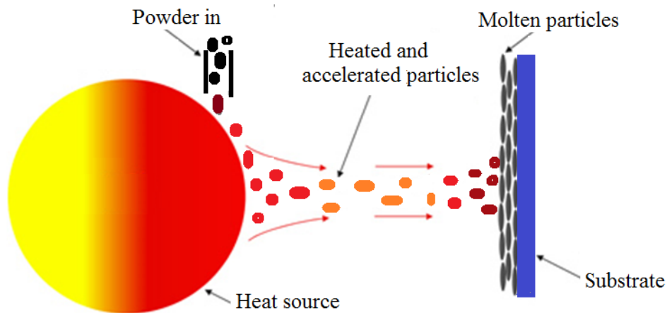
Figure H.6: Thermal spray process.
