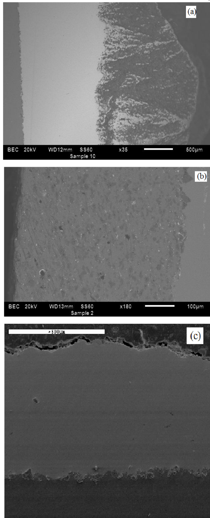
Figure P.10: Coatings for individual powders. Coatings: (a) Aluminium (b) copper (c) zinc 197
