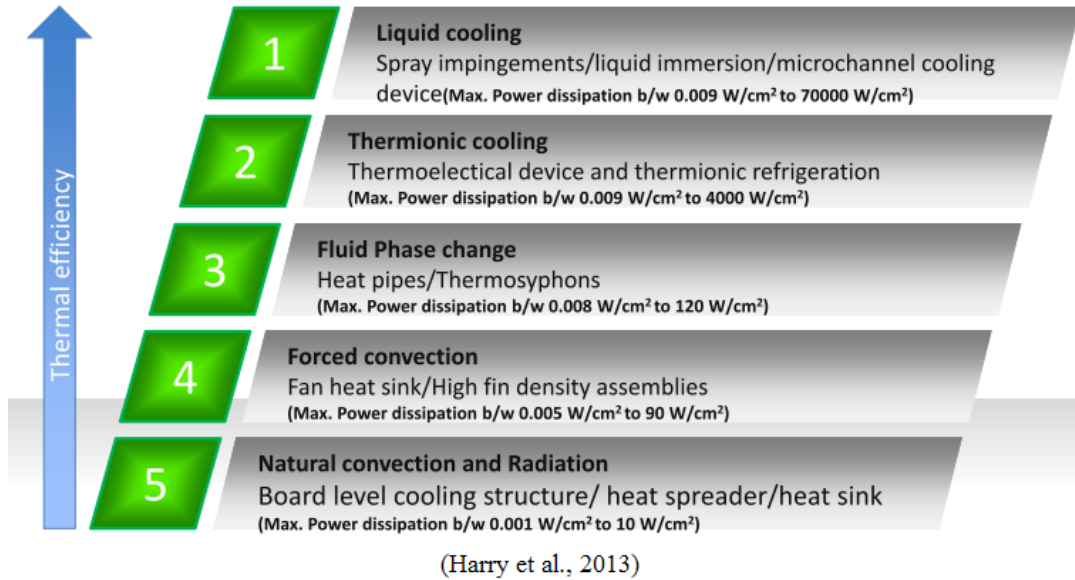
Figure C.1: Thermal solutions hierarchy.
