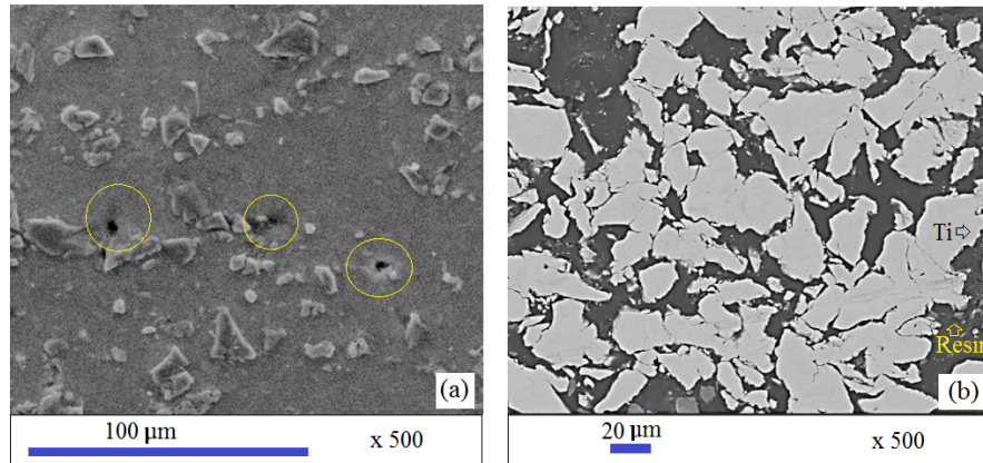
Figure 4.6: Coatings under sub-optimised conditions. (a) Aluminium-alumina, (b) titanium
