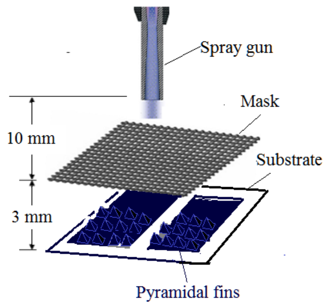
Figure 3.4: Pyramidal fins fabrication.
