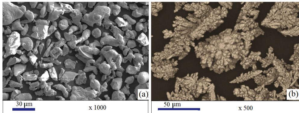
Figure 4.2: Morphology of aluminium and copper powders.
