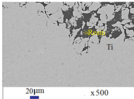
Figure 4.8: Titanium coating under optimised conditions.
