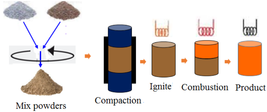
Figure 2.6: Self propagating synthesis process.
