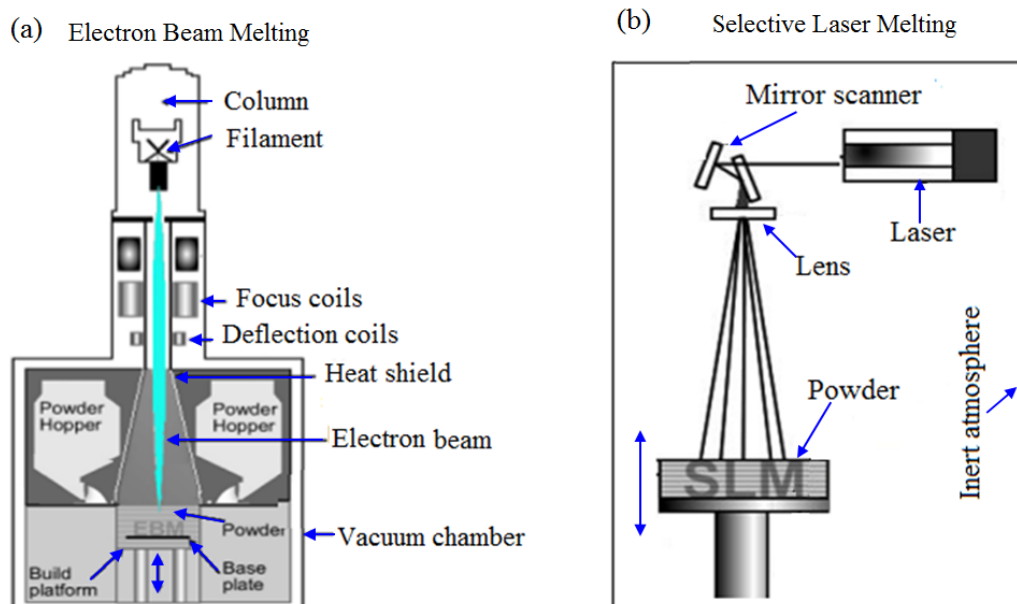
Figure H.13: Electron beam and selective laser melting.
