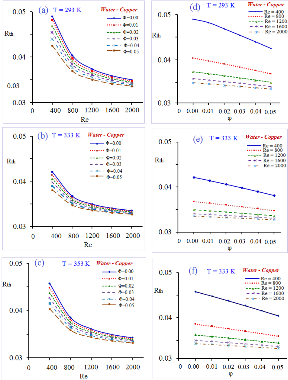
Figure O.5: Variation of thermal resistance for copper nanofluids.
