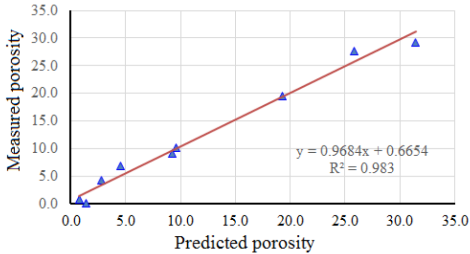
Figure 4.9: Measured Vs. predicted porosity for titanium.
