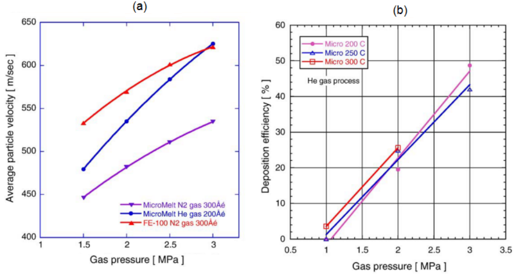
Figure L.4: Effect of gas pressure.
