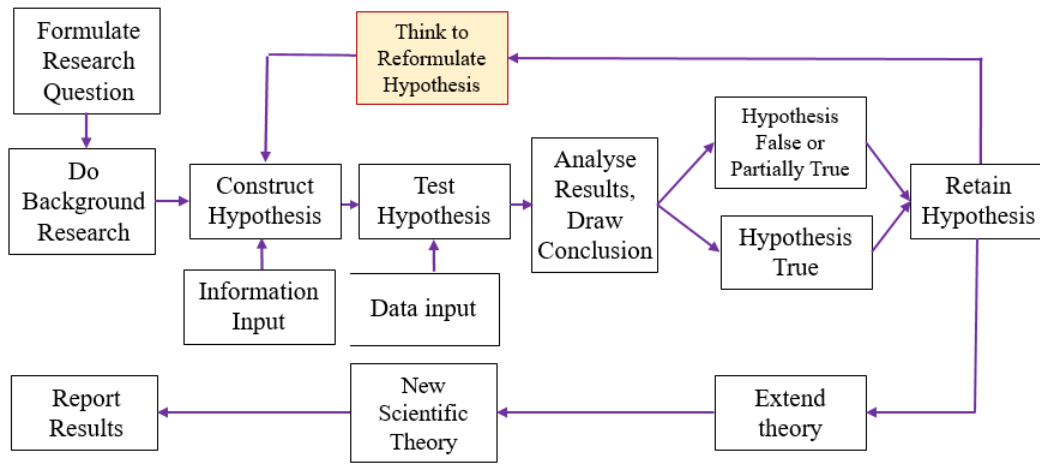
Figure 5.2: Hypotheses loop.
