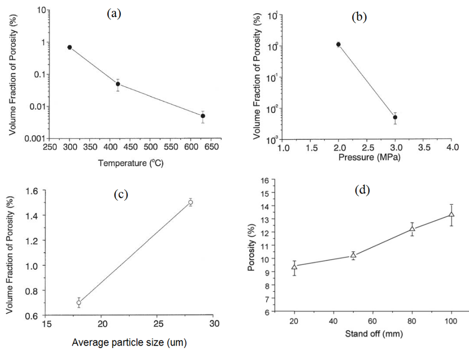
Figure I.5: Porosity minimisation in CS coatings.
