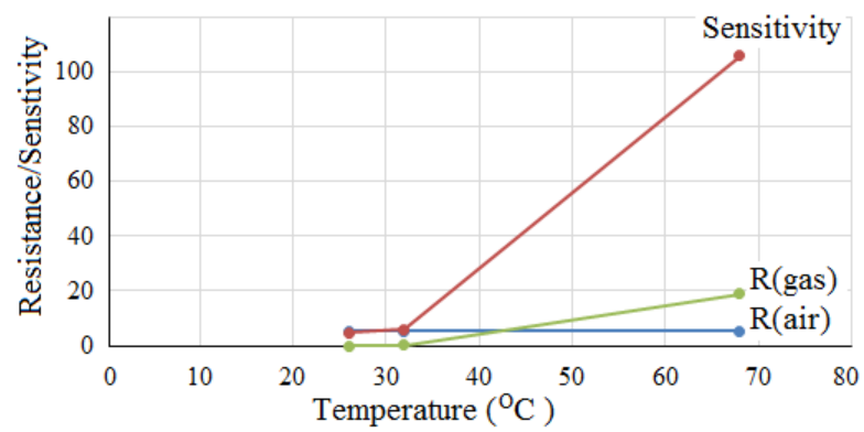
Figure 4.20: Graph for gas sensor sample 2.
