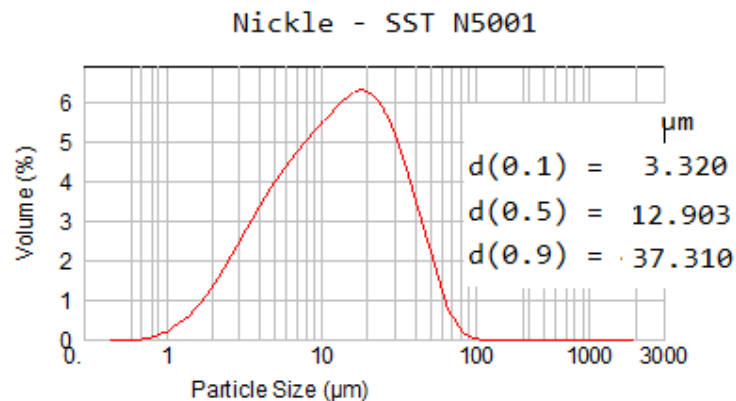
Figure P.5: Particle size distribution for nickel powder.
