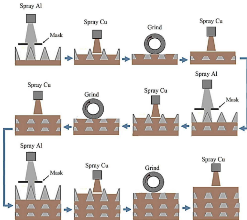
Figure J.4: Fabrication process for microchannels.
