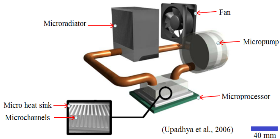
Figure C.2: Microfluidic cooling architecture.
