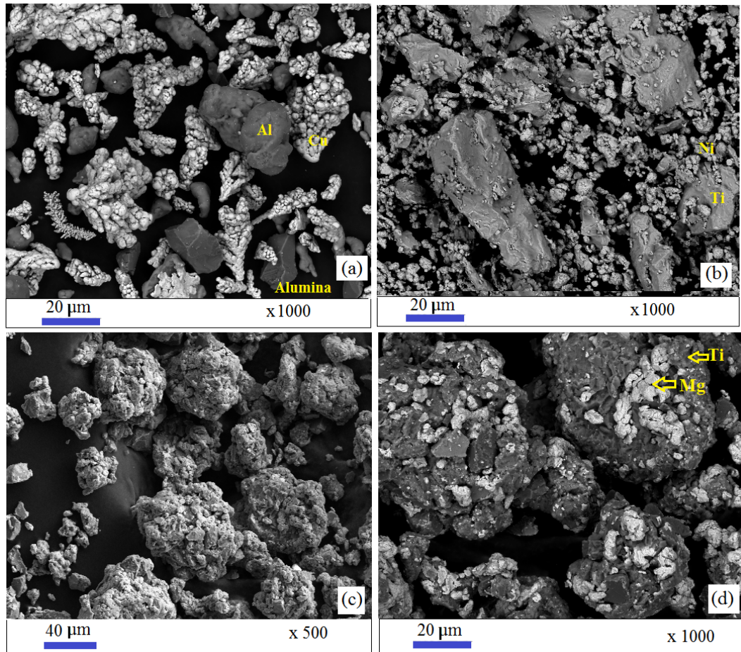
Figure 4.10: Morphology of powder mixtures. (a) Al-Alumina-Cu, (b) Ti-Ni, (c) Al-Alumina-Zn, and (d) Ti-Mg.
