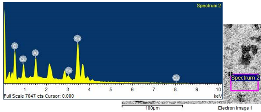
Figure 4.16: EDX spectra for gas sensing layer.
