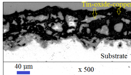
Figure 4.14: Tin-oxide-copper coating.
