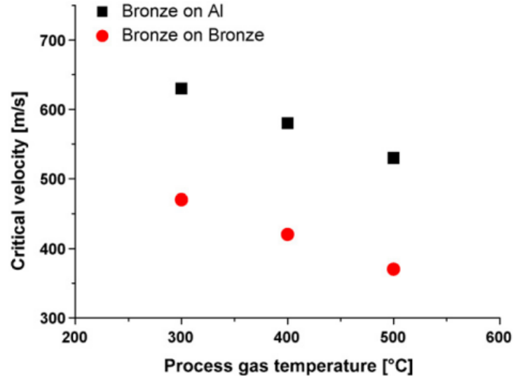
Figure L.3: Critical velocity Vs. process gas temperature.
