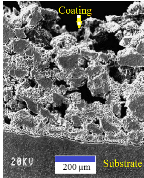
Figure H.8: Plasma spray coating Source: (Ryan et al., 2006).
