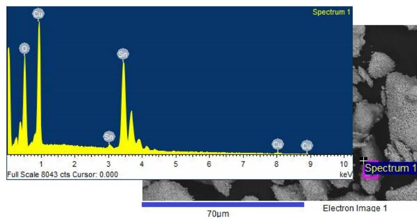
Figure 4.17: EDX spectra for gas sensing layer.
