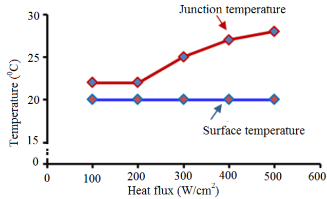
Figure 4.25: Graph of temperature Vs. heat flux.
