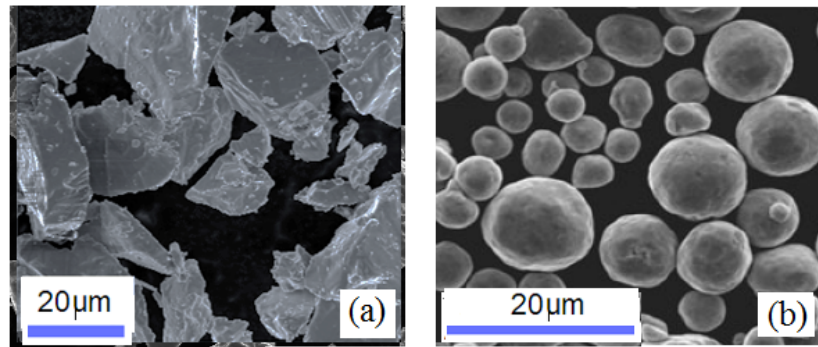
Figure L.13: Particle morphology.
