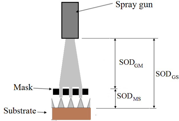
Figure J.3: Cold spray through mask
