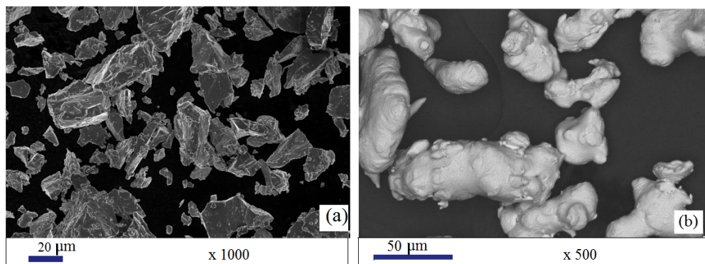
Figure 4.3: Morphology of titanium and zinc powders.
