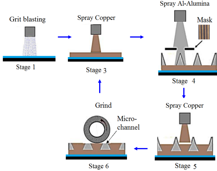
Figure 3.5: Fabrication of microchannels.
