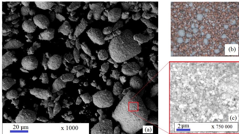
Figure 4.11: Tin-oxide-copper agglomerates. (a) Agglomerated, (b) Mixture, (c) Magnified view.
