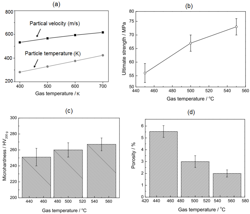
Figure L.1: Effect of stagnation gas temperature.
