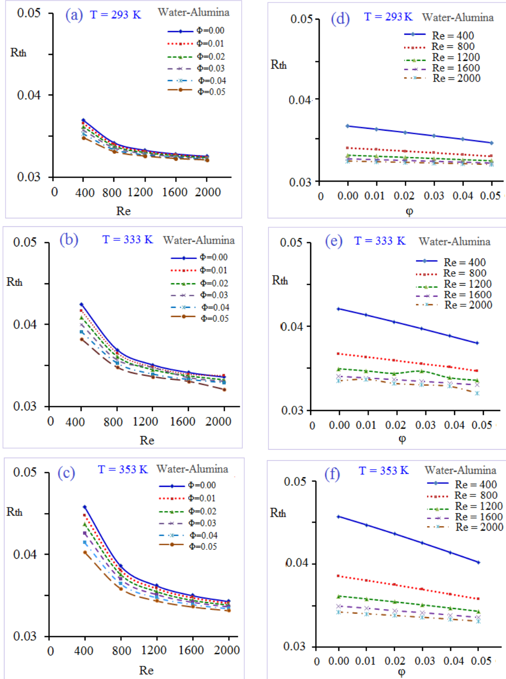
Figure O.4: Variation of thermal resistance for alumina nanofluids.
