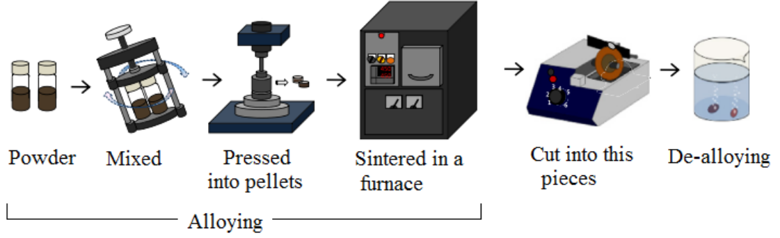
Figure 2.5: Alloy-de-alloy process.
