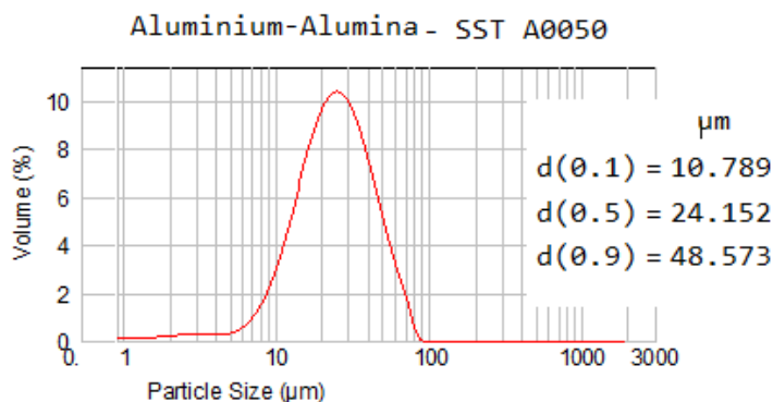
Figure P.1: Particle size distributions for aluminum-alumina
