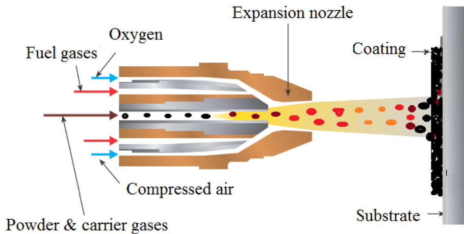
Figure H.9: HVOF process Source: (Ryan et al., 2006).
