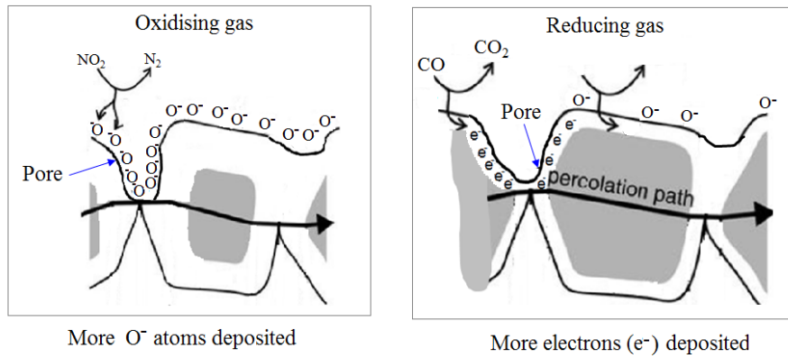
Figure F.2: Gas sensing mechanism.
