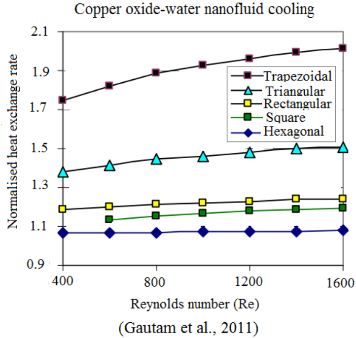
Figure C.6: Heat exchange rate Vs. Re for nanofluid cooling.
