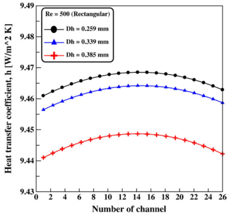
Figure C.3: Heat transfer coefficients.
