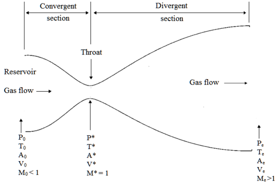
Figure K.1: Converging-diverging supersonic nozzle
