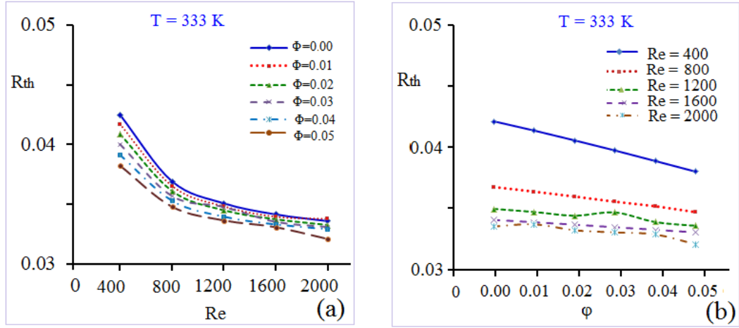
Figure 4.28: Thermal resistance graphs. Variation with: (a) Re , (b) volume of nanoparticles.
