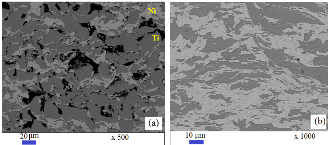
Figure 4.12: Titanium-nickel coatings (a) Porous, and (b) dense.
