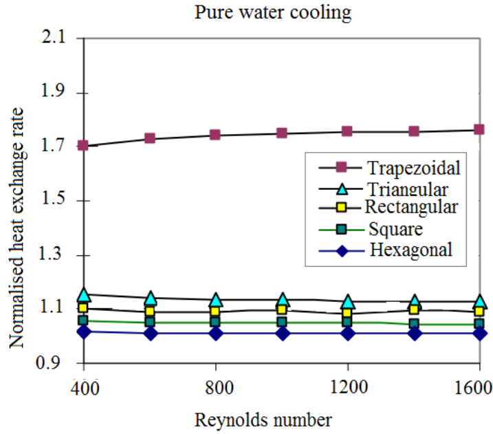
Figure C.5: Heat exchange rate Vs. R_e for water cooling.
