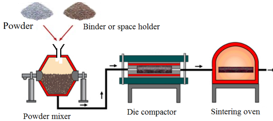
Figure H.5: Powder metallurgy process.
