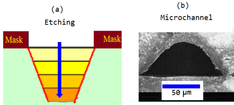
Figure H.10: Chemical etching method.
