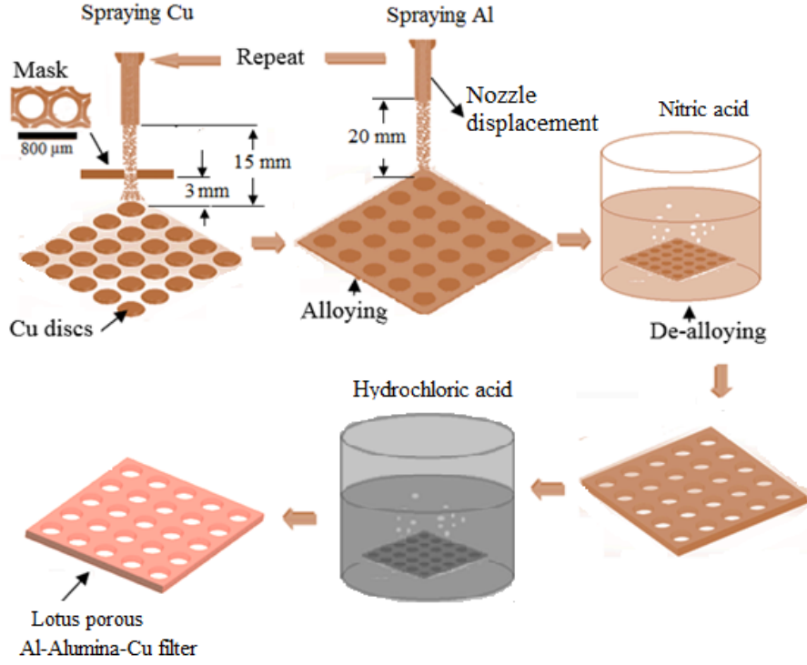
Figure 3.6: Process for antimicrobial filters.
