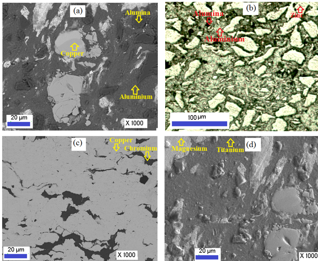
Figure P.9: Mixed powder coatings. (a) Al-Alumina-Cu, (b) Al-Alumina-Zn, (c) Cu-Cr, and (d) Ti-Mg.
