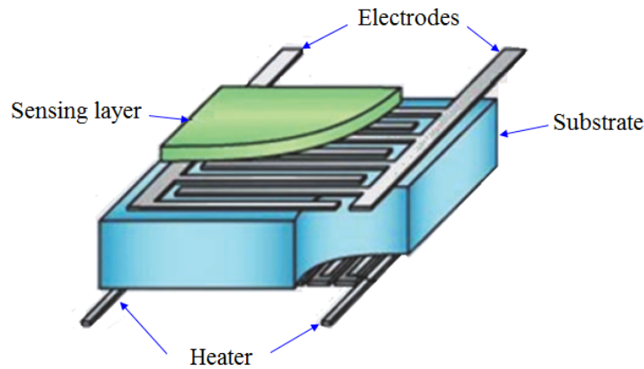
Figure F.1: Gas sensor configuration.
