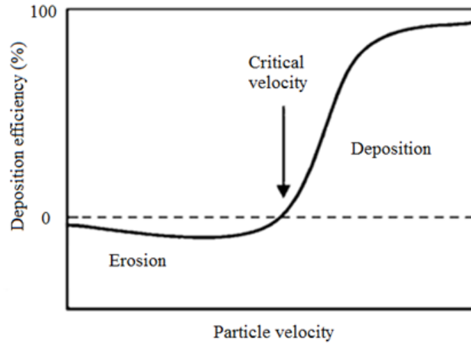
Figure L.7: Critical velocity Vs. deposition efficiency. Source: (Gartner, Schmidt, Stoltenhoff and Kreye, 2006)
