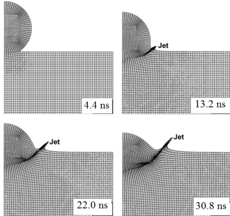
Figure I.4: Particle evolution during bonding
