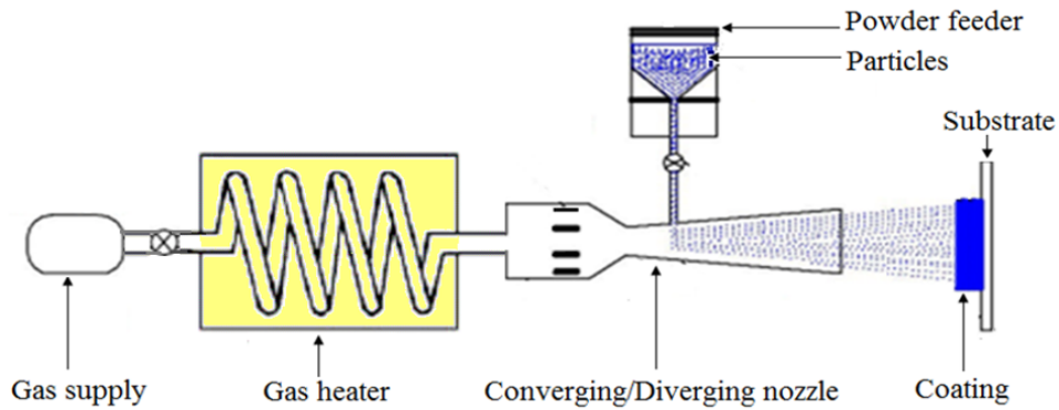
Figure 2.7: Downstream injection CS process.
