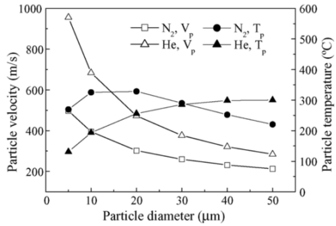
Figure L.12: Particle velocity Vs. particle diameter.
