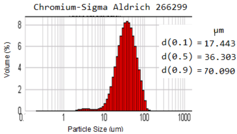
Figure P.2: Particle size distributions for chromium powder
