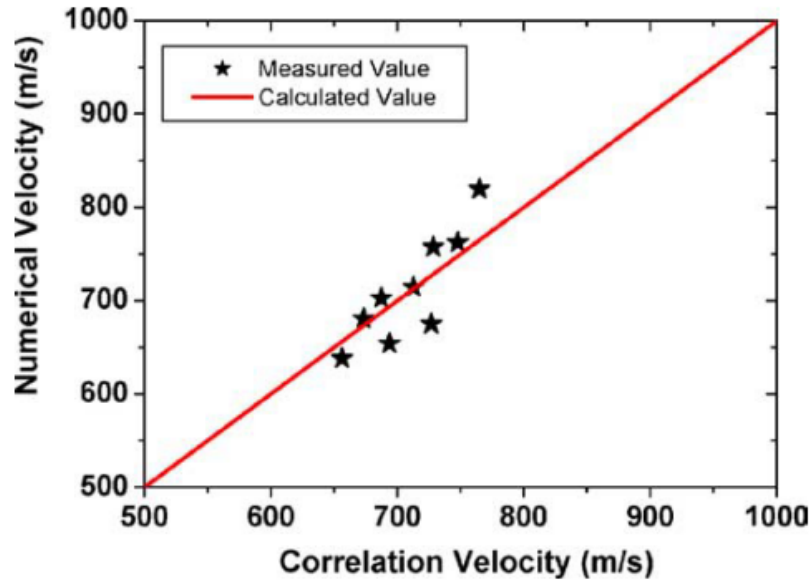
Figure L.6: Comparison of particle velocities. Source: (Wu et al., 2005)
