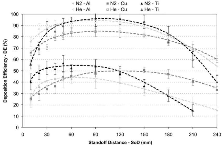
Figure L.5: Effect of standoff distance on deposition.
