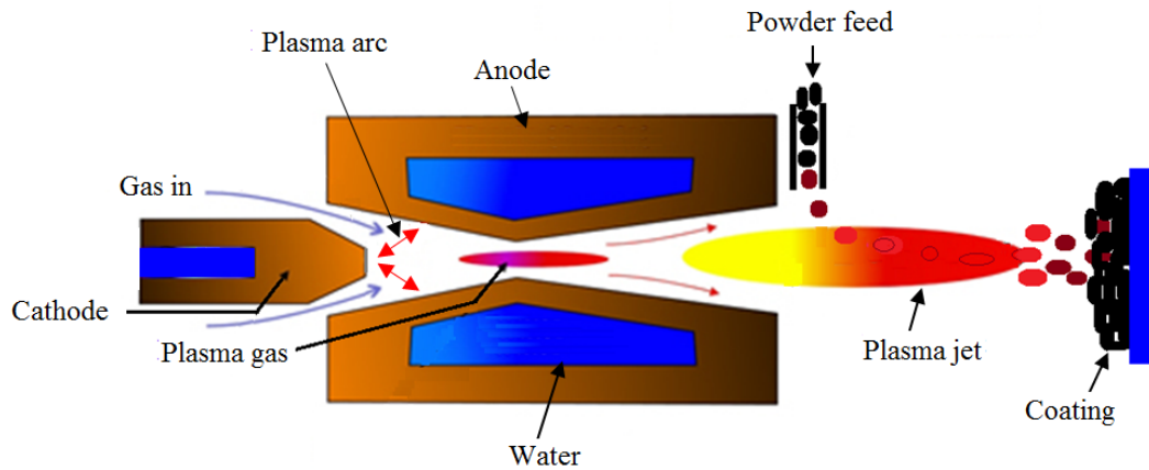
Figure H.7: Plasma spray process.
