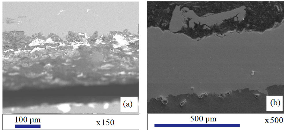
Figure 4.7: Surface porosity for copper and zinc coating. (a) Copper, (b) zinc coatings.
