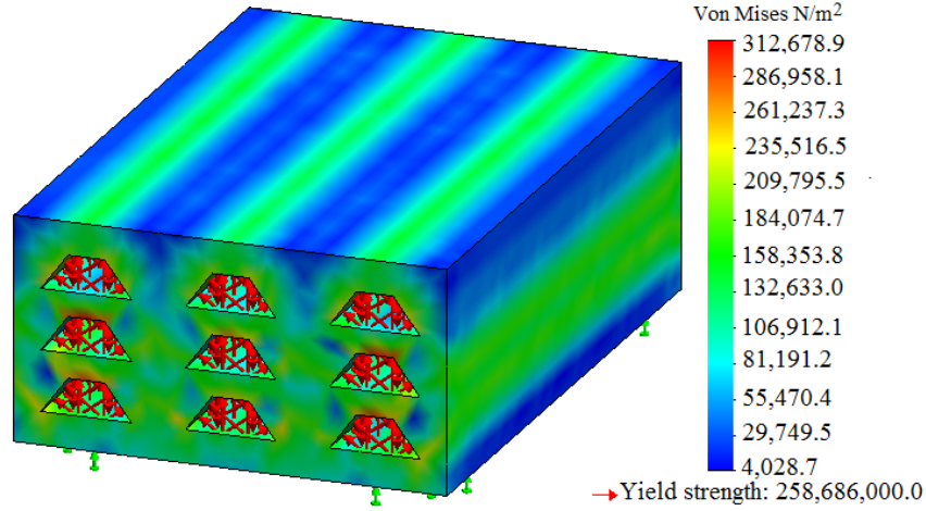
Figure 4.27: Simulated stress profile for micro heat sink.
