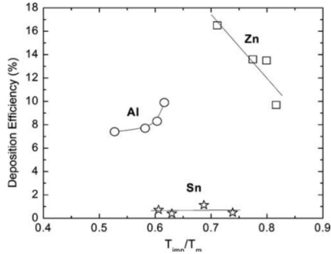
Figure L.14: Deposition efficiency Vs. melting temperature.
