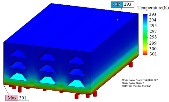
Figure 4.26: Simulated temperature profile for micro heat sink.
