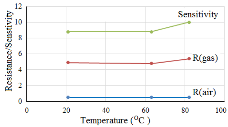
Figure 4.19: Graph for gas sensor sample 1.
