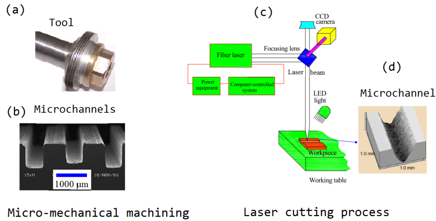
Figure H.11: Micro-mechanical and laser cutting.
