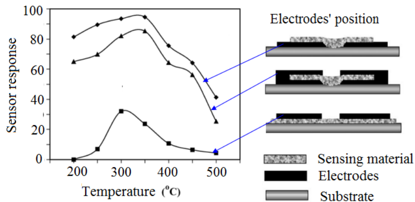
Figure F.3: Effects of electrodes position.
