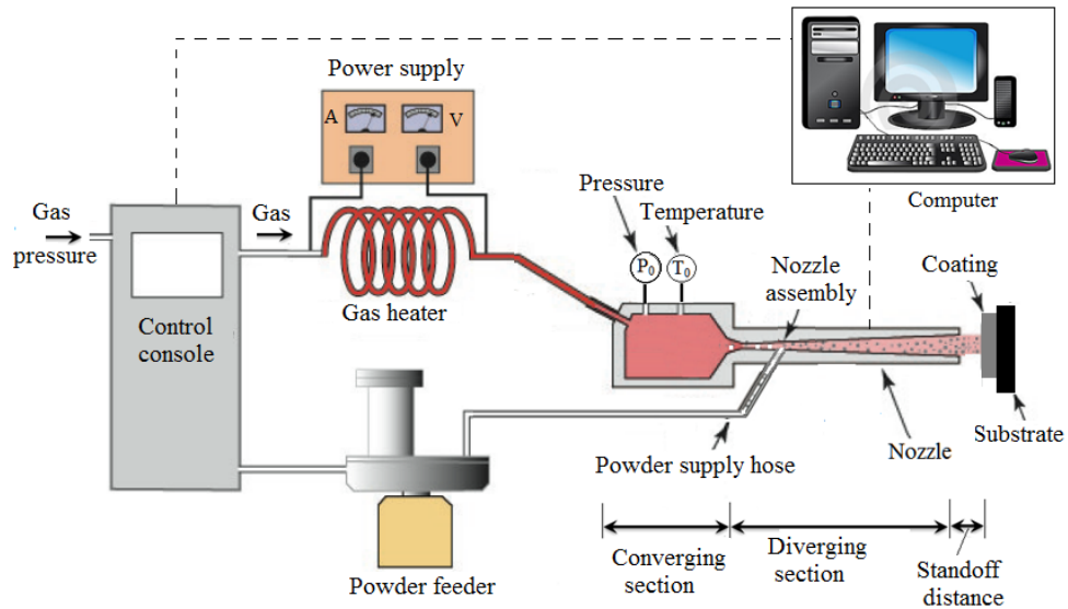
Figure I.3: CS process configuration.
