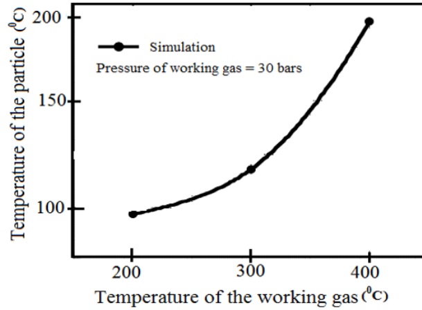
Figure L.9: Variation of particle temperature. Source: (Huang and Fukanuma, 2009)
