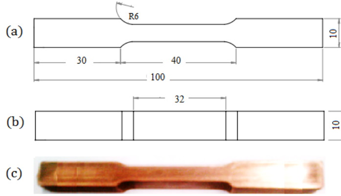
Figure 3.2: Tensile test substrate.
