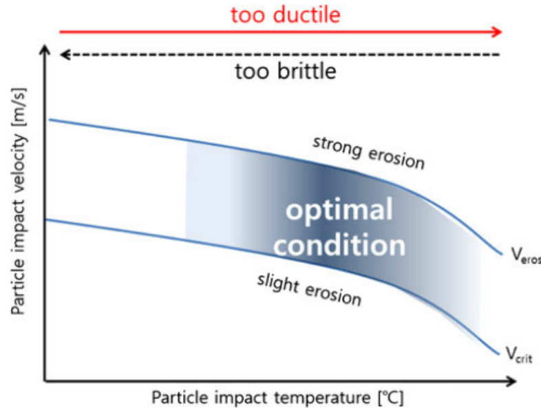
Figure L.2: Optimal CS conditions.
