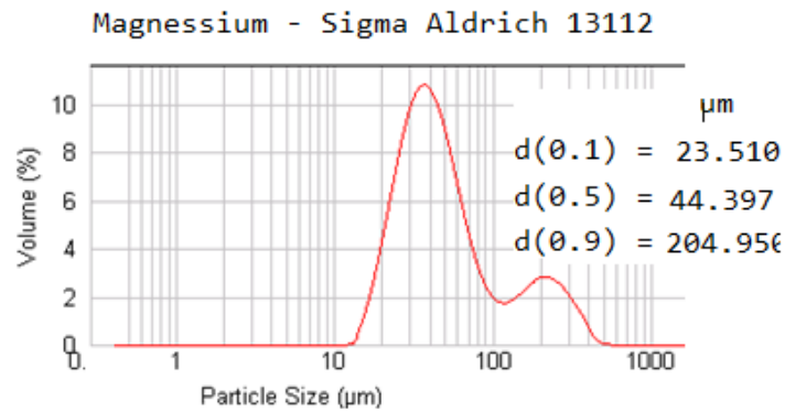
Figure P.4: Particle size distribution for magnesium Powder
