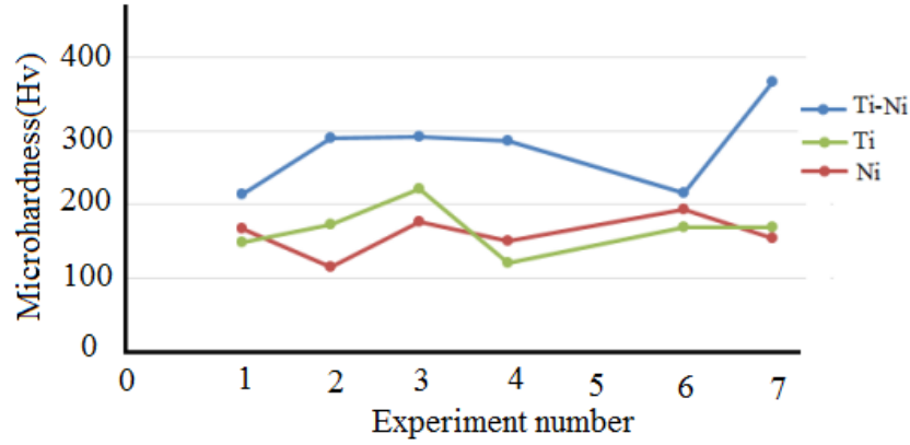
Figure 4.13: Microhardness graphs for coatings.
