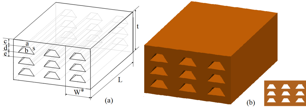
Figure 4.24: Microchannels dimension and model.
