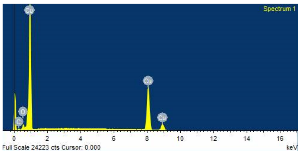
Figure P.6: EDX spectrum for copper powder.
