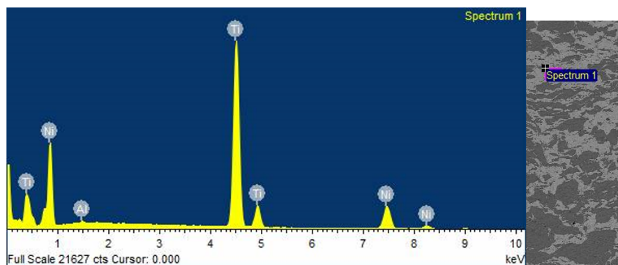
Figure P.11: EDX Spectrum for titanium-nickel coatings.
