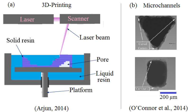
Figure H.12: 3D-printing process.
