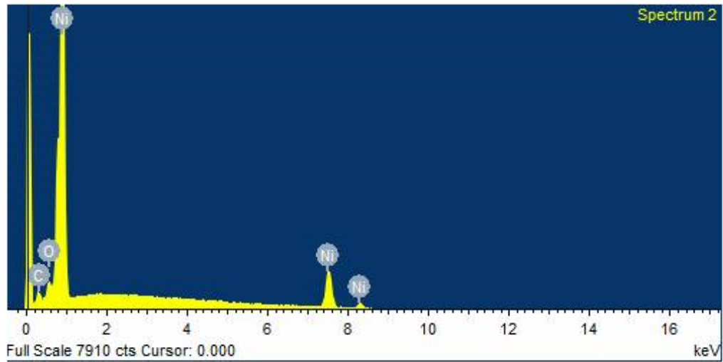
Figure P.8: EDX spectra for nickel powders.
