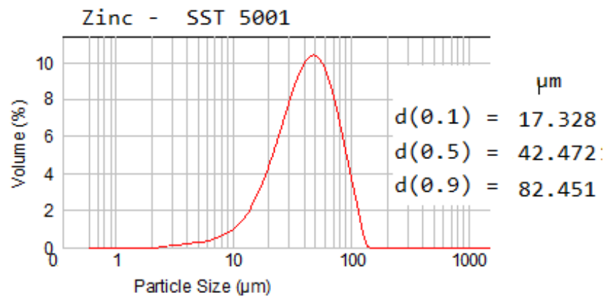
Figure P.3: Particle size distribution for zinc powder
