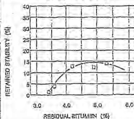
RETAINED STABILITY
