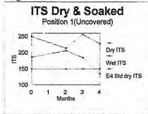
Material : Foam Stabilised Sand Figure 5.1.10
