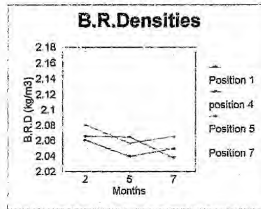
Material : Foam Stabilised RAP Figure 5.2.2
