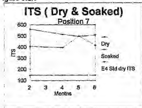
Material : Foam Stabilised RAP Figure 5.2.6
