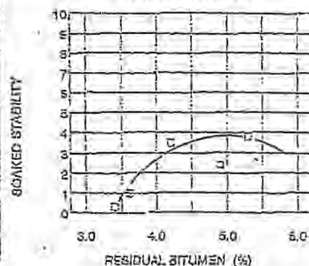
SOAKED STABILITY
