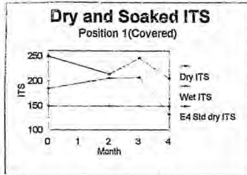
Material : Foam Stabilised Sand Figure 5.1.6
