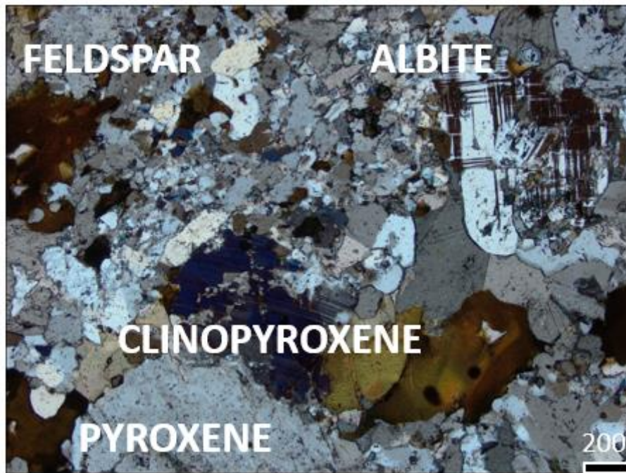
Figure 5-29. The chessboard twinning of albite (upper right corner) and presence of clinopyroxene are indicative of sodic alteration within Sequence 6, Shantumbu. Thin section is cross-polarised light of Sample E2243B from SPA027 at a depth of c. 370m.
