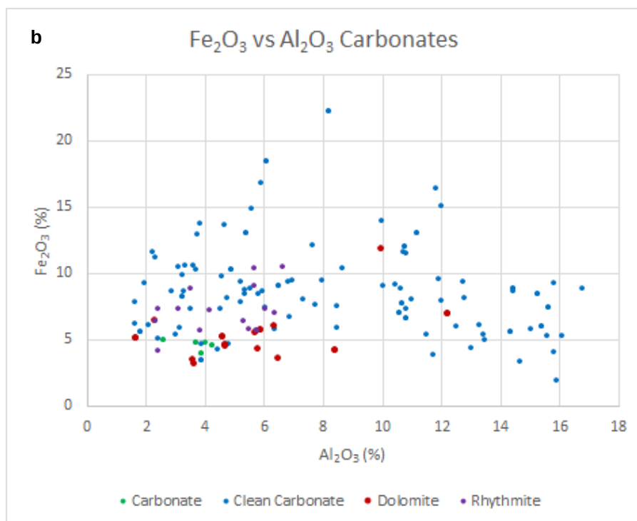
Figure 7-9. Scatterplot of the ICP-OES data for Fe 2 O 3 (%) versus Al 2 O 3 (%) for Sequences 1, 2, 4 and 5, Shantumbu. (a) Fe 2 O 3 versus Al 2 O 3 for the debris flow of Sequence 2 versus the arenites of Sequences 1, 2, 4 and 5. (b) Fe 2 O 3 versus Al 2 O 3 for the dolomitic carbonate of Sequence 4 on Shantumbu contrasted with the remaining carbonates. The dolomitic carbonate formed a tight grouping of values in comparison to the calcitic carbonates, perhaps because of less analyses. The calcitic carbonates reflect Sequence 5.
