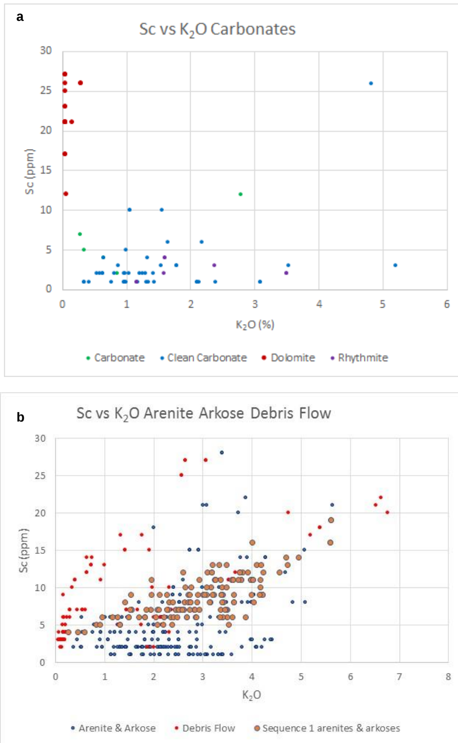
Figure 7-8. Scatterplot of the ICP-OES data for K 2 O versus Sc per sequence (a) Sc (ppm) versus K 2 O (%) for the dolomitic carbonate of Sequence 4 contrasted with the calcitic carbonates, Shantumbu. The dolomitic carbonate points are segregated from the remaining carbonates. (b) Sc (ppm) versus K 2 O (%) for the arkose and arenite units versus the debris flows of Sequence 2; Sequence 1 values are coloured separately.
