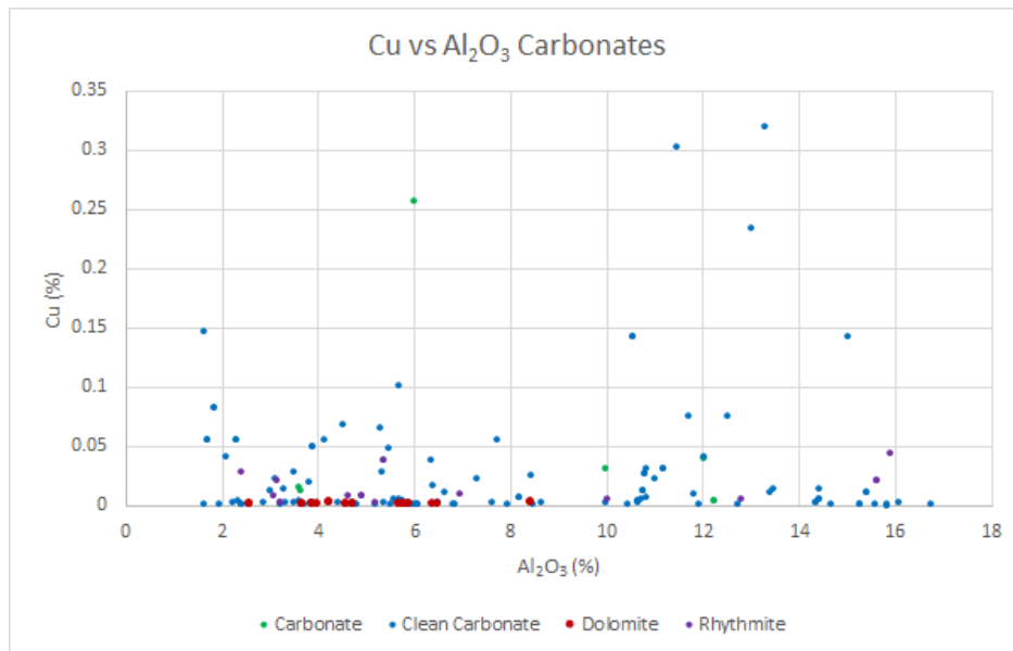
Figure 7-29. ICP-OES copper values (%) for Sequences 1, 2 and 5 against \text{Al}_2\text{O}_3 , an immobile oxide, Shantumbu.
