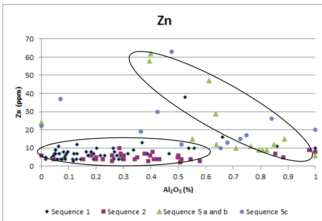
Figure 7-34. ICP-OES Zn values (ppm) for Sequences 1, 2 and 5 against \text{Al}_2\text{O}_3 , an immobile oxide, Shantumbu. The two populations are noted by the inserts.
