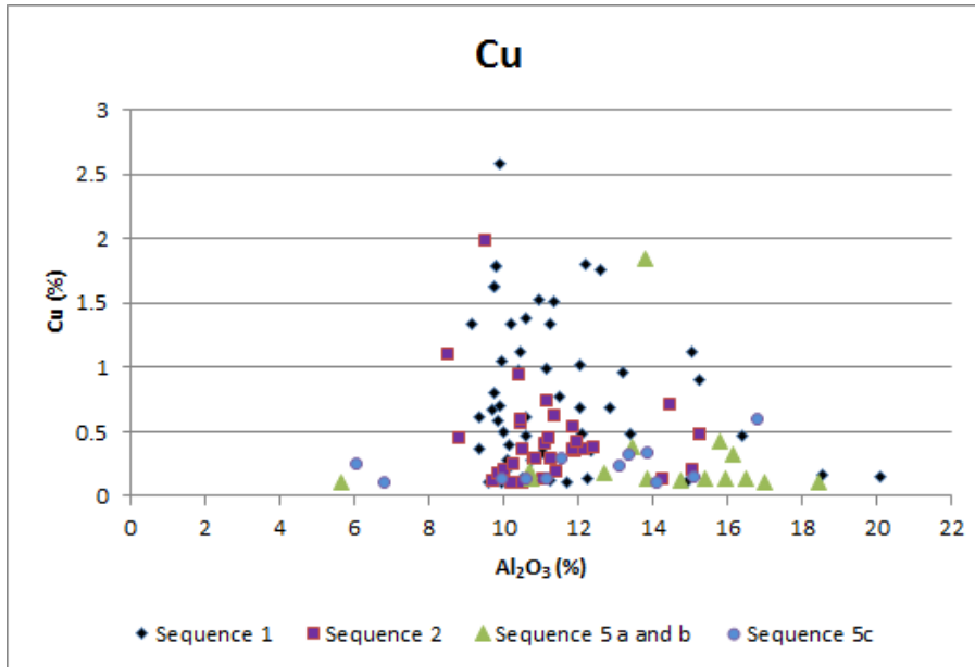
Figure 7-27. ICP-OES copper values (%) for Sequences 1, 2, and 5 against \text{Al}_2\text{O}_3 , an immobile oxide, Shantumbu.
