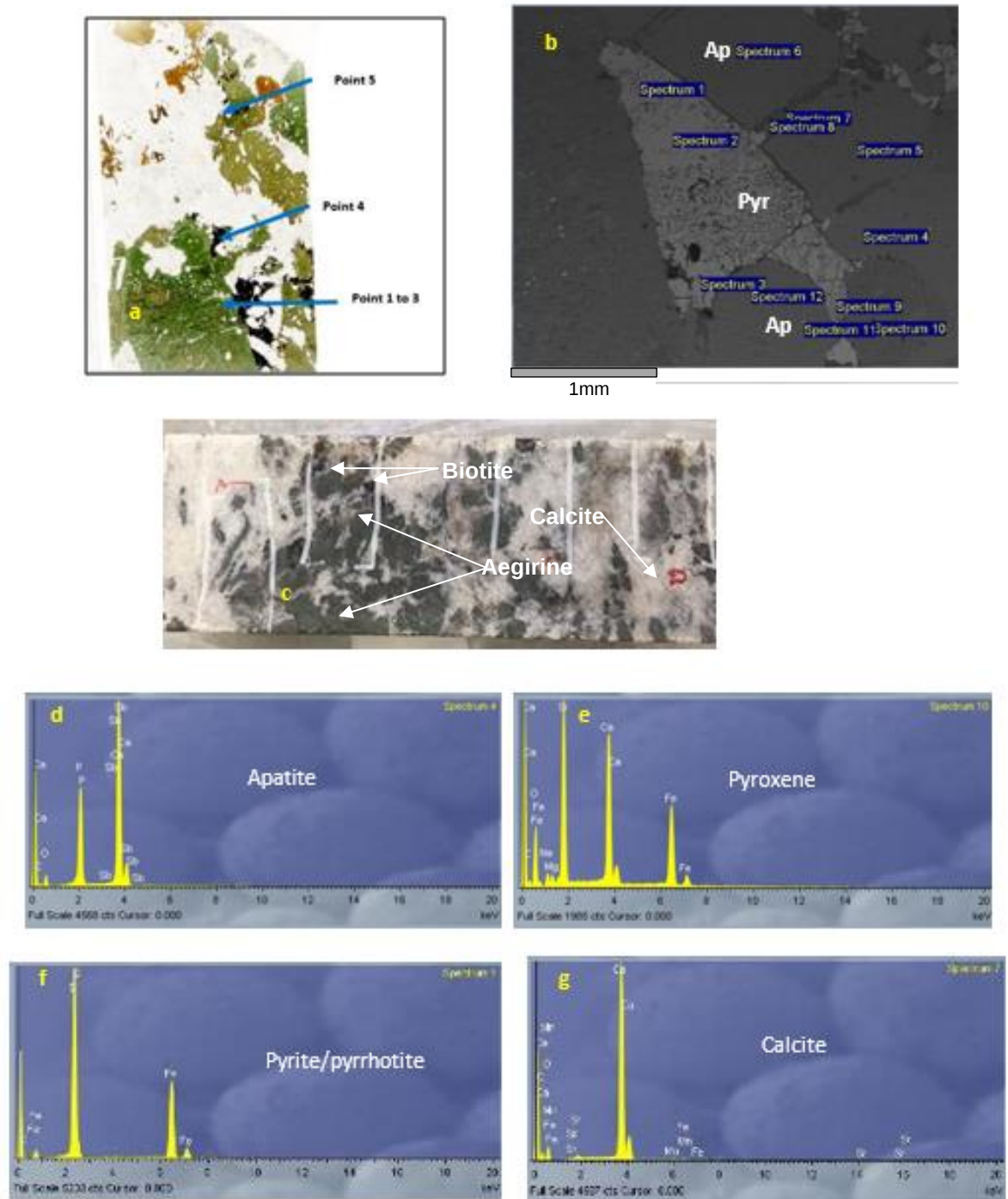
Figure 5-13. SEM data for sample E2213B (SPA015 at a depth of c. 30m) for Sequence 5, facies c, Shantumbu. (a) Thin section showing Points 1 to 5. (b) Backscattered electron image with locations of the eleven spectra; Ap – apatite, Pyr - pyrrhotite. (c) Half core sample from which the thin section was derived. (d) Mineral spectrum for apatite. (e) Mineral spectrum for pyroxene. (f) Mineral spectrum for pyrite/pyrrhotite. (g) Mineral spectrum for calcite.
