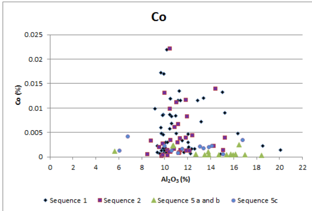
Figure 7-33. ICP-OES Co values (%) for Sequences 1, 2 and 5 against \text{Al}_2\text{O}_3 , an immobile oxide, Shantumbu.
