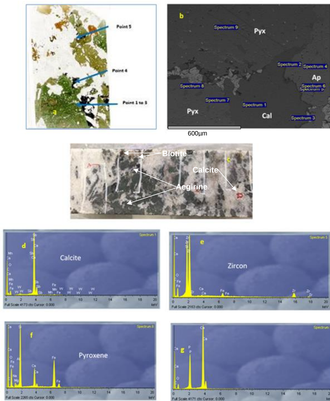
Figure 5-16. SEM data for sample E2213B (SPA015 at a depth of c. 30m) for Sequence 5, facies c, Shantumbu. (a) Thin section showing Points 1 to 5. (b) Backscattered electron image with locations of the nine spectra; Ap – apatite, Cal – calcite, Pyx - pyroxene. (c) Half core sample from which the thin section was derived. (d) Mineral spectrum for calcite. (e) Mineral spectrum for zircon. (f) Mineral spectrum for pyroxene. (g) Mineral spectrum for apatite.
