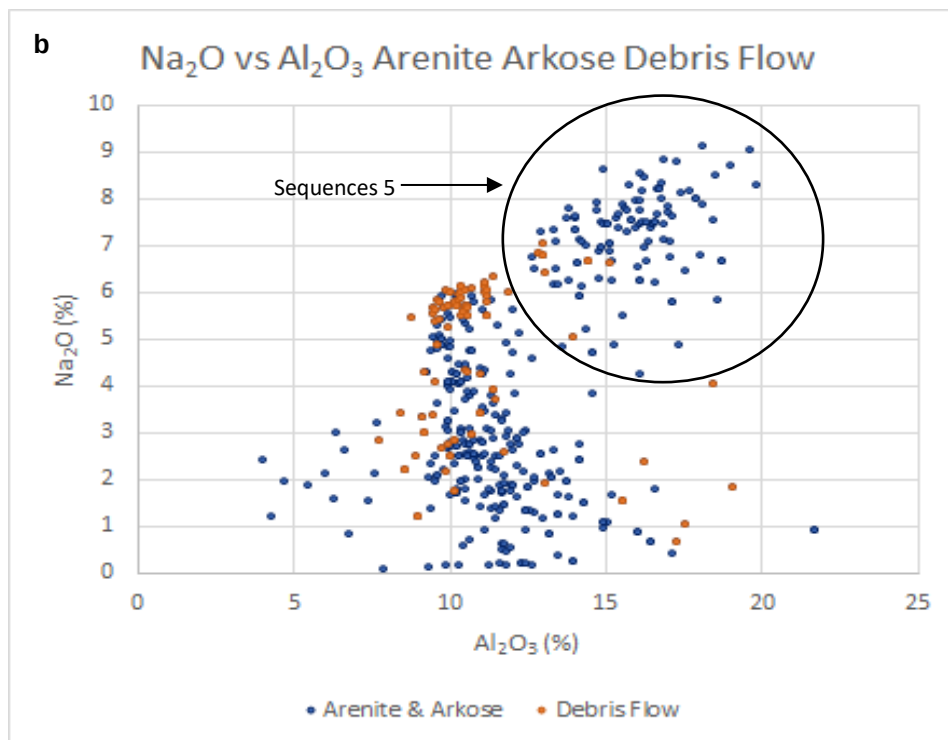
Figure 7-6. Scatterplot of the ICP-OES dataset illustrating the alteration of the detrital metasediments on Shantumbu. (a) \text{K}_2\text{O} (%) versus \text{Al}_2\text{O}_3 (%) of the Sequence 2 (Kafue Arenite Member) debris flows, contrasted with the arenite and arkoses of Sequences 1, 2, 4, and 5. (b) \text{Na}_2\text{O} (%) versus \text{Al}_2\text{O}_3 (%) of the Sequence 2 debris flows deposits, contrasted with the arenite and arkoses of Sequences 1, 2, 4, and 5.
