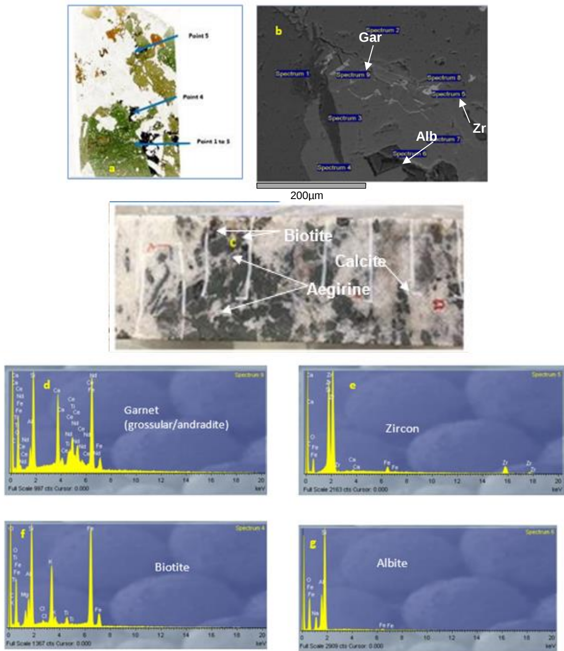
Figure 5-17. SEM data for sample E2213B (SPA015 at a depth of c. 30m), for Sequence 5, facies c, Shantumbu. (a) Thin section showing Points 1 to 5. (b) Backscattered electron image with locations of the nine spectra Gar – garnet, Cal – calcite, Zr - zircon, and Alb - albite. (c) Half core sample from which the thin section was derived. (d) Mineral spectrum for garnet. (e) Mineral spectrum for zircon. (f) Mineral spectrum for biotite. (g) Mineral spectrum for albite.
