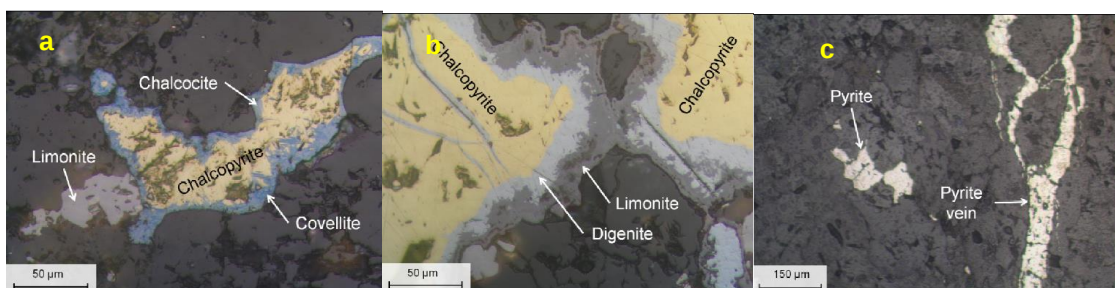
Figure 6-3. Vein hosted and disseminated chalcopyrite, digenite, chalcocite, covellite and pyrite of Sequence 2, Shantumbu. (a) Alteration of chalcopyrite to covellite and chalcocite (H08293 from PSH001 at a depth of 80.4m). (b) Alteration of chalcopyrite to digenite and goethite (H08293 from PSH001 at a depth of 80.4m). (c) Pyrite vein and disseminated pyrite (H08292 from PSH008 at a depth of 52m). All images in plane polarised reflected light.
