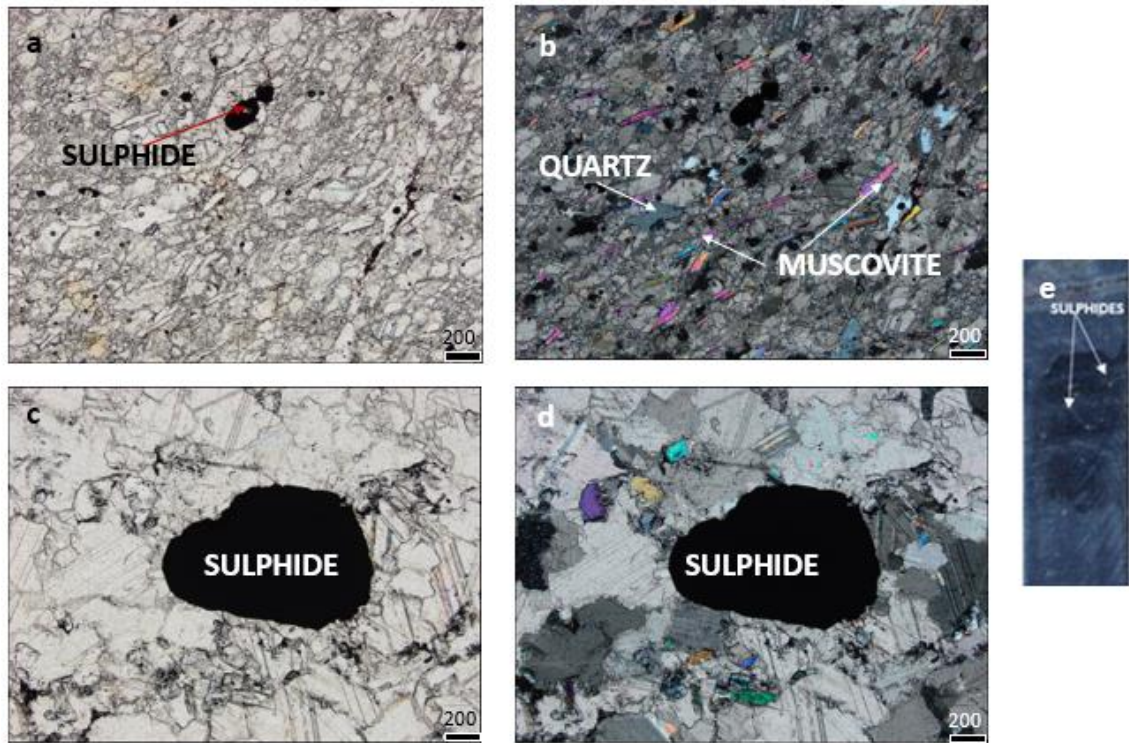
Figure 5-35. Sulphide mineralisation in Sequence 7 carbonates, Shantumbu. (a) Disseminated and rounded sulphide (pyrite) within matrix of muscovite and quartz; plane polarised light. Sample E2231A plane polarised light (200µm) (SPQ002 at a depth of c. 220m). (b) Disseminated and rounded sulphide (pyrite) within matrix of muscovite and quartz; cross polarised light. Sample E2231A cross polarised light (200µm) (SPQ002 at a depth of c. 220m). (c) Disseminated and rounded sulphide (pyrite) within matrix of muscovite and quartz; plane polarised light. Sample E2227B plane polarised light (200µm) (SPQ002 at a depth of c. 110m). (d) Disseminated and rounded sulphide within matrix of muscovite and quartz; cross polarised light. Sample E2227B cross polarised light (200µm) (SPQ002 at a depth of c. 110m). (e) Core sample of blue carbonate with disseminated sulphides. Sample E2227of drill hole (SPQ002 at a depth of c. 110m).
