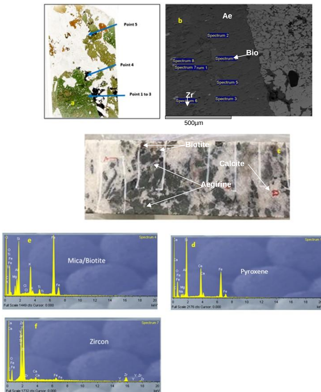
Figure 5-14. SEM data for sample E2213B (SPA015 at a depth of c. 30m) for Sequence 5, facies c, Shantumbu. (a) Thin section showing Points 1 to 5. (b) Backscattered electron image with locations of the eight spectra; Ae – aegirine, Bio – biotite, Zr - zircon. (c) Half core sample from which the thin section was derived. (d) Mineral spectrum for pyroxene. (e) Mineral spectrum for mica/biotite. (f) Mineral spectrum for zircon.
