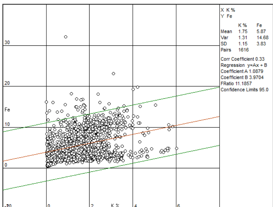
Figure 7-20. Positive correlation (33%) between K and Fe (%) for the ICP-OES dataset; all Sequences are combined into a single plot, Shantumbu.
