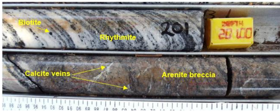
Figure 4-14. Biotite-dominated bands, grey carbonate, and brecciated arenite of facies 5c (SPA015 at a depth of c. 201m), Shantumbu.
