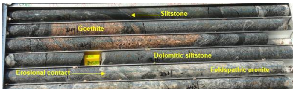
Figure 4-17. Goethite-rich carbonate and erosional contact between the arenite and underlying carbonate in Sequence 6 (SPA018 at a depth of c. 245m), Shantumbu.
