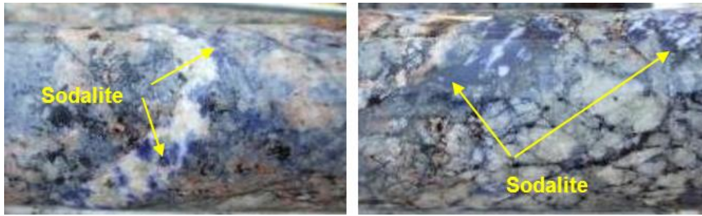
Figure 5-27. Coarse-grained sodalite pervasive through the brecciated arenite of Sequence 6, Shantumbu core sample (SPA018; drill core size is BQ; depth at c. 312m).
