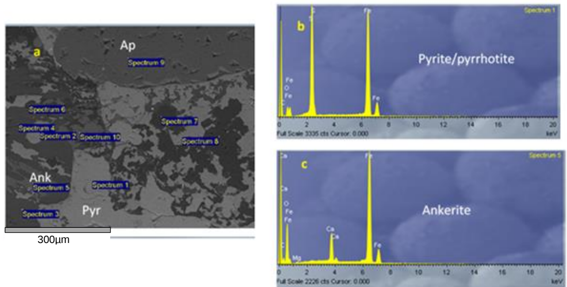
Figure 5-23. SEM data for sample E2213D, Sequence 5, facies c, Shantumbu. (a) Backscattered electron image with locations of the ten spectra. (b) Mineral spectrum for pyrite/pyrrhotite. (c) Mineral spectrum for ankerite. Ap – apatite; Ank – ankerite; Pyr – pyrite.
