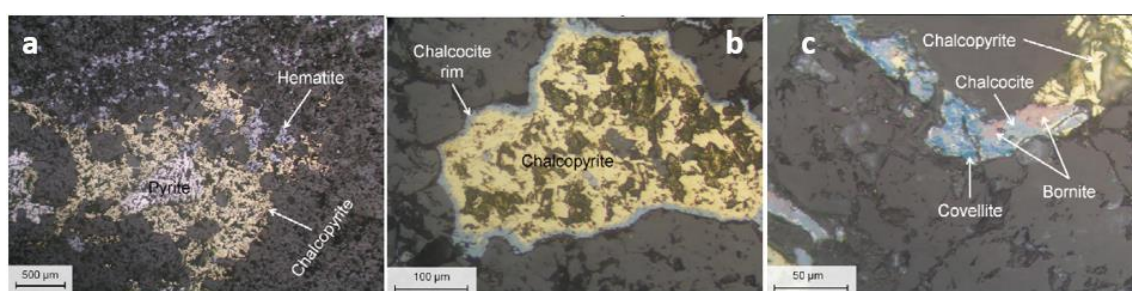
Figure 6-2. Copper-bearing sulphide veins and quartz-plagioclase-muscovite-bearing veins with accessory hematite \pm malachite \pm goethite, Shantumbu. (a) Rims of chalcopyrite and hematite on sulphides. (b) Chalcocite rim of a chalcopyrite grain (H08294 from PSH001 at a depth of 36.24m). (c) Vein-hosted copper-sulphides within arenite of Sequence 1 (H08300 from PSH001A at a depth of 43.42m). All images in plane polarised reflected light.
