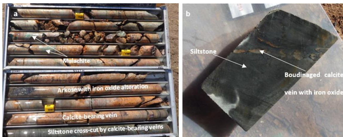
Figure 4-5. Arkose and siltstone units of Sequence 1, Shantumbu. (a) Alternating siltstone and iron-oxide-bearing arkose layers of Sequence 1. (b) Siltstone from Sequence 1 cross-cut by a boudinaged calcite-bearing vein (H08291 from PSH007 at a depth of 100.1m).
