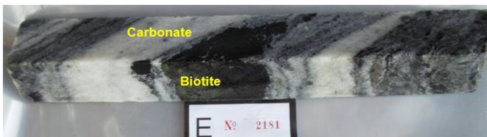
Figure 4-13. Alternating laminations of calcite and biotite within the rhythmites of facies 5c (SPA018, sample E2181 at a depth of c. 86m), Shantumbu.
