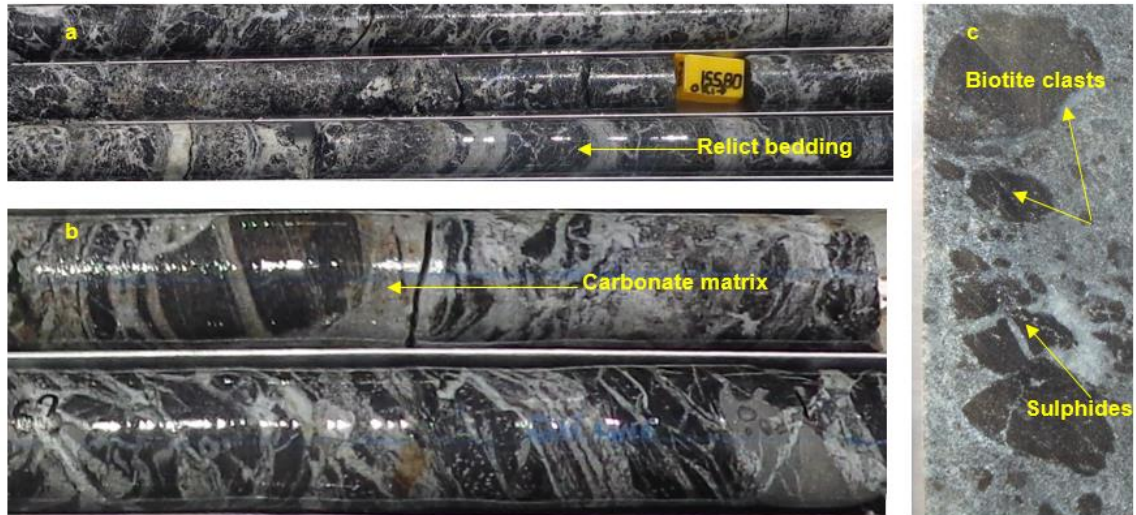
Figure 4-12. Breccias of facies 5b, Shantumbu. (a) Brecciated siltstone and relict bedding within facies 5b in PSH007. (b) Brecciated argillite cemented by carbonate matrix of facies 5b. (c) Sulphides cross-cutting a brecciated biotite clast in facies 5b (PSH007).
