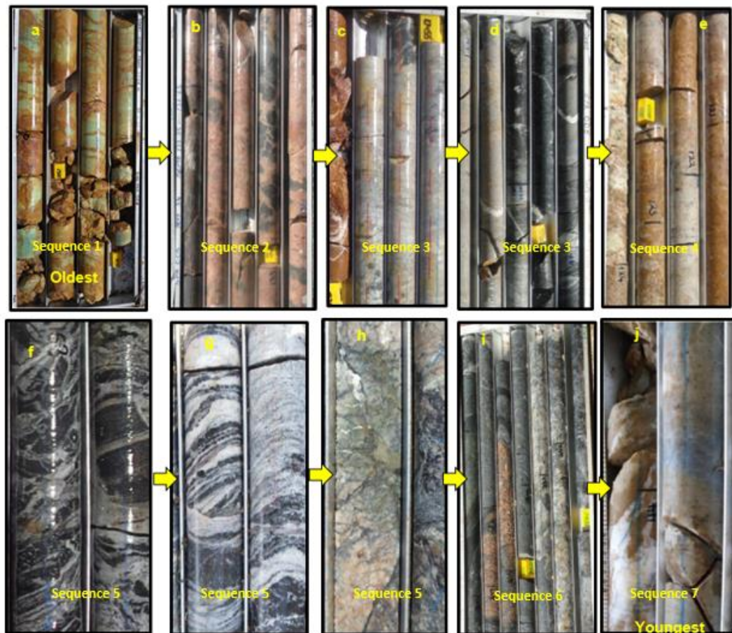
Figure 2-1. The seven sequences and related metasediments intersected in the Shantumbu drill cores. (a) The fine-grained arkose of Sequence 1 is the oldest unit intersected in the drilling and is host to copper mineralisation. (b) Red, cream and grey arenite of Sequence 2. (c) Dolomite calc-silicate of Sequence 3. (d) Siltstone and grey carbonate of Sequence 3. (e) Iron oxide-rich calc-silicate of Sequence 4. (f) Siltstone carbonate breccia of Sequence 5. (g) Siltstone carbonate rhythmite of Sequence 5. (h) Brecciated arenite of Sequence 5. (i) Goethite-rich carbonate and arenite of Sequence 6. (j) Finely laminated grey-blue to yellow-brown carbonate of the youngest succession, Sequence 7.
