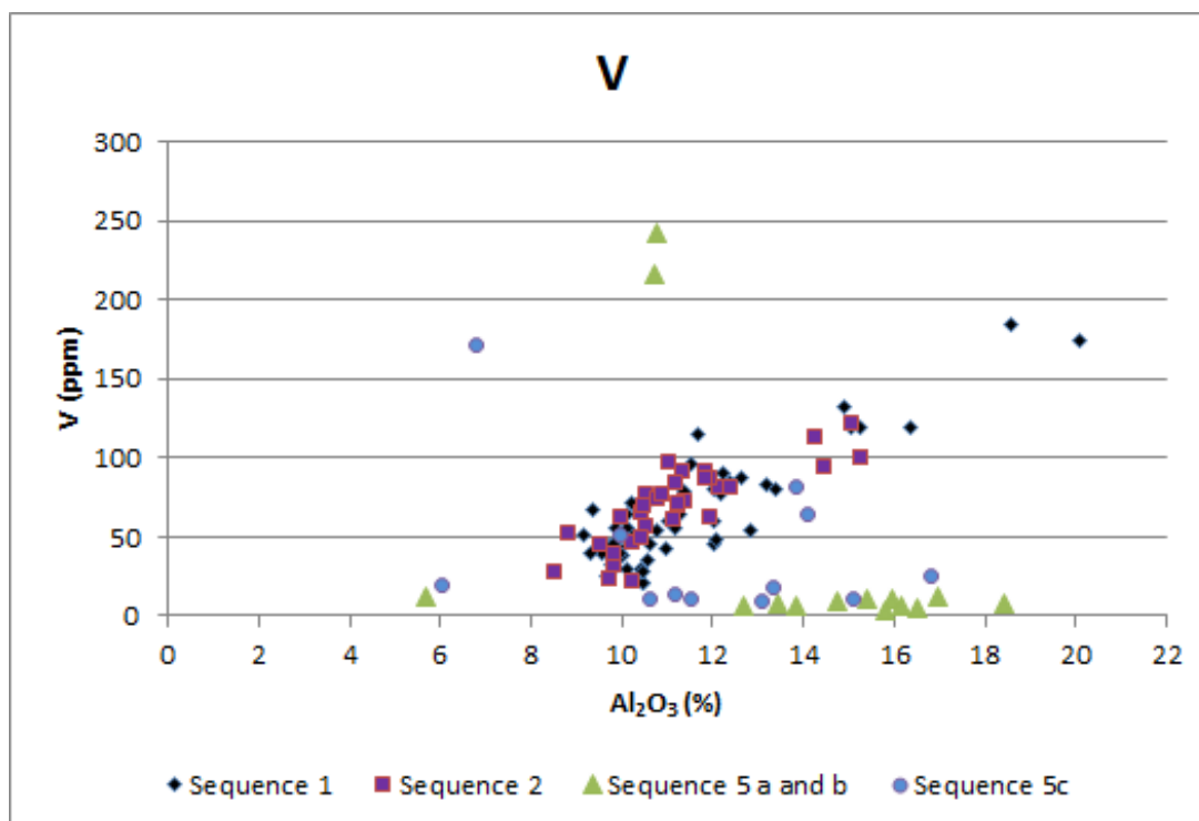
Figure 7-24. ICP-OES V values (ppm) for Sequences 1, 2 and 5 against \text{Al}_2\text{O}_3 (%), an immobile oxide, Shantumbu.
