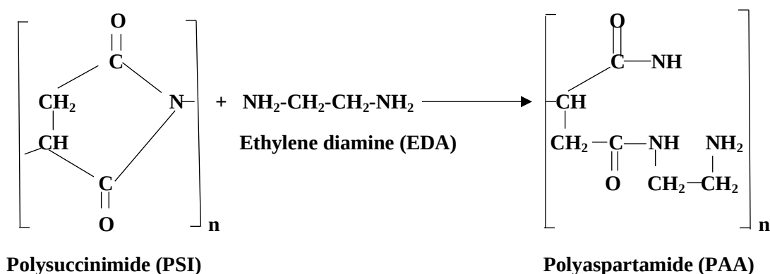
Figure 2.6 Formation of polyaspartamide (Miyata et al., 2008)
