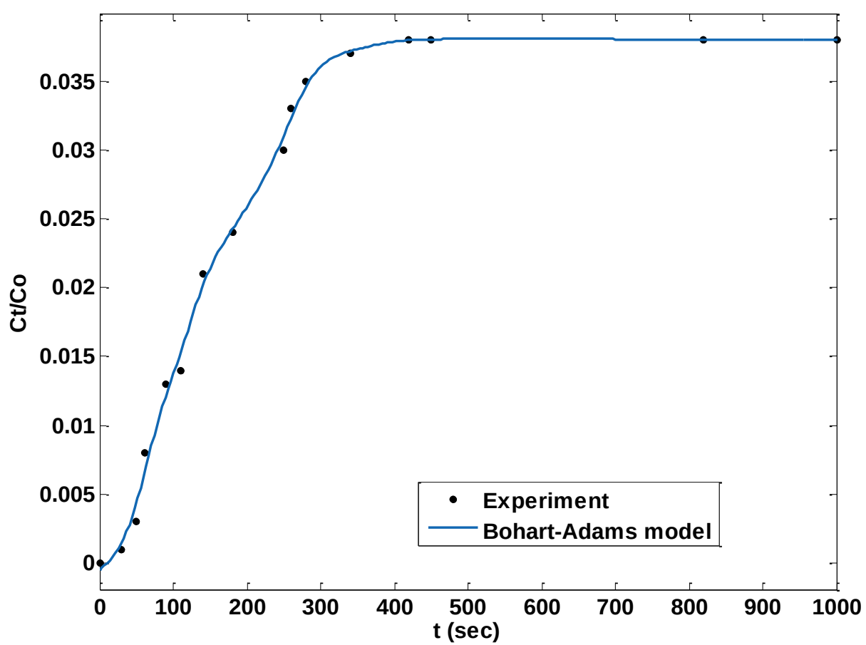
Figure 7.4. Experimental breakthrough curve at 30°C and corresponding fit to the Bohart-Adams model
