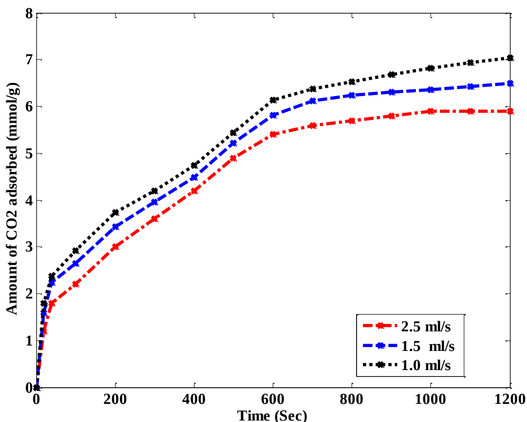
Figure 6.4 Effect of flow rates on the amount of CO 2 adsorbed onto polyaspartamide.
