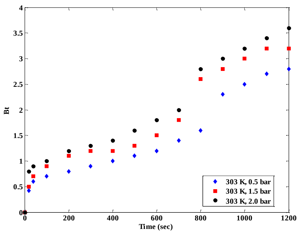
Figure 5.2. Boyd's film diffusion model for CO 2 adsorption on polyaspartamide at different pressure.
