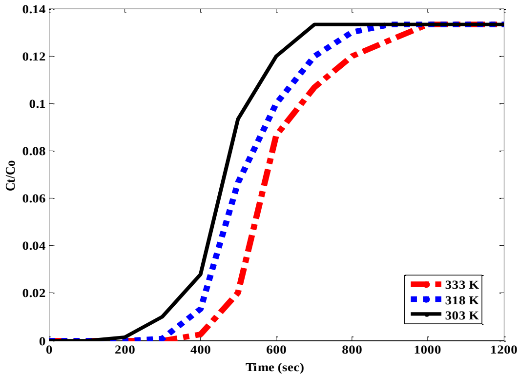
Figure 2. Experimental breakthrough curves at various adsorption temperatures, constant flow rate and constant pressure.
