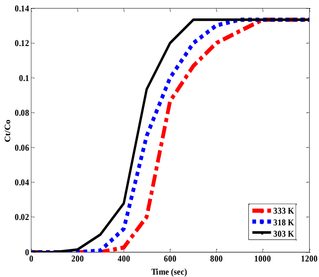
Figure 4.1 Experimental breakthrough curves (Conditions: Pressure 2 bar, Temperature: 303-333 K)
