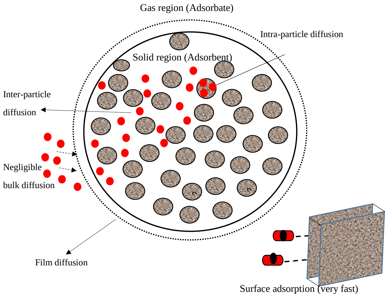
Figure 5.1 Adsorption mechanisms for CO 2 onto a solid sorbent (Adapted from Song et al. , 2016).
