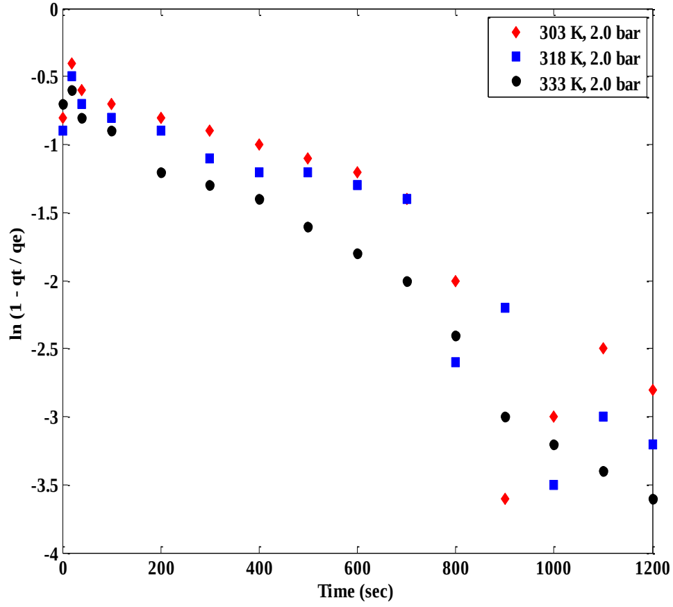
Figure 5.4. Inter-particle diffusion model plots for CO 2 adsorption on polyaspartamide at different adsorption temperature and constant pressure.
