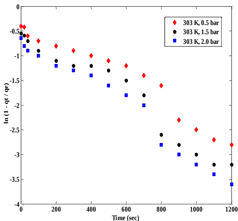
Figure 5.5 Inter-particle diffusion model plots for CO 2 adsorption on polyaspartamide at different CO 2 partial pressures.
