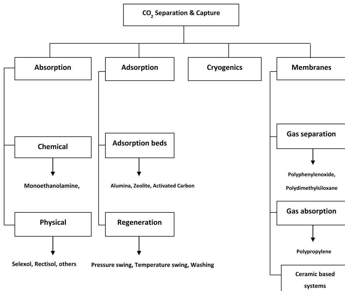
Figure 1. Different CO 2 separation and capture technologies for post-combustion CO 2 capture [82].
