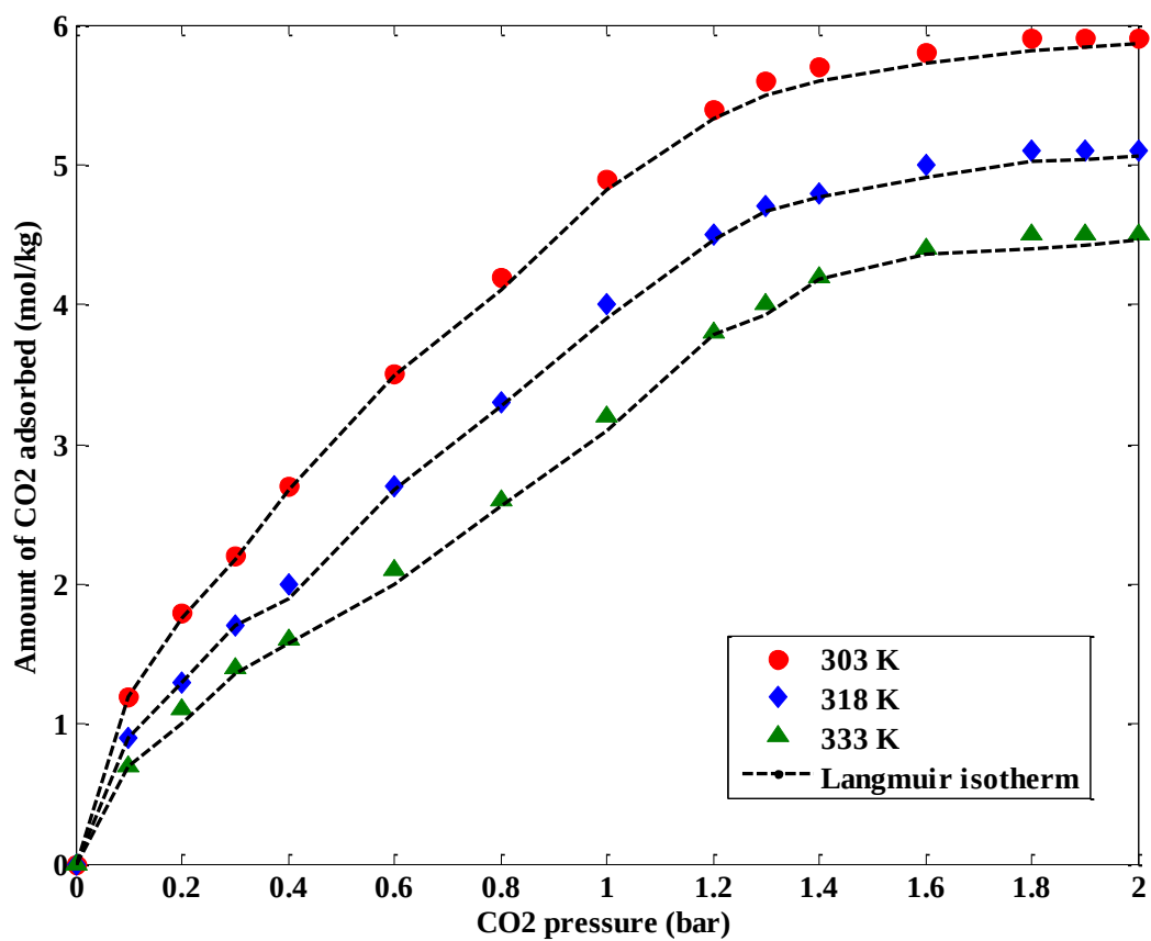
Figure 6.2 CO 2 adsorption isotherms of polyaspartamide at various temperatures (Experimental Vs Langmuir Isotherm).
