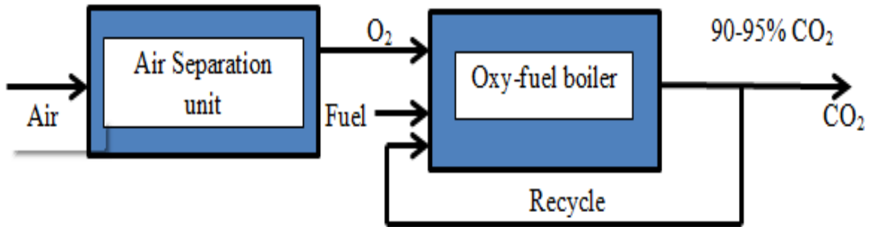
Figure 2.4 Oxy-fuel combustion capture.
