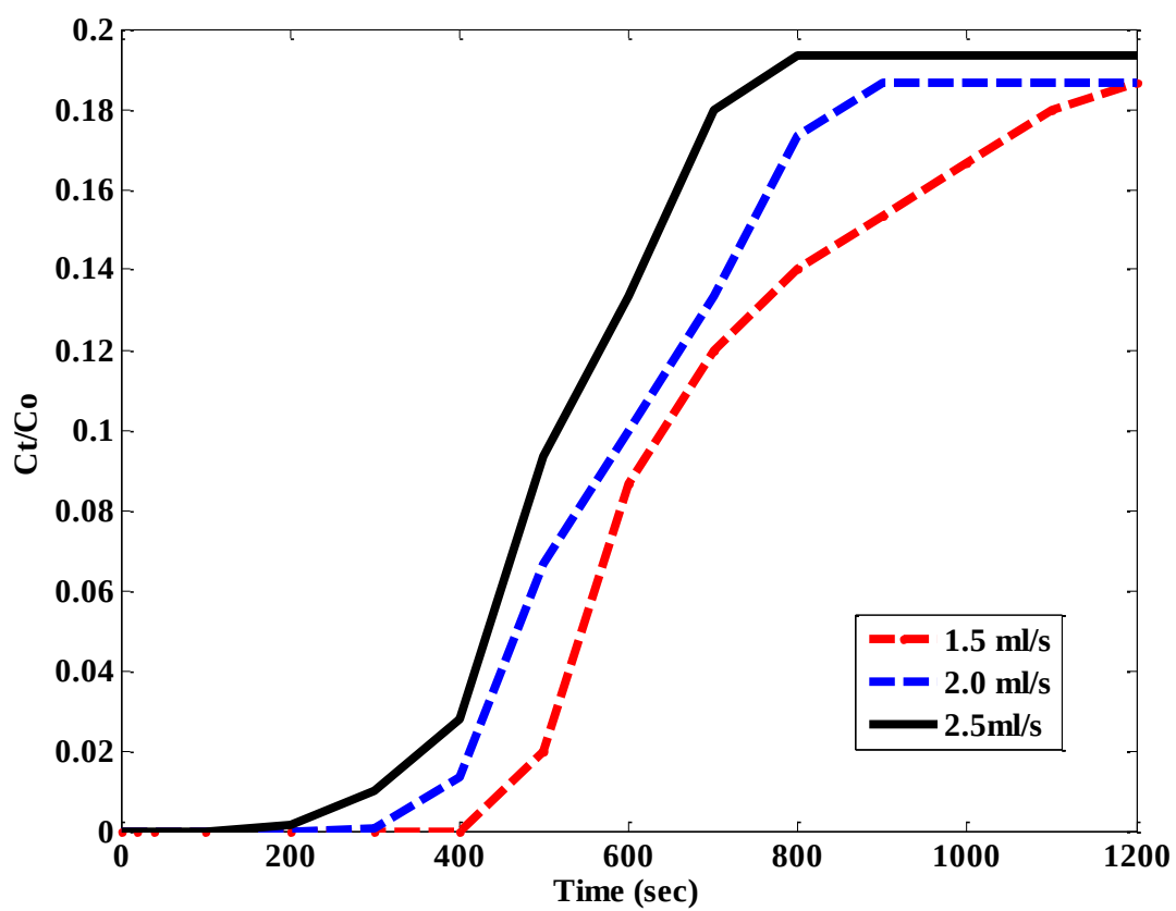
Figure 4.2 Effect of feed flow rate as a function of time. (Experimental conditions: feed pressure, 2 bar, and temperature 303 K).
