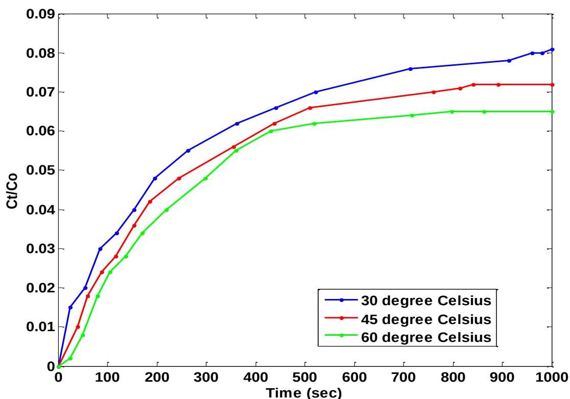
Figure 7.3 Experimental Breakthrough curves of 15 % CO 2 balance N 2 on Sod-ZMOF/Chitosan at various temperatures
