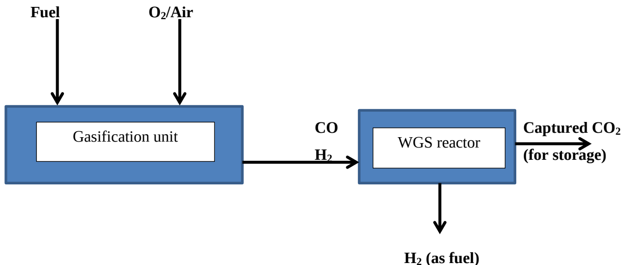
Figure 2.3 Schematic representation of the pre-combustion CO 2 capture process
