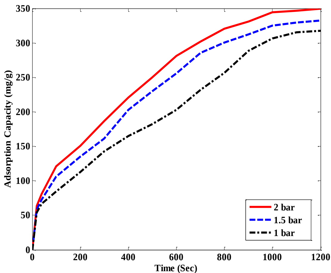
Figure 6.3 Effect of operating pressure on the adsorption capacity of polyaspartamide
