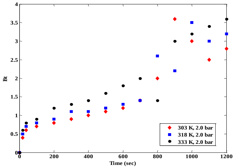
Figure 5.3 Boyd's film diffusion model for CO 2 adsorption onto polyaspartamide at different adsorption temperature and constant pressure.
