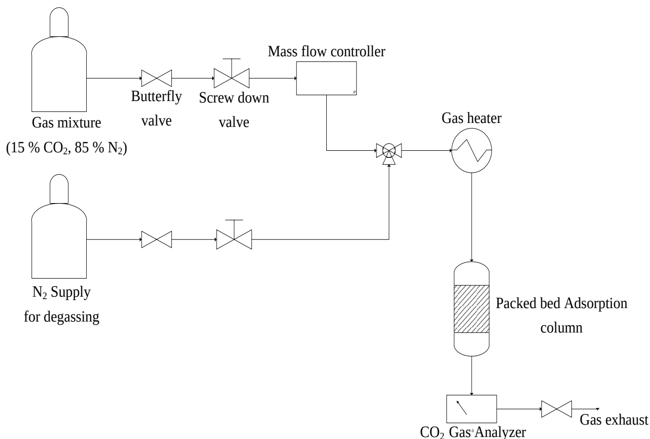
Figure 3.1 Experimental flow diagram for CO 2 adsorption on polyaspartamide.
