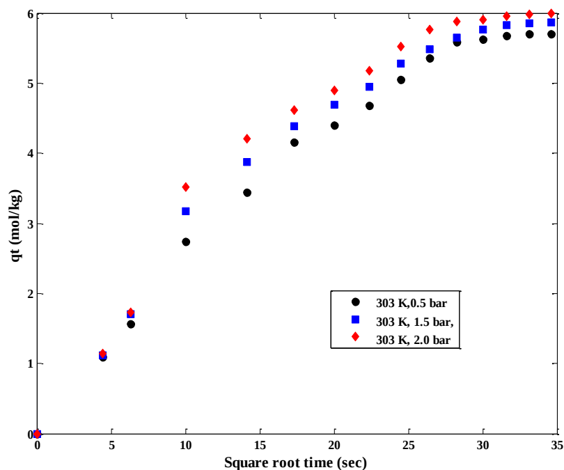
Figure 5.7 Intra-particle diffusion model plots for CO 2 adsorption on polyaspartamide at different CO 2 partial pressures.
