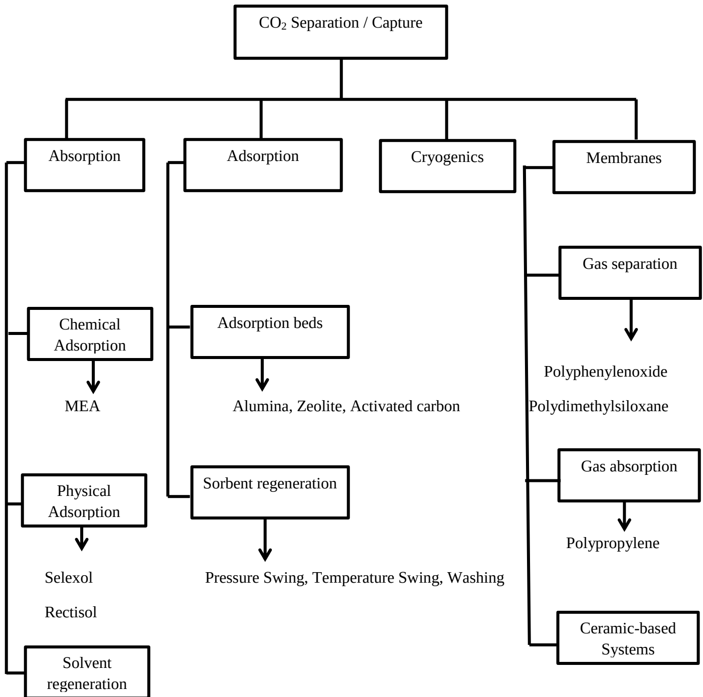
Figure 2.5 Different CO 2 separation and capture technologies for post-combustion CO 2 capture (Adapted from: Siriwardane et al., 2001).
