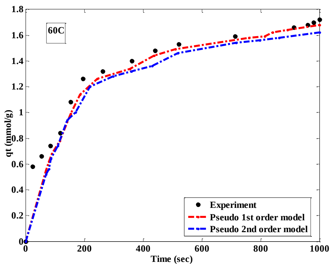
Figure 7.5. Experimental and predicted CO 2 adsorption curves of Sod-ZMOF/Chitosan material at constant pressure and different temperatures; (A) 2bar, 30°C, (B) 2bar 45°C (C) 2bar 60°C
