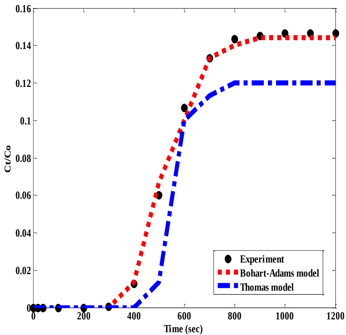
Figure 4.3 Experimental results versus model results. (Experimental conditions: 303 K, 2 bar)
