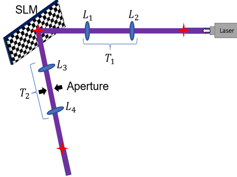
Figure 2.2: SLM setup: The object plane (represented by the red star) on the right is imaged by means of a telescope ( T_1 ), consisting of lenses L_1 and L_2 , onto the SLM. This object plane is then further imaged by telescope T_2 to the next object plane (star at the bottom of the image). The aperture is placed between lenses L_3 and L_4 for the purpose of spatial filtering.
