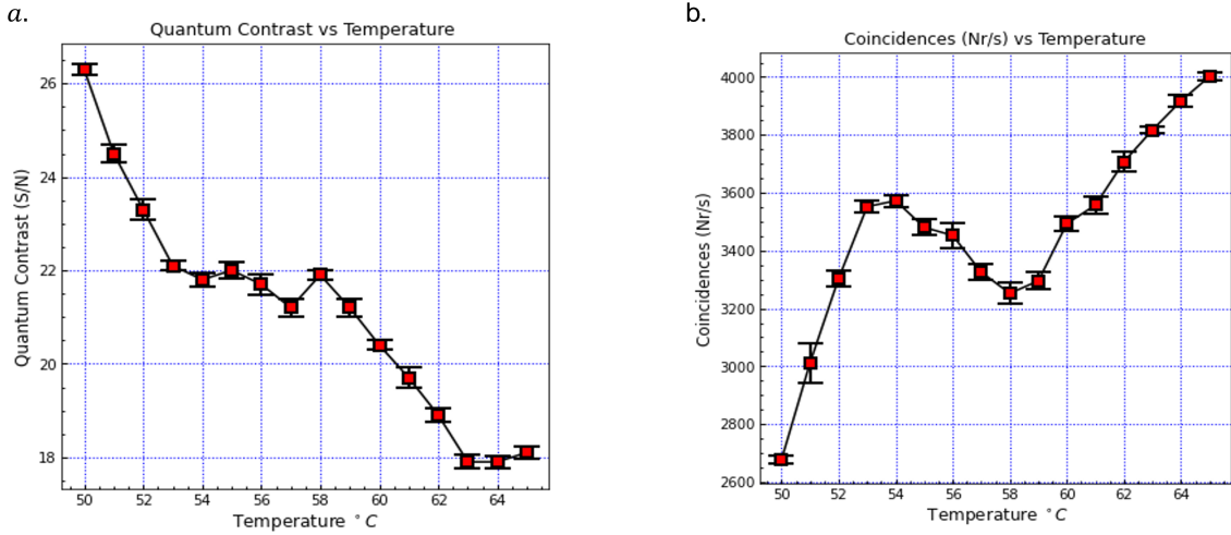
Figure 4.4: Temperature dependence: In a. the relationship between the quantum contrast and temperature is shown while in b. the relationship between the coincidence counts and temperature is shown.
