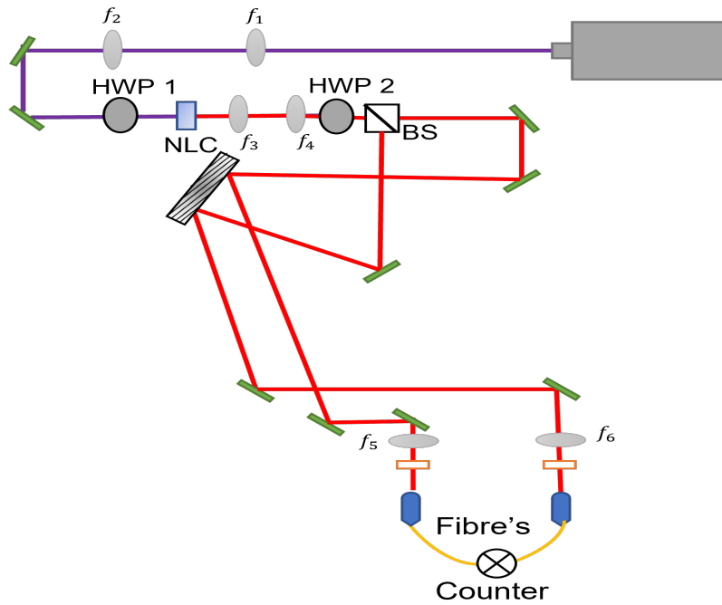
Figure 4.1: Experimental setup: The labels f_i refer to the lenses used in the setup. They are set up in pairs of two to work as a telescope imaging system. HWP 1 and 2 refer to the half wave plates before the crystal and SLM respectively. NLC is the non-linear crystal which in this case was a PPKTP crystal. BS is the beam splitter, and the two orange boxes before the fibres and fibre couplers are the 810nm bandpass filters which allow only photons with that wavelength to pass through.
