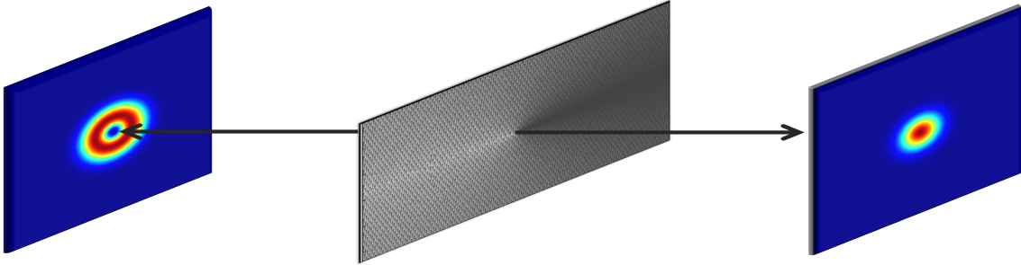
Figure 4.2: Reciprocity of light: Passing a Gaussian through a hologram would result in a particular desired mode. When reversing the procedure, and passing this mode through the hologram with the conjugate phase of the current mode encoded on it, the returned mode would then be a Gaussian again.
