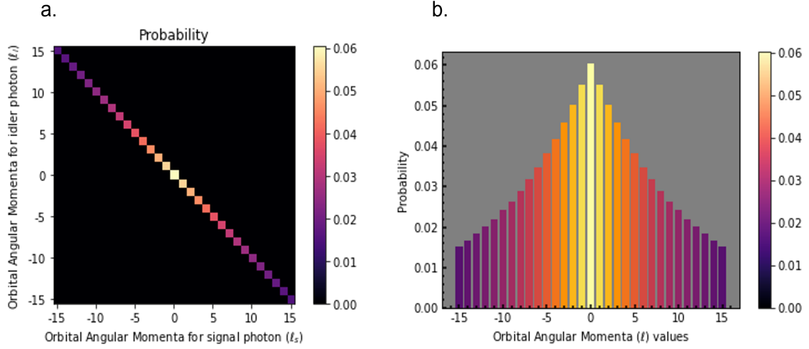
Figure 3.2: Theoretical spiral bandwidth plots: The concept of the OAM spectrum is depicted here. This is for the case when \ell_p = 0 . As discussed, the probability is maximum at the centre when \ell_s = \ell_i = 0 and drops off for higher order modes. The reason that we only have an anti-diagonal in a . in this case is due to the restriction imposed on the values of \ell_s and \ell_i . Since there are only elements along the anti-diagonal, it is easy to visualize a 2D cross-sectional probability distribution as show in b .
