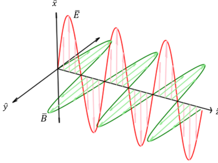
Figure 1.4: Electric and magnetic field oscillation: The electric ( \vec{E} ) and magnetic fields ( \vec{B} ) oscillate perpendicular to one another, and the direction of propagation ( \hat{z} ).
