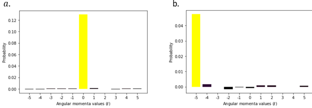
Figure 4.9: Cross-sections of the \ell = \{-5, 5\} spectrum: The cross-section in a. shows the well defined peak at \ell_s = 0 , where the cross-section has also been created by looking at the elements corresponding to \ell_i = 0 . It can be seen that most elements, other than the peak, is near but not precisely at 0. The same trend can be seen in b. only this time with the defined peak at \ell_s = -5 for the cross-section about \ell_i = 5 .
