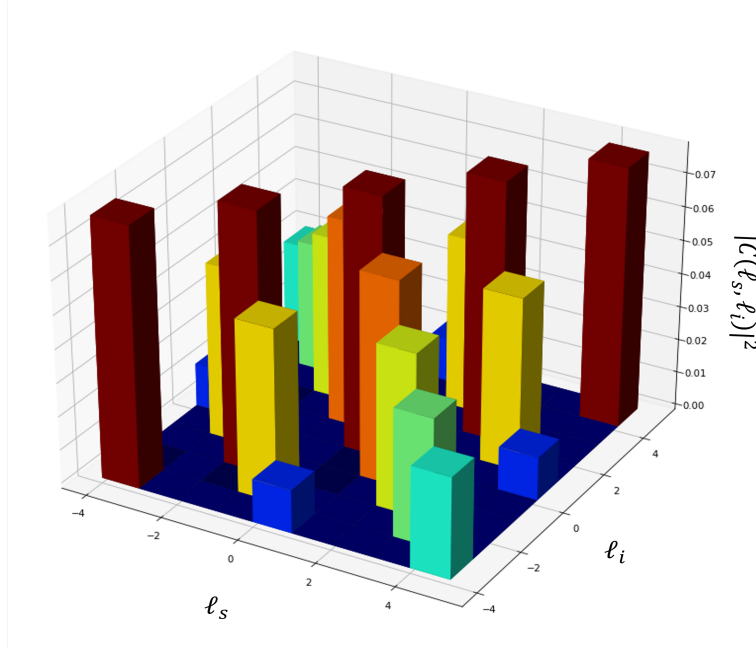
Figure 5.1: LG spectrum from \ell_{s,i} = -4 to \ell_{s,i} = 4 : The desired spectrum with equalized coefficients C_{-4,-4} = C_{-2,-2} = C_{0,0} = C_{2,2} = C_{4,4} = \frac{1}{\sqrt{5}} is shown here.
