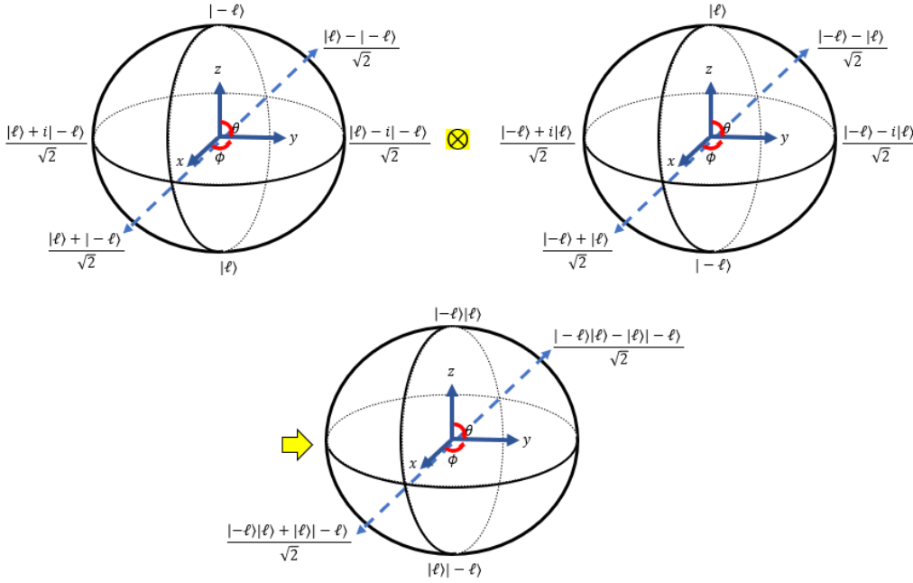
Figure 3.5: Higher Order Bloch Sphere: This depicts what is meant by the higher order Bloch sphere. The states on the surface of the first two Bloch spheres represent the state of each individual photon respectively. The substates |l\rangle are used since the OAM subspace is used.
