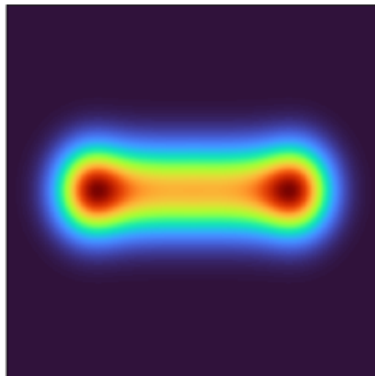
Figure 5.4: HG pump profile: The pump profile for the chosen desired spectrum whose coefficients are given by C_{0,0} = C_{1,1} = C_{2,2} = C_{3,3} = C_{4,4} = C_{5,5} = C_{6,6} = C_{7,7} = C_{8,8} = \frac{1}{\sqrt{9}} .
