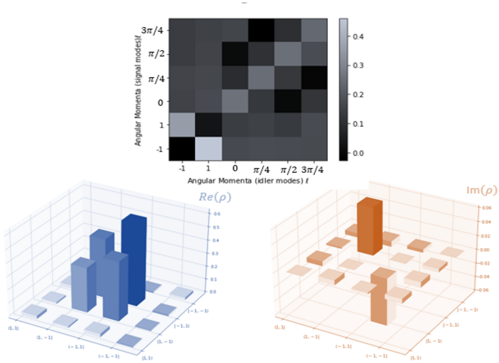
Figure 4.13: 2D QST: This figure shows a QST measurement, as well as the reconstructed real and imaginary density matrices for the basis states \ell = 1 and \ell = -1 . The blocks with labels 0, \frac{\pi}{4}, \frac{\pi}{2}, and \frac{3\pi}{4} correspond to the phase difference between the superposition states (blocks with 1 and -1 ).
