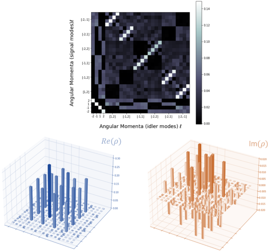
Figure 4.15: 4D QST: A 4D QST and its density matrices are shown here.
