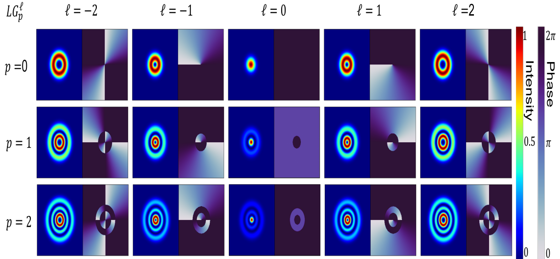
Figure 1.3: Laguerre-Gaussian modes: The left side in each image represents the intensity profile of the LG beam, while the right side represents the phase profile. It is clearly noticeable that the intensity profile is the same for \ell values of opposite sign, but the phase profiles are not. The optical vortex also becomes larger for a higher topological charge \ell , and when we increase the radial index p , rings are added around the initial doughnut structure.
