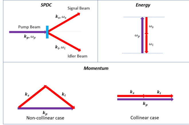
Figure 3.1: Spontaneous Parametric Down Conversion: The concept of SPDC is illustrated as well as the momentum and energy conservation between the signal, idler, and pump beams.
