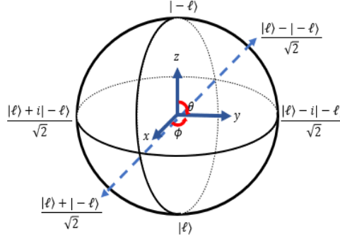
Figure 3.3: Bloch Sphere: This demonstrates what is meant by the Bloch sphere. The states on the surface of the Bloch sphere represent the state of the photon. The substates |\ell\rangle are used since one works in the OAM subspace.
