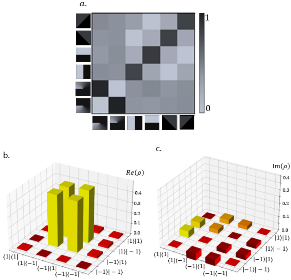
Figure 3.6: Two-Dimensional QST: This shows the full tomography measurement of the coincidence counts of an entangled two-photon system, projected into the measurement states corresponding to the given phase maps (a.), as well as the real (b.), and imaginary (c.) components of the density matrix.
