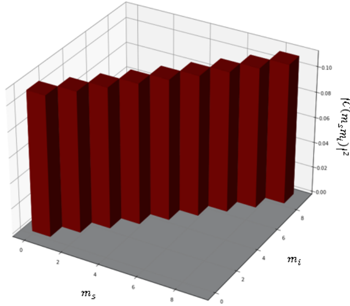
Figure 5.3: HG spectrum from m_{s,i} = 0 to m_{s,i} = 8 : The desired spectrum with coefficients C_{0,0} = C_{1,1} = C_{2,2} = C_{3,3} = C_{4,4} = C_{5,5} = C_{6,6} = C_{7,7} = C_{8,8} = \frac{1}{\sqrt{9}} is shown here.
