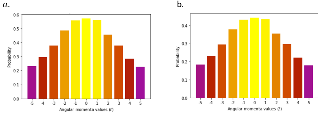
Figure 4.8: Accidental component of the coincidence counts: a. gives an indication of the spiral bandwidth with the accidentals not being removed from the data. b. shows what the spectrum of only the accidental coincidences looks like. Clearly the contribution of the accidentals cannot be noticed by simply examining the spectrum from Figure 4.7 c. One has to explicitly aim to notice this contribution which could potentially result in a large error if this is not accounted for.
