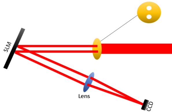
Figure 2.4: Calibration setup: It can be seen here that an expanded beam passes through a double pinhole, creating two thinner beams hitting either side of the SLM and reflecting off of it. These two beams pass through the same lens and focuses to the same point, at which a CCD camera is placed.
