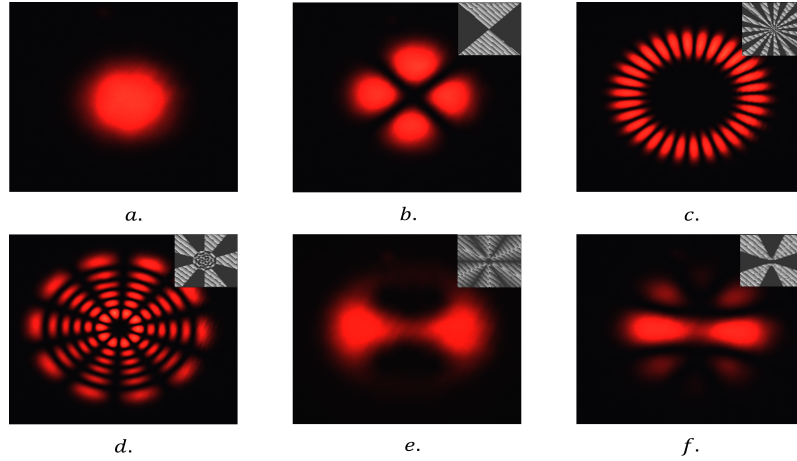
Figure 2.7: Generated modes: Each of these images shows a different mode to which the light intensity profile was shaped. The holograms corresponding to the modulated modes, other than the Gaussian mode, is given on the inset of each image.
