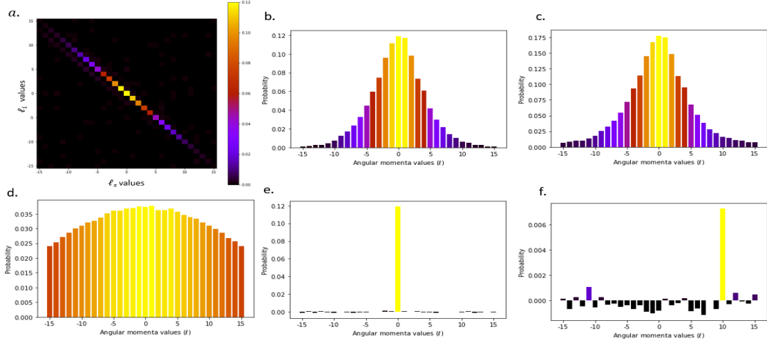
Figure 4.10: Spiral bandwidth analysis for \ell = \{-15, 15\} : a. is once again the OAM intensity spectrum and b. is the corresponding spiral spectrum for the entangled photons. c. shows the spectrum when the accidentals are included in the data set and d. is the spectrum showing the contribution of only the accidentals. Cross-sections of the spiral bandwidths about \ell_i = 0 and \ell_i = -10 is shown in e. and f. respectively.
