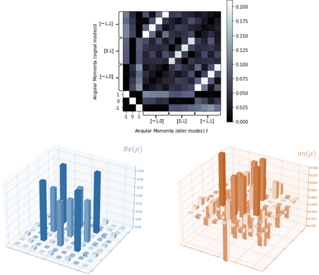
Figure 4.14: 3D QST: A 3D QST measurement is displayed with its corresponding density matrices. The labels denoted with square brackets show which OAM states are superpositioned with one another.
