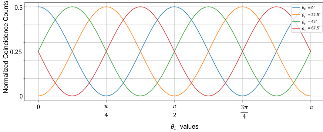
Figure 3.4: Bell Measurement: This is a simulated perfect Bell measurement case displaying the trend of the bell measurement curve. The normalized coincidence counts would usually be plotted as a function of the relative angle between the superposition of OAM states. The \theta_s (corresponding to the signal photons hitting its SLM) values are kept at a constant value, while the \theta_i (corresponding to the idler photons hitting its SLM) values are varied. This is done for four cases of \theta_s = \{0, \frac{\pi}{4}, \frac{\pi}{2}, \frac{3\pi}{4}\} .
