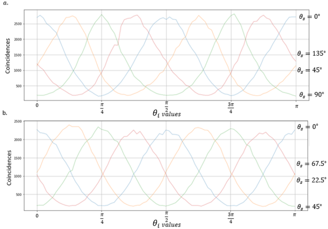
Figure 4.12: Bell measurements using the CHSH inequality: These results show the normalized coincidence counts plotted as a function of the \theta_i values while keeping the \theta_s values constant as shown in the legends. This is done for the |\ell| = 1 subspace in a. and the |\ell| = 2 subspace in b.
