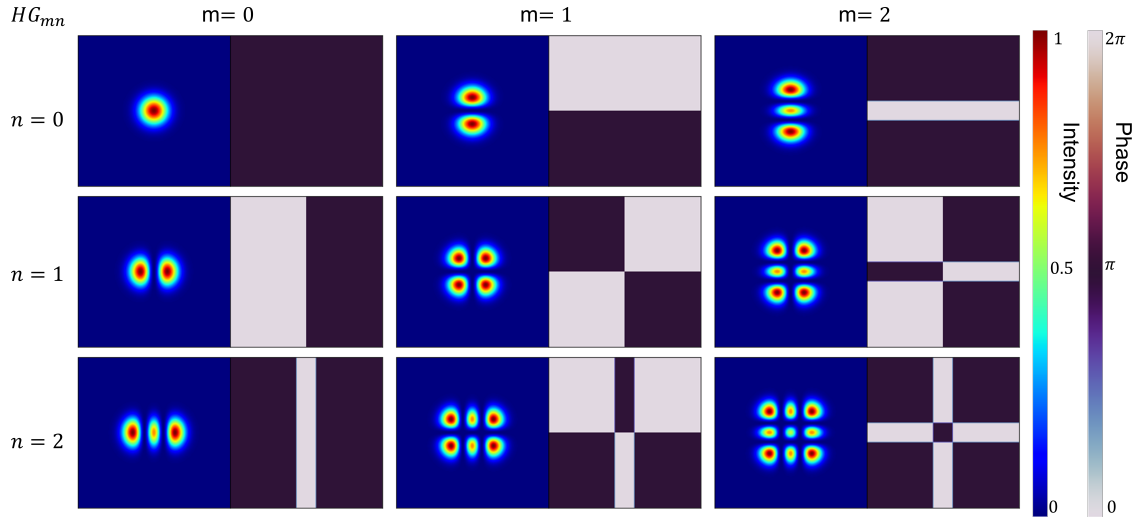
Figure 1.1: Hermite-Gaussian modes: These are the intensity profiles (left) and phase profiles (right) of the Hermite-Gaussian modes. They are respectively determined by the equations from before, (1.15) and (1.16). A trend can be seen where the n index dictates the amount of dark nodes in the horizontal direction and m the amount of dark nodes in the vertical direction [10].
