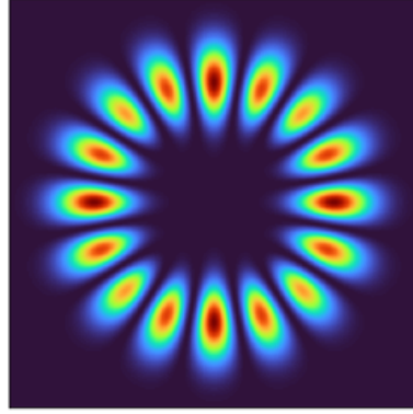
Figure 5.2: LG pump profile: The requisite pump profile for the chosen desired coefficients C_{-4,-4} = C_{-2,-2} = C_{0,0} = C_{2,2} = C_{4,4} = \frac{1}{\sqrt{5}} .
