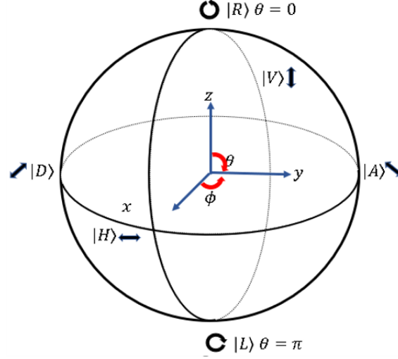
Figure 1.5: Poincaré sphere: By setting \theta = 0 with \phi = 0 , and examining the sphere, the state corresponding to right circular polarization is realized. This logic can be repeated for all other states by simply searching for the desired polarization state on the surface of the sphere, and reading off the respective corresponding \theta and \phi values.
