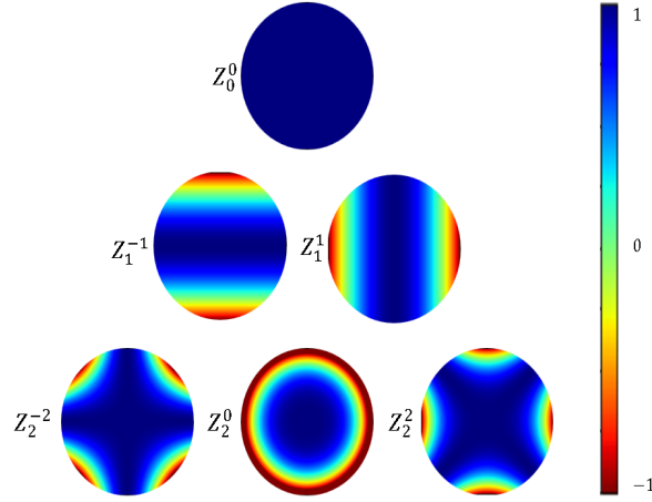
Figure 2.6: Zernike modes: These represent the contribution of the main lower order Zernike modes to what the wavefront would like. These are thus also the modes one would adjust to correct for the corresponding aberration. The Z_0^0 mode is usually referred to as the piston mode. When one would like to correct for squashing in either the vertical or horizontal direction, the y-tilt ( Z_1^{-1} ) and x-tilt ( Z_1^1 ) is respectively adjusted. To correct for astigmatism either the Z_2^{-2} mode or Z_2^2 mode is adjusted, and if the aberration occurs in the centre, the defocus ( Z_2^0 ) is used [44, 45].
