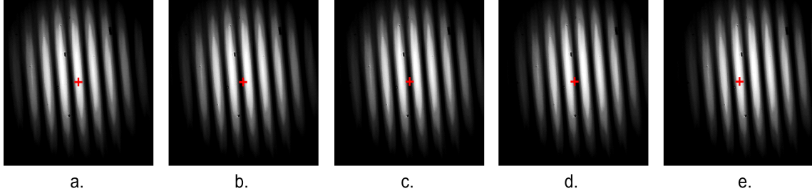
Figure 2.5: Shifting fringes during calibration: The red crosshair represents the reference point about which the fringes shift. The goal is to set the voltages of the SLM such that with a 2\pi phase shift, the crosshair appears on the bright fringe next to the initial one. These images show the crosshair at various locations as the phase shift was changed. The phase shifts in a , b , c , d , and e are 0, 0.5\pi, \pi, 1.5\pi , and 2\pi respectively.
