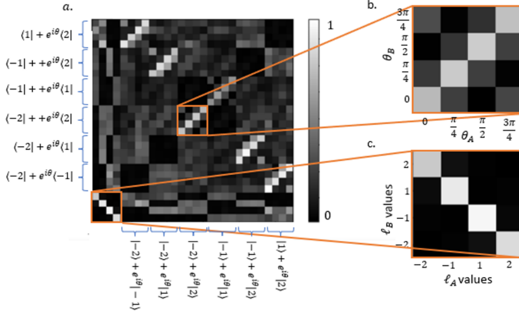
Figure 3.7: 4-dimensional QST: This shows the complete QST measurement (a.) for a four-dimensional ( \ell = \{-2, -1, 1, 2\} ) case of a two-photon entangled system. The block in (c.) represents the four pure states (The bras and kets are omitted for notational simplicity). Each mini block indicates the normalized coincidence counts for the corresponding states. The block in (b.) shows how the QST measurement can be read, in terms of the superposition of two states. The equations in (a.) display the superposition OAM states that correspond to each curly bracket.
