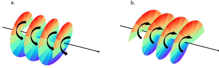
Figure 1.2: Twisting OAM wavefront: This shows what is meant by the twisting of light. The wavefront forms a helix about the direction of propagation. It can easily be noticed that for \ell = 1 (a.), the helix spirals clockwise and for \ell = -1 (b.) the helix spirals anti-clockwise.
