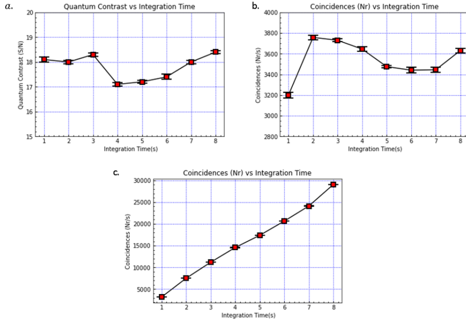
Figure 4.5: Integration time dependence: In a , the plot of the quantum contrast vs the integration time is shown. In b , the numbers of coincidences per second is plotted against the integration time. In c , a plot of the total coincidence counts as a function of the changing integration time can be seen.
