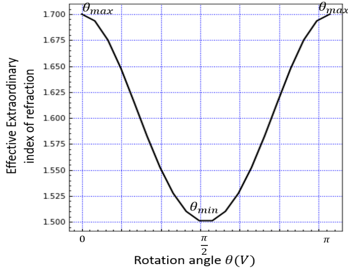
Figure 2.1: Liquid crystal rotation: The effective extraordinary index of refraction varies as the rotation angle changes. The choice for the refractive indices, merely for demonstrative purposes, were n_e = 1.7 and n_o = 1.5 . This rotation angle is further affected by the applied voltage to the liquid crystals. There is clearly a minimum and maximum value for the refractive index corresponding to different rotations of the liquid crystal.
