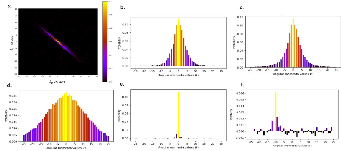
Figure 4.11: Spiral bandwidth analysis for \ell = \{-25, 25\} : The OAM intensity spectrum is presented in a. while b. shows the corresponding spiral spectrum. In c. and d. one can see the spiral spectrum of the total coincidences and accidentals respectively. The spectrum of the cross-section about \ell_i = 0 is shown in e. , and about \ell_i = 10 , whose corresponding highest peak is at \ell_s = -10 , is shown in f.
