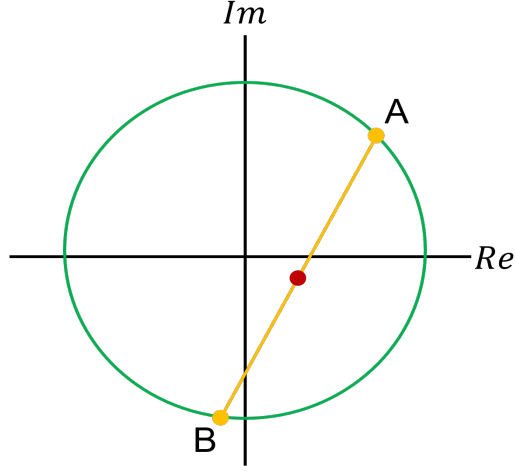
Figure 2.3: Phase and Amplitude Modulation: The green circle shows the unitary circle that defines phase only modulation. To perform the amplitude modulation as well involves moving to a point within this circle (the brown dot) say between two points A and B . This can be generalized for any position within the circle allowing one to effectively modulate to attain any phase and amplitude required.
