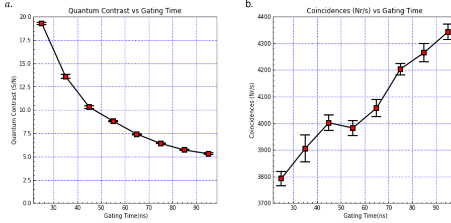
Figure 4.6: Gating time dependence: In a. a plot of the quantum contrast as a function of the gating time is shown, while b. shows the plot of the coincidences as a function of the gating time.
