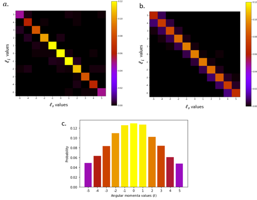
Figure 4.7: Spiral bandwidth for \ell = \{-5, 5\} : a. displays the OAM intensity spectrum when the measurement is made in a completely dark room. In b. one can see an OAM intensity spectrum where external light sources have been introduced. The spiral bandwidth for the 'good' case (shown in a. ) is shown in c.
