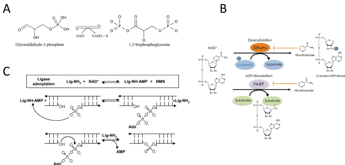
Fig. 3. Biochemical reactions demonstrating the biological roles of NAD + . A. NAD + serves as a coenzyme during the conversion of glyceraldehyde 3-phosphate to 1,3-bisphosphate by the enzyme glyceraldehyde phosphate dehydrogenase, reducing NAD + to NADH. B. The depiction illustrates NAD + functioning as a substrate for the enzymes Sirtuins (Sir2) and ADP-ribose transferases, wherein it donates ADP-ribose. C. Bacterial DNA ligases employ NAD + as a cofactor for the adenylation of the ligase active site, resulting in the formation of an adenylated nicked substrate [24].
