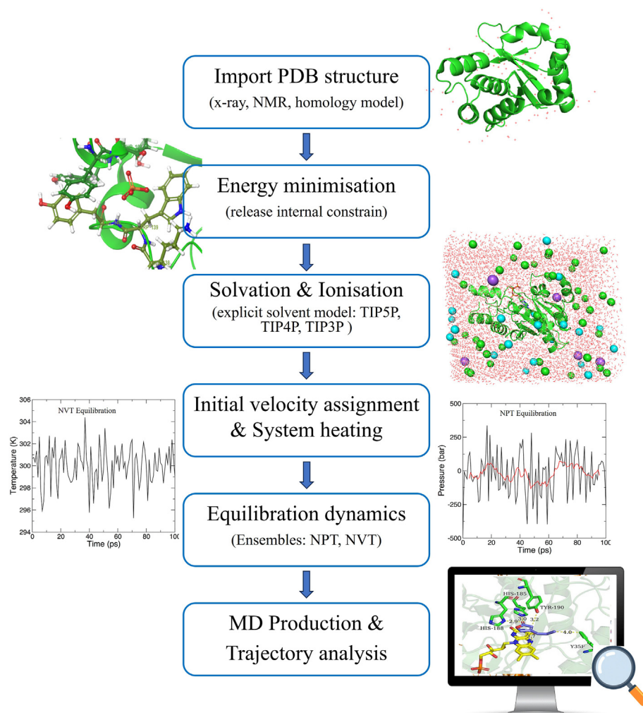
Fig. 11. Illustrates a schematic depiction of the sequential steps encompassed in molecular dynamics (MD) simulation of a protein according to Patodia [86], NMR, Nuclear magnetic resonance; MD: Molecular Dynamics; NVT: Number of molecules/atoms in assembly, Volume, Temperature; NPT: Number of molecules/atoms in assembly, Pressure, Temperature; TIP3P/4P/5P: Transferable Intermolecular Potential 3/4/5-site water models.
