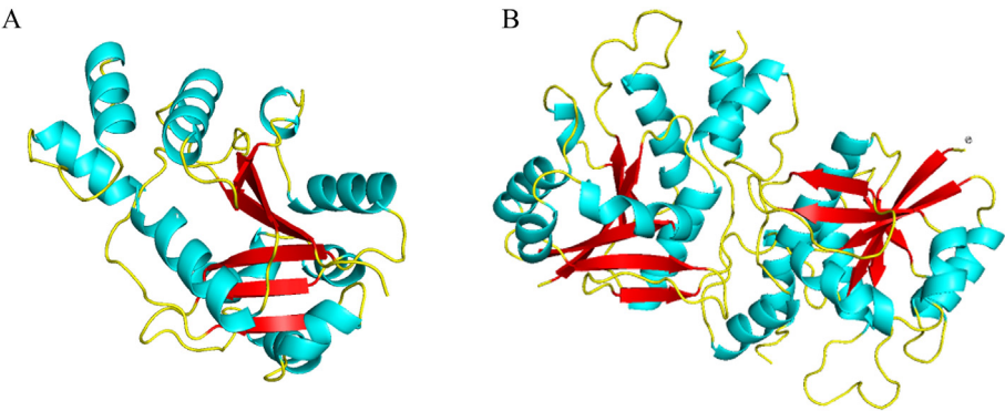
Fig. 7. Homology Model of (A) KpNNAT and (B) EfNNAT. The KpNNAT model was constructed using the 1k4k.4A template and EfNNAT using the 2qtn.1A model. The \alpha -helices are depicted in cyan, red repr; reds the \beta -strands, and the ordered coils in yellow. Both homology models were generated via SwissModel.
