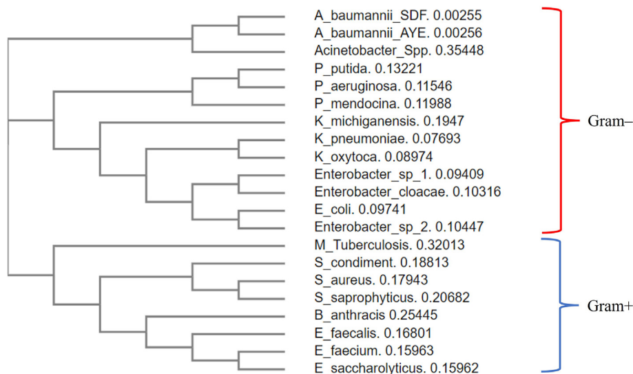
Fig. 1. A phylogram depicting the evolutionary divergence of NNAT across various bacterial species, highlighting the differentiation between Gram-positive and Gram-negative bacteria. The numerical values shown in the figure correspond to the distances between sequences. The similarity between sequences increases as the numerical values approach each other. The Clustal Omega multiple sequence alignment tool was utilised to conduct the analysis [17].
