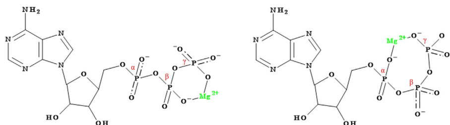
Fig. 10. The structural representation of the various isomeric configurations of the ATP-Mg^{2+} complex. According to Jeremy M. Berg [60], enzyme binding can be facilitated by the direct coordination of Mg^{2+} with either of the two oxygen atoms in the phosphate group, depending on the specific enzyme.
