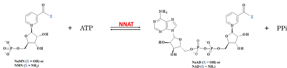
Fig. 6. The enzymatic reaction facilitated by nicotinate/nicotinamide mononucleotide adenylyltransferase. The provided diagram illustrates the catalytic reaction of the NNAT enzyme involving two substrates, leading to the synthesis of either \text{NAD}^+ or NaAD [41].
