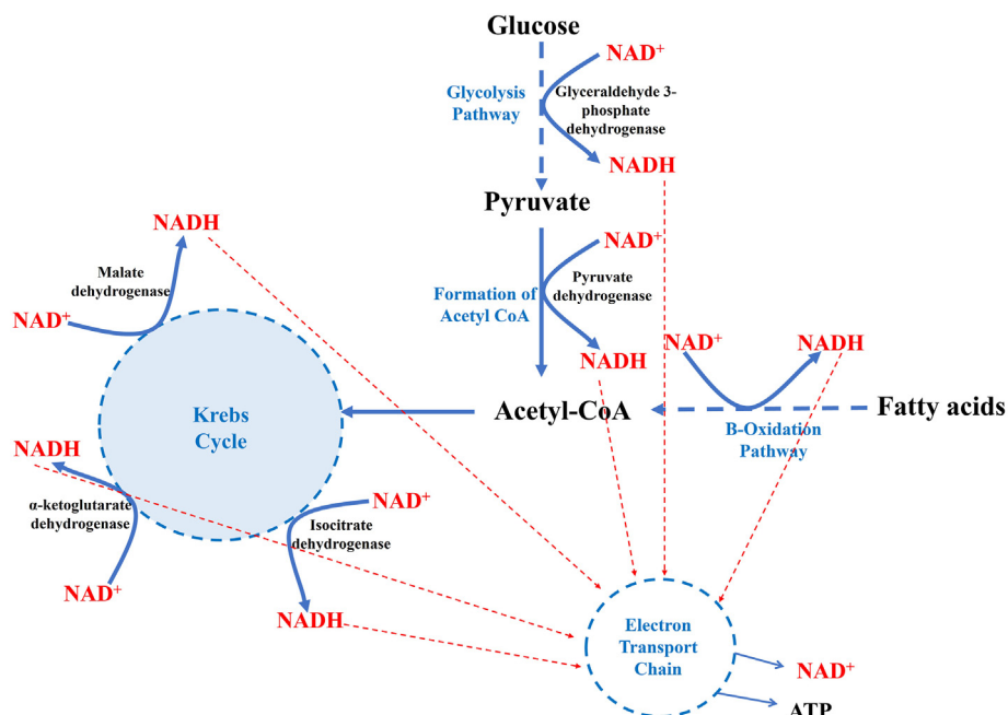
Fig. 4. A schematic illustration of interconnected metabolic pathways involving the redox activity of \text{NAD}^+/\text{NADH} for energy generation [27,28].
