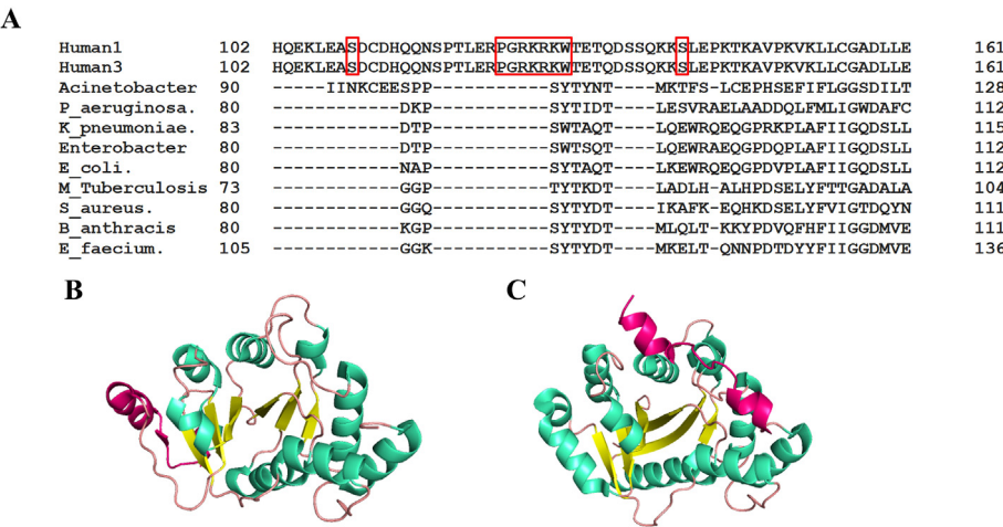
Fig. 9. Sequence Alignment and structural comparison of bacteria NNAT and human NMNAT. (A) The nuclear localisation signal (NLS) sequence and the two phosphorylation site serine residues conserved to the hNMNAT are indicated in the red box. The regions with no corresponding residues are designated in space. Ribbon representation of (B) E. coli NNAT (1k4k) and (C) human NMNAT (1kq0) protomer structure showing their structural difference. The secondary structures are labelled green for helices, yellow for strands, and salmon for the random coils. The region in hot-pink indicates the portions that are not present in both structures ( \alpha\beta\gamma insertion in E.coli NNAT and the C-terminal helical structure extension in the human NMNAT). RMSD = 15.755 Å (492–492 atoms) [49].
