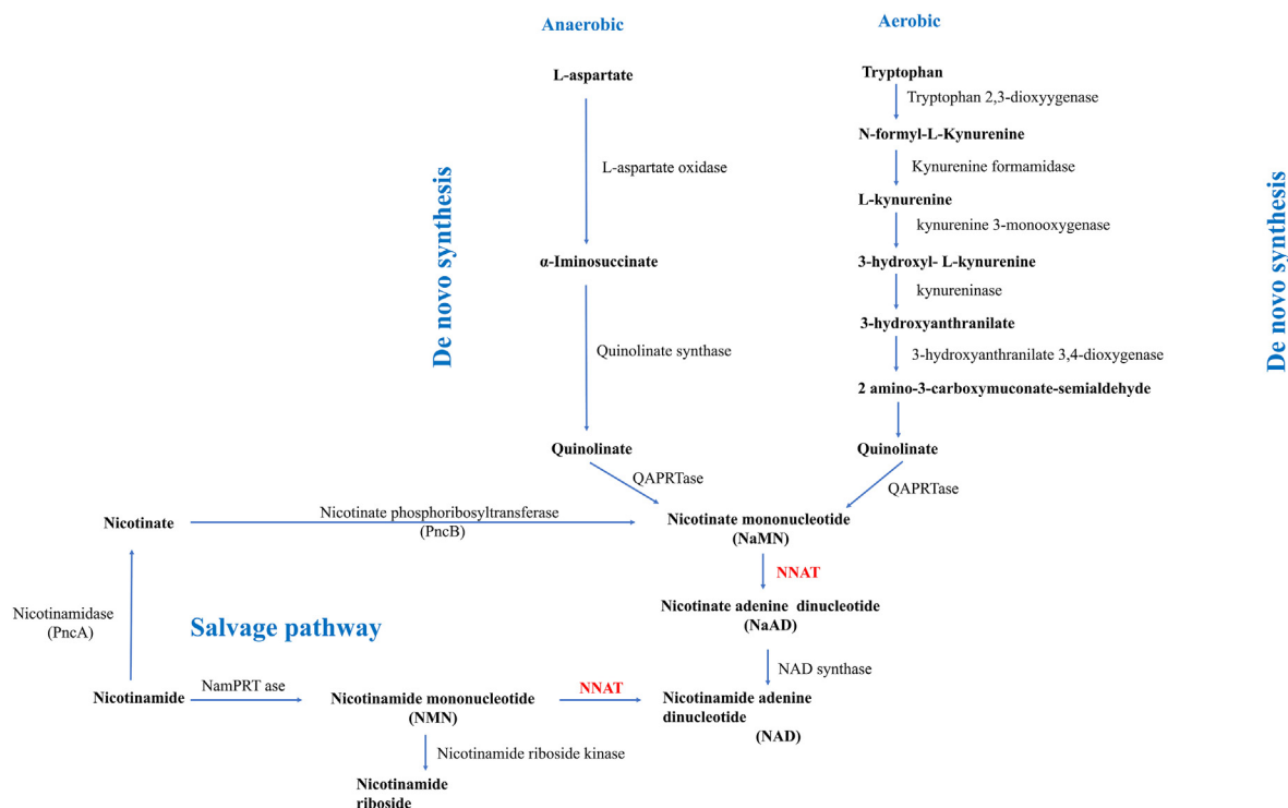
Fig. 5. A schematic representation illustrating de novo processes and salvage synthesis of NAD + in bacteria and humans. Source [36].
