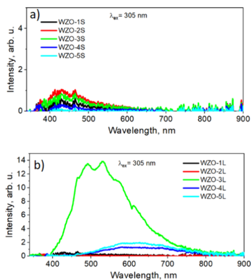
Figure 8. Photoluminescence spectra of the various WZO nano-heterostructures. (a) Small particle sizes and (b) large particle sizes.
