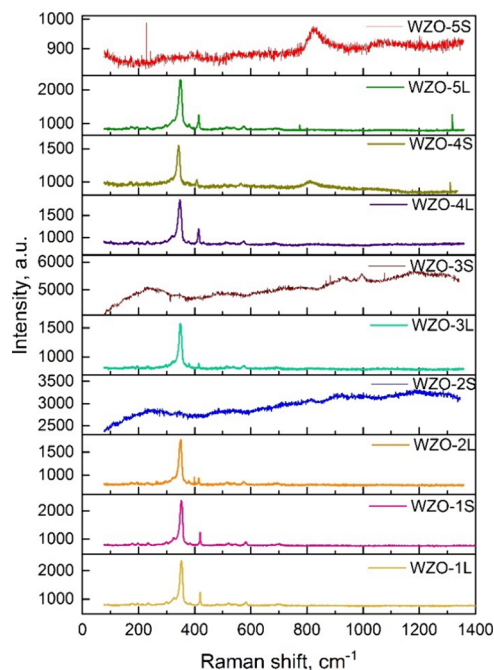
Figure 5. Raman spectra of the prepared WZO nanoheterostructures.
