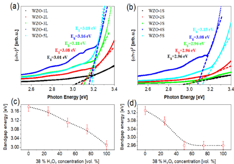
Figure 7. Tauc plots of the WZO heterostructures with various size fractions (a, b). Variation of the bandgap energy of WS 2 –ZnO nanoheterostructures according to the H 2 O 2 concentration of the original 38% solution used in the ESE procedure (c, d).
