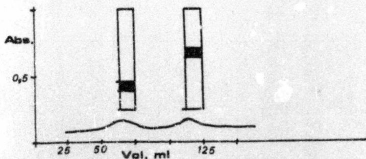
Fig. 20. Elution pattern of fractions 13 and 16 obtained by preparative gel electrophoresis with SDS.
