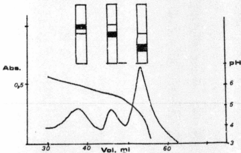
Fig. 19. Isoelectric focusing of sample 2 in fig. 18.
