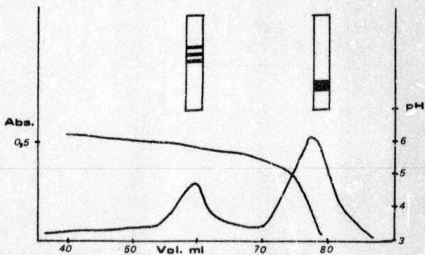
Fig. 22. Elution pattern of B. holubi protein on Sephadex G-100. Tris-HCl buffer, pH 8,0
