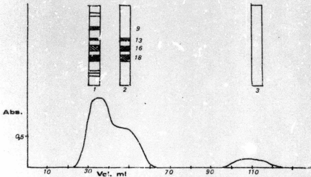
Fig. 18. Elution pattern of L. capensis protein on Sephadex G-100. Tris-HCl buffer, pH 7,5.
