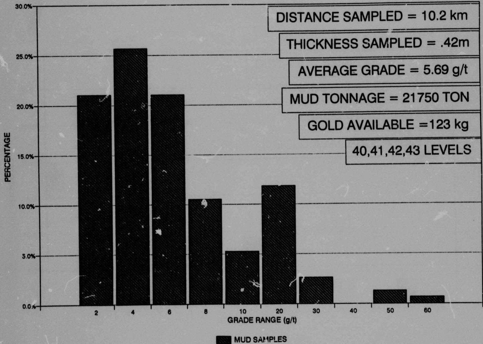
Graph 24. Western Holdings Mine, mud grade distribution.
