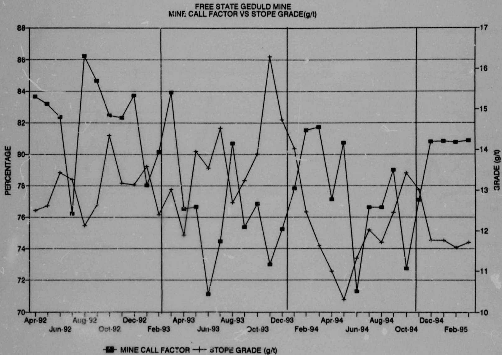
Graph 35. Free State Geduld Mine, MCF vs. stope grade. 1992 to 1995.
