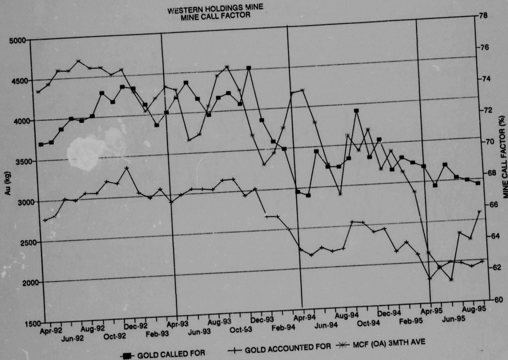
Graph 15. Western Holdings Mine, Gold called for / accounted for / MCF, 1992 to 1995.
