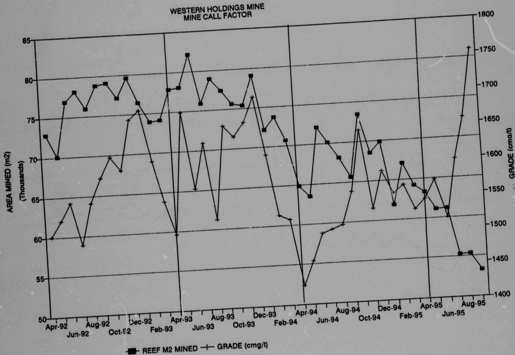
Graph 17. Western Holdings Mine, M 2 vs. slope grade, 1992 to 1995.
