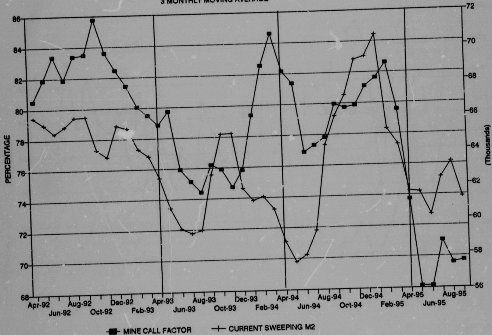
Graph 31. Freddie's Mine, MCF vs. sweepings(m 2 ), 1992 to 1995.
