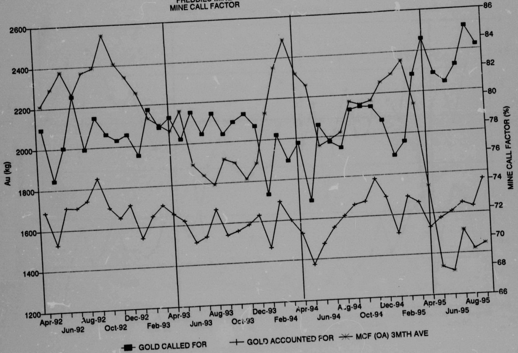
Graph 26. Freddie's Mine, Gold called for / accounted for 1992 to 1995.
