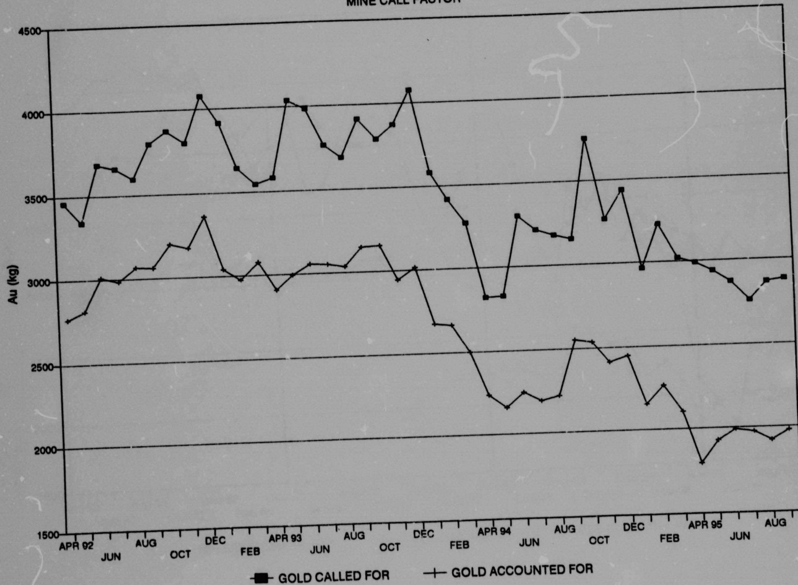
Graph 14. Western Holdings Mine, Gold called for / accounted for, 1992 to 1995.
