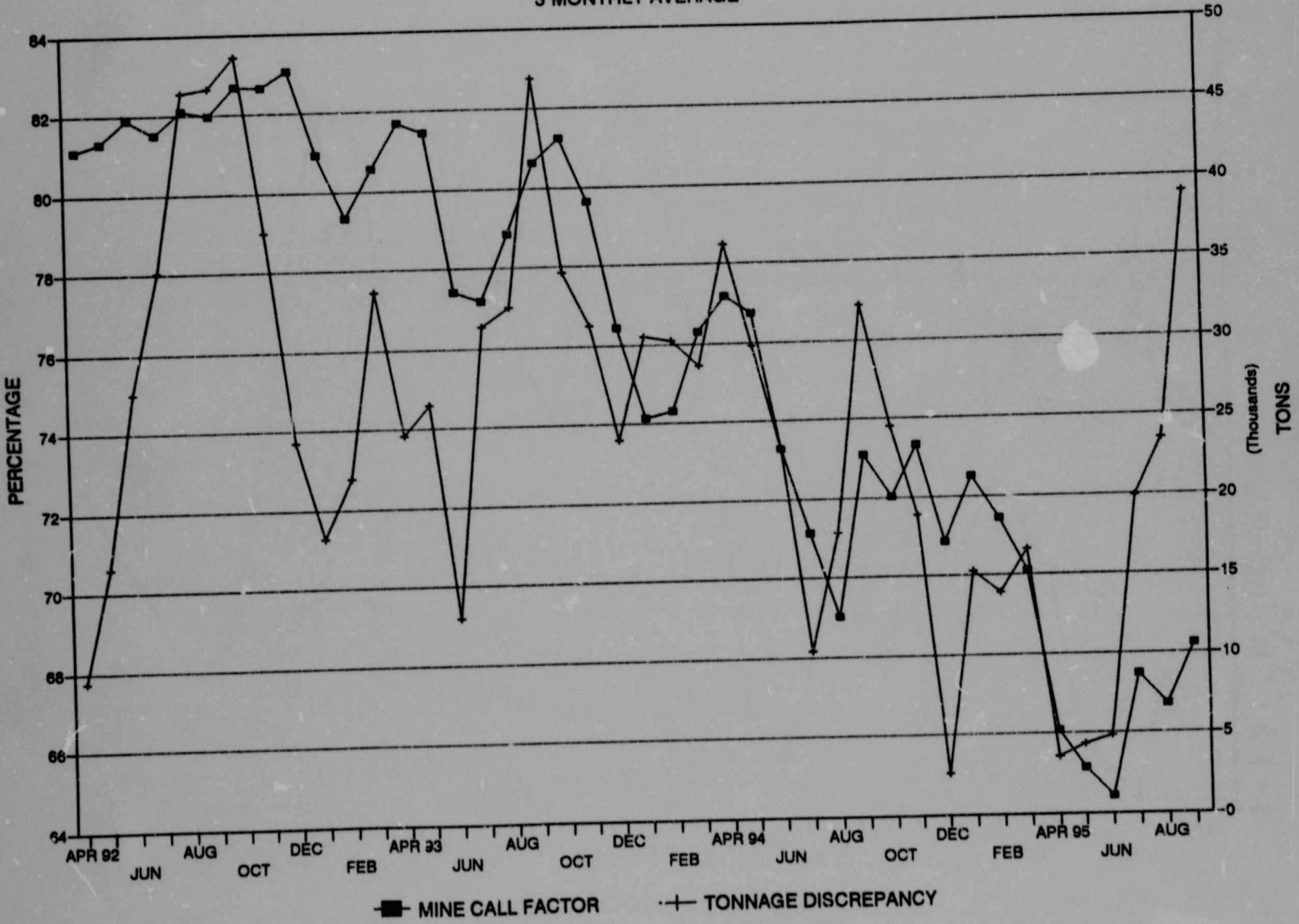
Graph 22. Western Holdings Mine, MCF vs. tonnage discrepancy, 1992 to 1995.
