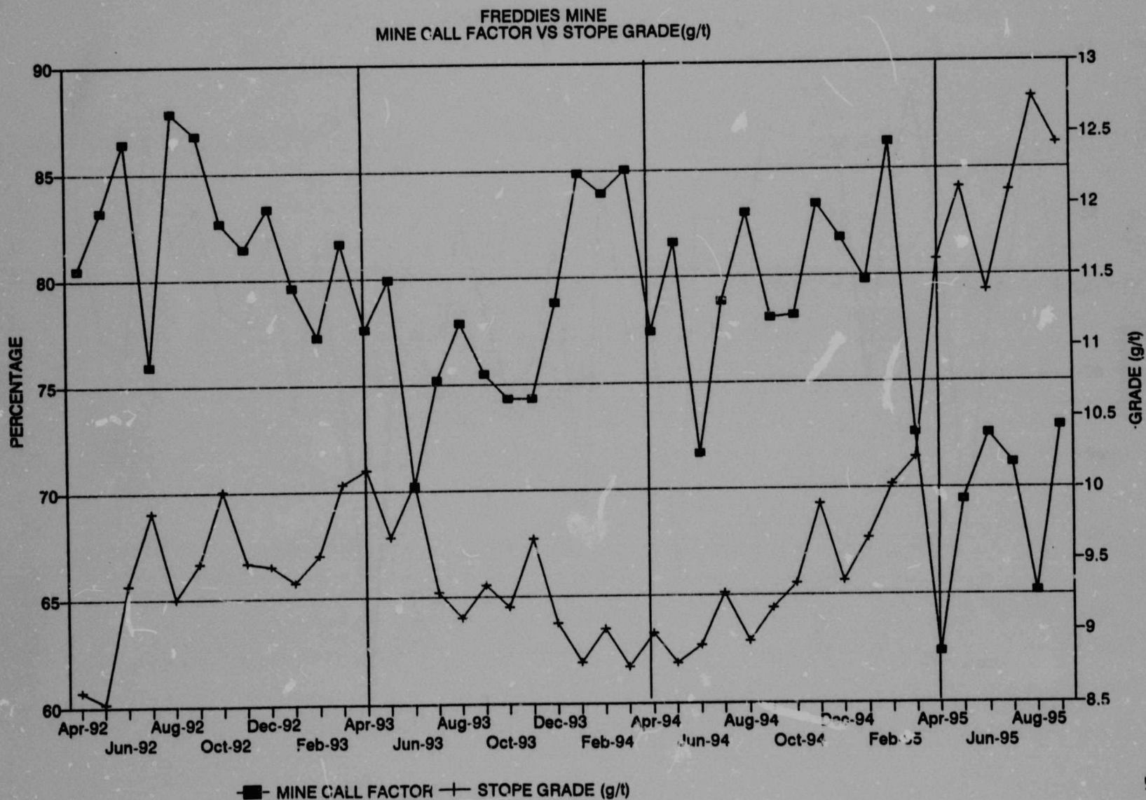
Graph 27. Freddie's Mine, MCF vs. stope grade. 1992 to 1995.
