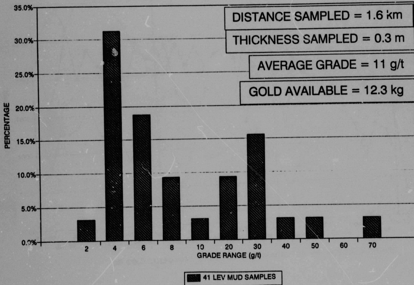
Graph 25. Western Holdings Mine, mud grade distribution.
