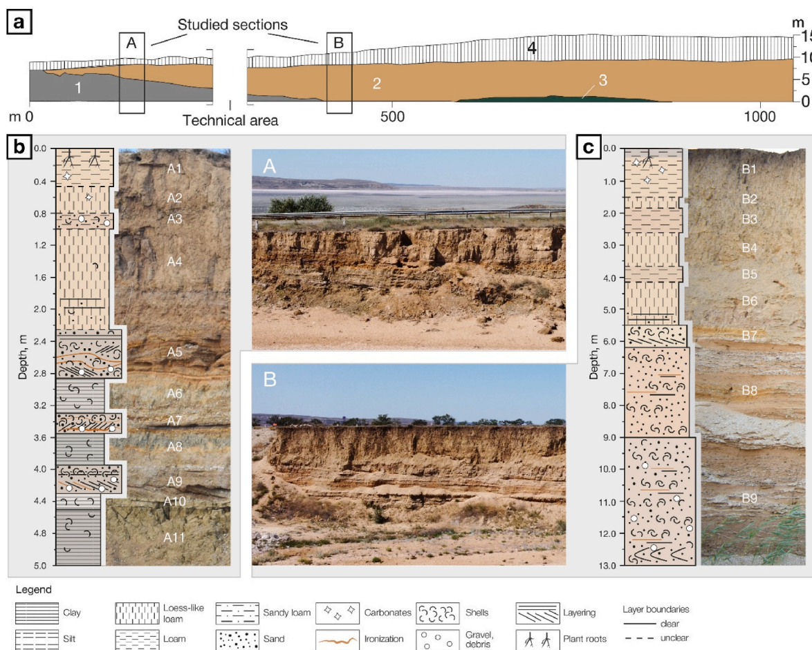
Fig. 4. Eltigen Section: (a) general scheme of the section (Dodonov et al., 2000): 1 — facies variable thickness of alternating sands and clays; 2 — coastal-marine sandy deposits; 3 — Sarmatian clays (Neogene); 4 — loess-soil formation; (b) outcrop A; (c) outcrop B.
