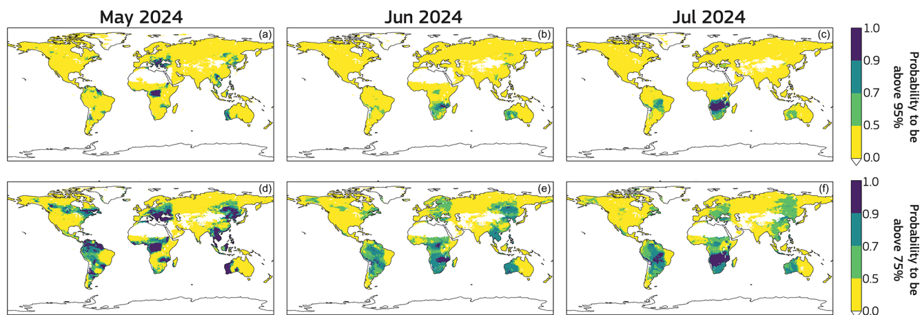
Figure 16. Probability for the monthly average FWI exceeding the (a–c) 95th percentile threshold (anomalous conditions) and (d–f) 75th percentile threshold (extremely anomalous conditions) of the monthly climatological distributions. The probability is calculated using the 51-ensemble-member realisation from ECMWF’s long-range forecasting system, ECMWF-SEAS5 FWI, and comparing it with the 1991–2016 climatology (Copernicus Emergency Management Service, 2019).
