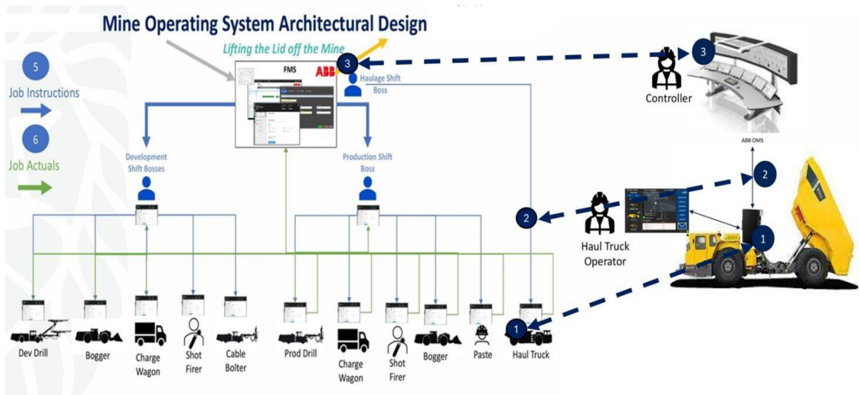
Figure 4.7: Mine System Architectural Design and Underground Automated Hauling Fleet System
