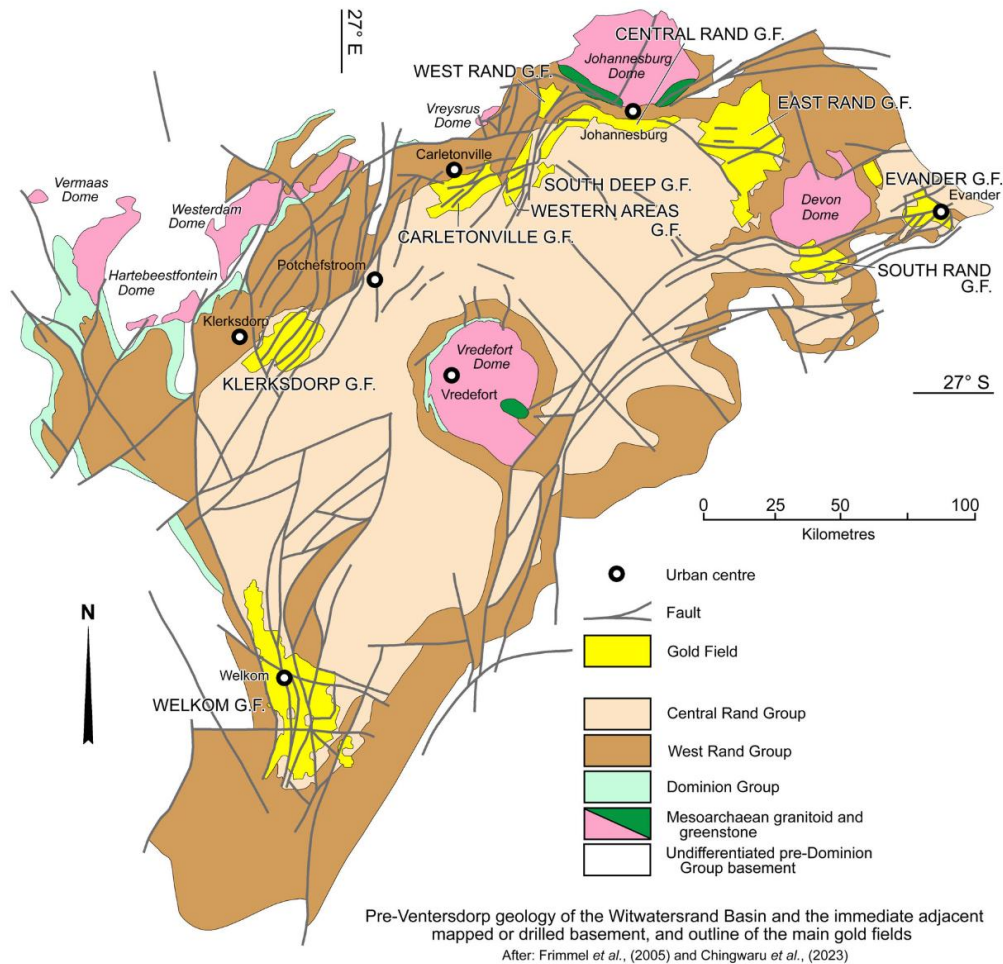
Figure 1.2: Geological map of the Witwatersrand Basin, showing the main gold field of the West Rand
