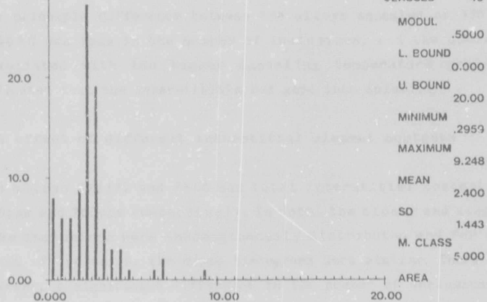
Figure 4.50 Area distribution of needle-like precipitates.
