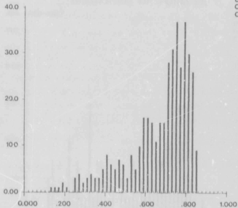
Figure 4.51 Typical shape factor distribution of blocky/round precipitates. The histogram is skewed towards unity (perfect circularity).
