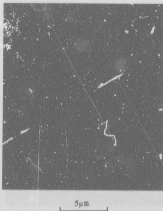
Figure 4.38 Residual grain boundary precipitation in alloy V4/0,1, ductile.
