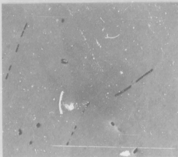
Figure 4.44 (Iron and chromium) oxide inclusions in the V1/1 alloy.
