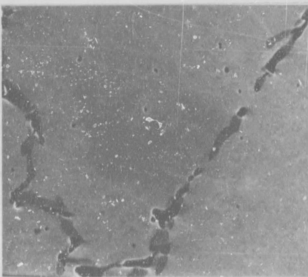
Figure 4.46 Cored oxide inclusions in the V4/O alloy. The cores of the oxides contain less oxygen than the rims.
