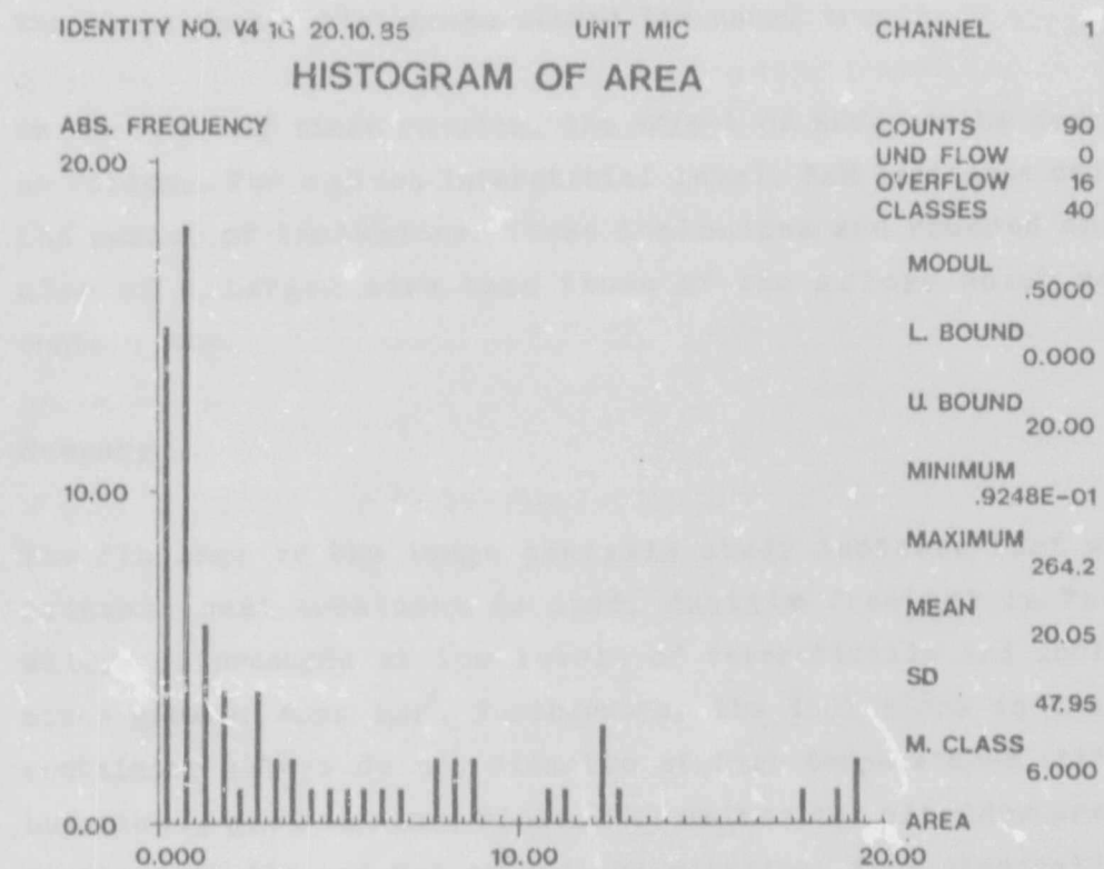
Figure 4.54 Area distribution of a ductile REM-containing alloy. The REM addition separated the inclusions into definite size groupings.
