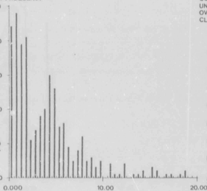
Figure 4.49 Area distribution of round/blocky precipitates
