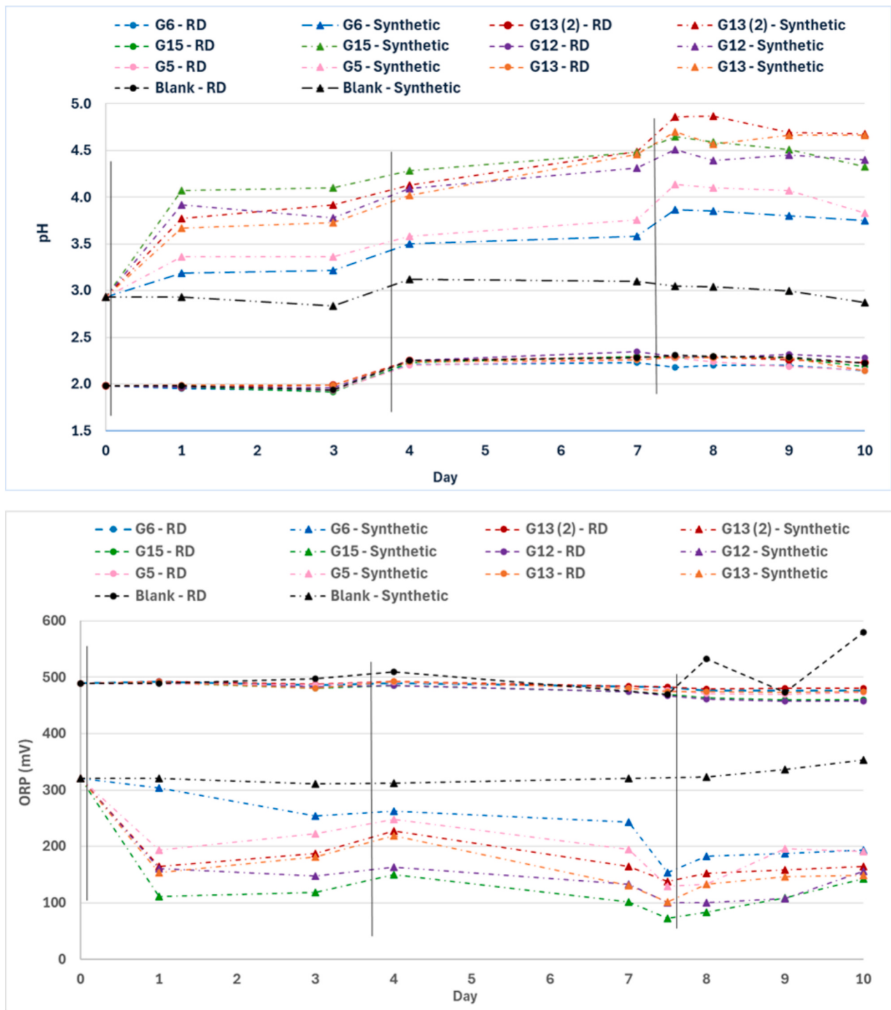
Fig. 3. pH and Eh data for synthetic and return dam (RD) AMD solutions after subsequent grass addition.
