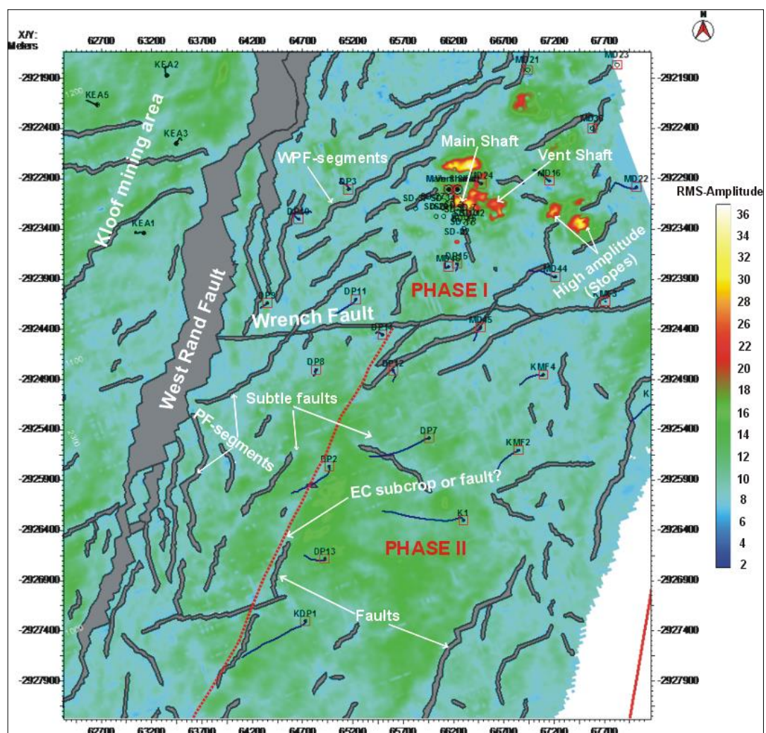
Fig. 8. The VCR map derived from the Root Mean Square (RMS) Amplitude attribute. The map shows detection of subtle faults that fall below seismic resolution limit and location of shaft infrastructures. PF: Panvlakte Fault; WPF: Waterpan Fault.
