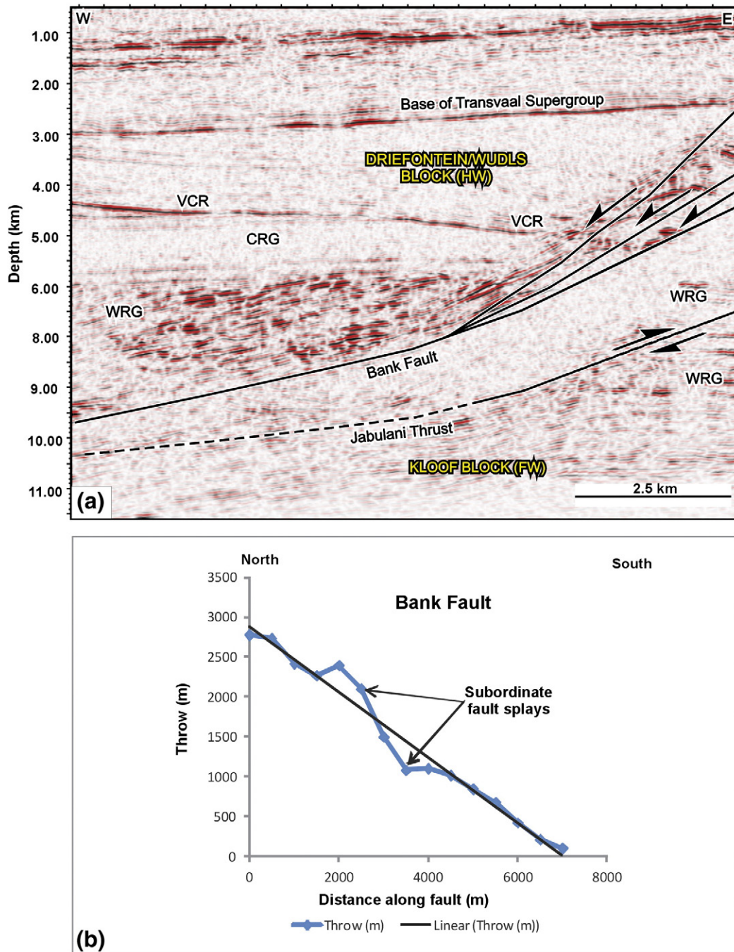
Fig. 4. (a) Seismic section (line CC' in Fig. 1) across the listric Bank Fault, showing the hanging wall (Driefontein/WUDLS) and shallow dipping Jabulani Thrust in the footwall block (Kloof). (b) Displacement (throw) measured in seismic sections perpendicular to the Bank Fault strike at 250 m interval. FW: Footwall; HW: Hanging wall; VCR: Ventersdorp Contact Reef; WRG: West Rand Group; CRG: Central Rand Group.
