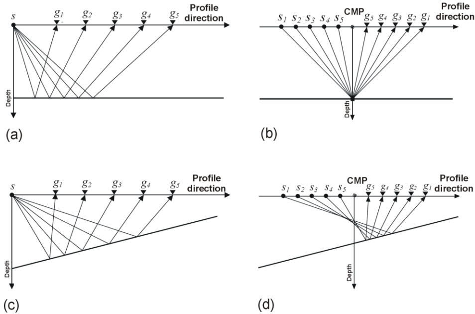
Figure 2.3: Seismic survey geometry. (a) Recording of a single source for a horizontal layer, (b) Common midpoint (CMP) gather for a horizontal layer, (c) Recording of a single source for a dipping layer, (d) Common midpoint gather for a dipping layer. If a horizontally-layered model is considered, rays in a CMP gather are reflected from the same depth point under different angles.
