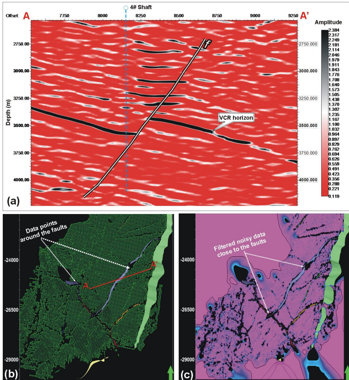
Figure 2.8: (a) Seismic section (amplitude display) across Kloof Gold Mine. (b) Manually picked and autotracked seismic horizon data points. (c) Smoothed horizon by bi-harmonic smoothing operator.
