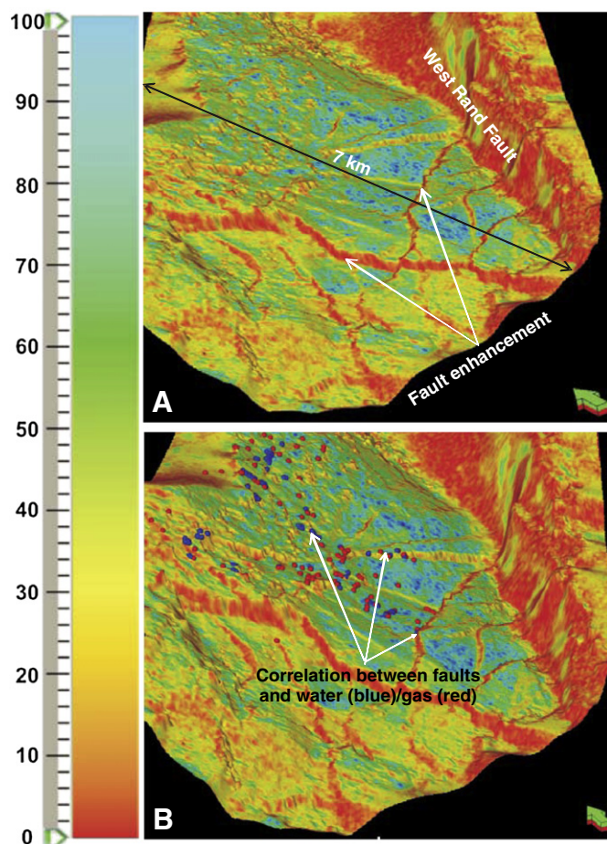
Fig. 12. (A) 3D visualization of the VCR edge attribute map at the Kloof Gold Mine. (B) Edge attribute of the VCR overlain with water and methane data from the Kloof Gold Mine. A number of minor structures show a very good correlation with water and methane data. The edge detection map is the combination of dip and azimuth maps, normalized to the local noise of the surface. The color bar is given in % where low values indicate edges such as faults and dykes. (For interpretation of the references to color in this figure legend, the reader is referred to the web version of this article.)
