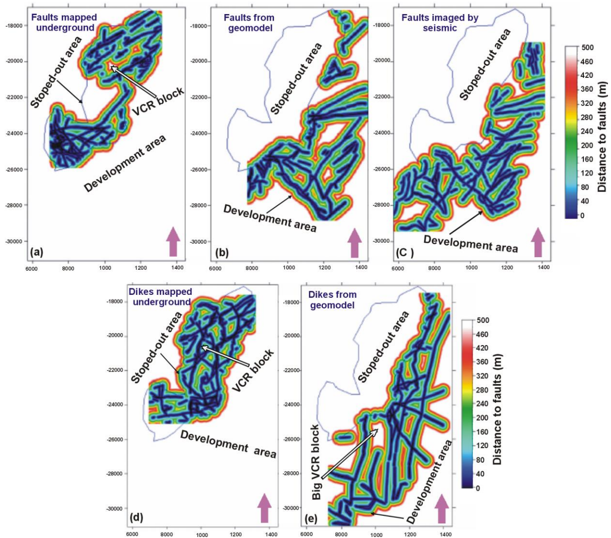
Fig. 13. Fault spacing maps (compartment sizes) for the various structural elements. (a) Faults mapped underground in the stoped-out area. (b) Faults from geomodel in the development area. (c) Seismically-imaged fault in the development areas, note the larger compartment sizes in the seismic model. (d) Dikes mapped underground in the stoped-out areas. (e) Dikes from geomodel in development area.
