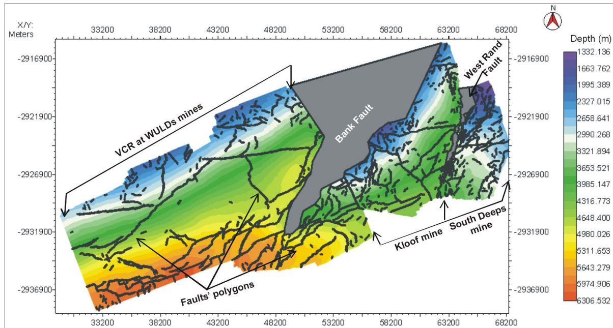
Figure 2.7: Detailed depth structure map of the Venterdorp Contact Reef (VCR) derived from conventional picking across survey areas, showing faults polygons of all strikes and dips.
