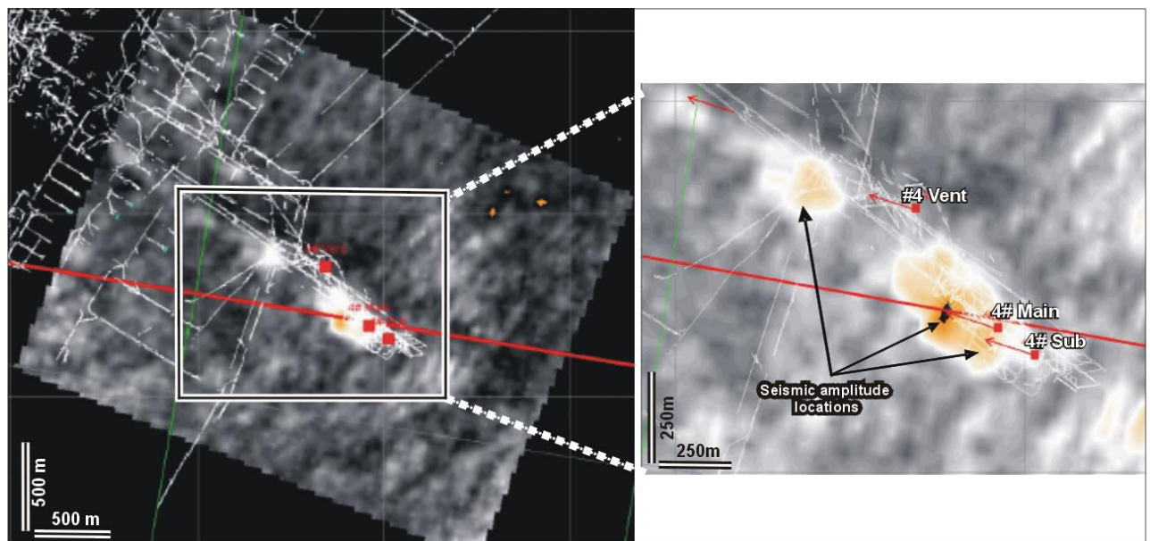
Fig. 10. Seismic volume slice amplitude versus 4 Shaft infra-structure. The multiple high amplitude (hot colours) isolated bodies appear to tie with the shaft barrels but the seismic appears to offset by \sim 200 m to the west and \sim 40 m, to the north.
