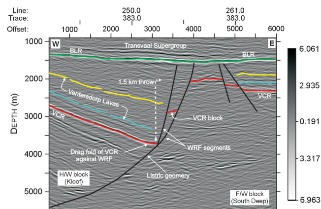
Figure 5. Seismic section (amplitude display) across the West Rand Fault with a throw of 1.5 km in the north of study area, showing sympathetic faults bounding a VCR block in the fault zone.
