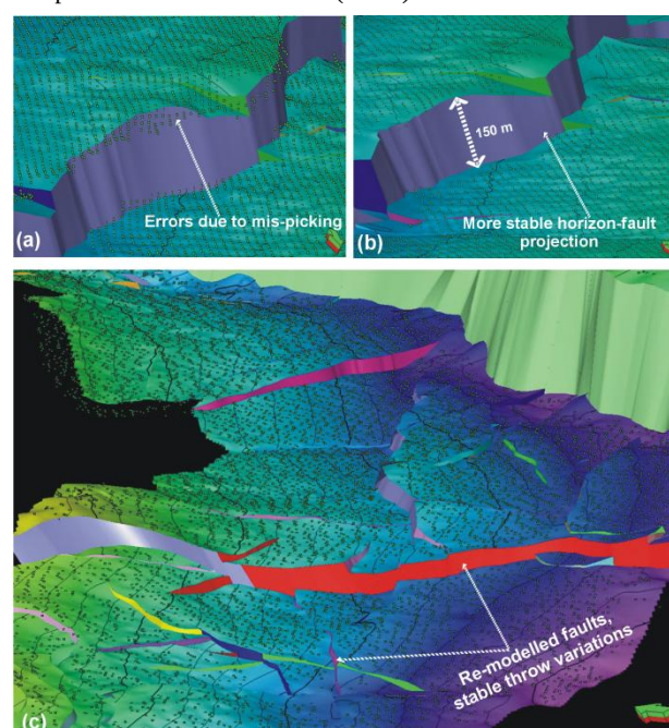
Figure 4. (a) Seismic horizon data points overlap across the fault throw, the dip of the fault is thus in error. (b) Horizon is projected in a sensible manner to the fault. (c) Re-modelled faults and horizon, showing the stable throw variations.
