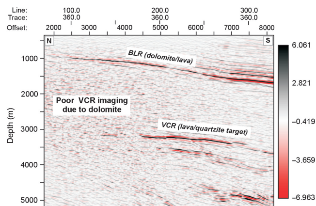
Figure 4. North-south depth-converted PSTM section (amplitude display) clearly showing poor VCR imaging over dolomite outcrop area.
