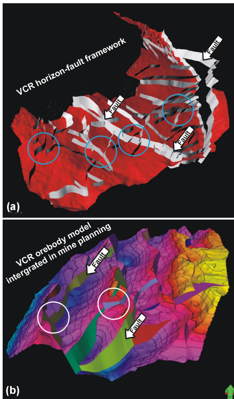
Fig. 15. Final orebody model integrated into data mine packages. (a) The VCR surface and faults are in Auto Cad package in the mine datum. (b) Direct integration in mine planning.
