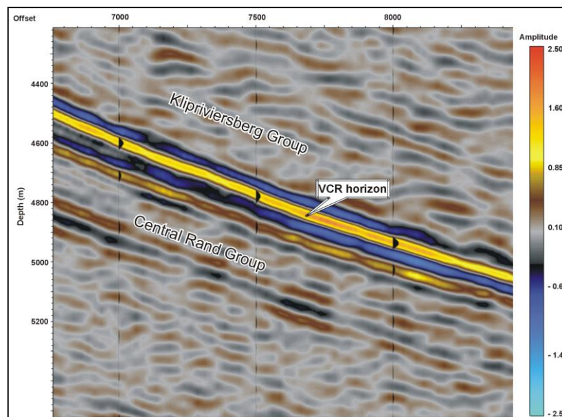
Figure 2.2: Seismic section (amplitude display) across the Driefontein gold mine showing the imaging of a reflective contact between metamorphosed basalts of the Klipriviersberg Group and the quartzites of the Central Rand Group, which coincides with the Ventersdorp Contact Reef (VCR) horizon.
