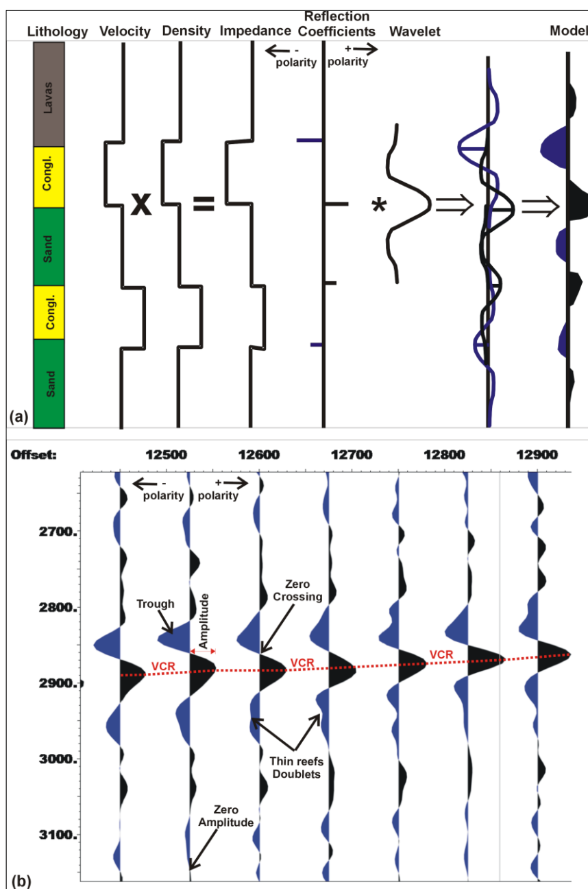
Fig. 2. (a) The model showing reflection coefficient (RC) series as defined from lithological boundaries. The convolved RC with the field wavelet produces a simulated raw field trace showing both a trough and peak of the wavelet. (b) Wiggle trace section extracted from South Deep data volume. The composite trace has a reflection with 90^\circ phase. Black is a positive polarity and blue is a negative polarity. The highest amplitude event corresponds to the top of the Ventersdorp Contact Reef (VCR) and the summed wavelets, or doublets correspond to the thin reefs.
