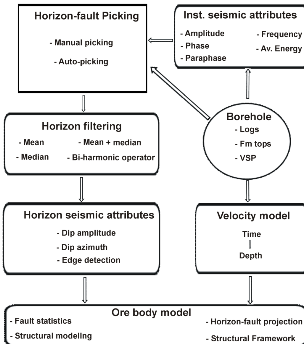
Figure 2.11: Integrated structural ore body modeling workflow. Inst.: Instantaneous. Steps listed above complement each other, yet they are applied at different stages during interpretation and modeling of the ore body.
