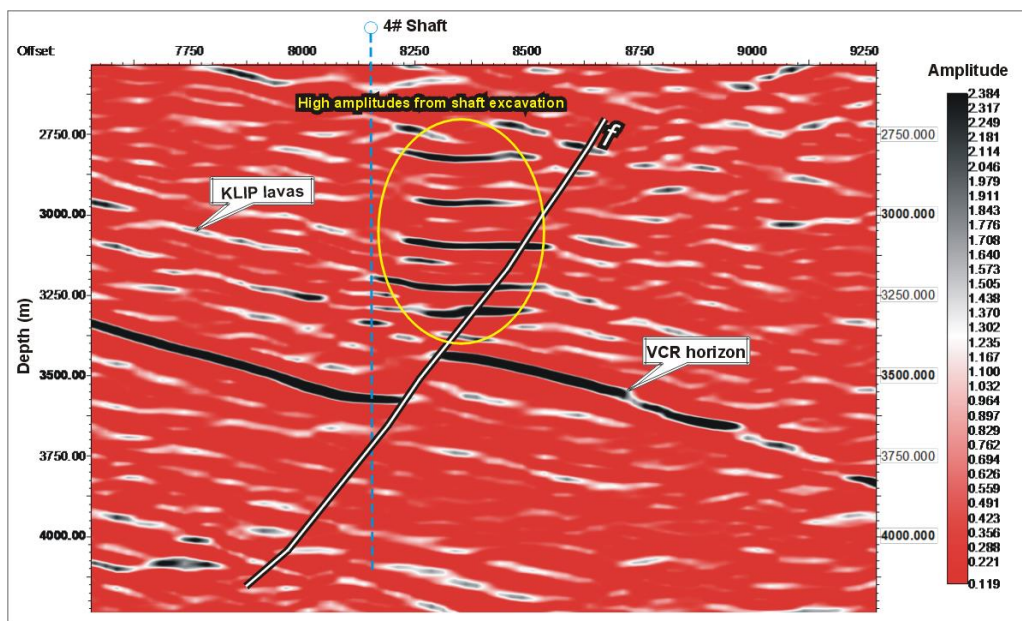
Fig. 6. Seismic section (amplitude display) showing the imaging of shaft locations, coinciding with high amplitude reflection events. Note that the #4 Shaft intercepts the fault at depth of about 3.5 km below surface.
