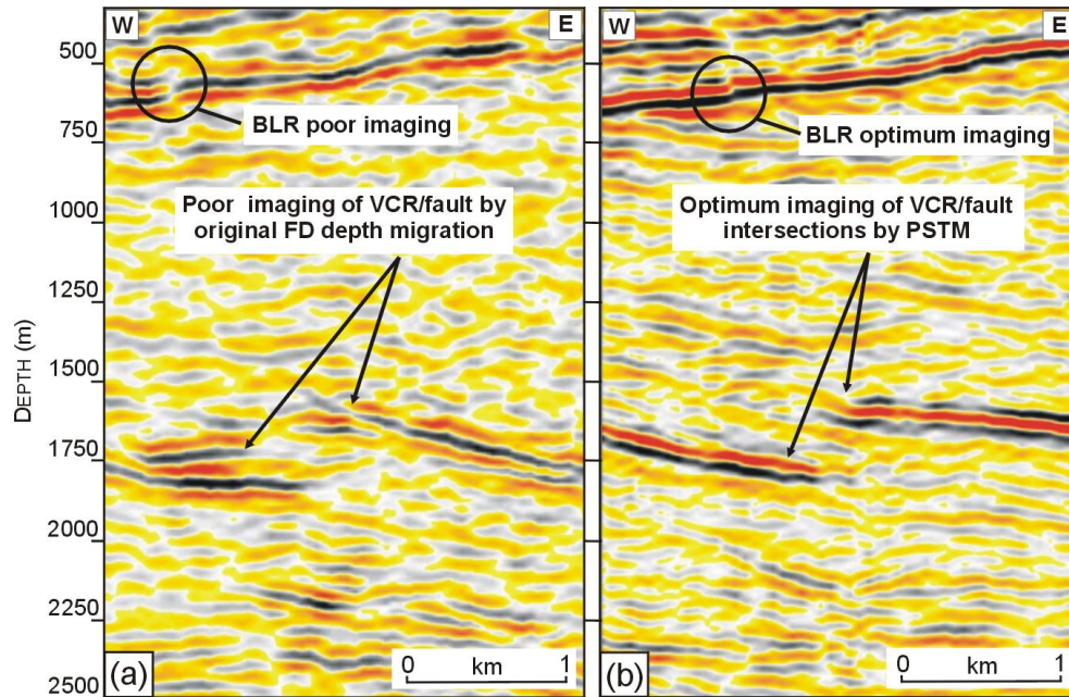
Figure 2.5: Depth-converted (amplitude display) seismic sections from 1994 Leeudoorn data. (a) The 3D poststack finite difference depth migrated (PostSDM) section. (b) The 3D prestack Kirchhoff time migrated (PreSTM) section. Note that PSTM shows better resolution relative to the poststack depth migration that was originally applied to the same data set, shown in (a).
