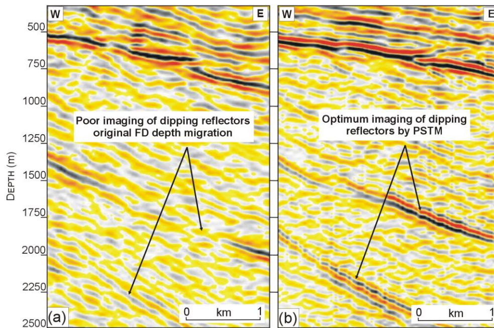
Figure 2.6: Depth-converted (amplitude display) seismic sections from 1994 Leeudoorn data. (a) The 3D poststack depth migrated (PostSDM) section. (b) The PreSTM section. The PreSTM provides better imaging of the dipping reflectors.
