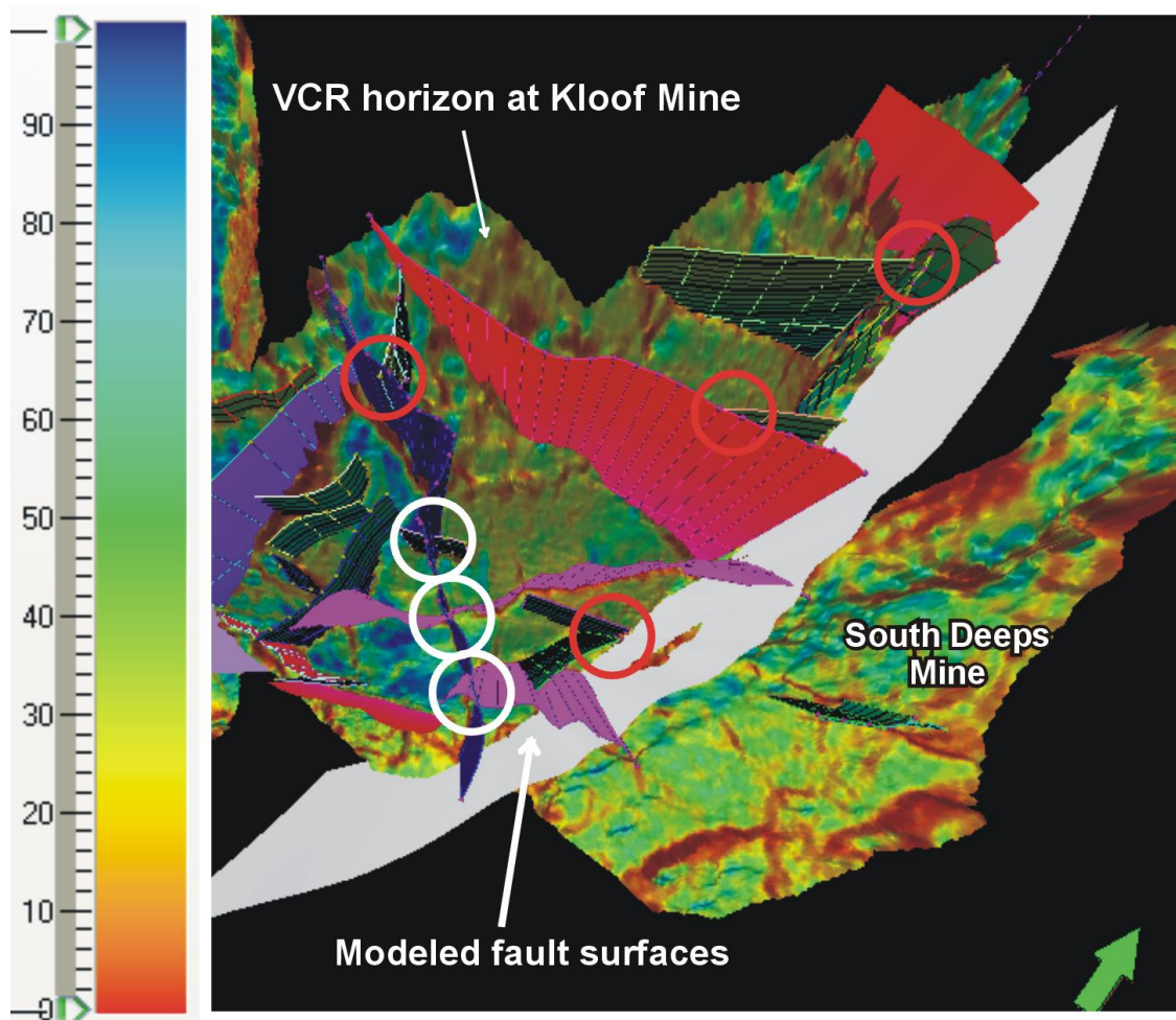
Fig. 11. VCR horizon-fault framework defined from edge detection seismic attribute. Model shows bifurcation of faults from a single plane into two branches (red circles) and cross-cutting relationship between faults (white circles).
