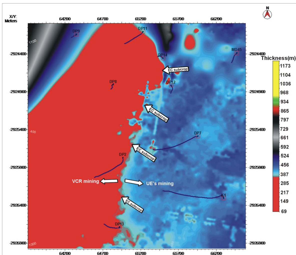
Fig. 13. VCR-Klip 1 Isopach map showing EC subcrop position. Notice how the isopach thins to the west of the mining area, coinciding with the interference zone where the Klip1 onlaps onto the VCR surface.
