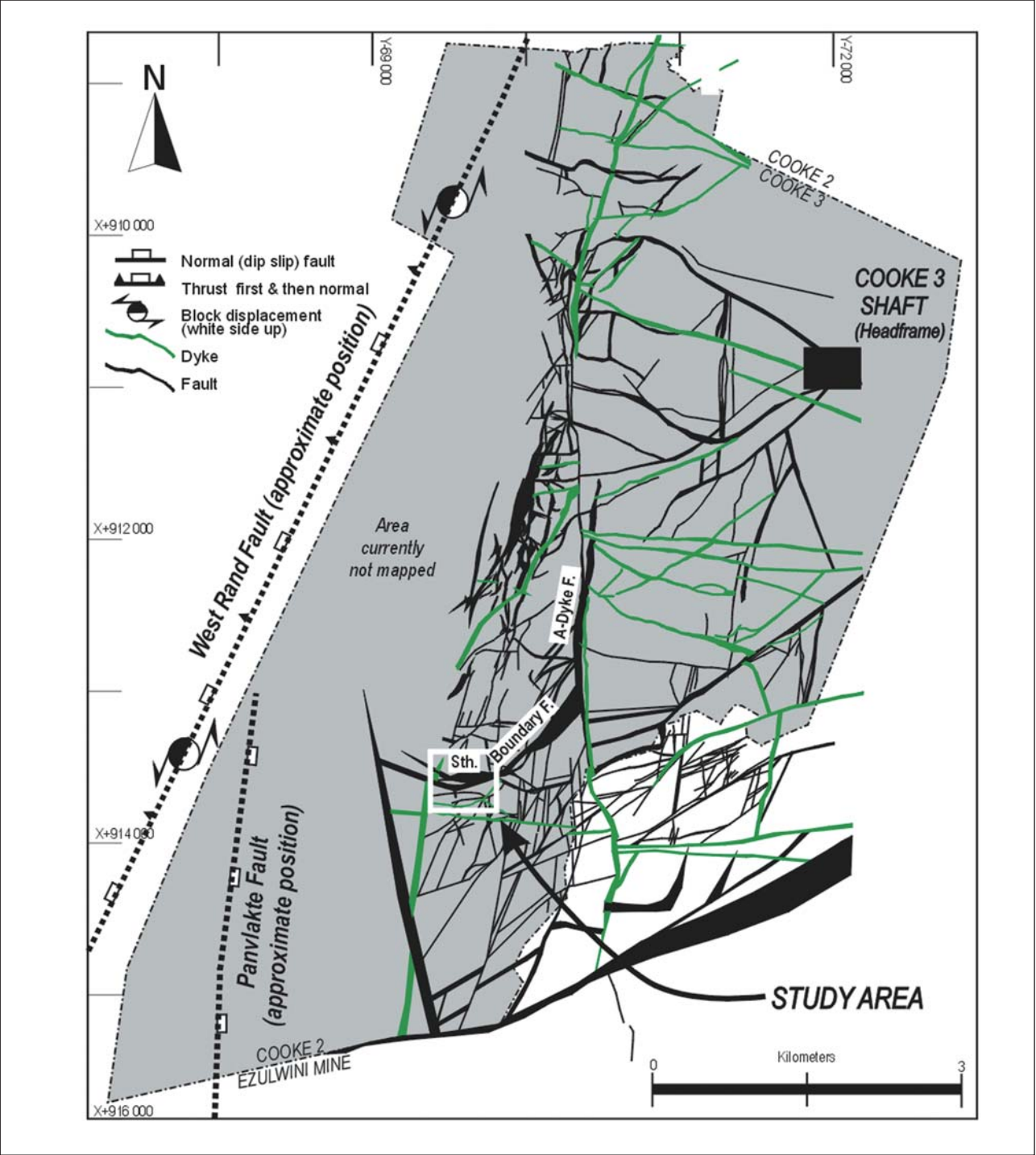
Figure 2. Schematic geological map of faults and mafic dykes in the Cooke Section at the level of the Kimberley Reefes. This complex array of faults and dykes is located in the footwall (eastern block) of the West Rand Fault Zone and forms a macroscopic breccia.
