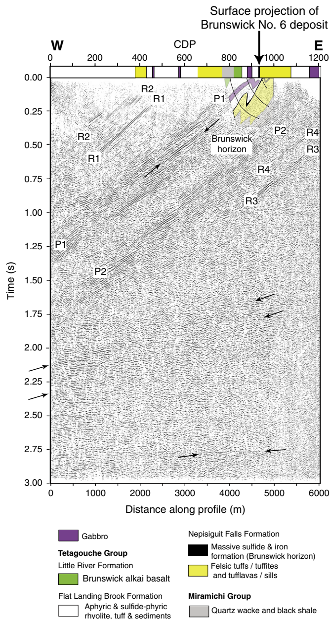
Fig. 17. Stacked section along the BRN991001 profile, showing a series of westward, steeply dipping reflections imaged down to about 1.7 s (i.e., about 5 km depth). Reflectivity pattern shows a sequence of reflective and transparent package repeating from the east to the west. The Brunswick horizon and associated structures appear within the reflective package P1. See text for interpretation of P1, P2, R1, R2, R3 and R4. See Cheraghi et al. (2011) for more details about the projected cross-section onto the profile.
