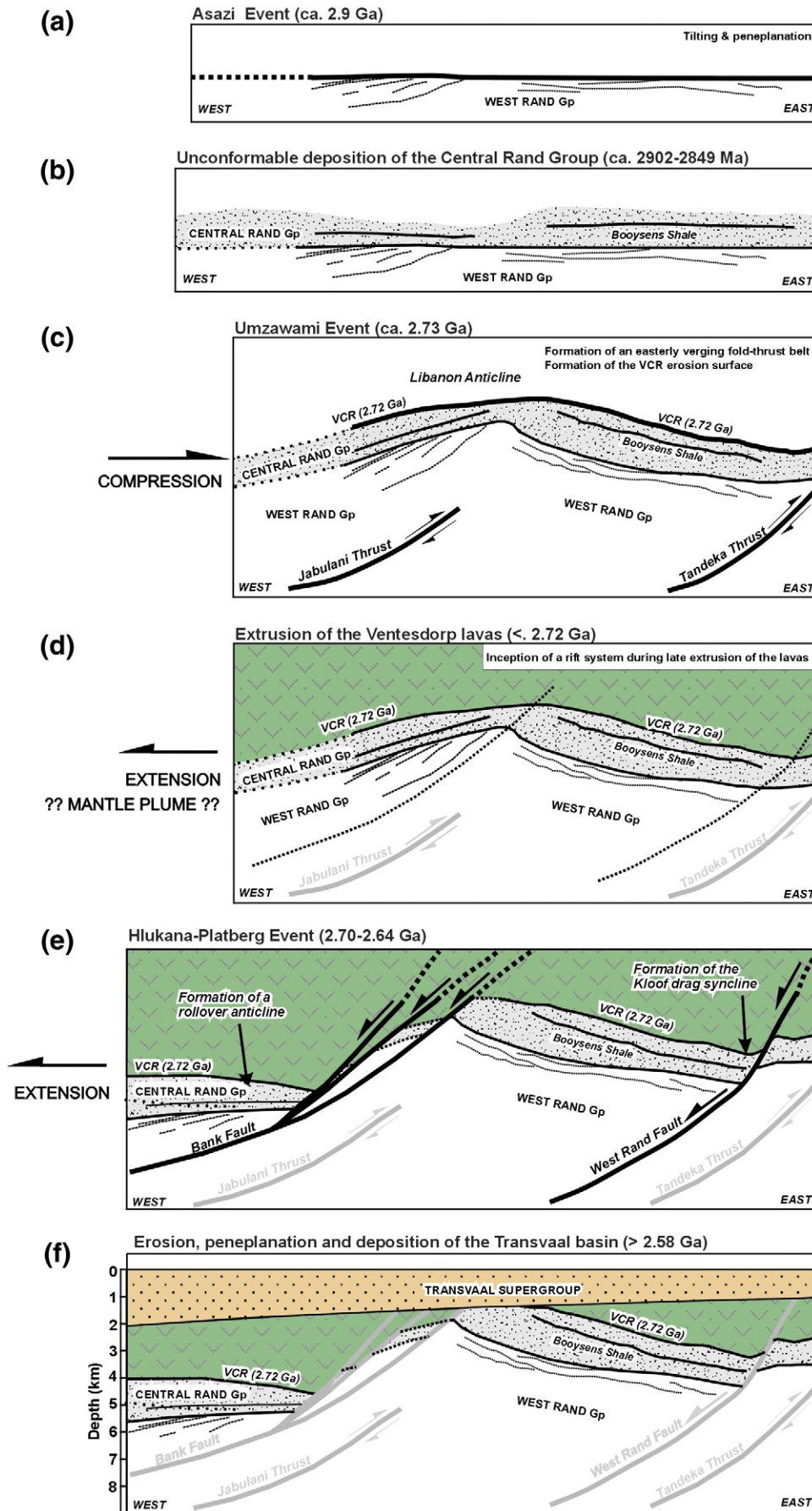
Fig. 6. Schematic model of the evolution of the Neoarchaean tectonic history of the Witwatersrand Basin and Ventersdorp Supergroup as interpreted from high-resolution 3D seismic reflection data; for explanation see text.
