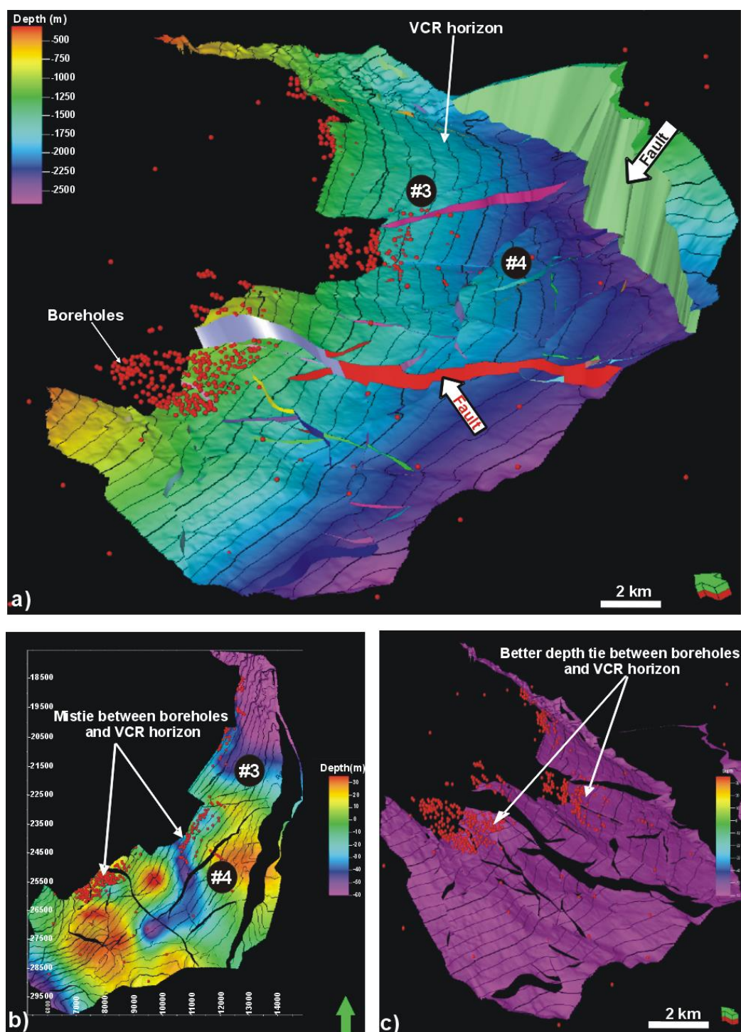
Fig. 9. The tieing of the VCR to the exploration boreholes. (a) VCR depth mistie with boreholes. Note how the borehole intersections to the north (around #3 Shaft) are generally below the VCR. Some holes in the northwest of #3 Shaft are located in the faulted zones, thus causing major misties (b) De-spiked error grid. Note the misties between the boreholes and the seismically defined VCR surface. (c) Depth corrected model. Note how the borehole VCR intersections (red spheres) coincide with the VCR surface.
