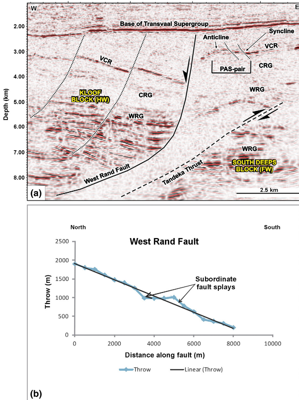
Fig. 3. (a) Seismic section (line BB' in Fig. 1) across the listric West Rand Fault, showing the steeply dipping hanging wall (Kloof block), Tandeka Thrust and PAS-pair in the footwall block (South Deeps). (b) Displacement (throw) measured in seismic sections perpendicular to the West Rand Fault strike at 250 m interval. FW: Footwall; HW: Hanging wall; VCR: Ventersdorp Contact Reef; WRG: West Rand Group; CRG: Central Rand Group; PAS: Panvlakte Anticline Syncline.
