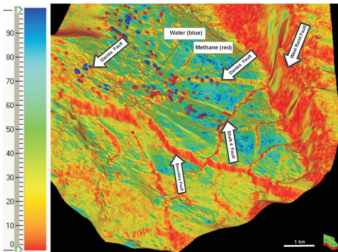
Figure 2.9: VCR edge attribute map of the VCR overlain with water and methane data in Kloof gold mine. Structures such as Danies Fault and Shaft 4 Fault show good correlation with water and methane data (color bar is given in %).
