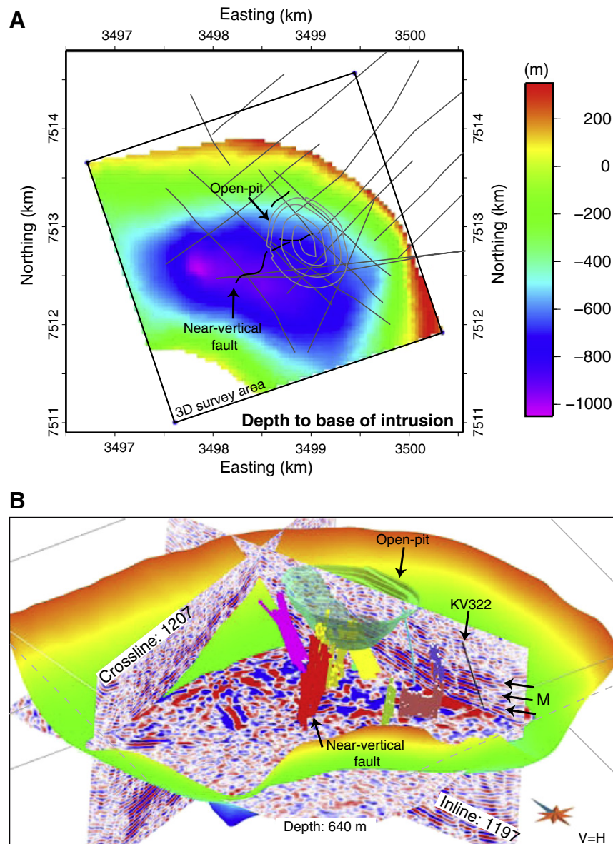
Fig. 8. (A) Depth to the base of the Kevitsa intrusion constrained by the 3D seismic and available borehole data in the study area. Solid black lines represent near-vertical faults mapped from the seismic volume. (B) 3D visualization of the seismic data with the planned open-pit mine and the picked near-vertical faults and the base of the Kevitsa intrusion. KV322 is a borehole that intersects a series of sulfide mineralization and shows a good correlation with the reflections observed in the seismic volume (see events marked as M). Modified from Malehmir et al. (2012a).
