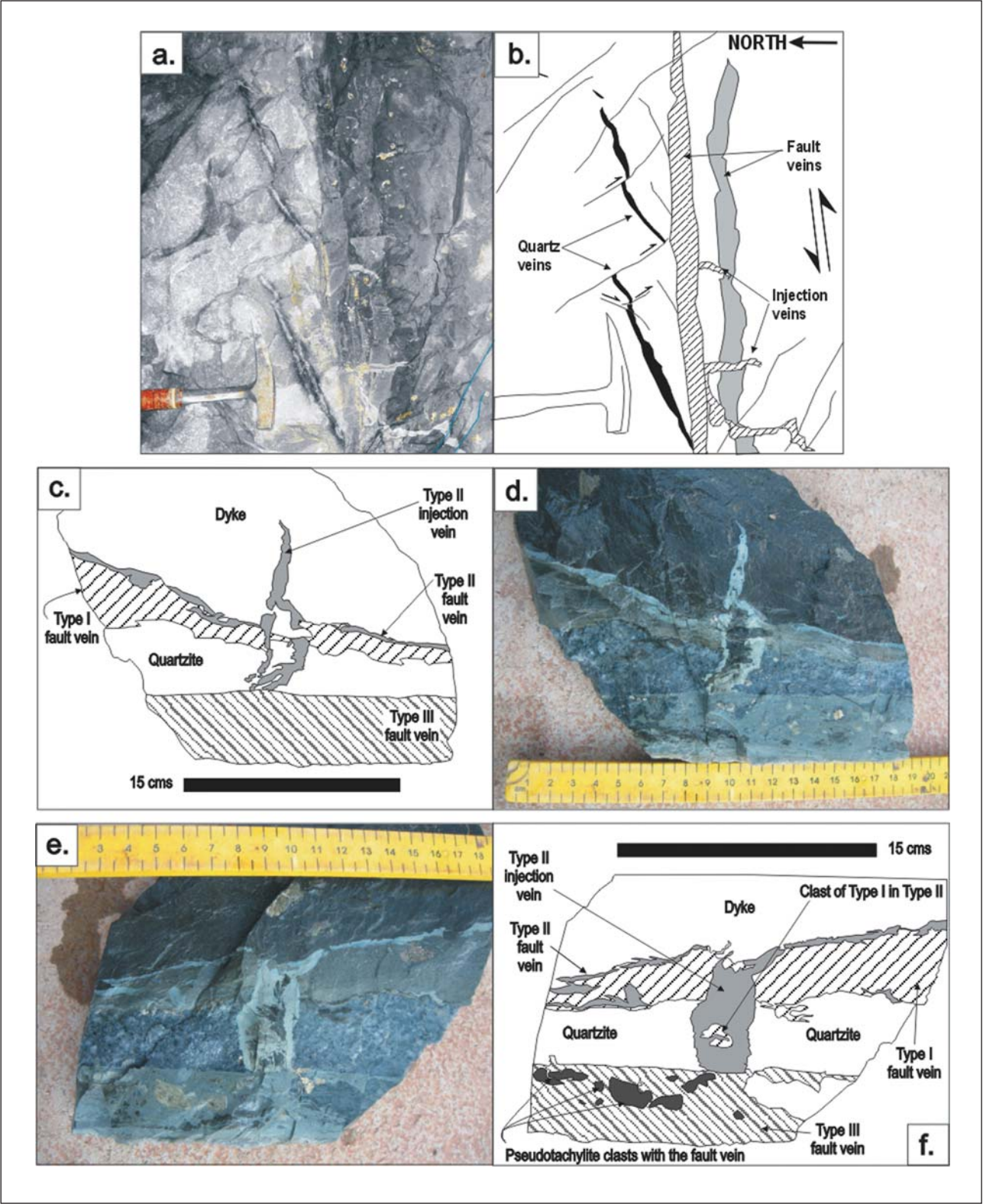
Figure 6. (a, b) Photograph and sketch of eastern face of the 128 Level West 15 baulage. Psuedotachylite as fault and injection veins, crosscuts en echelon quartz veins but also pre-existing fault veins. Pseudotachylite-bearing faults are steep to moderate south-dipping with a calculated mean strike and dip of 092°/50°S. The overall displacement on the faults is reverse with south block up. (c, d) At least three generations of veins associated with pseudotachylite-bearing faults (Type-I, Type-II and Type-III) are exposed on the eastern wall of the 128 Level West 15 baulage. Type-II veins occur as fault veins and injection veins with a distinct pale-blue to light-green groundmass. Type-III veins crosscut Type II veins which crosscut Type 1 veins. (d, e) (back and front of the same sample): Type II fault veins frequently host clasts and slivers of younger pseudotachylite veins and indicate that several events of pseudotachylite formation have taken place. The dark mass that lies central to Type II injection veins is predominately glass.
