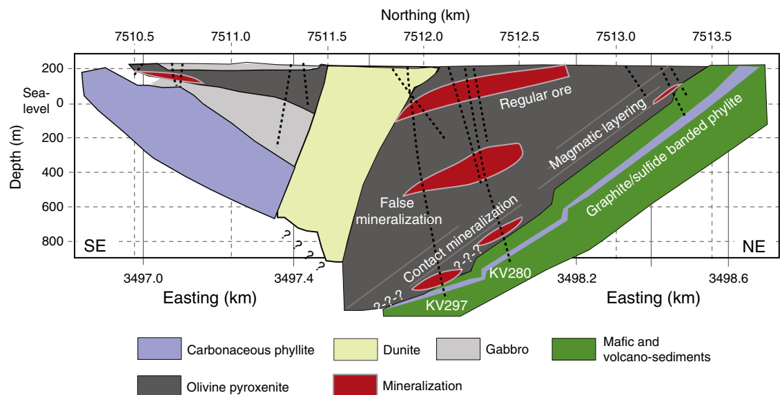
Fig. 6. Schematic cross-section constrained by deep magnetotelluric and borehole data, showing the main Kevitsa intrusion (hosting the main mineralization-regular ore) and proven massive sulfide mineralization occurring as false and contact mineralization in the study area. Modified from Malehmir et al. (2012a).
