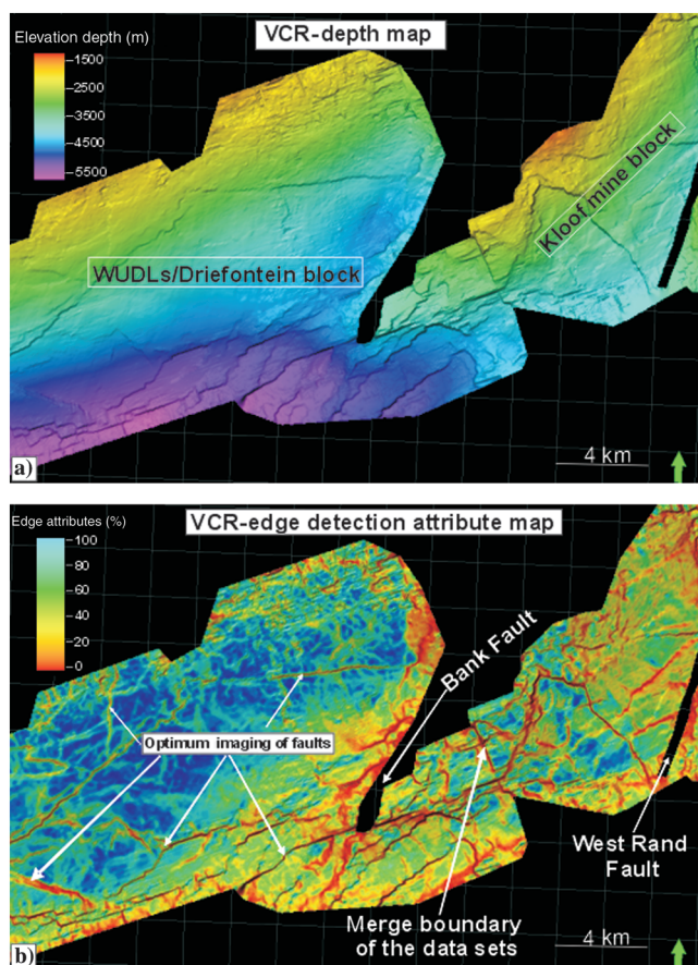
Figure 12. VCR maps showing imaging of faults before and after the computation of edge detection attributes. (a) VCR depth map (gridded) showing imaging of faults through conventional interpretation. (b) VCR edge attribute map showing high-resolution imaging of the faults, mostly with throws as small as 10 m.
