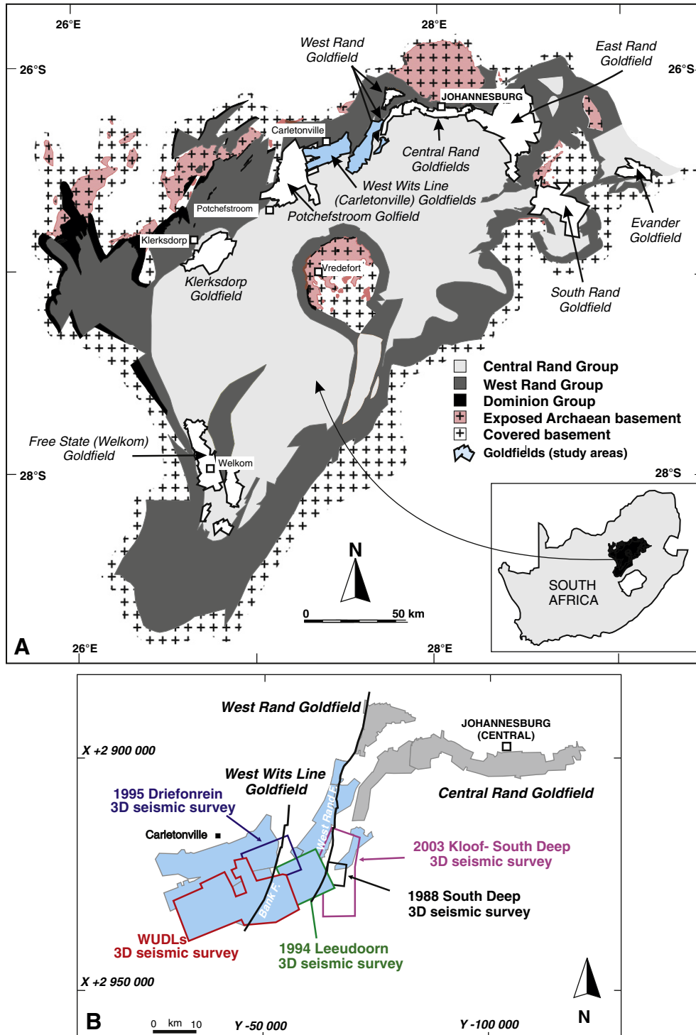
Fig. 9. (A) The location map of the West Rand and West Wits Line (Carletonville) Goldfields of the Witwatersrand Basin in South Africa (after Dankert and Hein, 2012). (B) The location of historical surveys for Kloof, South Deep, Driefontein and Western Ultra Deep Levels (WUDLs) (after Manzi et al., 2012a,b).
