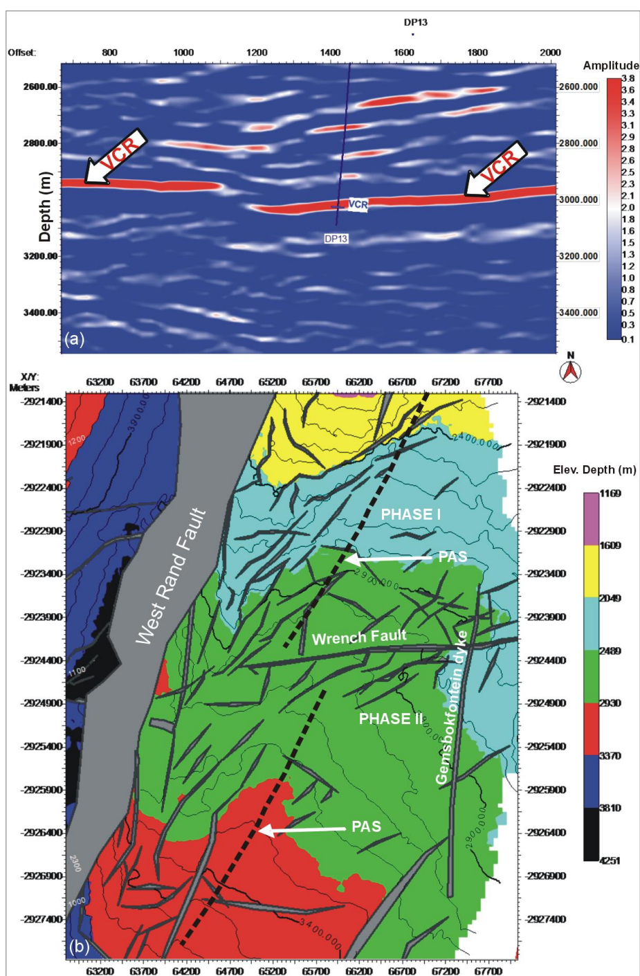
Fig. 7. (a) Amplitude display of the seismic section showing strong and consistent VCR horizon, constrained by borehole (DP13). (b) Depth structure contour map of the VCR horizon showing fault polygons and prominent West Rand and Wrench faults. PF: Panvlakte Fault; WPF: Waterpan Fault.
