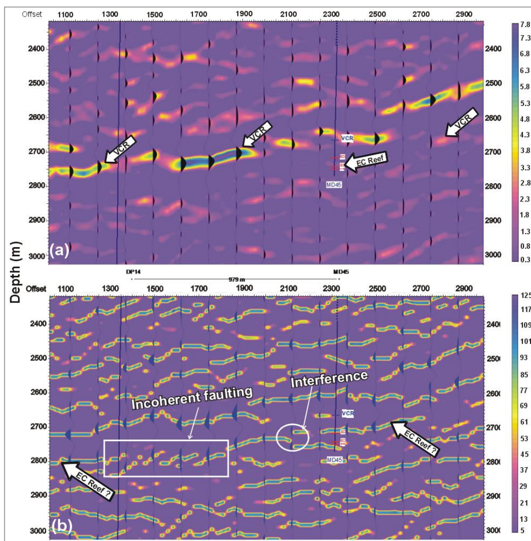
Fig. 12. Seismic section (L5 in Figure 1) with major faulting and low signal-to-noise ratio (a) Amplitude display (b) Paraphase display. Notice how well the EC reef is enhanced by paraphase attribute. VCR: Ventersdorp Contact Reef; EC: Elsburg Conglomerate.
