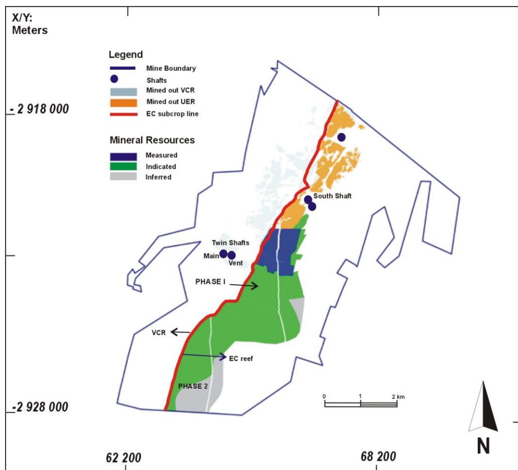
Fig. 5. South Deep underground resource model showing the Elsburg Conglomerate (EC) subcrop positioning, mined-out and development areas.
