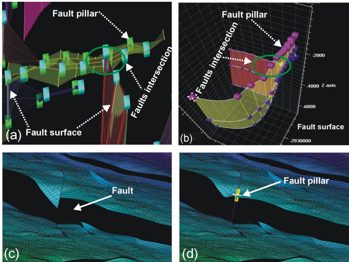
Figure 2.10: (a) Modelled fault surfaces and fault pillars (changed dip of faults from vertical) using NURBS. (b) Modelled fault surfaces, showing fault intersections. (c) Horizon modeling around the fault zones. (d) Projection of fault pillars into horizon breaks (faults).
