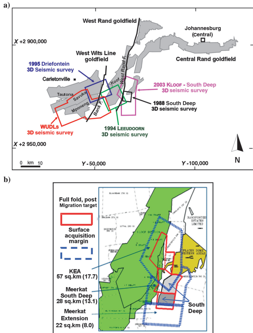
Figure 3. (a) The location of historical surveys for Kloof, South Deep, Driefontein, and WUDLs (after Manzi et al., 2012). (b) KEA and Meerkat (South Deep) seismic survey acquisition margin and targeted areas.
