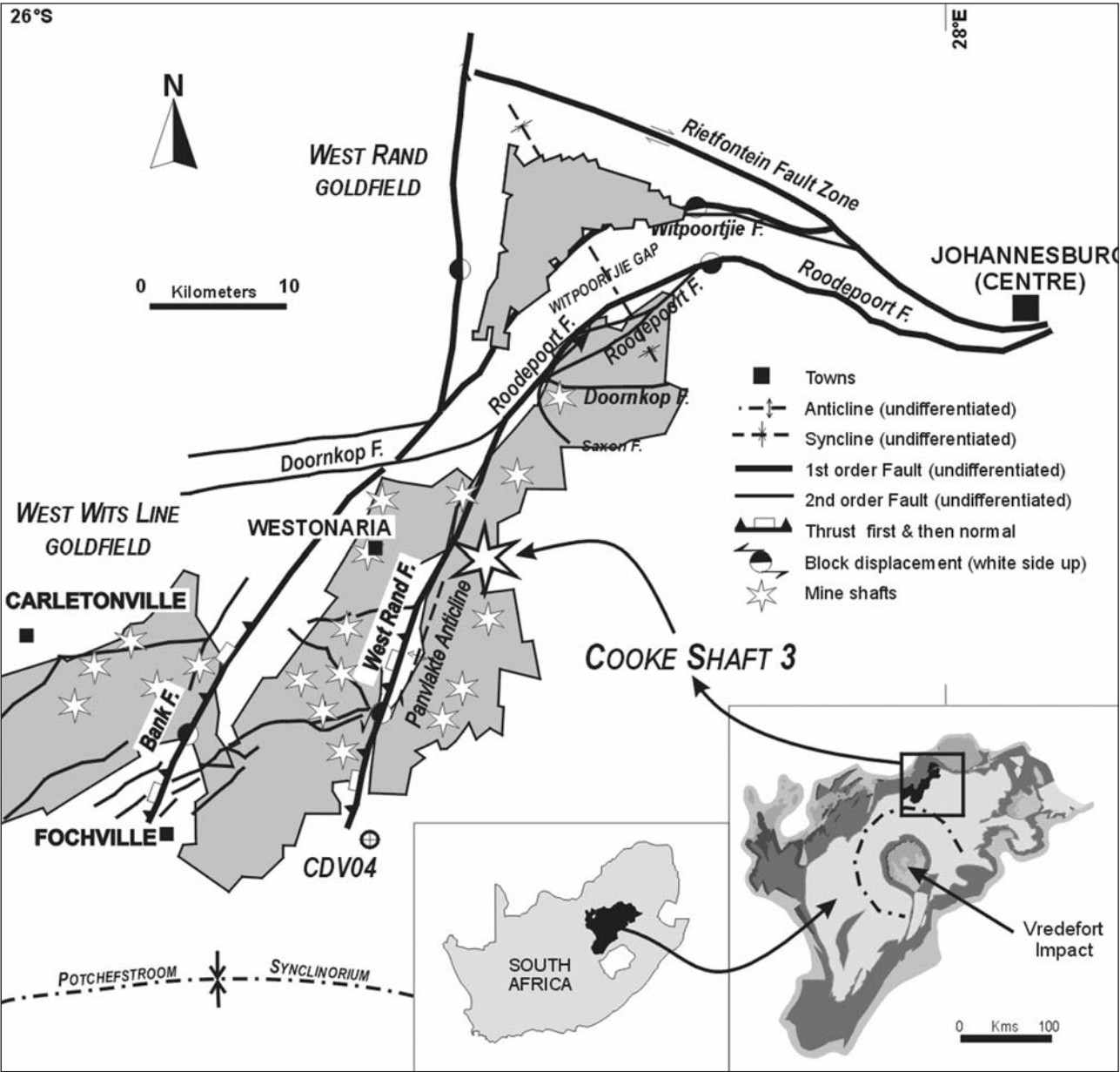
Figure 1. Schematic geological map of the West Rand goldfield and position of Cooke Shaft 3, with Transvaal Basin sequences and Karoo Supergroup cover removed (modified after Dankert and Hein, 2010). Borehole CVD4, which was collared approximately 25 km south-southwest of Cooke Shaft 3 on the northern limb of the Potchefstroom Synclinorium, is also shown. Its approximate position is after Brink et al. (2000).
