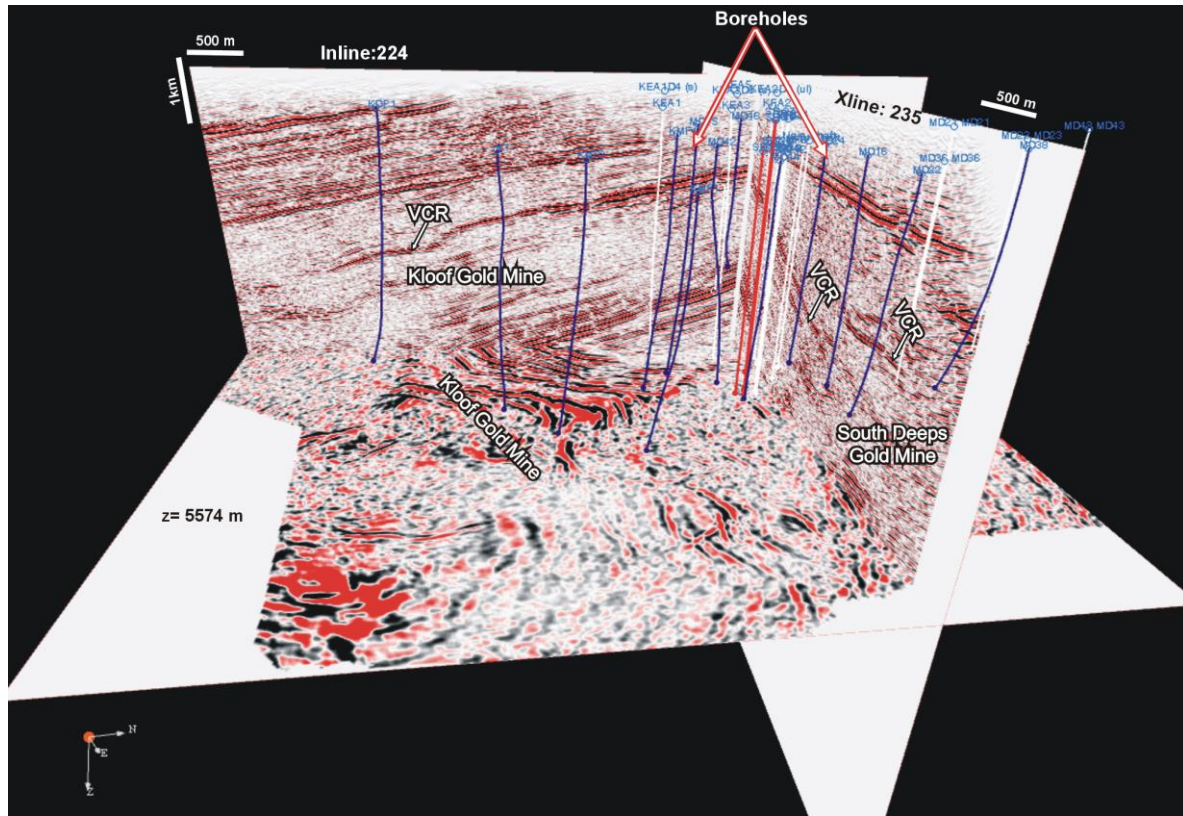
Fig. 4. 3D depth-converted prestack time migrated seismic cube (amplitude display) covering Kloof and South Deeps Gold mines, showing location of exploration boreholes.
