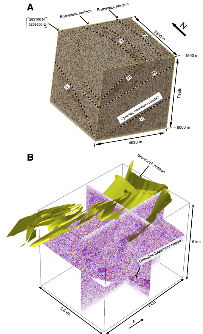
Fig. 18. 3D views from the seismic volume. (A) Unmigrated stack volume showing the depth extent of the Brunswick horizon (P1 and P2) and a high amplitude reflection (I1) interpreted to mark the base of the Brunswick volcano–sedimentary belt. (B) Migrated stacked volume and correlation of a strong high amplitude reflection with the geological model of the Brunswick horizon. A portion of the seismic cube for a time slice at 500 ms. See Fig. 14 for the surface projection of the cube and text for interpretation of events marked as P1, P2, and I1. Figure is modified from Cheraghi et al. (2012).
