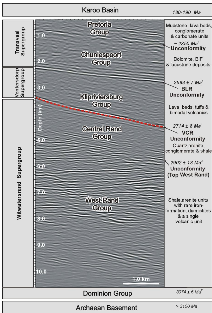
Fig. 2. Generalized seismic stratigraphy, with dates and ages are derived from Krapež [32], Myers et al. [61], Armstrong et al. [62], Kositsin and Krapež [63] and Dankert and Hein [23]. VCR: Ventersdorp Contact Reef; BLR: Black Reef Formation. a Unpublished; b Martin et al. (1998; zircon U-Pb SHRIMP) [64]; c Armstrong et al. (1991; single zircon U-Pb SHRIMP); d Kositsin and Krapež (2004; zircon U-Pb SHRIMP).
