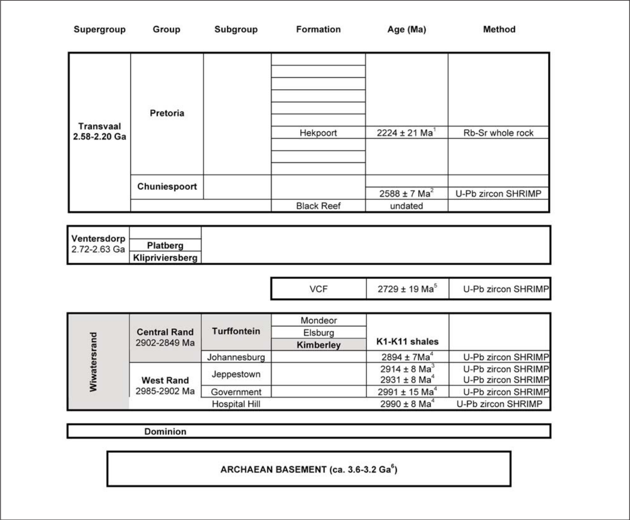
Figure 3. Abridged lithostratigraphy (groups, subgroups and formations) of the Dominion Group, Witwatersrand, Ventersdorp supergroups and the Transvaal Basin sequences constrained to absolute geochronology. KEY: (1) Burger and Coertze (1973 to 1974; Rb-Sr whole rocks age); (2) Martin et al. (1998; single zircon U-Pb SHRIMP); (3) Armstrong et al. (1991; single zircon U-Pb SHRIMP); (4) Youngest concordant detrital zircon grain (Kositcin and Krapež, 2004); (5) Igneous-detrital xenotime/zircon aggregate Kositcin et al. (2003); (6) From Poujol et al. (2003). VCF = Ventersdorp Contact Formation
