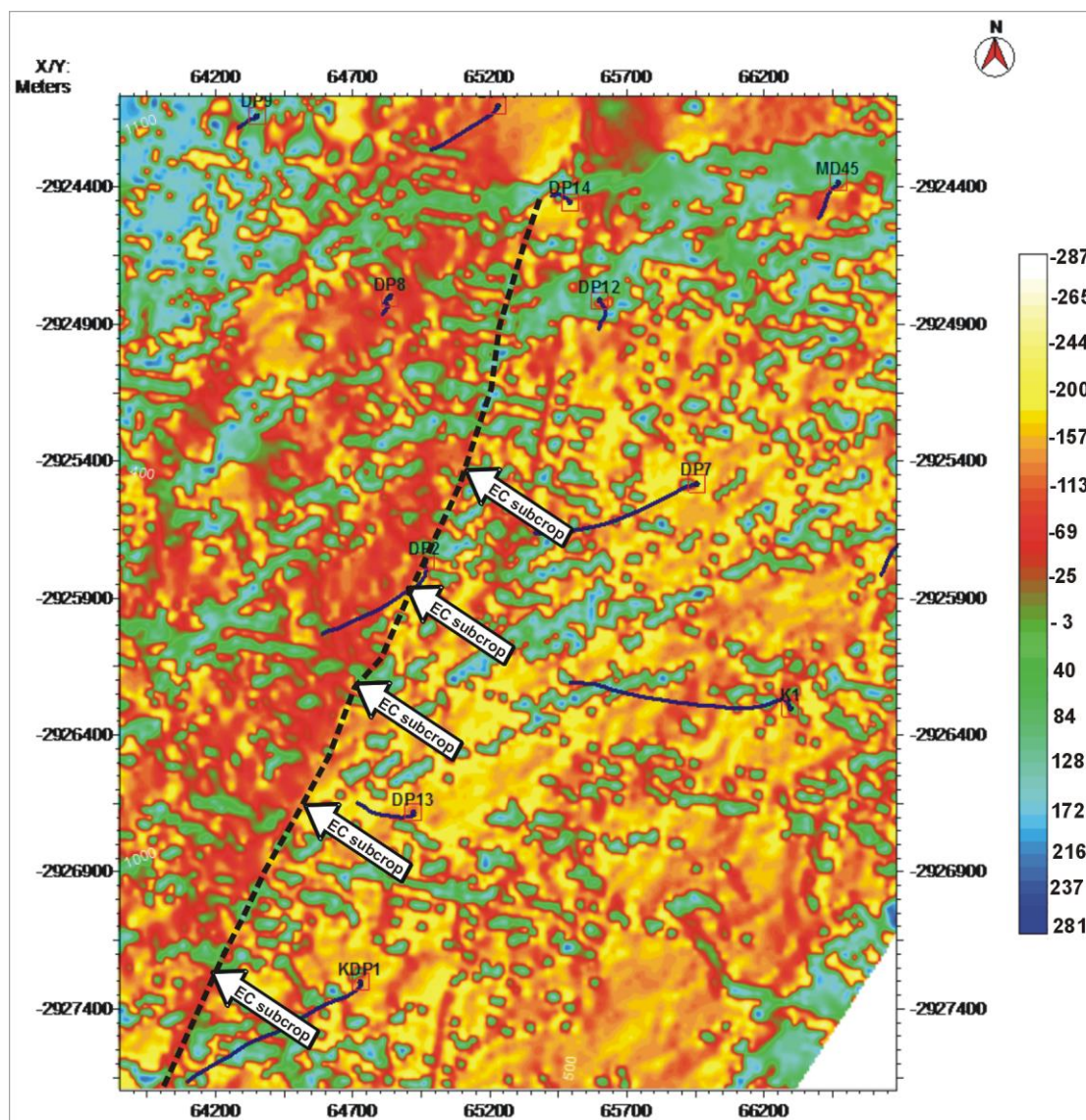
Fig. 14. The zero-crossing attribute map between Klip 1 and VCR confirming the Elsburg Conglomerates subcrop position and its orientation as predicted by isopach map in Fig. 13 and the mine model in Fig. 5.
