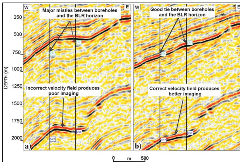
Figure 2.4: Depth converted time migrated sections using finite difference migration algorithm. (a) Unsmoothed velocity field produces stretched seismic horizons and distorted structures (possibly under-migrations), and shows a large depth mis-tie between the VCR and BLR horizons and borehole control. (b) Smoothed velocity field provides stable seismic horizons and structures, and a very good depth tie between the VCR and BLR horizons and boreholes.
