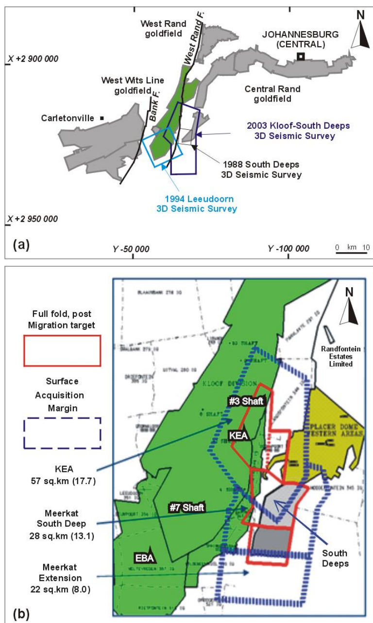
Fig. 3. (a) The location map showing the historical surveys overlain by the 2003 3D Kloof-South Deep seismic survey (after Gibson et al., 2000; Manzi et al., 2012a). (b) Kloof Development area and South Deeps seismic survey acquisition margin and targeted areas (after Manzi et al., 2012b). KEA: Kloof Extension areas, EBA: Eastern Boundary Area.
