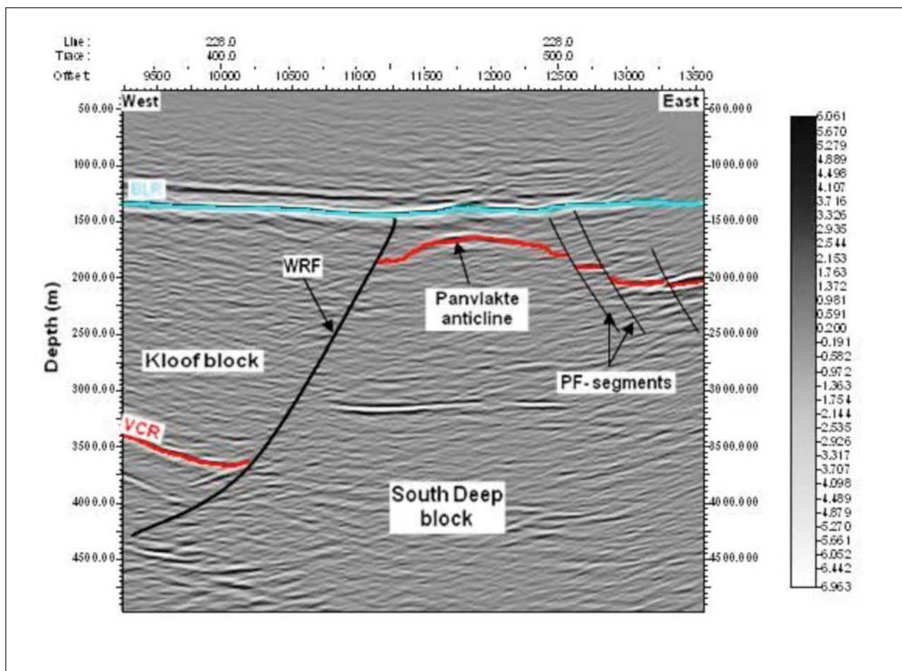
Figure 4. An east-west seismic section (amplitude display) across the Panvlakte Anticline south of the Cooke Shaft permit. The section shows that the major West Rand Fault and minor fault segments do not breach the base (unconformity) of the Transvaal Basin which is dated at 2.58–2.20 Ga (Kositcin and Krapež, 2004; U-Pb detrital zircon), i.e., Black Reef Formation. Displacement on the faults thus predates 2.58 Ga. Keys to Abbreviations, VCR: Ventersdorp Contact Reef; BLR: Black Reef Formation; PF: Panvlakte Fault.
