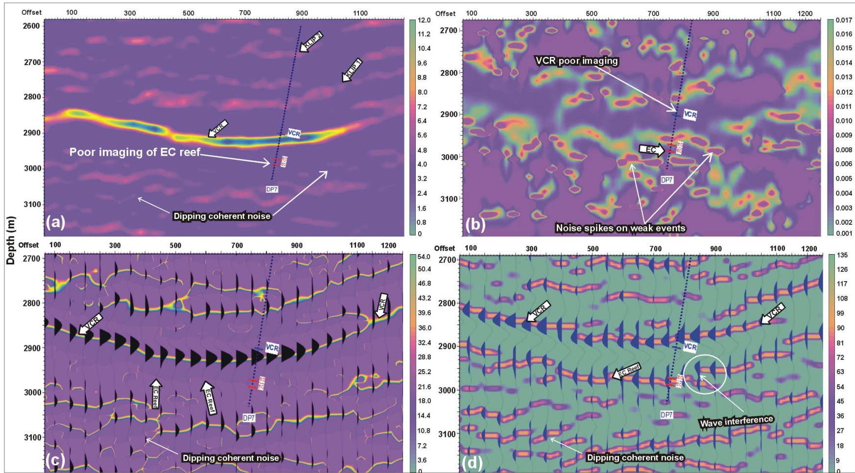
Fig. 11. Seismic section (L3 in Figure 1) (a) Amplitude display showing strong and continuous VCR horizon. (b) Instantaneous frequency contaminated by noise and showing poor detection of weak events (c) Instantaneous phase (wiggle trace) highlighting weak events as thin and continuous reflections. (d) Paraphase display making weaker events much stronger and continuous. Notice how well the EC reef ties with the borehole control (DP7). VCR: Ventersdorp Contact Reef; EC: Elsburg Conglomerate.
