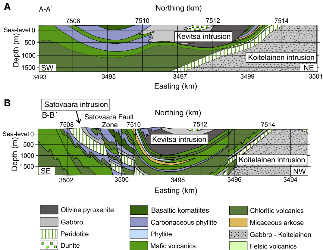
Fig. 5. (A) Simplified geologic cross-sections along southwest–northeast and (B) southeast–northwest directions showing expected geometry of the Kevitsa intrusion and fault systems (courtesy of First Quantum Minerals Ltd.). Modified from Koivisto et al. (2012).
