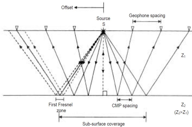
Figure 2.1: Schematic reflection raypaths over a horizontal interface across which there is a contrast in impedance, Z ( Z_2 > Z_1 or Z_2 < Z_1 ) (after Trickett et al., 2004).
