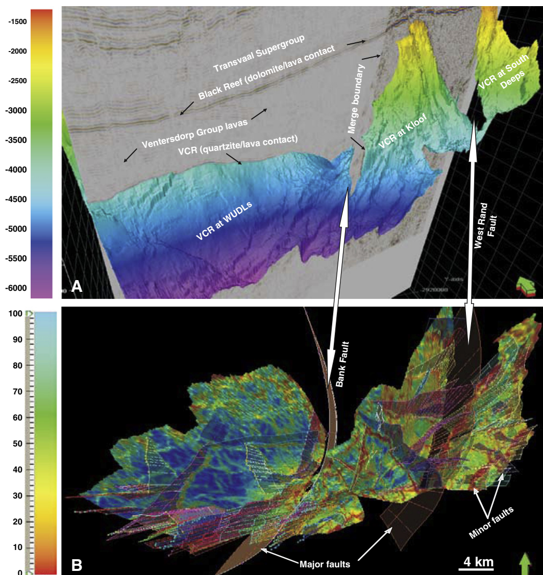
Fig. 13. (A) 3D visualization of the VCR, clearly showing the imaging of the mega-scale and meso-scale structures (color bar represents an elevation depth and is given in meters). (B) The fault framework model projected onto the VCR horizon defined from edge detection attribute (color bar represents edges and is given in % where low values indicate edges such as faults and dykes). The model incorporates the major West Rand Fault and Bank Fault, as well as a suite of minor structures. (For interpretation of the references to color in this figure legend, the reader is referred to the web version of this article.)
