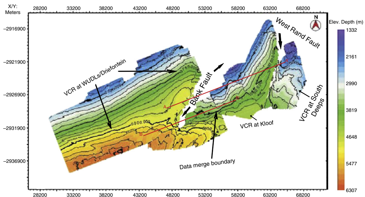
Fig. 10. Depth structure map of the Ventersdorp Contact Reef (VCR) derived from conventional picking across survey areas, showing the Bank and West Rand faults and the location of seismic sections shown in Fig. 11. The contour interval is 250 m.
