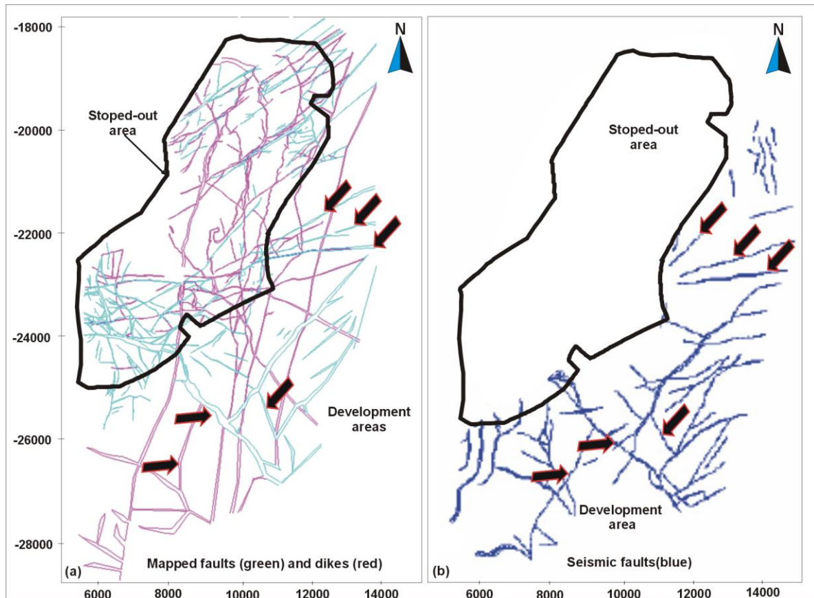
Fig. 8. The comparisons between seismic and mine underground mapped faults and dikes. (a) Faults mapped underground (green) and dikes mapped underground (red). (b) The seismically defined faults from development area. Note the structures that are present in both models as shown by arrows.
