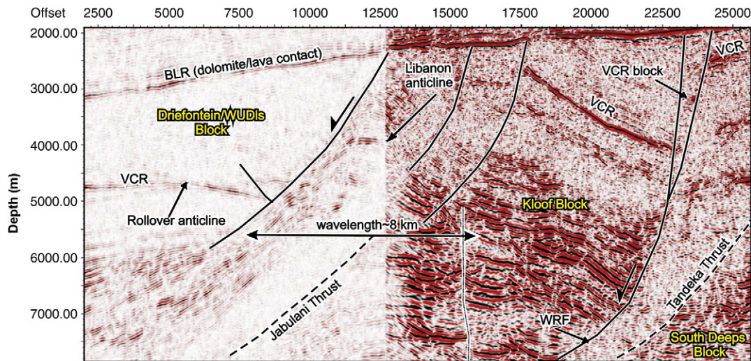
Fig. 5. Seismic section (line DD' in Fig. 1) showing the geometry of the Libanon Anticline at the merge boundary between the footwall (Kloof) and hanging wall (Driefontein/WUDLs) blocks. The Jabulani Thrust and its subordinate faults in the footwall of the Bank Fault crosscut the Libanon Anticline. The hanging wall block hosts minor rollover anticline and a subordinate fault. FW: Footwall; HW: Hanging wall; VCR: Ventersdorp Contact Reef; WRF: West Rand Group; CRG: Central Rand Group; BLR: Black Reef Formation.
