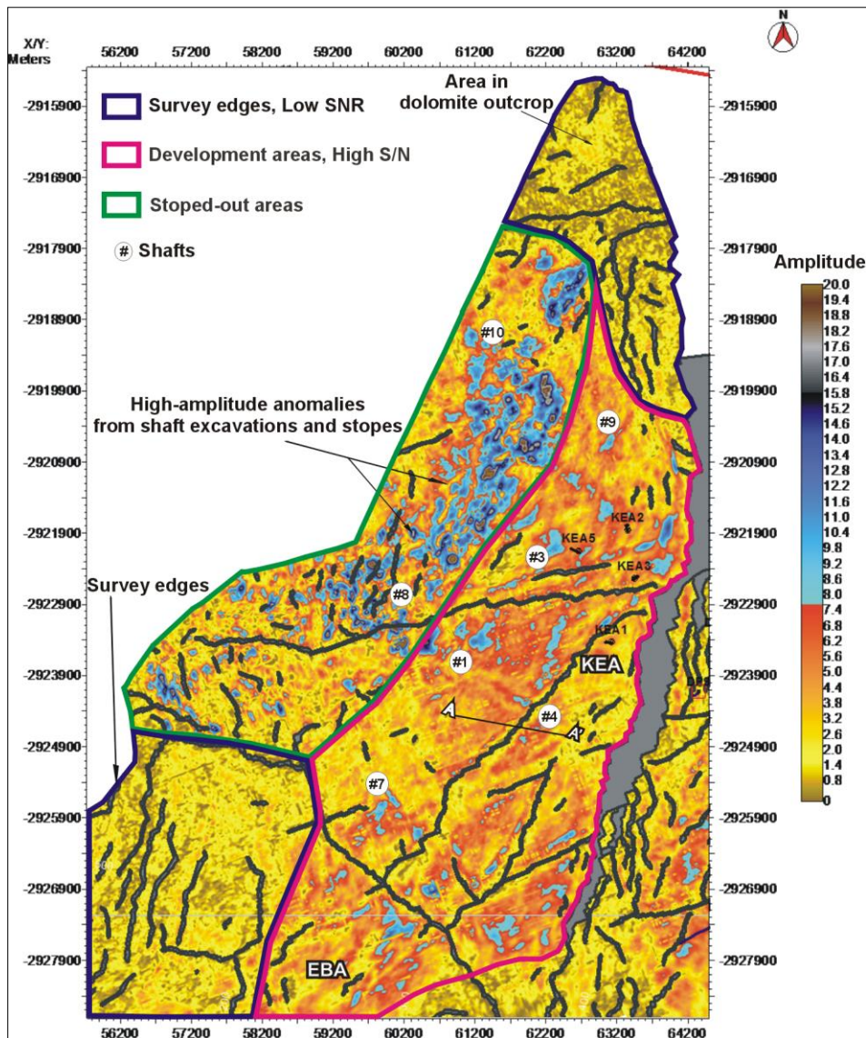
Fig. 5. Amplitude attribute computed for the VCR horizon across the Kloof survey area. The map shows the location of shaft excavations, stopped-out and development areas, and the imaging faults.
