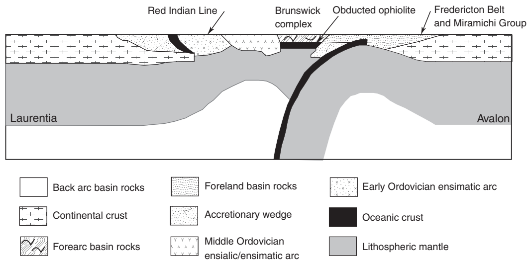
Fig. 15. Tectonic model of the Brunswick complex in the late Ordovician–early Silurian (450–440 Ma; modified from van Staal, 1994). The Brunswick horizon (massive sulfide and iron formation) is part of the Brunswick complex and is strongly folded and deformed. Note that large blocks of thrust/obducted ophiolite rocks are expected to be trapped in the upper crust beneath the BMC.
