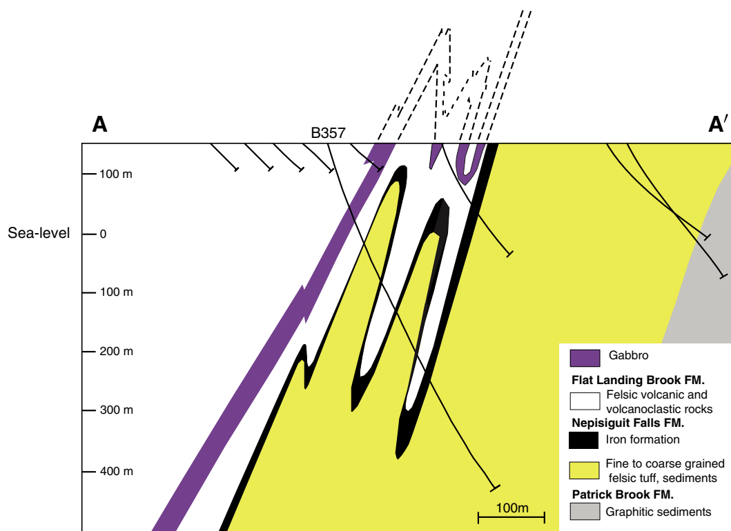
Fig. 16. Geological cross-section along the profile A–A' shown in Fig. 14 obtained from a series of shallow and deep boreholes, including borehole B-357. The cross-section shows complex structures near Brunswick No. 6 and associated Brunswick Horizon (modified from Wills et al., 2006). Petrophysical measurements obtained from wireline logging in borehole B-357 are shown in Cheraghi et al. (2011).
