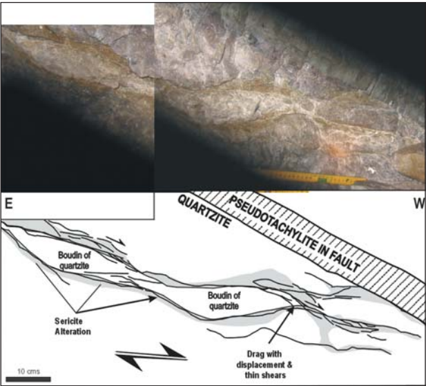
Figure 5. The macroscopic sub-horizontal boudins in the 128 Level West 15 haulage. View is along the haulage to the south. Sericite alteration of the wall-rock quartzite around the boudins is marked by a distinct yellowish-brown colouration in thin shears. The overall sense of displacement is interpreted as normal with top block to the west. The boudins are crosscut by a pseudotachylite-bearing fault indicating they formed before the fault.
