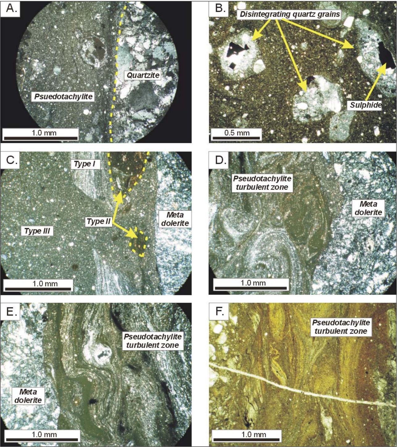
Figure 7. (a) Photomicrograph of the contact between quartzite (wall rock) and pseudotachylite (sample P/T 4). The contact is sharp and darker in colour, which Barker (2005) described as chilled margin. The quartzite exhibits sub grain development and fragmentation. (b) Photomicrograph of disintegrating quartzite (wall rock) grains in a pseudotachylite Type III matrix (sample P/T 5). The grains have a rind of fine quartz rock flour (corona texture). Sulphides occur in the core of some grains. (c) Photomicrograph of three crosscutting pseudotachylite types adjacent to the contact of metadolerite (sample PT 10). The contact is sharp between dolerite and Type III pseudotachylite and between pseudotachylite Types I, II and III. (d, e, f) Photomicrograph of turbulence of Types I and II pseudotachylite adjacent to meta-dolerite, with micro-folding clearly evident (sample PT 10 and PT 35).
