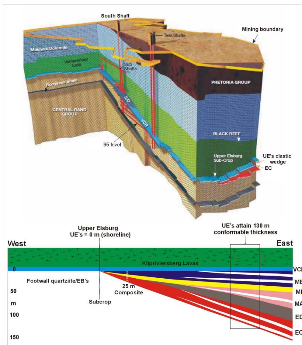
Fig. 4. Three (top) and two (bottom) dimensional schematic illustration of an easterly divergent Upper Elsburg clastic wedge (UER) with low acoustic-impedance package of multi-stacked gold-bearing reefs. The maximum thickness of the wedge is approximately 120 – 130 metres in the eastern boundary of the mine (After Erismann, 2007; South Deep Gold Mine, 2007).
