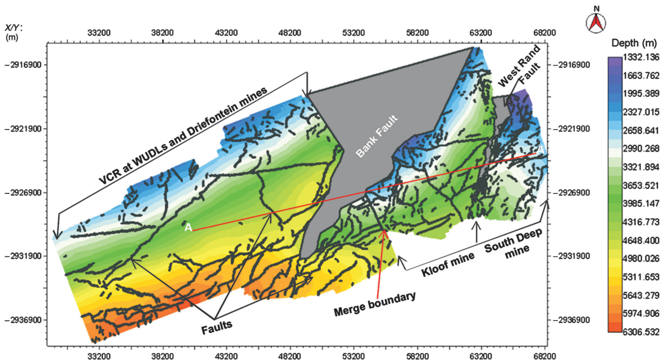
Figure 6. Detailed depth structure map of the Ventersdorp Contact Reef (VCR) derived from conventional picking across survey areas, showing faults of all strikes and dips.
