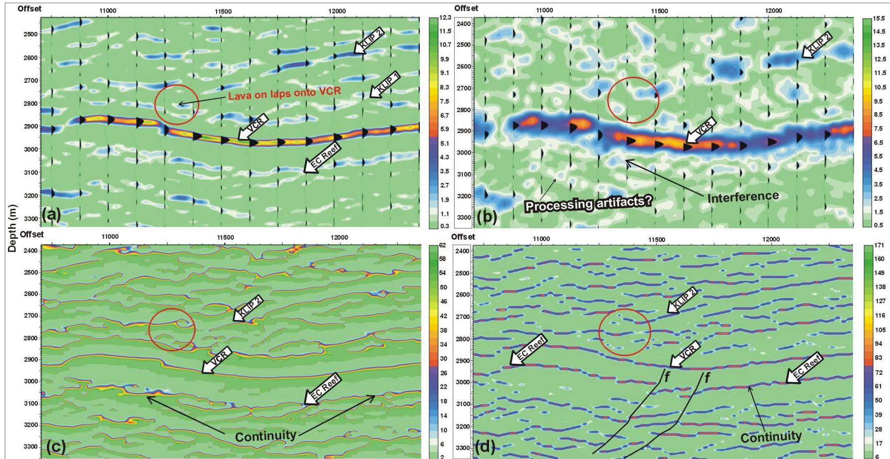
Fig. 10. Seismic section (L2 in Figure 1) (a) Reflection strength display (wiggle trace) highlighting the KLIP 1 horizon event onlapping onto the VCR and VCR continuity. (b) Instantaneous frequency display (wiggle trace) showing noisy spikes associated with thin seismic events and poor imaging of the VCR when compared to Figure 10 (a). (c) Instantaneous phase display continuous events associated with VCR and EC reef. (d) Paraphase display providing much better imaging of the EC reef. Observe the imaging of faults in Figure 10 (d) that was not prominent in other attribute displays. VCR: Ventersdorp Contact Reef; EC: Elsburg Conglomerate; KLIP: Klipriviersberg.
