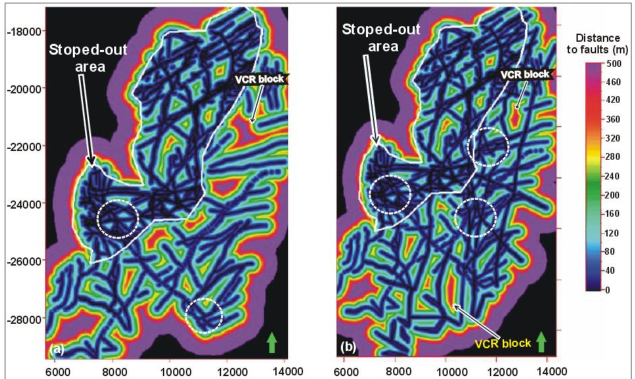
Fig. 14. Compartment size maps for all structures. (a) Seismically imaged faults and underground mapped structures from stoped-out areas. (b) The integration of seismically imaged faults with underground mapped faults and dikes from both stoped-out and development areas. White circles represent the zones of complex ground conditions that are not ideal for mining.
