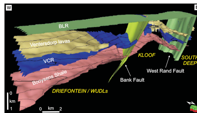
Figure 8. The 3D regional model constructed from reflectors of the BLR, Ventersdorp lavas, VCR, and Booyens Shale.
