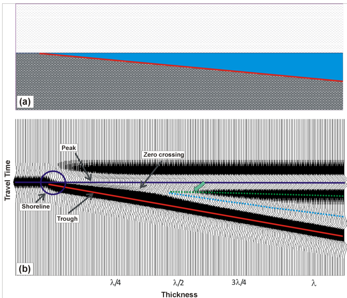
Fig. 3. (a) Geological wedge-shaped models. The top layer is the metabasalts of the Klipriviersberg (white); the layer below is quartzite (black) and the middle layer (blue) is the alternation of sand, quartzite and conglomerates. (b) Synthetic seismic section of the wedge model, with a wavelet dominant frequency of 65 Hz. The wedge thickness ranges from \lambda/4 (close to the shoreline or subcrop position) to \lambda (away from the shoreline position).
