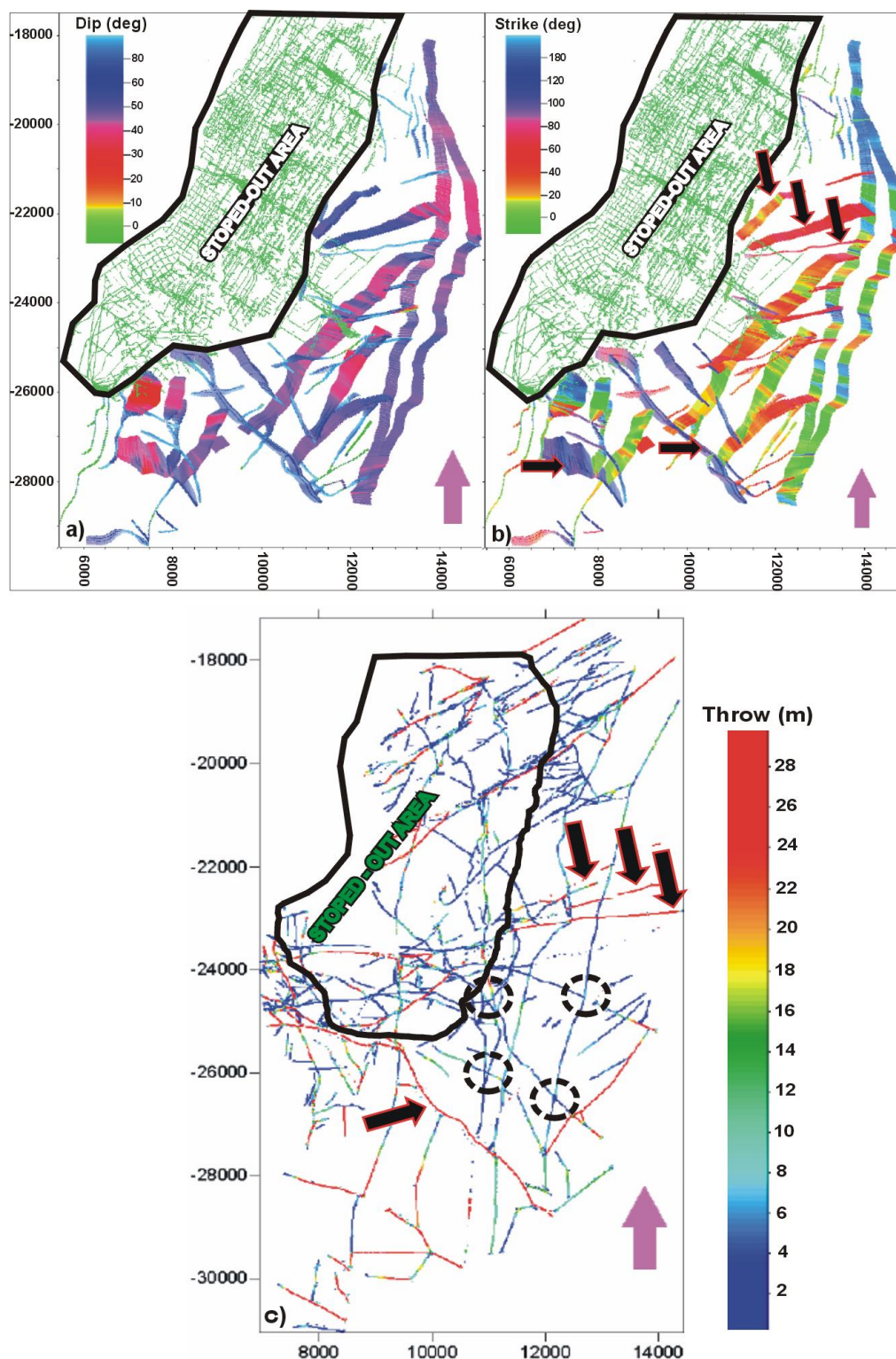
Fig. 12. Geometrical attributes for the seismically imaged faults. (a) Faults colour coded for dip. (b) Faults colour coded for strike. (c) Fault throw map for stopped-out and development area showing throw linear colour gradient. Note that the structures that are present in the model developed from mapping (geomodel) (c) and seismics (a) are indicated as red arrows.
