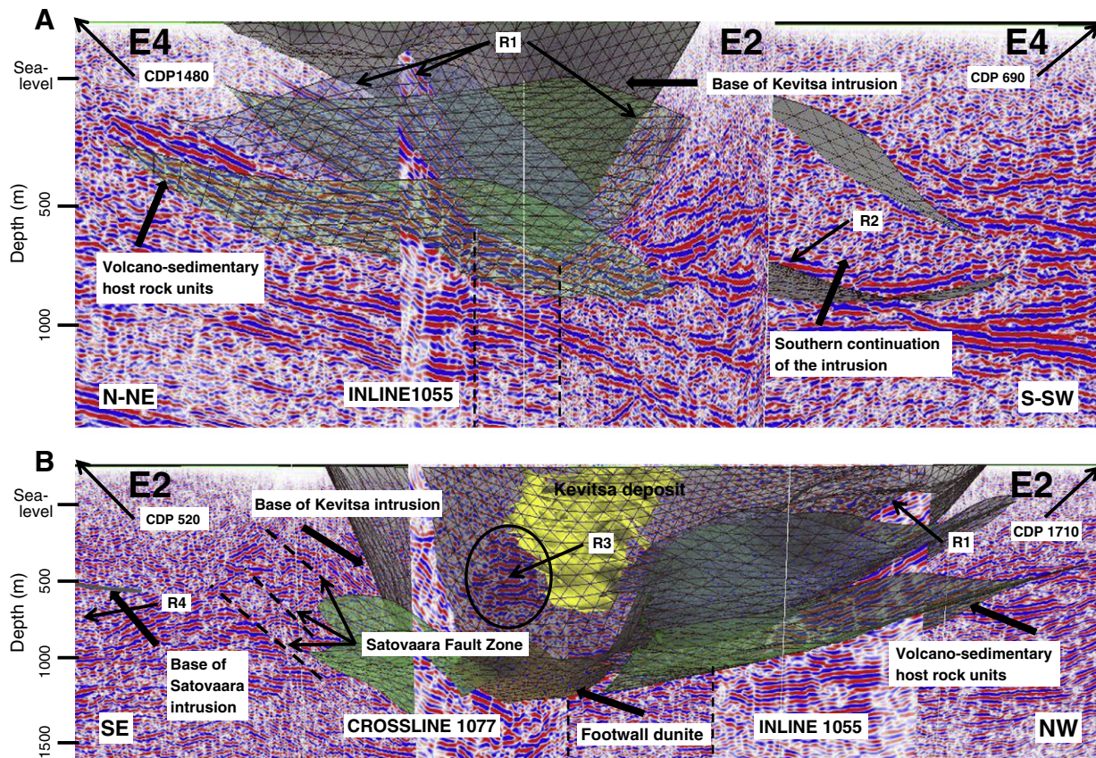
Fig. 7. (A) 3D visualization of Kevitsa 2D seismic lines E4 and E2 and an inline from the 3D seismic volume (Fig. 4) with the interpreted base of the Kevitsa intrusion, southern continuation of the intrusion, and some interpreted host rock units. Coloring of the host rock units follows the coloring on the surface geological map in Fig. 4. R1 marks the continuous reflectors at the contact to the Kevitsa intrusion and R2 the continuous reflectors, which have been interpreted as a previously unknown southern continuation of the Kevitsa intrusion (compare with the cross-sections in Fig. 5). (B) 3D visualization of Kevitsa 2D seismic line E2 and 3D seismic data (Fig. 4) with the interpreted bases of the Kevitsa and Satovaara intrusions, Satovaara Fault Zone, some host rock units and footwall dunite unit beneath the Kevitsa intrusion. Coloring of the host rock units follows the coloring on the surface geological map in Fig. 4. The Kevitsa deposit is shown in yellow (courtesy of the Kevitsa Mining Oy/First Quantum Minerals Ltd). R1 marks the continuous reflectors at the contact to the Kevitsa intrusion and R3 the reflectivity internal to the intrusion that has been interpreted to indicate spatially discontinuous magmatic layering within the intrusion. R4 indicated continuous reflectivity that is interrupted by the Satovaara Fault Zone, but continues again beneath the Satovaara intrusion.
