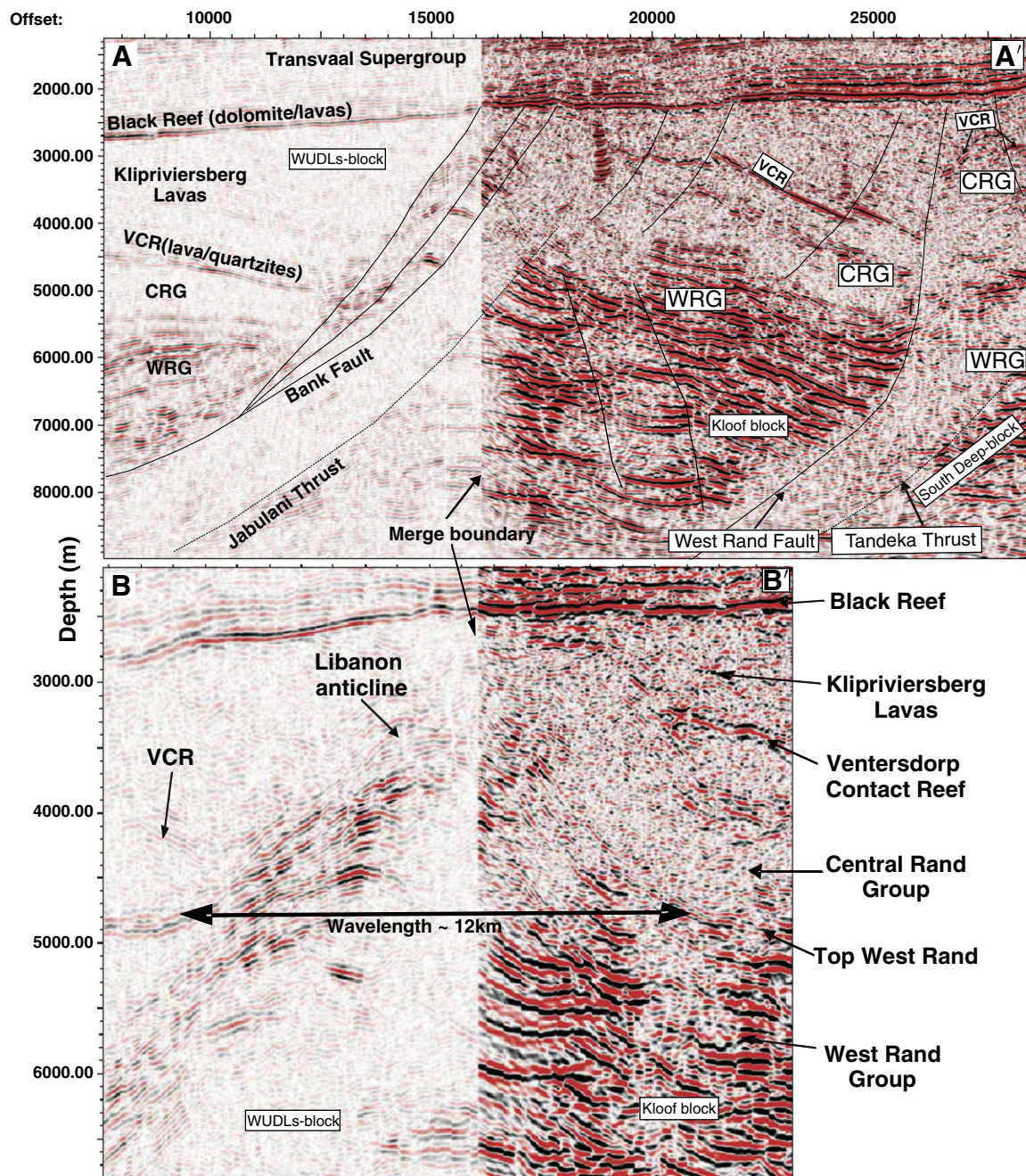
Fig. 11. (A) Seismic section (amplitude display) across the West Rand and Bank faults, showing the Jabulani and Tandeka thrusts at about 1.2 km below the Bank Fault and West Rand Fault, respectively. (B) Seismic section (amplitude display) across the major Libanon anticline at the merge boundary of the 1995 WUDLs and 2003 Kloof seismic survey. WUDLs: Western Ultra Deep Levels; WRG: West Rand Group; CRG: Central Rand Group; VCR: Ventersdorp Contact Reef. Note sharp change in the amplitudes is due to different datasets that were merged together.
