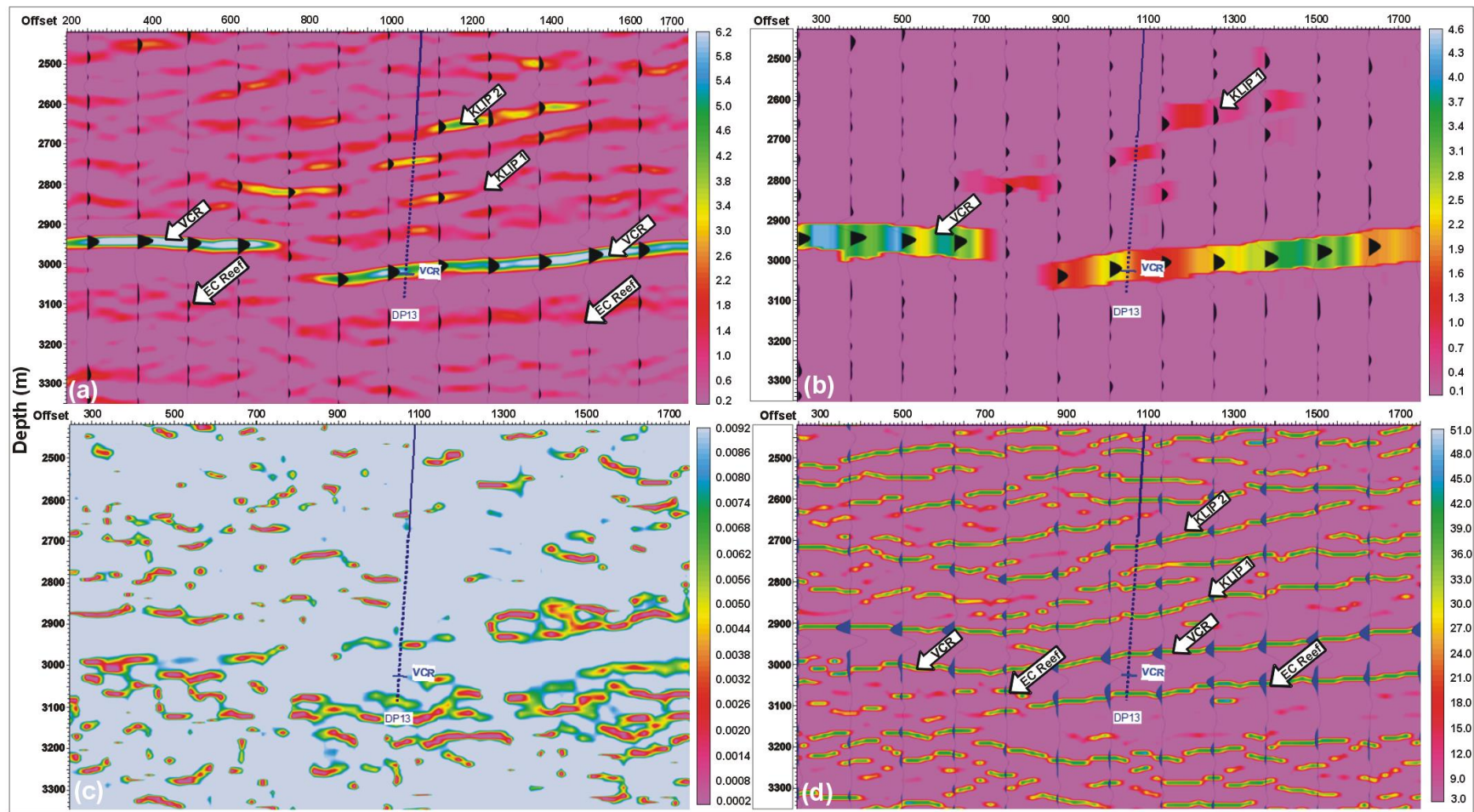
Fig. 9. Seismic section (L1 in Figure 1) (a) Reflection strength display (wiggle trace) showing strong seismic amplitude related to the VCR imaging. (b) Average energy display (wiggle trace) showing optimum imaging of the VCR but poor EC reef imaging. (c) Instantaneous frequency display showing poor imaging for both VCR and EC reef. (d) Paraphase display (wiggle trace) highlighting lateral continuity of the EC reef and enhancement of minor faults. The color overlays exhibit more information than is visible on traditional black and white seismic sections. VCR: Ventersdorp Contact Reef; EC: Elsburg Conglomerate; KLIP: Klipriviersberg
