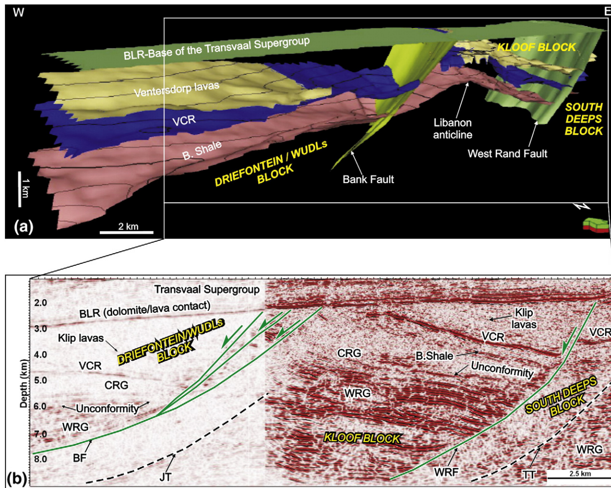
Fig. 2. Seismic model across the Witwatersrand goldfields. (a) 3D regional seismic model incorporating the BLR, Ventersdorp lavas, VCR and B. Shale. The model shows the geometry of West Rand Fault, Bank Fault and Libanon Anticline. (b) Regional crossline seismic section (line AA' in Fig. 1) through WUDLS, Driefontein, Kloof and South Deep surveys, showing WRF and BF zones and their adjacent TT and JT, respectively. WRF: West Rand Fault; BF: Bank Fault; TT: Tandeke Thrust; JT: Jabulani Thrust; WRG: West Rand Group; CRG: Central Rand Group; Klip: Klipriviersberg; VCR: Ventersdorp Contact Reef; BLR: Black Reef Formation; B. Shale: Booyensens Shale.
