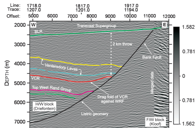
Figure 6. Seismic section (amplitude display) across the Bank Fault with a throw of 2 km showing the listric (concave-up) nature of the fault.
