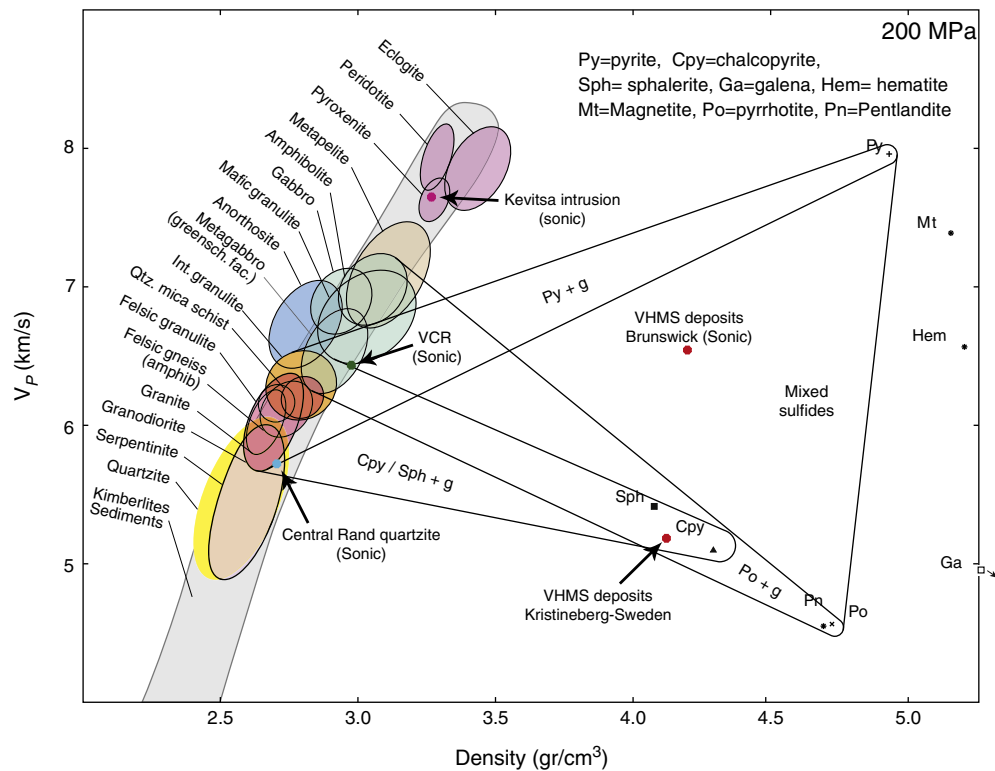
Fig. 3. Acoustic properties of most common crystalline rocks and ores (modified after Salisbury et al., 2003). Shown are also VHMS samples from the Brunswick No. 6 (Malehmir and Bellefleur, 2010) and Kristineberg mine in Sweden (Malehmir et al., 2013), Kevitsa olivine–pyroxenite (Koivisto et al., 2012; Malehmir et al., 2012a) and the lava in the hanging wall of the Ventersdorp Contact Reef (VCR) and the Central Rand quartzite in its footwall. (Manzi et al., 2012a,b).
