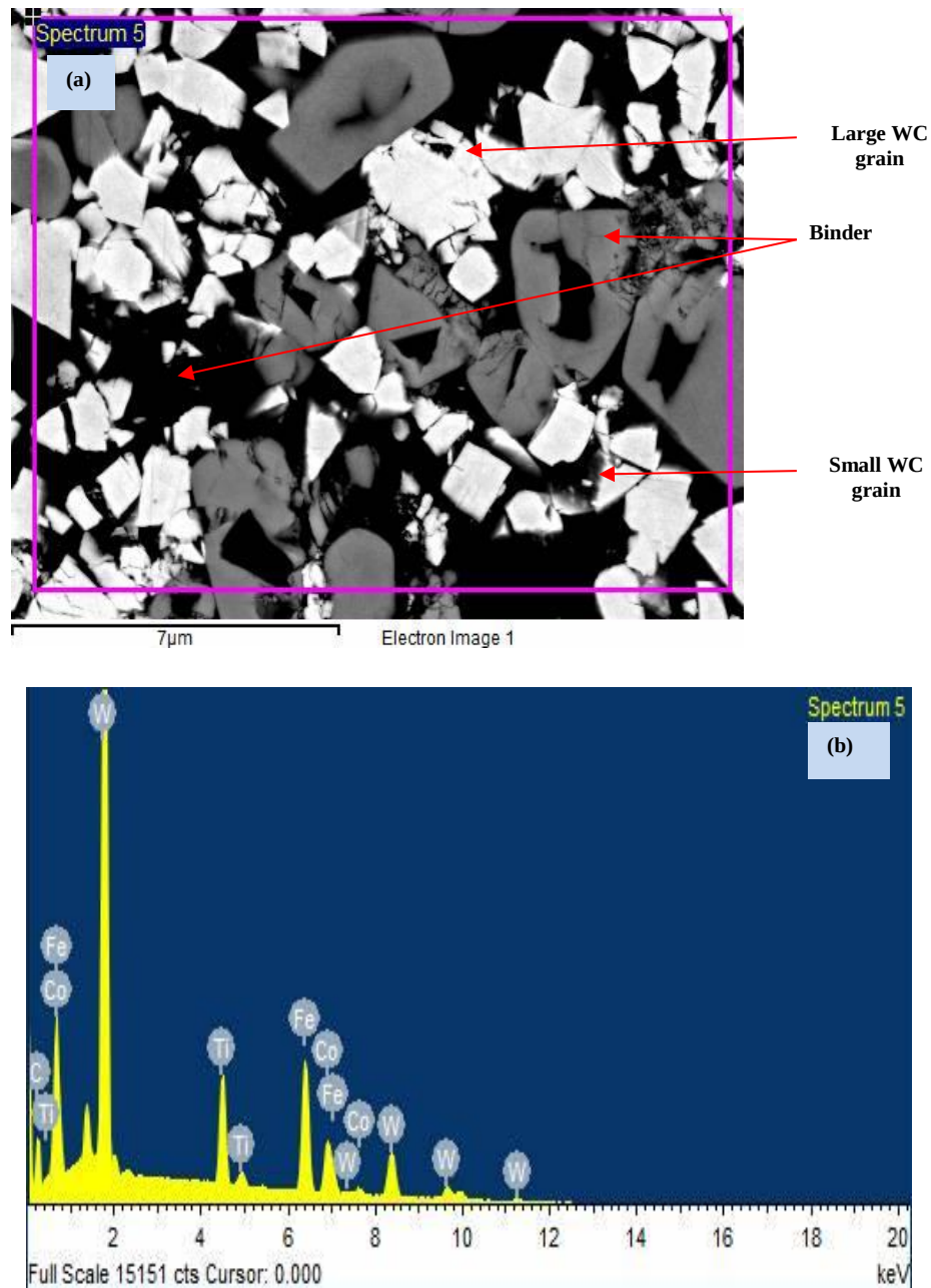
Figure 4.6: (a) SEM-BSE micrograph on the overall average and (b) the spectrum of elements present in the as-sintered sample B.
