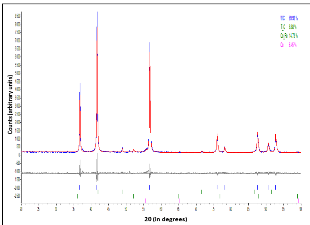
Figure 4.18: Rietveld analysis for the as-milled powder sample B.
