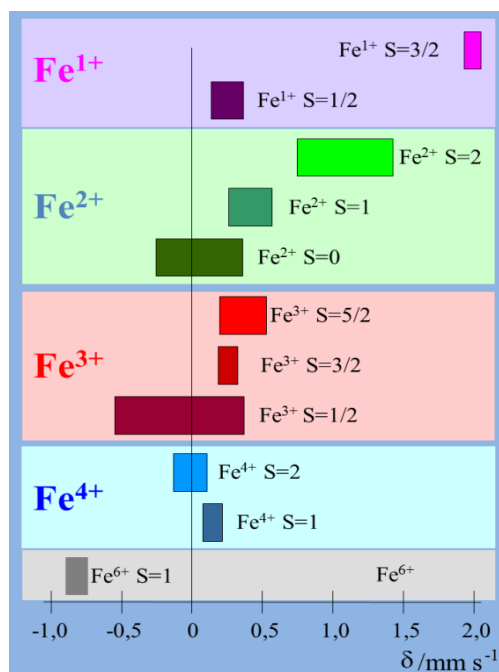
Figure 2.8: Isomer shift values and oxidation states observed for ^{57}\text{Fe} compounds measured at room temperature [53].
