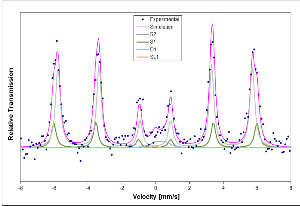
Figure 4.21: CEM spectrum for the as-sintered WC-Co-TiC-Fe sample obtained at room temperature.
