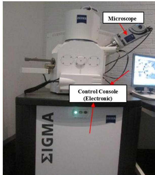
Figure 3.4: Carl Zeiss Sigma field emission scanning electron microscopy (FESEM).
