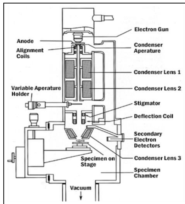
Figure 3.5: Schematic diagram of a scanning electron microscope [63] .
