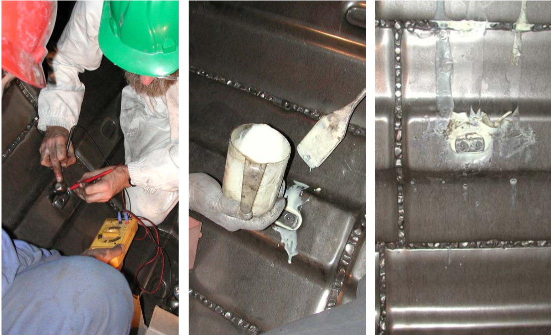
Figure A3.1.1: Conductivity probe installation process: Probe electrical isolation (left); Mixing and pouring of the resin between the bolt and liner (middle). Solidified resin, ready for surface grinding (right).
