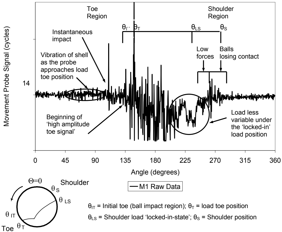
Figure 4.6: Typical movement probe profile, indicating toe and shoulder region characteristics (second experimental program, Test 3 (OR-Gatedata), Cycle 14).
