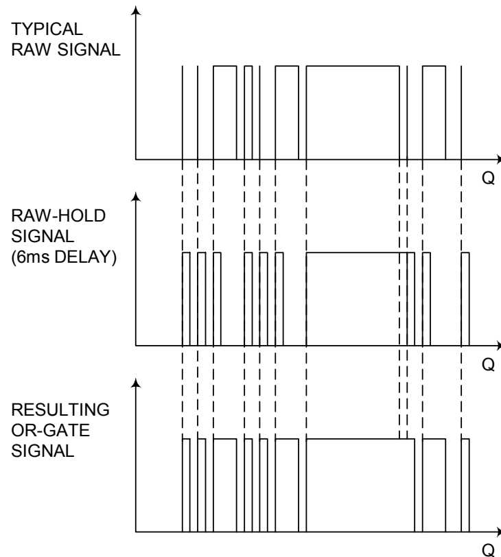
Figure 3.13: Graphical illustration indicating how a typical raw signal is transformed using raw-hold and OR-Gate signals.
