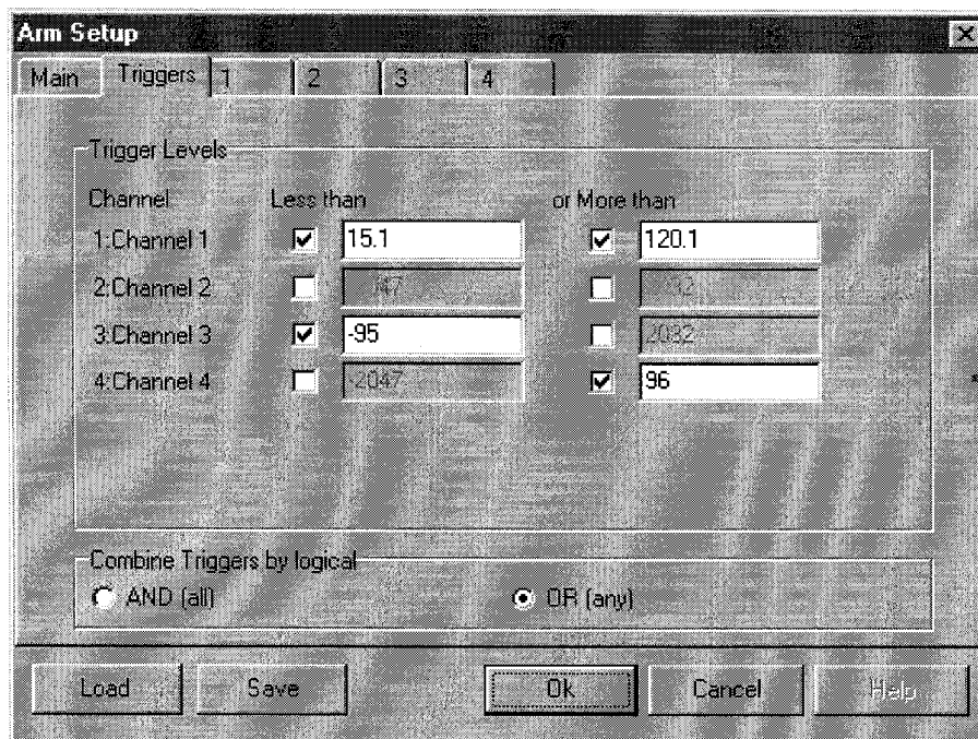
Figure A1.3 Triggered Start Setup Window
