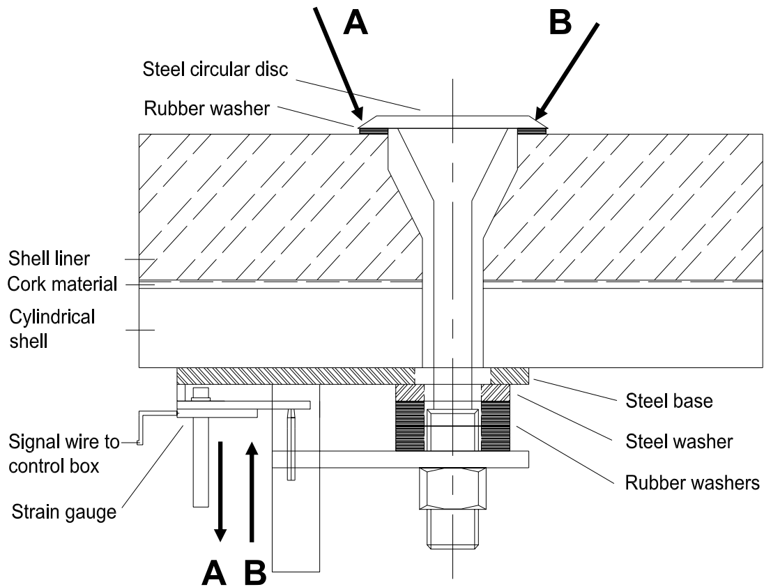
Figure 4.8: Diagram illustrating movement probe installation and effect of different forces on the strain bridge and in turn movement probe results. Force A tends to bend the probe downwards, while force B bends the probe upwards.
