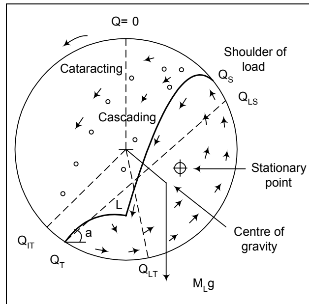
Figure 2.1: Load orientation in a grinding mill
