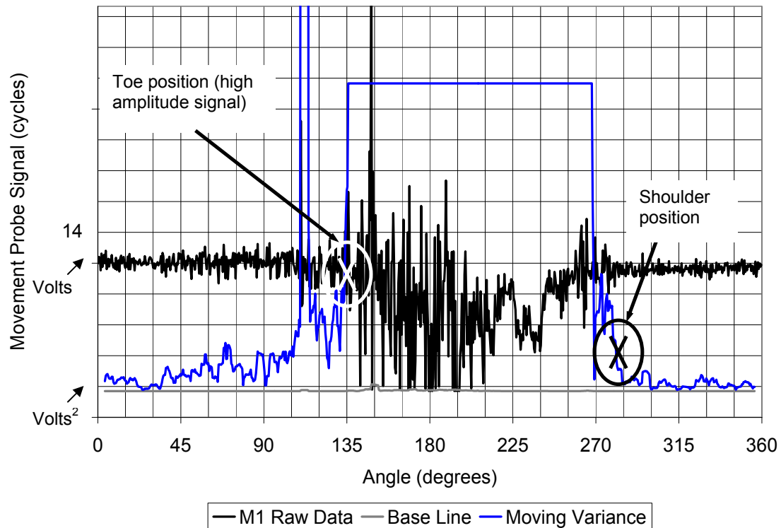
Figure 4.7: Processed movement probe data profile (M1), using moving variance analysis. Second experimental program, Test 3 (OR-Gatedata), cycle (14). Moving variance graph is truncated for clarity purposes.
