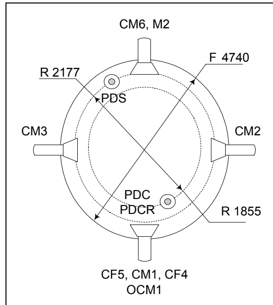
Figure 3.12: Experimental apparatus positioning on mill 2C for the second experimental program, indicating additional conductivity, photo-detector and movement probe locations.
