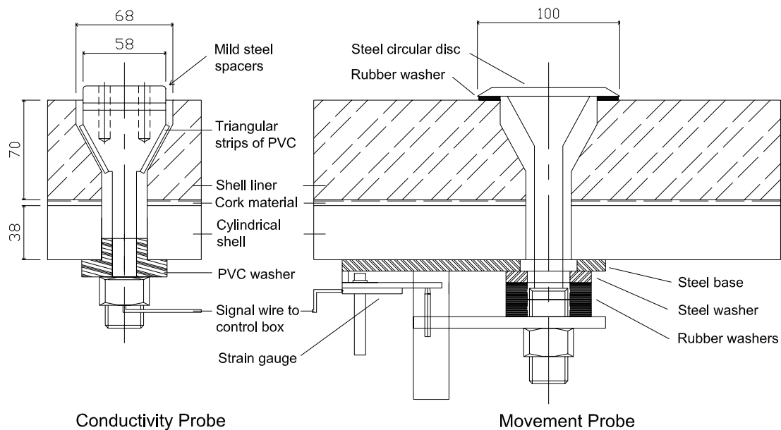
Figure 3.3: Cross-sectional view of conductivity and movement probes used to extract data from inside the mill shell.
