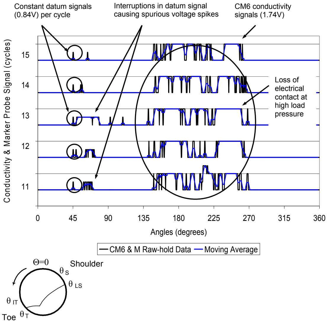
Figure 4.4: Conductivity probe data profiles from first experimental program (probe CM6 and datum signal, Test 3 (Raw-hold5minDelay), Cycles (11-15)). Profile indicates datum signals; voltage spikes; and probe CM6 conductivity signals per cycle.
