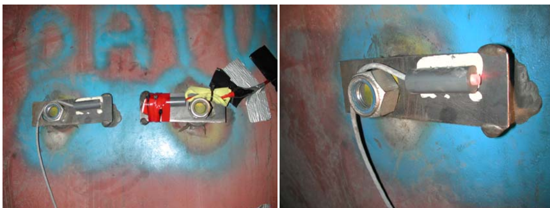
Figure A3.2.6: Picture illustrates marker signal setup (left); and photo-detector (right) with its base supported by quickset Pratley putty.
