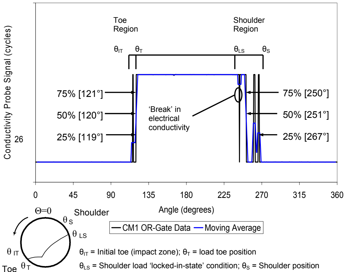
Figure 4.3: Detailed analysis of cycle 26 extracted from second experimental program (probe CM1, Test 3 (OR-Gatedata)). Profile indicates moving average analysis used in the selection of toe and shoulder positions.
