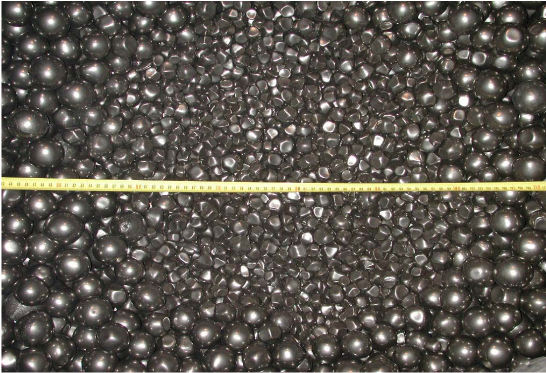
Figure 3.9: Ball load distribution at the surface; 800mm from mill feed drive end in a hole 100mm deep after barring.
