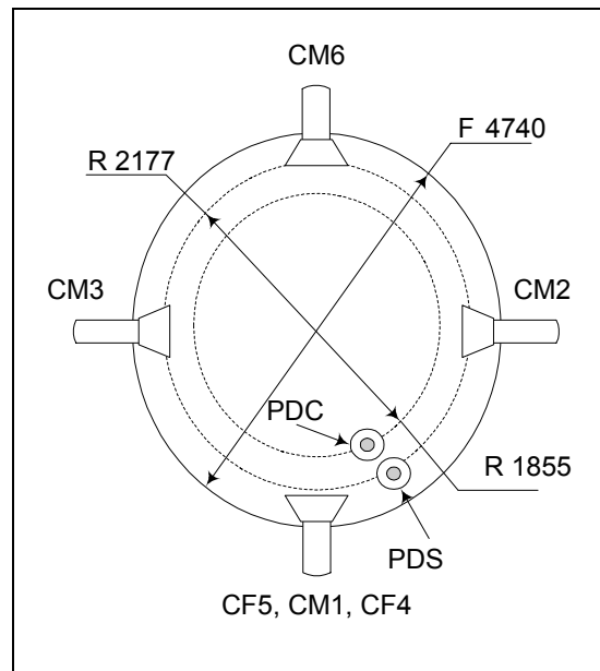
Figure 3.7: Experimental apparatus positioning on mill 2C for the first experimental program, indicating conductivity and photo-detector probe locations.
