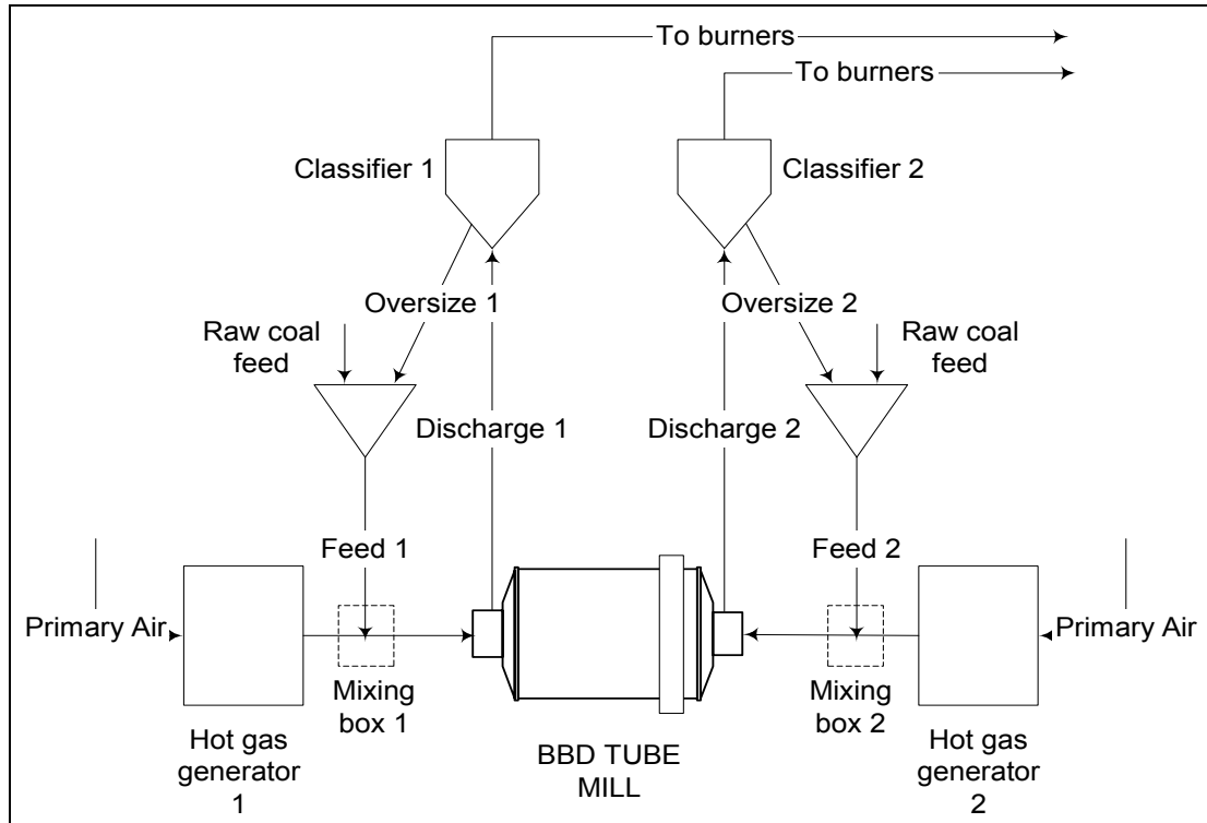
Figure 3.1: Flow diagram indicating Mill 2C's direct firing cycle.
