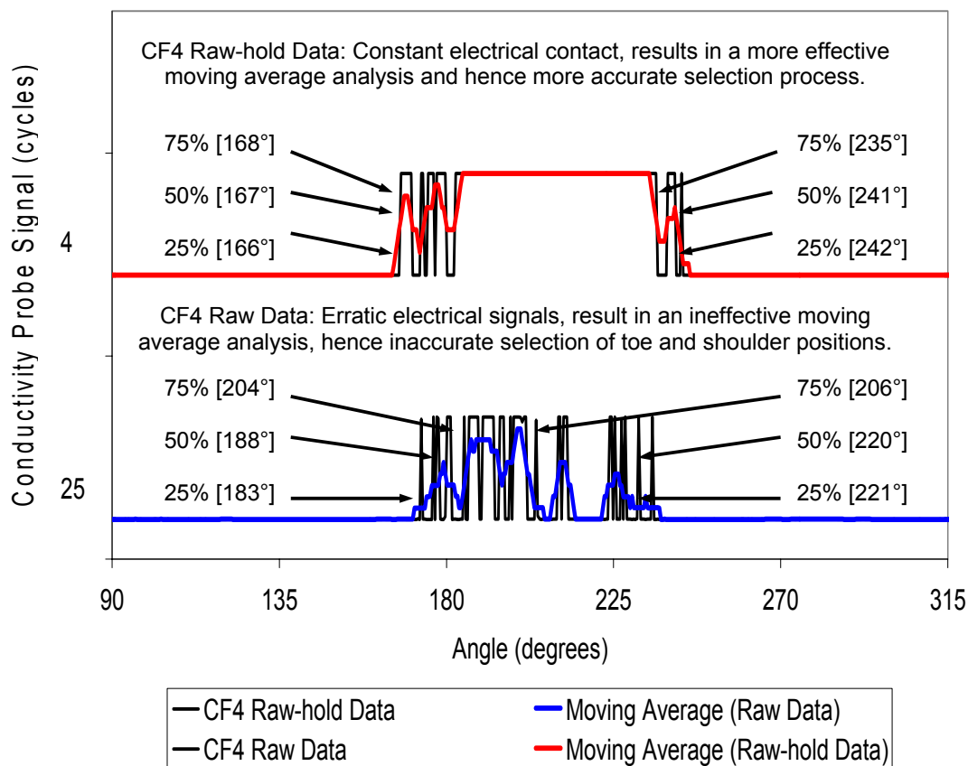
Figure 4.5: Conductivity probe data profile from first experimental program (probe CF4: Test 2 (Raw-holdNoDelay), Cycle (4) and Test 4 (RawNoDelay), Cycle (25)). Figure compares the raw-hold to raw signal electrical conductivity signal and affect these signals have on the moving average trend line and hence data selection process.
