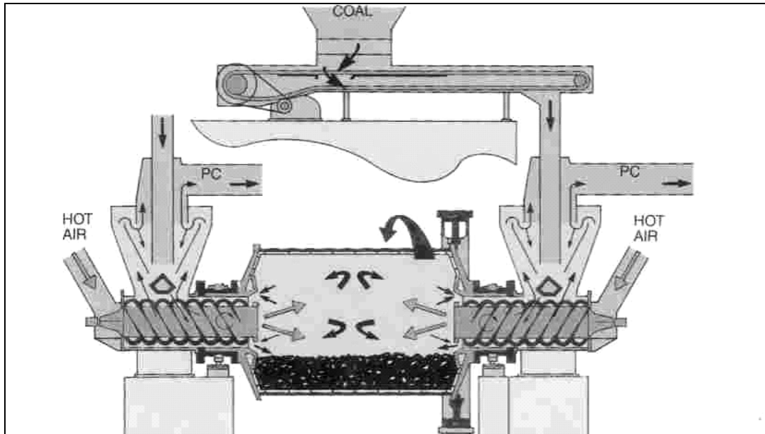
Figure 2.4: Illustration of coal flow process through a typical Stein Industrie BBD type tube mill
