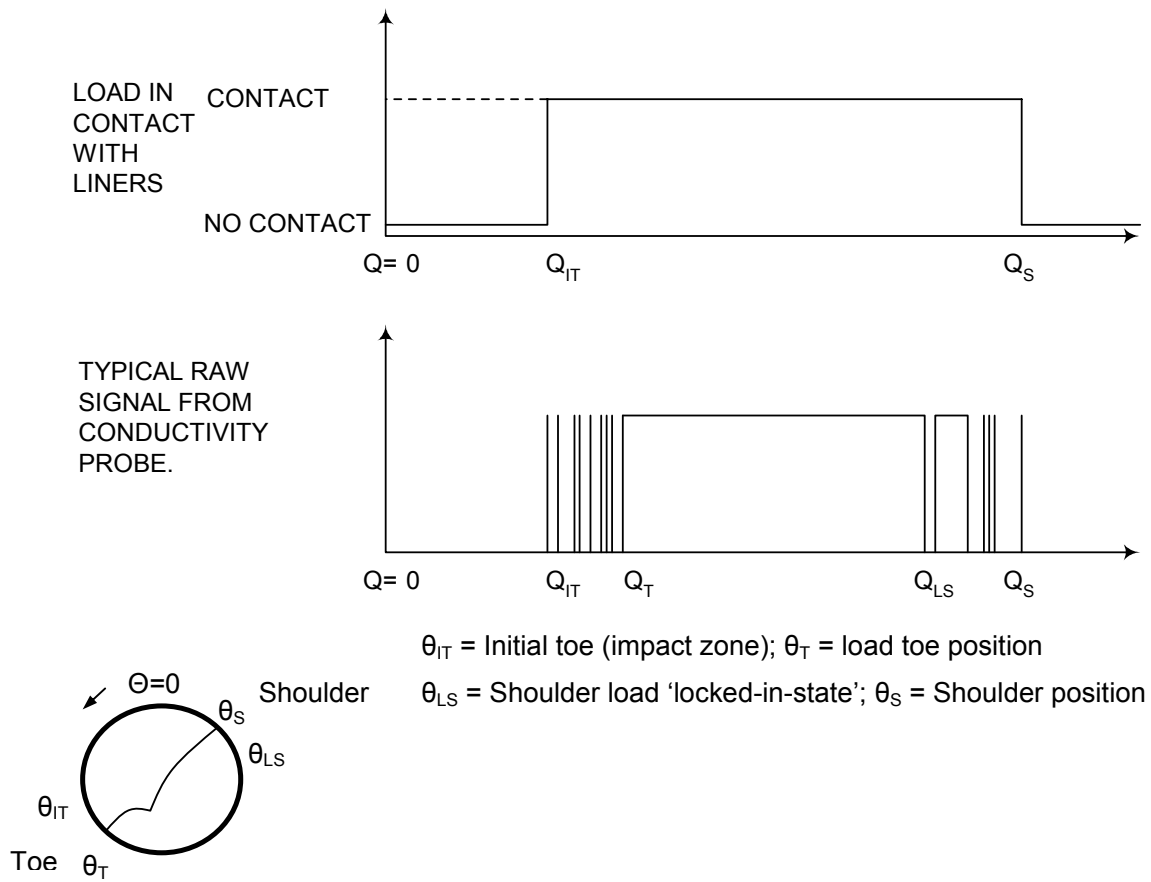
Figure 3.5: Variation of key conductivity signals during a rotation in the mill.
