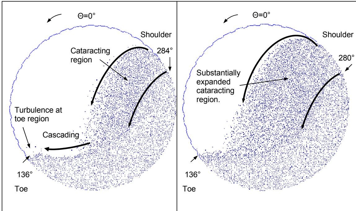
Figure 4.14: Ball density plot representing worn liner load behaviour for a \Phi 4.74\text{m} ball mill (effective diameter \Phi 4.656\text{m} ); 19.4% load volume; 50mm balls. Display indicates turbulent toe region thought to have been caused by the cascading ball action rushing towards the toe.
