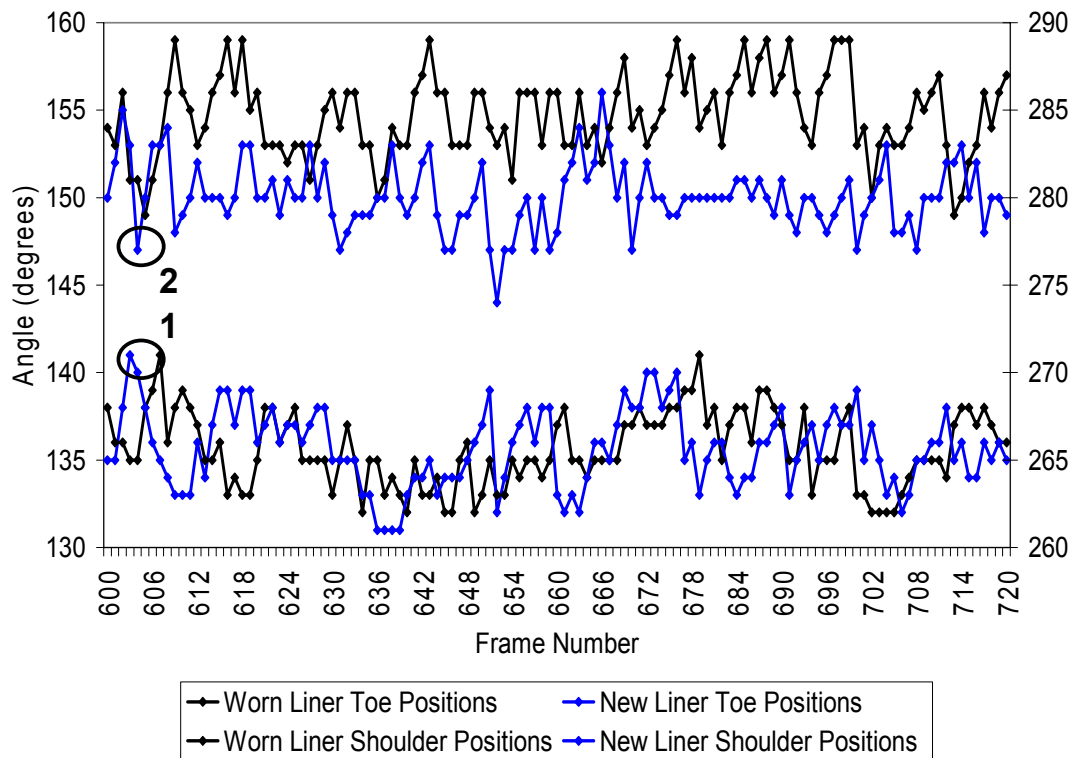
Figure 4.15: Millsoft plot comparing simulation results selected from worn and new liners simulations (revolution 11, 121 frames (frame no. 600 -720)). Plot indicates similarity in toe positions and a higher shoulder position for worn liners, implying more cataracting ball action
