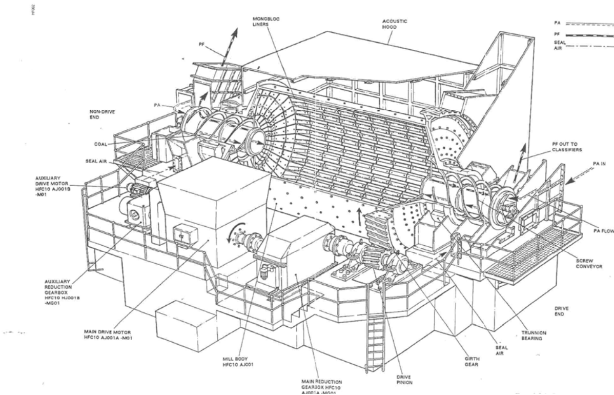
Figure 2.2: Cross-sectional view of typical Stein Industrie type tube mill (Spiral direction to be reversed)
