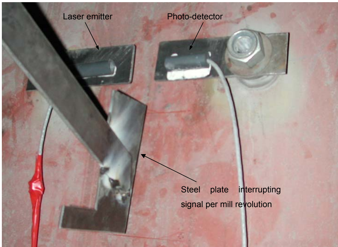
Figure A3.2.3: Picture illustrates marker signal setup; laser and photo-detector mounted on mill shell; steel plate positioned to interrupt laser signal per mil revolution.
