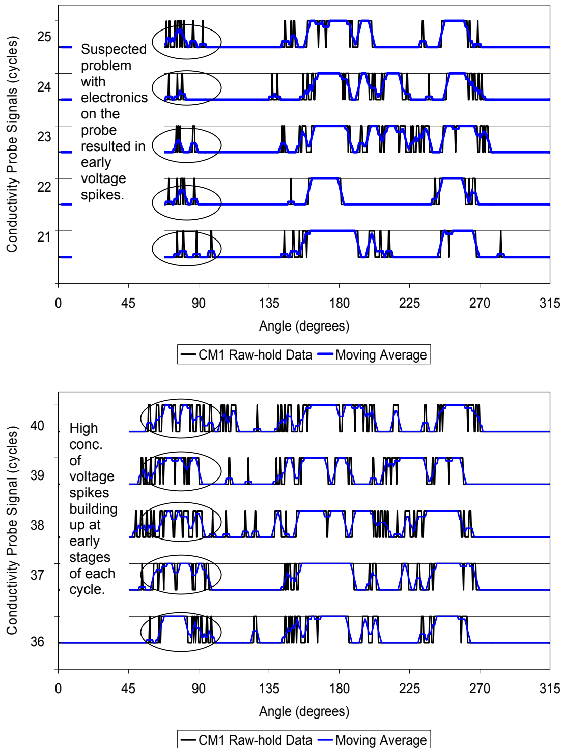
Figure A5.1: Conductivity probe CM1 data profiles from first experimental program: TOP: Test 2 (Raw-holdNoDelay), Cycles (21-25)); BOTTOM: Test 3 (Raw-hold 5minDelay), Cycles (36-40)). Conductivity cycles illustrate the increase in magnitude and duration of voltage spikes and their affect on the moving average trend line.
