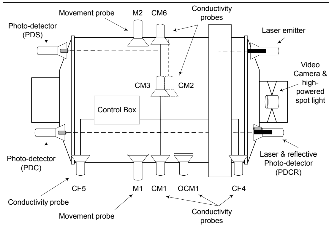
Figure 3.11: Experimental apparatus positioning on mill 2C for the second experimental program.
