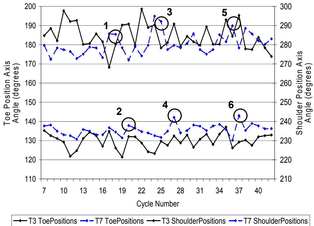
Figure 4.9: Movement probe (second experimental program) toe and shoulder position plots (cycles 7-42) for: Test 3 (ORGateNODelay) and Test 7 (DatumTestNoDelay).
