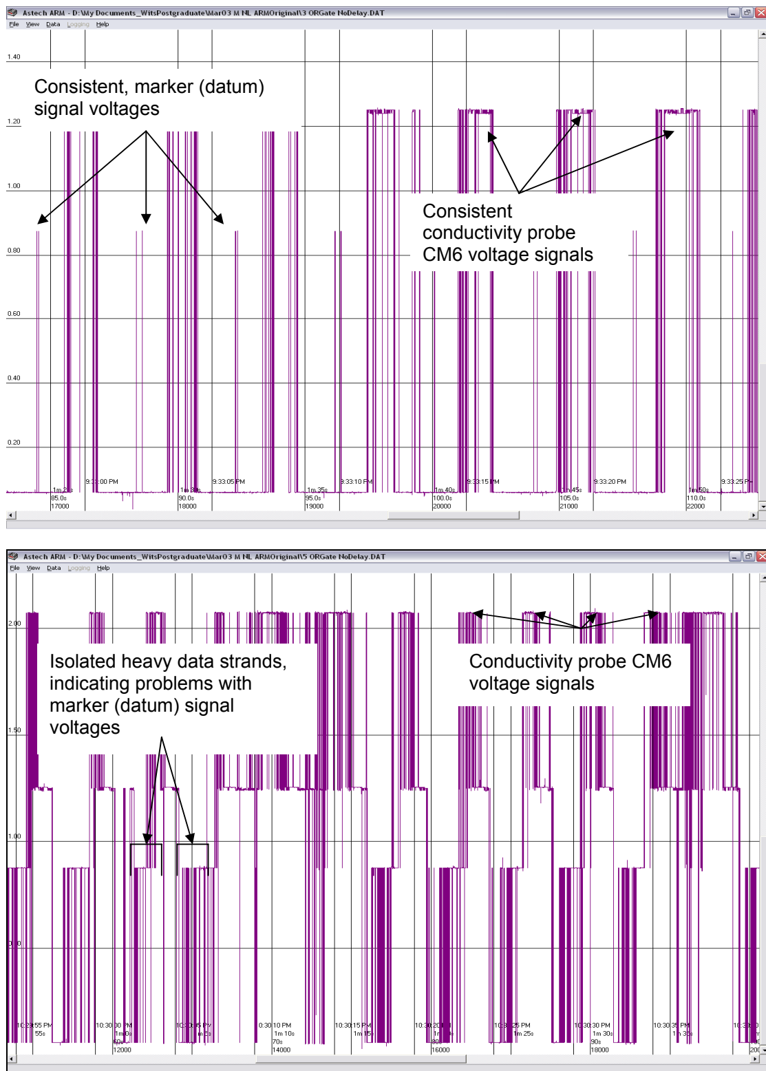
Figure A5.2: ARM graphical display of conductivity probe CM6 and marker signal data from second experimental program. X and Y scales represent time and voltage, respectively. TOP: Test 3 (ORGateNoDelay) Cycles (17-24), well defined marker and CM6 voltage signals; BOTTOM: Test 5 (ORGateNoDelay) Cycles (17-27)), poor data (less than 40% of useful data).
