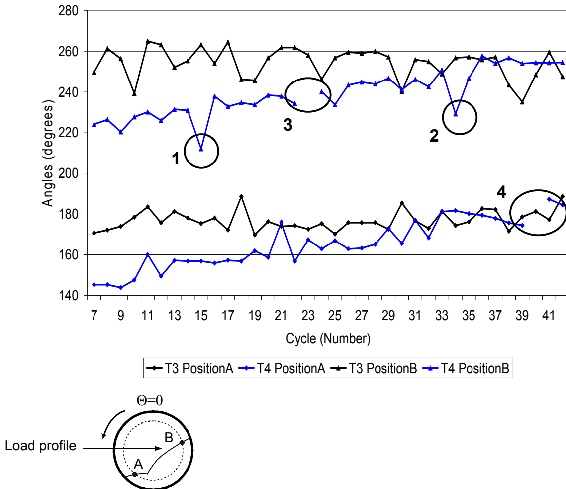
Figure 4.12: Photo-detector (PDCR) plot comparing test 3 (ORGateNoDelay) and test 4 (ORGate2minDelay) 75 per cent degree values for positions A and B, between cycles 7 - 42.
