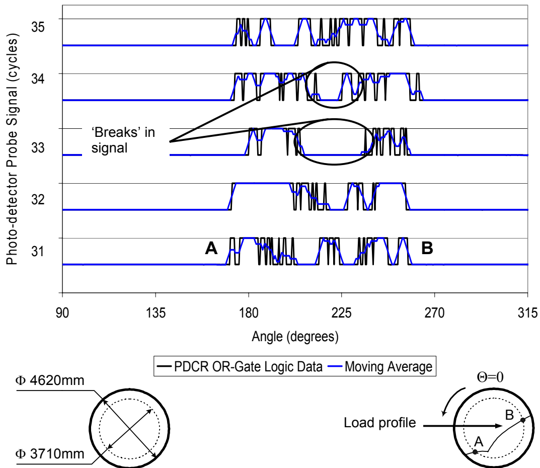
Figure 4.10: Typical (PDCR) photo-detector probe profile, including moving average analysis, indicating positions A and B (second experimental program, Test 3 (OR-Gatedata), cycles (31-35).
