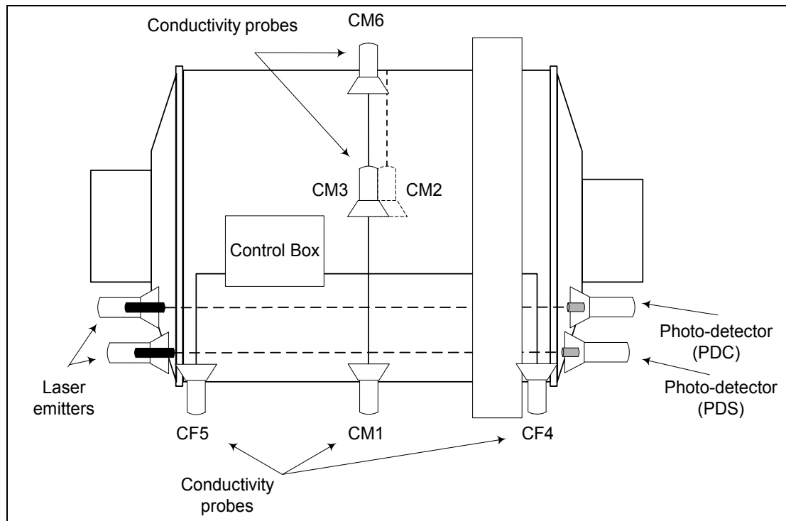
Figure 3.6: Diagram representing experimental apparatus positioning on mill 2C for the first experimental program.
