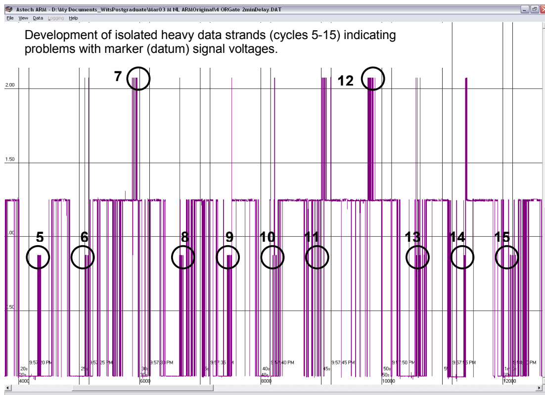
Figure 4.11: ARM graphical display of conductivity probe CM6 and datum signal data from second experimental program. X and Y scales represent time and voltage, respectively. Test 4 (ORGate2minDelay) Cycles (5-15).
