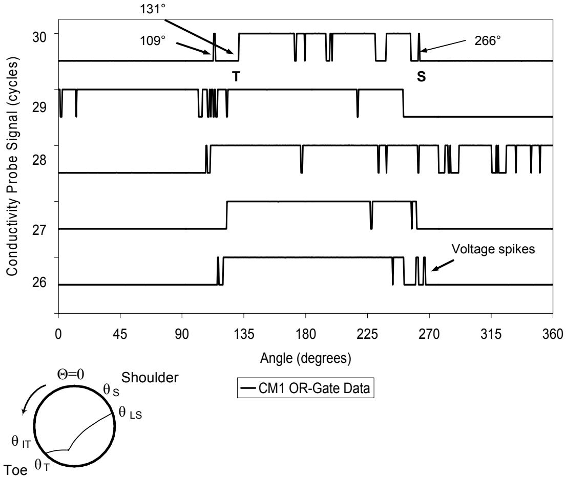
Figure 4.2: An example of typical conductivity probe data profiles from second experimental program (probe CM1, Test 3 (OR-Gate data), Cycles (26-30)). Profile indicates load toe (T) and shoulder (S) positions as well as other load shape characteristics.
