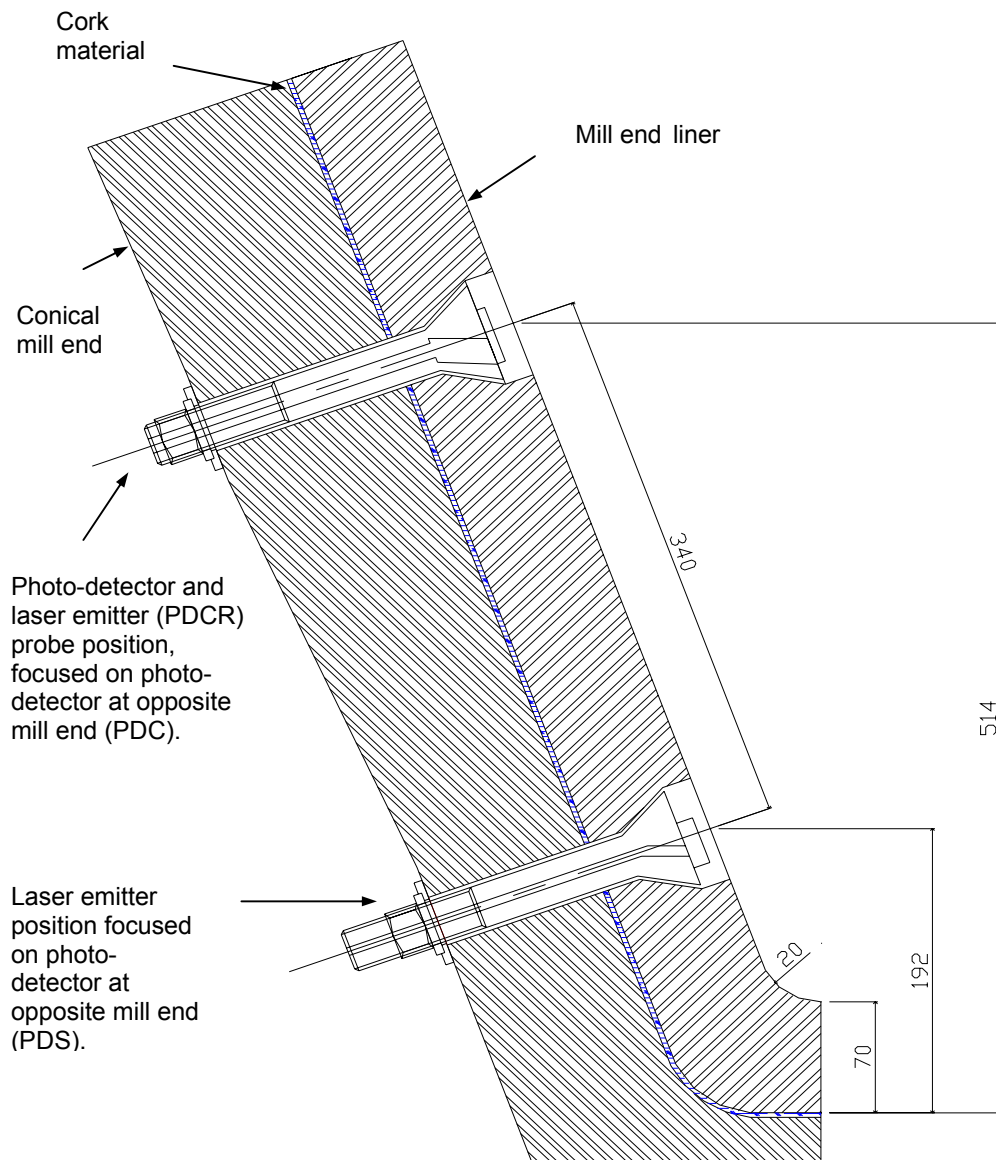
Figure 3.4: Cross-sectional view displaying typical positioning of the of emitter and receiver probes as installed at the mil ends to extract data from inside the mill shell.
