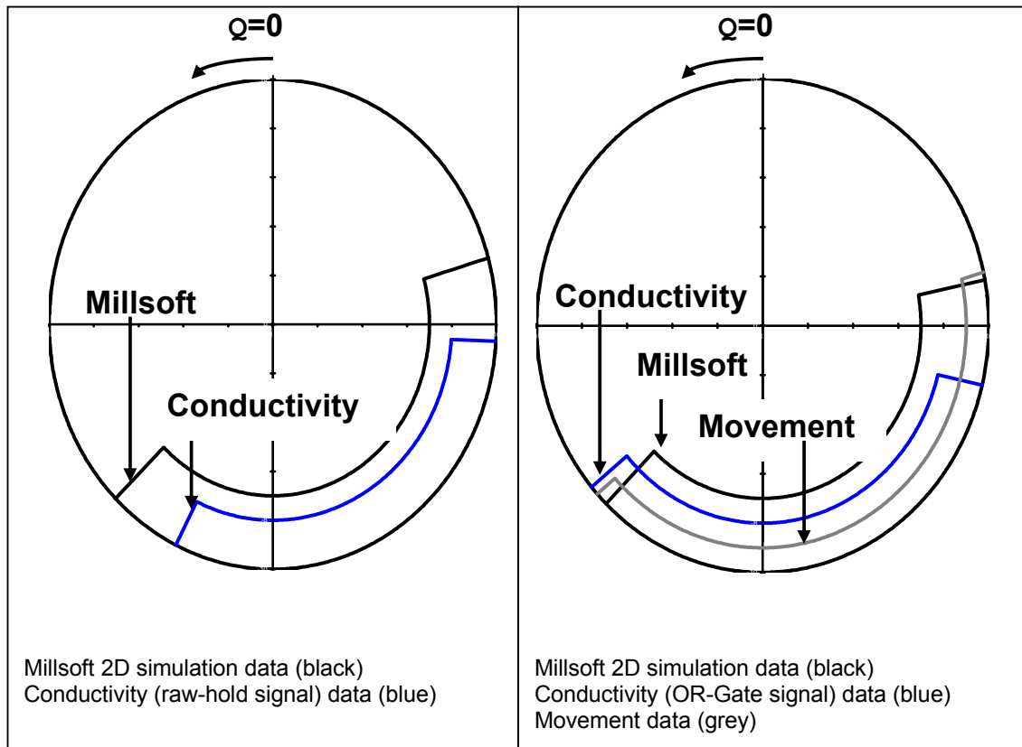
Figure 4.16: First experimental program (worn liner) load arithmetic mean toe and shoulder results indicated along the mill shell
