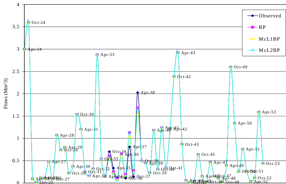
Figure 8.2b Comparison of ANNs in terms of hydrographs at D1H004 (13.3 % missing seasonal mean flows from 1934) using base gauge D1H001
