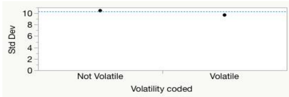
Figure 10: Variance analysis in terms of equal distribution
