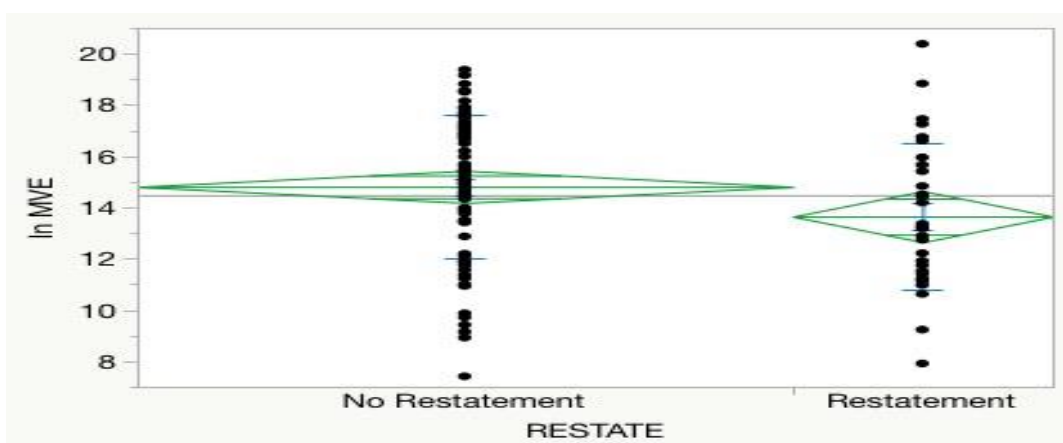
Figure 5: ANOVA restatement grouping
