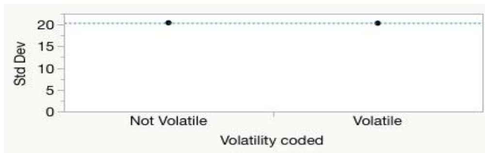
Figure 18: Variance analysis in terms of equal distribution
