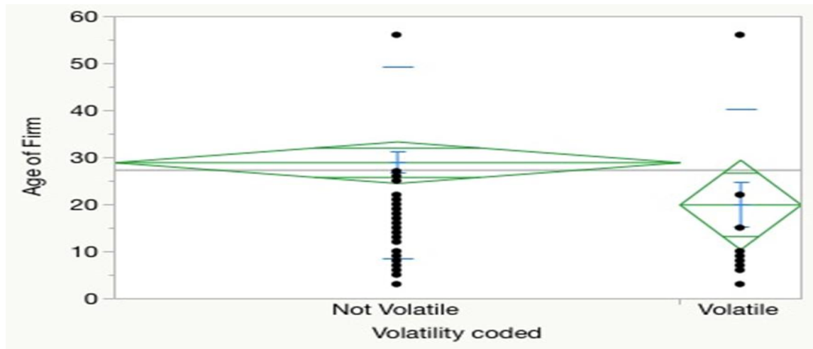
Figure 17: ANOVA restatement grouping
