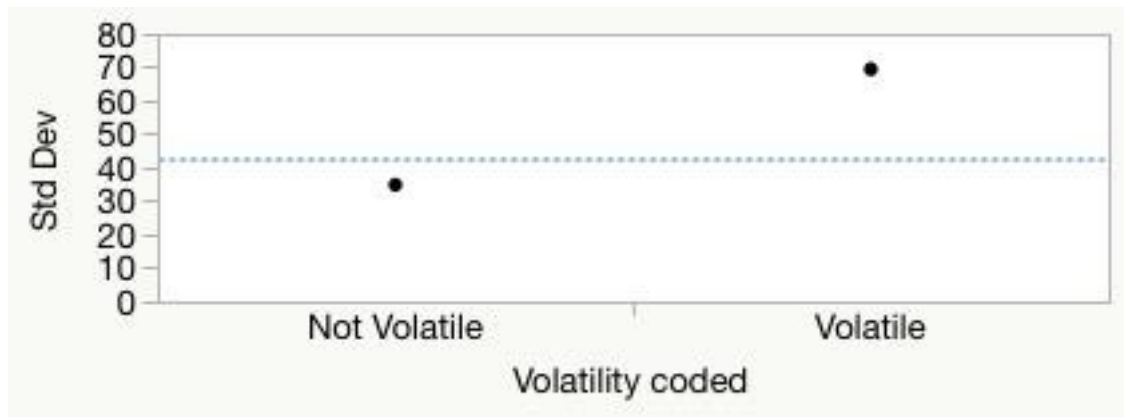
Figure 20: Variance analysis in terms of equal distribution
