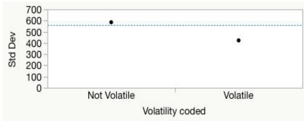
Figure 16: Variance analysis in terms of equal distribution
