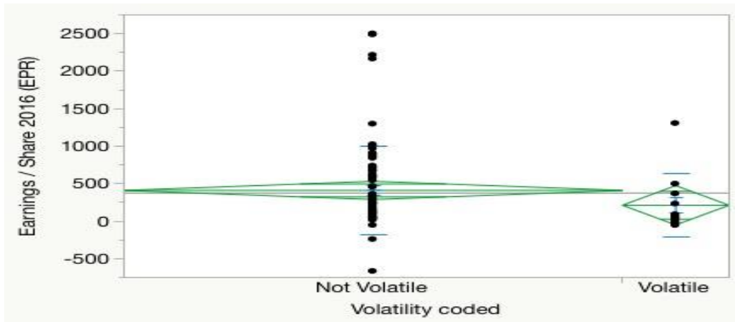
Figure 15: ANOVA restatement grouping
