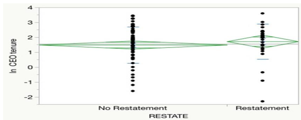
Figure 3: ANOVA restatement grouping
