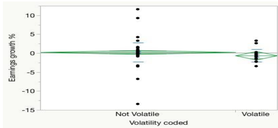
Figure 11: ANOVA restatement grouping
