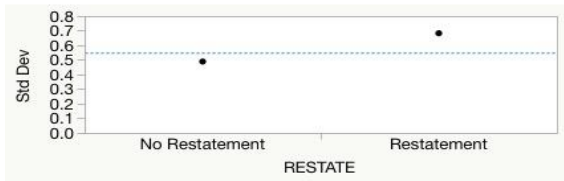
Figure 8: Variance analysis in terms of equal distribution
