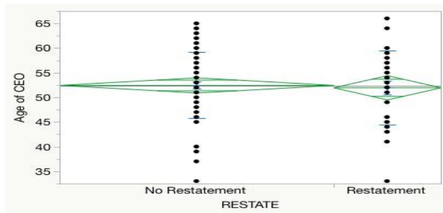
Figure 1: ANOVA restatement grouping
