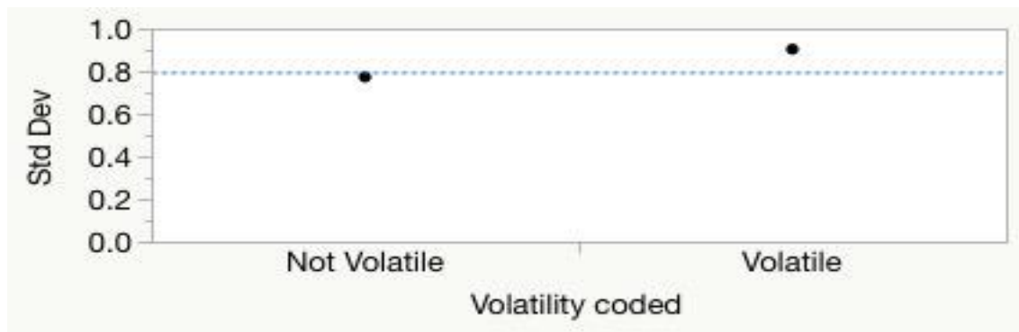
Figure 22: Variance analysis in terms of equal distribution
