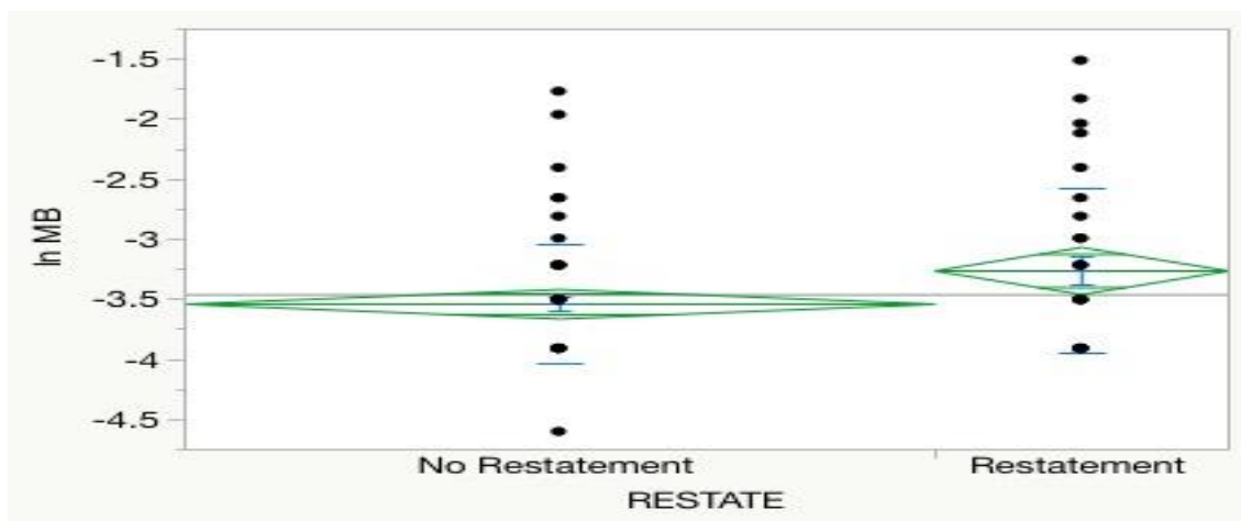
Figure 7: ANOVA restatement grouping
