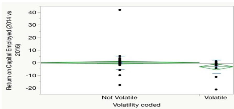
Figure 13: ANOVA restatement grouping
