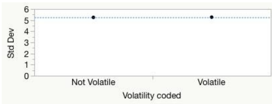
Figure 14: Variance analysis in terms of equal distribution
