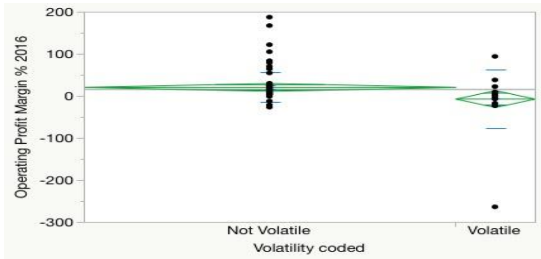
Figure 19: ANOVA restatement grouping
