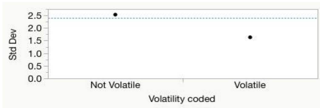
Figure 12: Variance analysis in terms of equal distribution
