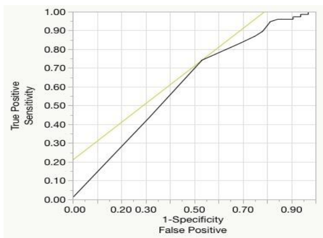
Figure 24: ROC [Receiver Operating Characteristics]
