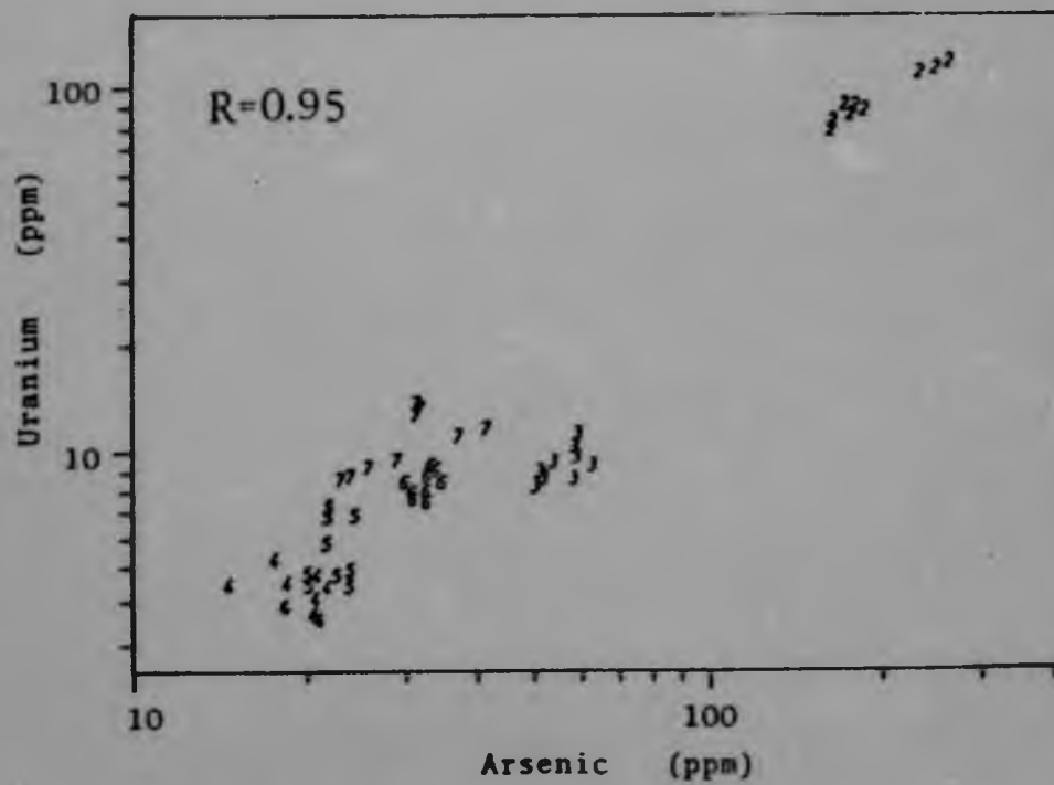
Figure 12.10 SCATTER DIAGRAM OF URANIUM AND ARSENIC
