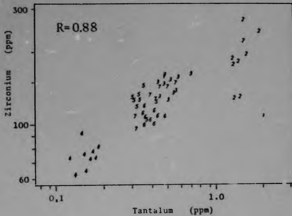
Figure 12.7 SCATTER DIAGRAM OF ZIRCONIUM AND TANTALUM
