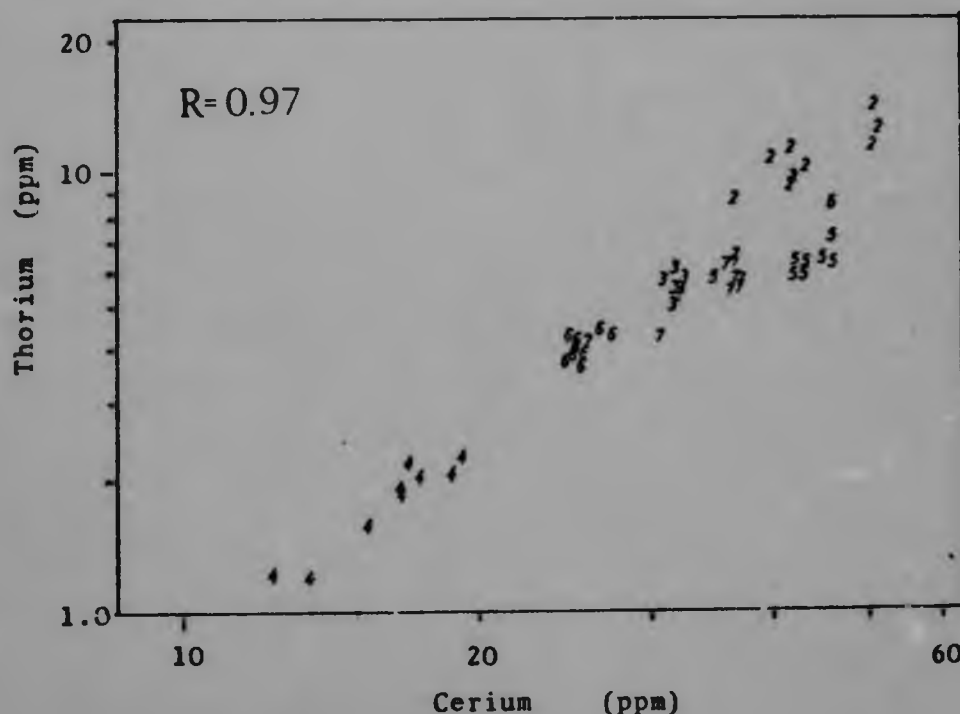
Figure 12.5 SCATTER DIAGRAM OF THORIUM AND CERIUM
