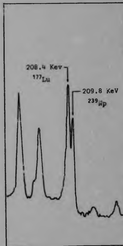
(b) Lutetium - Uranium Interference
