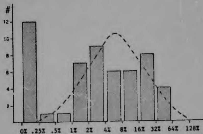
Figure 8.2 FREQUENCY DISTRIBUTION OF RELATIVE ERRORS FOR THE DETERMINATION OF 23 ELEMENTS IN FOUR U.S.G.S. STANDARDS
