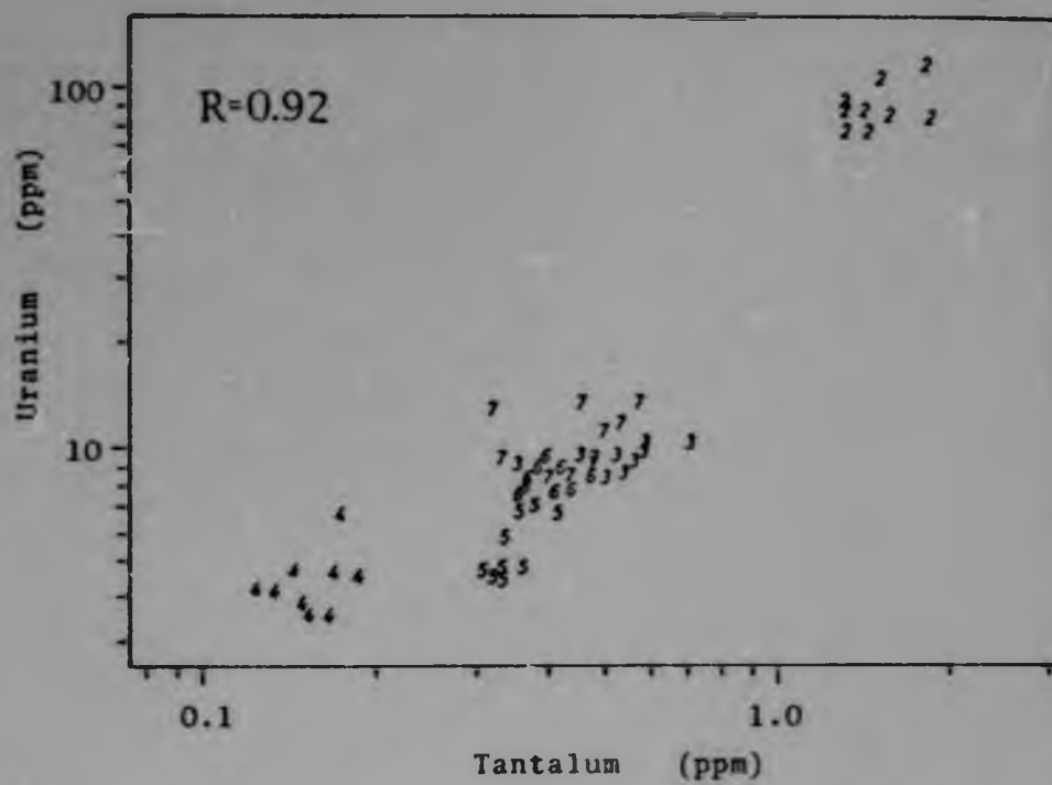
Figure 12.9 SCATTER DIAGRAM OF URANIUM AND TANTALUM
