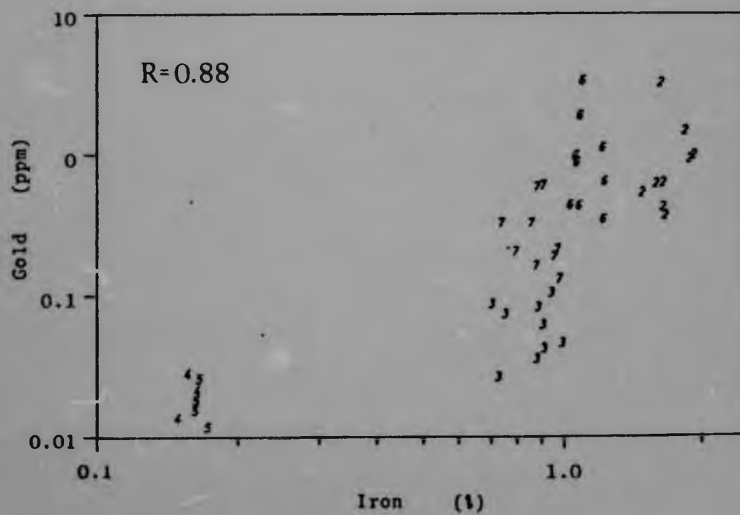
Figure 12.12 SCATTER DIAGRAM OF GOLD AND IRON
