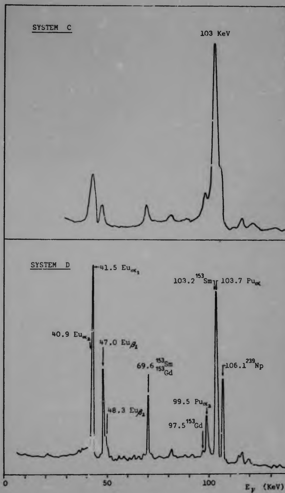
Figure 6.4 COMPARISON OF NORMAL AND HIGH RESOLUTION COUNTING SYSTEMS
