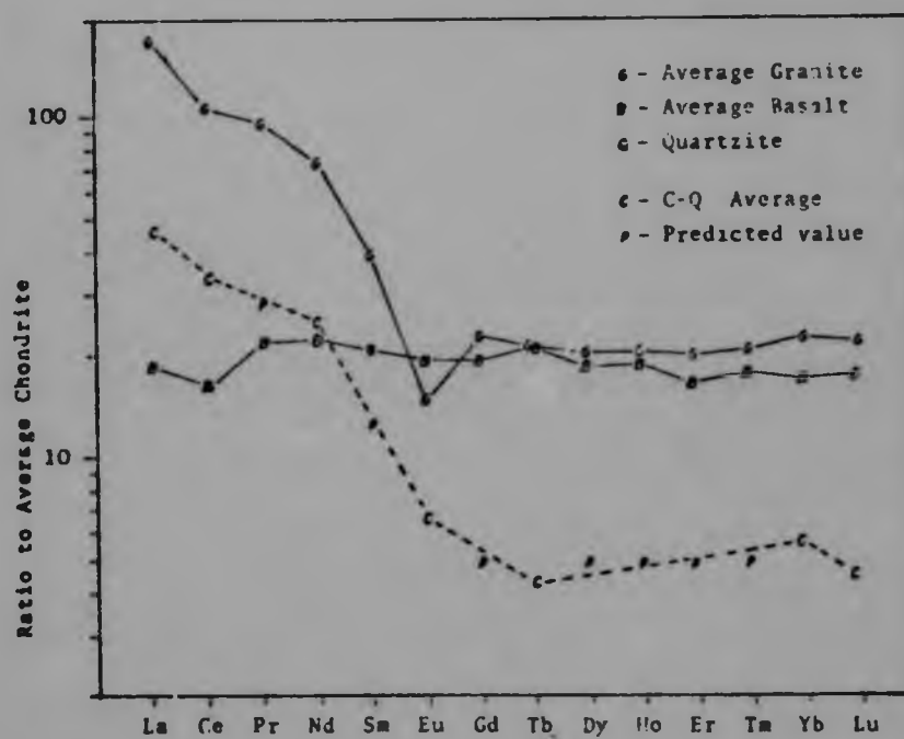
Figure 12.2 RARE EARTH PATTERNS OF AVERAGE ROCK TYPES RELATIVE TO CHONDRITES
