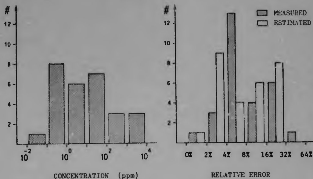
Figure 7.3 FREQUENCY DISTRIBUTION OF ELEMENT CONCENTRATIONS AND ERRORS FOR QUARTZITE SAMPLES
