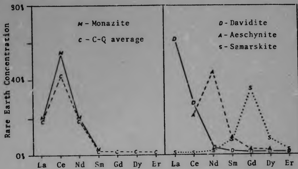
Figure 12.3 DISTRIBUTION OF RARE EARTH ELEMENTS IN SOME RARE EARTH MINERALS (Quoted from He70)
