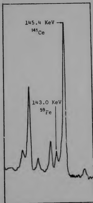
(a) Cerium - Iron Interference
