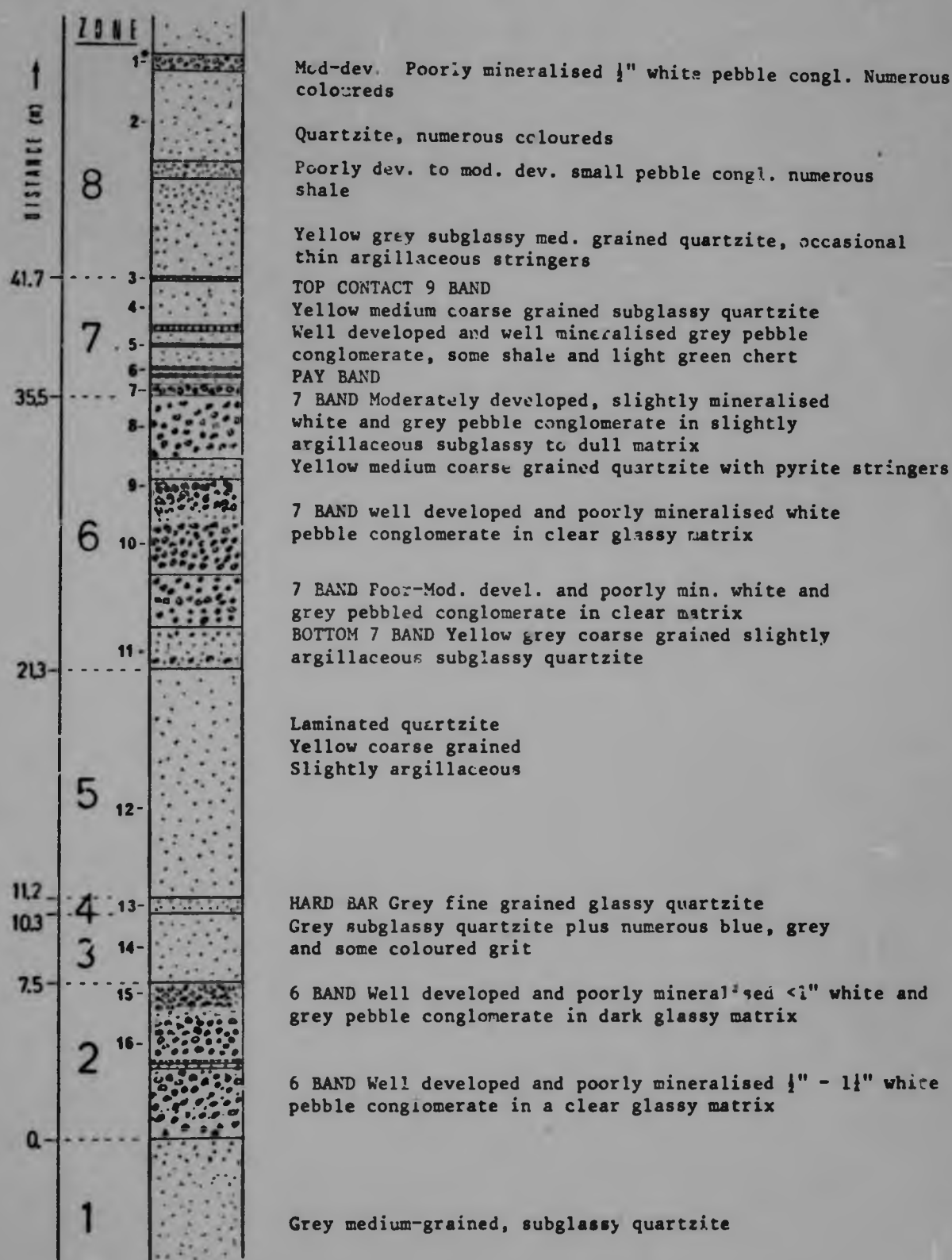
Figure 3.1 DESCRIPTIVE GEOLOGICAL CROSS SECTION OF AREA SAMPLED
