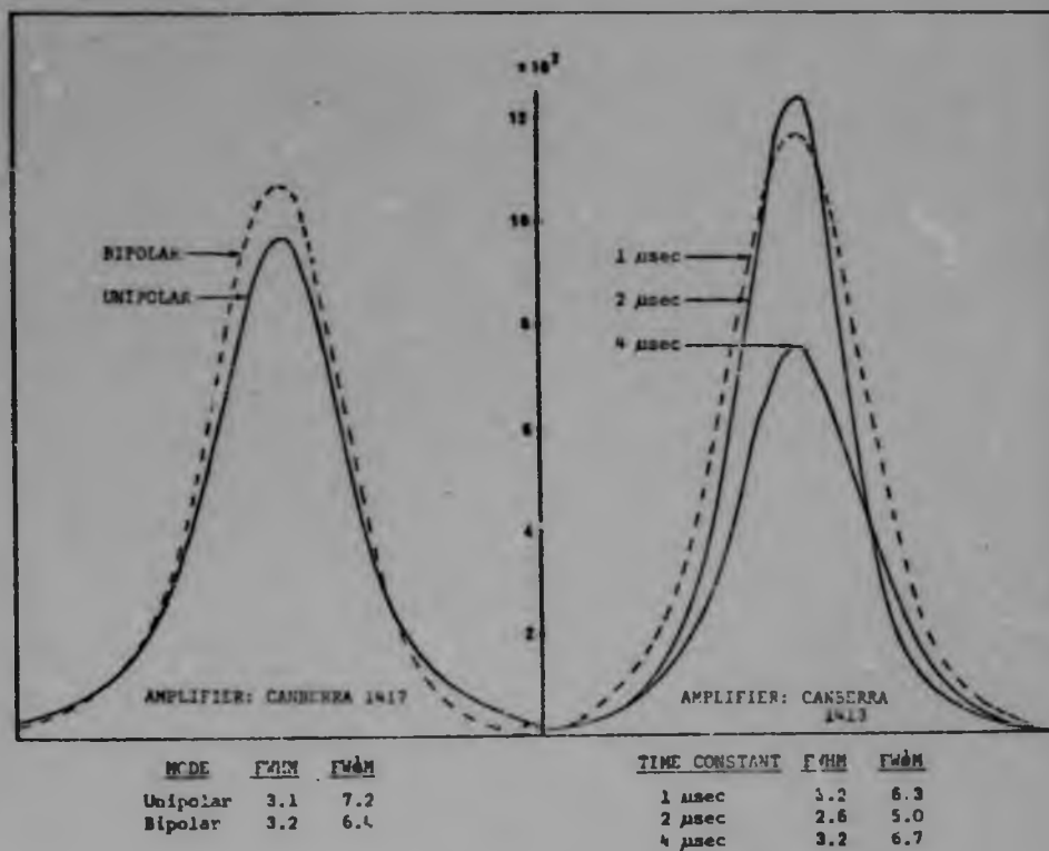
Figure 5.6 Peak Degradation at High Count Rates
