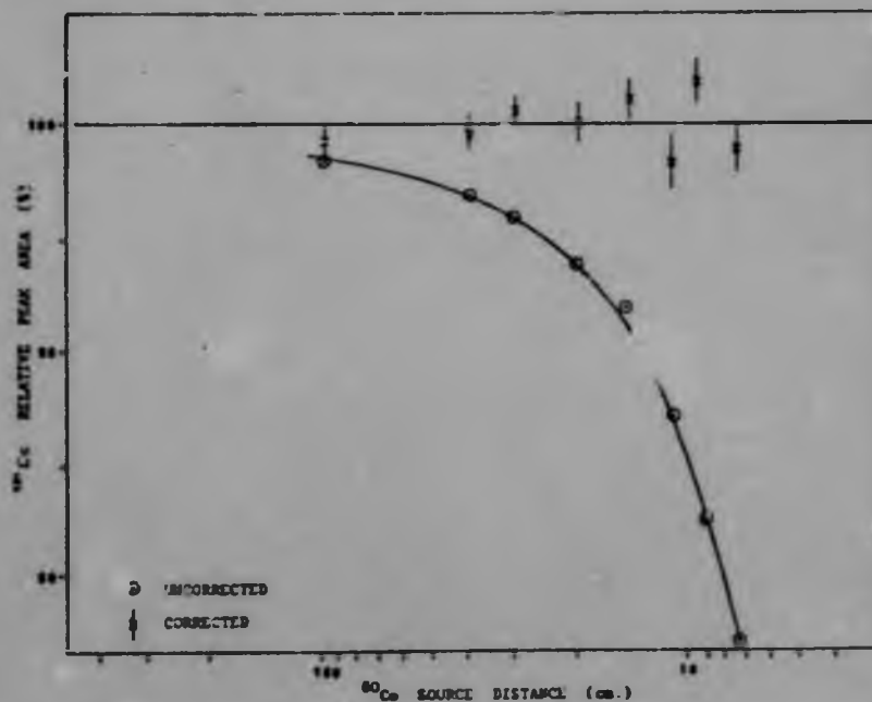
Figure 5.9 DEAD TIME CORRECTION BY PULSER PEAK NORMALISATION
