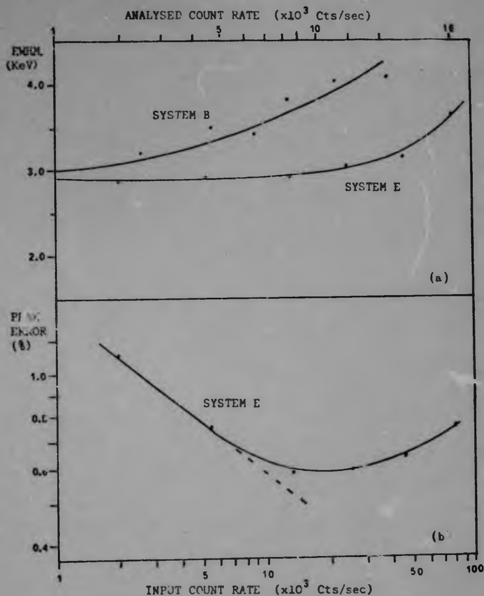
Figure 5.5 COUNT RATE PERFORMANCE OF SYSTEMS B AND E
