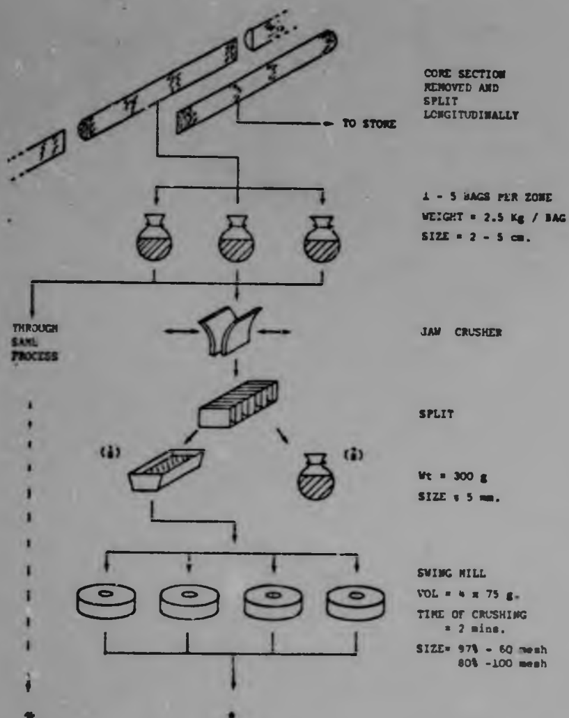
Figure 3.2 FLOW DIAGRAM FOR POWDERED SAMPLE PREPARATION
