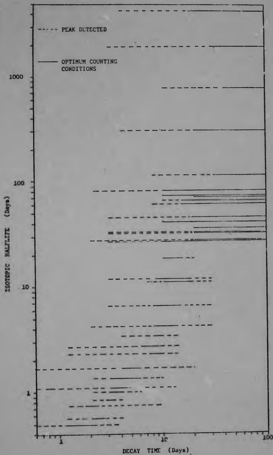
Figure 6.3 OPTIMUM DECAY TIMES
