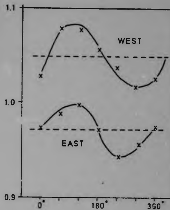
Figure 5.1 NEUTRON FLUX DISTRIBUTION MEASURED USING IRON FOIL MONITORS
