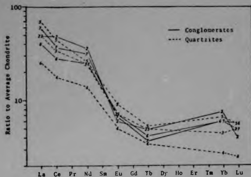
Figure 12.1 RARE EARTH PATTERNS OF EACH ZONE RELATIVE TO CHONDRITES
