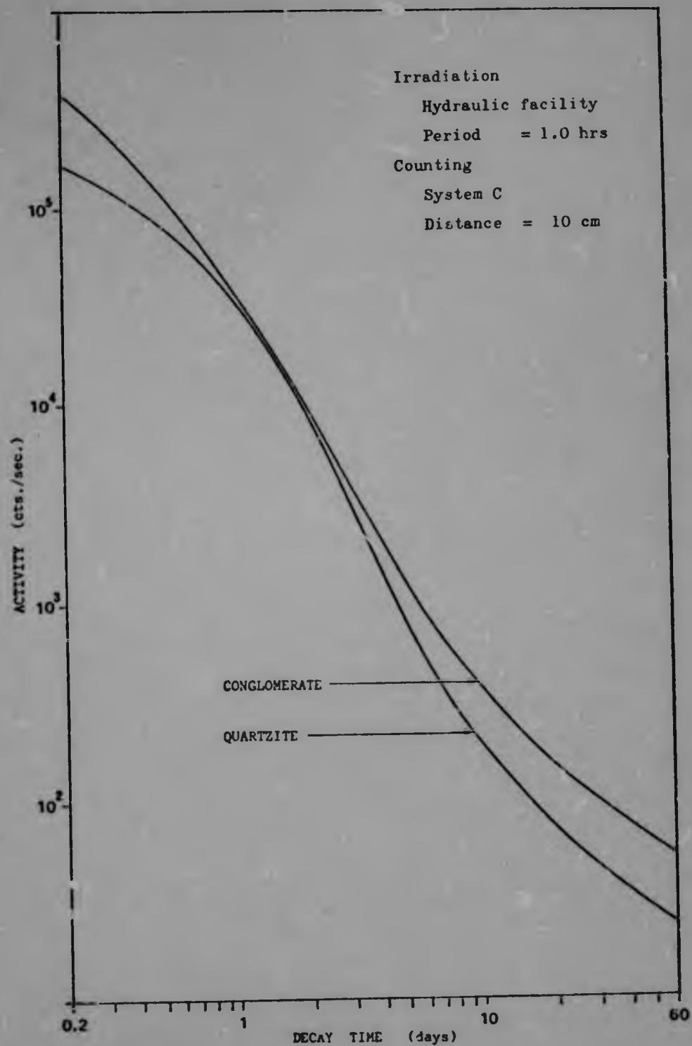
Figure 6.1 TOTAL ACTIVITY DECAY CURVE OF REPRESENTATIVE SAMPLES
