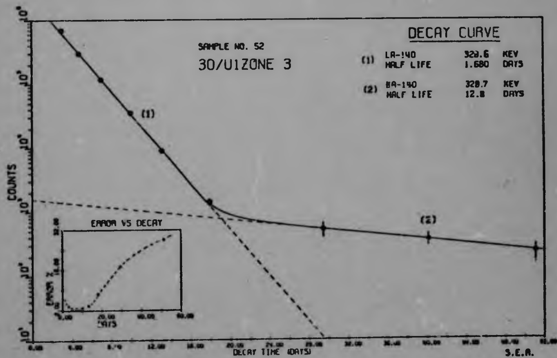
(b) Decay Curve of 328 KeV Peak Showing Interference
