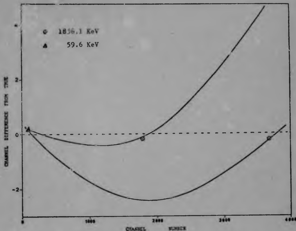
Figure 5.8 DIFFERENTIAL LINEARITY OF SYSTEM C
