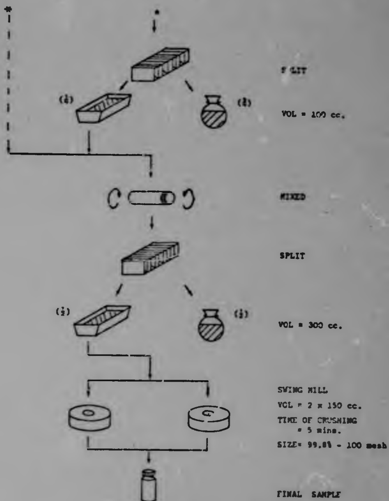
Figure 3.2 FLOW DIAGRAM FOR POWDERED SAMPLE PREPARATION
