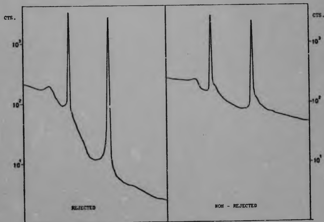
Figure 5.7 Pile-up Rejection Using The Elscint CAV-N-3 Amplifier
