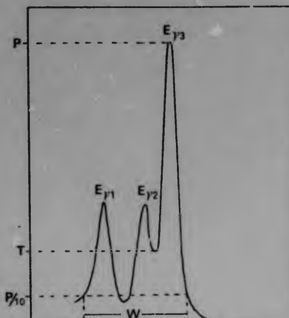
Resolution of the ^{192}\text{Ir} triplet
