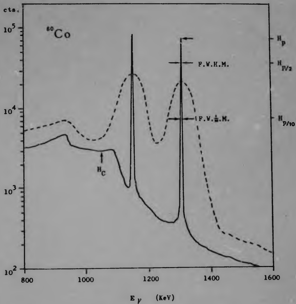
Figure 4.3 COMPARISON OF NaI(Tl) AND Ge(Li) DETECTORS
