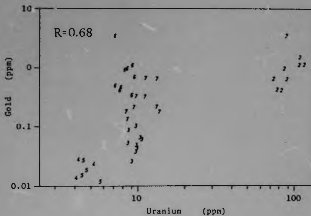
Figure 12.11 SCATTER DIAGRAM OF GOLD AND URANIUM
