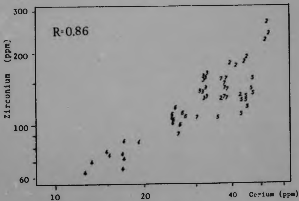
Figure 12.6 SCATTER DIAGRAM OF ZIRCONIUM AND CERIUM
