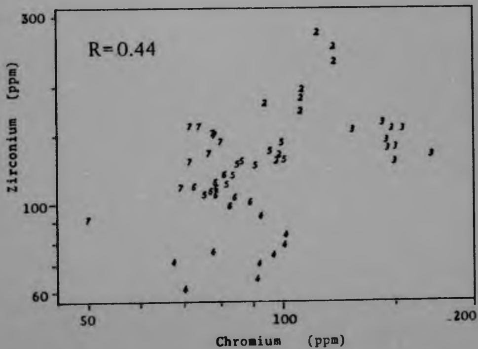
Figure 12.8 SCATTER DIAGRAM OF ZIRCONIUM AND CHROMIUM
