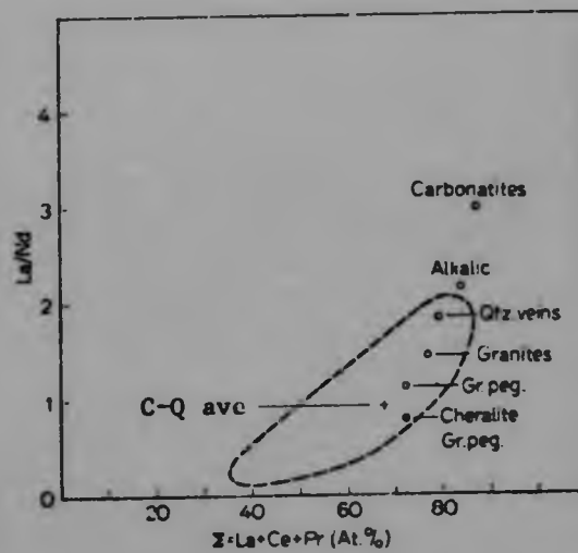
Figure 12.4 DISTRIBUTION OF MONAZITES FROM DIFFERENT PARAGENESES (Quoted from He70)
