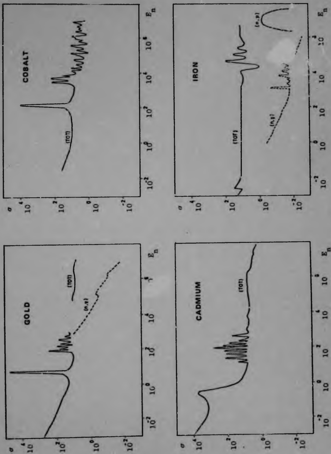
Figure 4.2 NEUTRON EXCITATION FUNCTIONS (ref. S164)
