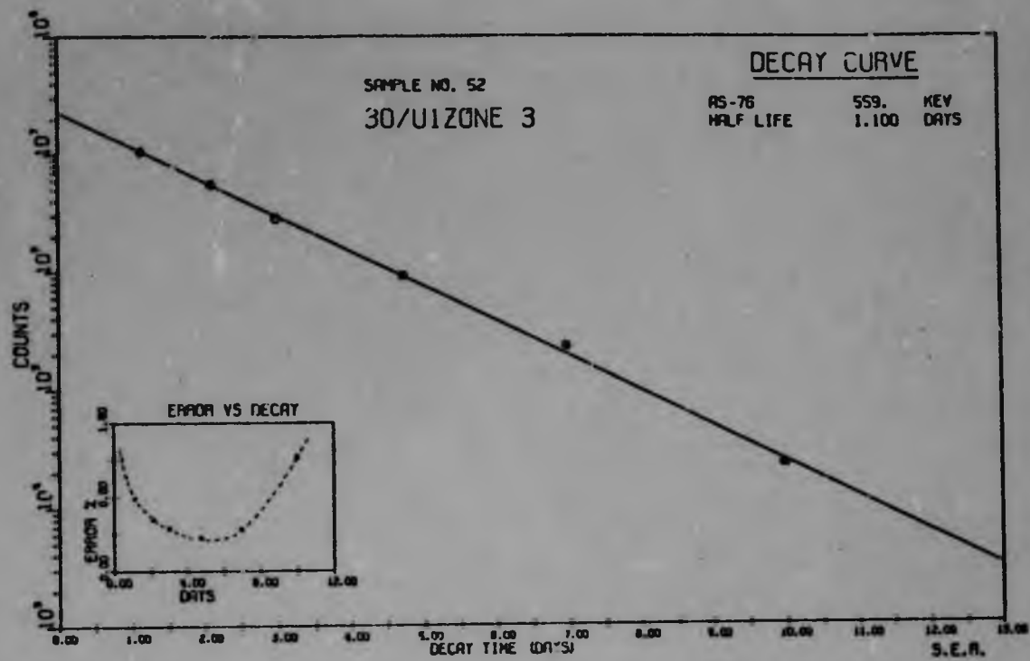
(a) Decay Curve of 559 KeV Peak of ^{76}\text{As}
