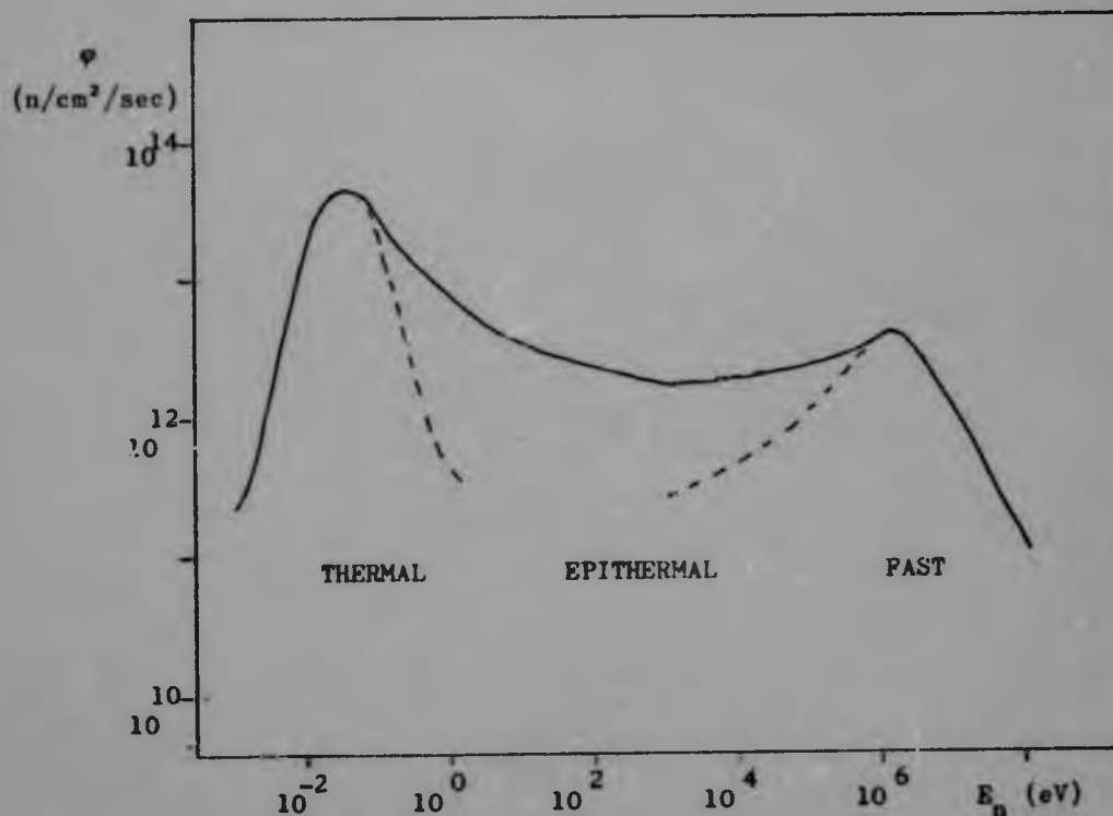
Figure 4.1 TYPICAL REACTOR NEUTRON FLUX DISTRIBUTION
