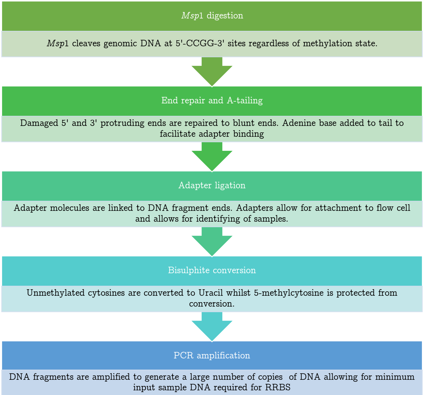
Figure 2. 1: Flow diagram showing step wise RRBS procedure.
