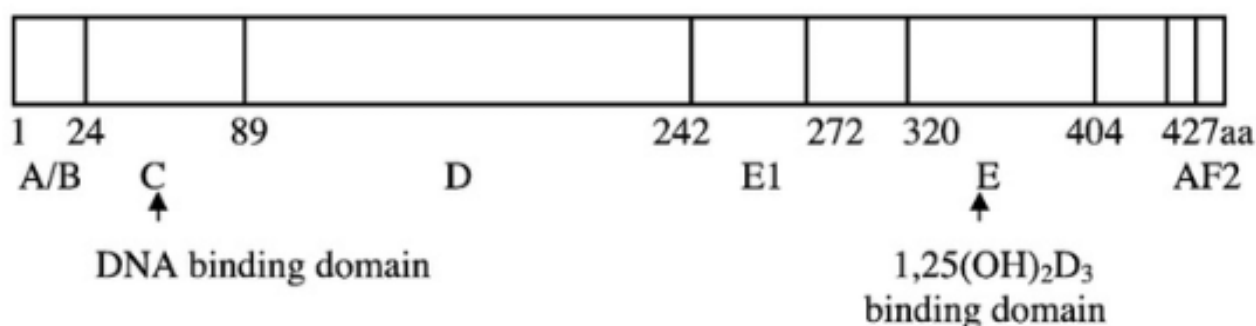
Figure 1. 2: Schematic representation of the domain structure of the VDR protein. The DNA binding domain is found in the N-terminal, while the ligand binding (E) and dimerization (E1) domains are found in the C-terminal. The complete protein is 427 amino acids long. The largest region is the hinge region (D), which spans 153 amino acids (Taken from Ramasamy, 2008).
