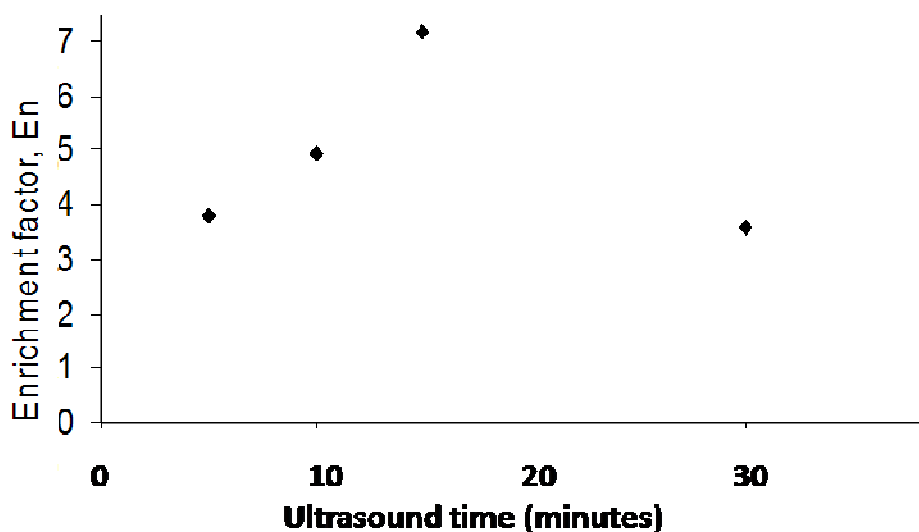
Figure 5.13: The effect of ultrasound on extraction process. A 200 watt equipped with a 4 mm diameter probe was used with probe depth of about 1cm. The whole acceptor phase with 30 mg of MIP was used.
