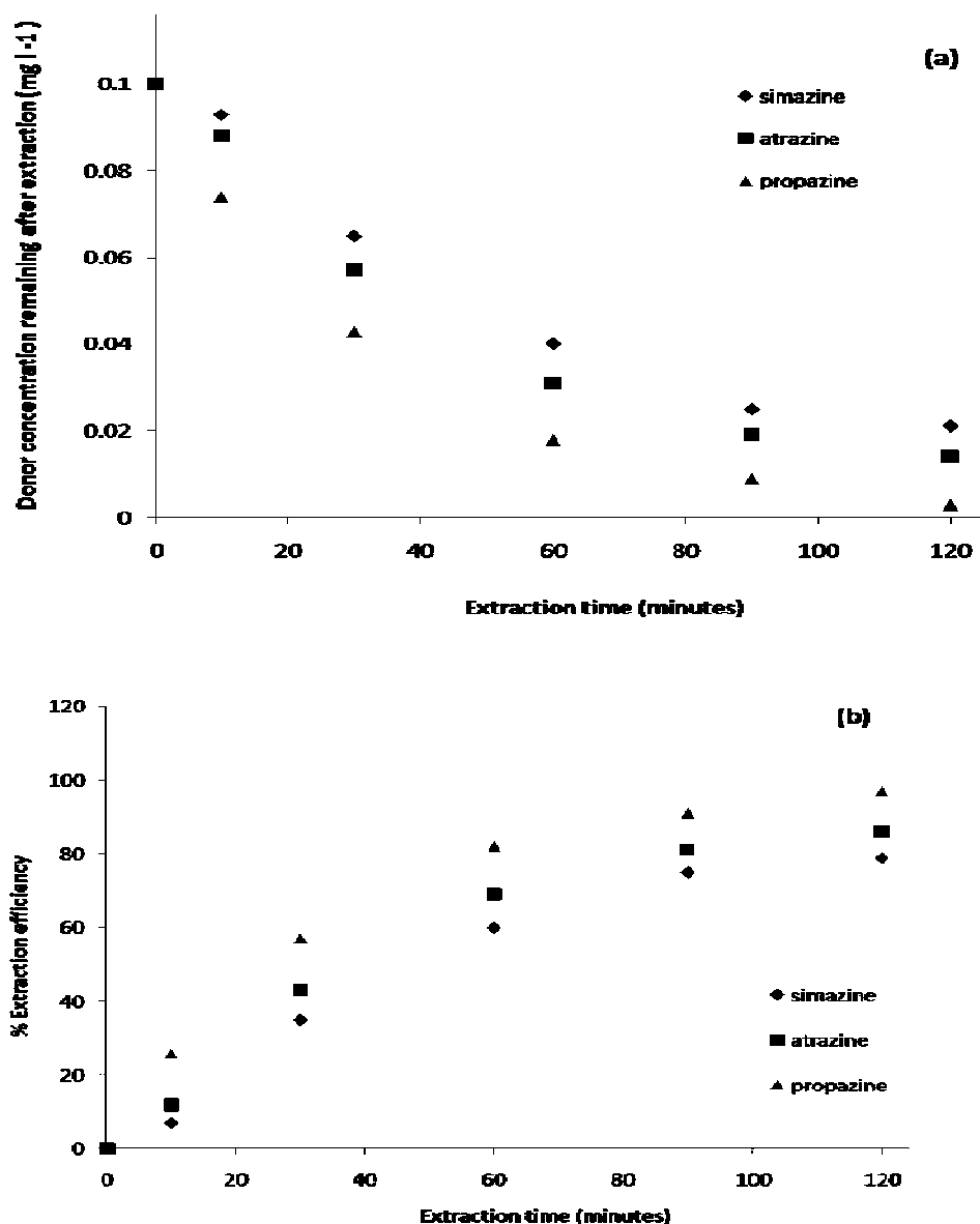
Figure 5.7: Influence of extraction time on the extraction efficiency without MIP particles in the acceptor phase. 0.1 mg l -1 of triazines mixture spiked in deionised water was extracted with 2.5 ml of toluene in the organic acceptor compartment. (a) The donor concentration remaining after extraction. (b) Percent extraction efficiency against extraction time determined from the donor side of the membrane.
