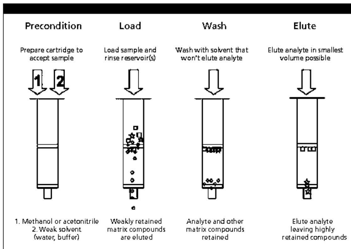
Figure 2.7: Schematic diagram representing the steps involved in solid phase extraction
