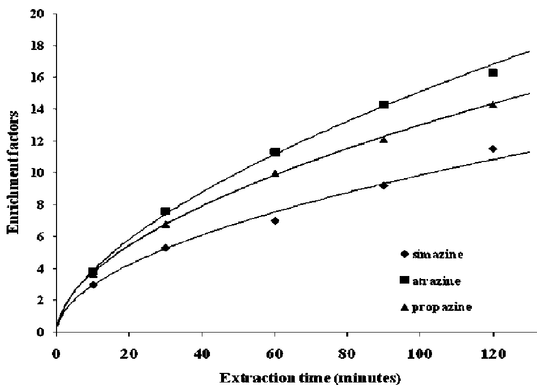
Figure A1: The enrichments factors of triazines plotted against extraction time after desorption from the MIP in the MMLLE – MIP extraction. These enrichments factors were obtained before concentration of the elution solvent (90 % methanol / 10% water). After concentration of the solvent, the enrichments factors were in the region of 40s.
