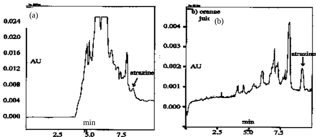
Figure 2.16: Electropherograms of atrazine in orange juice after, (a) SPE only and (b) SLM-SPE extractions. Taken from Khrolenko et al. , (2002).
