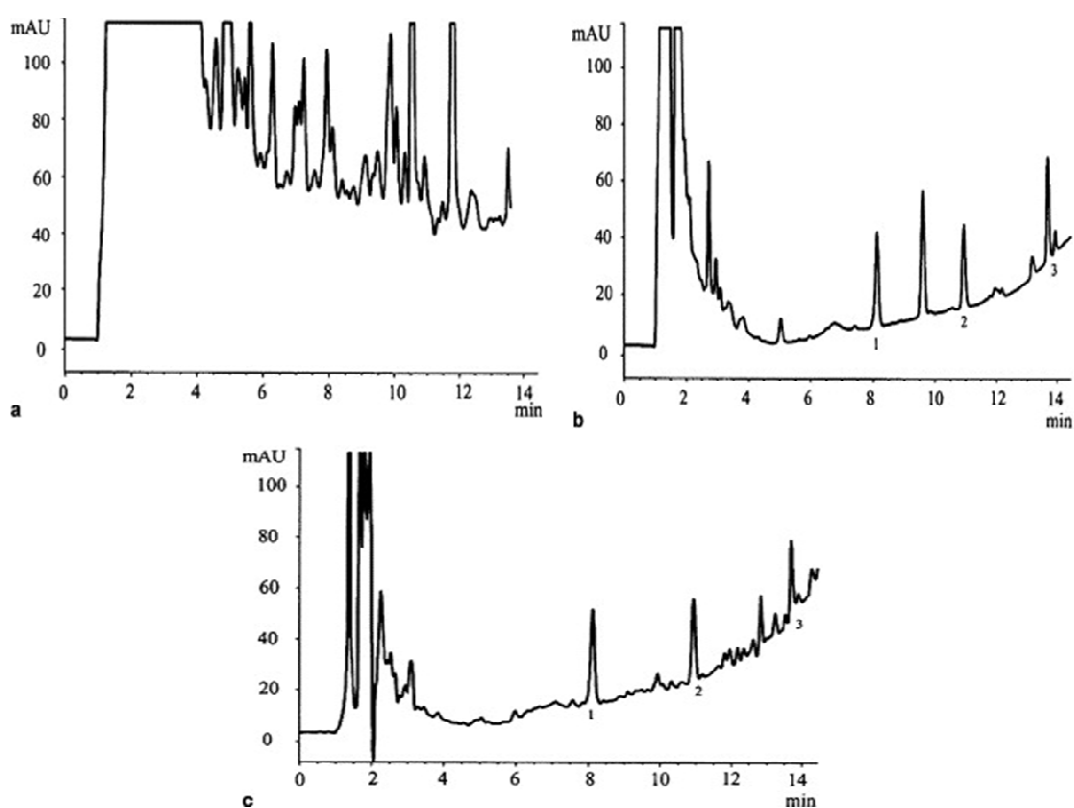
Figure 2.11: Chromatogram obtained after the injection of a soil extract containing 20 \text{ ng g}^{-1} of triazines: (a) without and (b) with a clean-up step on the MIP; and (c) on the anti-triazine immunosorbent. Peak assignment: (1) atrazine; (2) simazine; and (3) terbutylazine (Chapius et al. , 2004).
