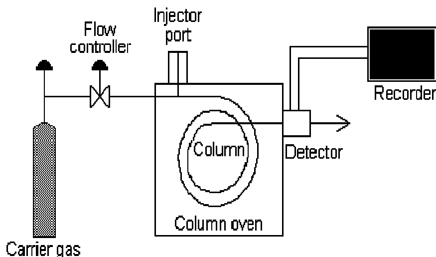
Figure 3.2: A schematic diagram of gas chromatograph (McCarthy, 2001).
