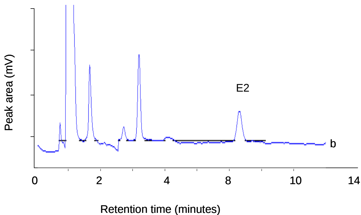
Figure 5.17: Chromatogram obtained after MMLLE extraction of wastewater effluent spiked with 500 \mu\text{g l}^{-1} E2, (a) without MIP particles and (b) with MIP particles in the acceptor. Extraction time was for 60 minutes and 3 ml acetonitrile was used to desorb E2 from the MIP beads.
