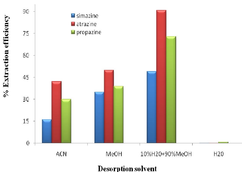
Figure 5.6: Influence of desorption solvent on extraction efficiency. Extraction time was for 60 minutes. 0.1 \text{ mg l}^{-1} of triazine mixture spiked in deionised water was extracted with 10 mg of MIP in the organic acceptor solution (2.5 ml toluene). 2 ml of dichloromethane was used as a washing solution of MIP followed by desorption of the solvents.
