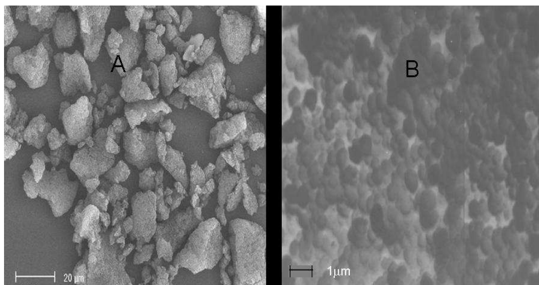
Figure 5.1 (a) represents the morphology of the MIPs prepared using bulk method and (b) represent the morphology of the MIPs prepared by precipitation method (Nemulenzi et al. , 2008).
