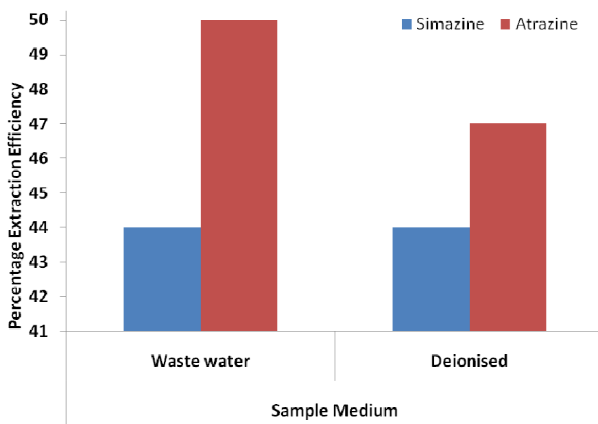
Figure 5.14: The percentage extraction efficiencies obtained when wastewater and deionised water was spiked with 5 \mu\text{g l}^{-1} reference standard was extracted at optimised conditions. Only simazine and atrazine were quantified.
