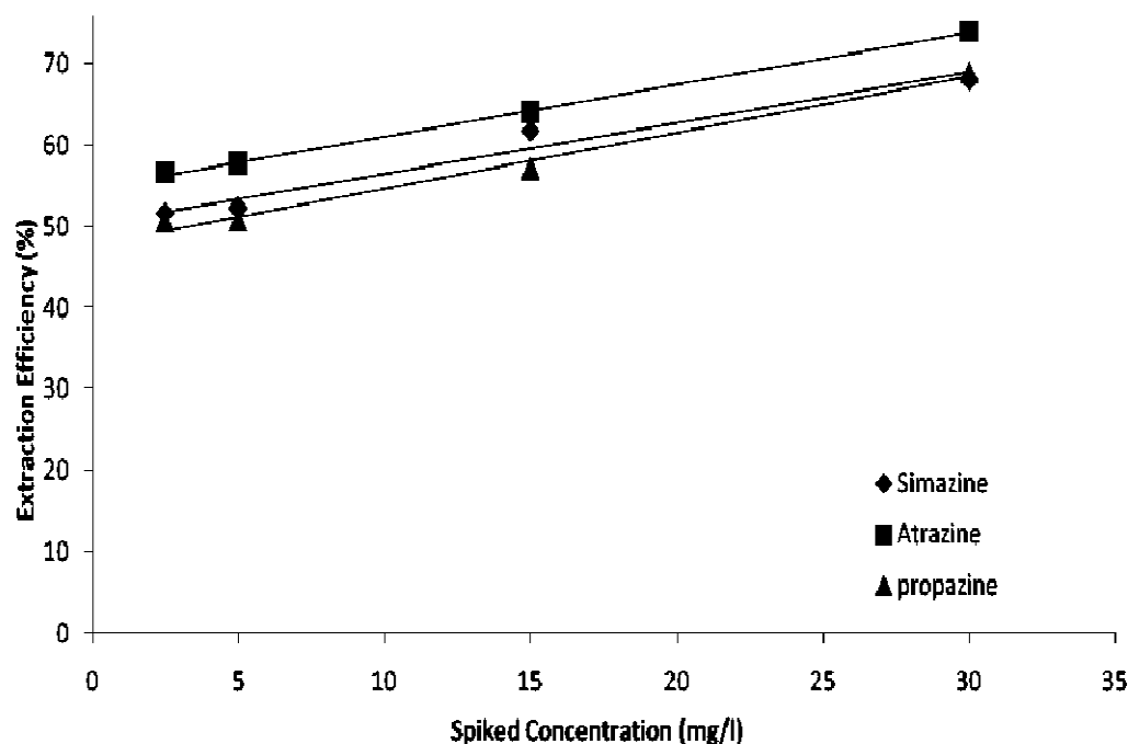
Figure 5.10: The influence of donor concentration on extraction efficiency. n = 3 , average coefficient of variance (CV) across the four concentration studied are; simazine = 8%, atrazine = 5% and for propazine = 7%, see Table 5.4.
