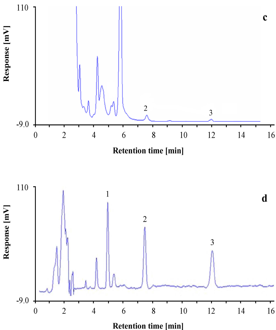
Figure 5.16: Chromatograms obtained after direct injection of apple extract spiked with 100 \mu\text{g l}^{-1} of the triazine mixtures (a), MMLLE extraction of apple extract spiked with 30 \mu\text{g l}^{-1} of the triazine mixture (b), MMLLE-NIP extraction of same apple extract spiked with 30 \mu\text{g l}^{-1} of the triazine mixture (c) MMLLE-MIP extraction of same apple extract spiked with 30 \mu\text{g l}^{-1} of the triazine mixture (d). For experimental conditions, see Figure 5.14.
