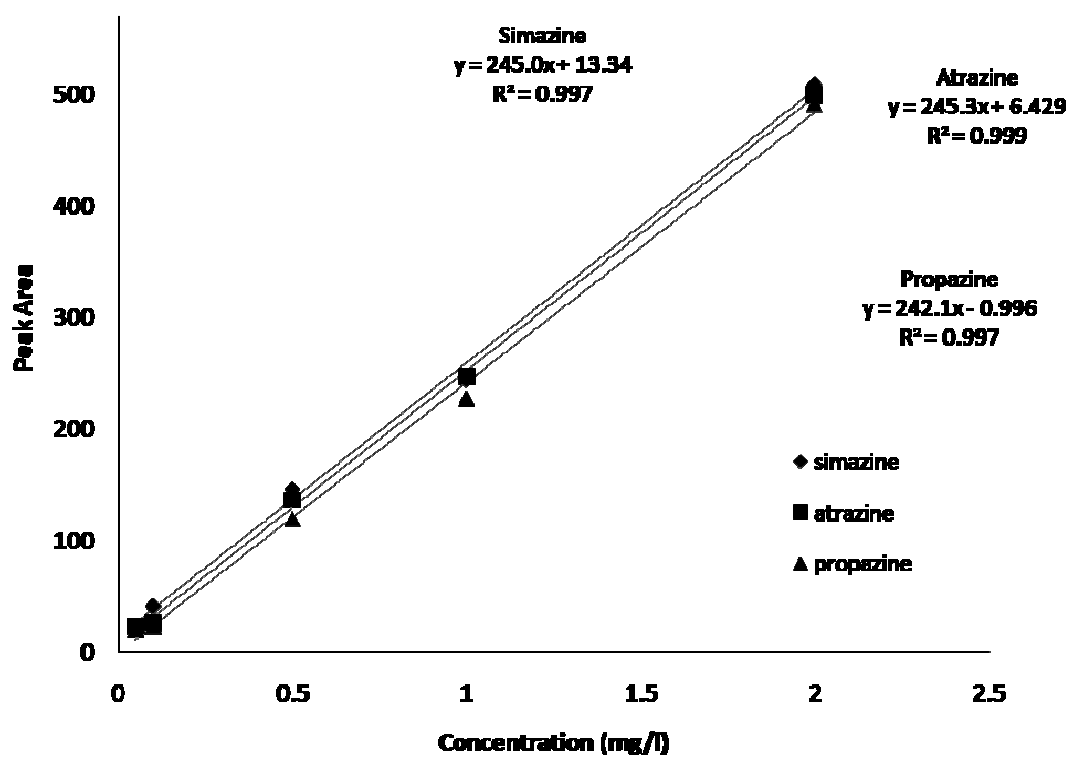
Figure 4.4: A typical calibration curve of triazines.
