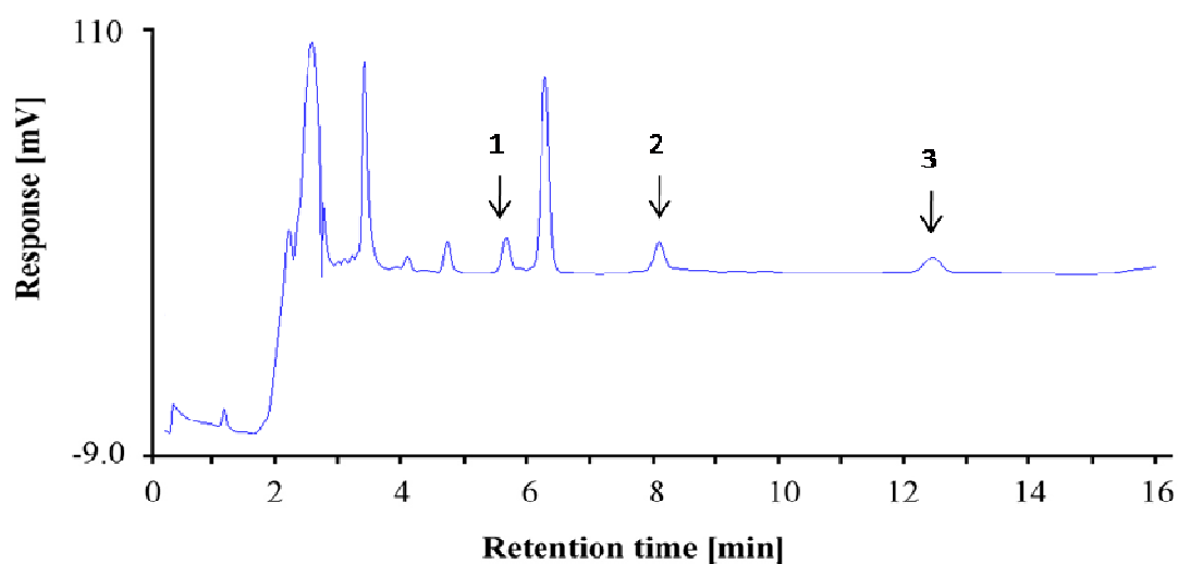
Figure 5.12: Chromatogram obtained following MMLLE – MIP extraction of a sample spiked with 20 \text{ mg l}^{-1} humic substances. The sample was spiked with humic substances and 30 \text{ } \mu\text{g l}^{-1} triazines. Note the absence of a huge peak at the beginning of the chromatogram as in most SPE. 1 = simazine, 2 = atrazine and 3 = propazine.
