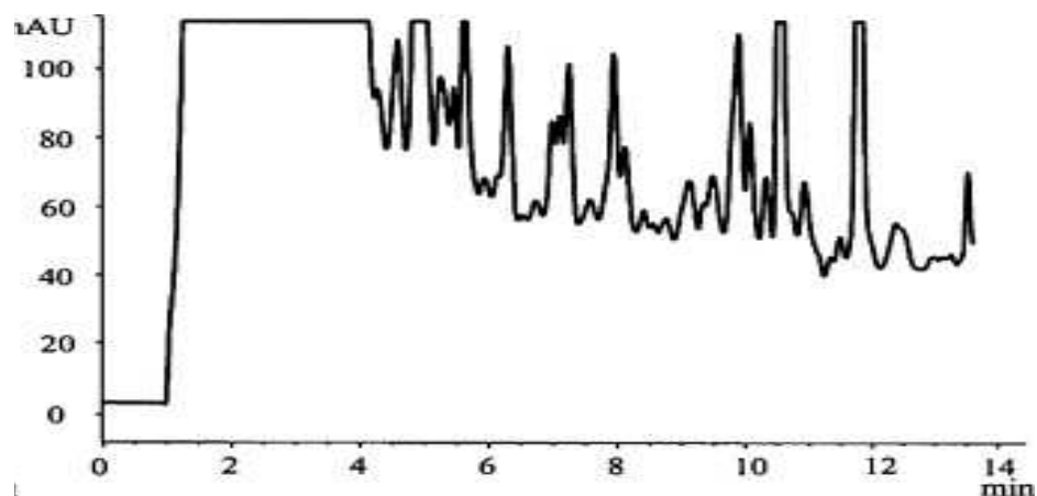
Figure 5.11: Chromatogram obtained after the injection of a soil extract containing 20 \text{ ng g}^{-1} of triazines. Compounds extracted were atrazine, simazine, terbutylazine. Note the huge peak at the beginning of the chromatogram (Chapius et al. , 2004).
