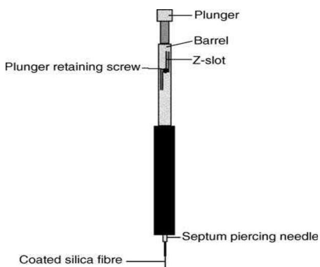
Figure 2.8: Components of SPME
