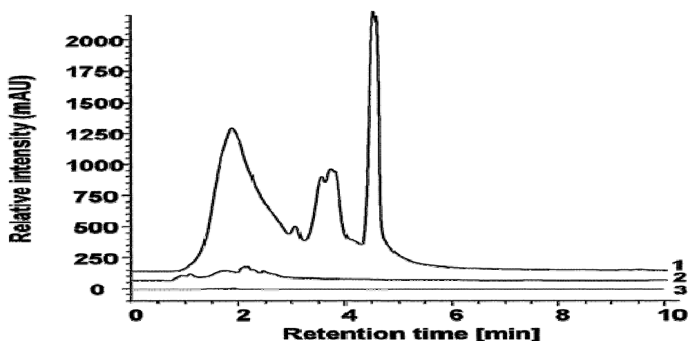
Figure 2.17: The reduction of interfering matrix components (1) HPLC column only, (2) RAM – LC coupling, and (3) RAM – MIP –LC Coupling (Taken from Koeber et al. , 2001).
