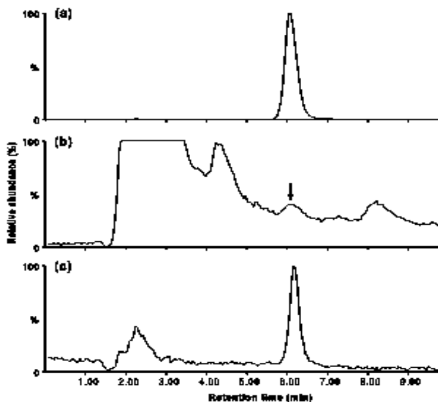
Figure 2.9: Comparison of LC–MS analyses of human serum sample processed by (b) solid-phase extraction, (the melatonin peak indicated by an arrow) and by (c) immunoaffinity purification and (a) LC–MS analysis of melatonin standard (Rolcik et al. , 2002).
