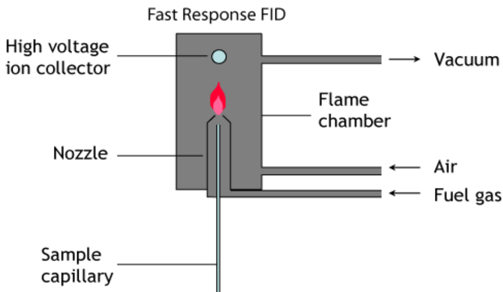
Figure 3.3. Schematic representation of flame ionisation detector (Smith et al. , 2005).
