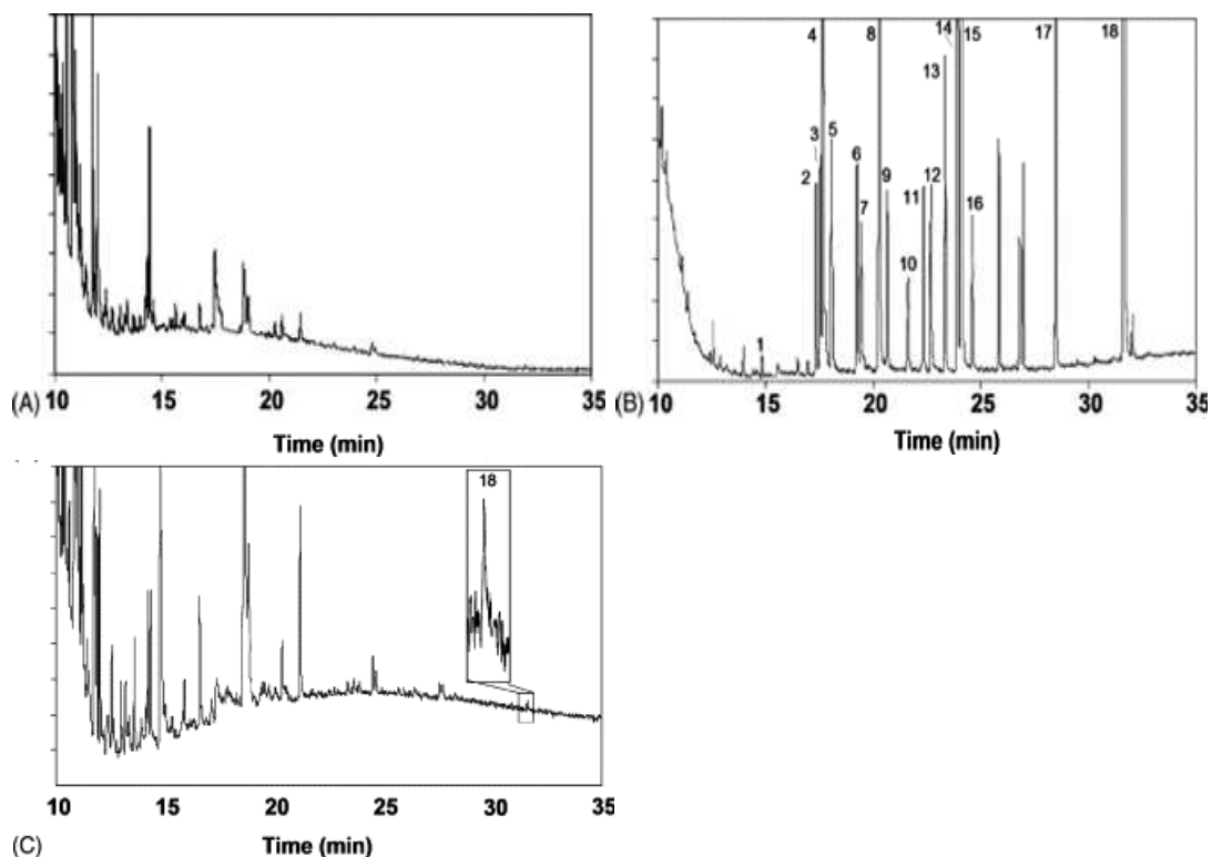
Figure 2.6: MMLLE-GC-FID determination of (A) a blank wine, (B) a MMLLE extract of a spiked red wine sample ( c = 0.05 \text{ mg l}^{-1} ) and (C) a MMLLE extract of an Italian red wine containing tetradifon. Peak identification: 1, aldicarb; 2, diphenylamine (ISTD); 3, simazine; 4, atrazine; 5, lindane; 6, terbuthylazine; 7, metoxuron; 8, metobromuron; 9, vinclozolin; 10, isoproturon; 11, chlortoluron; 12, metazachlor; 13, quinalphos; 14, procymidone; 15, endosulfan I; 16, endosulfan II; 17, endosulfan sulfate; 18, tetradifon (Hyötyläinen et al. , 2002).
