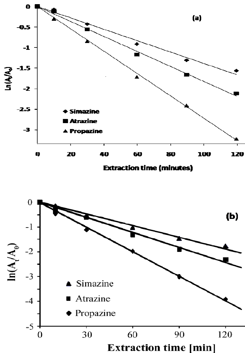
Figure 5.9: Relative triazine concentration in the donor compartment as a function of extraction time. 0.1 mg l -1 of triazine mixture spiked in deionised water was extracted, (a) with 2.5 ml of the acceptor solution and (b) with 10 mg of MIP plus organic acceptor solution (2.5 ml toluene). 2 ml of dichloromethane was used as a washing solution of MIP followed by desorption with 90% methanol in water.
