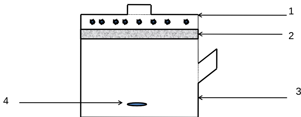
Figure 4.1: Schematic set-up of the extraction unit. 1=Acceptor compartment filled with 2.5 ml of the acceptor solution and the MIP (represented as black dots) (10 mg for triazine extraction and 30 mg for E2 extraction), 2 = PTFE membrane soaked with acceptor solution, 3 = Donor compartment with filled with 23 ml of aqueous sample, 4 = magnetic stirrer.
