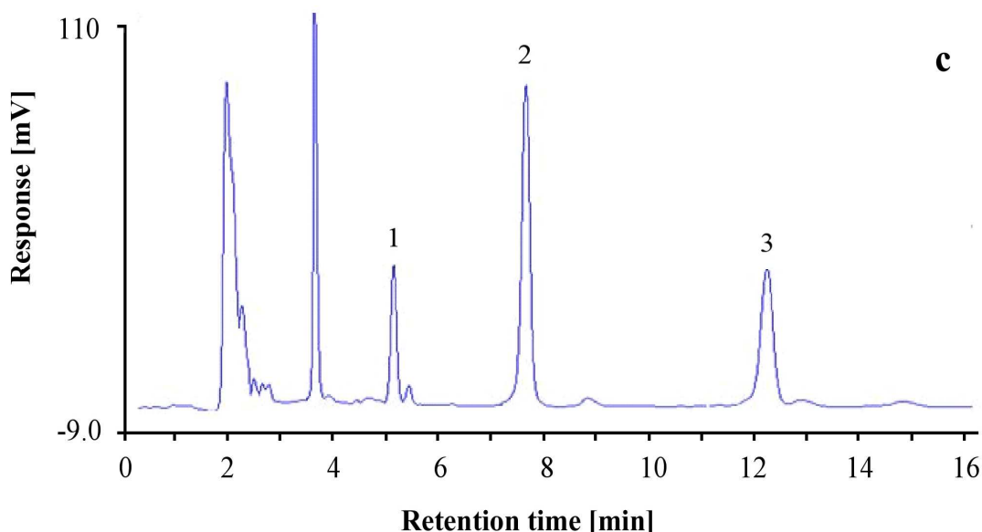
Figure 5.15: Chromatograms obtained after direct injection of lettuce extract spiked with 100 \mu\text{g l}^{-1} of the triazine mixture (a), MMLLE extraction of lettuce extract spiked with 30 \mu\text{g l}^{-1} of the triazine mixture (b), MMLLE-MIP extraction of same vegetable extract spiked with 30 \mu\text{g l}^{-1} of the triazine mixture (c). Experiments performed under optimised conditions of 10 mg of MIP in toluene as part of the acceptor solution, 2 ml of dichloromethane as a washing solution of MIP followed by desorption with 90% methanol in water. Extraction time was for 90 minutes. 1 = simazine, 2 = atrazine, 3 = propazine
