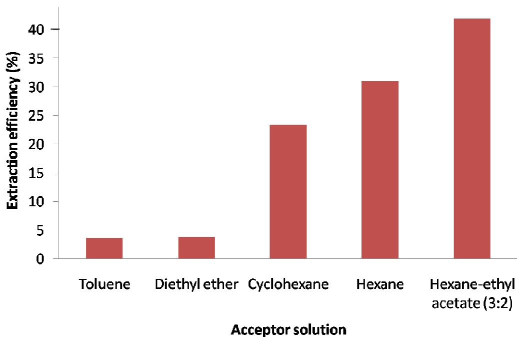
Figure 5.5: Varying organic solvent in liquid-liquid extraction. 100 ml of deionised spiked with 1 \text{ mg l}^{-1} of E2 was extracted with 20 ml of the organic acceptor.
