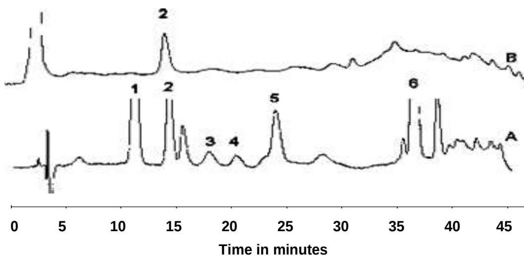
Figure 2.5: Standards mixture of compounds (A) and corresponding circulating nutrient sample solution after SLM extraction (B). (1) p-hydroxybenzoic acid, (2) vanillic acid, (3) salicylic acid, (4) benzoic acid, (5) ferulic acid, and (6) phenazine-1-carboxylic acid (Jung et al. , (2002).
