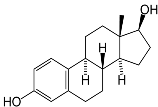
Figure 2.2: The structure of 17 \beta -estradiol (E2)
