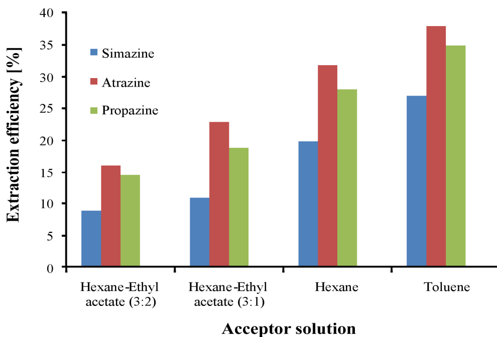
Figure 5.4: Influence of acceptor solution on extraction efficiency. Extraction time was for 60 minutes and 1 \text{ mg l}^{-1} of triazine mixture spiked in deionised water was extracted with 7 mg of MIP in the organic acceptor solution. 2 ml of hexane – ethyl acetate (3:2) was used as a washing solution of the MIP followed by 3 ml of methanol as desorption solvent.
