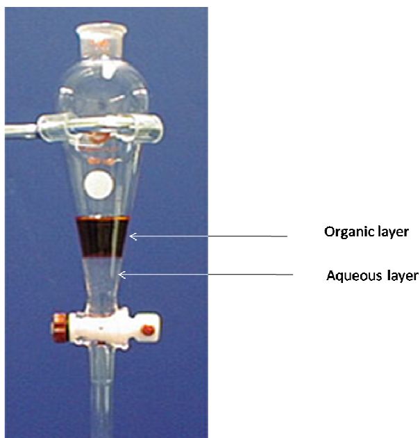
Figure 2.3: Apparatus used in conventional liquid -liquid extraction.
