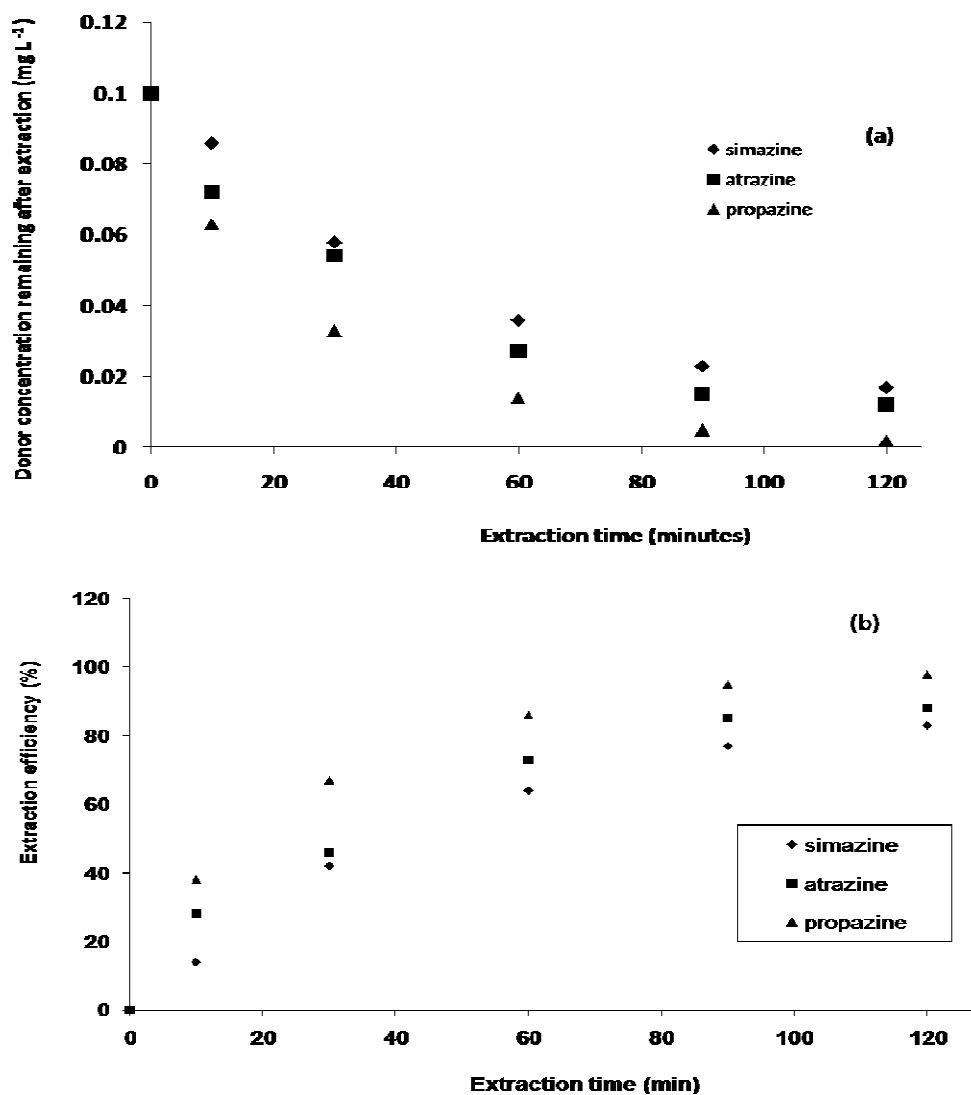
Figure 5.8: Influence of extraction time on extraction efficiency. 0.1 mg l -1 of triazine mixture spiked in deionised water was extracted with 10 mg of MIP in the organic acceptor solution (2.5 ml toluene). 2 ml of dichloromethane was used as a washing solution of MIP followed by desorption with 90% methanol in water. The extraction efficiency was monitored from the donor side of the membrane (see equation 4.3). (a) The donor concentration remaining after extraction, (b) percent extraction efficiency against extraction time determined from the donor side of the membrane.
