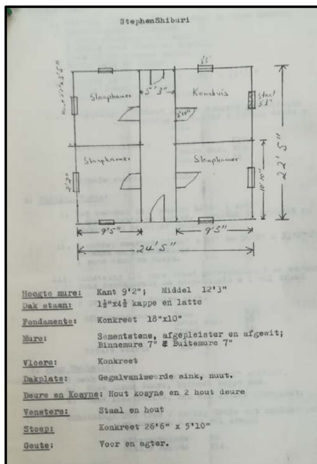
Figure 18: Plan of Mamelete Location home drafted by the Agricultural Official of the Potgietersrus Bantu Affairs Commissioner detailing the components to be pulled apart. 351
