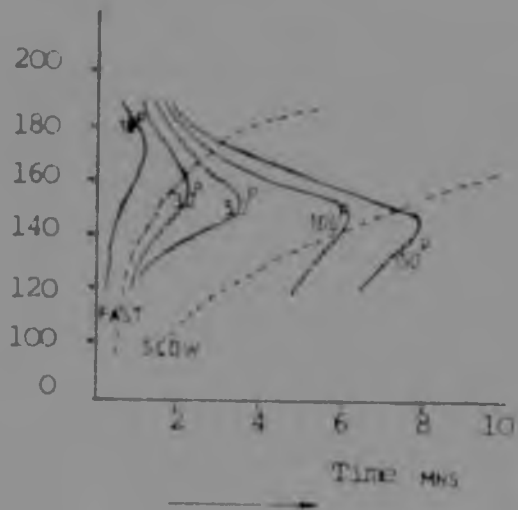
Figure 1 Trace from differential scanning calorimeter. Temp ° C'
