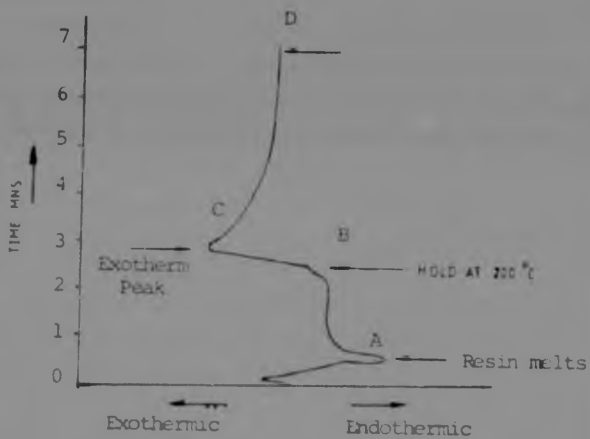
Figure 1 Trace from differential scanning calorimeter. Temp ° C'
