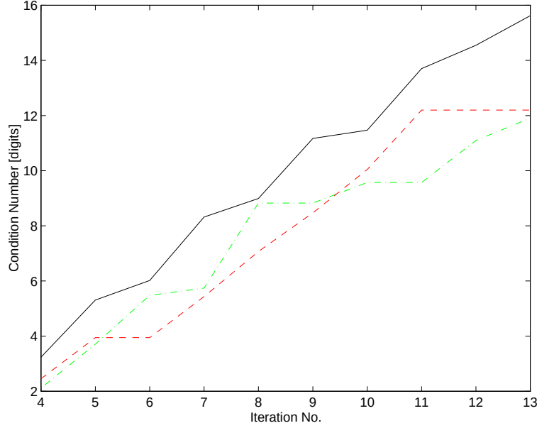
Figure 8.12: The condition number expressed in digits of the helicopter input impedance FMs 1,2 and 3, plotted as a function of iteration number.
