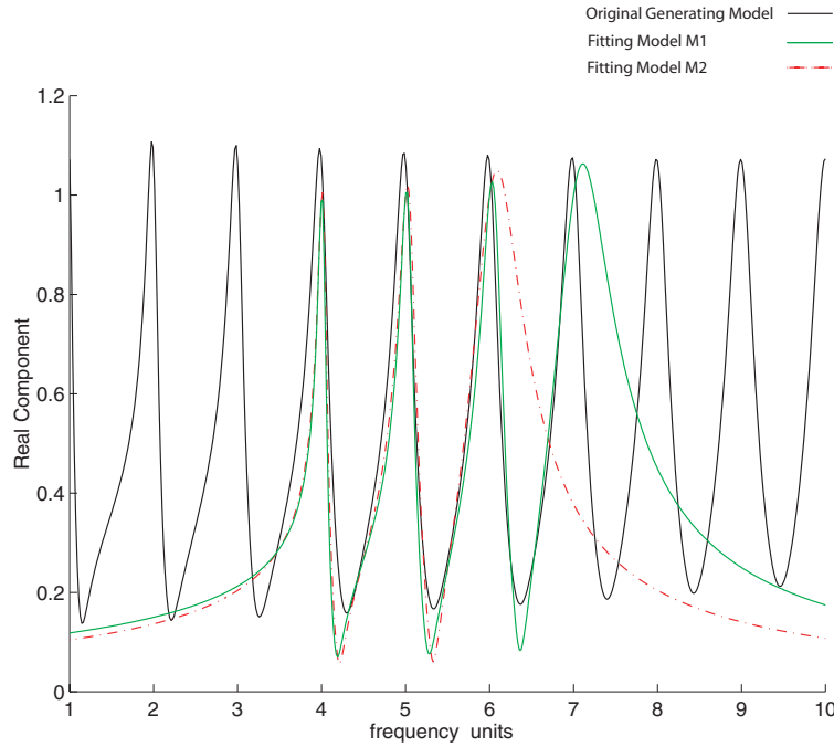
Figure 7.4: The original GM with continuous fitting models M_1 and M_2 superimposed
