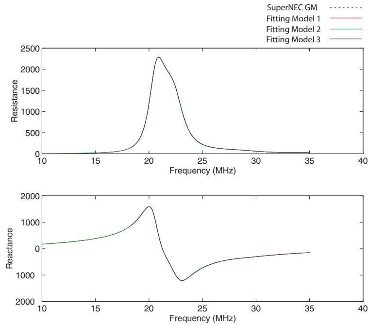
Figure 8.11: An attack helicopter segmented at 25 MHz. TFE applied over the range 10-35 MHz: Iteration no. 13.
