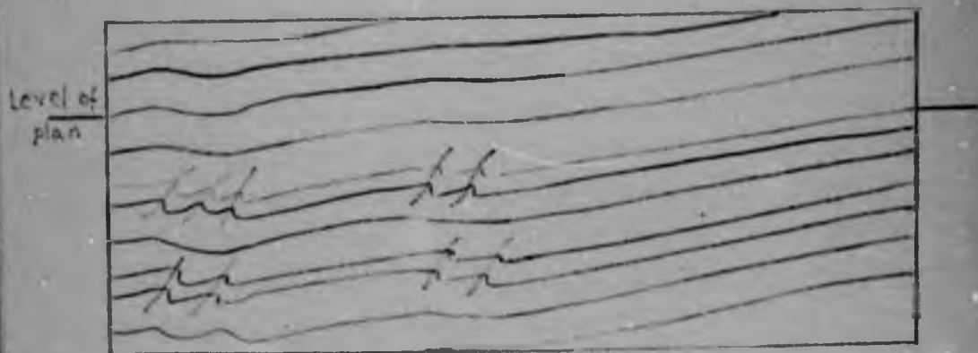
Section Through A-B Illustrating Differential Folding In The Pod-Shaped Structures.
