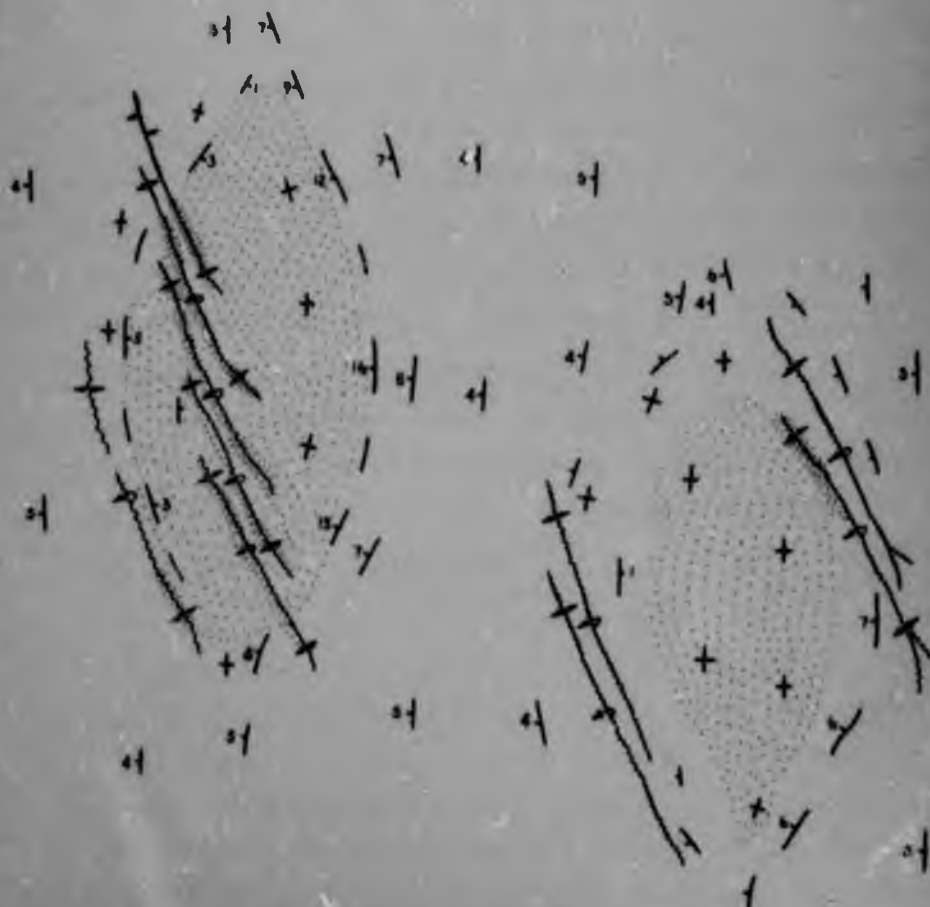
SCHEMATIC PLAN OF LEFT HAND EN ECHELON "POD"-SHAPED FOLDS WITH CROSS-CUTTING FLEXURES AND CROCIDOLITE CONCENTRATIONS
