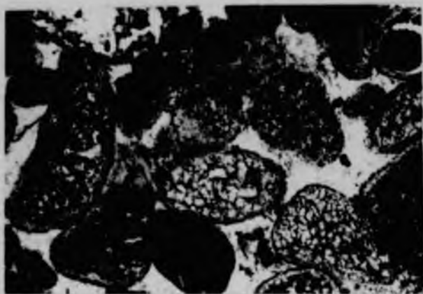
Figure 25. Unweathered Main Magnetite Chert Marker, containing oolites composed of magnetite, magnetite-chert and chert-carbonate with stilpnomelane-chert-carbonate rims set in a chert matrix. Ordinary light, X 37 \frac{1}{2} - Ettrick Mine - Near Kuruman.
