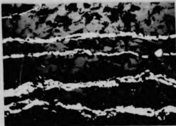
Figure 14. Micrograph showing magnetite bands (white) set in mass fibre (light grey). Crocidolite (medium to dark grey) formed on some magnetite bands only. Polished section, Ordinary light, X 37 1/2. 7 Level, Bretby Mine.
