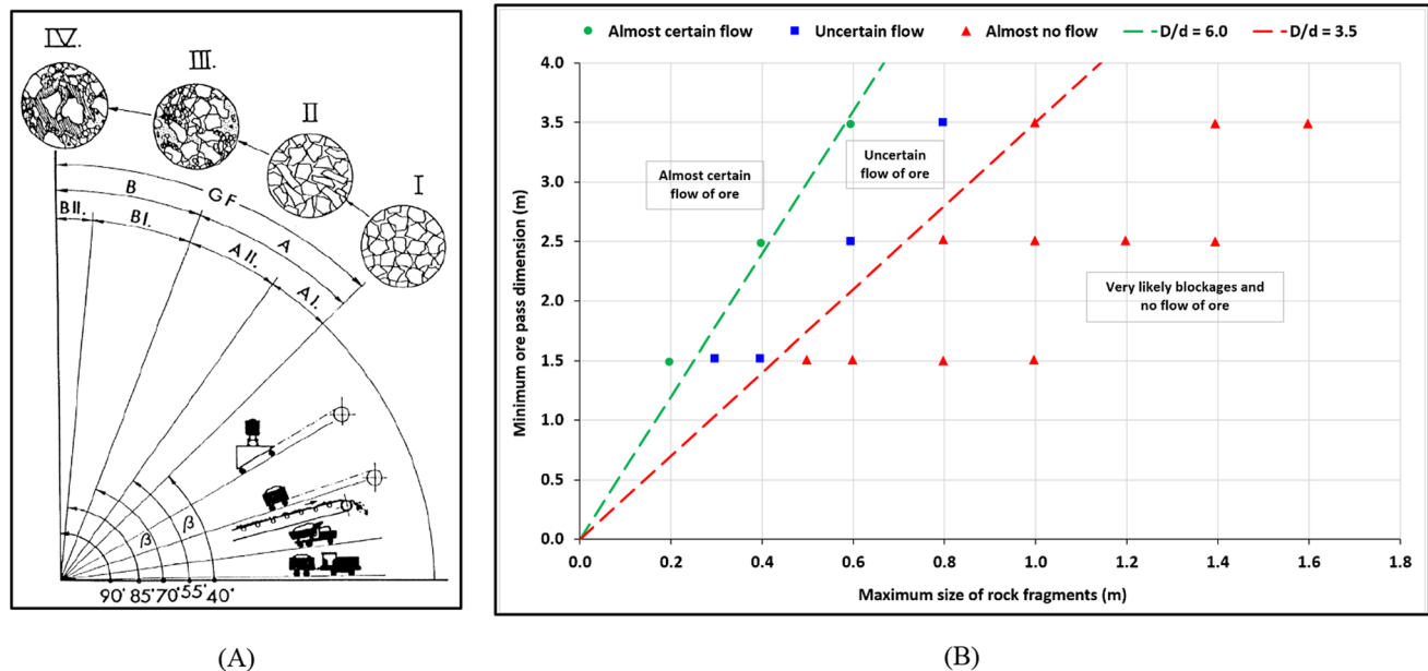
Fig. 7 A Different classes of material and their mobility as a function of ore pass inclination (Kvapil 1998), and B example of numerical modelling results for muck flow in ore passes with a 65° inclination (data collected from Turcotte 2004)
