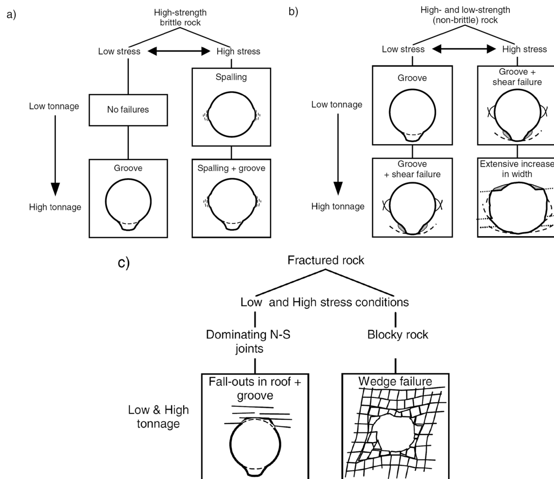
Fig. 2 Failure modes categorized based on governing factors ( a —high-strength, brittle rock conditions, b —non-brittle rock conditions, c —fractured rock conditions) [adopted from Sjöberg et al. (2003) with permission from the authors and publisher]
