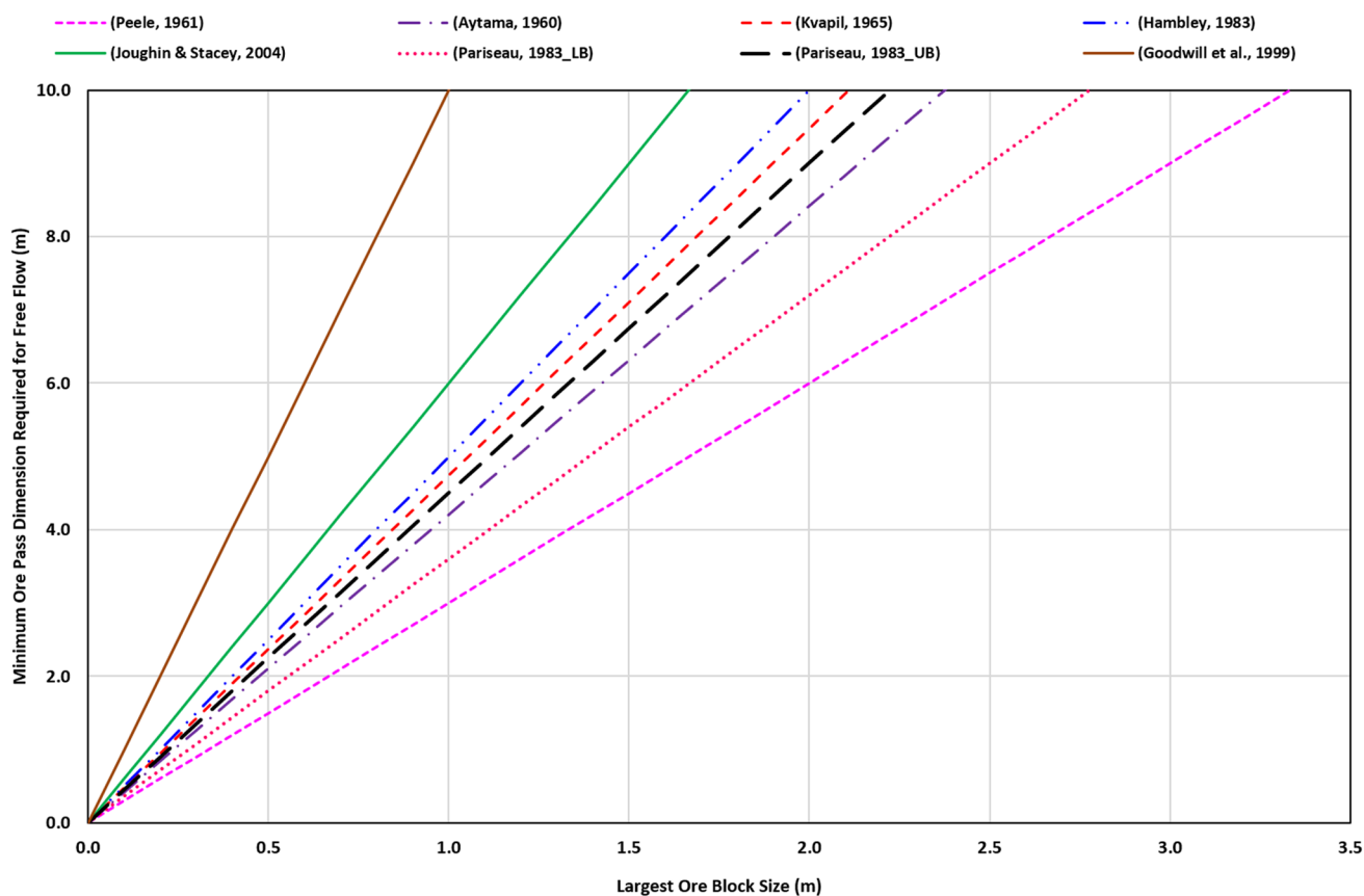
Fig. 16 Guidelines to ensure free flows from past literature (adopted and modified from Hadjigeorgiou and Lessard 2007)
