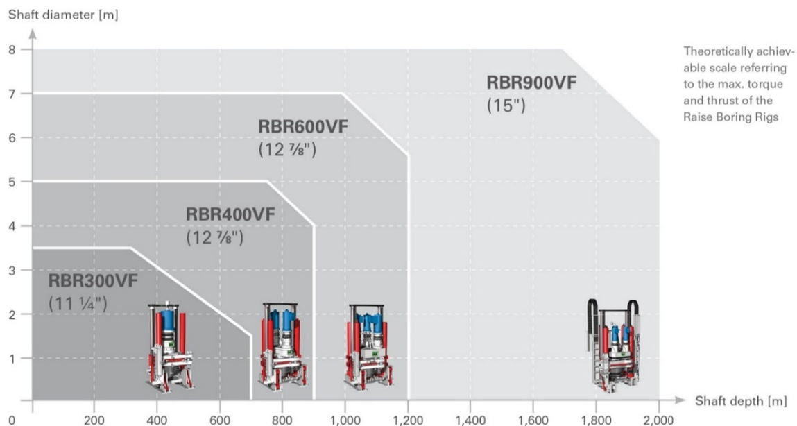
Fig. 11 Example of Herrenknecht Raise Boring Rigs capabilities (Küstle and Frey 2014)
