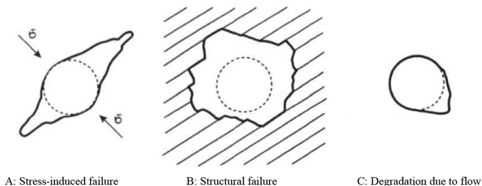
Fig. 14 Schematic view of the main modes of failure in ore passes (adopted from Esmaili (2010) with permission from the author)
