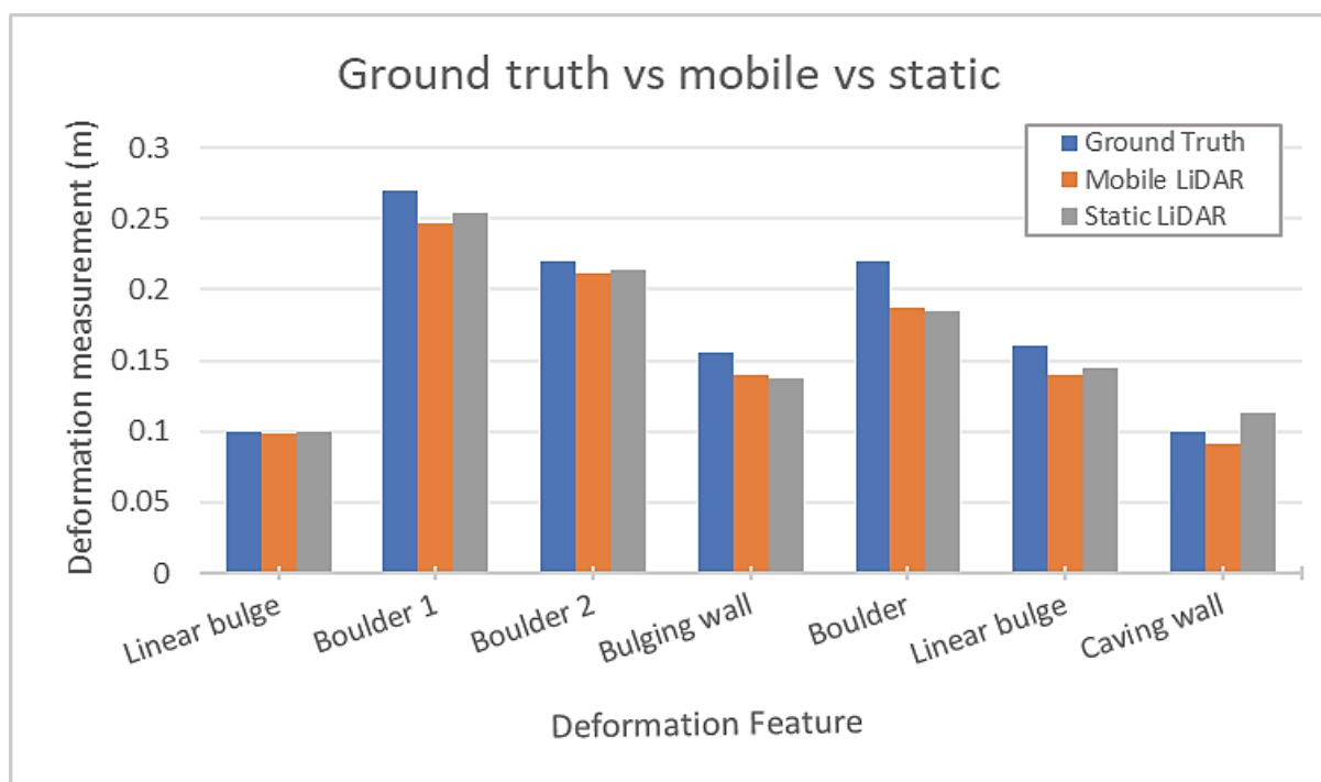
Figure 27: Comparison of deformation measurements computed from the LiDARs tested against the ground truth measurements.
