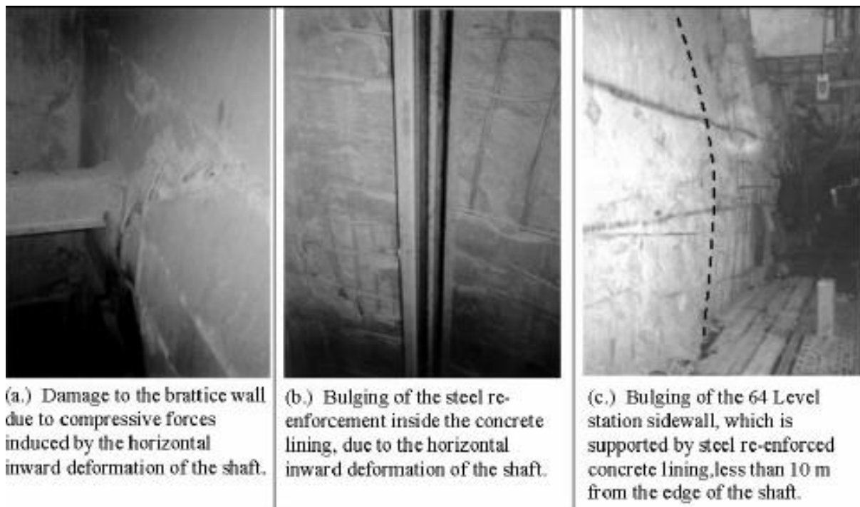
Figure 5: Observed damage to the brattice wall, shaft concrete lining and the sidewall of the 64 Level station (Judeel, 2003).
