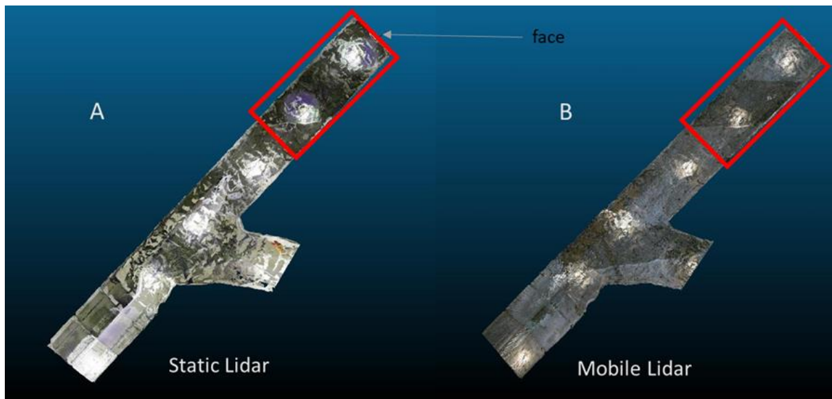
Figure 20: Static and mobile LiDAR point cloud model of the tunnel, with the red block showing the segmented section along the tunnel where the analysis occurred.
