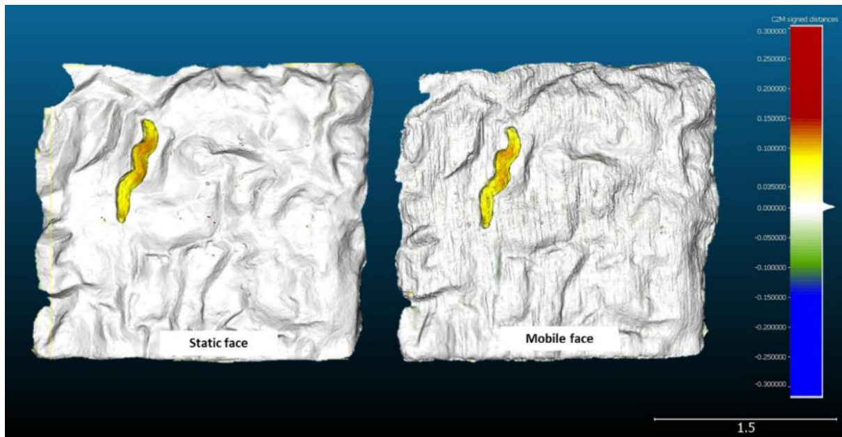
Figure 26: Contrast of static and mobile LiDAR face segments, presenting localised deformation. The deformation analysis of the tunnel face (Figure 26), as shown in the static and mobile LiDAR scans, highlights a localised deformation zone. Both scans display a consistent pattern of deformation, represented by the yellow region in the centre of the tunnel face, corresponding to positive displacement or outward deformation. This suggests bulging in this specific area.
