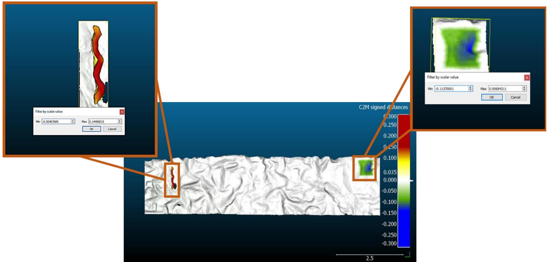
Figure 24: Computation of maximum/minimum deformation distance from detected areas of deformation using statistical computation function. Deformation areas are colour-coded, with warm colours indicating outward deformation and cool colours showing inward deformation.
