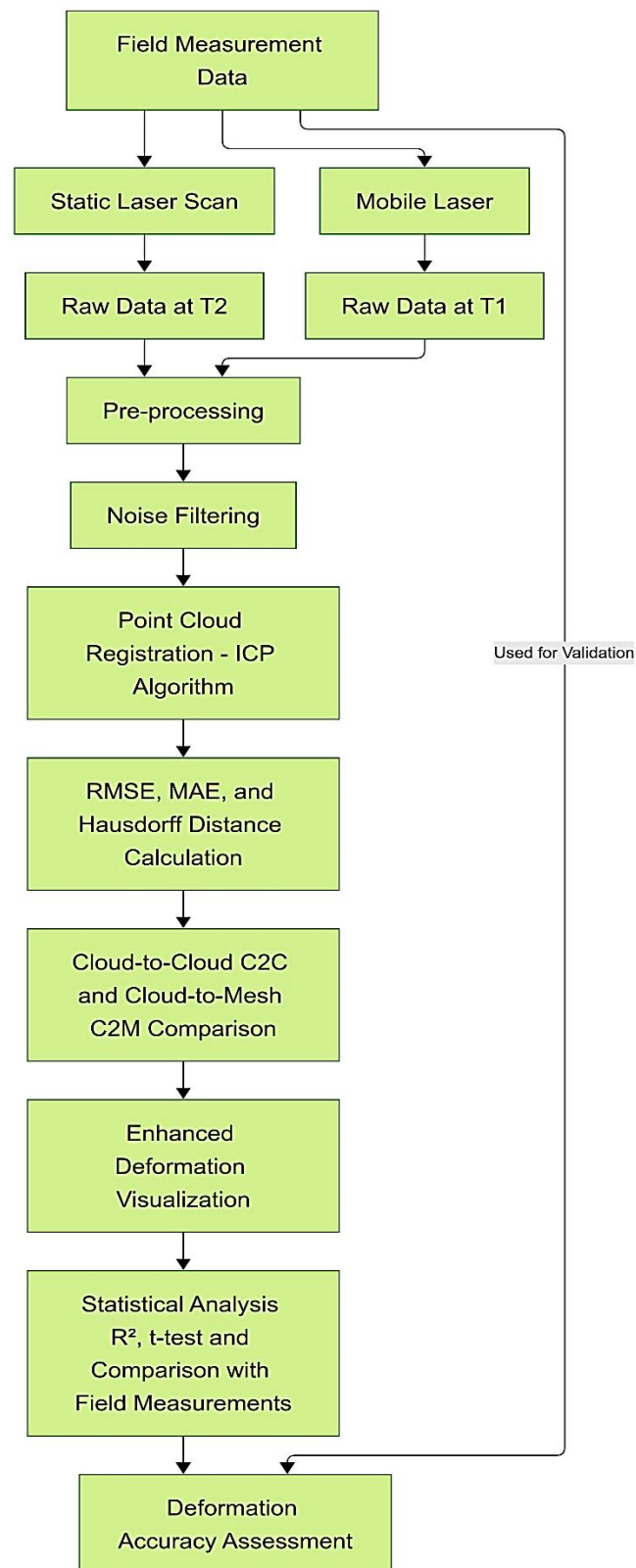
Figure 9: Technical process for calculating deformation based on point cloud data.
