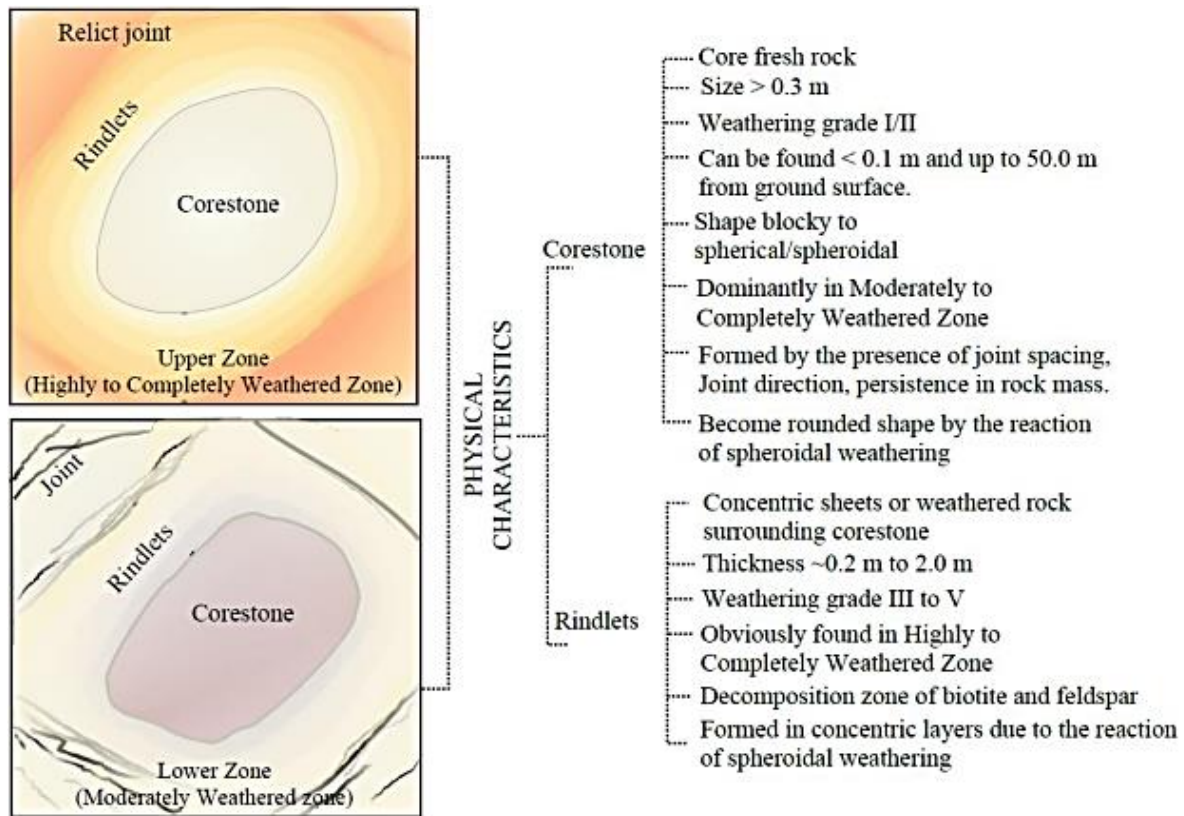
Figure 3: Summarization of the occurrence and characteristics boulder weathered rock mass (M. Dan et al., 2016)
