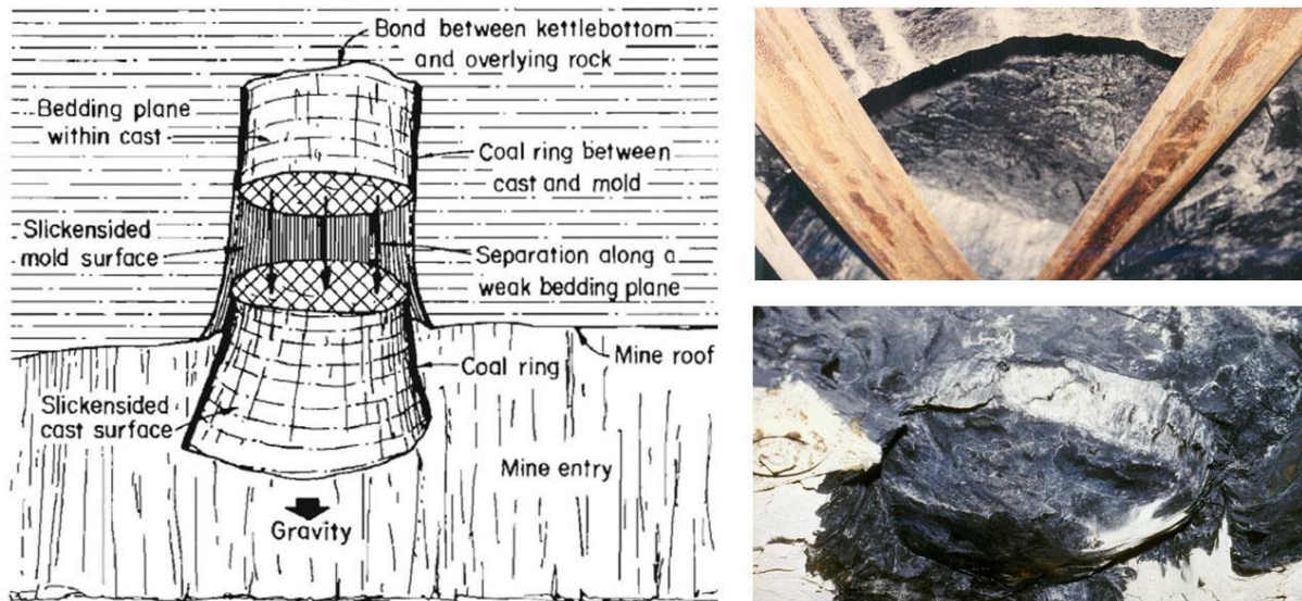
Figure 4: Isolated semi-circular rock mass in a mine roof. With a rounded or flat bottom when viewed from below (Kentucky Geological Survey, (2019))
