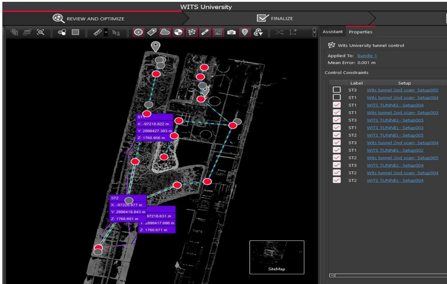
Figure 19: Registration of scans to a unified coordinate system, showing a closed-loop trajectory of mobile laser scanning with total station positions and computed X, Y, and Z values.
