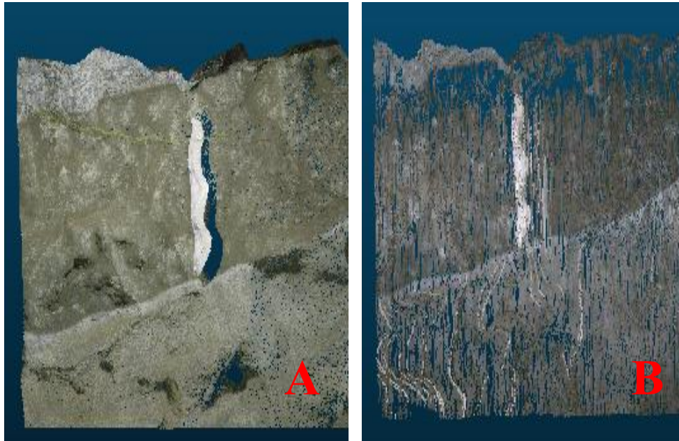
Figure 22: Comparison of occlusion effects in static and mobile LiDAR scans. A (static LiDAR), occlusion is visible behind the object leaving gaps due to restricted line of sight. B (mobile LiDAR), reduced occlusion because of moving scanner capturing multiple perspectives
