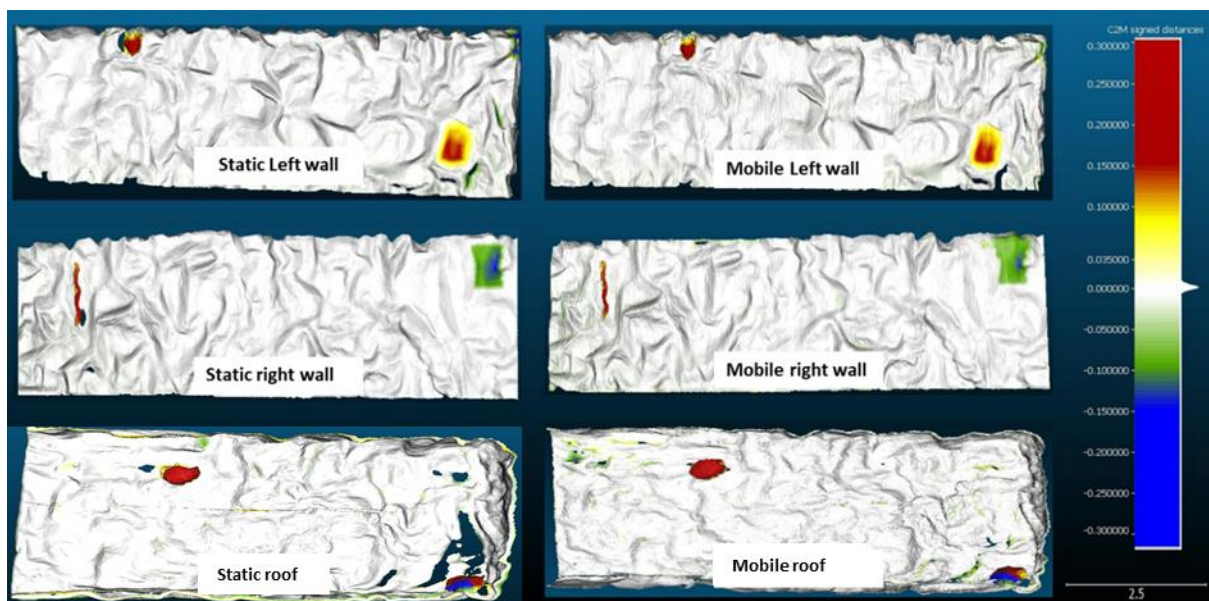
Figure 25: Contrast of static and mobile LiDAR segments, presenting localised deformations. Warm colours (red and yellow) indicate outward deformation or material addition, and cool colours (blue and green) signify inward deformation or material loss.
