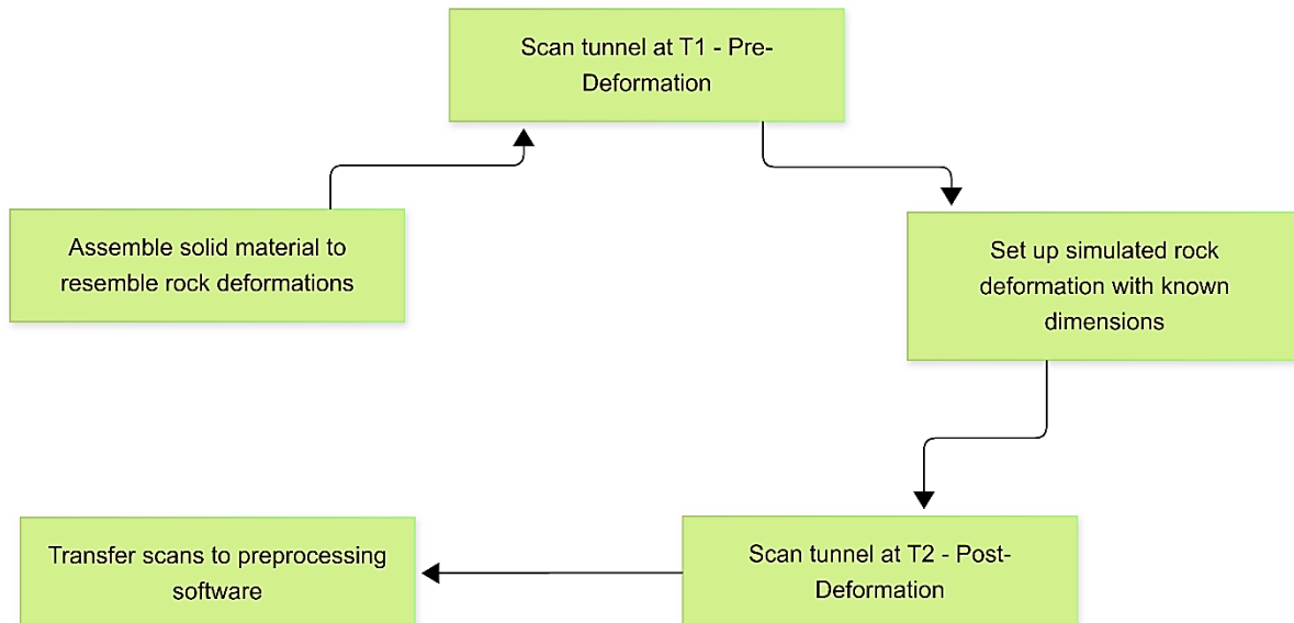
Figure 8: Acquisition process for deformation simulation and measurement.
