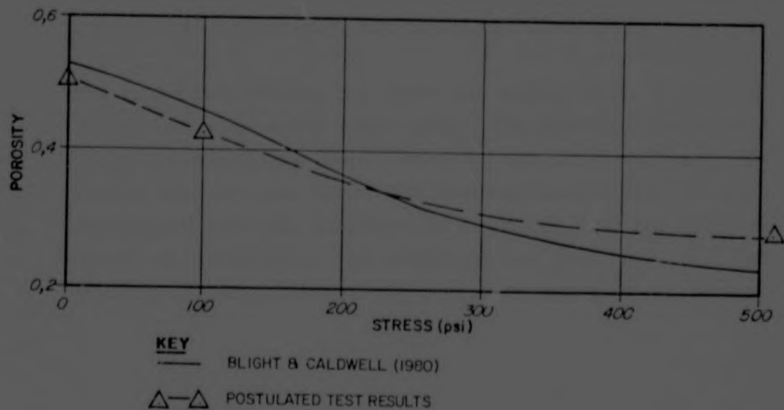
FIGURE 6.5 COMPARISON OF CHANGES IN POROSITY
