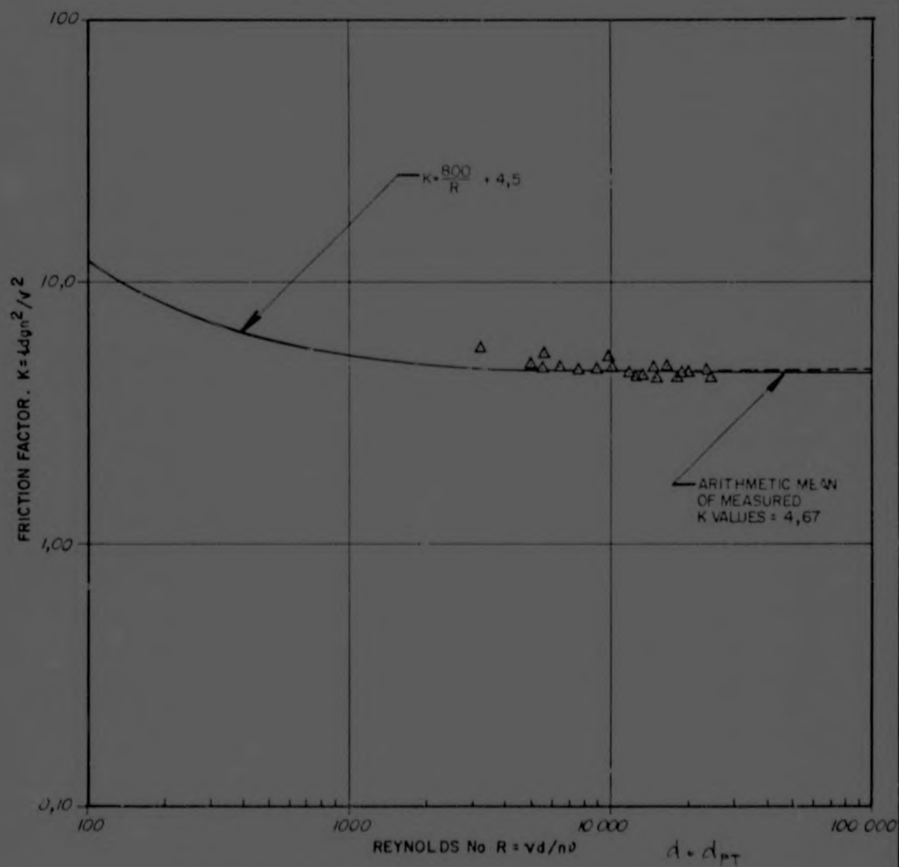
FIGURE 6.10 TEST No. 2: PLOT OF FRICTION FACTORS
