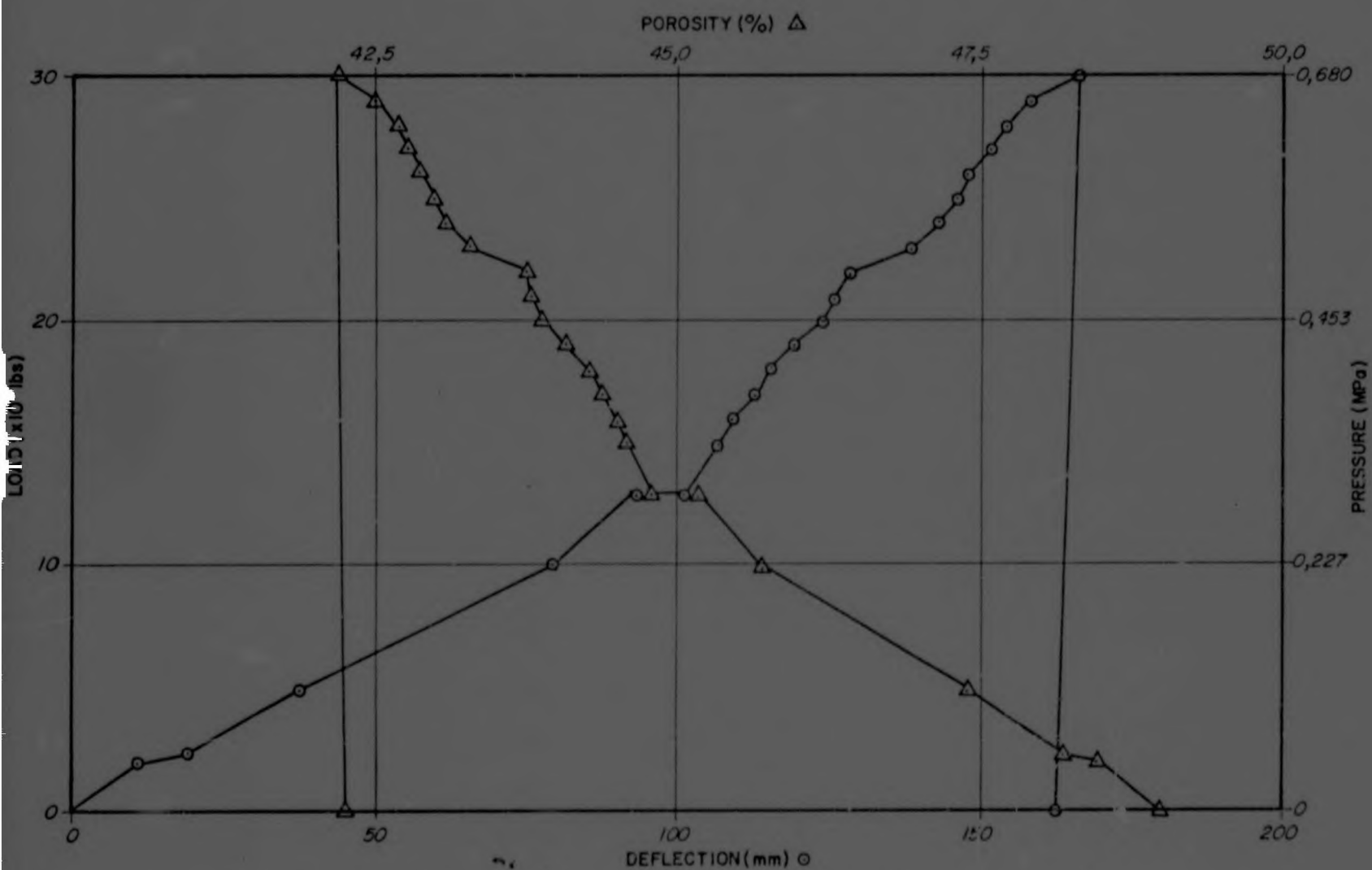
FIGURE 6.3 PLOT OF LOAD & PRESSURE vs DEFLECTION & POROSITY FOR LOAD TEST No 1
