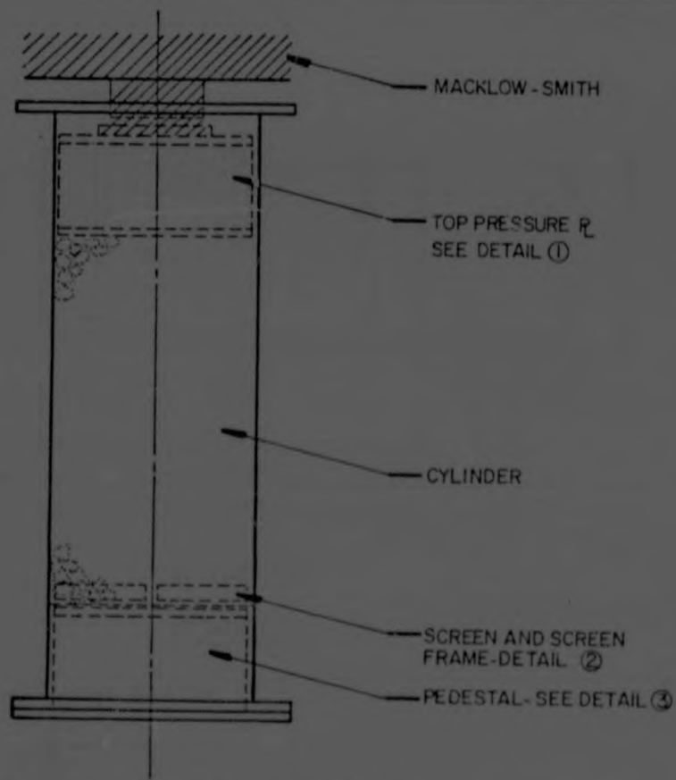
ELEVATION ON PERMEAMETER IN LOADING RIG
