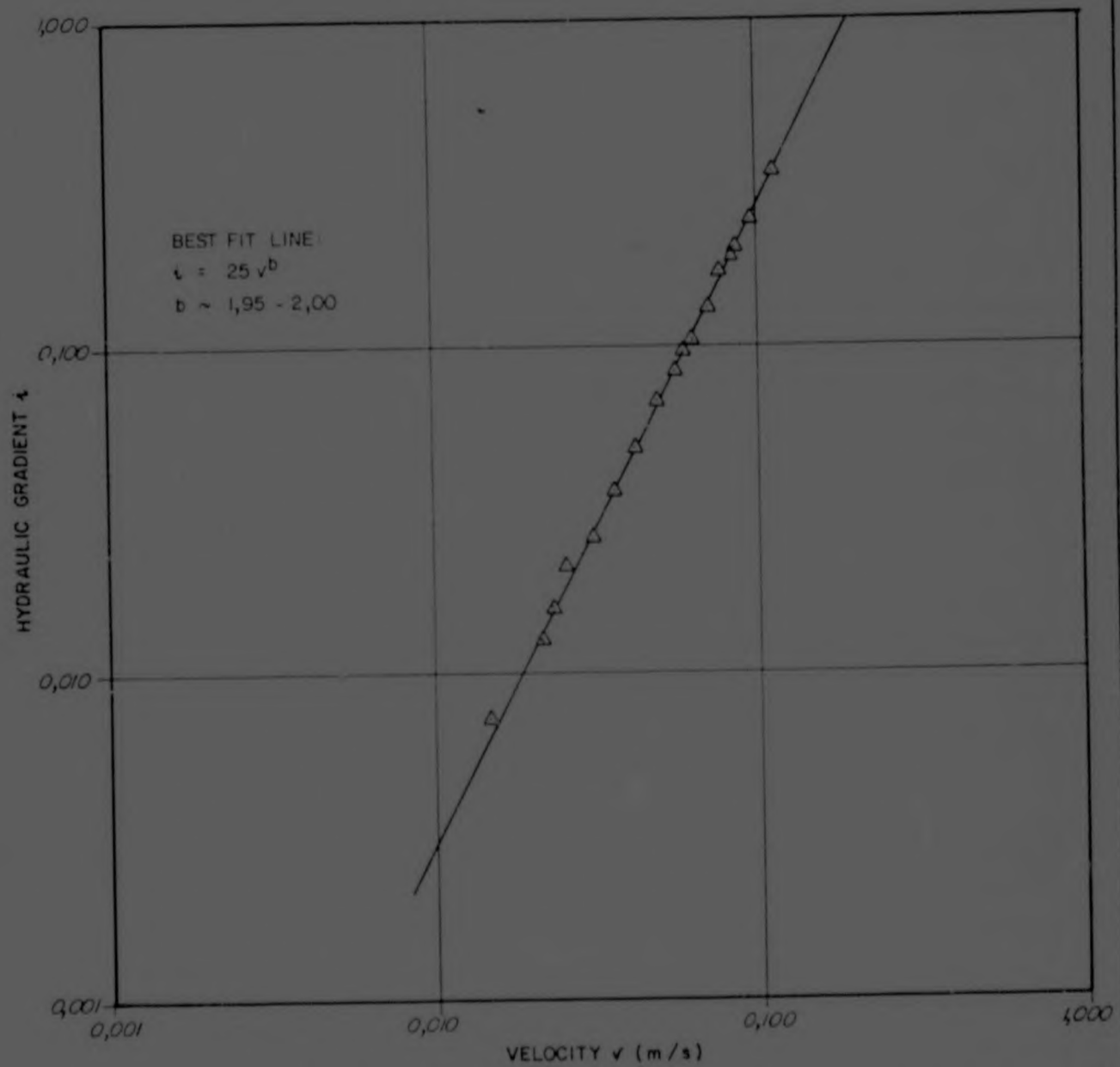
FIGURE 6.7 TEST No 2 : PLOT OF VELOCITY AGAINST HYDRAULIC GRADIENT
