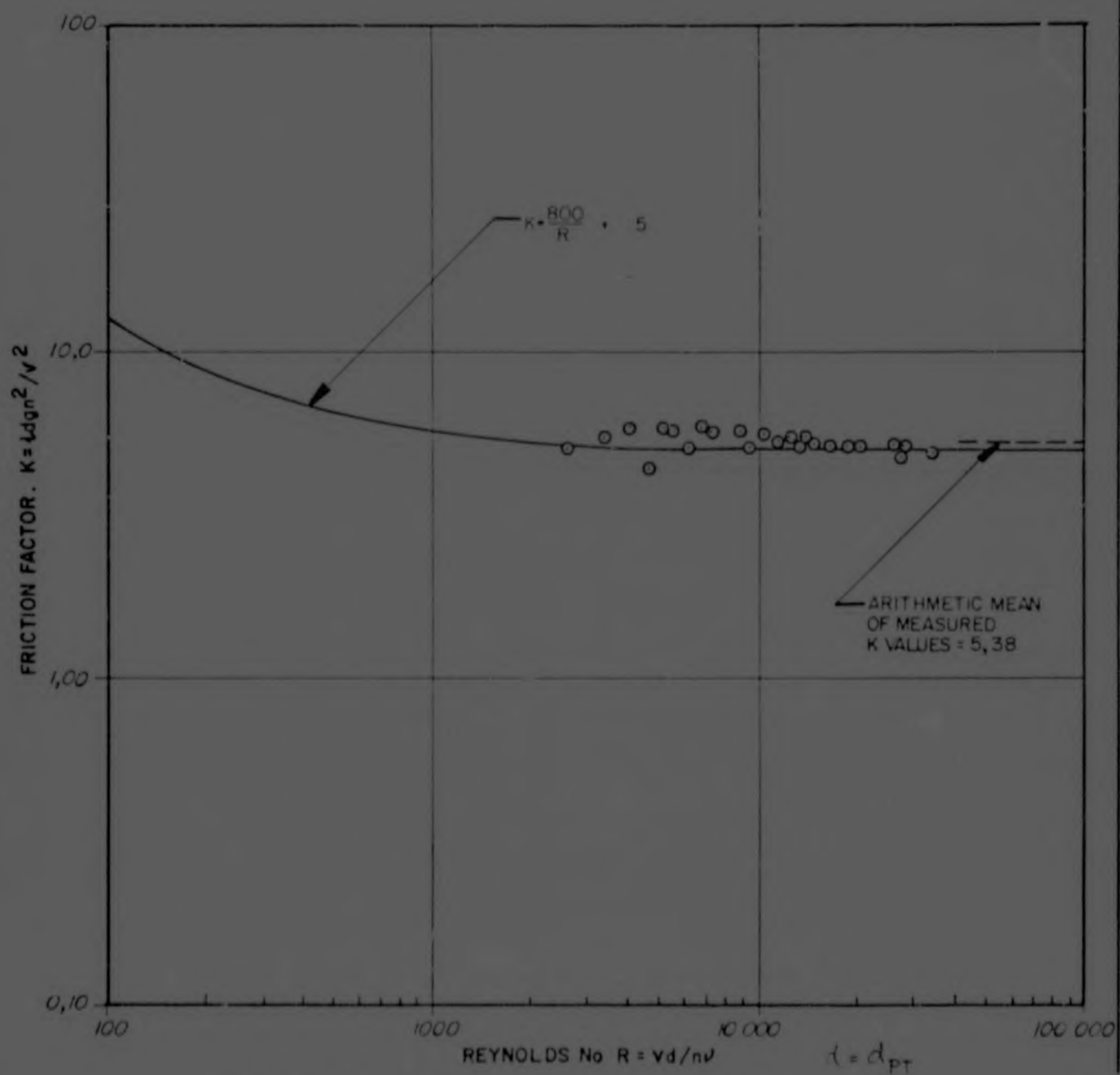
FIGURE 6.9 TEST No I : PLOT OF FRICTION FACTORS
