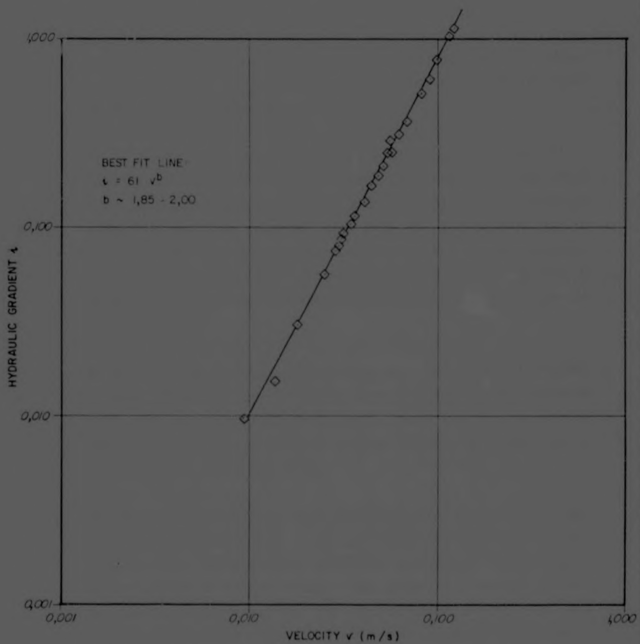
FIGURE 68 TEST No 3: PLOT OF VELOCITY AGAINST HYDRAULIC GRADIENT
