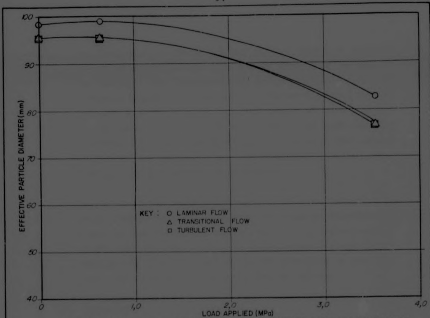
FIGURE 6.2a CHANGE IN EFFECTIVE PARTICLE DIAMETER-PARALLEL LAYER MODEL
