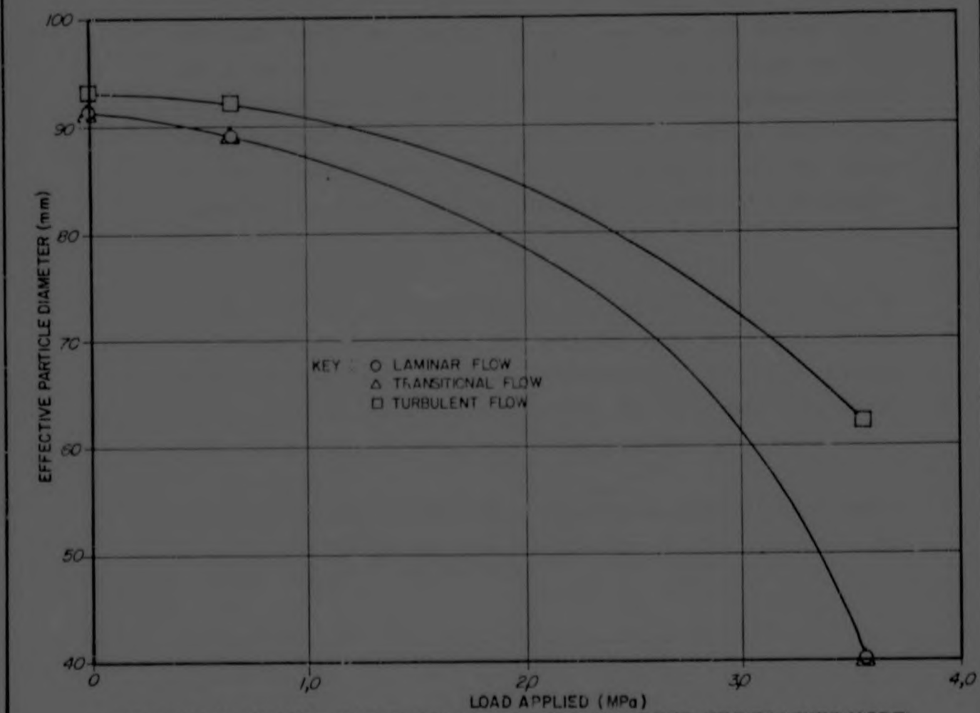
FIGURE 6.2b CHANGE IN EFFECTIVE PARTICLE DIAMETER-SERIES LAYER MODEL
