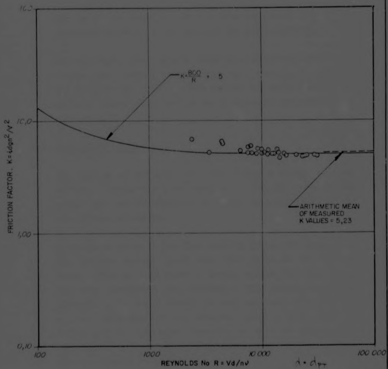
FIGURE 6.11 TEST No 3: PLOT OF FRICTION FACTORS
