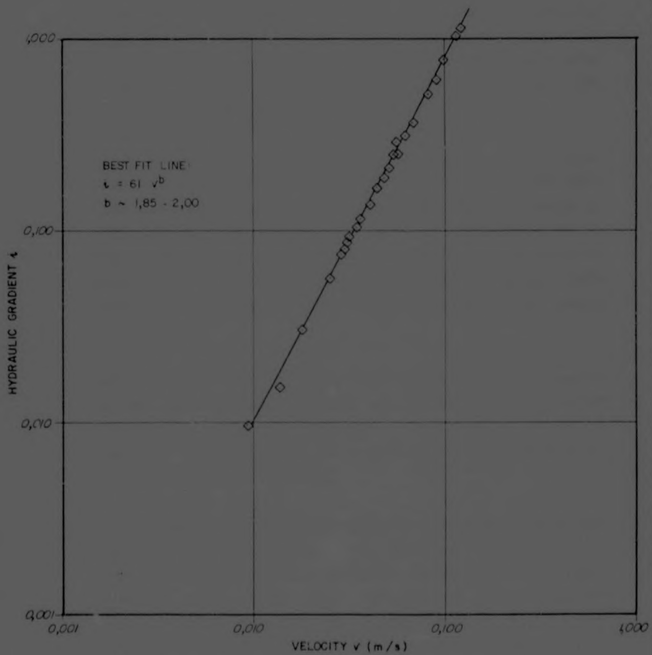
FIGURE 6B TEST No 3: PLOT OF VELOCITY AGAINST HYDRAULIC GRADIENT
