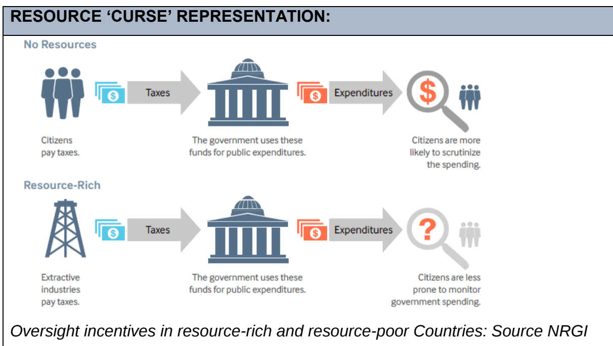
Figure 2: Resource-curse phenomenon
