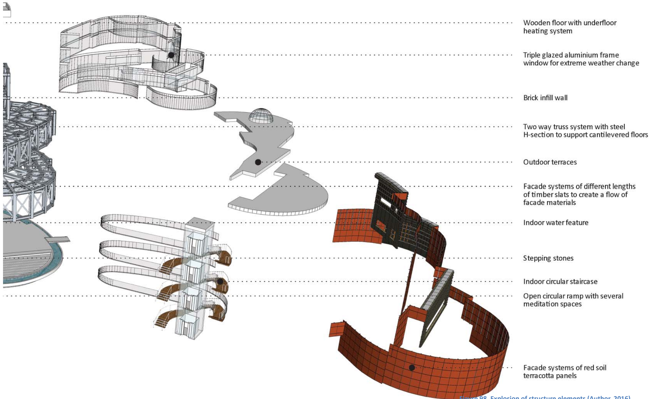
Figure 98_Explosion of structure elements (Author, 2016)
