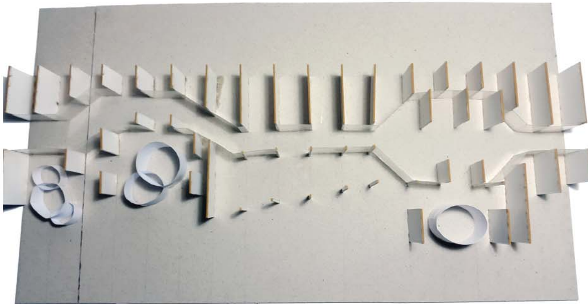
Figure 82_Models of blending phenomena (Author, 2016)
