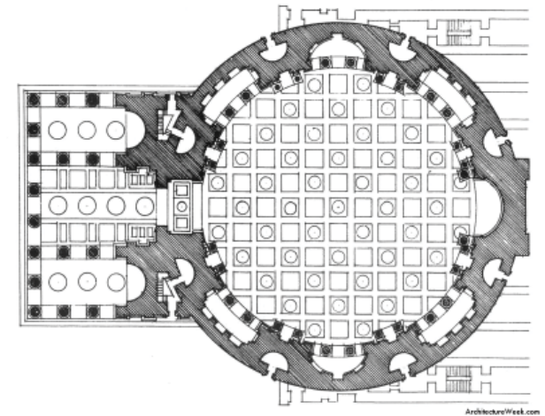
Figure 22_Plan of the Pantheon (Guest, 2014)
