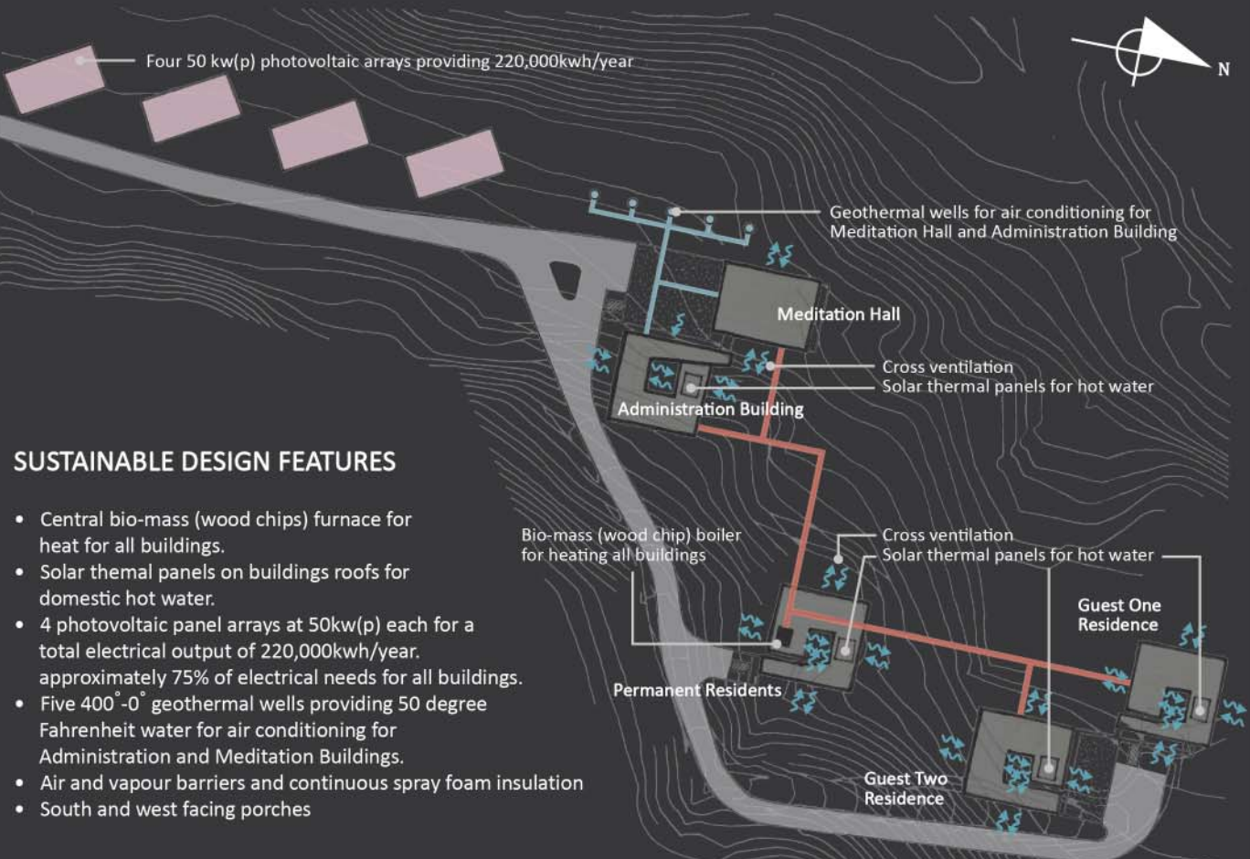
Figure 32_Diagram of green feature (Hanrahan Meyers Architects, n.d.) 22
