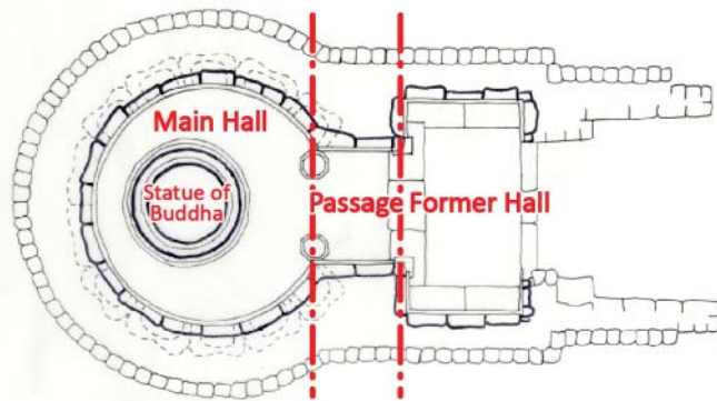
Figure 24_Plan of Sokkuram grotto (Mokin, 2011) 17
