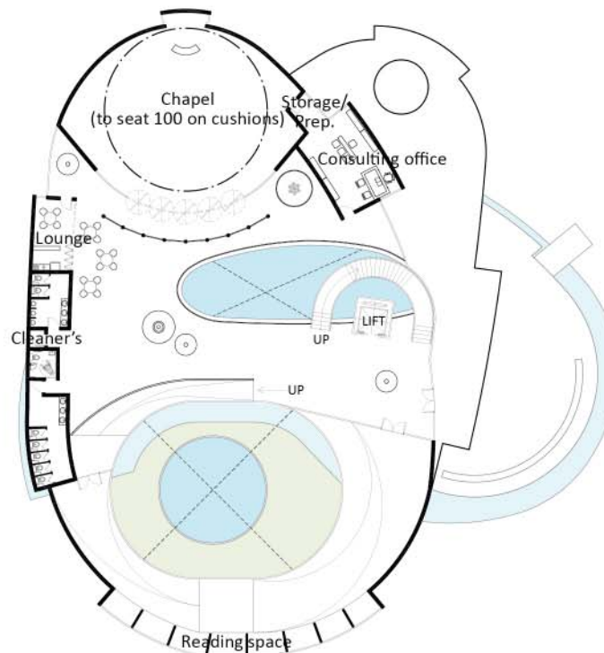
Second Floor_1:500
