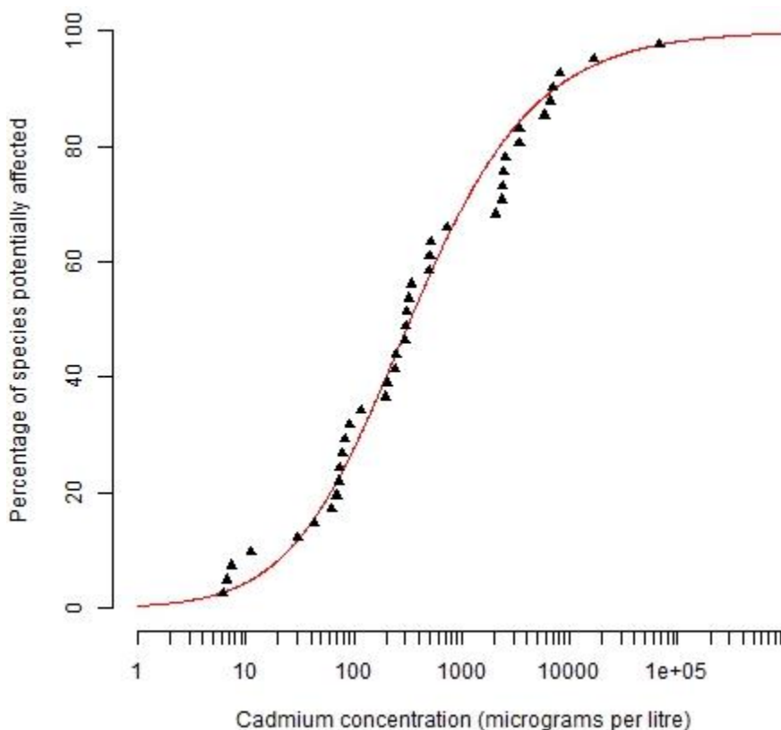
Figure 4.1 SSD (Burr Type III Distribution) for dissolved cadmium fitted over LC50 toxicity data for freshwater macroinvertebrates obtained from scientific publications
