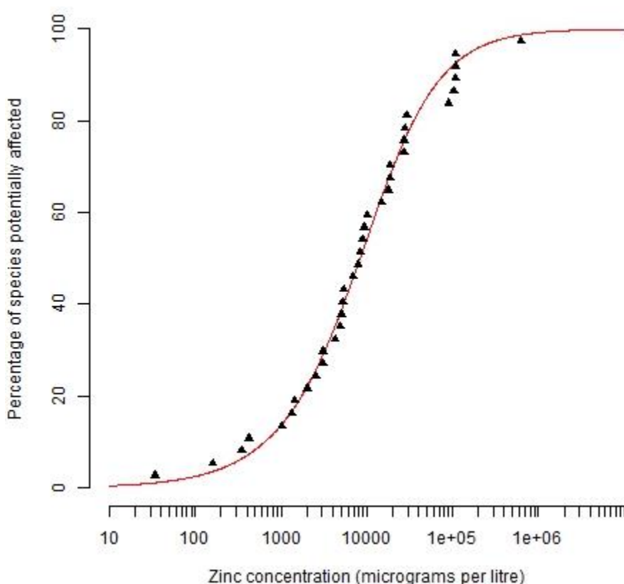
Figure 4.8 SSD (Burr Type III Distribution) for zinc fitted over LC50 toxicity data for freshwater macroinvertebrates obtained from scientific publications
