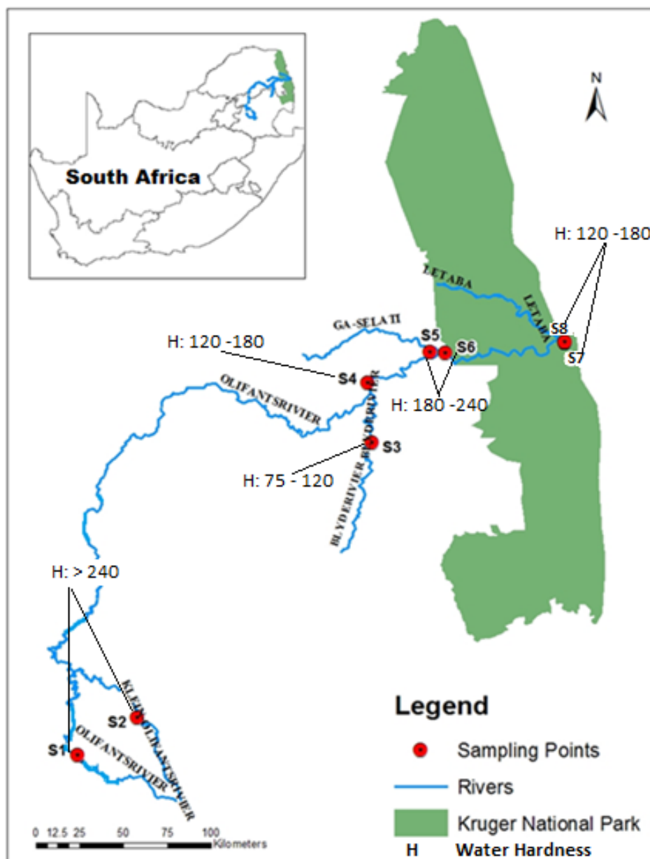
Figure 6.1 Olifants River study sites and corresponding water hardness (mg/L as \text{CaCO}_3 ) levels based on water hardness records (2006-2016) sourced from the South African Department of Water and Sanitation.
