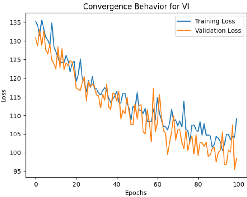
Figure 4.3: Model Training and Validation Loss Using 50% of the Dataset
