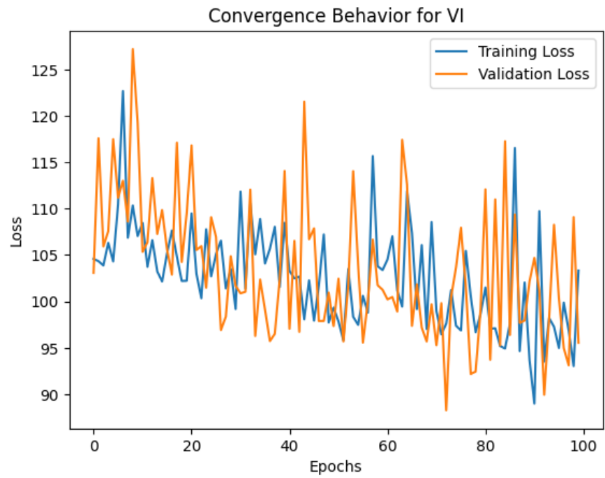
Figure 4.1: Model Training and Validation Loss Using Full Dataset
