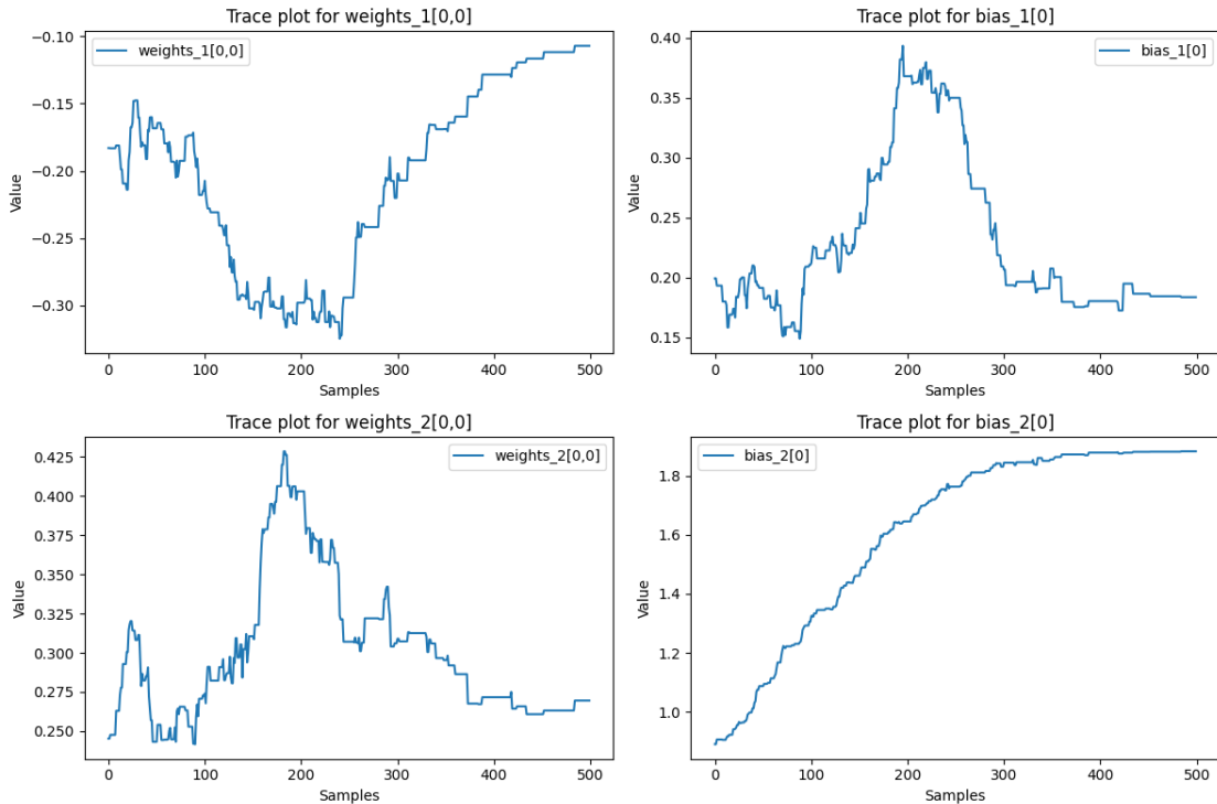
Figure 4.4: Parameter Trace Plots from MCMC Sampling using Full Dataset
