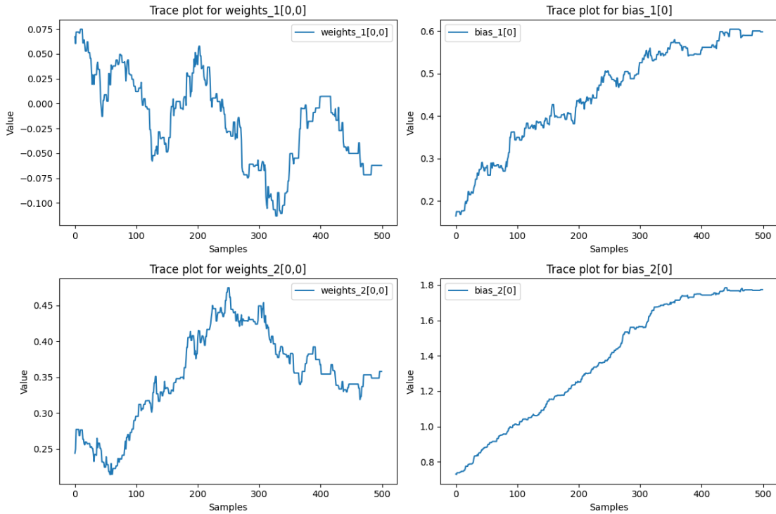
Figure 4.6: Parameter Trace Plots from MCMC Sampling using 50% of the Dataset
