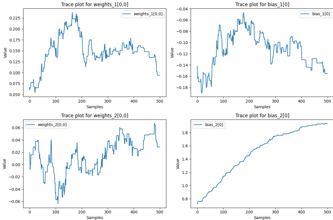
Figure 4.5: Parameter Trace Plots from MCMC Sampling using 75% of the Dataset
