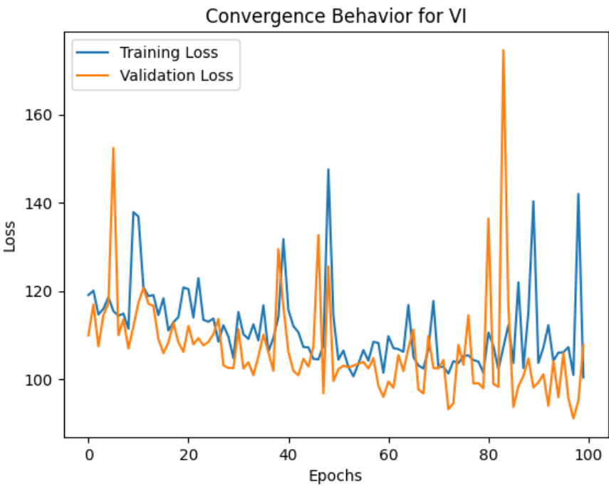
Figure 4.2: Model Training and Validation Loss Using 75% of the Dataset
