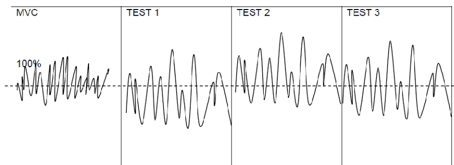
Figure 2.5 Normalisation process
