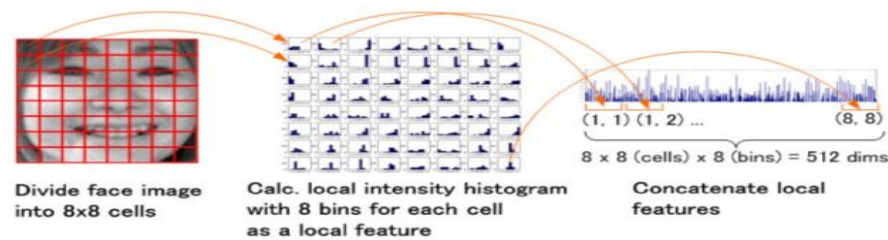
Figure 13: (Shimada et al (2010, pages 277–286,[6])). Appearance-based smile intensity estimation by cascaded support vector machines.
