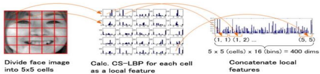
Figure 14: (Shimada et al (2010, pages 277–286,[6])). Appearance-based smile intensity estimation by cascaded support vector machines.
