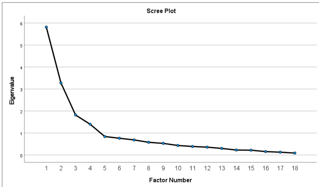
Figure 4-4: Scree Plot
