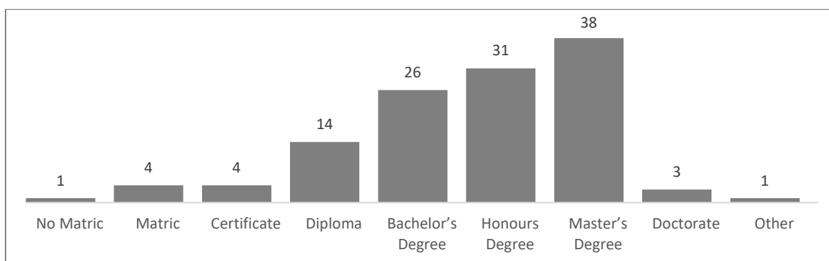
Figure 4-1: Level of Education
