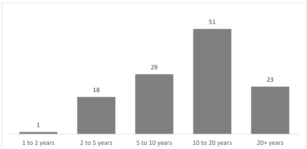
Figure 4-3: How many years have you been in a decision-making role?
