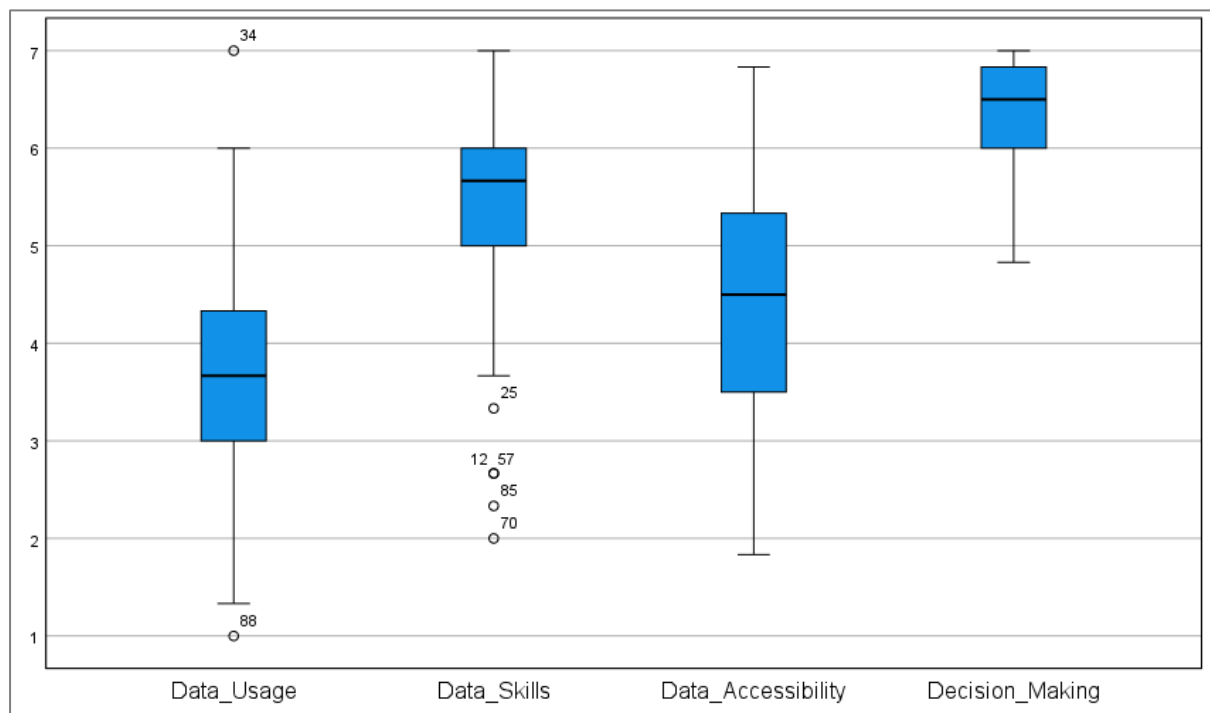
Figure 4-6: Boxplots with Outliers Addressed
