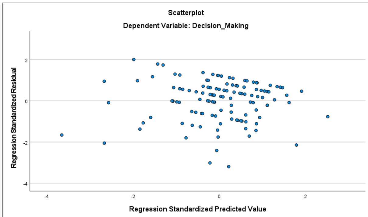
Figure 4-7: Scatterplot
