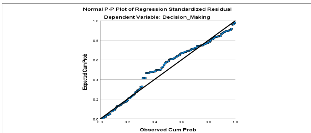
Figure 4-8: Normal P Plot of Regression Standardised Residual
