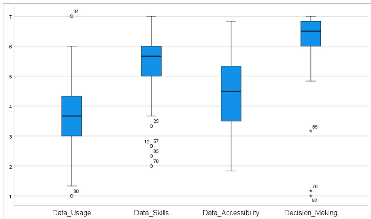
Figure 4-5: Boxplots with Outliers
