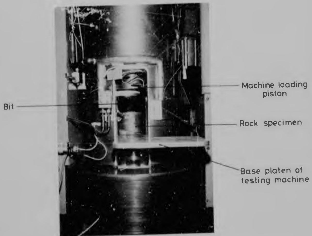
FIGURE 89 : Method of mounting the bit and the rock in the testing machine for indentation experiments.
