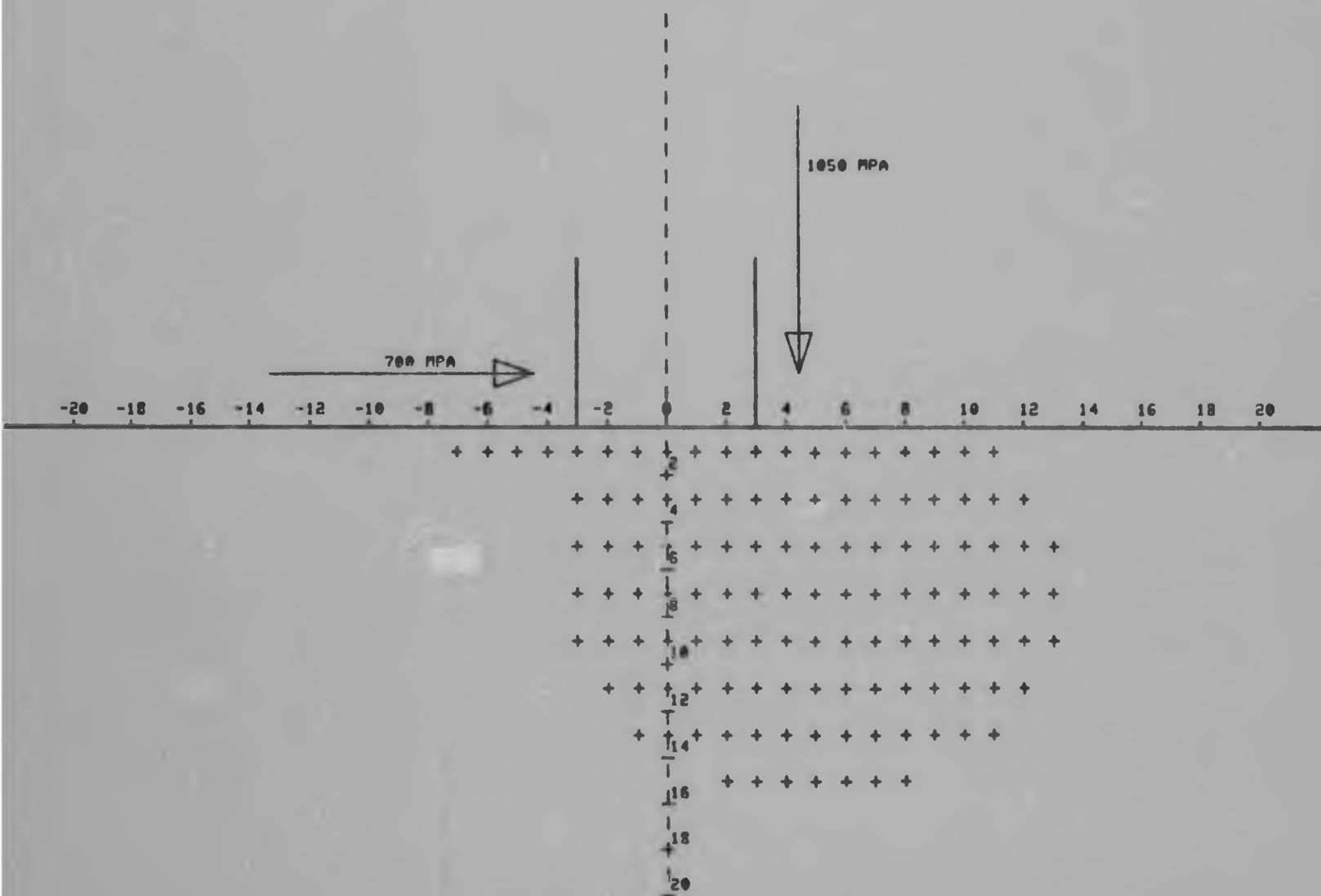
FIGURE 128 : Zone of excess mass when both a normal pressure 1 050 MPa and a shear pressure 700 MPa are applied to the surface of the body.
