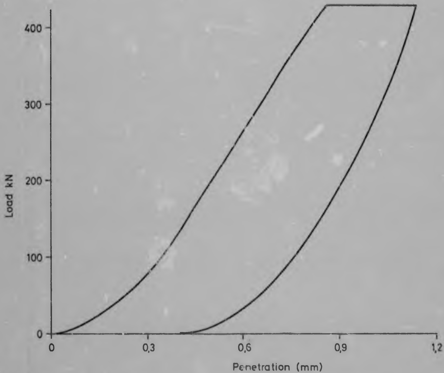
FIGURE 99 : Indentation load plotted against bit penetration for second norite specimen.
