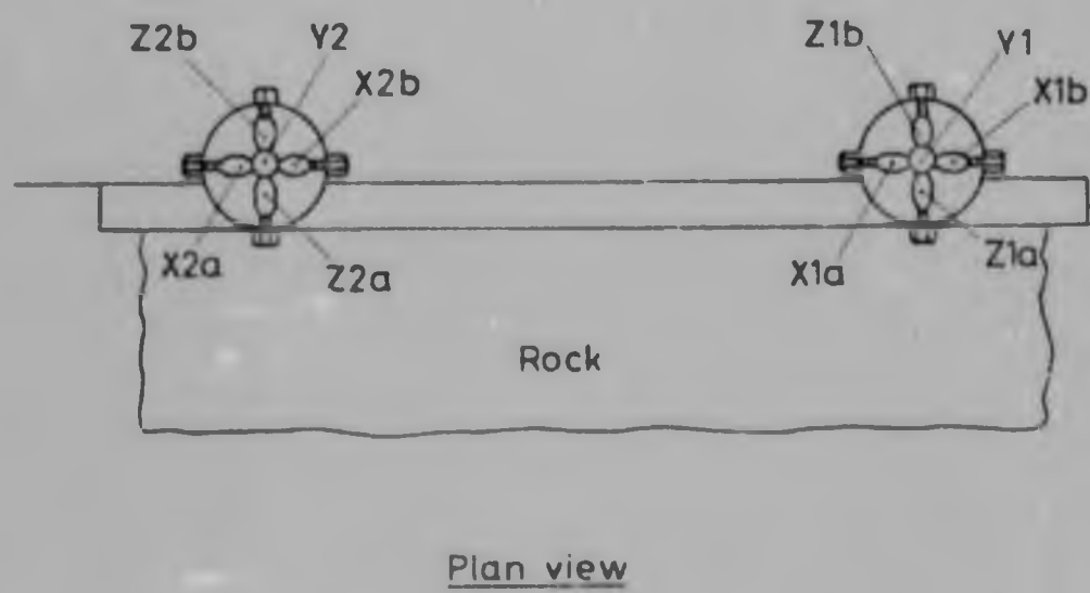
FIGURE 22 : Mounting of load cell billets relative to the block of rock.
