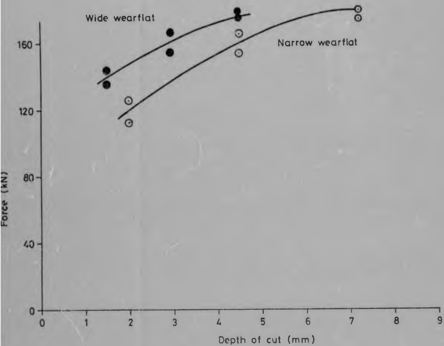
FIGURE 44 : Mean peak bit penetrating force using a standard wearflat and a narrow wearflat bit.
