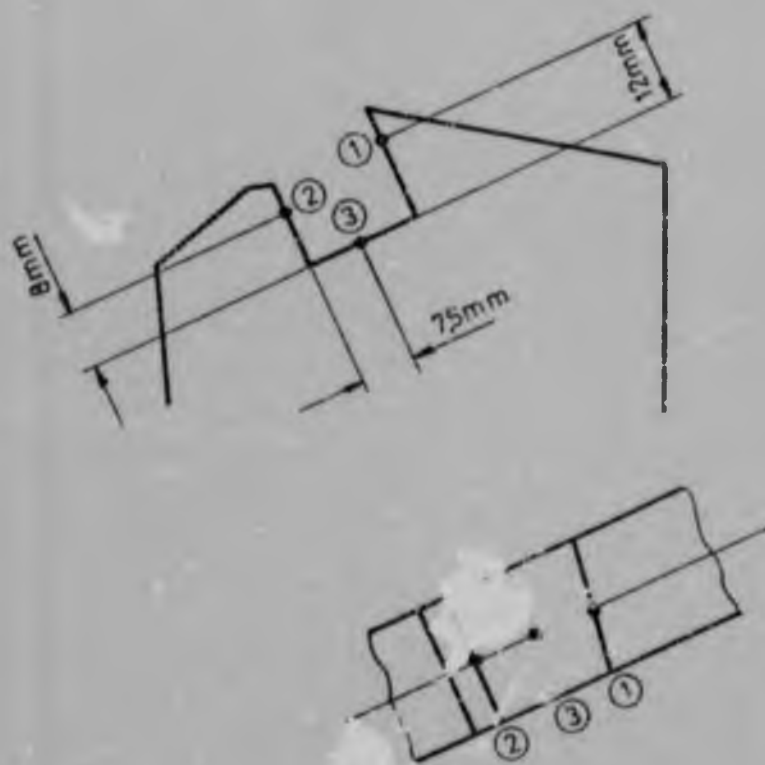
FIGURE 30 : Diagram illustrating the position of thermocouples mounted in the bit.
