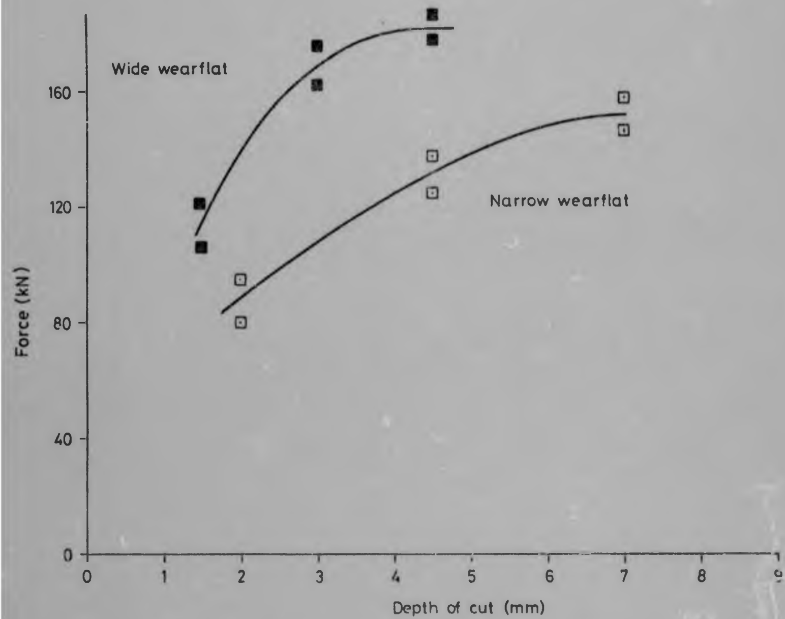
FIGURE 45 : Mean bit penetrating force using a standard wearflat and a narrow wearflat bit.
