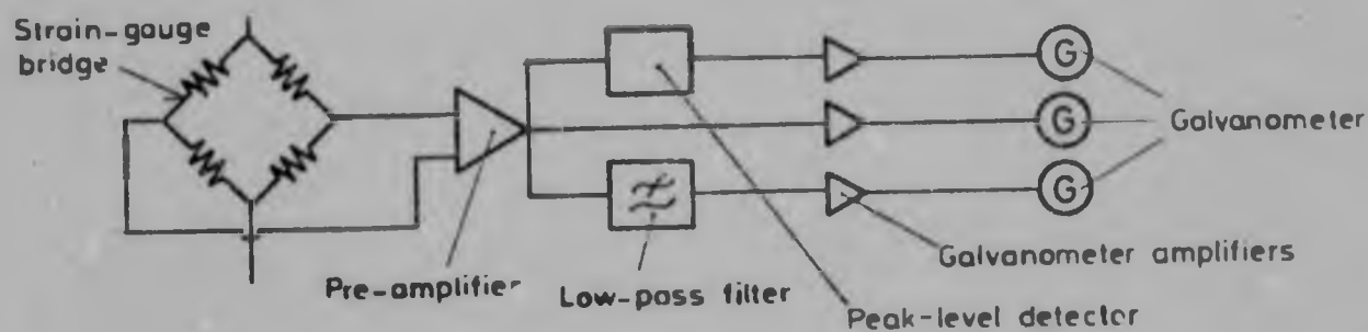
Cutting force instrumentation diagram.
