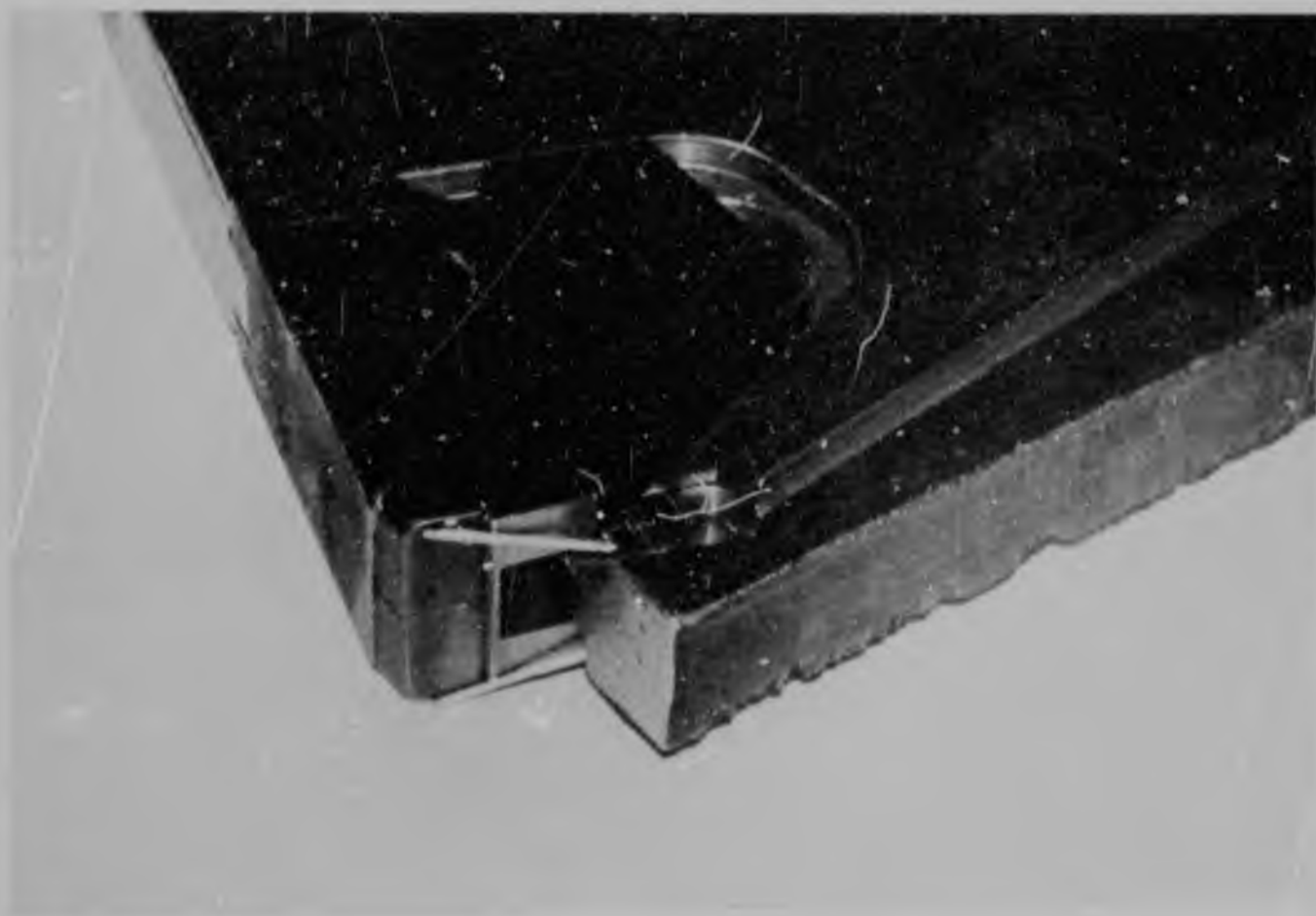
FIGURE 61. Method of mounting nozzles in the blade. White markers have been inserted into the nozzles to indicate the position of the water jets relative to the bit.
