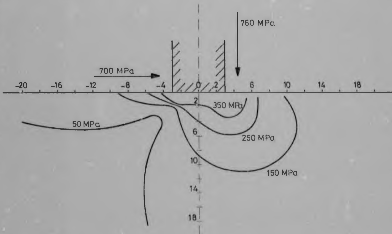
FIGURE 123 : Stress contours \tau_{max} when both a normal pressure 760 MPa and a shear pressure 700 MPa are applied to the surface of the body.
