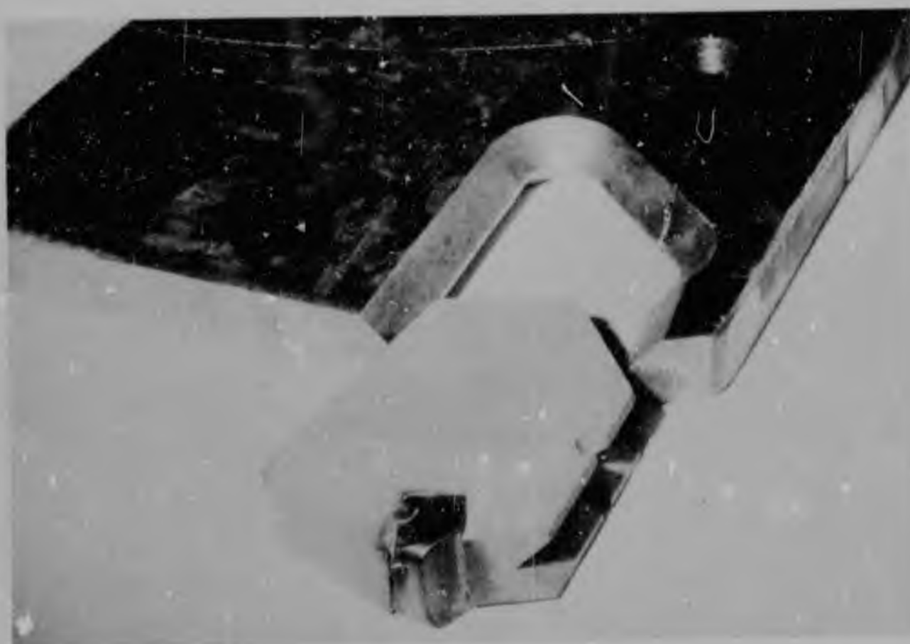
FIGURE 9. Detachable rockcutter bit, 23 mm thick, in use at the start of the pilot production trials of mining by rockcutting.
