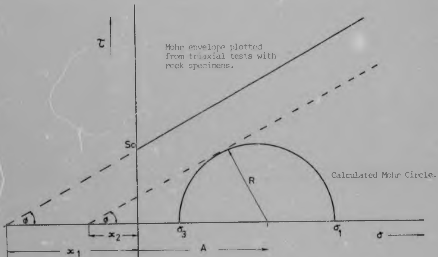
FIGURE 107 : Diagram illustrating the criterion used to determine the state of stress at points in the rock underneath an indenter.
