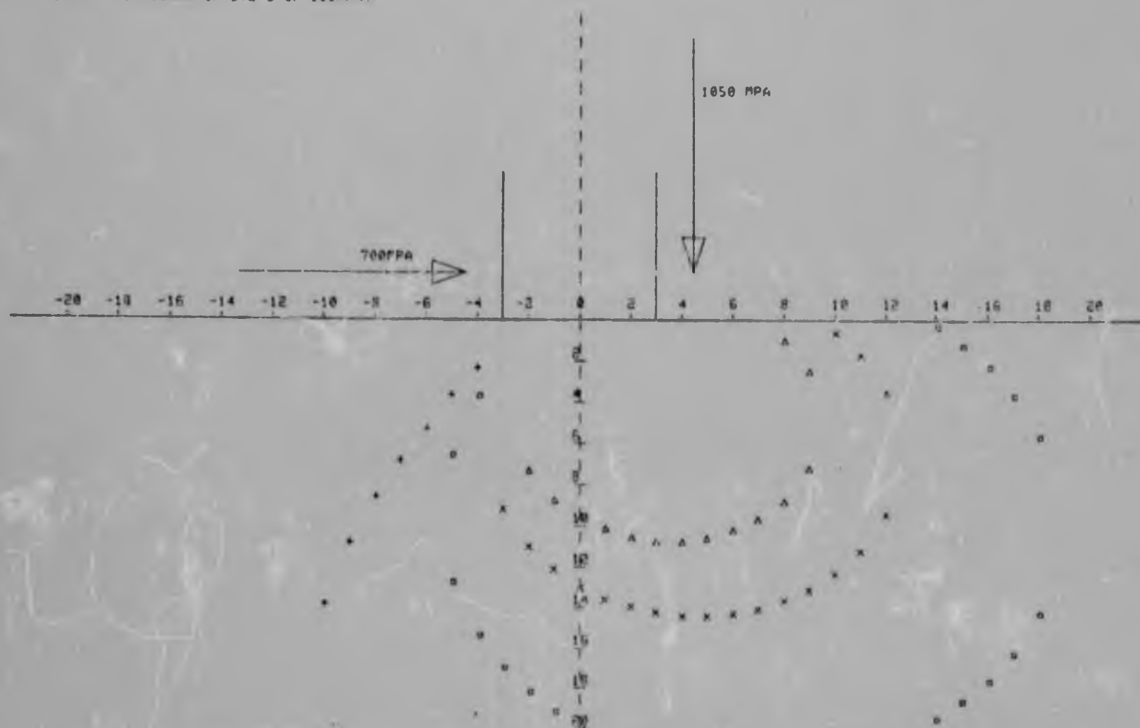
FIGURE 4.2 - An example of the generated plot of stress contours.
