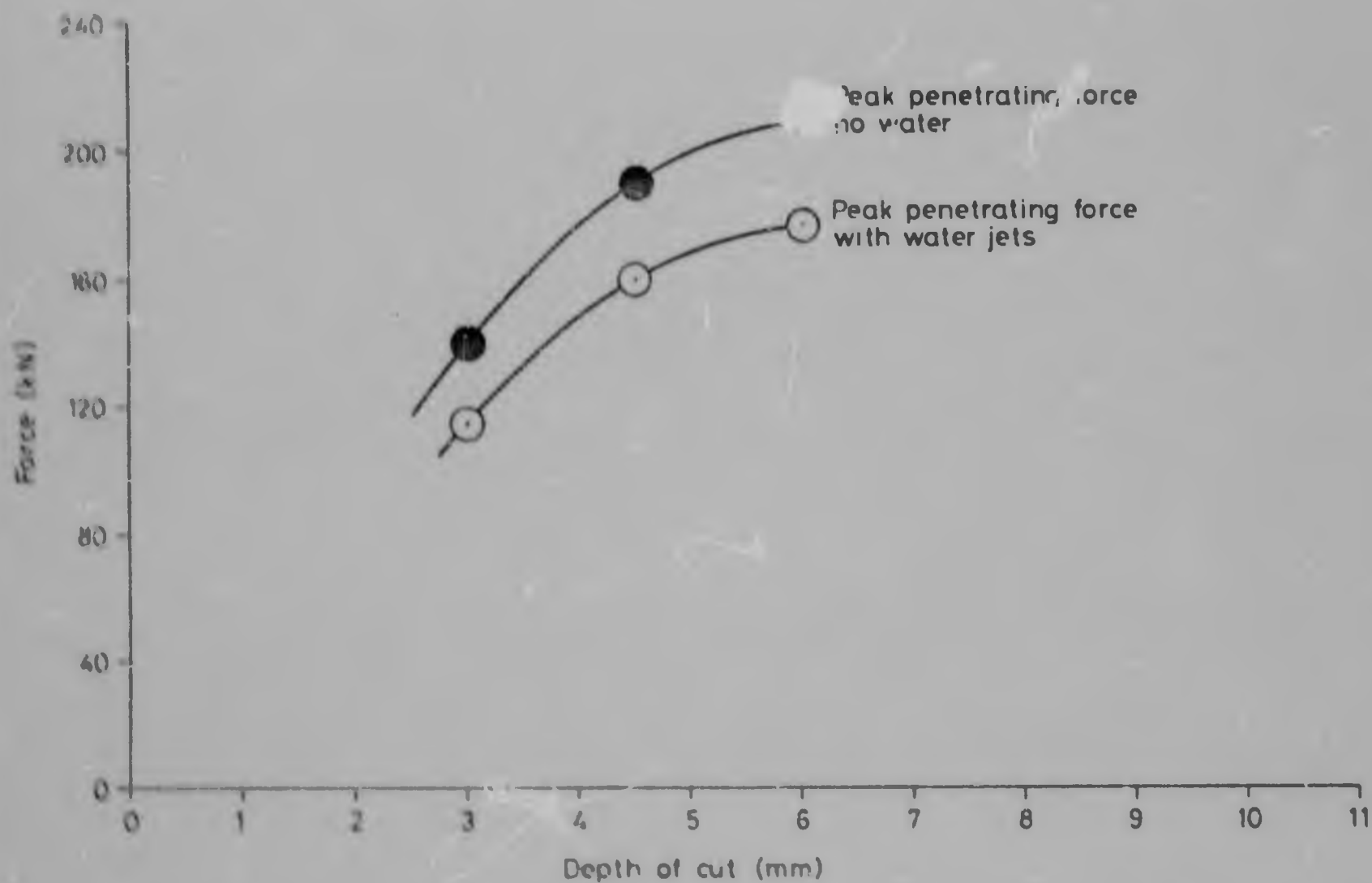
FIGURE 10. Mean peak jet penetrating force plotted against depth of cut, with a 'flat-fan' water jet and with no water jets.
