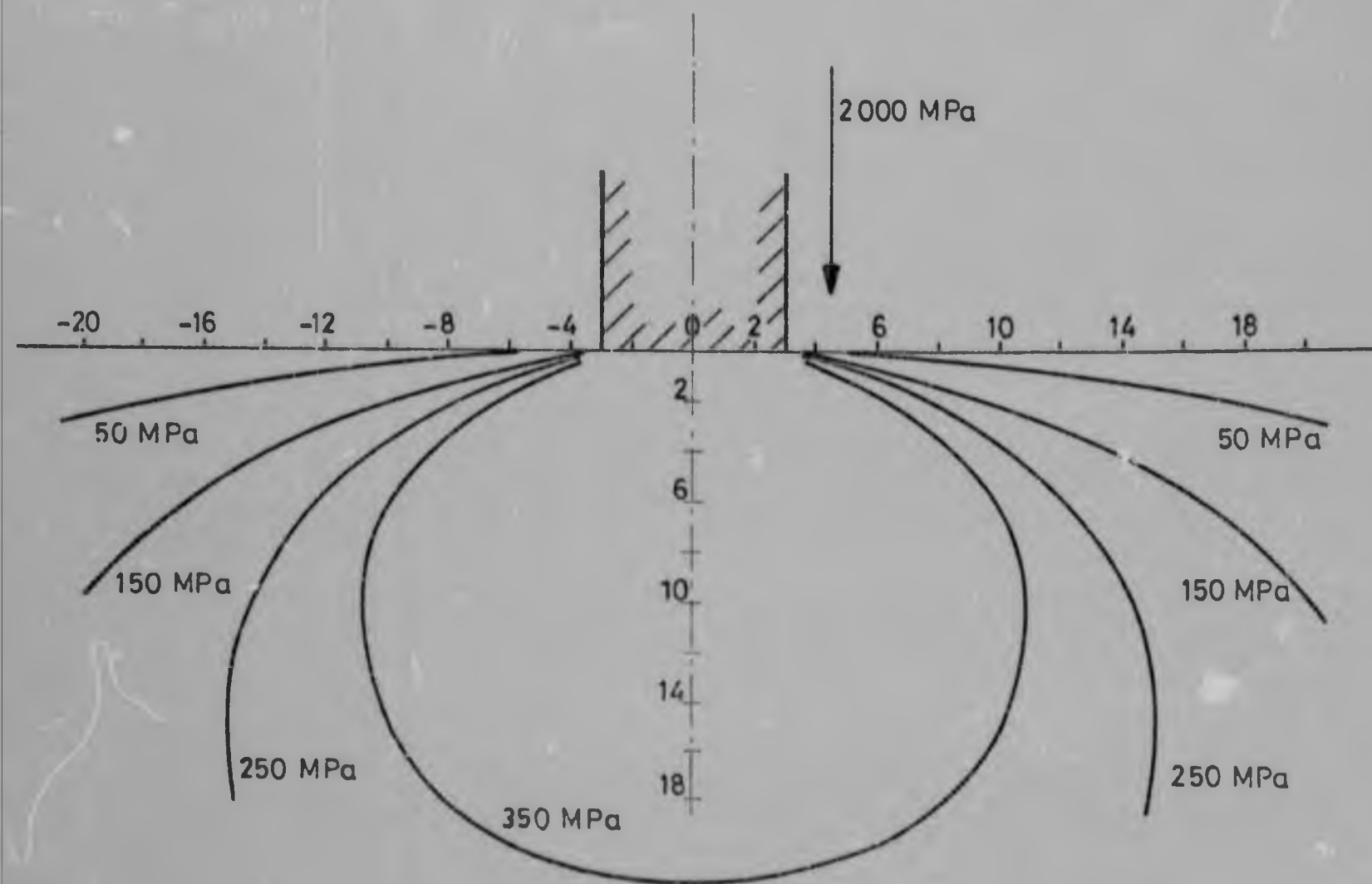
FIGURE 124 : Stress contours \sigma_1 when a normal pressure 2 000 MPa is applied to the surface of the body.
