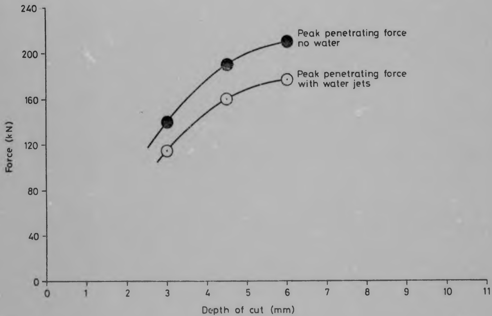
FIGURE 58 : Mean peak bit penetrating force plotted against depth of cut, with a 'flat-fan' water jet and with no water jets.
