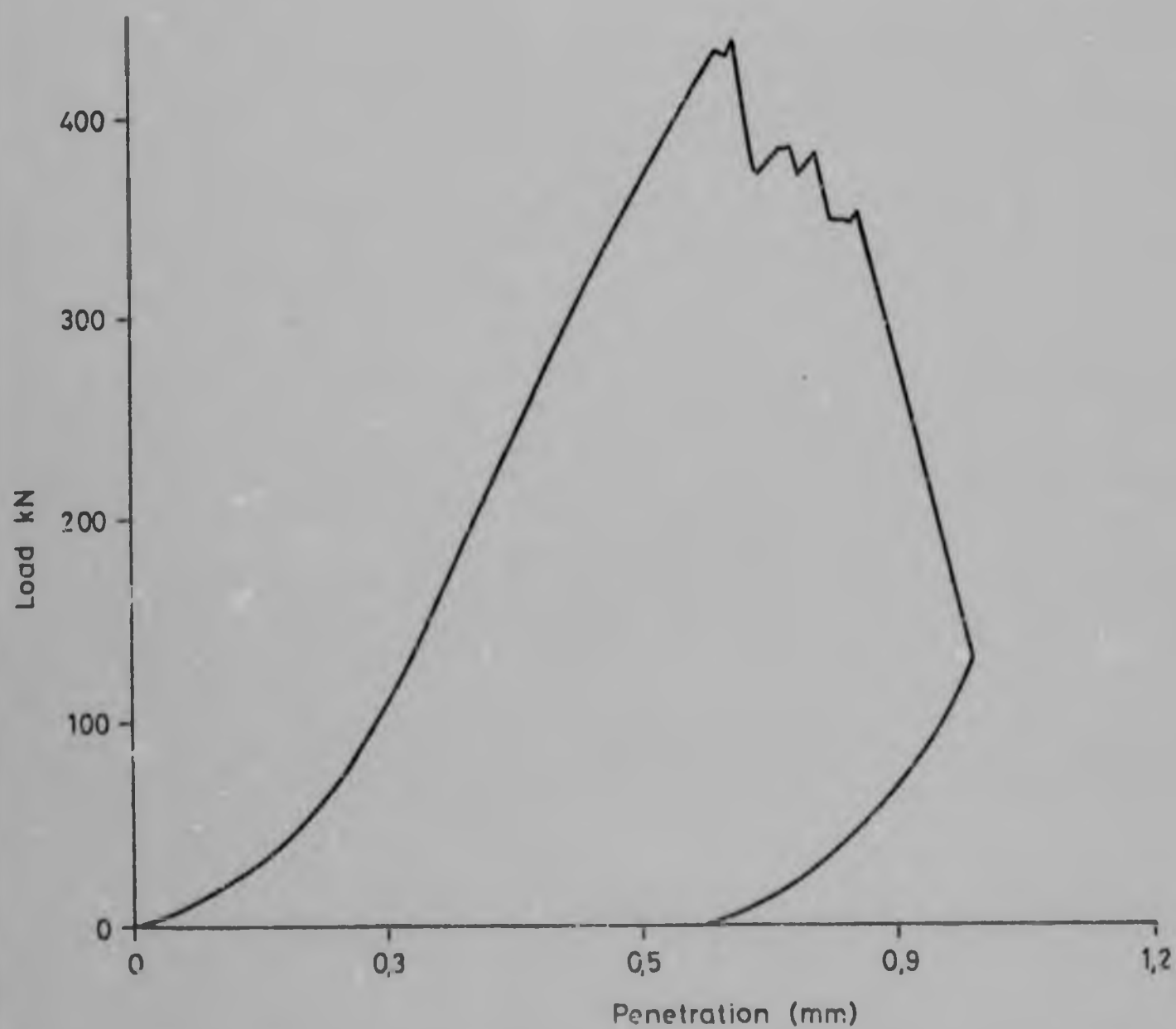
FIGURE 91 : Indentation force required to form a rock chip in norite, plotted against penetration of the bit.
