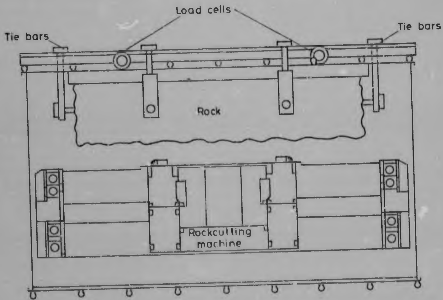
FIGURE 17 : Diagram of test frame. Plan view illustrating the rockcutting machine set up to cut against the norite block.
