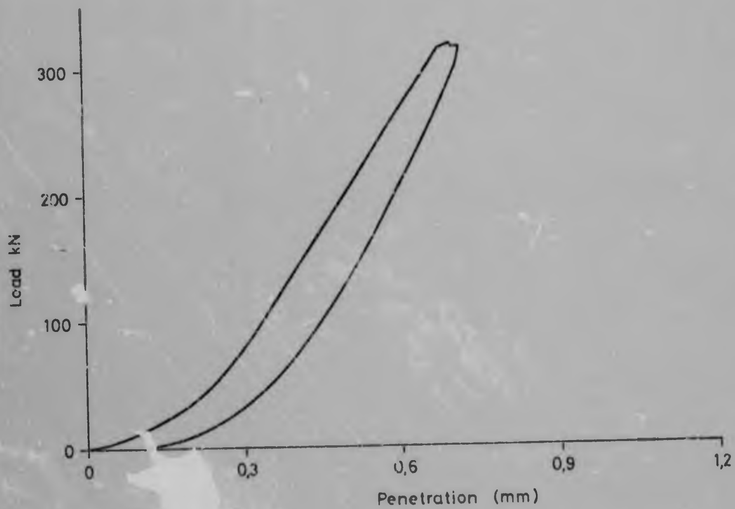
FIGURE 100 : Indentation load plotted against bit penetration for first quartzite specimen.
