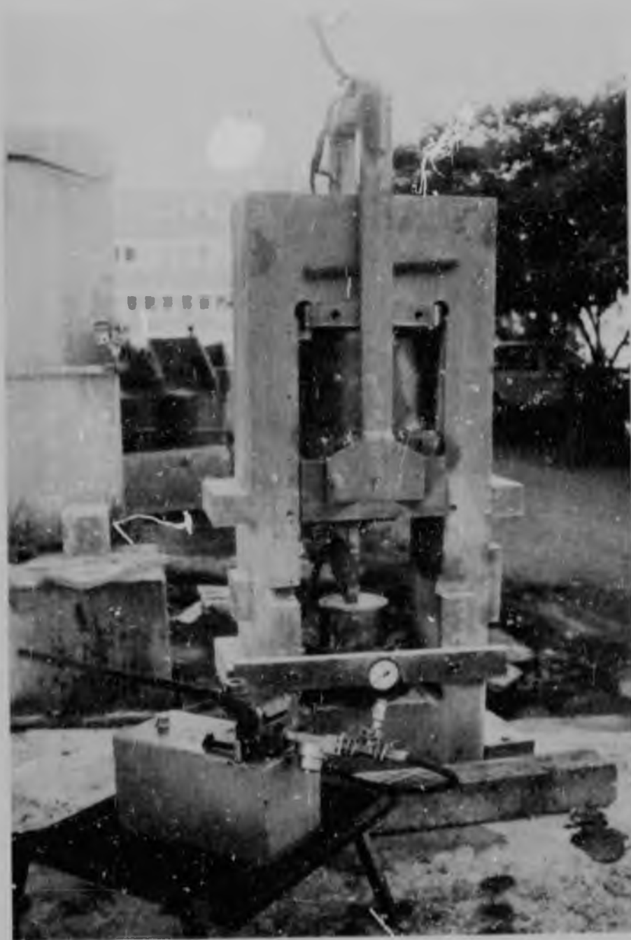
FIGURE 134 : Press used for indentation tests with high pressure water jets.
