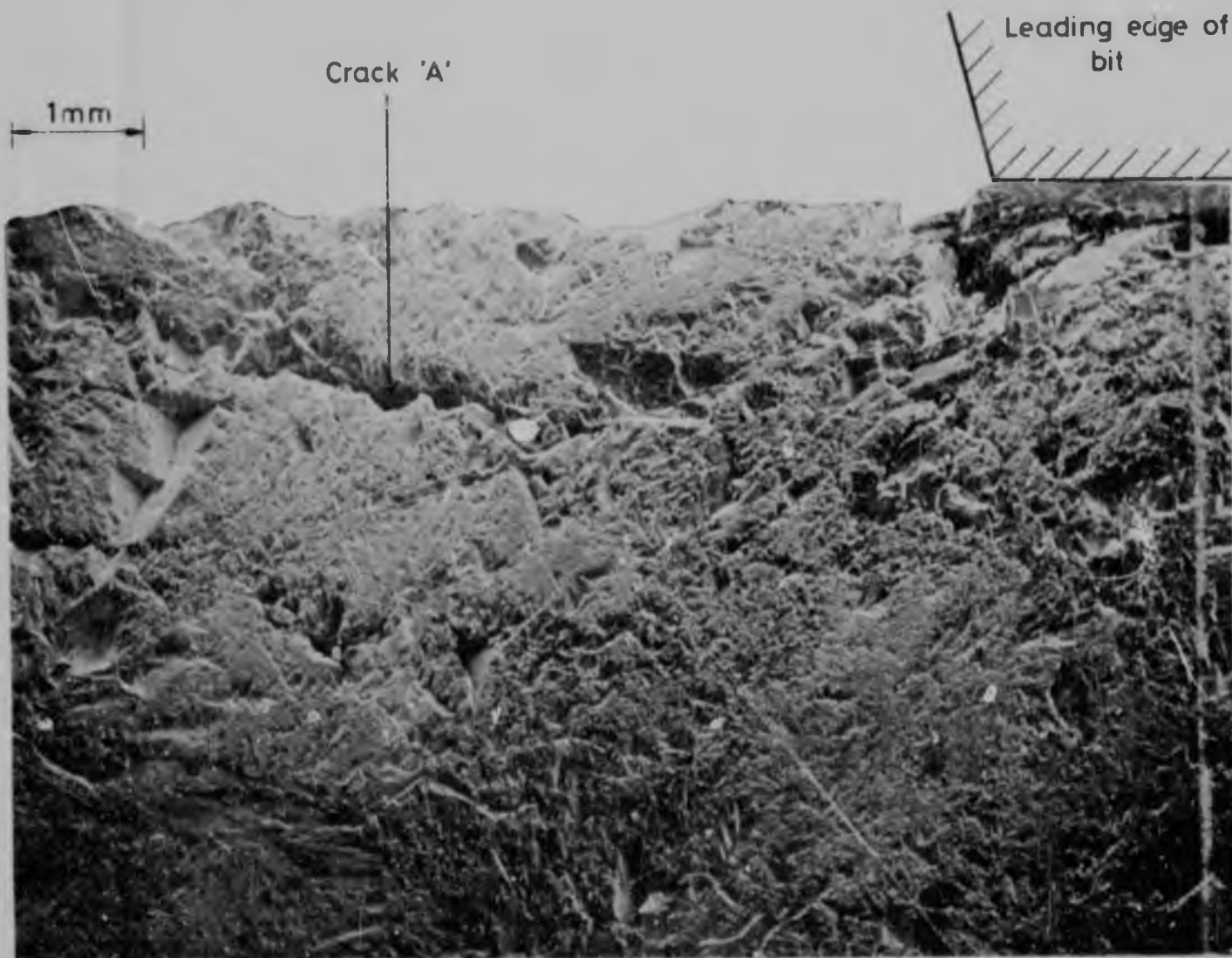
FIGURE 102 : Photo-micrograph of section through second norite specimen.
