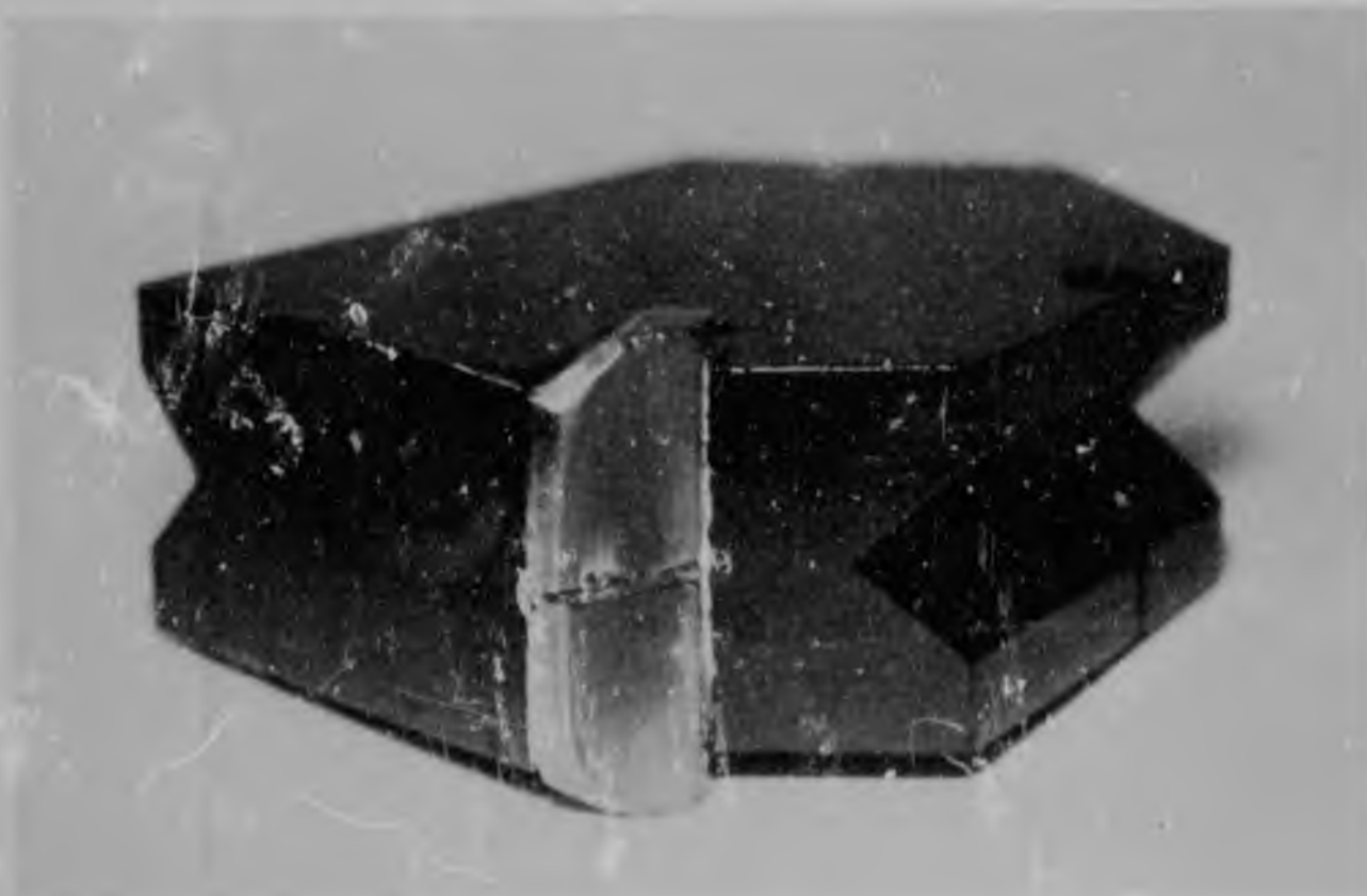
FIGURE 41. Detachable 35 mm rockcutter bit with a 2 mm wearflat width.
