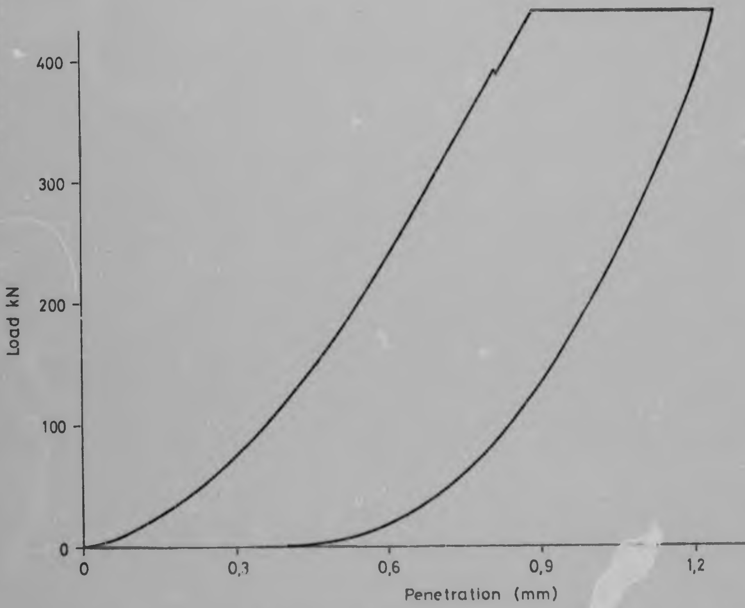
FIGURE 98: Indentation load plotted against bit penetration for first norite specimen.
