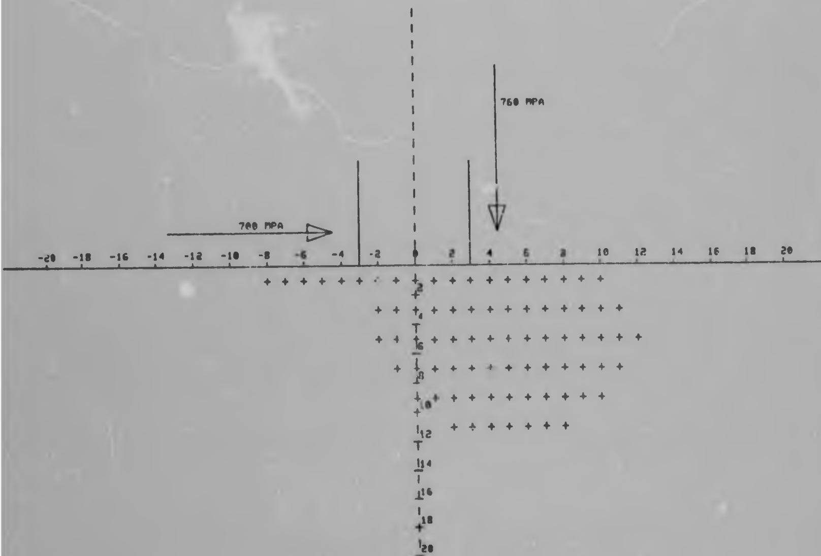
FIGURE 129 : Zone of excess stress when both a normal pressure 760 MPa and a shear pressure 700 MPa are applied to the surface of the body.
