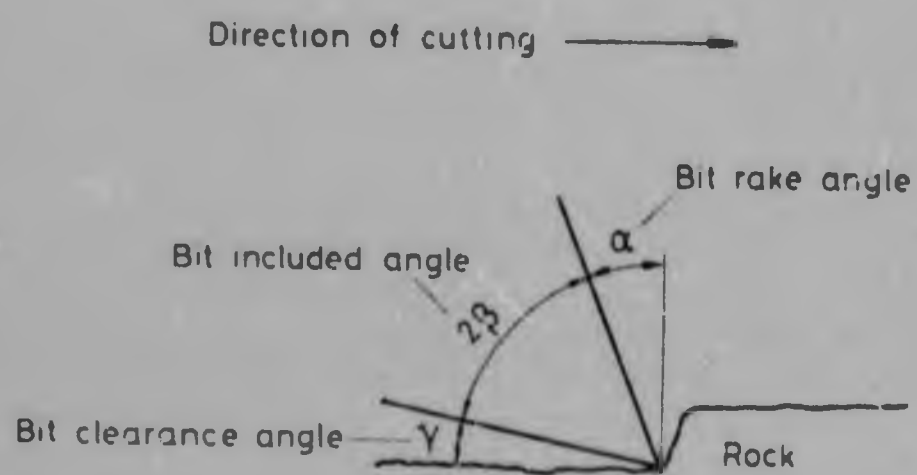
FIGURE 3 : Diagrammatic representation of a wedge shaped drag bit.
