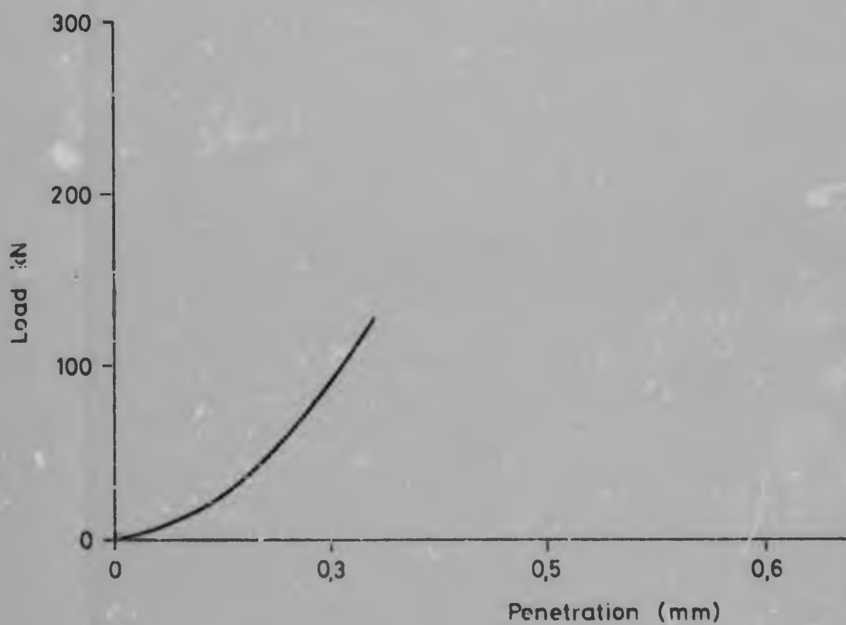
FIGURE 101 : Indentation load plotted against bit penetration for second quartzite specimen.
