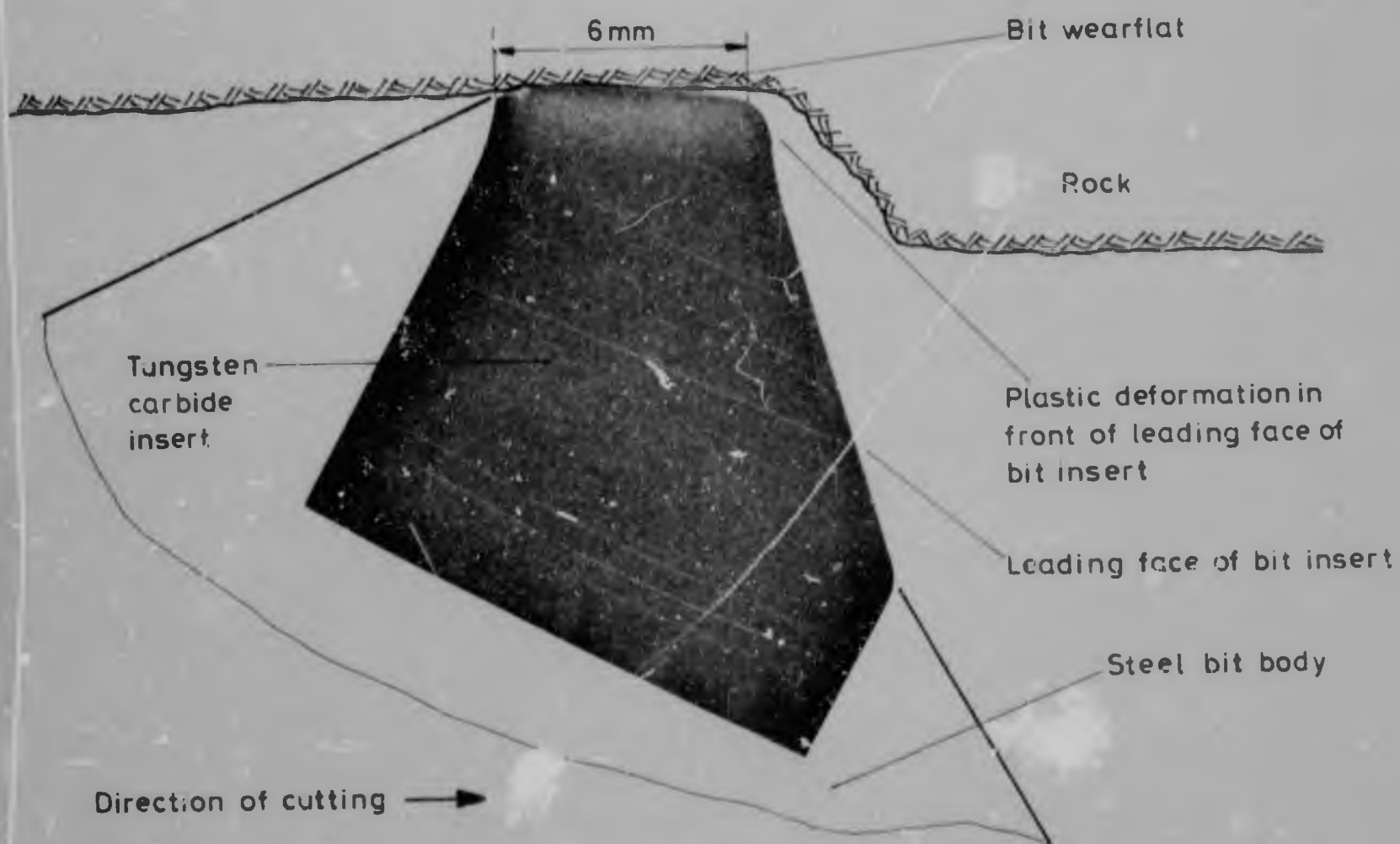
FIGURE 12 : Magnified section of a tungsten carbide bit insert, showing plastic deformation of the insert ahead of the leading face.
