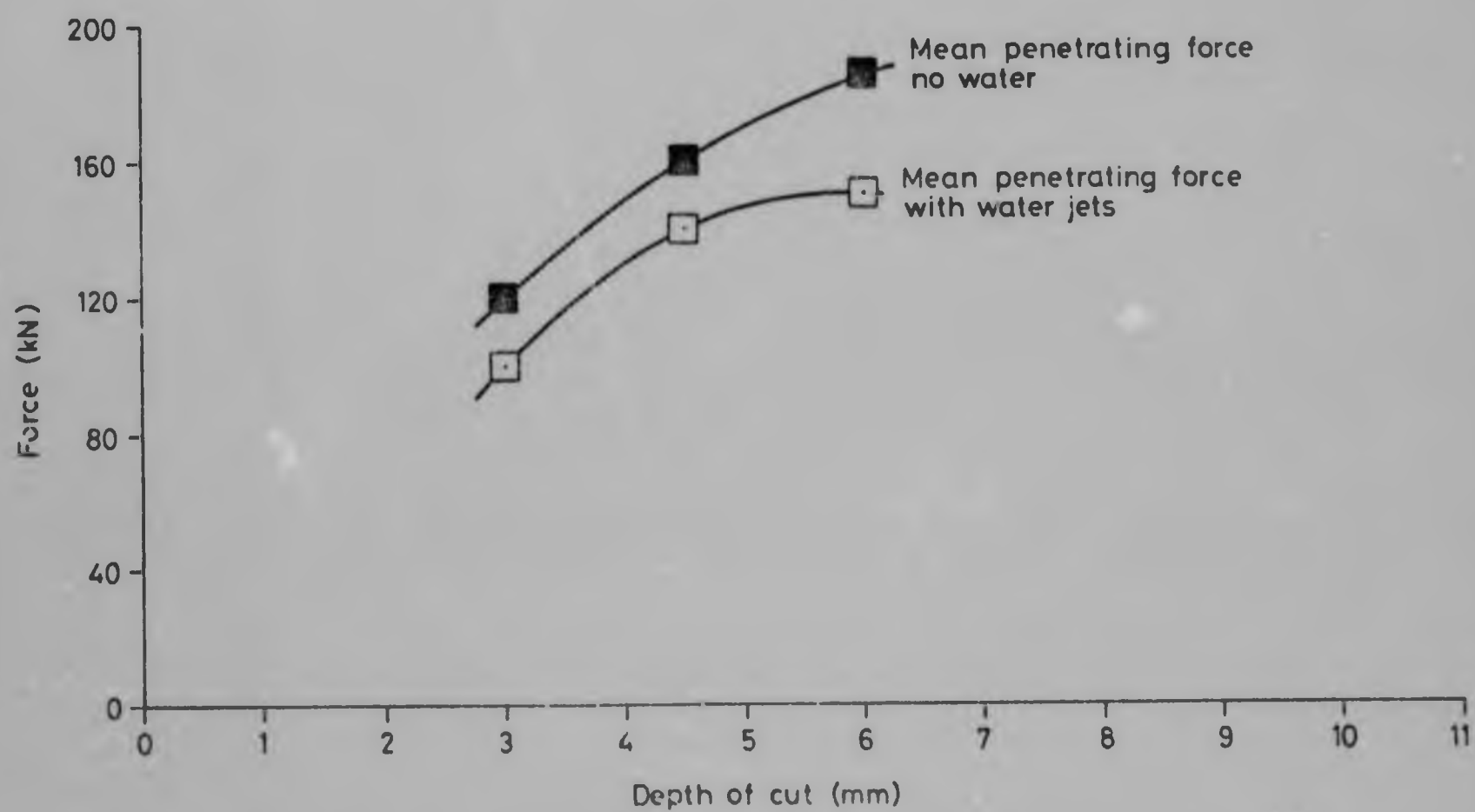
FIGURE 59 : Mean bit penetrating force plotted against depth of cut, with a 'flat-fan' water jet and with no water jets.
