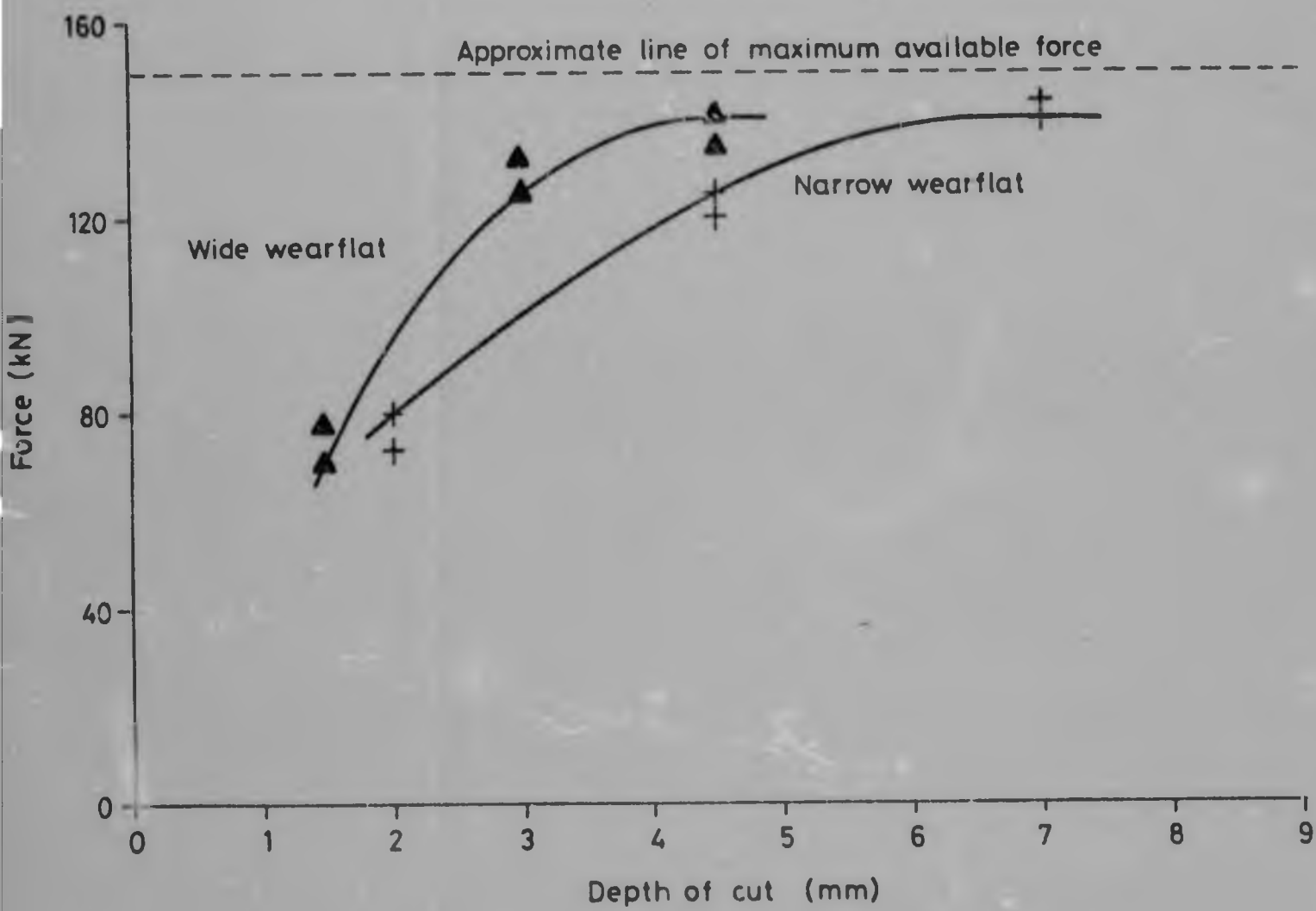
FIGURE 42 : Mean peak bit cutting force using a standard wearflat and a narrow wearflat bit.
