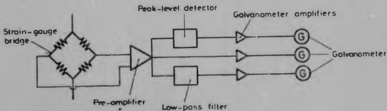
Penetration force instrumentation diagram.
