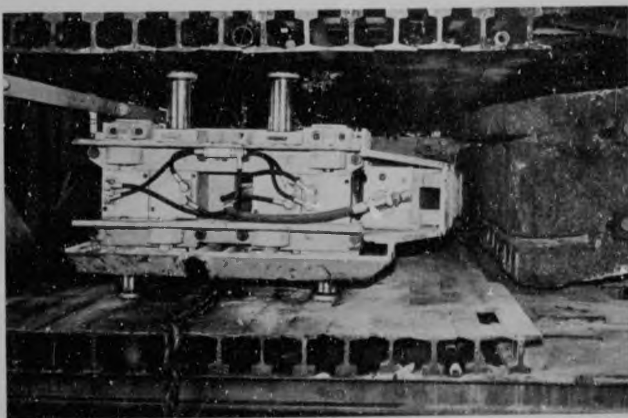
FIGURE 18. Rockcutting machine in test frame, side view.
