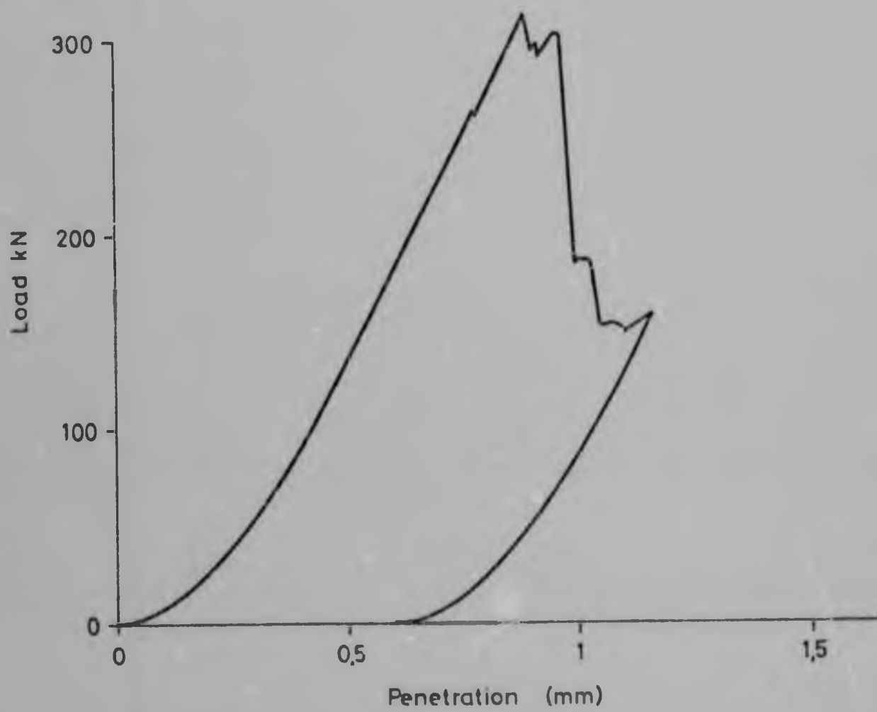
FIGURE 92 : Indentation force required to form rock chip in quartzite, plotted against penetration of the bit.
