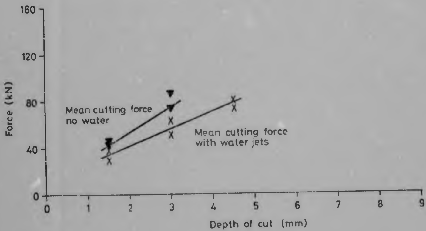
FIGURE 79 : Mean bit cutting force plotted against depth of cut, with water jets directed 10 mm ahead of the bit.
