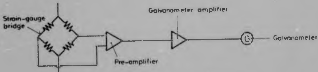
Vertical force instrumentation diagram.
