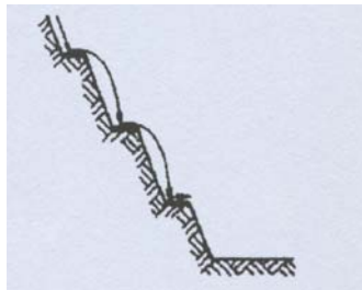
Figure 1.4. Catch benches (Spang, 1987).
