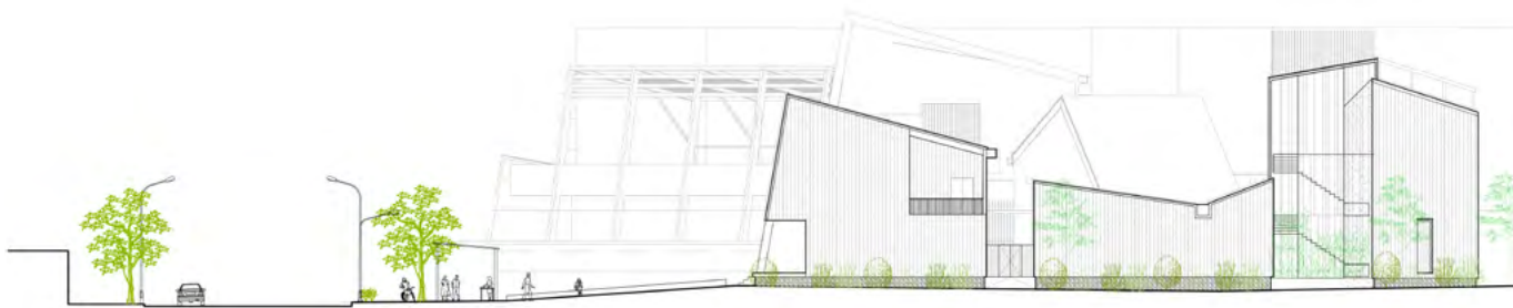
EAST ELEVATION (PINE AVENUE) SCALE 1:200
