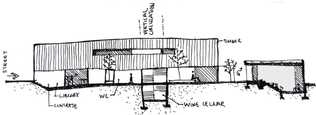
Fig 40- Section Elevation A-A (Forlee, 2020)
