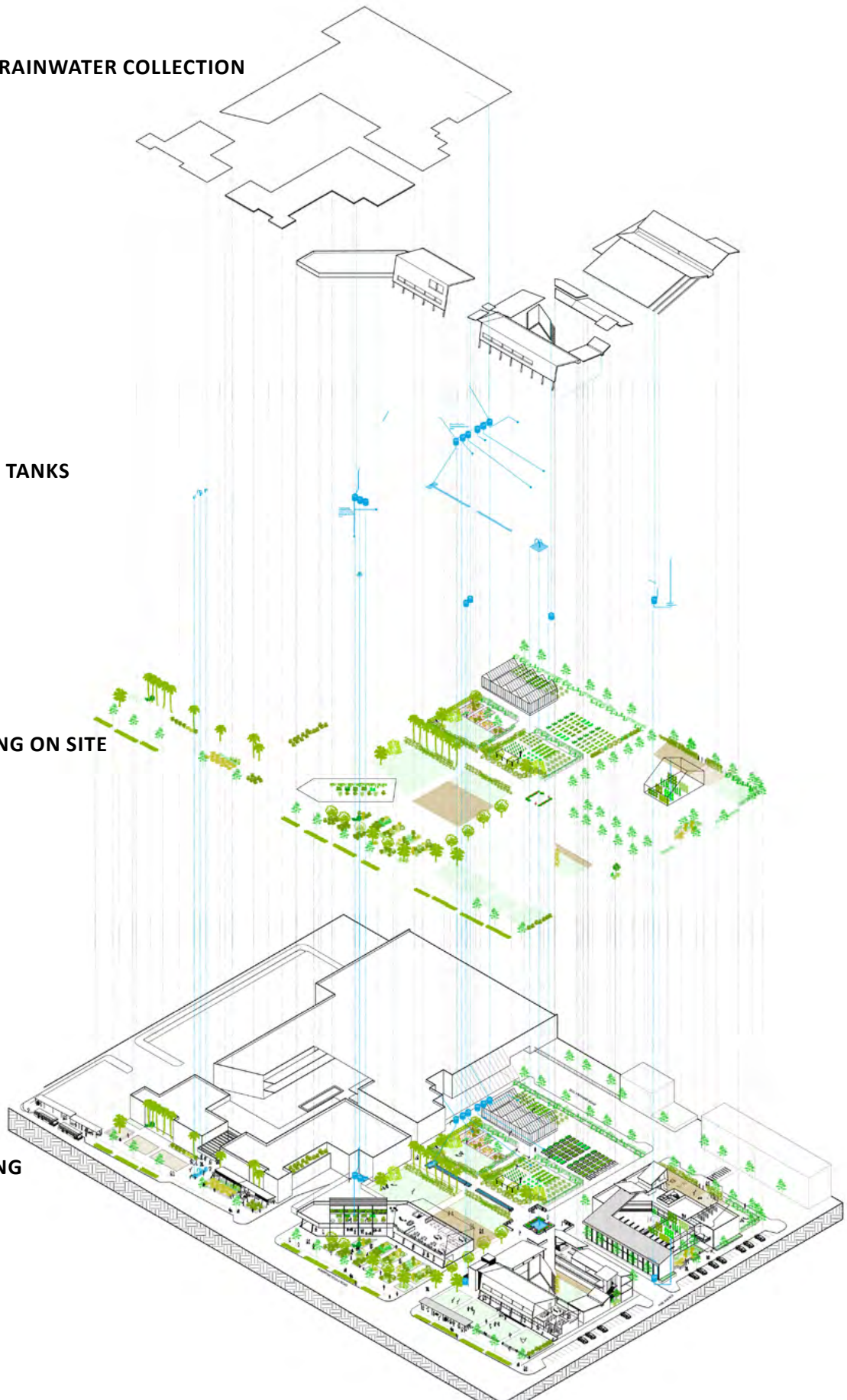
Fig 133 - Exploded axonometric showing landscape systems. Scale 1:2000 on A1 (Forlee, 2020)
