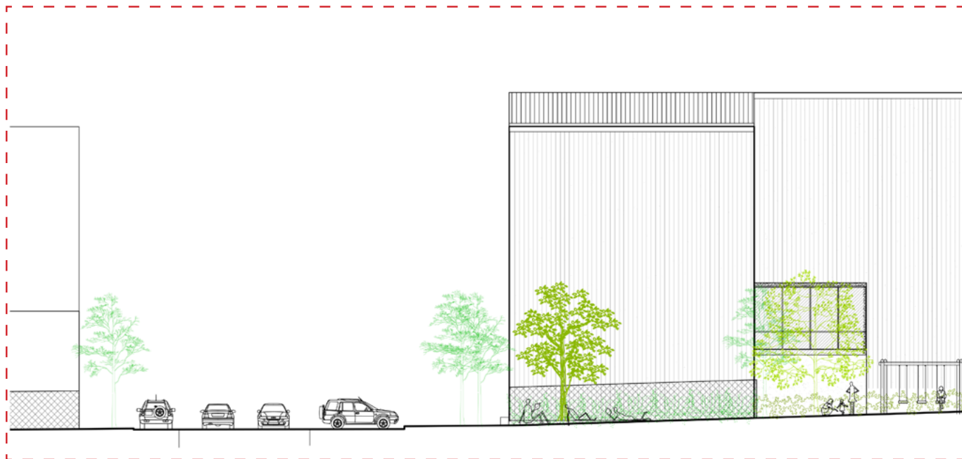
NORTH ELEVATION OF AGRICULTURAL RESEARCH CENTRE SHOWING ACTIVITIES IN THE PARK SCALE 1:100
