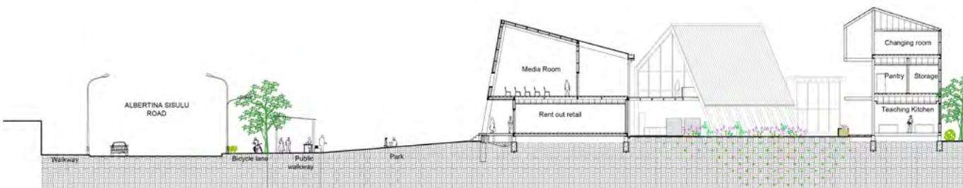
SECTION B-B SCALE 1:200
