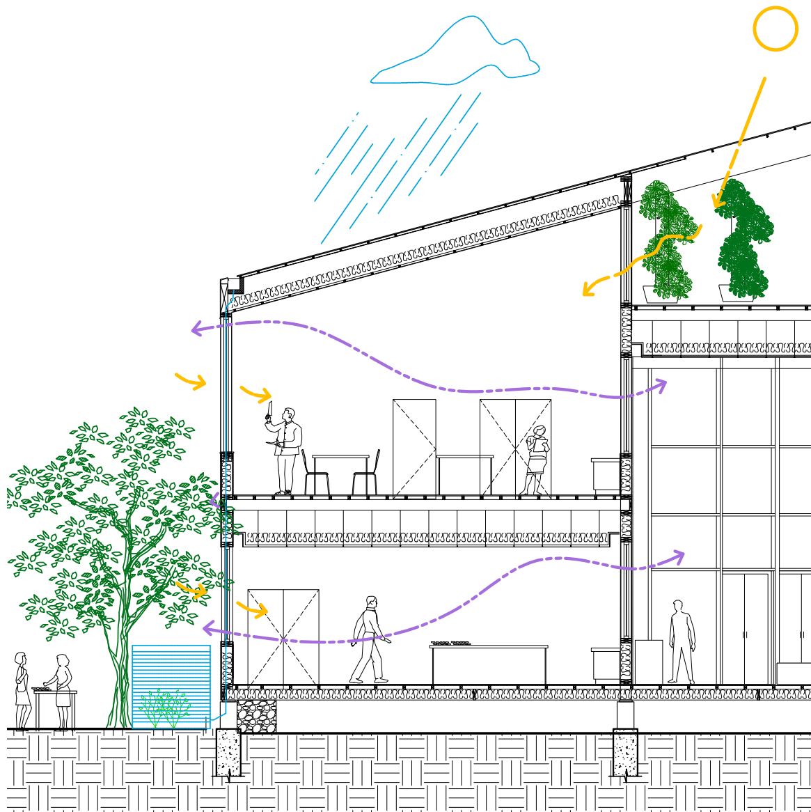
Fig 132 - Section through Agro-processing station (Forlee, 2020)
