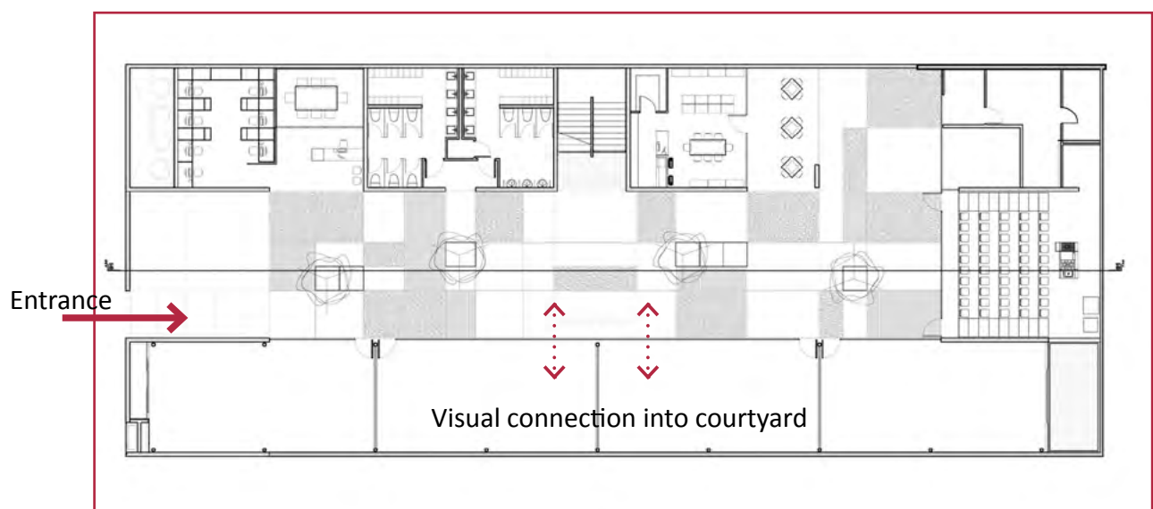
Fig 41 - Ground floor plan (Gracia Studio, 2011)
