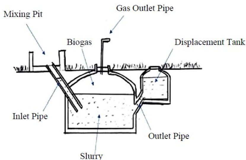
Fig 95 - Fixed Dome Biogas Digester (Ainomugisha, 2017)
