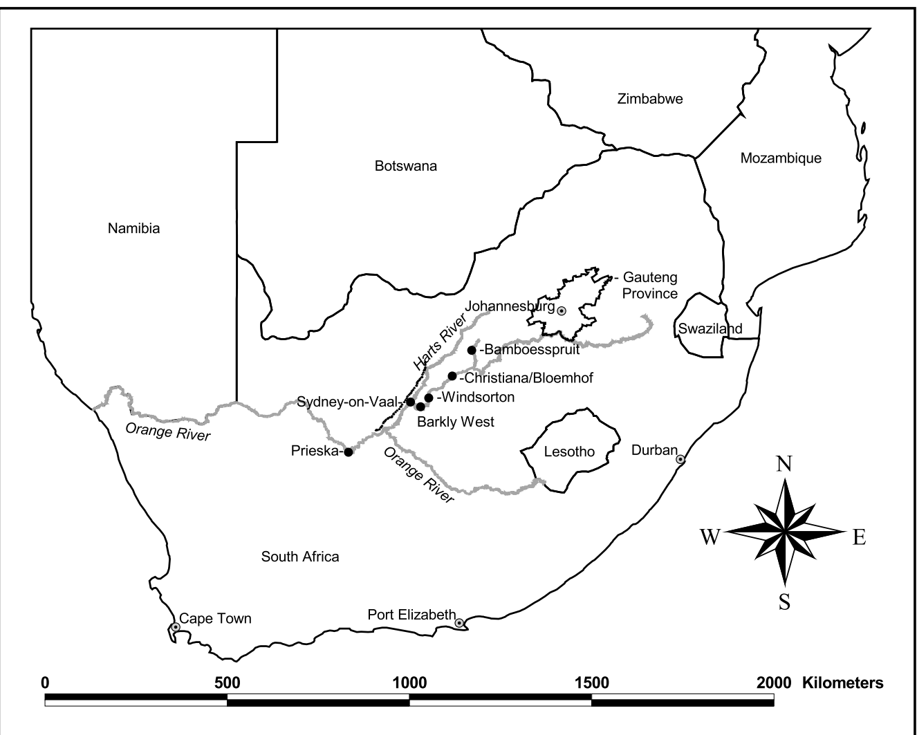
Figure 4.1: Map of South Africa and neighbouring countries showing locations of sites referred to in the text. Cosmogenic nuclide burial dating samples were collected from the Bamboesspruit; Christiana/Bloemhof; Windsorton; Barkly West; Sydney-on-Vaal; and along the middle Orange River between the Vaal/Orange confluence and Prieska.
