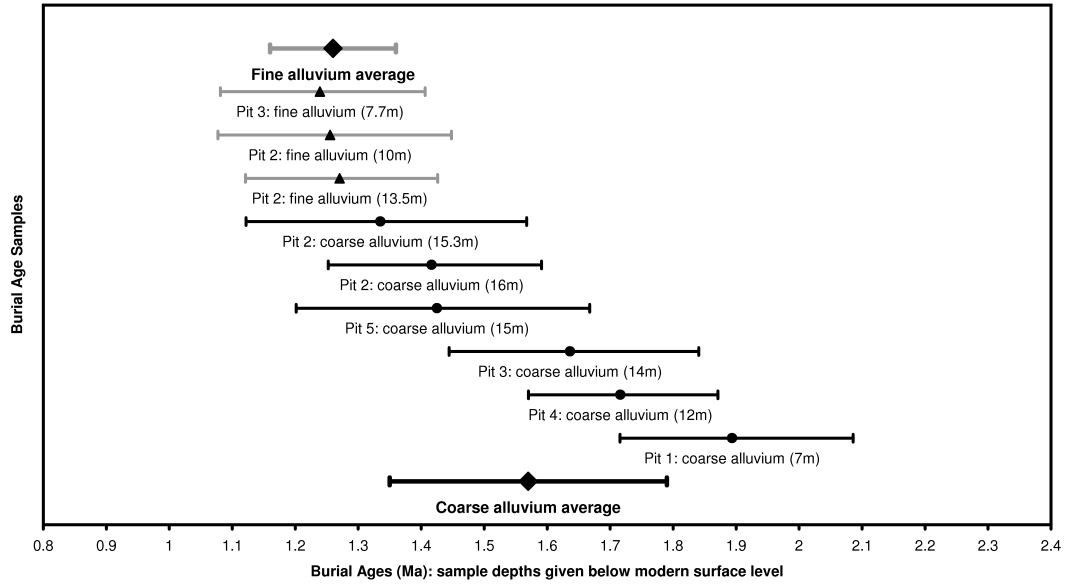
(a) Burial ages showing errors for the Rietputs Formation. Ages are in stratigraphic order for individual pits. The average burial age for both the fine and coarse alluvium is shown.
