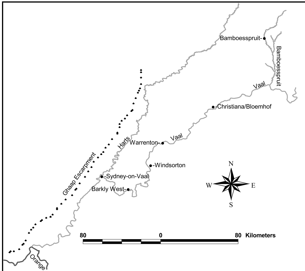
Figure 5.2: Plan view of the study area within the Vaal River catchment. Two prominent knick-zones occur between Warrenton and Windsorton, and between Barkly West and Sydney-on-Vaal. Upstream of these knick-zones, and the Vaal/Orange River confluence, the Vaal River can be seen to meander more extensively.
