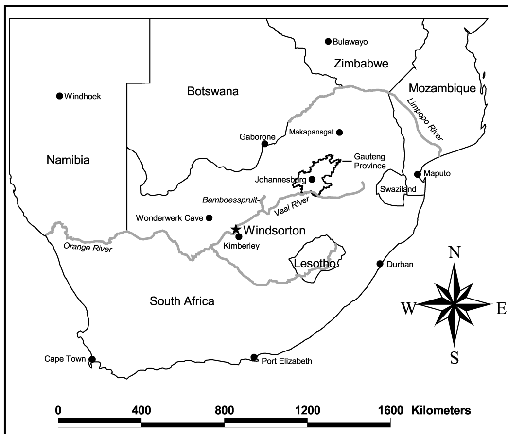
Figure 6.1: Map of South Africa and neighbouring countries showing locations of sites referred to in the text.
