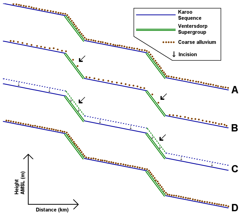
Figure 5.3: Schematic representations of the Vaal River long profile from the infall of the Bamboesspruit to the confluence with the Orange River showing how bedrock incision takes place within the lower catchment. Generalised outcroppings of the Ventersdorp Supergroup and the Karoo Sequence are shown. A: Bedrock along the river is protected by a covering of coarse alluvium which prevents incision. B: A shift to climatic conditions characterised by an increase in the number and amplitude of formative discharges begins to remove the gravel armouring along the steeper pre-Karoo knick-zone reaches, particularly as these provide higher hydraulic power conditions. C: The now exposed, easily erodible Karoo rocks lining the valley bottom along the knick-zone reaches are incised as a result of repeated impacts and abrasion by saltating hard clasts on the soft bedrock. Incision along the knick-zone reaches results in knickpoint migration upstream, resulting in incision of alluvium, as well as bedrock in these flatter regions. D: Either a reduction in formative discharge strength, or an increase in coarse sediment supply, or a combination of both, causes the aggradation again of protective gravels which stops bedrock incision.
