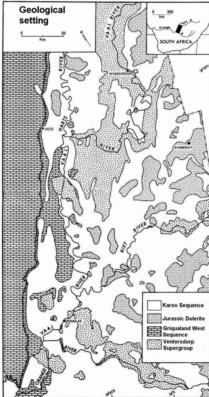
Figure 2.2: Generalised geology of the lower Vaal River catchment taken from Helgren (1979, 70). Helgren's map is unmodified from its original form and still provides an accurate generalised geological overview. Only the geological names have been updated. The pre-Karoo surface is prominently exposed where the Vaal River flows over the Ventersdorp Supergroup.
