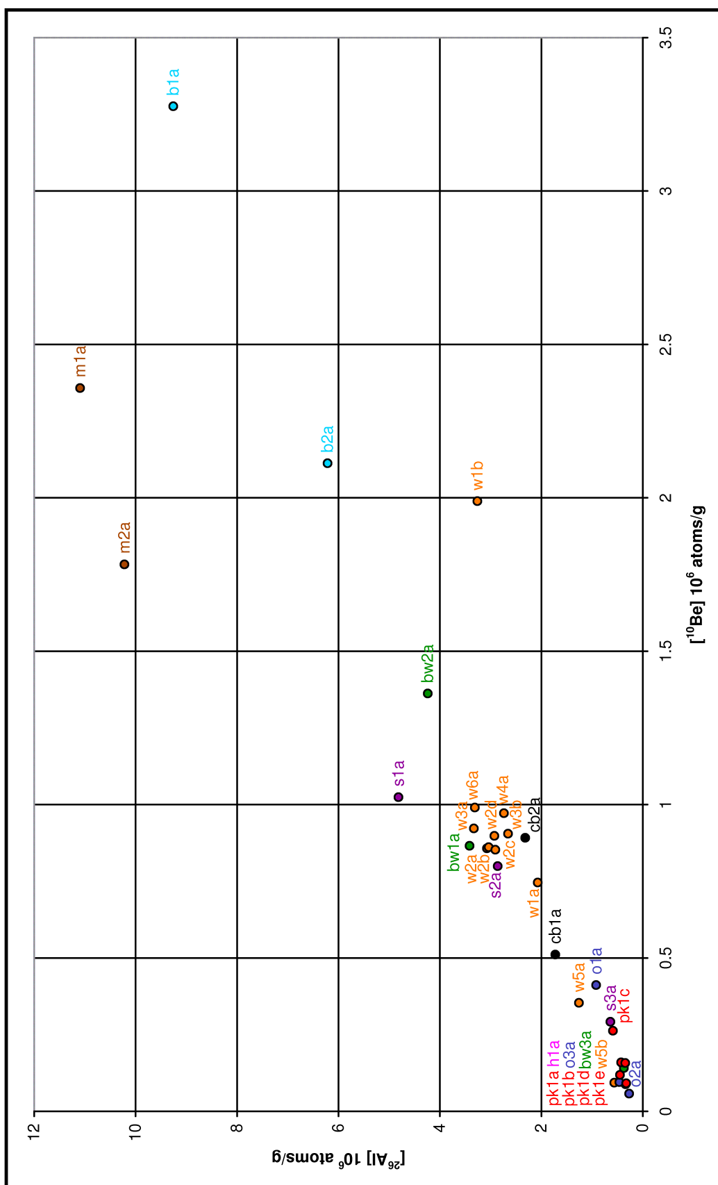
Figure 4.6: Scatter plot of the measured concentrations of ^{26}\text{Al} and ^{10}\text{Be} for each burial dating sample.
