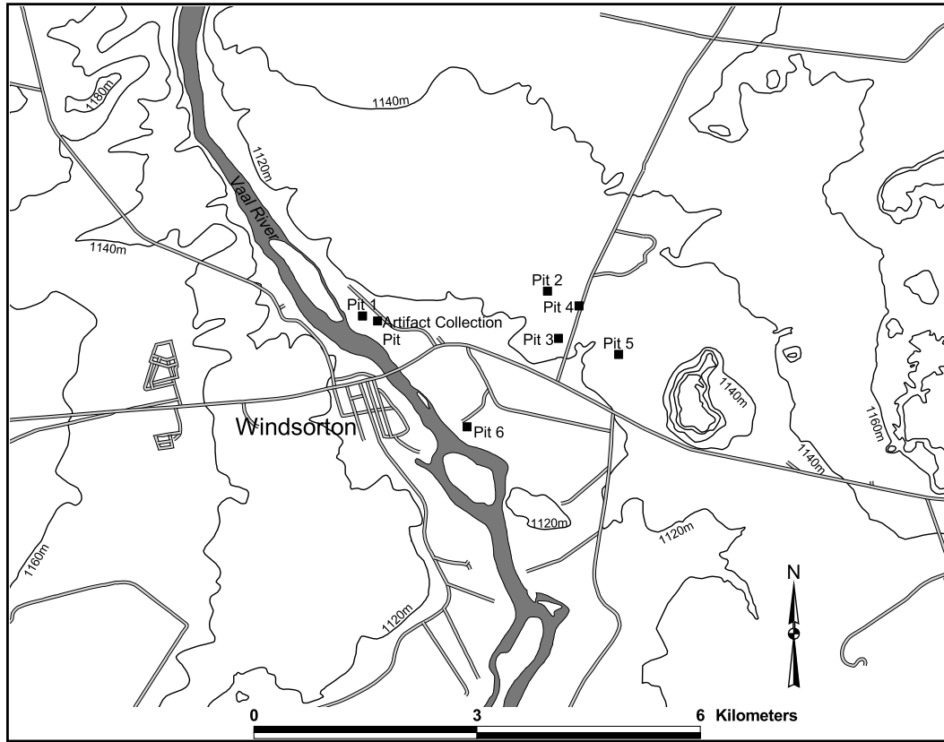
Figure 4.4: Type-site of the Rietputs Formation near to the town of Windsorton, Northern Cape Province, South Africa. The Rietputs Formation occurs along both sides of the river but is more extensive on the east. Riverton Formation deposits are situated along the immediate river banks. The ‘older gravel’ deposits are found to the west of the river at increasing altitudes, with a few remnants of the Wedburg terrace deposits sitting on bedrock pedestals above the Rietputs and Riverton Formations on the east bank. Mining pits from which cosmogenic nuclide burial dating samples were obtained are numbered, as well as the pit from which stone artefacts were collected (discussed later).
